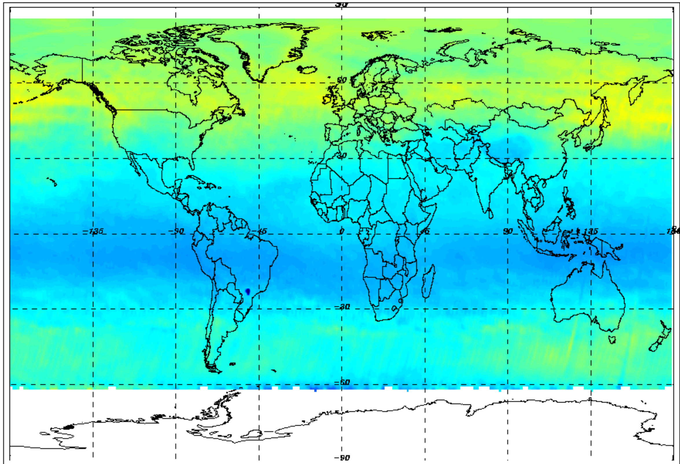
03 VCD (DU) monthly mean - June 2011
