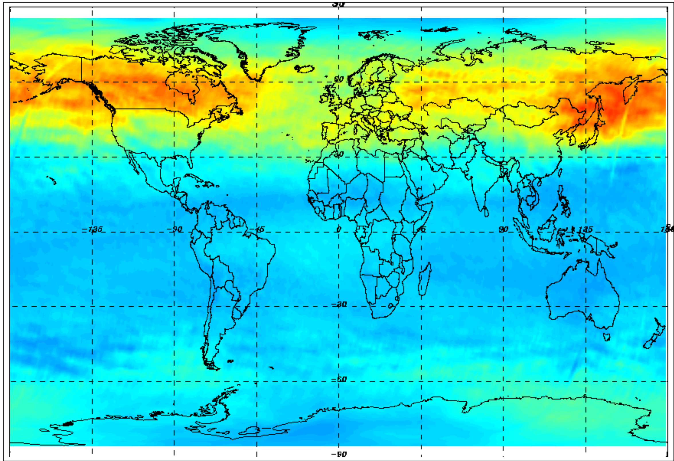
03 VCD (DU) monthly mean - March 2011
