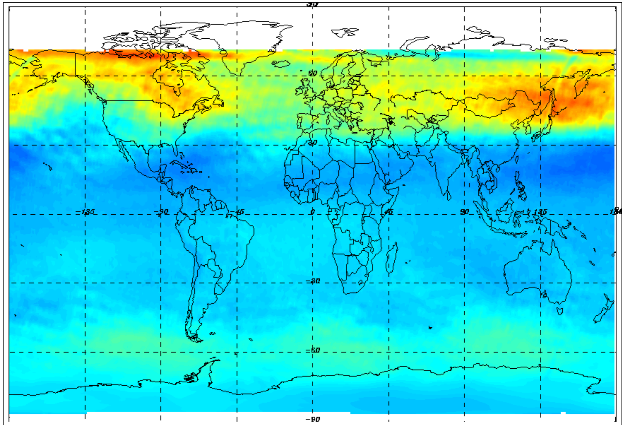
03 VCD (DU) monthly mean - January 2011
