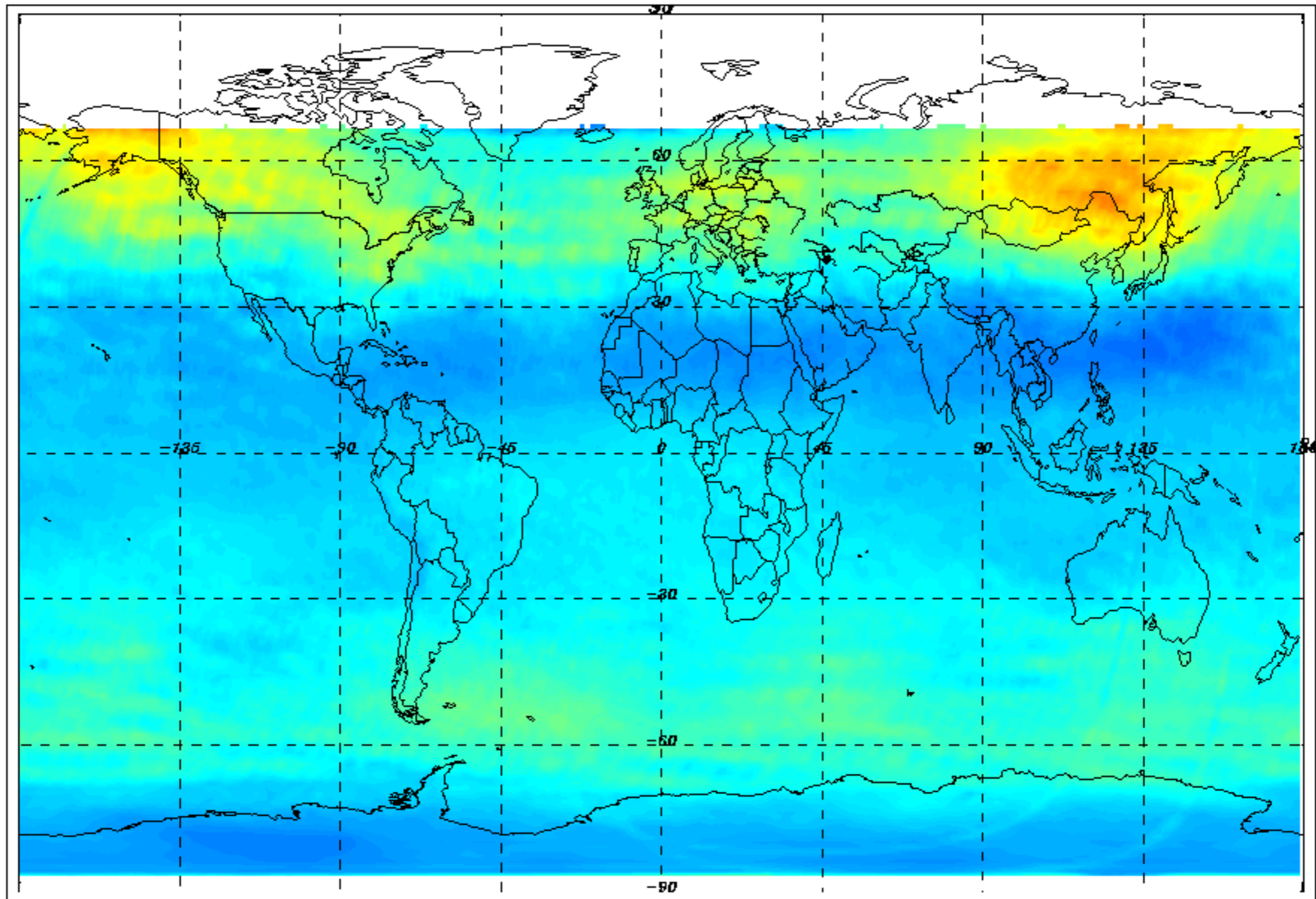
03 VCD (DU) monthly mean - December 2010
