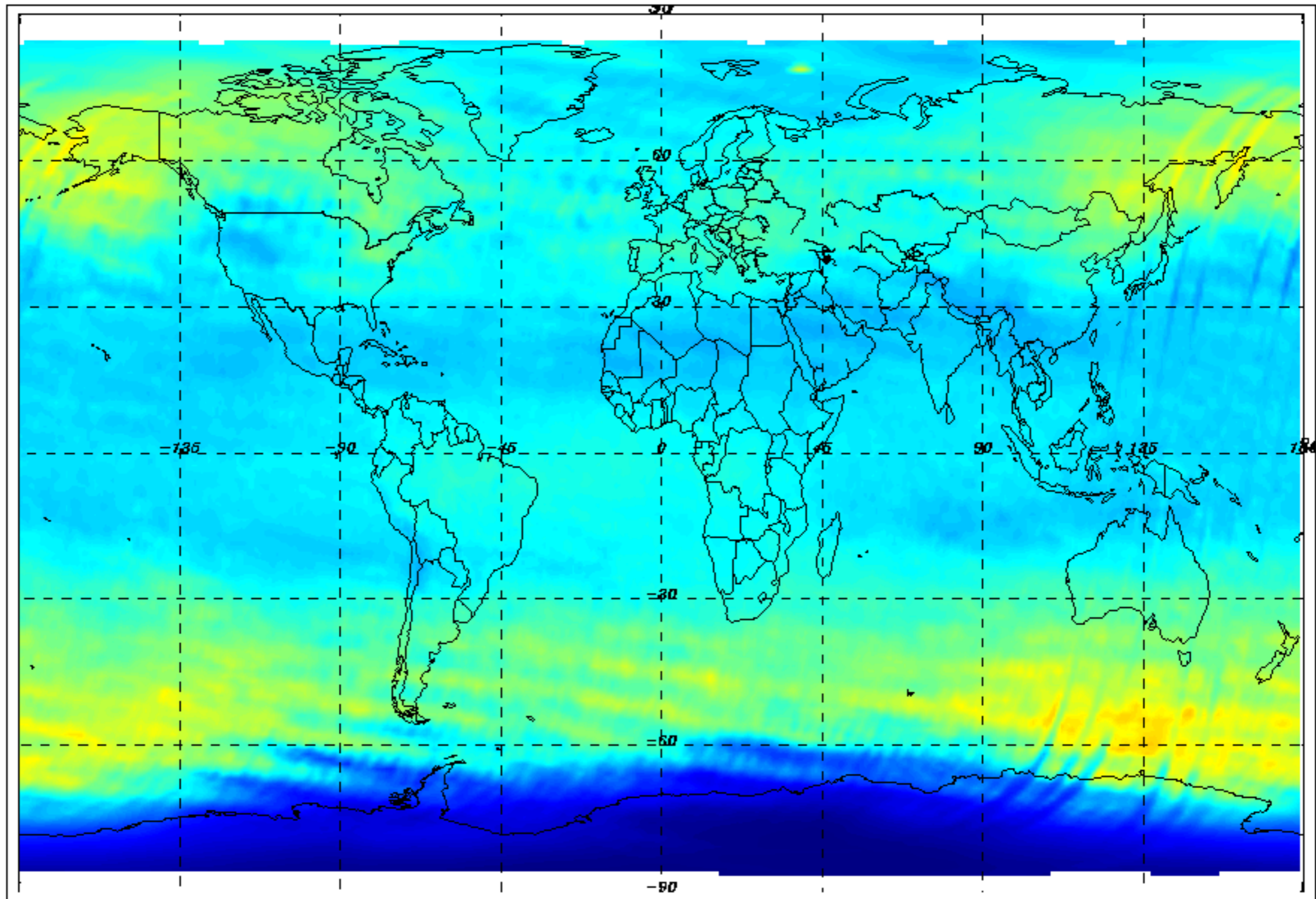
03 VCD (DU) monthly mean - October 2010
