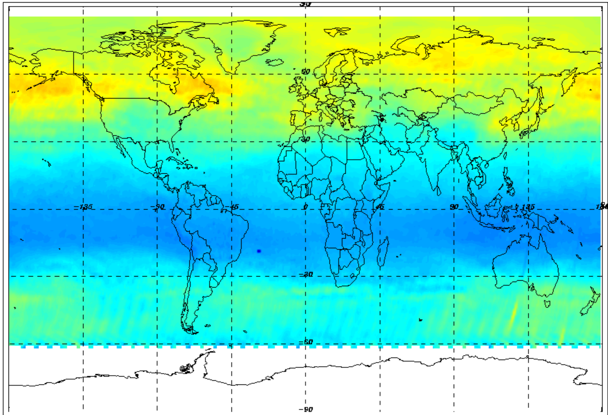
03 VCD (DU) monthly mean - June 2010
