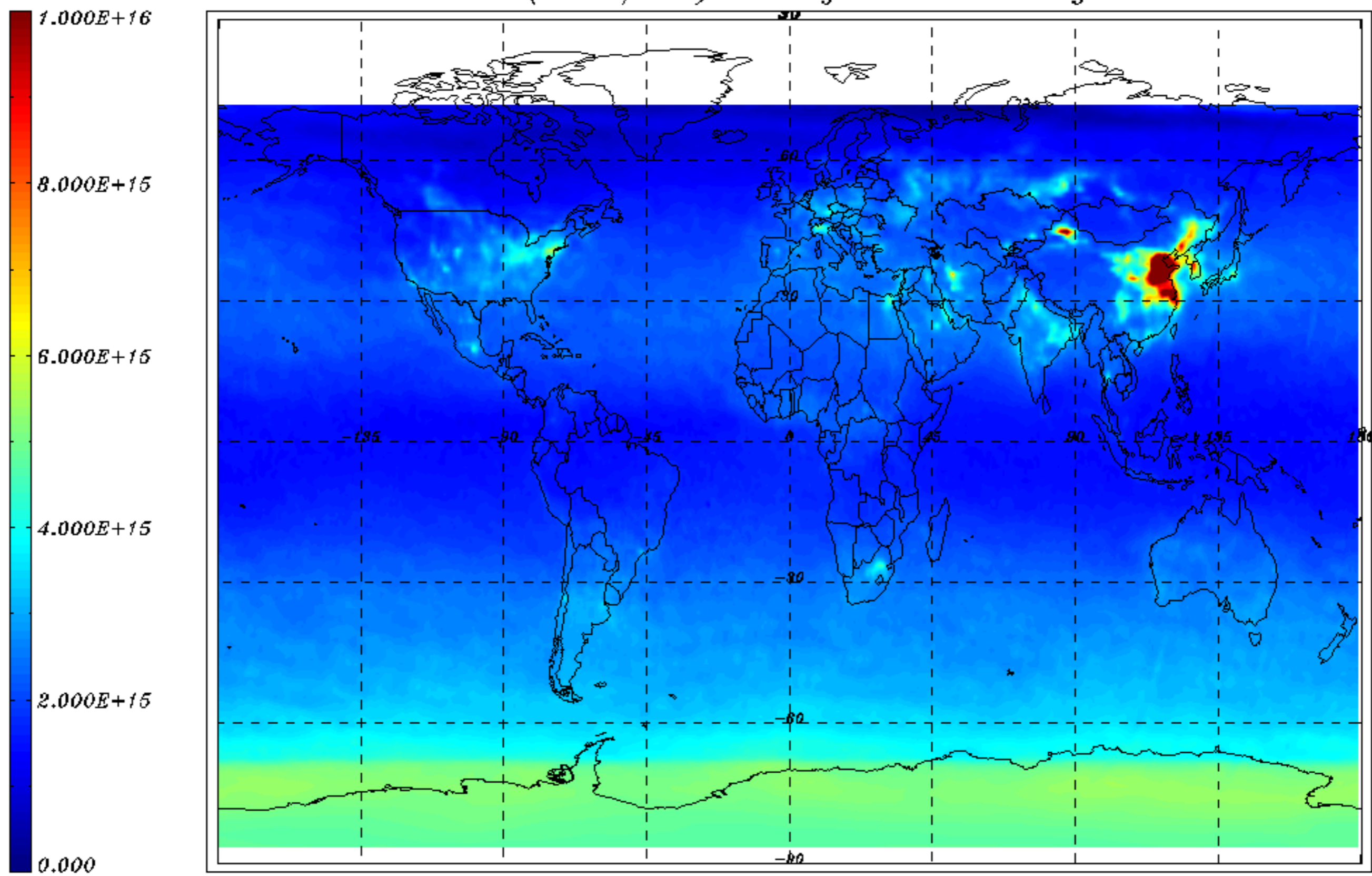
NO2 VCD (molec/cm2) monthly mean - January 2011
