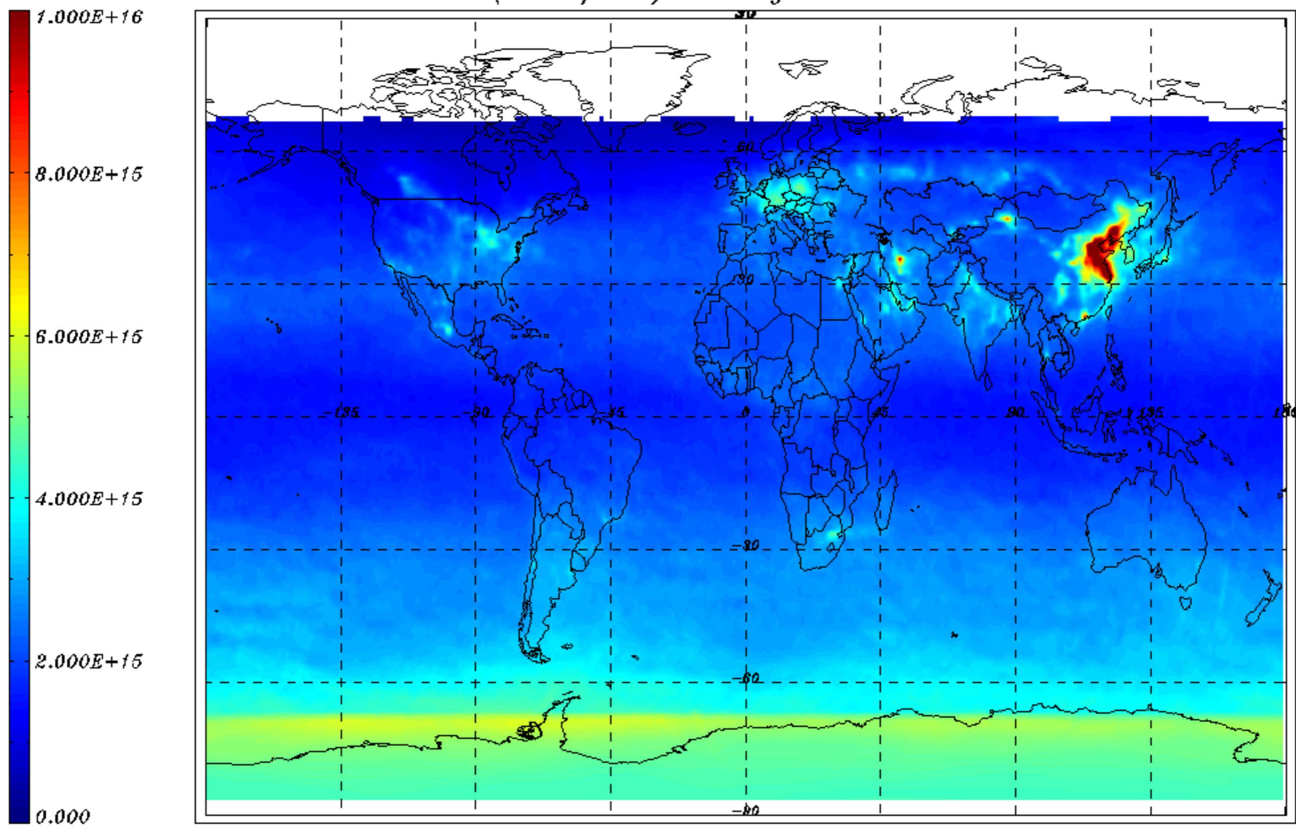
NO2 VCD (molec/cm2) monthly mean - December 2010
