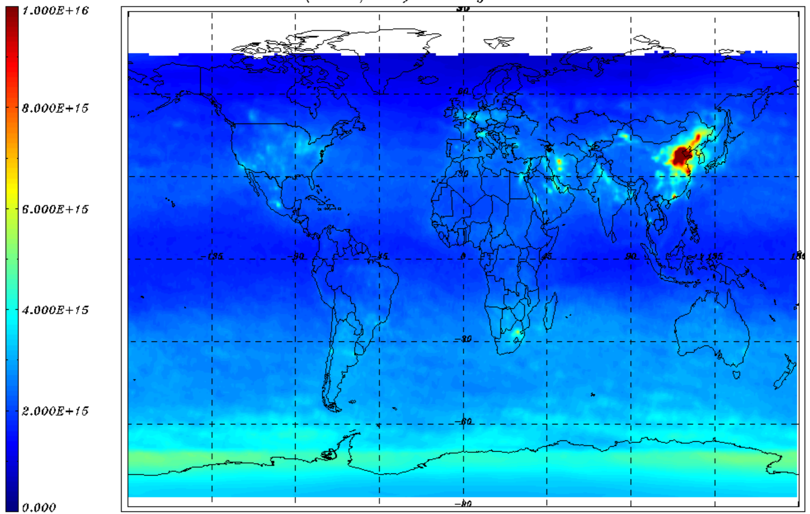
NO2 VCD (molec/cm2) monthly mean - November 2010
