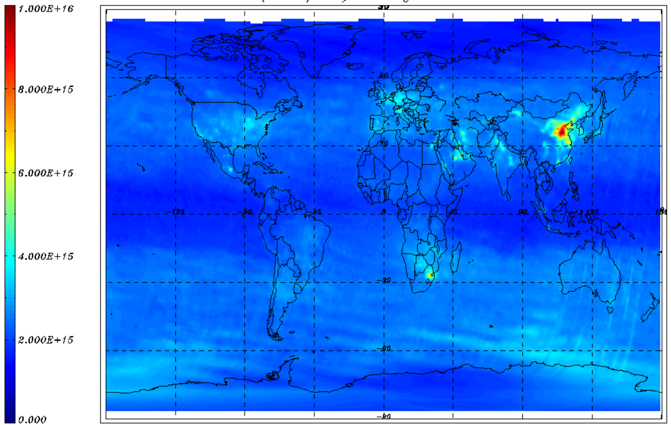
NO2 VCD (molec/cm2) monthly mean - October 2010
