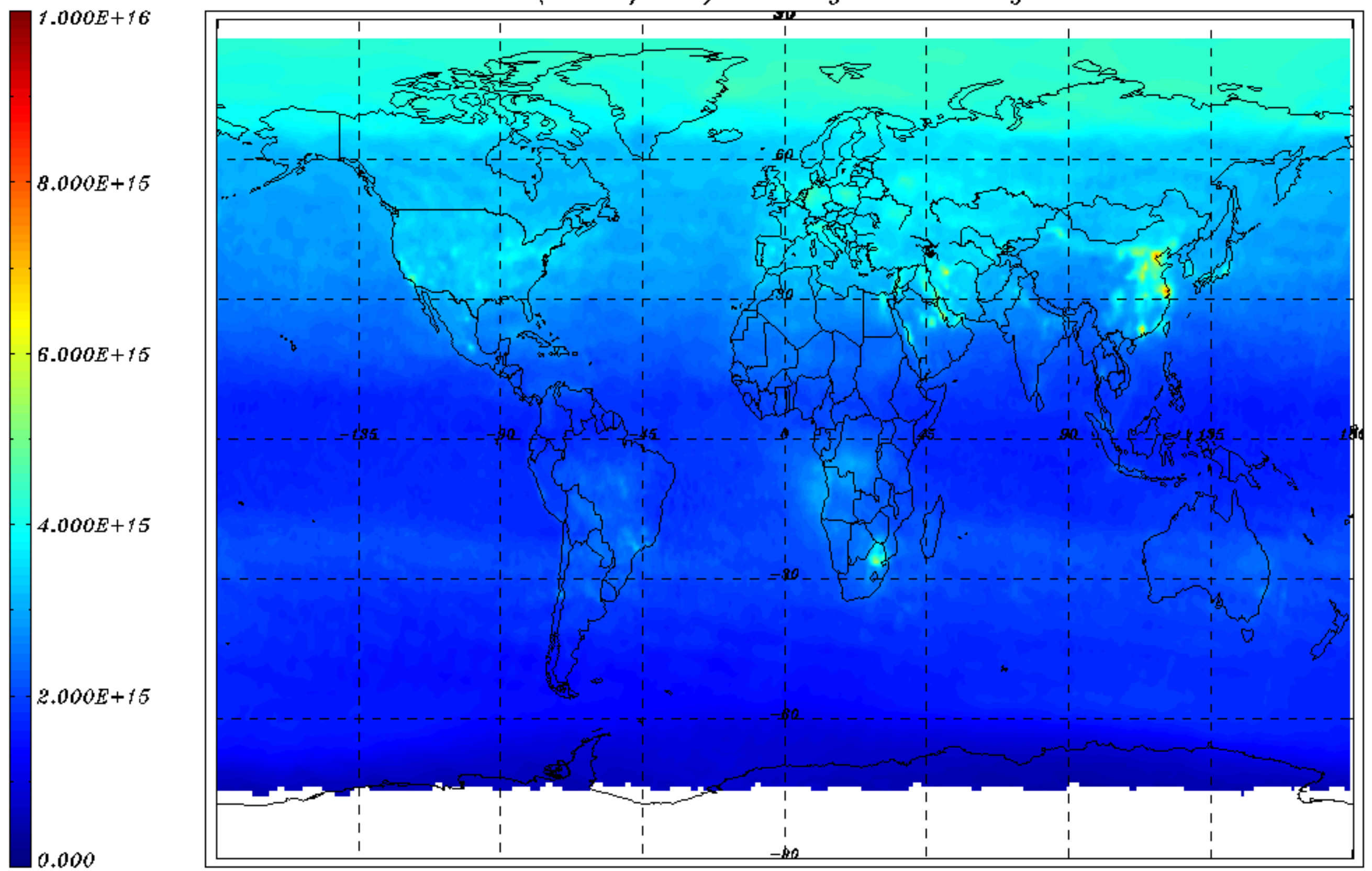
NO2 VCD (molec/cm2) monthly mean - August 2010
