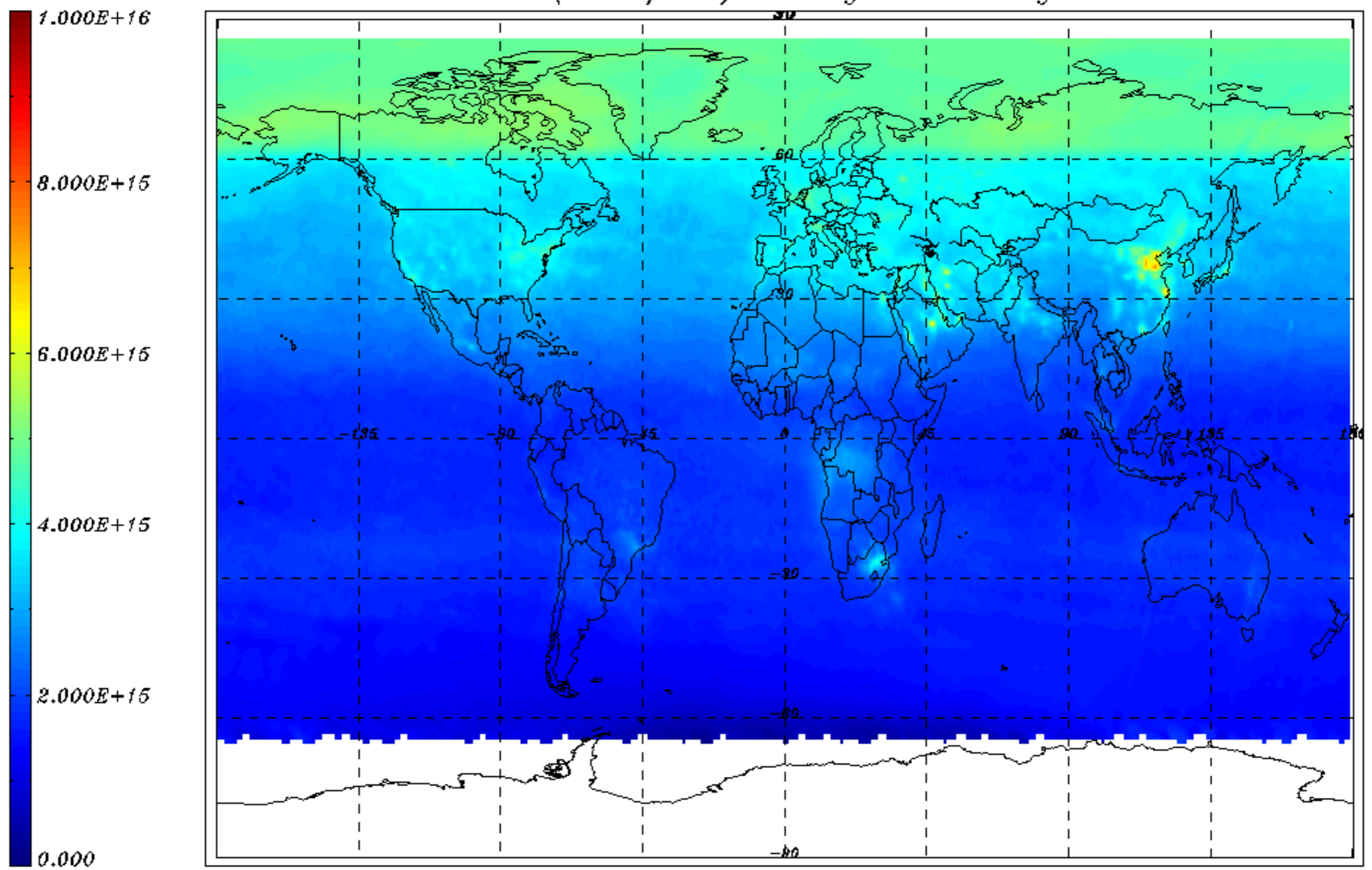
NO2 VCD (molec/cm2) monthly mean - July 2010
