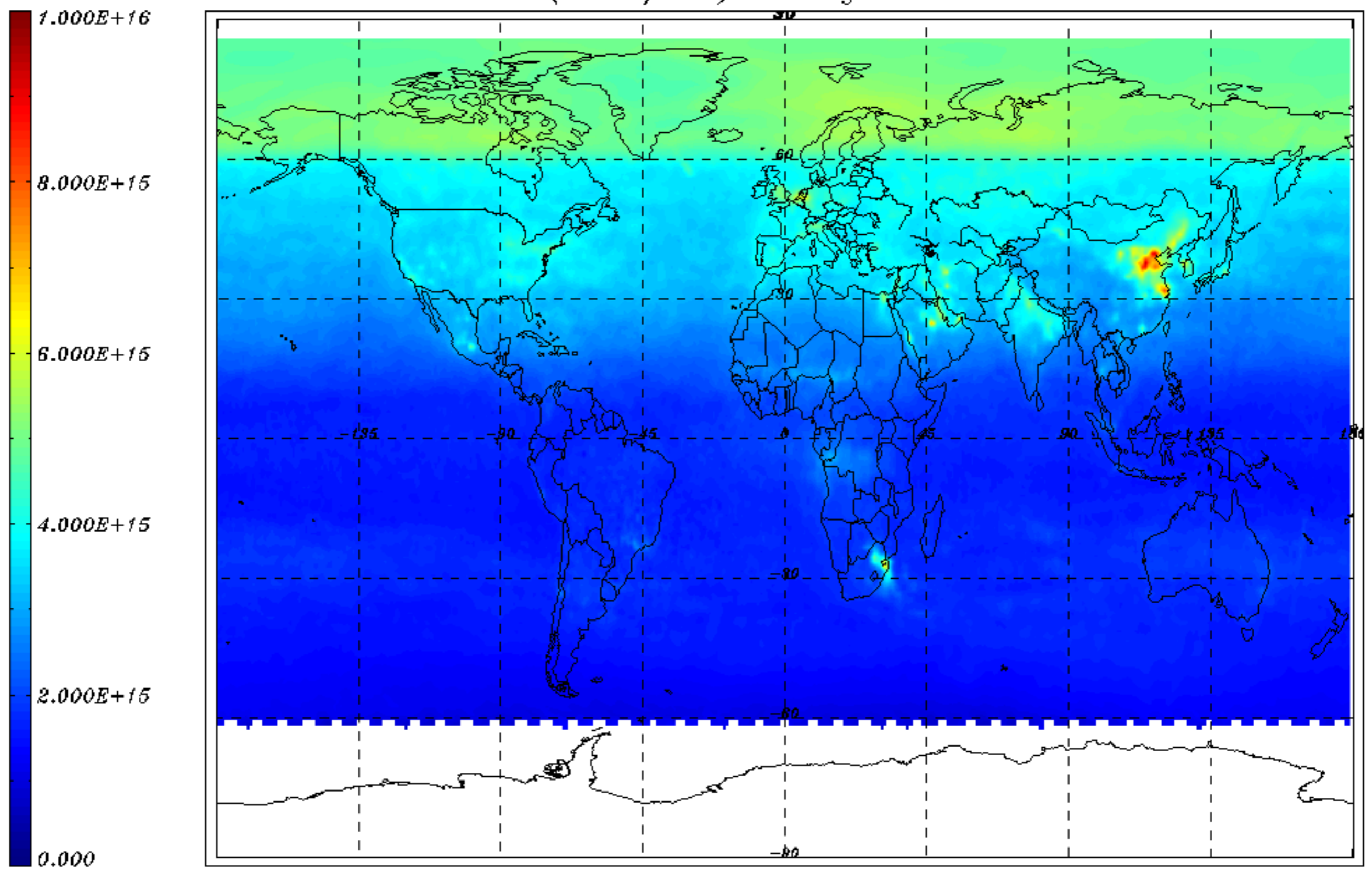
NO2 VCD (molec/cm2) monthly mean - June 2010
