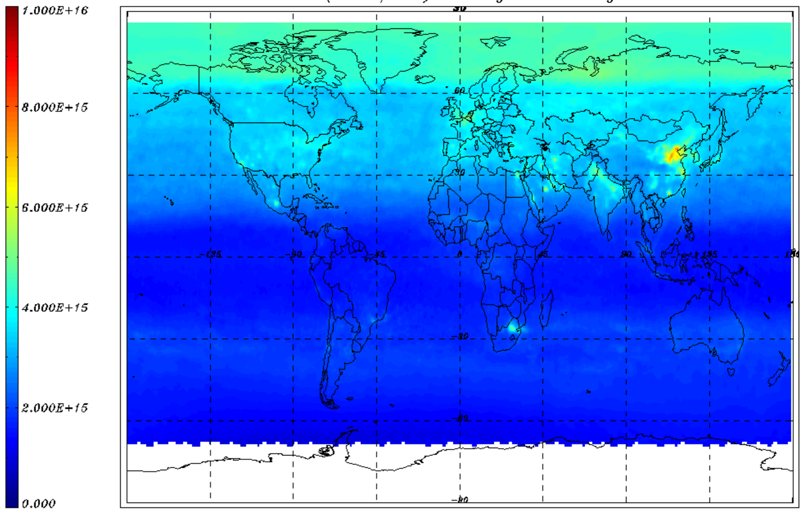
NO2 VCD (molec/cm2) monthly mean - May 2010
