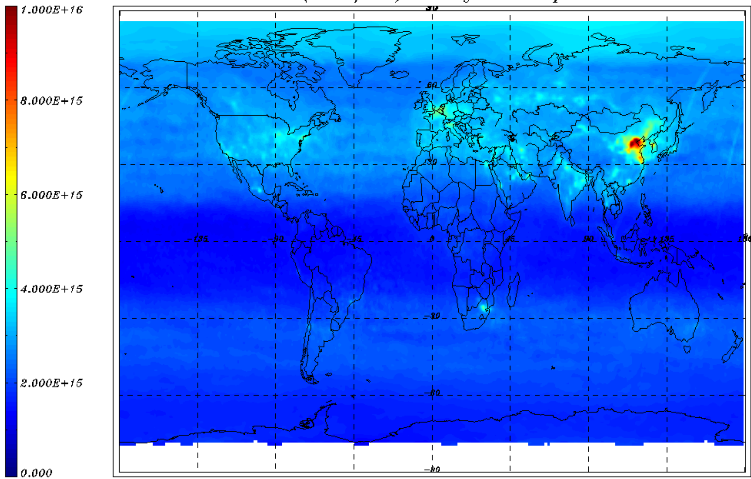
NO2 VCD (molec/cm2) monthly mean - April 2010
