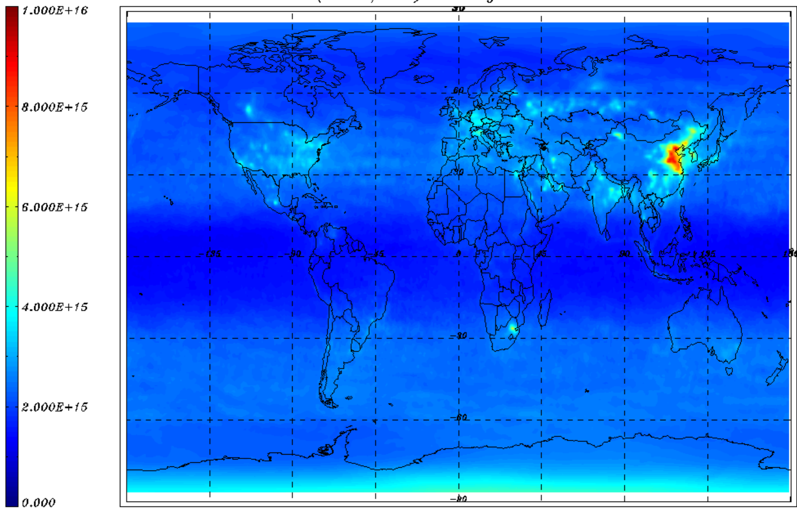
NO2 VCD (molec/cm2) monthly mean - March 2010
