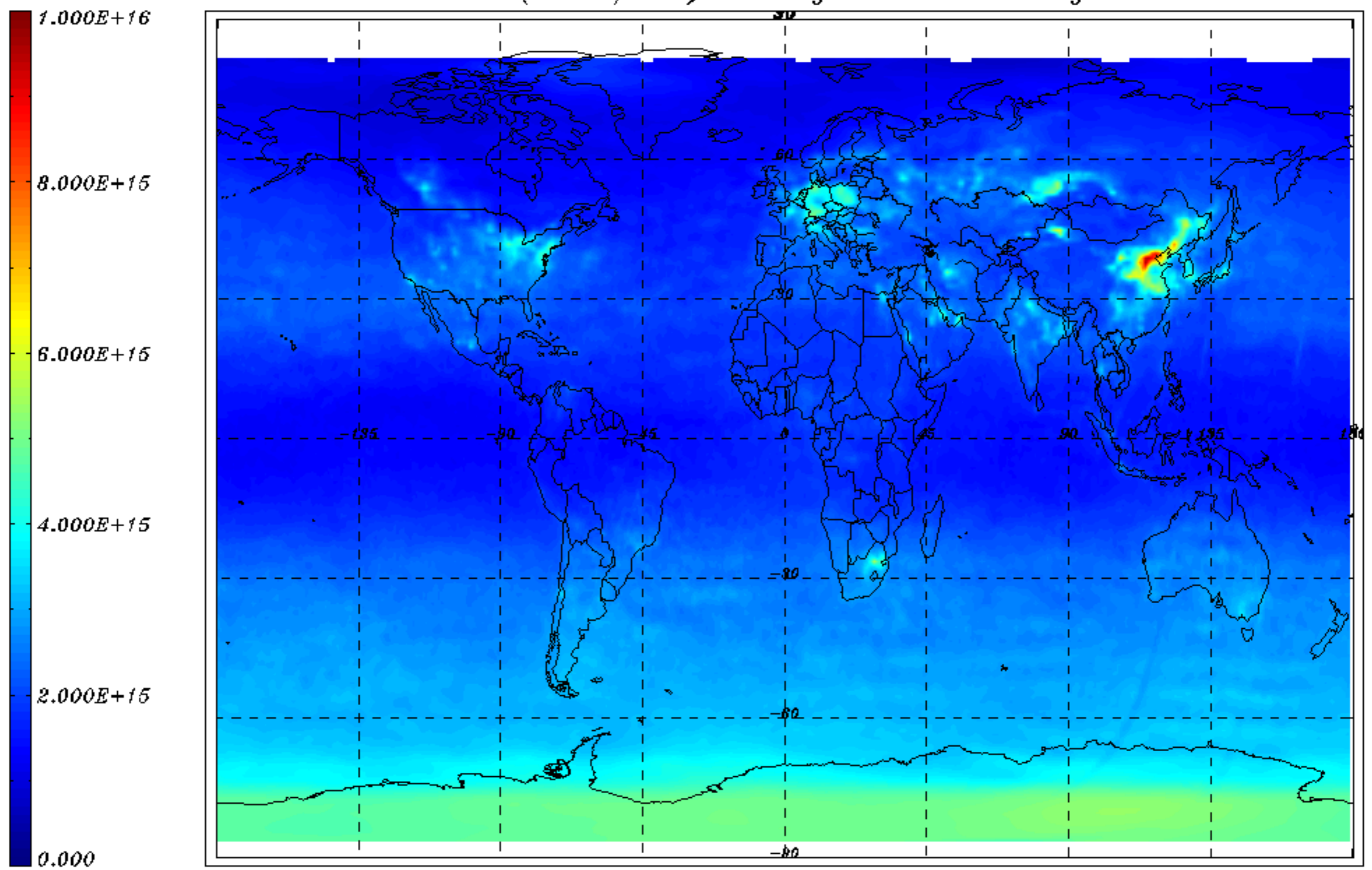
NO2 VCD (molec/cm2) monthly mean - February 2010
