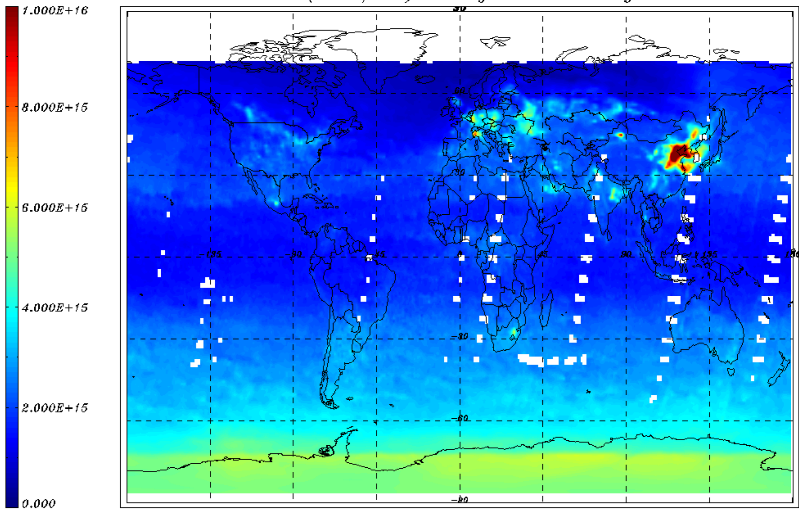
NO2 VCD (molec/cm2) monthly mean - January 2010
