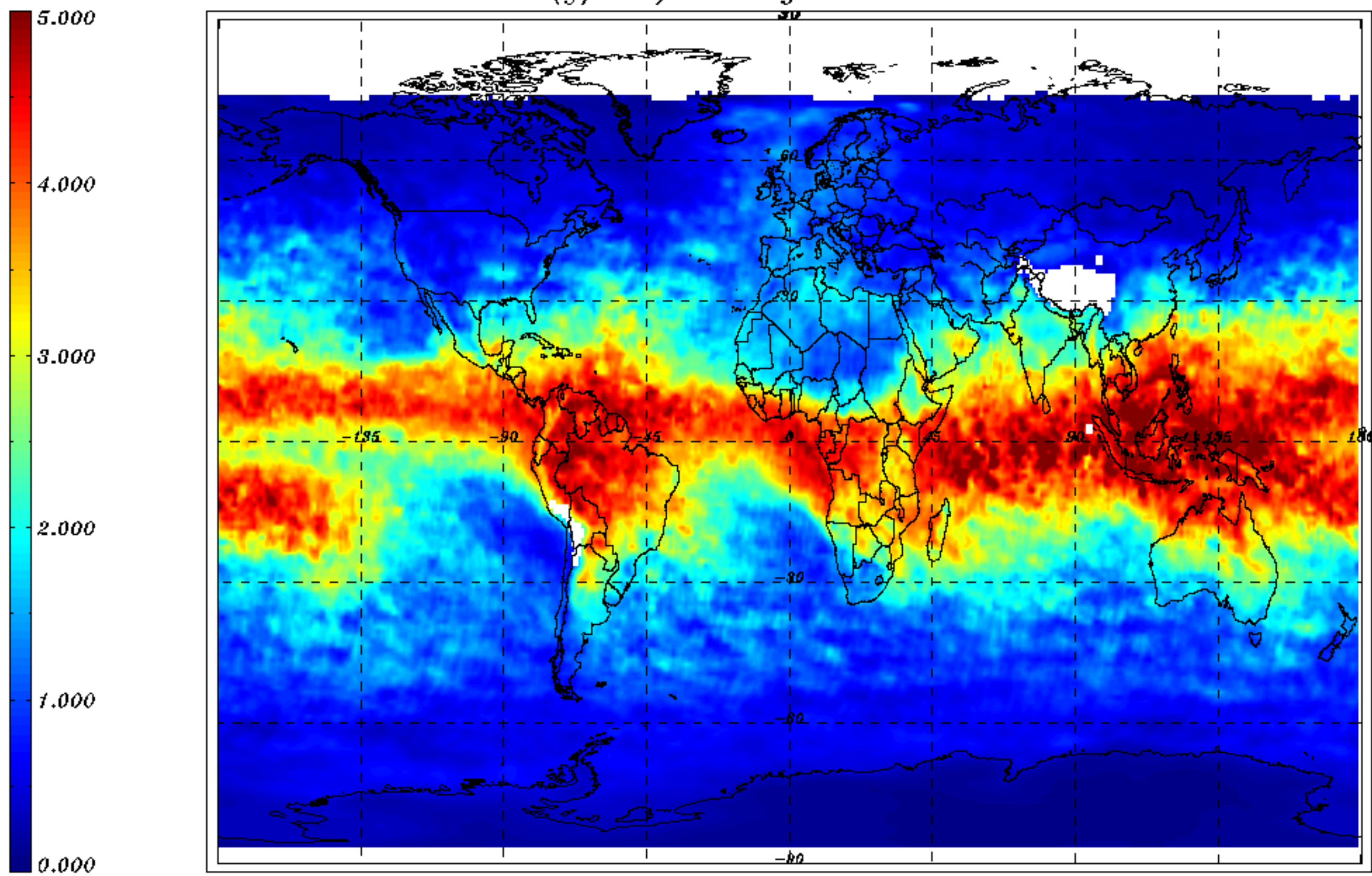
H2O VCD (g/cm 2 ) monthly mean - November 2011
