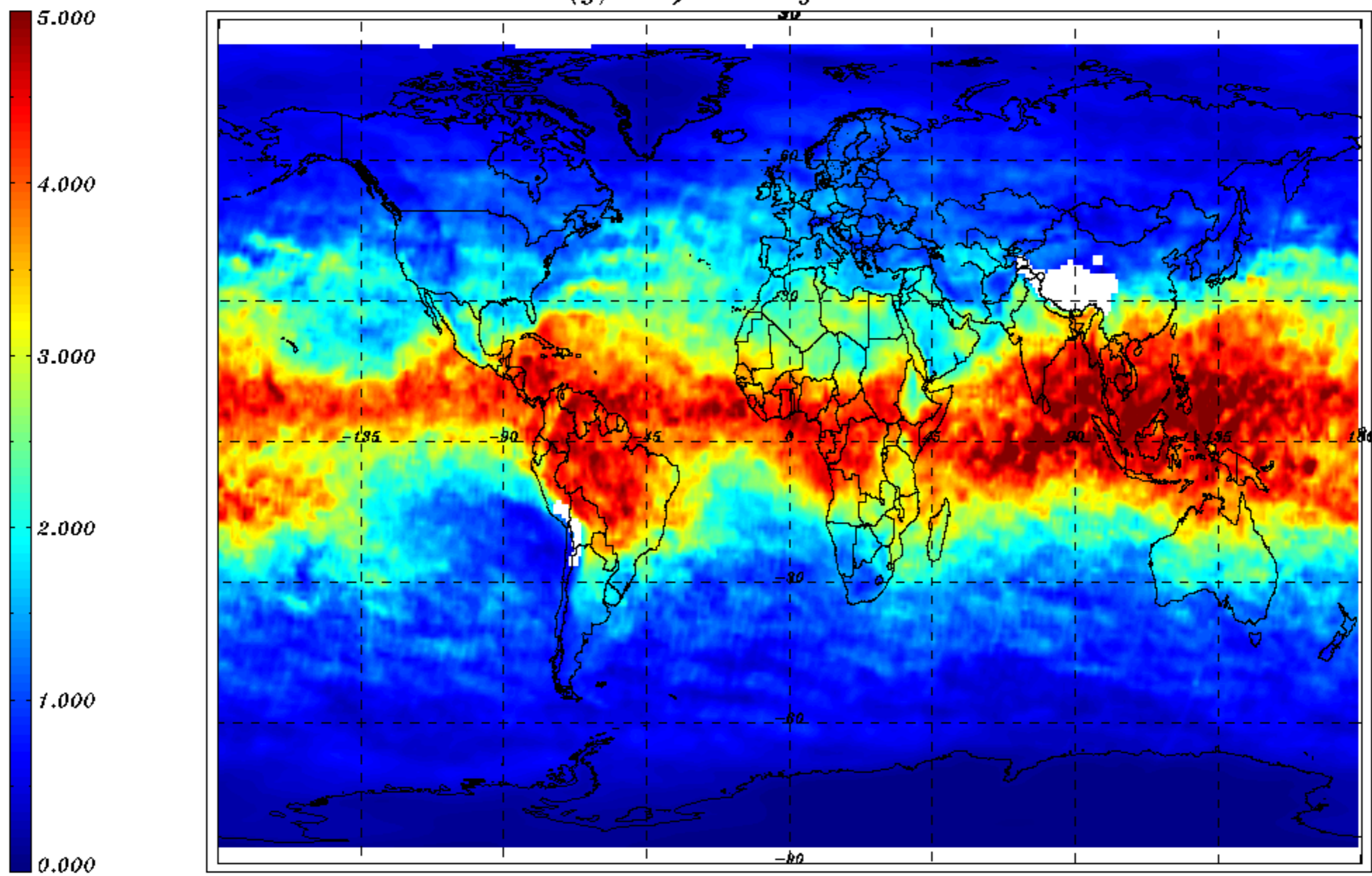
H 2 O VCD (g/cm 2 ) monthly mean - October 2011
