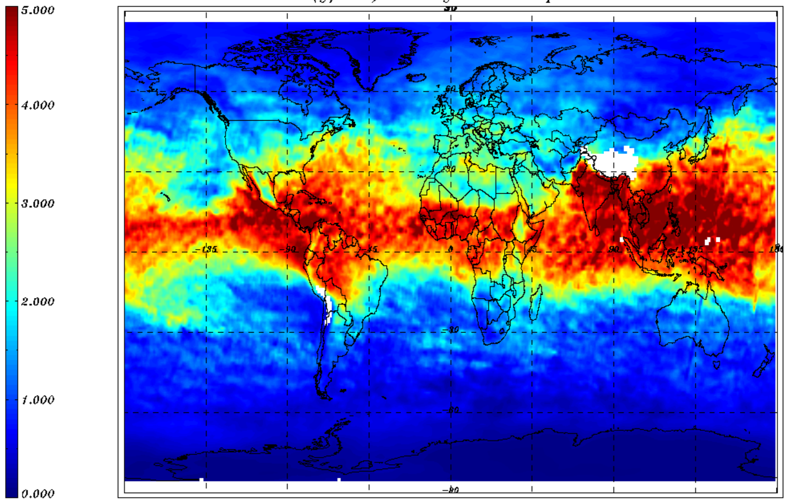
H 2 O VCD (g/cm 2 ) monthly mean – September 2011
