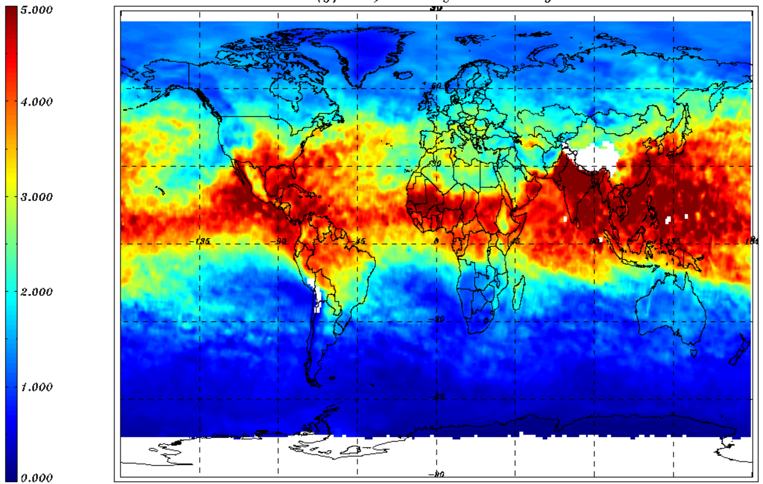
H2O VCD (g/cm 2 ) monthly mean - August 2011
