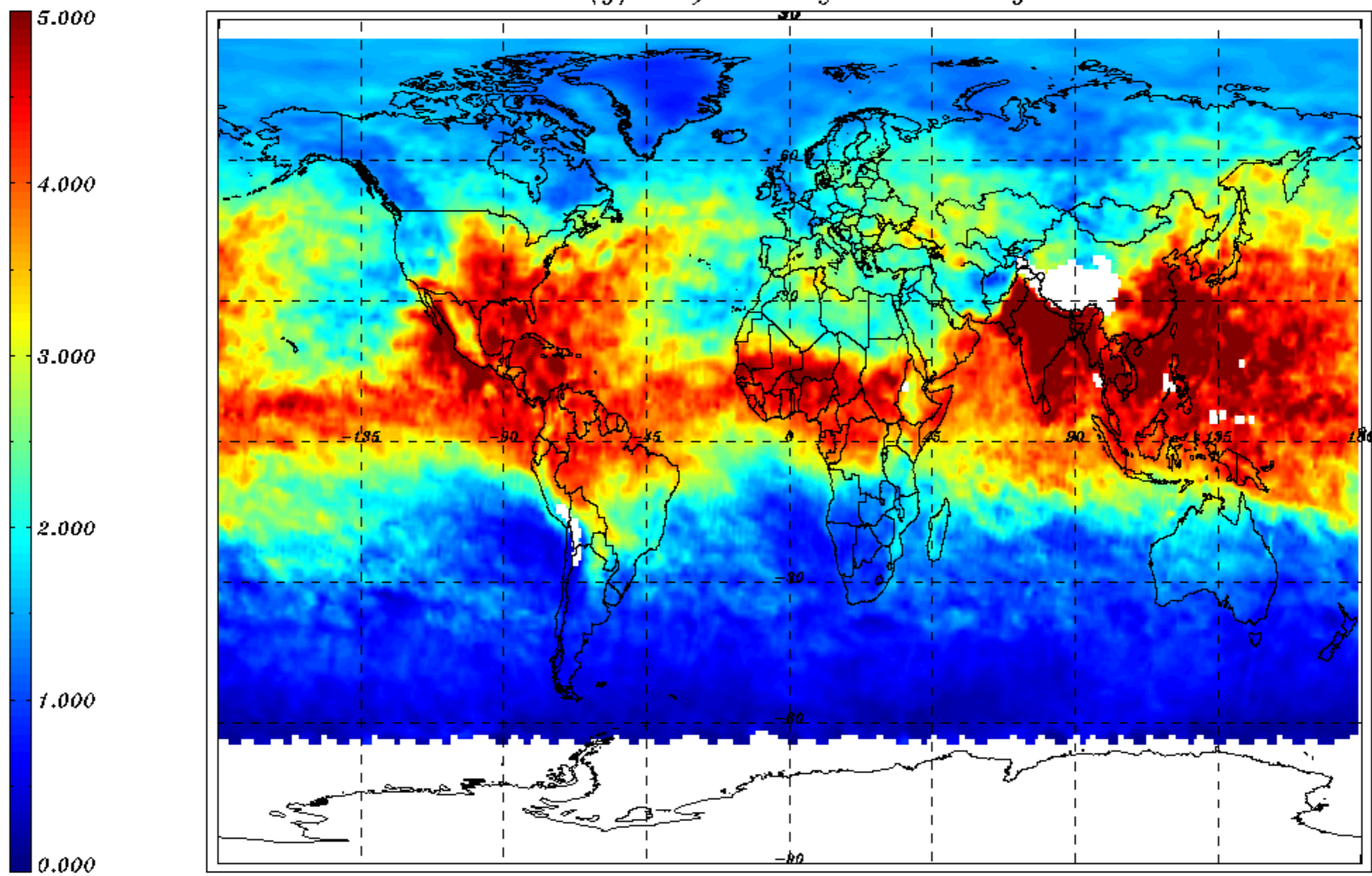
H2O VCD (g/cm 2 ) monthly mean - July 2011
