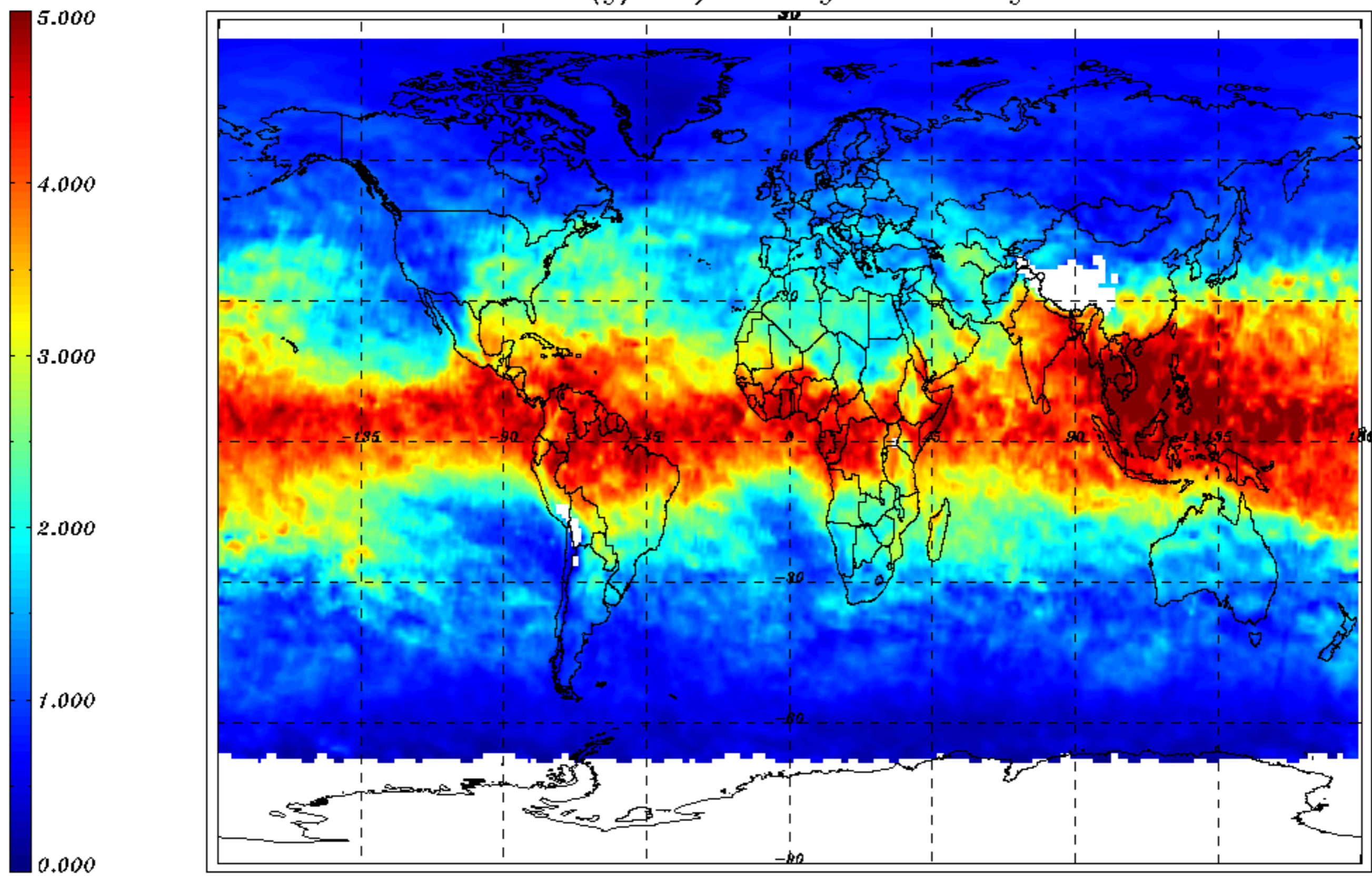
H 2 O VCD (g/cm 2 ) monthly mean - May 2011
