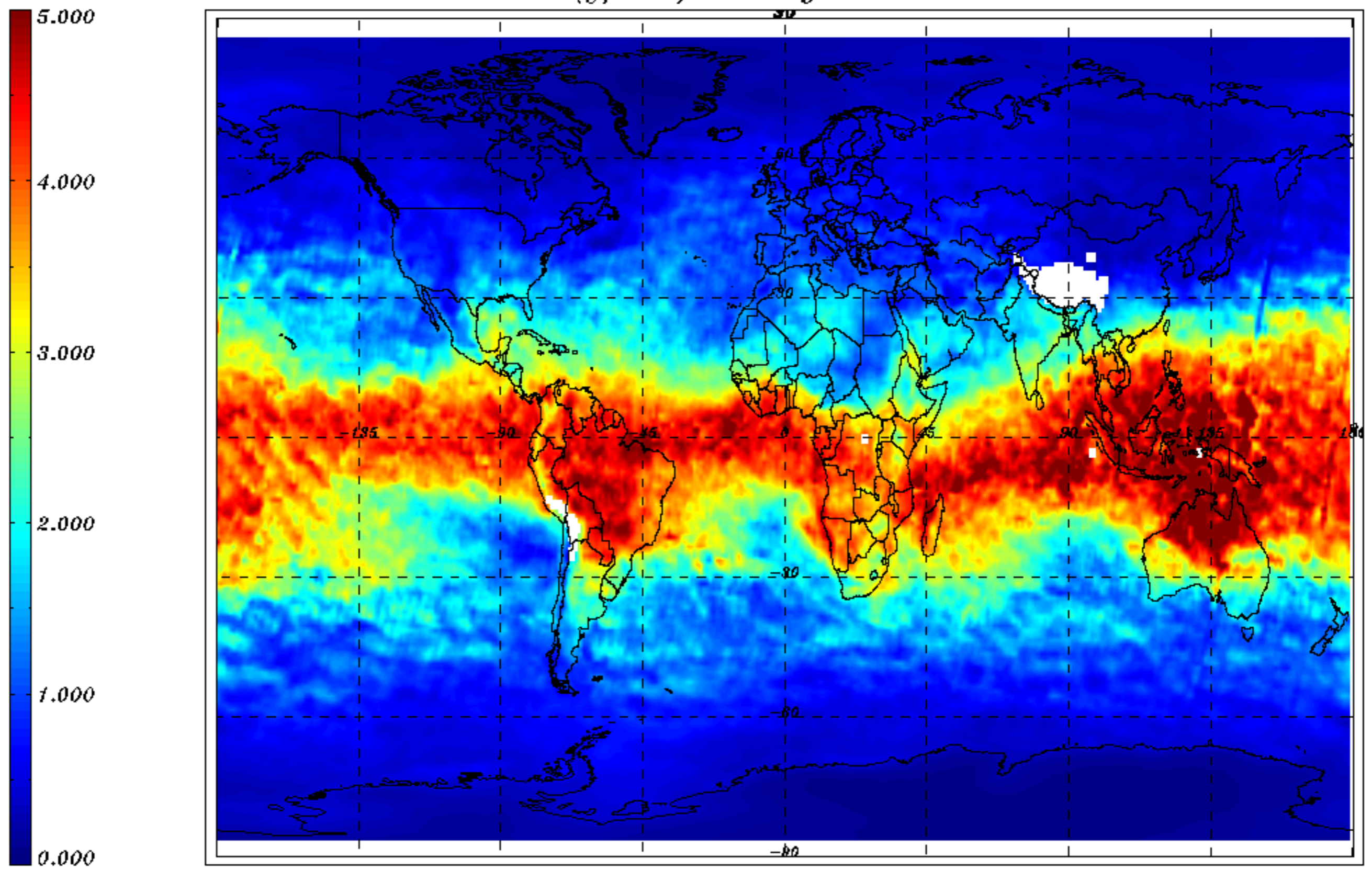
H2O VCD (g/cm 2 ) monthly mean - March 2011
