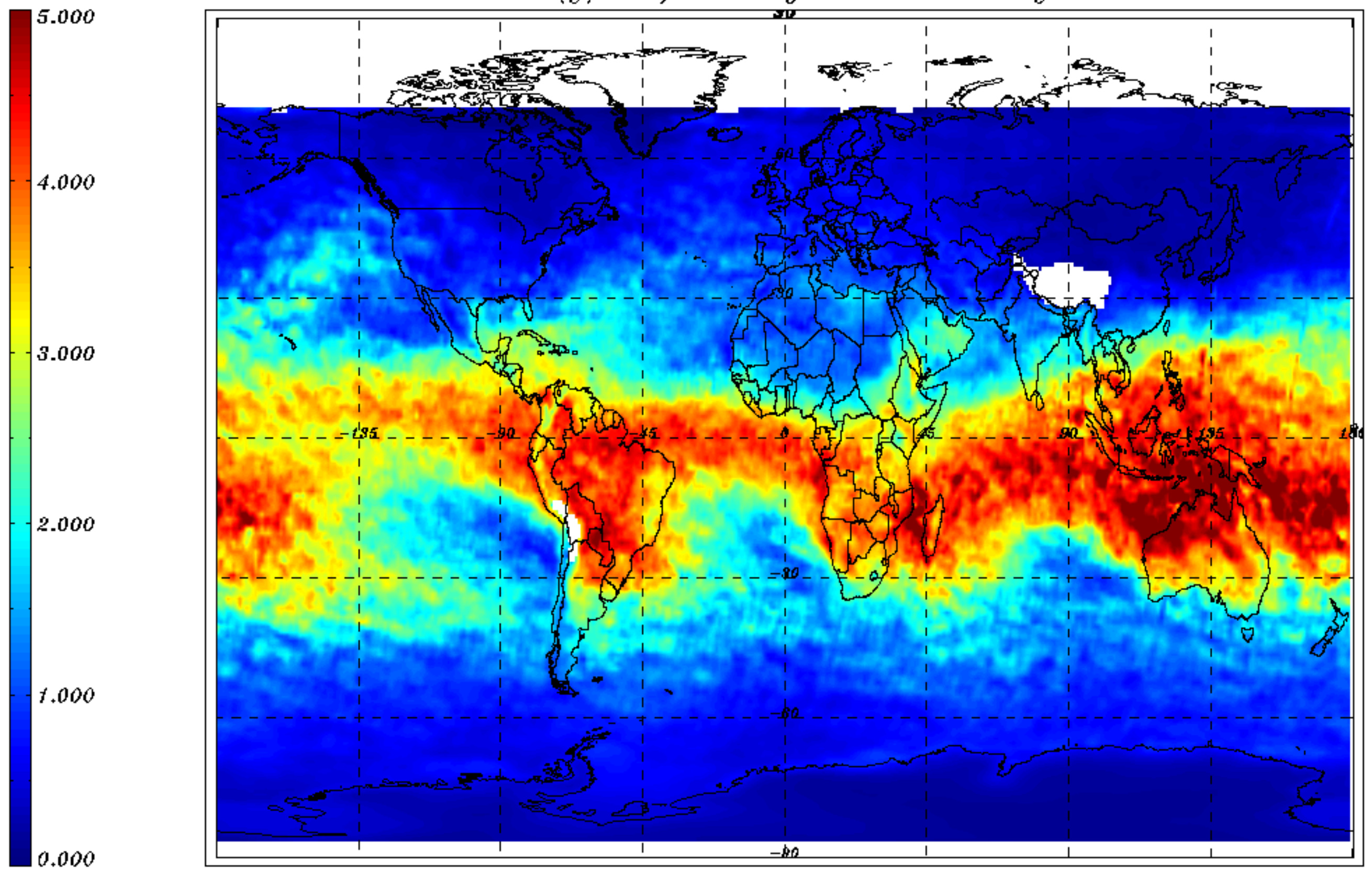
H 2 O VCD (g/cm 2 ) monthly mean - January 2011
