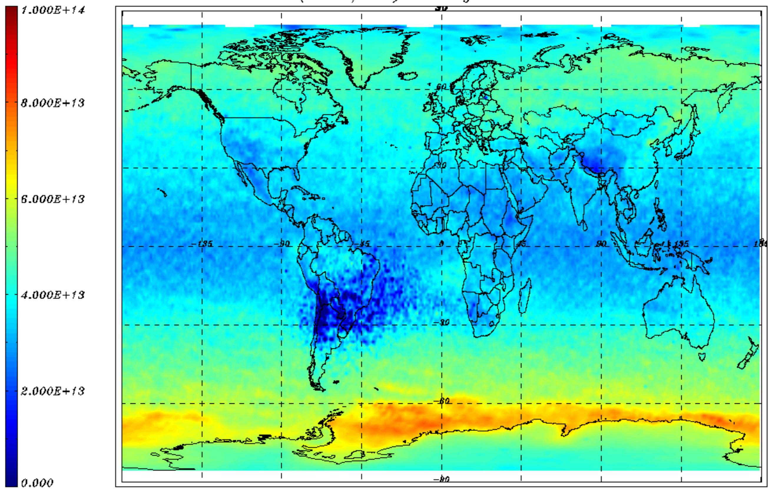
BrO VCD (molec/cm 2 ) monthly mean - October 2011
