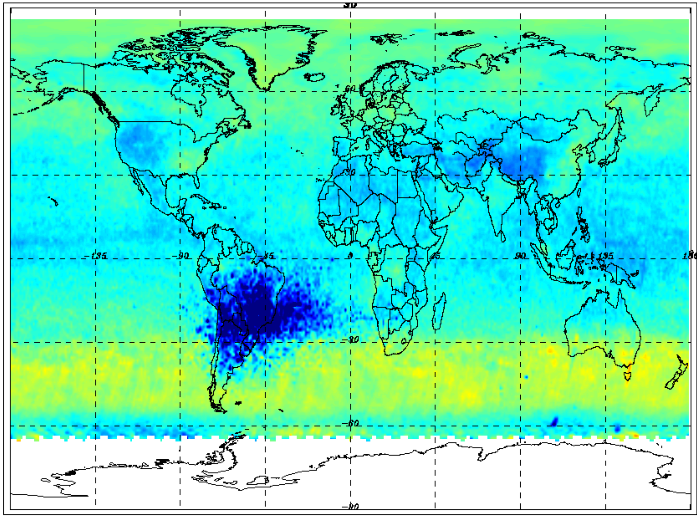
BrO VCD (molec/cm 2 ) monthly mean – July 2011
