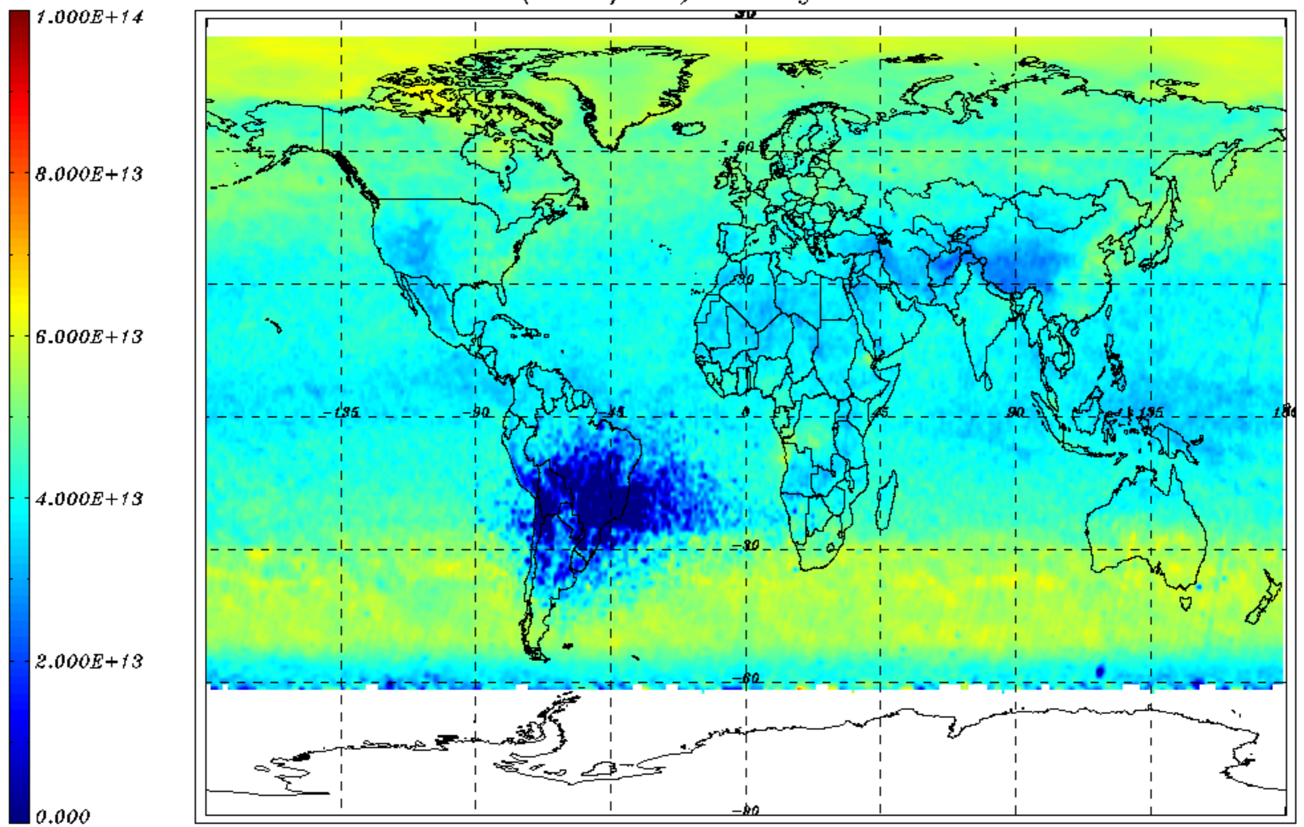
BrO VCD (molec/cm 2 ) monthly mean - June 2011
