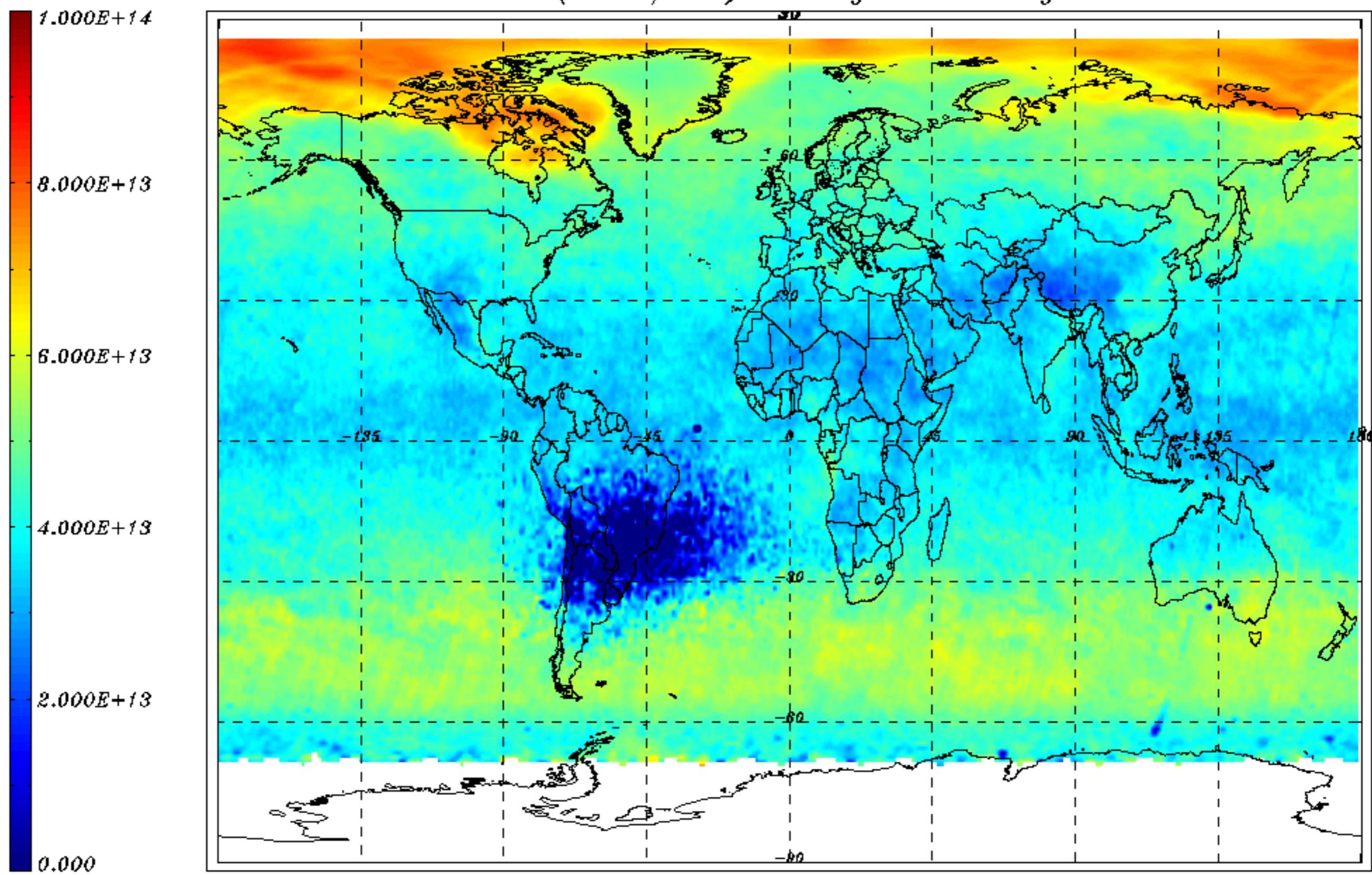
BrO VCD (molec/cm 2 ) monthly mean - May 2011
