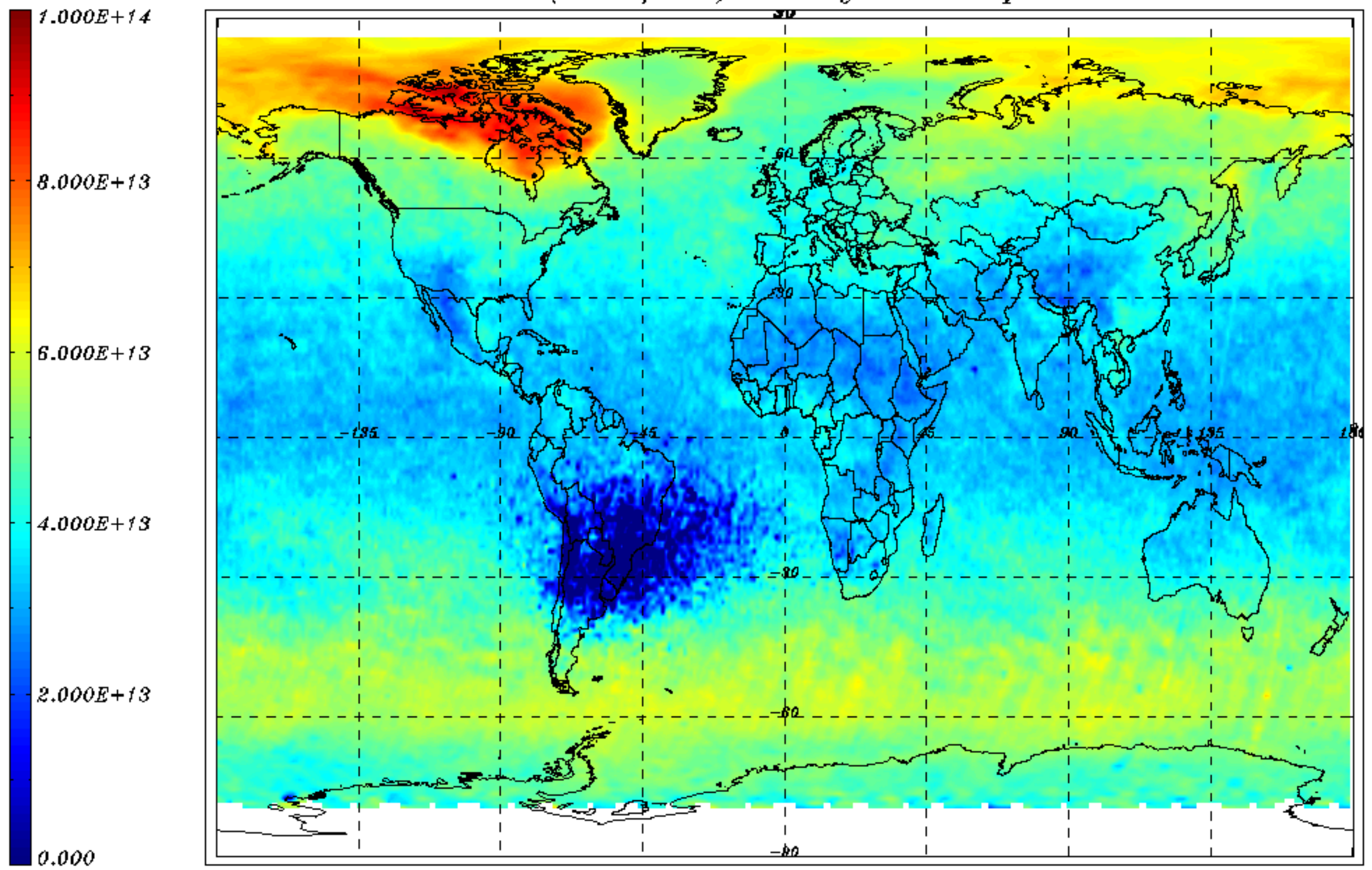
BrO VCD (molec/cm 2 ) monthly mean - April 2011
