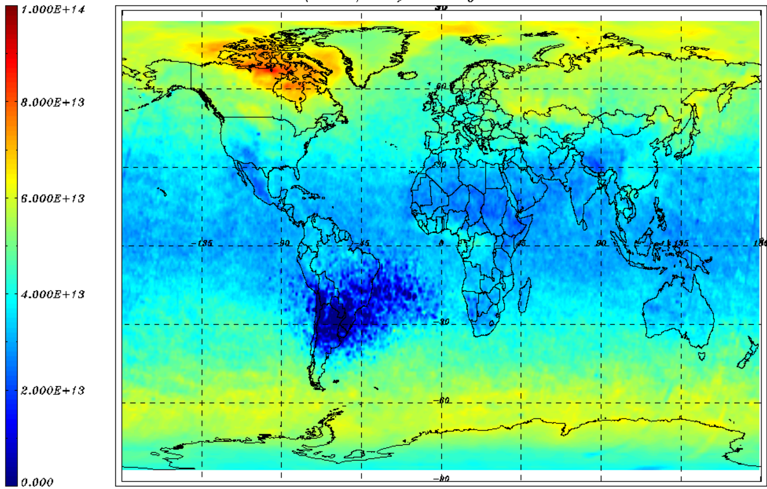
BrO VCD (molec/cm2) monthly mean - March 2011
