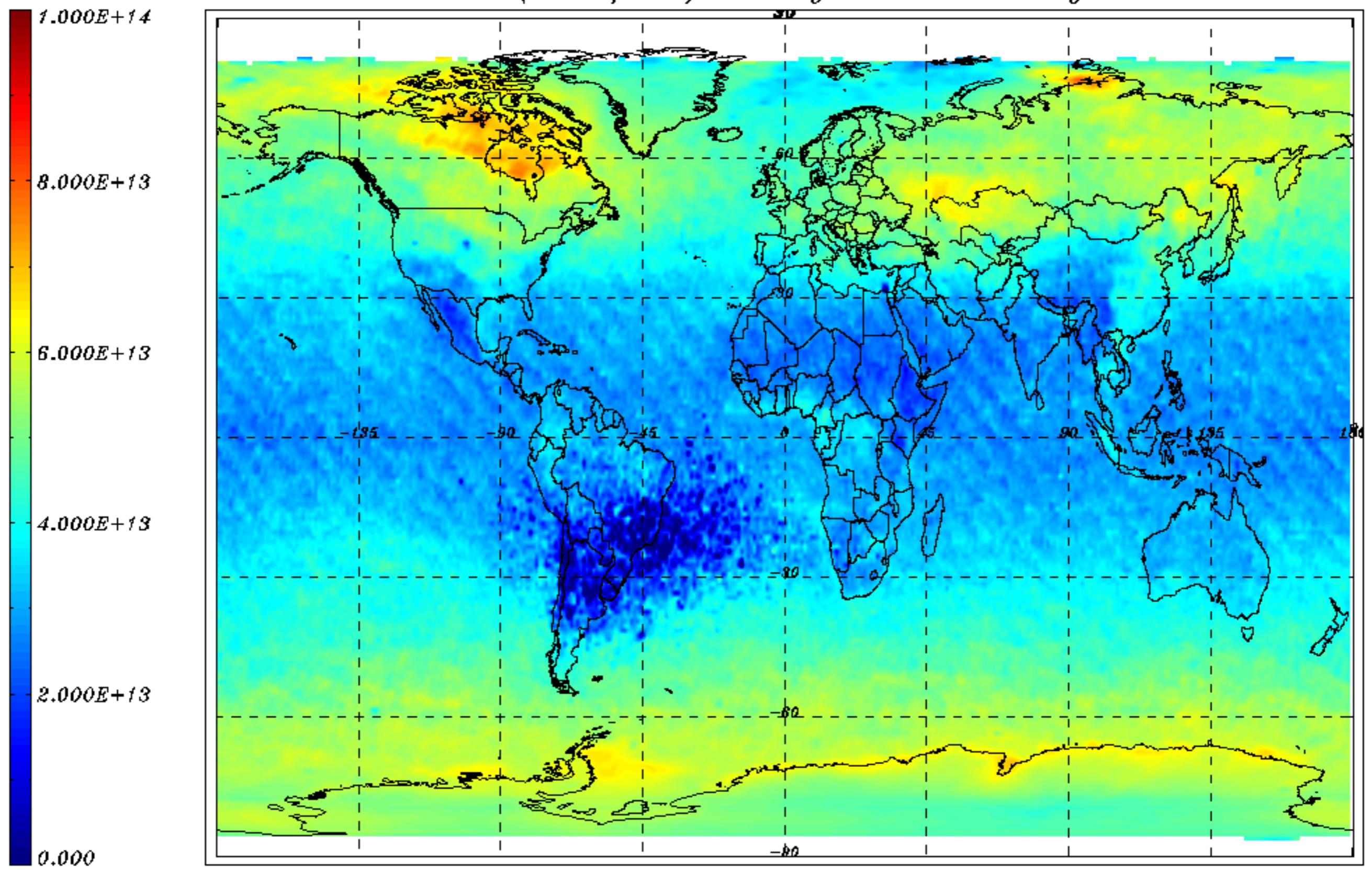
BrO VCD (molec/cm 2 ) monthly mean - February 2011
