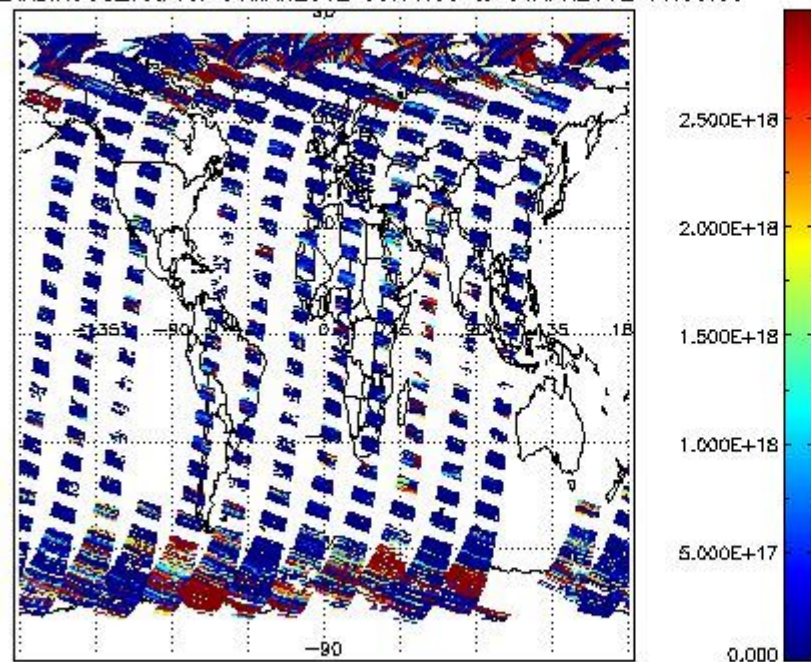
SCIDL2P_NADIR3CO_vcd for 31MAR2012 00:00:00 to 01APR2012 00:00:00
