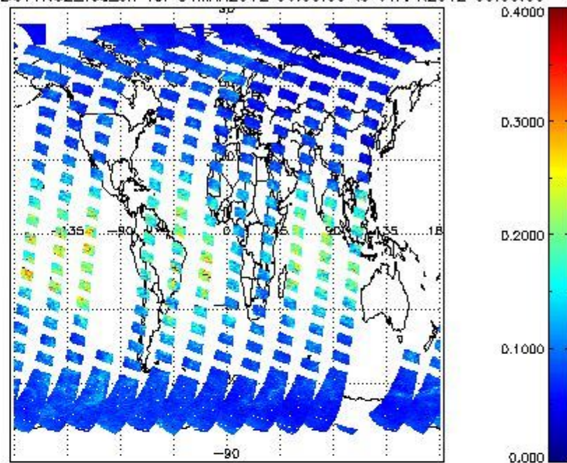
SCIOL2P_NADUV1NO2_vcd_err for 31MAR2012 00:00:00 to 01APR2012 00:00:00
