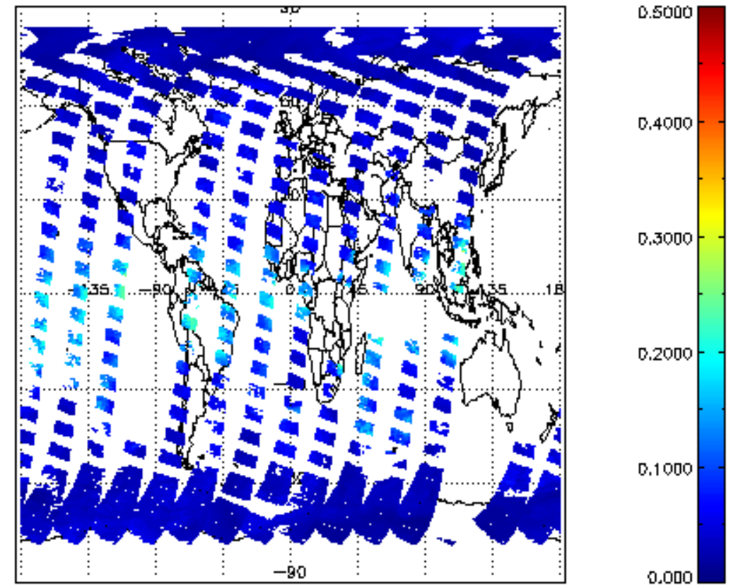
SCIOL2P_NADUV8H20_vcd_err for 31MAR2012 00:00:00 to 01APR2012 00:00:00
