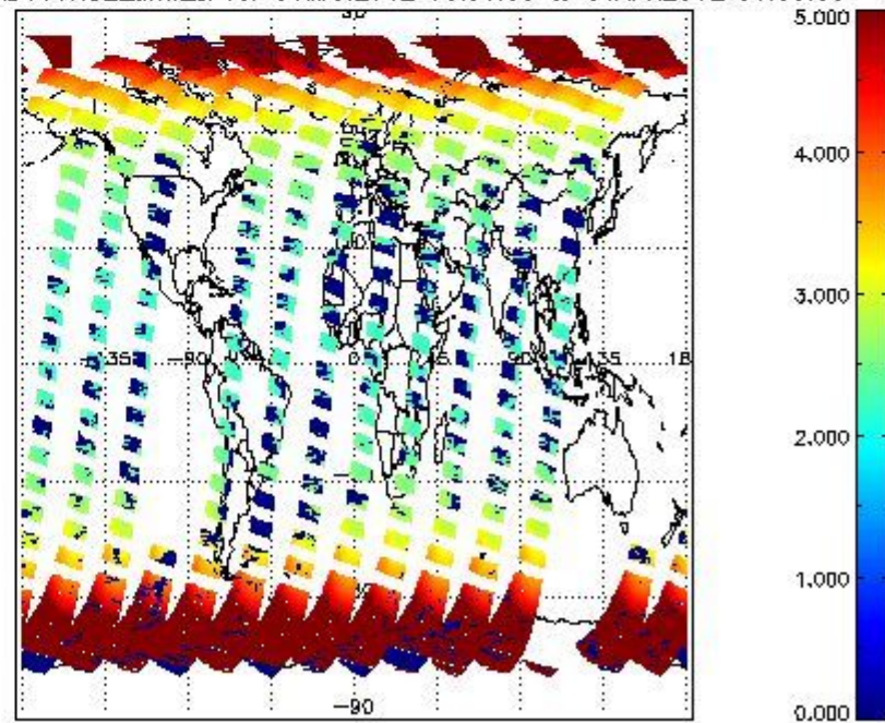
SCIOL2P_NADUV1NO2_amf_cl for 31MAR2012 00:00:00 to 01APR2012 00:00:00
