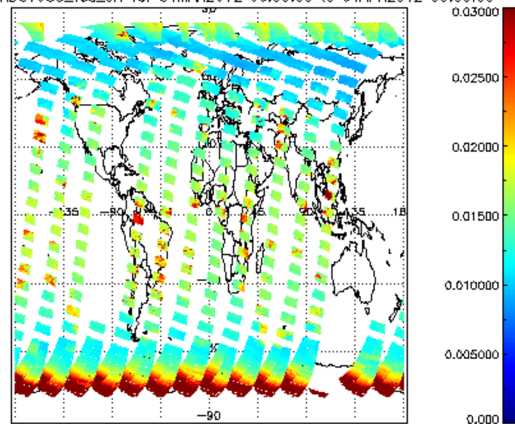
SCIOL2P_NADUV003_vcd_err for 31MAR2012 00:00:00 to 01APR2012 00:00:00
