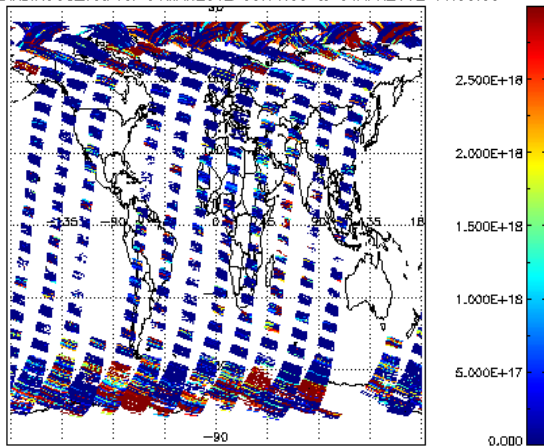
SCIOL2P_NADIR3CO_vcd for 31MAR2012 00:00:00 to 01APR2012 00:00:00
