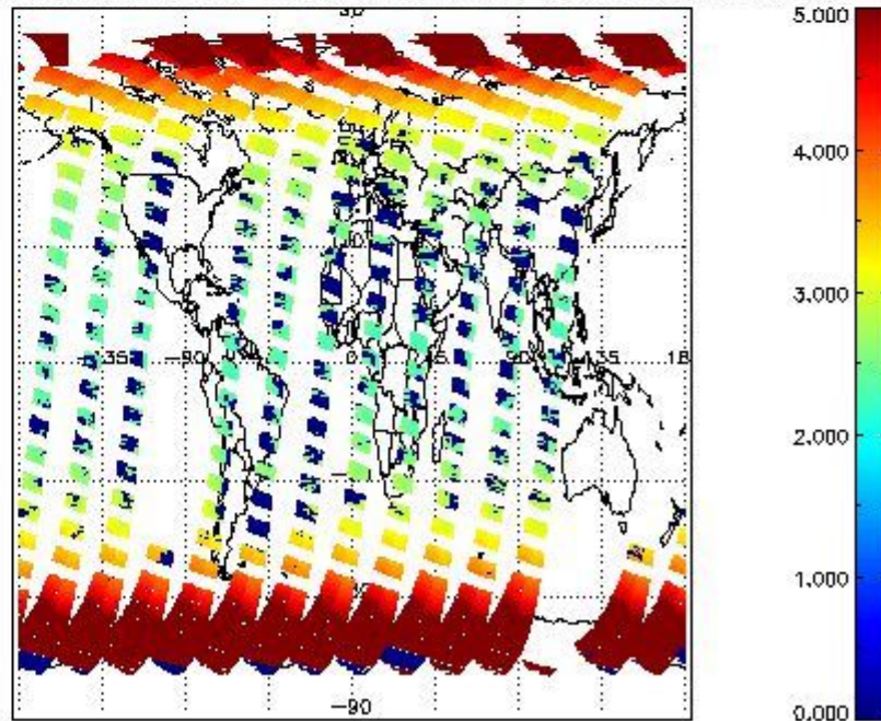
SCIOL2P_NADUV003_amf_cl for 31MAR2012 00:00:00 to 01APR2012 00:00:00
