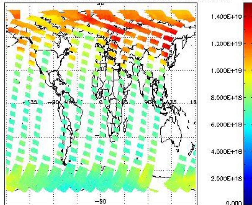
SCIOL2P_NADUV003_vcd for 31MAR2012 00:00:00 to 01APR2012 00:00:00
