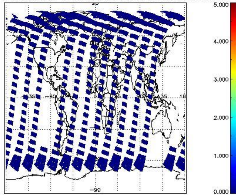
SCIOL2P_NADUV7S02_amf_cl for 31MAR2012 00:00:00 to 01APR2012 00:00:00
