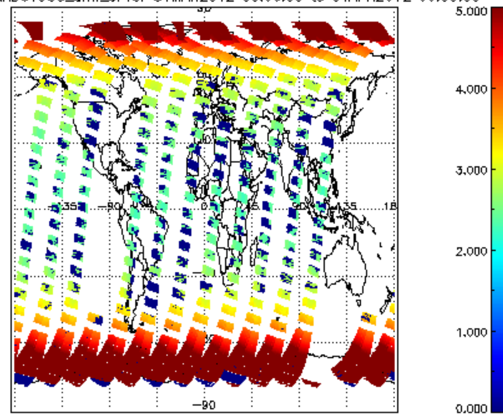
SCIOL2P_NADUV003_amf_cl for 31MAR2012 00:00:00 to 01APR2012 00:00:00
