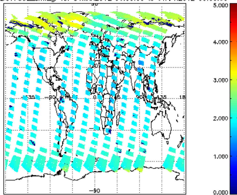
SCIOL2P_NADUV7S02_amf_gr for 31MAR2012 00:00:00 to 01APR2012 00:00:00
