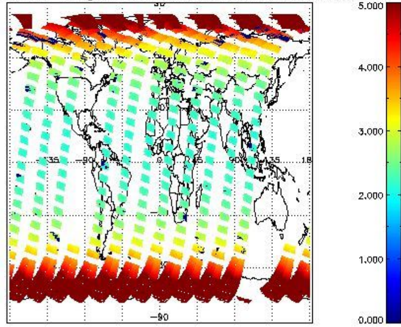
SCIOL2P_NADUV3BRO_amf_gr for 31MAR2012 00:00:00 to 01APR2012 00:00:00
