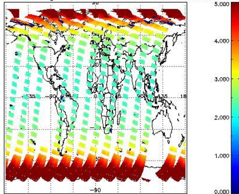
SCIOL2P_NADUV003_amf_gr for 31MAR2012 00:00:00 to 01APR2012 00:00:00
