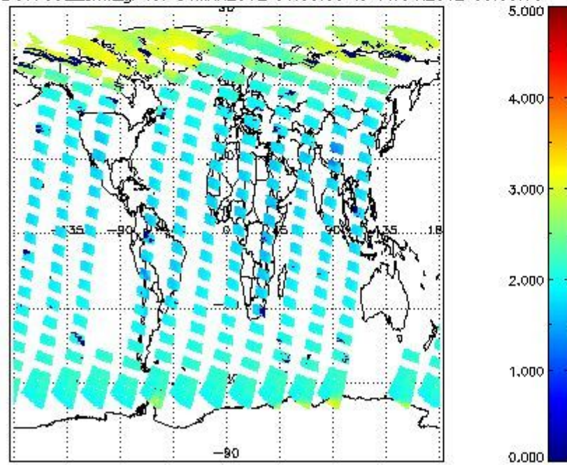
SCIOL2P_NADUV7S02_amf_gr for 31MAR2012 00:00:00 to 01APR2012 00:00:00
