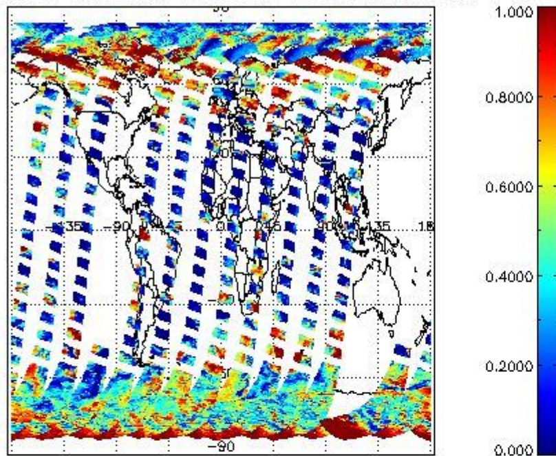
cLfrac for 31MAR2012 00:00:00 to 01APR2012 00:00:00
