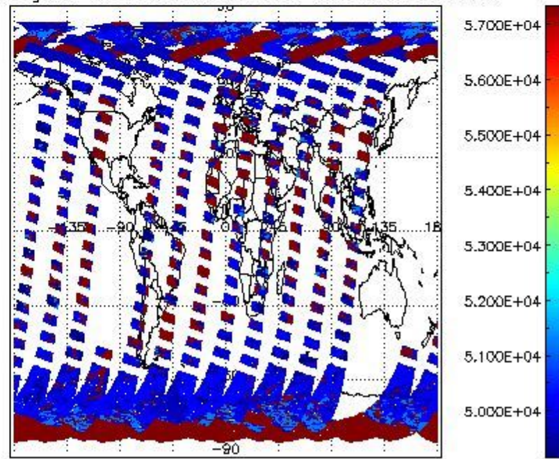
cloud_flags for 31MAR2012 00:00:00 to 01APR2012 00:00:00
