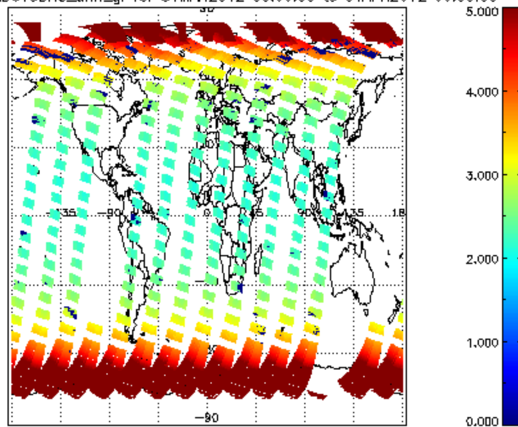
SCIOL2P_NADUV3BRO_amf_gr for 31MAR2012 00:00:00 to 01APR2012 00:00:00
