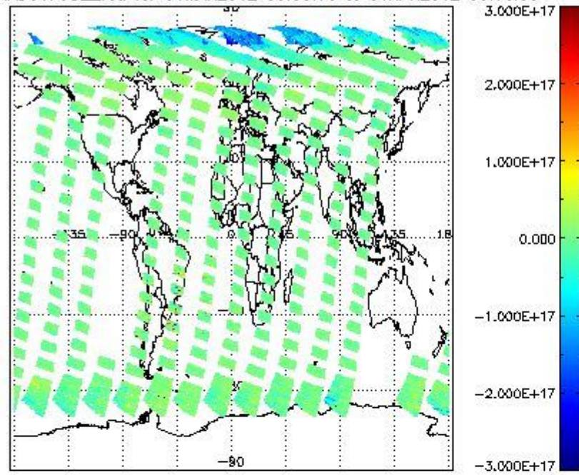
SCIOL2P_NADUV7S02_vcd for 31MAR2012 00:00:00 to 01APR2012 00:00:00
