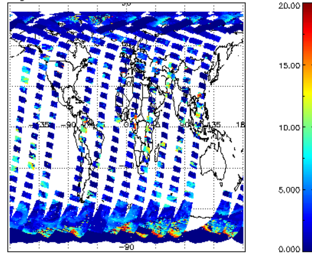
cL_top_height for 31MAR2012 00:00:00 to 01APR2012 00:00:00
