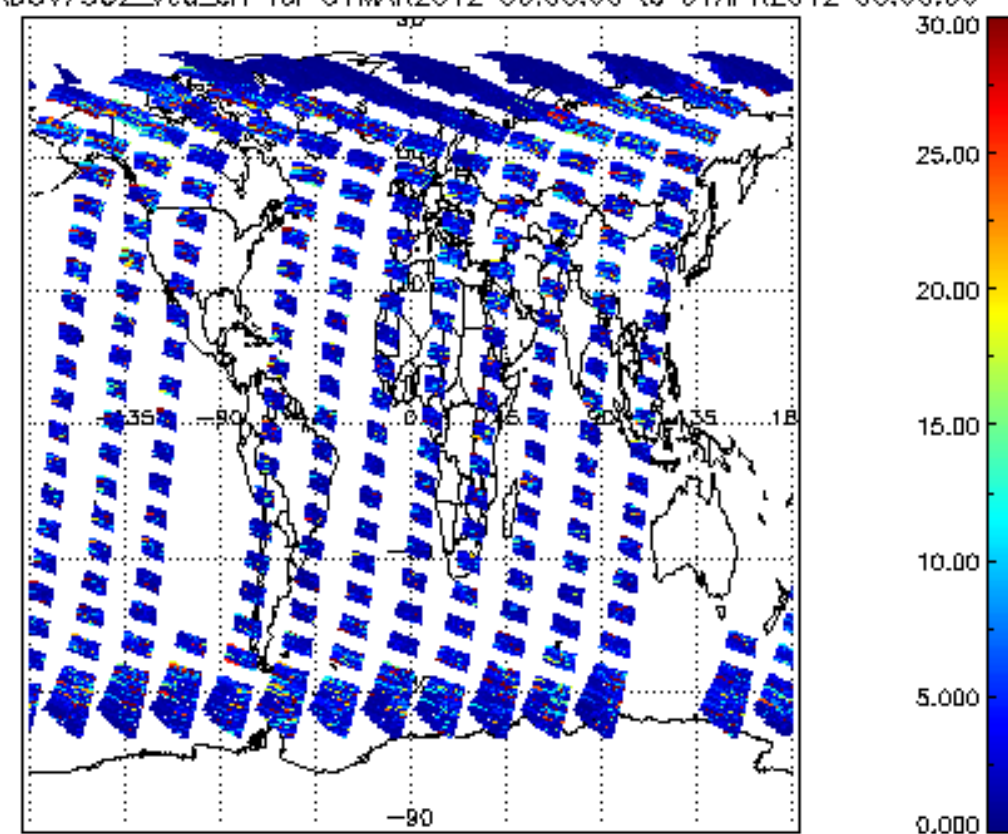
SCIOL2P_NADUV7S02_vcd_err for 31MAR2012 00:00:00 to 01APR2012 00:00:00
