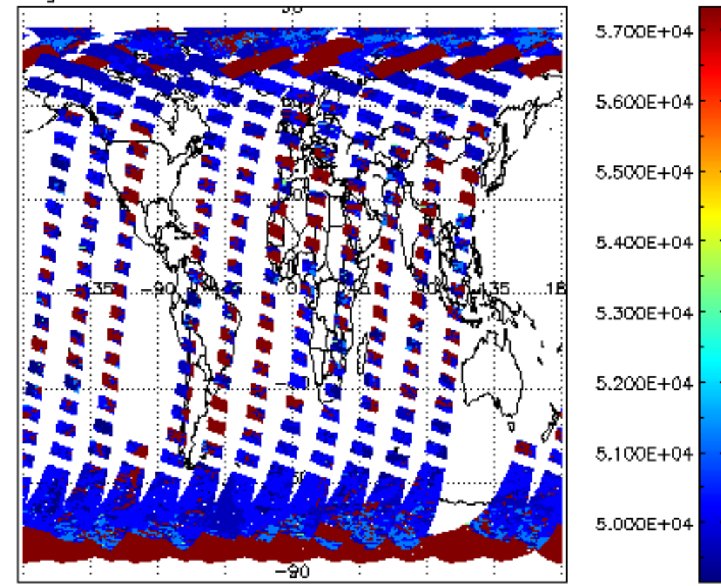
cloud_flags for 31MAR2012 00:00:00 to 01APR2012 00:00:00
