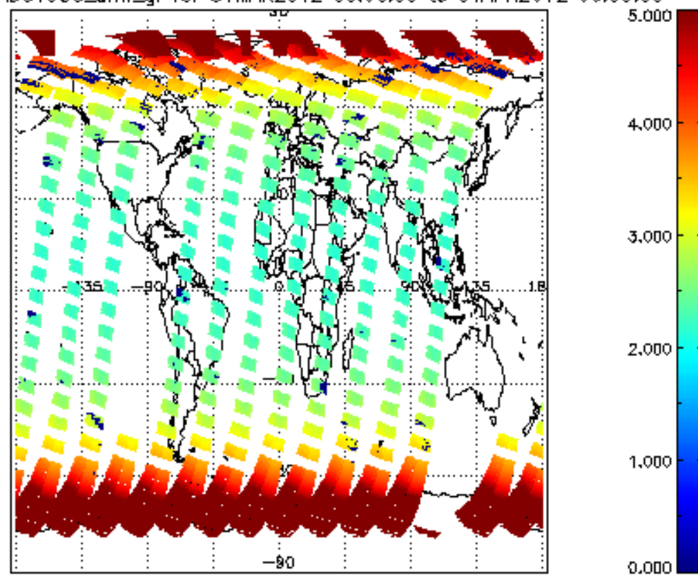
SCIOL2P_NADUV003_amf_gr for 31MAR2012 00:00:00 to 01APR2012 00:00:00
