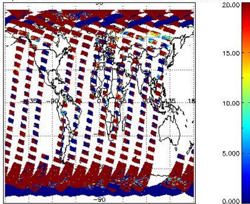
cLopt_depth for 31MAR2012 00:00:00 to 01APR2012 00:00:00
