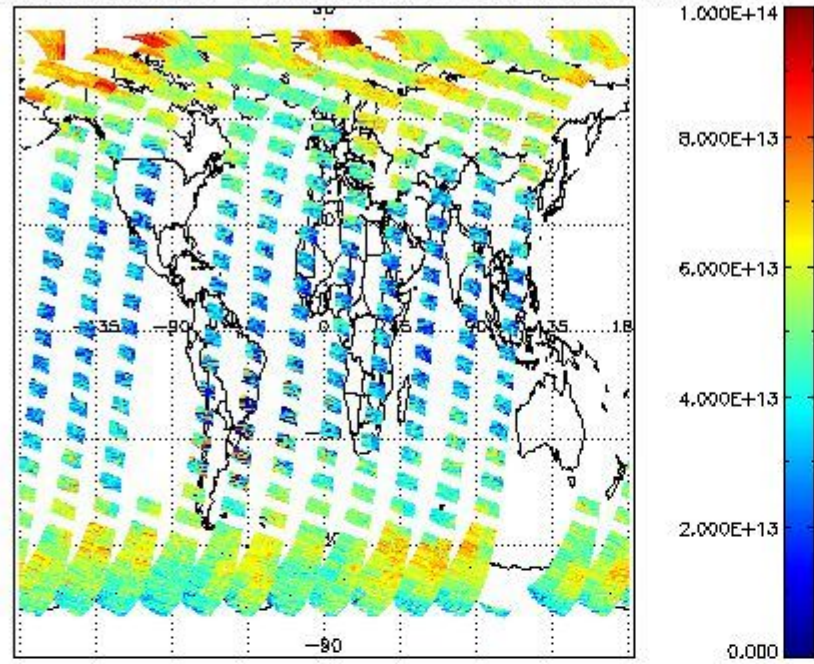
SCIOL2P_NADUV3BRO_vcd for 31MAR2012 00:00:00 to 01APR2012 00:00:00
