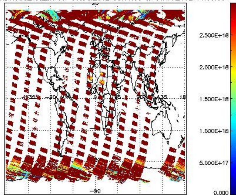
SCIDL2P_NADIR3CO_vcd_err for 31MAR2012 00:00:00 to 01APR2012 00:00:00
