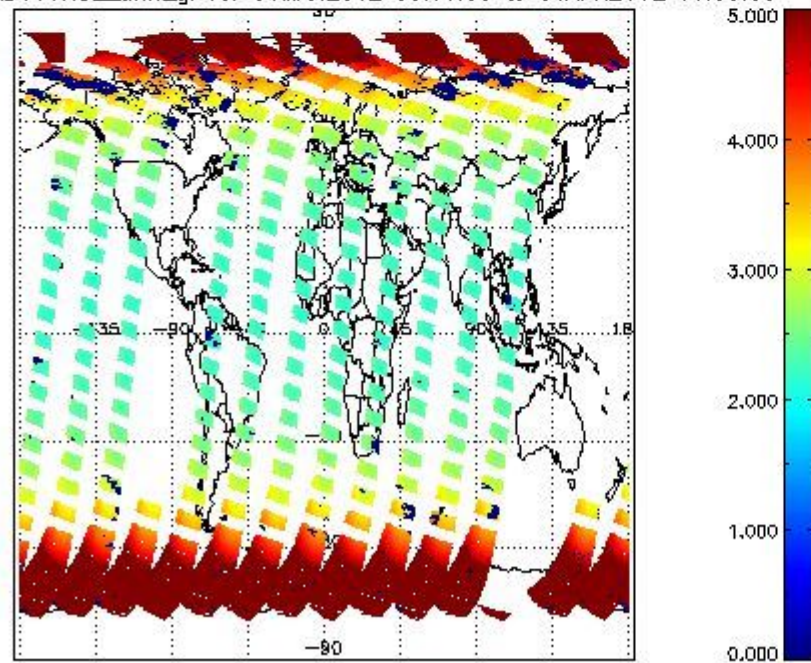
SCIOL2P_NADUV1NO2_amf_gr for 31MAR2012 00:00:00 to 01APR2012 00:00:00
