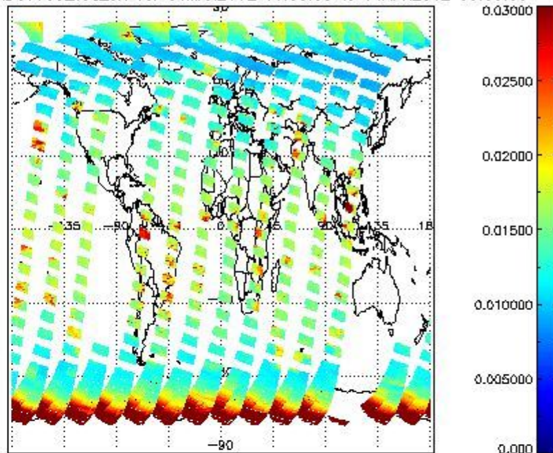
SCIOL2P_NADUV003_vcd_err for 31MAR2012 00:00:00 to 01APR2012 00:00:00
