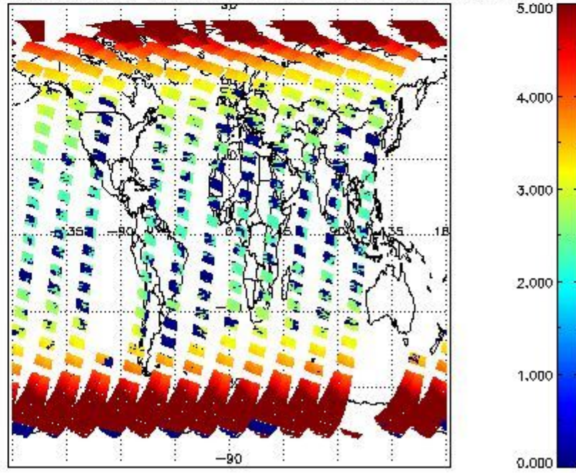
SCIOL2P_NADUV3BRO_amf_cl for 31MAR2012 00:00:00 to 01APR2012 00:00:00
