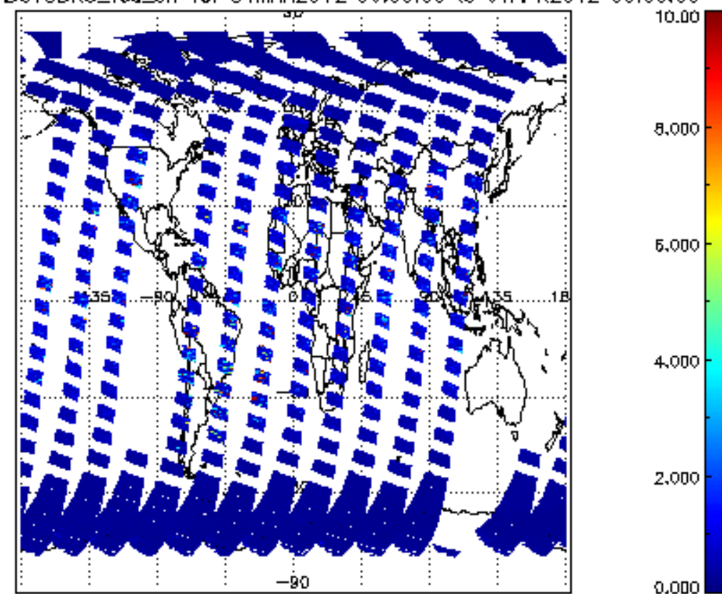
SCIOL2P_NADUV3BRO_vcd_err for 31MAR2012 00:00:00 to 01APR2012 00:00:00
