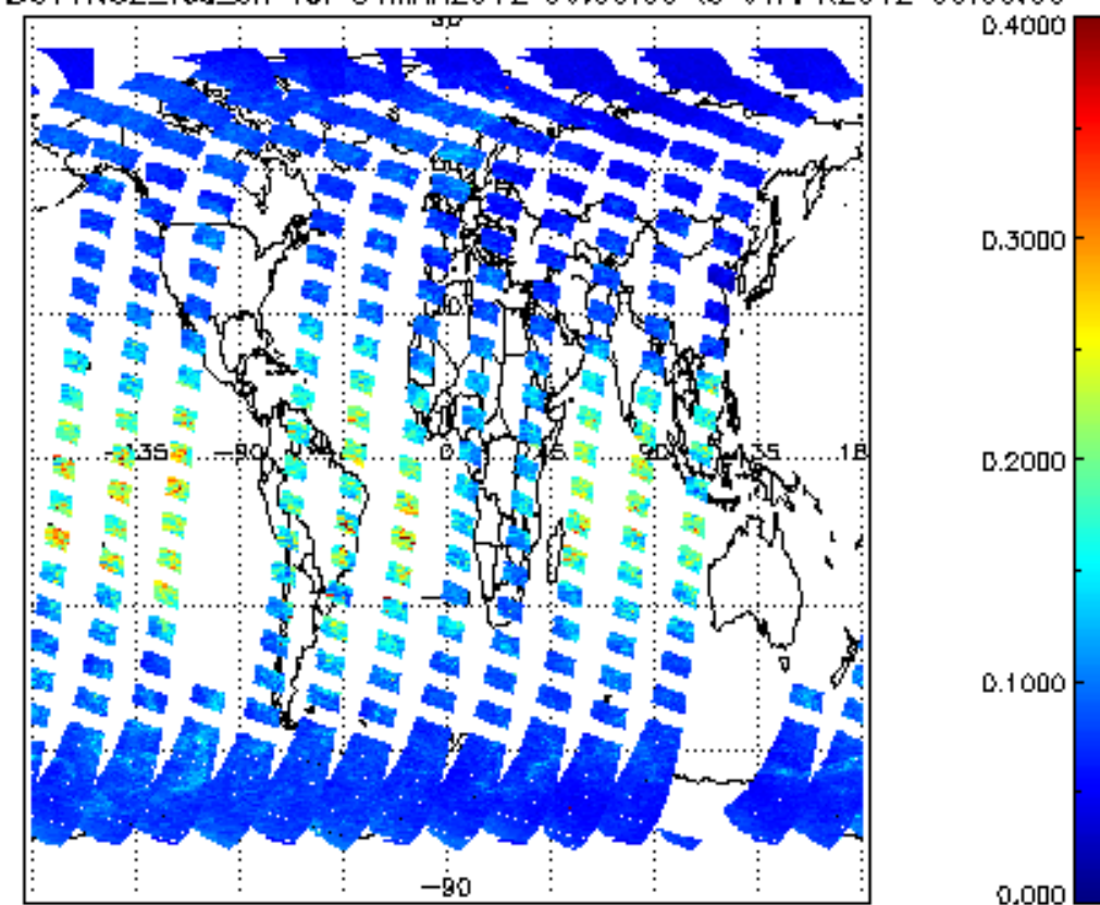
SCIOL2P_NADUV1NO2_vcd_err for 31MAR2012 00:00:00 to 01APR2012 00:00:00
