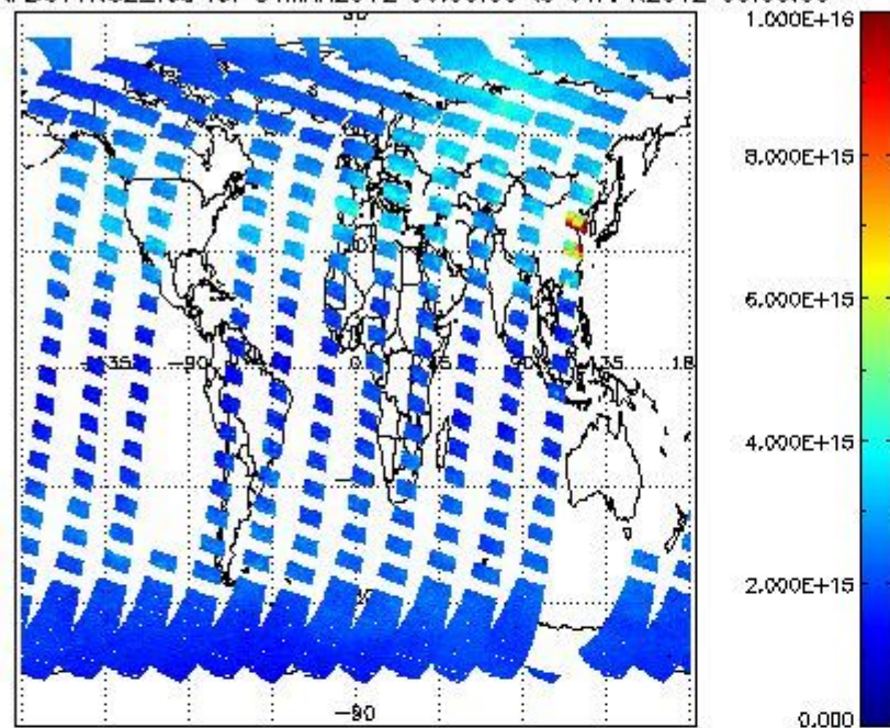
SCIOL2P_NADUV1NO2_vcd for 31MAR2012 00:00:00 to 01APR2012 00:00:00
