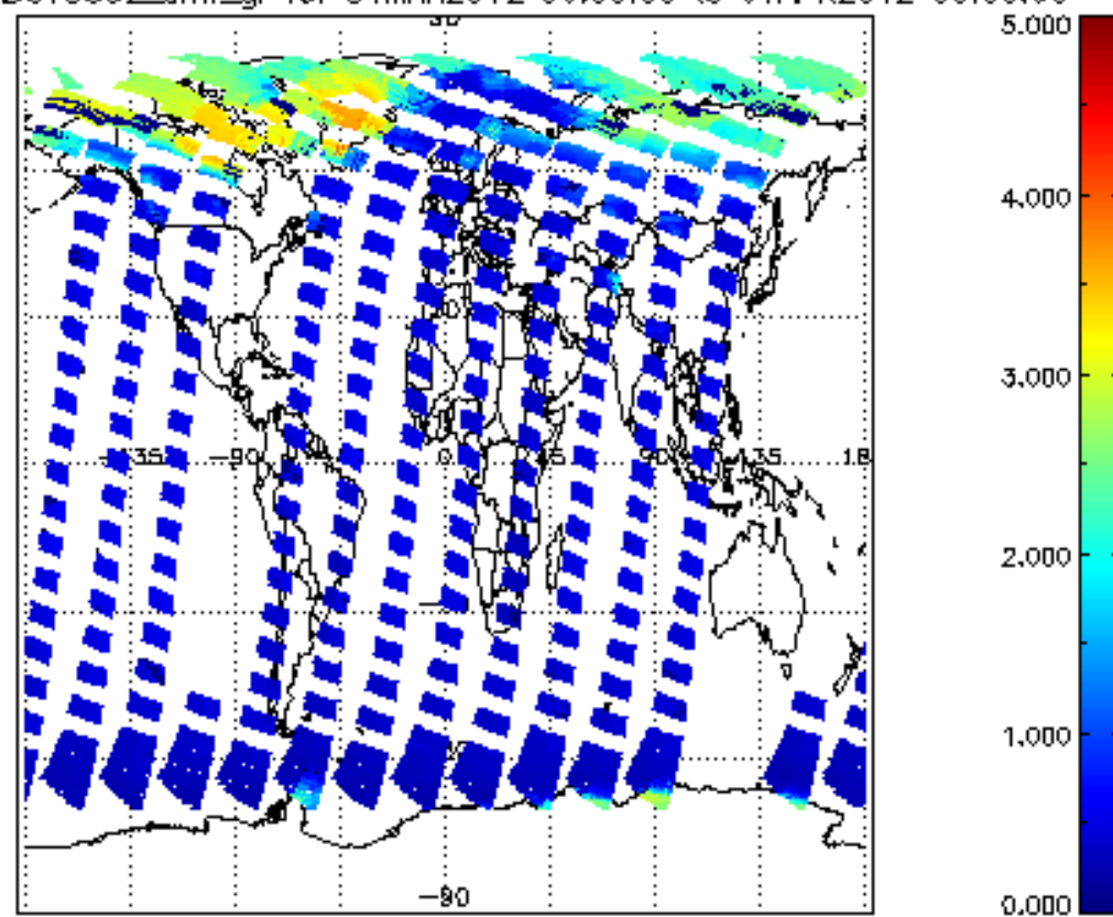
SCIOL2P_NADUV5S02_amf_gr for 31MAR2012 00:00:00 to 01APR2012 00:00:00
