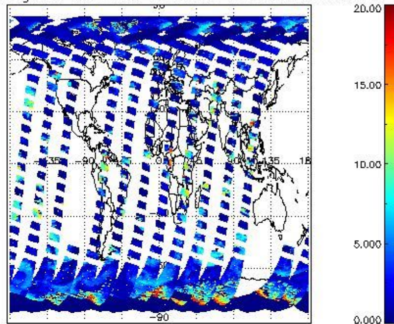
cL_top_height for 31MAR2012 00:00:00 to 01APR2012 00:00:00
