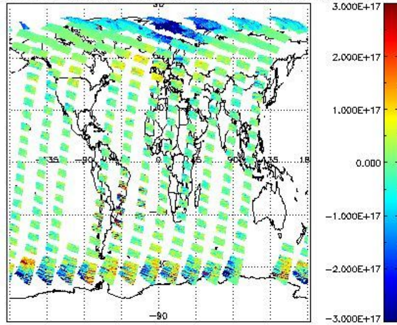
SCIOL2P_NADUV5SO2_vcd for 31MAR2012 00:00:00 to 01APR2012 00:00:00
