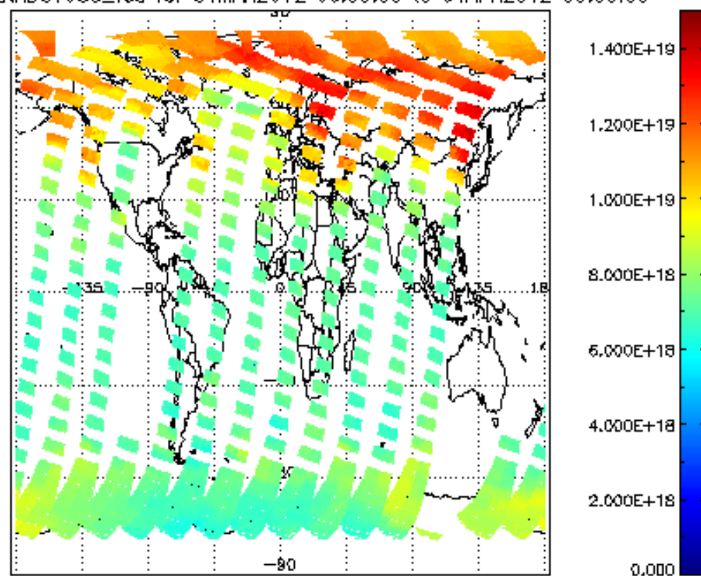
SCIOL2P_NADUV003_vcd for 31MAR2012 00:00:00 to 01APR2012 00:00:00
