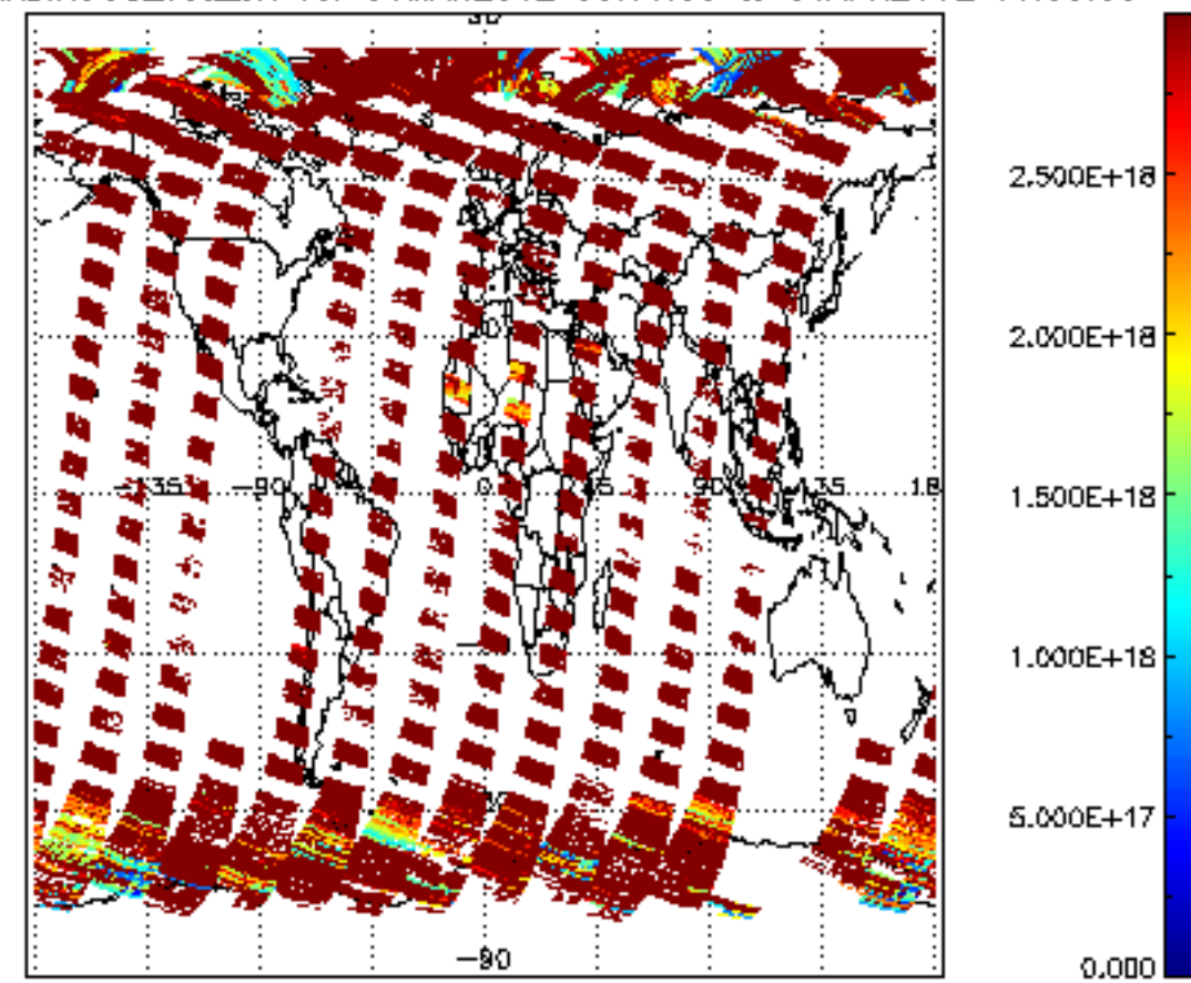
SCIOL2P_NADIR3CO_vcdLerr for 31MAR2012 00:00:00 to 01APR2012 00:00:00
