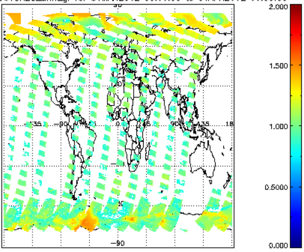
SCIOL2P_NADUV8H20_amf_gr for 31MAR2012 00:00:00 to 01APR2012 00:00:00
