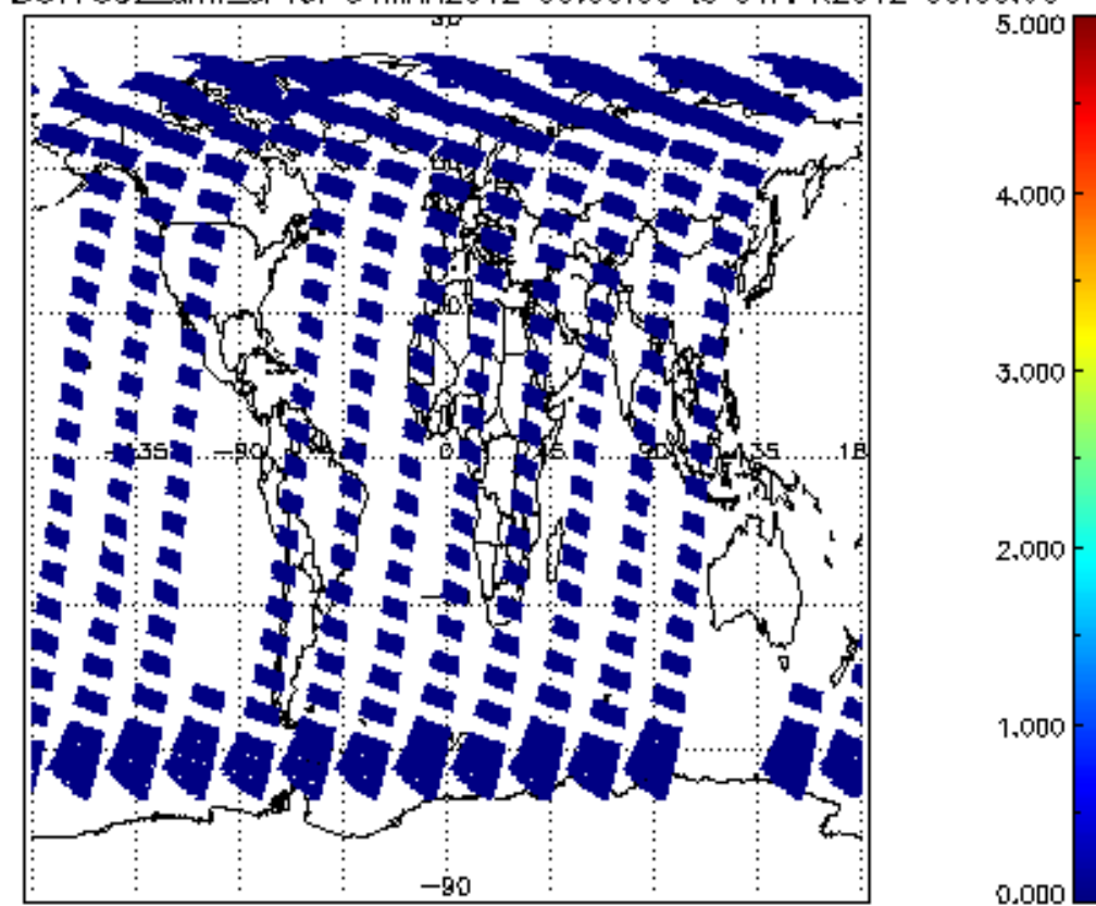
SCIOL2P_NADUV7S02_amf_cl for 31MAR2012 00:00:00 to 01APR2012 00:00:00
