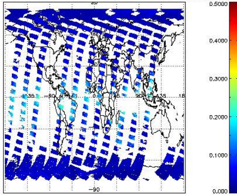
SCIOL2P_NADUVBH20_vcd_err for 31MAR2012 00:00:00 to 01APR2012 00:00:00
