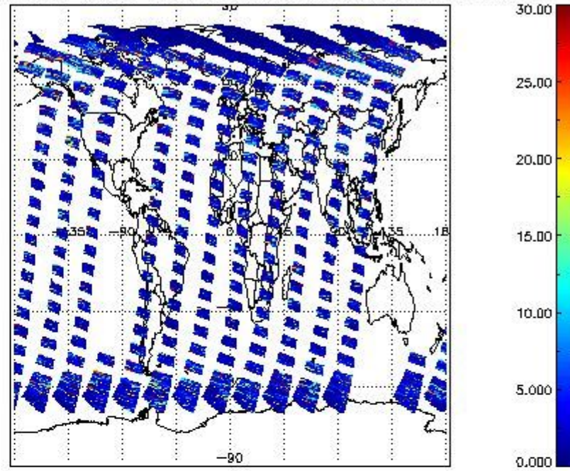
SCIOL2P_NADUV5SO2_vcd_err for 31MAR2012 00:00:00 to 01APR2012 00:00:00
