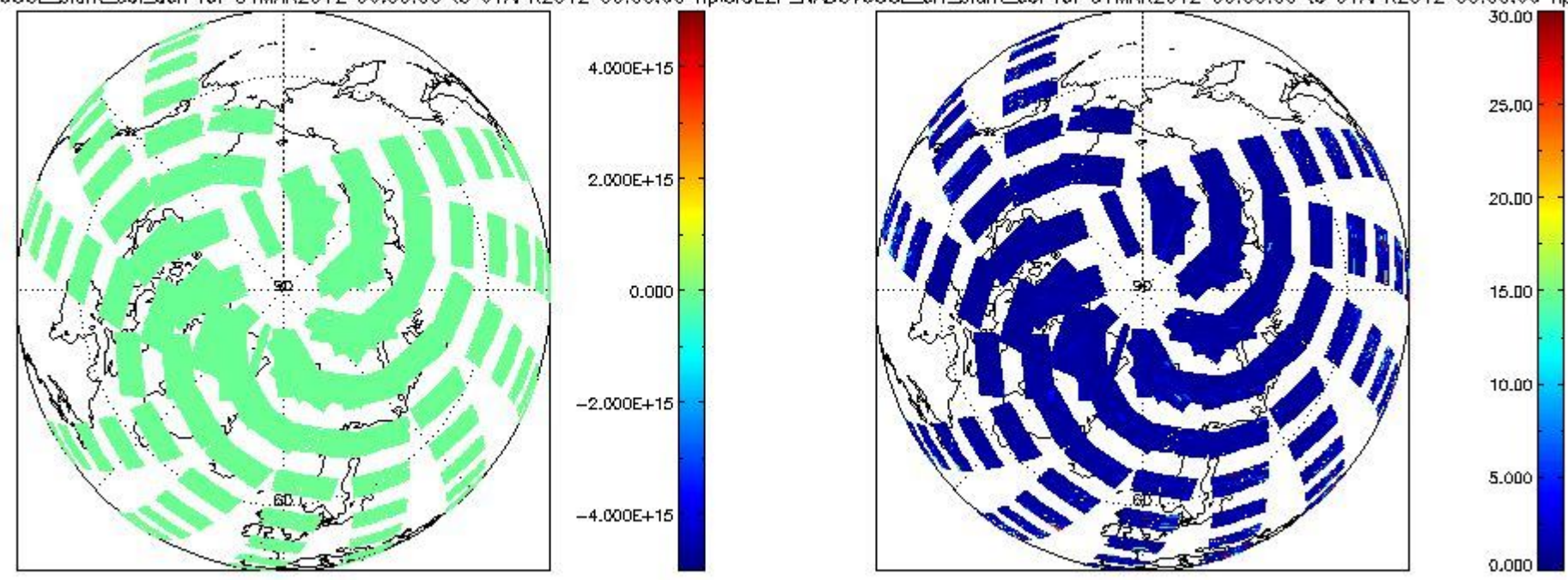
CIOL2P_NADUV6OCL_slant_col_den for 31MAR2012 00:00:00 to 01APR2012 00:00:00 np CIOL2P_NADUV6OCL_err_slant_col for 31MAR2012 00:00:00 to 01APR2012 00:00:00 np
