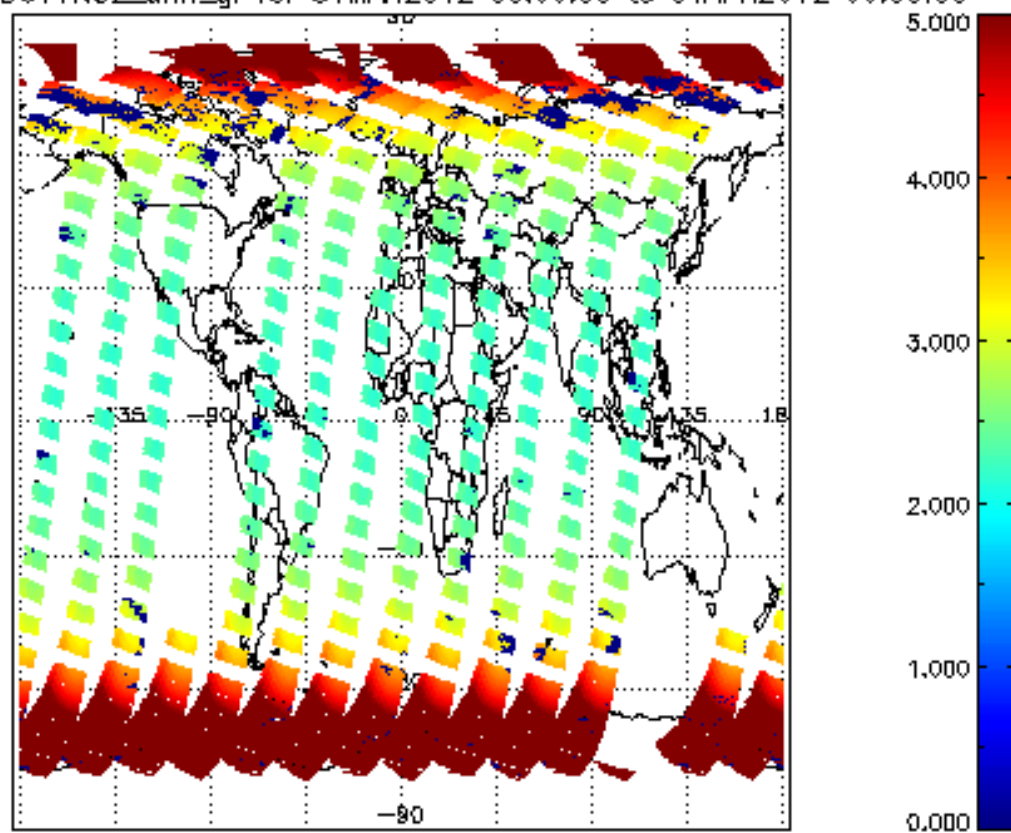
SCIOL2P_NADUV1NO2_amf_gr for 31MAR2012 00:00:00 to 01APR2012 00:00:00
