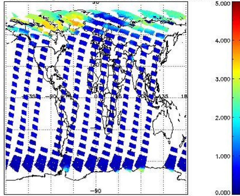
SCIOL2P_NADUV5SO2_amf_gr for 31MAR2012 00:00:00 to 01APR2012 00:00:00
