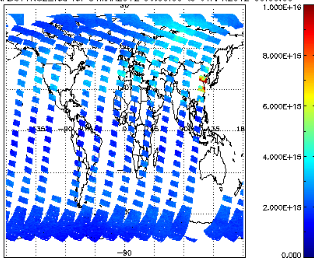
SCIOL2P_NADUV1NO2_vcd for 31MAR2012 00:00:00 to 01APR2012 00:00:00
