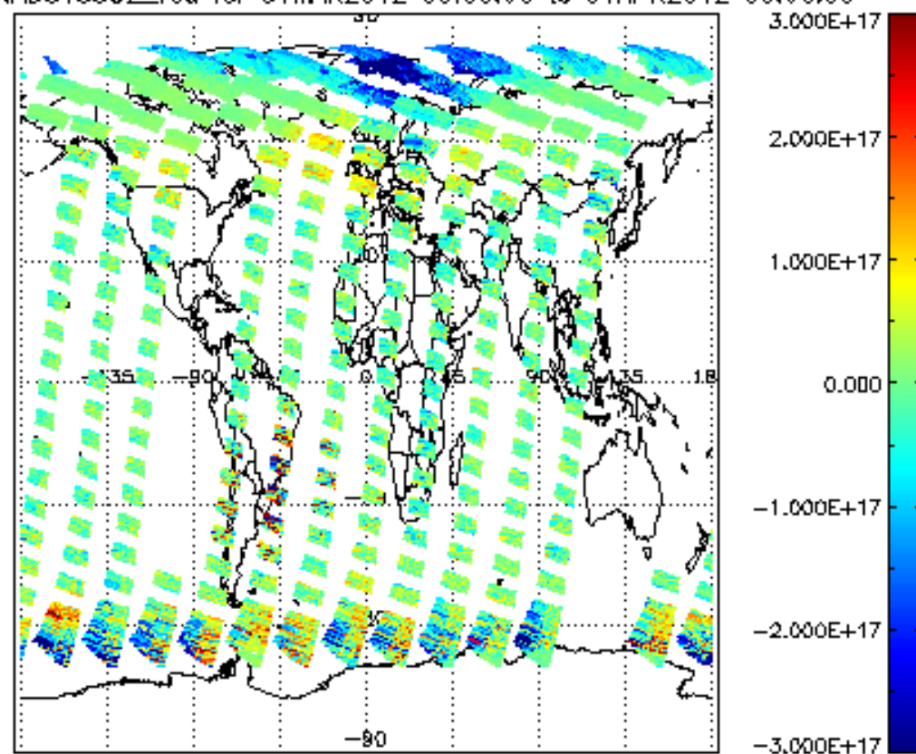
SCIOL2P_NADUV5S02_vcd for 31MAR2012 00:00:00 to 01APR2012 00:00:00
