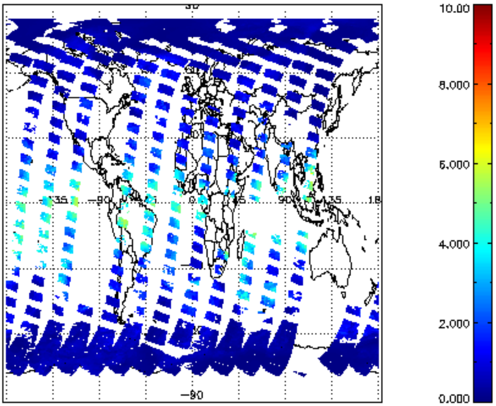
SCIOL2P_NADUV8H20_vcd for 31MAR2012 00:00:00 to 01APR2012 00:00:00
