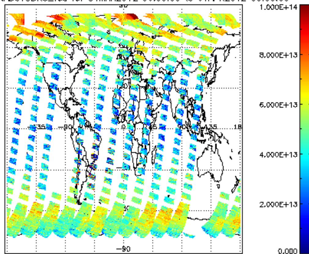
SCIOL2P_NADUV3BRO_vcd for 31MAR2012 00:00:00 to 01APR2012 00:00:00
