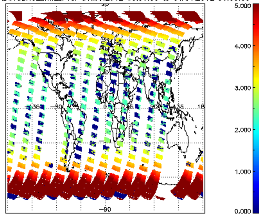
SCIOL2P_NADUV3BRO_amf_cl for 31MAR2012 00:00:00 to 01APR2012 00:00:00
