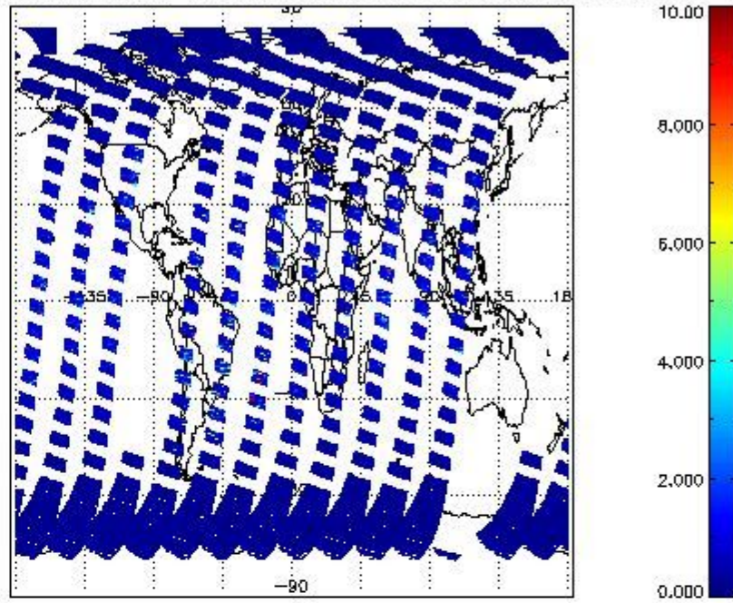
SCIOL2P_NADUV3BRO_vcd_err for 31MAR2012 00:00:00 to 01APR2012 00:00:00
