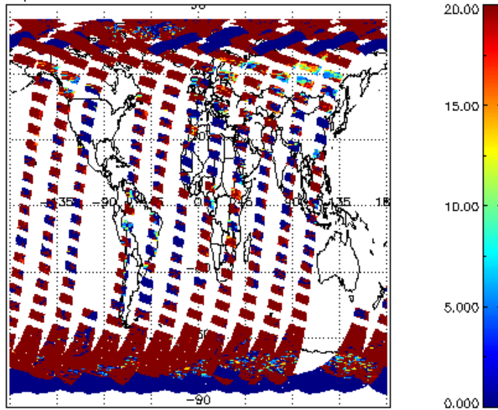
cL_opt_depth for 31MAR2012 00:00:00 to 01APR2012 00:00:00
