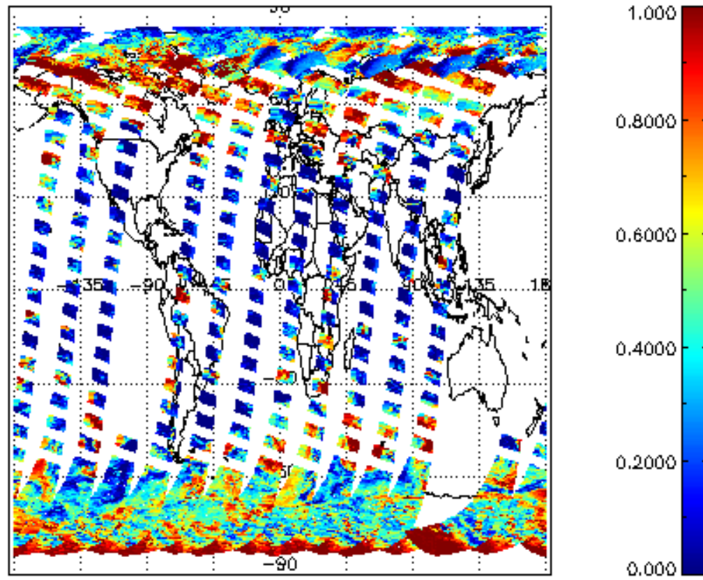
cL_frac for 31MAR2012 00:00:00 to 01APR2012 00:00:00
