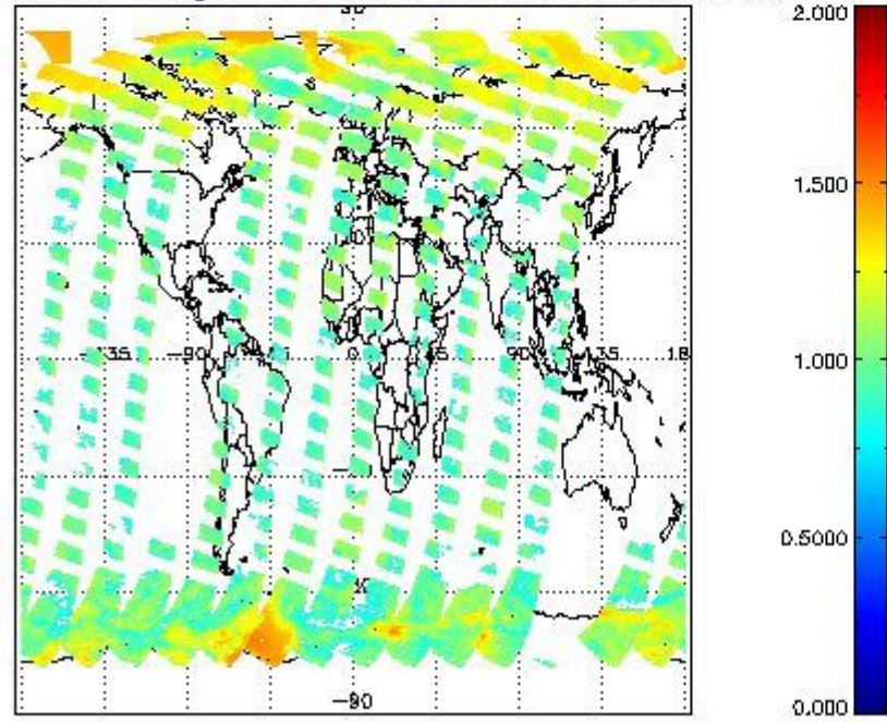
SCIOL2P_NADUV8H2O_amf_gr for 31MAR2012 00:00:00 to 01APR2012 00:00:00
