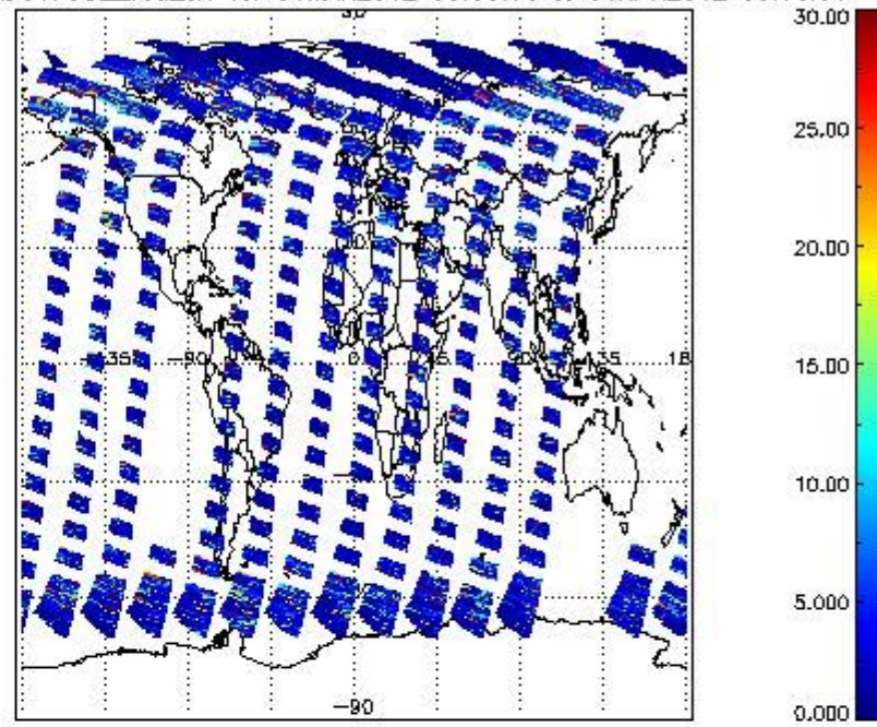
SCIOL2P_NADUV7S02_vcd_err for 31MAR2012 00:00:00 to 01APR2012 00:00:00
