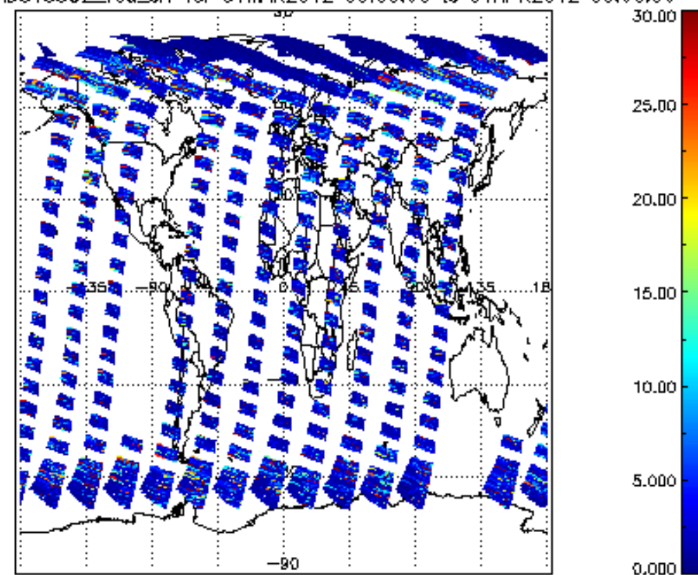
SCIOL2P_NADUV5S02_vcd_err for 31MAR2012 00:00:00 to 01APR2012 00:00:00
