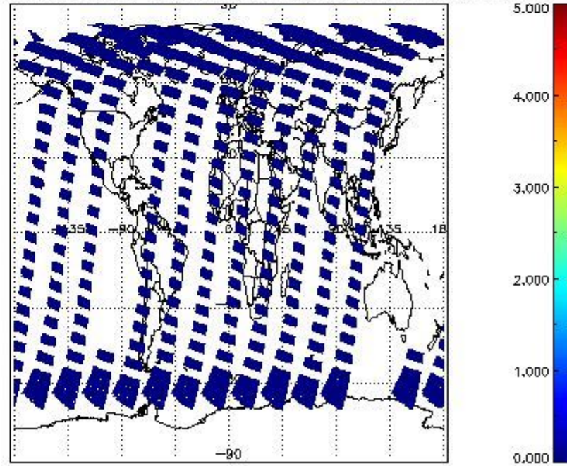
SCIOL2P_NADUV5SO2_amf_cl for 31MAR2012 00:00:00 to 01APR2012 00:00:00
