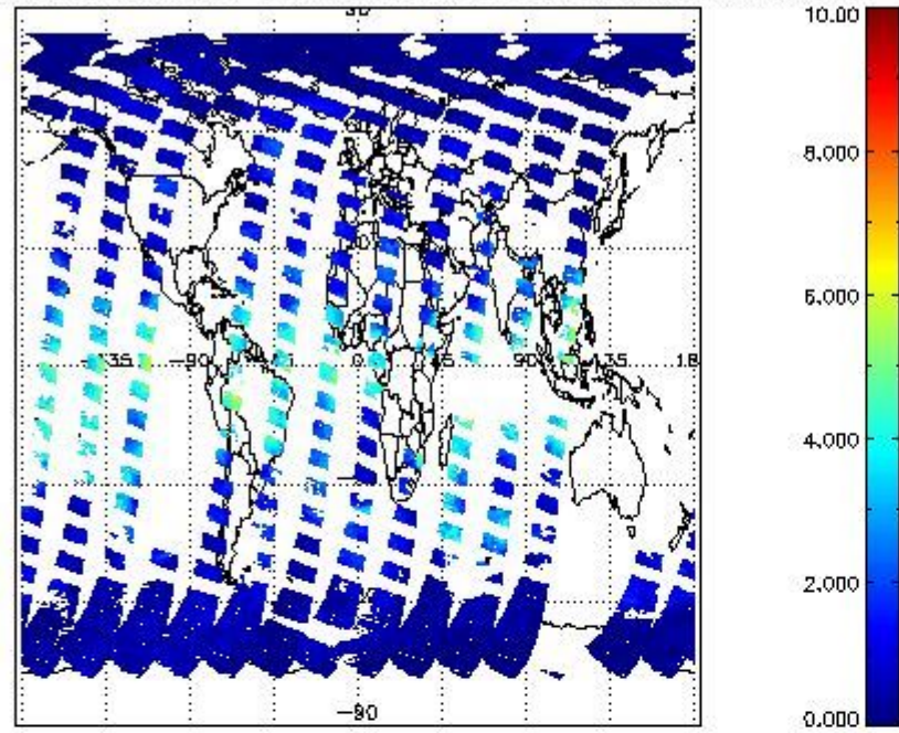
SCIOL2P_NADUVBH20_vcd for 31MAR2012 00:00:00 to 01APR2012 00:00:00
