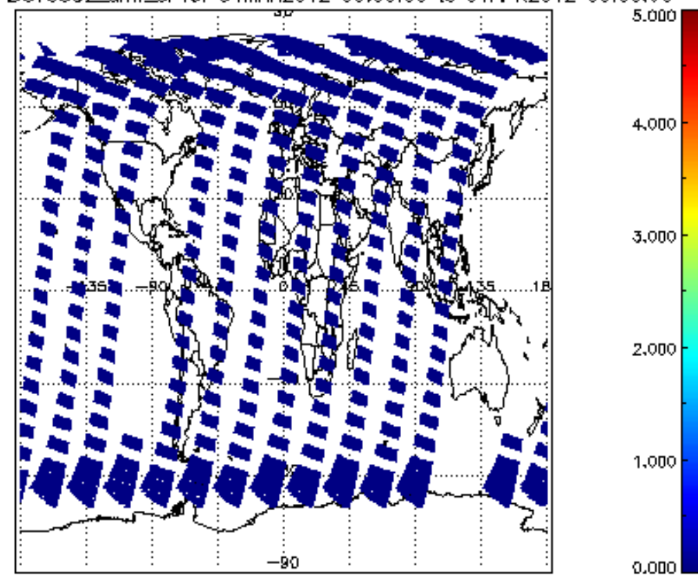
SCIOL2P_NADUV5S02_amf_cl for 31MAR2012 00:00:00 to 01APR2012 00:00:00
