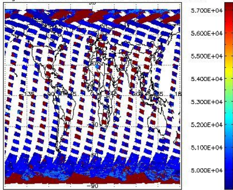
cloud_flags for 25MAR2012 00:00:00 to 26MAR2012 00:00:00
