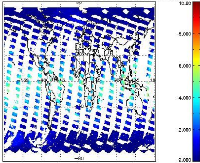
SCIOL2P_NADUV8H2O_vcd for 25MAR2012 00:00:00 to 26MAR2012 00:00:00
