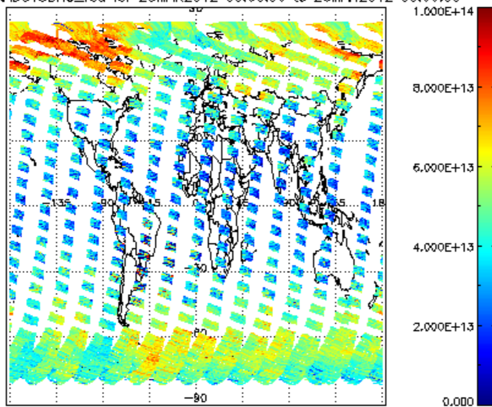
SCIOL2P_NADUV3BRO_vcd for 25MAR2012 00:00:00 to 26MAR2012 00:00:00
