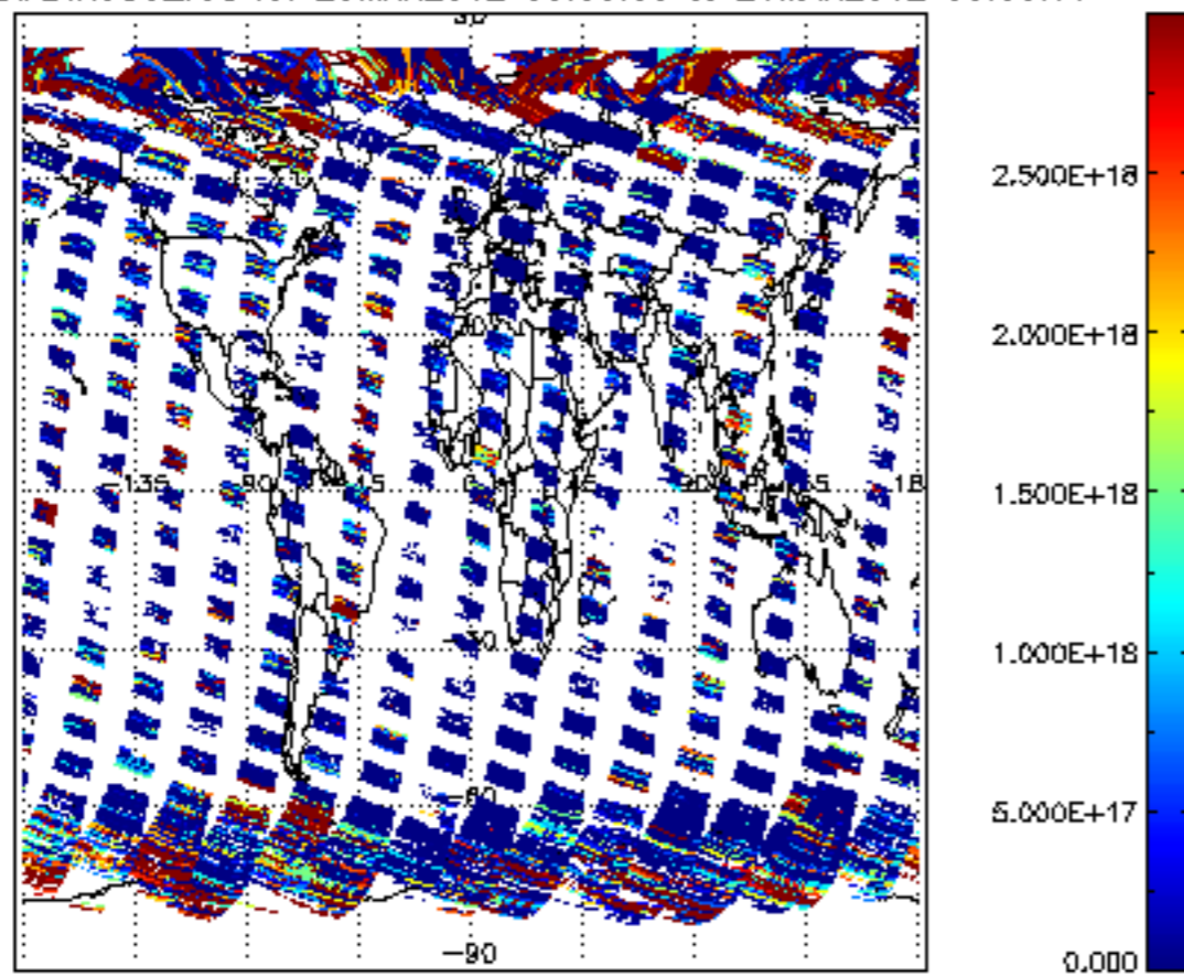
SCIOL2P_NADIR3CO_vcd for 25MAR2012 00:00:00 to 26MAR2012 00:00:00
