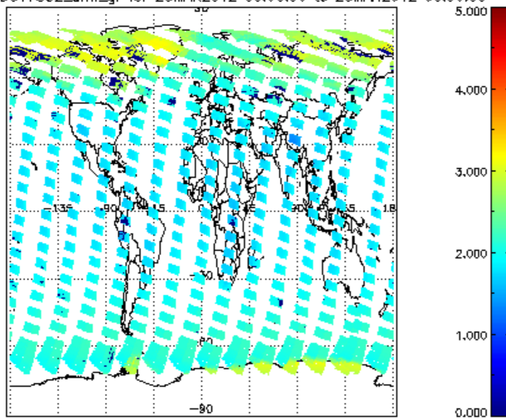
SCIOL2P_NADUV7S02_amf_gr for 25MAR2012 00:00:00 to 26MAR2012 00:00:00
