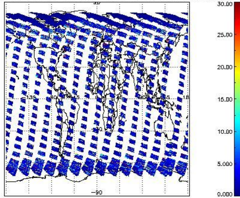
SCIOL2P_NADUV5SO2_vcd_err for 25MAR2012 00:00:00 to 26MAR2012 00:00:00
