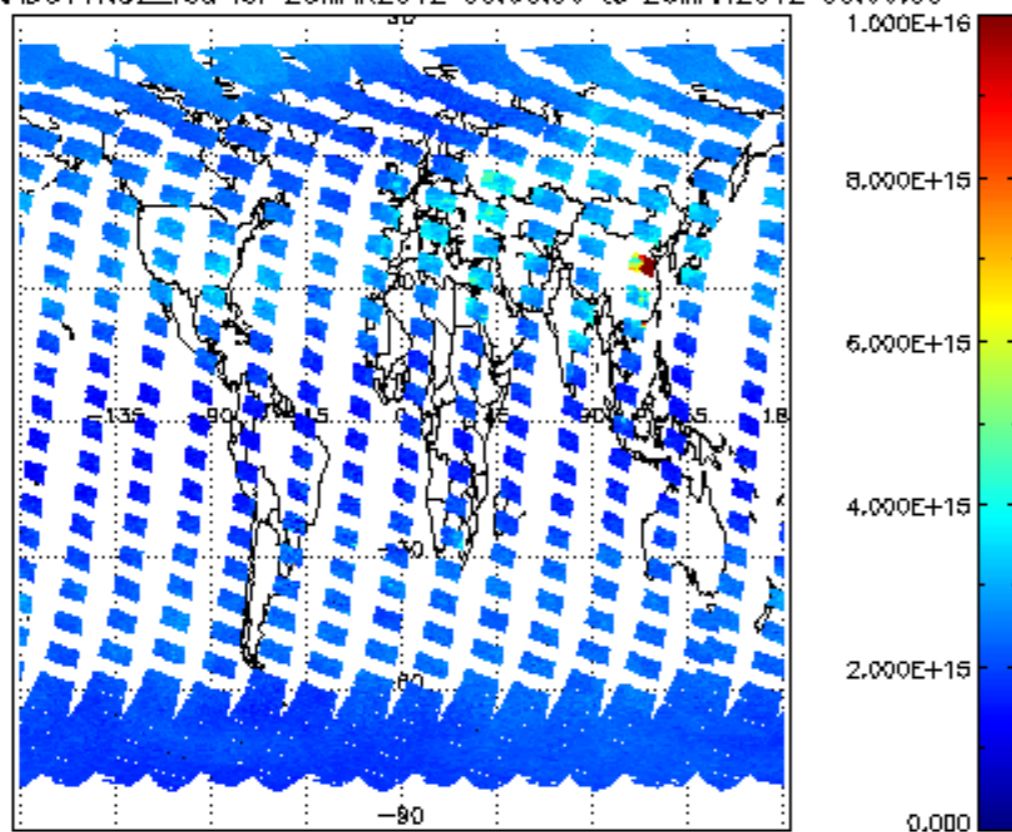
SCIOL2P_NADUV1NO2_vcd for 25MAR2012 00:00:00 to 26MAR2012 00:00:00
