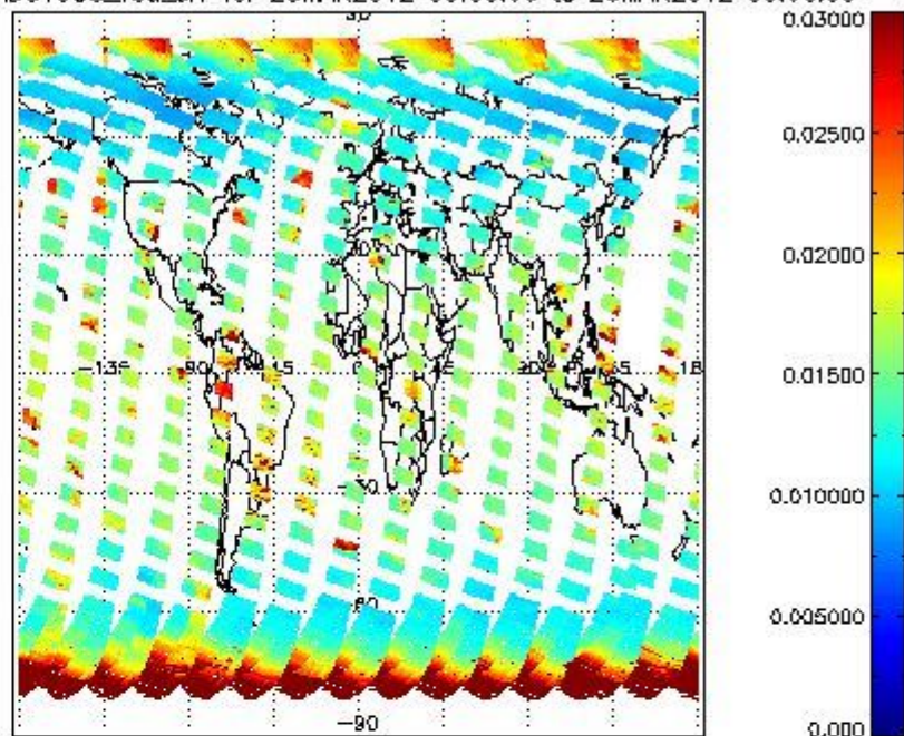
SCIOL2P_NADUV003_vcd_err for 25MAR2012 00:00:00 to 26MAR2012 00:00:00
