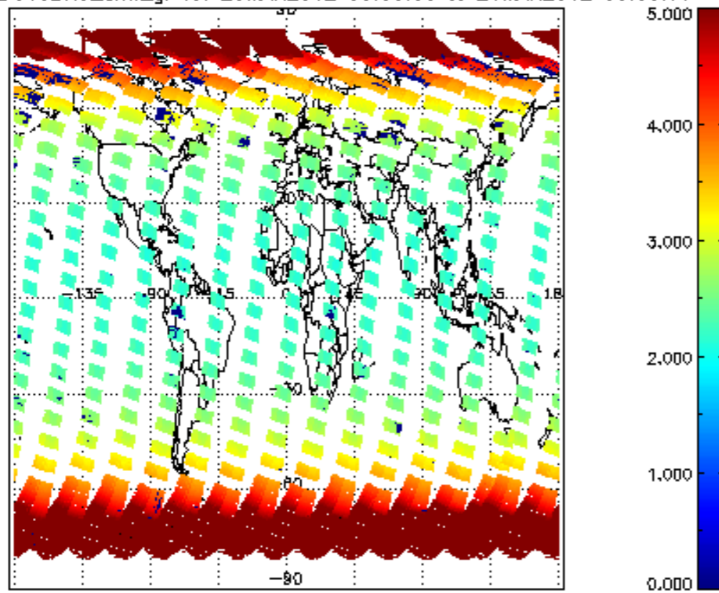
SCIOL2P_NADUV3BRO_amf_gr for 25MAR2012 00:00:00 to 26MAR2012 00:00:00
