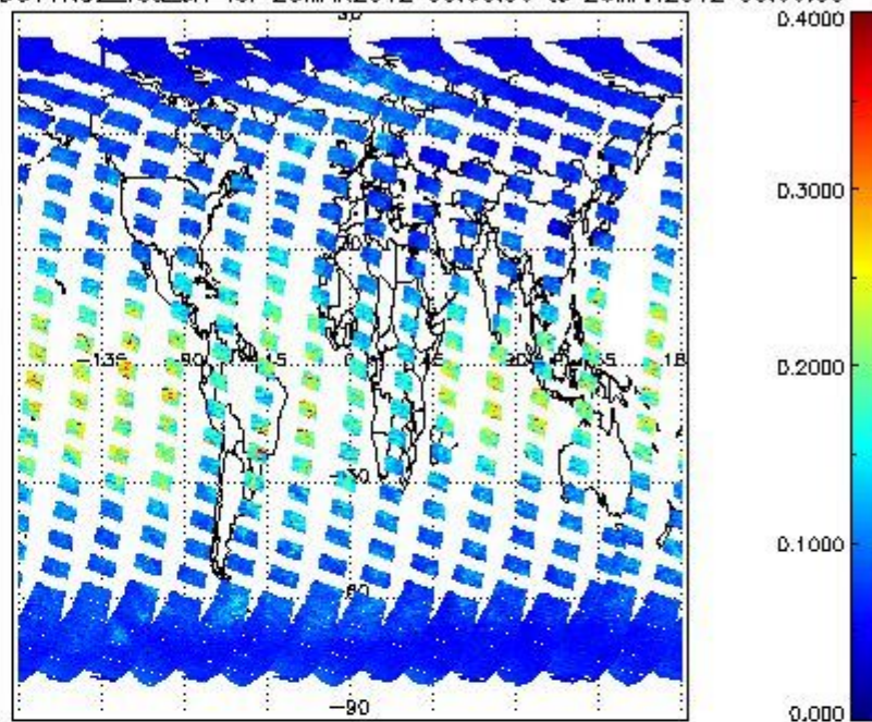
SCIOL2P_NADUV1NO2_vcd_err for 25MAR2012 00:00:00 to 26MAR2012 00:00:00
