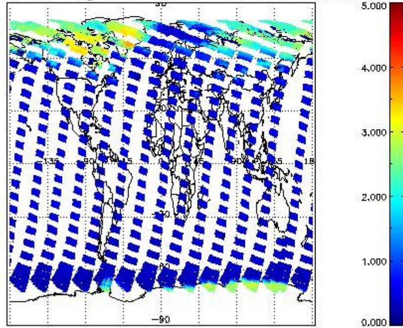
SCIOL2P_NADUV5SO2_amf_gr for 25MAR2012 00:00:00 to 26MAR2012 00:00:00
