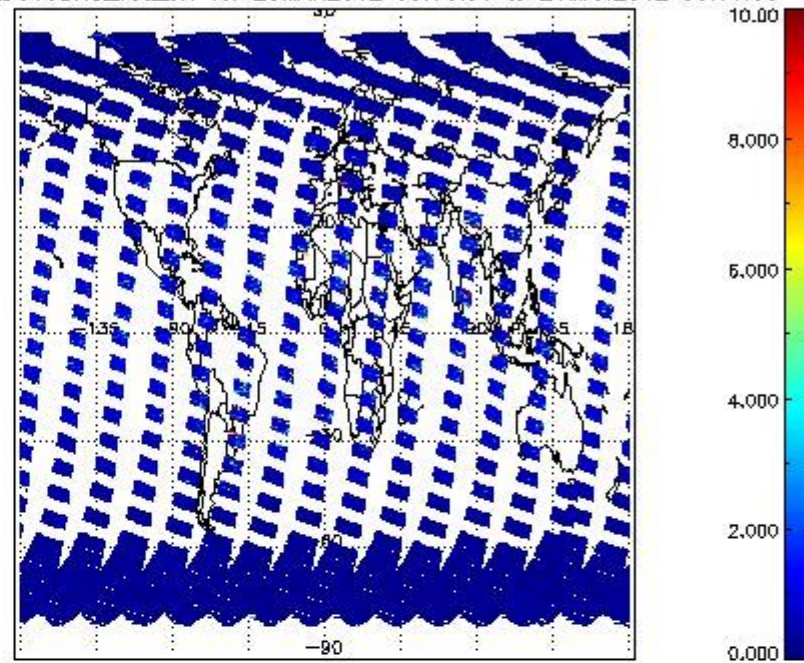
SCIOL2P_NADUV3BRO_vcd_err for 25MAR2012 00:00:00 to 26MAR2012 00:00:00
