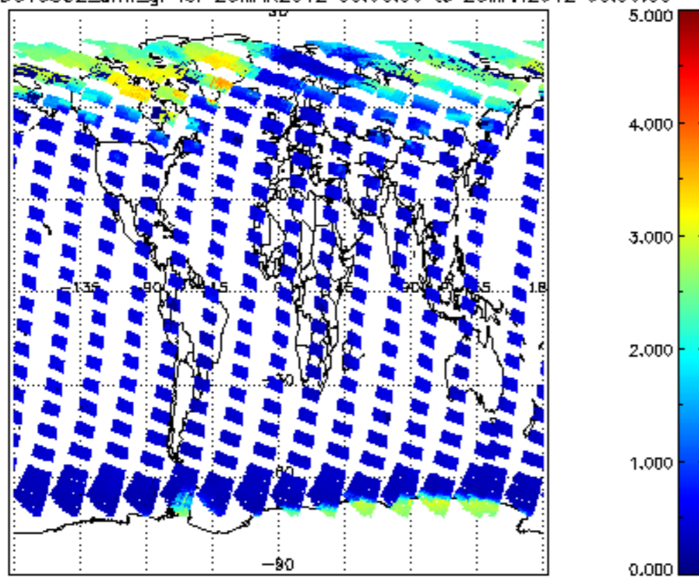
SCIOL2P_NADUV5S02_amf_gr for 25MAR2012 00:00:00 to 26MAR2012 00:00:00
