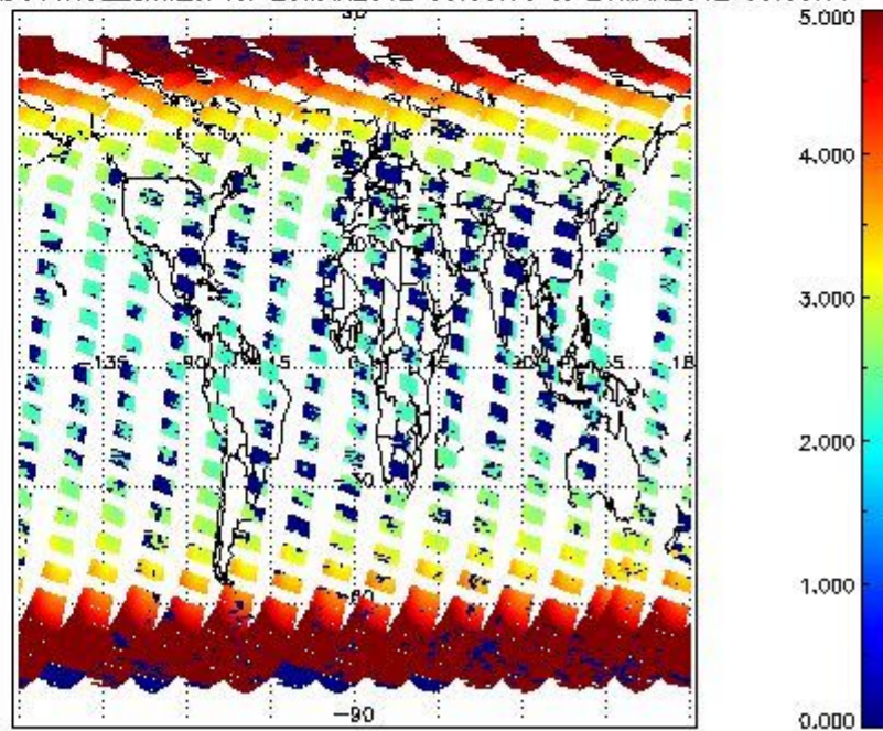
SCIOL2P_NADUV1NO2_amf_cl for 25MAR2012 00:00:00 to 26MAR2012 00:00:00
