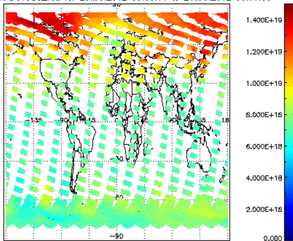
SCIOL2P_NADUV003_vcd for 25MAR2012 00:00:00 to 26MAR2012 00:00:00
