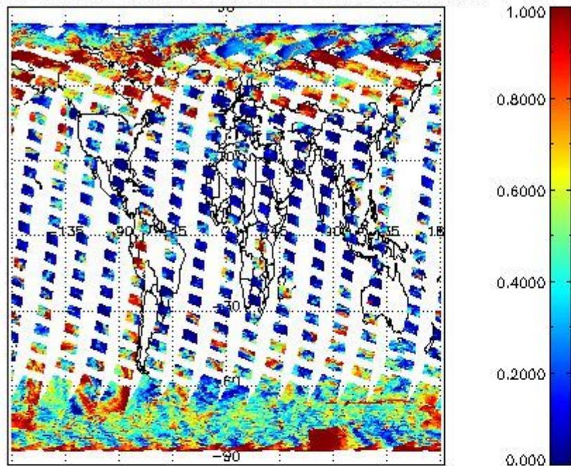
cL_frac for 25MAR2012 00:00:00 to 26MAR2012 00:00:00
