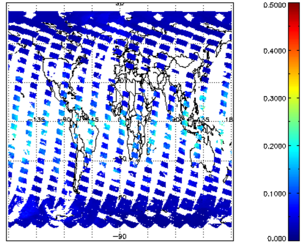
SCIOL2P_NADUV8H2O_vcd_err for 25MAR2012 00:00:00 to 26MAR2012 00:00:00
