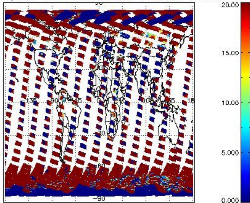
cL_opt_depth for 25MAR2012 00:00:00 to 26MAR2012 00:00:00
