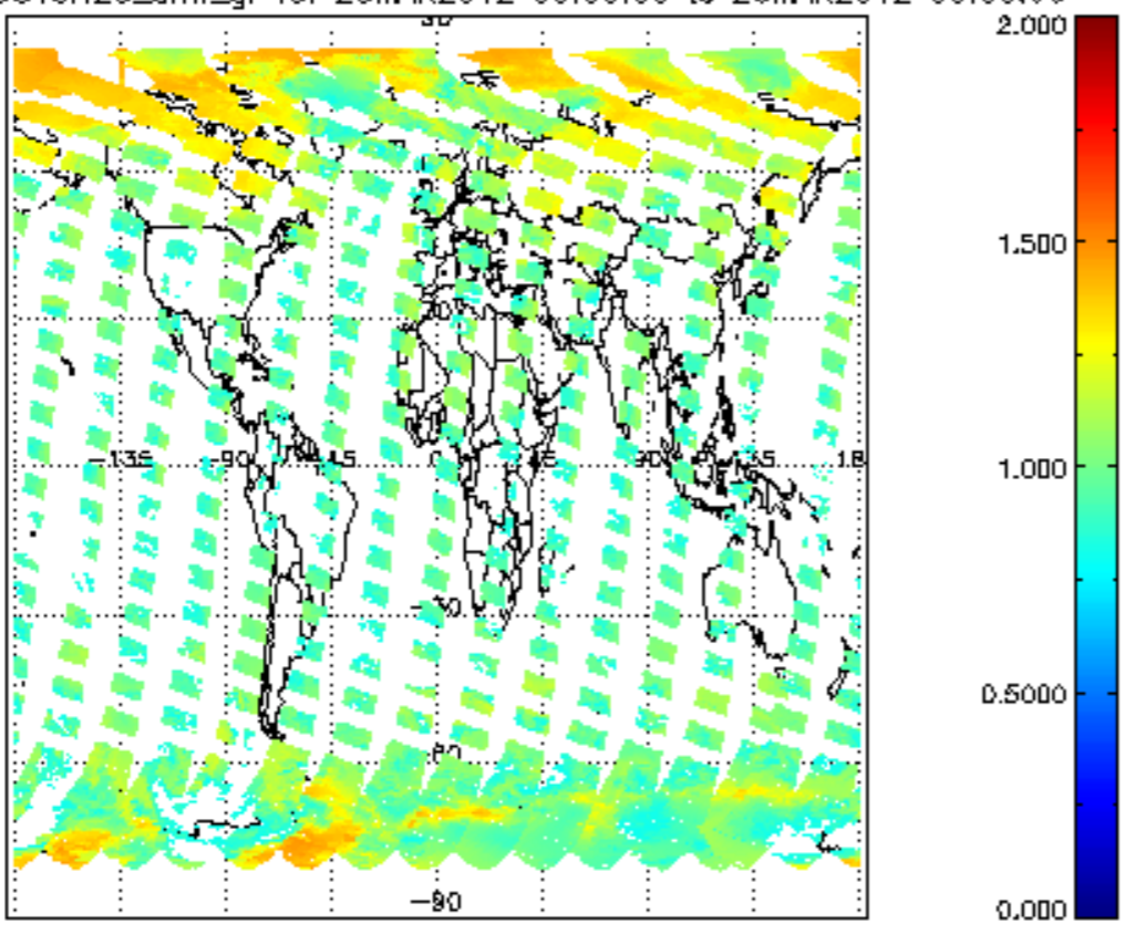
SCIOL2P_NADUV8H2O_arnf_gr for 25MAR2012 00:00:00 to 26MAR2012 00:00:00
