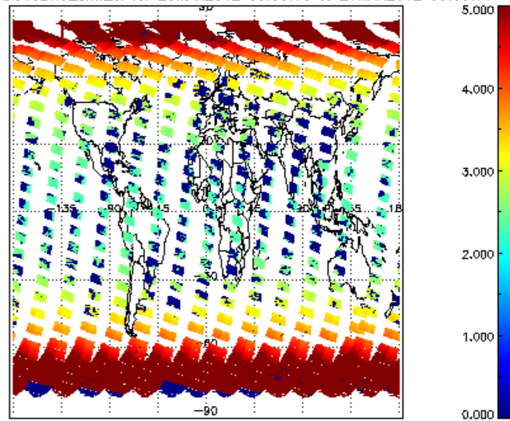
SCIOL2P_NADUV3BRO_amf_cl for 25MAR2012 00:00:00 to 26MAR2012 00:00:00
