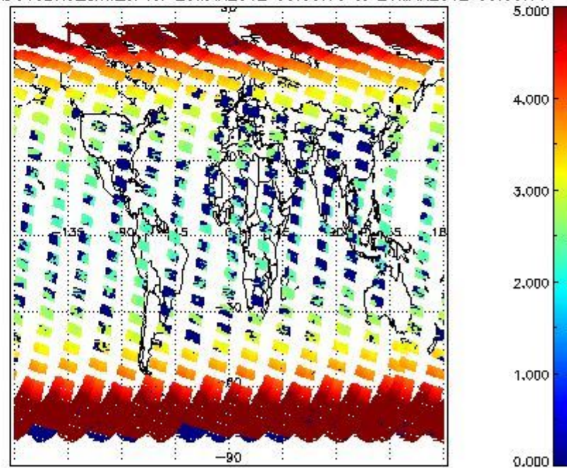
SCIOL2P_NADUV3BRO_amf_cl for 25MAR2012 00:00:00 to 26MAR2012 00:00:00
