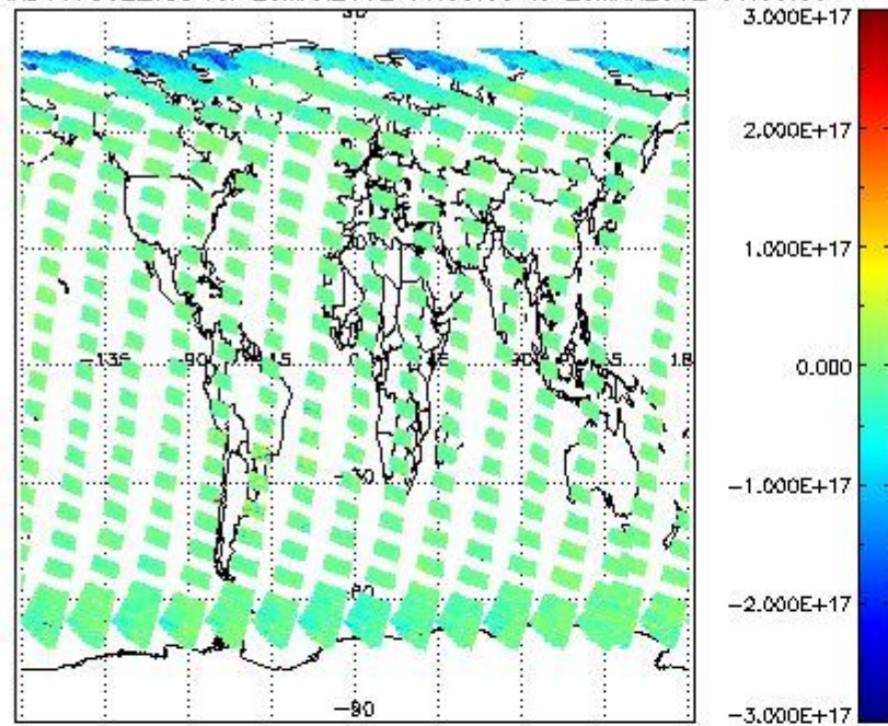
SCIOL2P_NADUV7S02_vcd for 25MAR2012 00:00:00 to 26MAR2012 00:00:00
