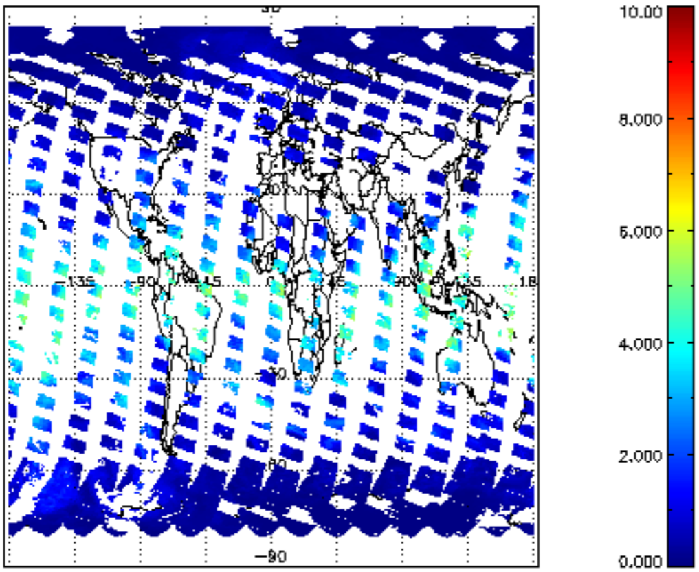
SCIOL2P_NADUV8H2O_vcd for 25MAR2012 00:00:00 to 26MAR2012 00:00:00
