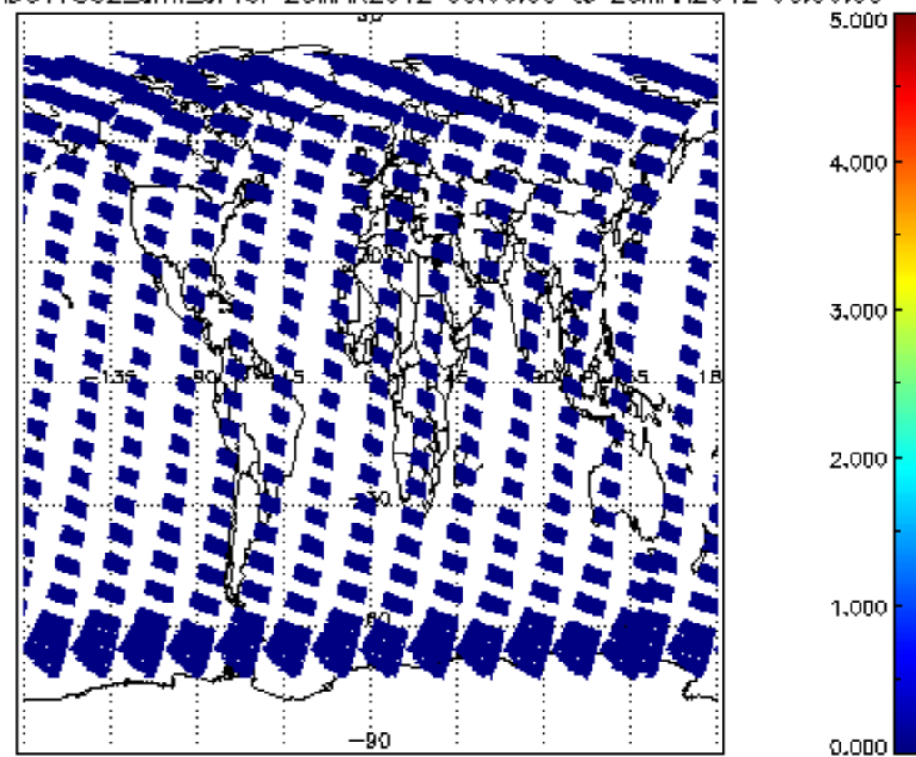
SCIOL2P_NADUV7S02_amf_cl for 25MAR2012 00:00:00 to 26MAR2012 00:00:00
