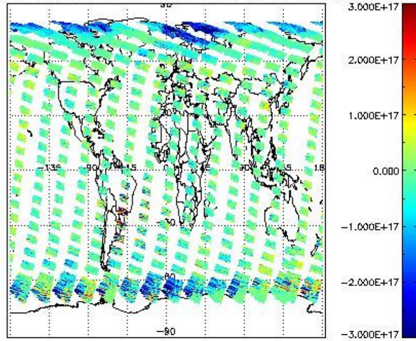
SCIOL2P_NADUV5SO2_vcd for 25MAR2012 00:00:00 to 26MAR2012 00:00:00
