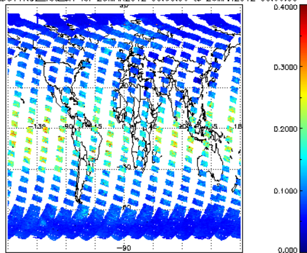
SCIOL2P_NADUV1NO2_vcd_err for 25MAR2012 00:00:00 to 26MAR2012 00:00:00
