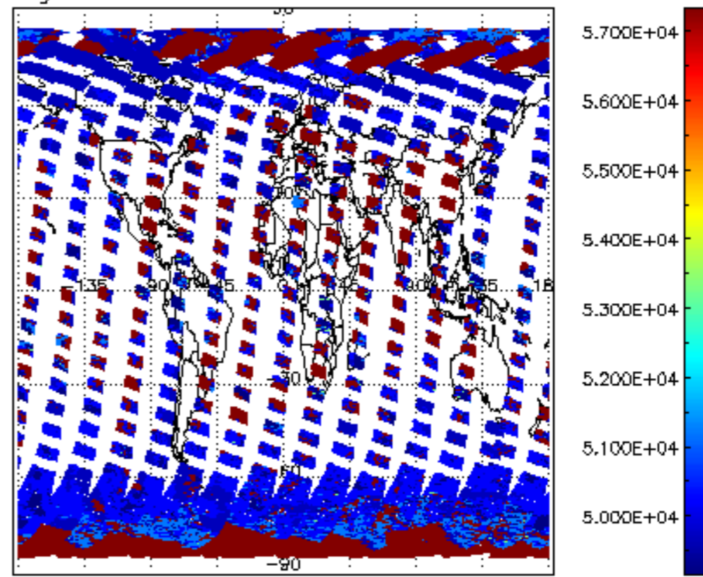
cloud_flags for 25MAR2012 00:00:00 to 26MAR2012 00:00:00
