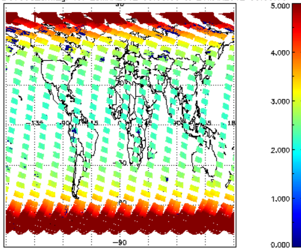
SCIOL2P_NADUV003_arnf_gr for 25MAR2012 00:00:00 to 26MAR2012 00:00:00
