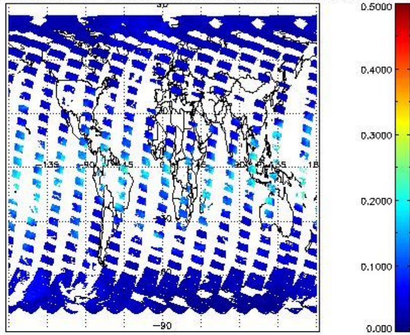
SCIOL2P_NADUV8H2O_vcd_err for 25MAR2012 00:00:00 to 26MAR2012 00:00:00
