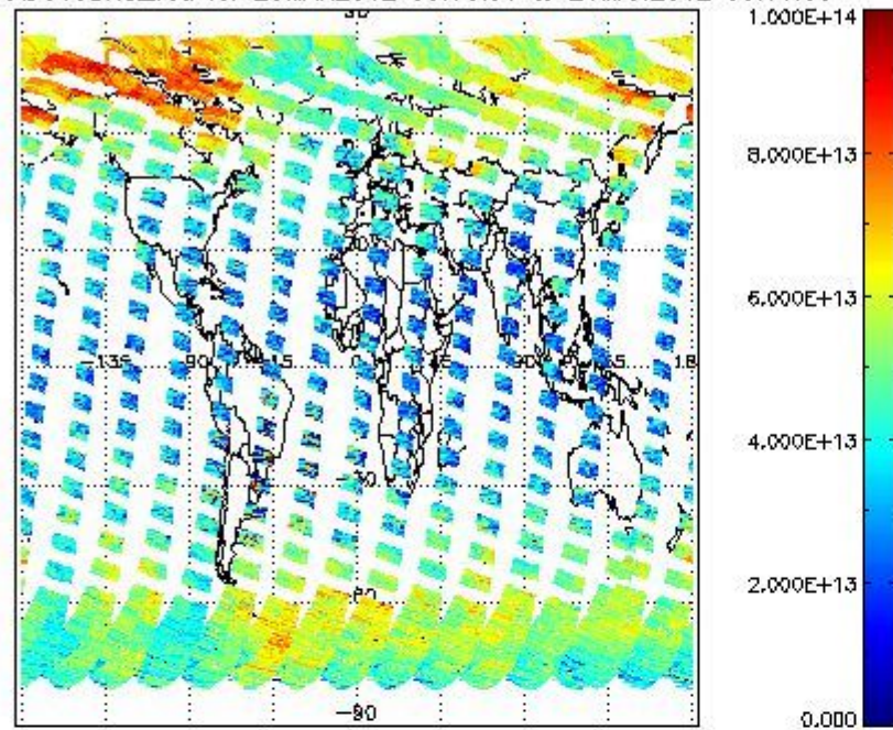
SCIOL2P_NADUV3BRO_vcd for 25MAR2012 00:00:00 to 26MAR2012 00:00:00
