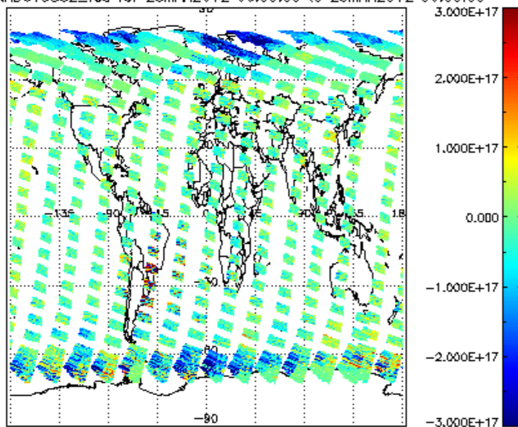
SCIOL2P_NADUV5S02_vcd for 25MAR2012 00:00:00 to 26MAR2012 00:00:00
