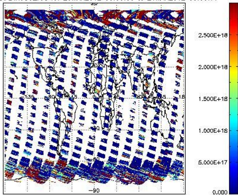
SCIOL2P_NADIR3CO_vcd for 25MAR2012 00:00:00 to 26MAR2012 00:00:00
