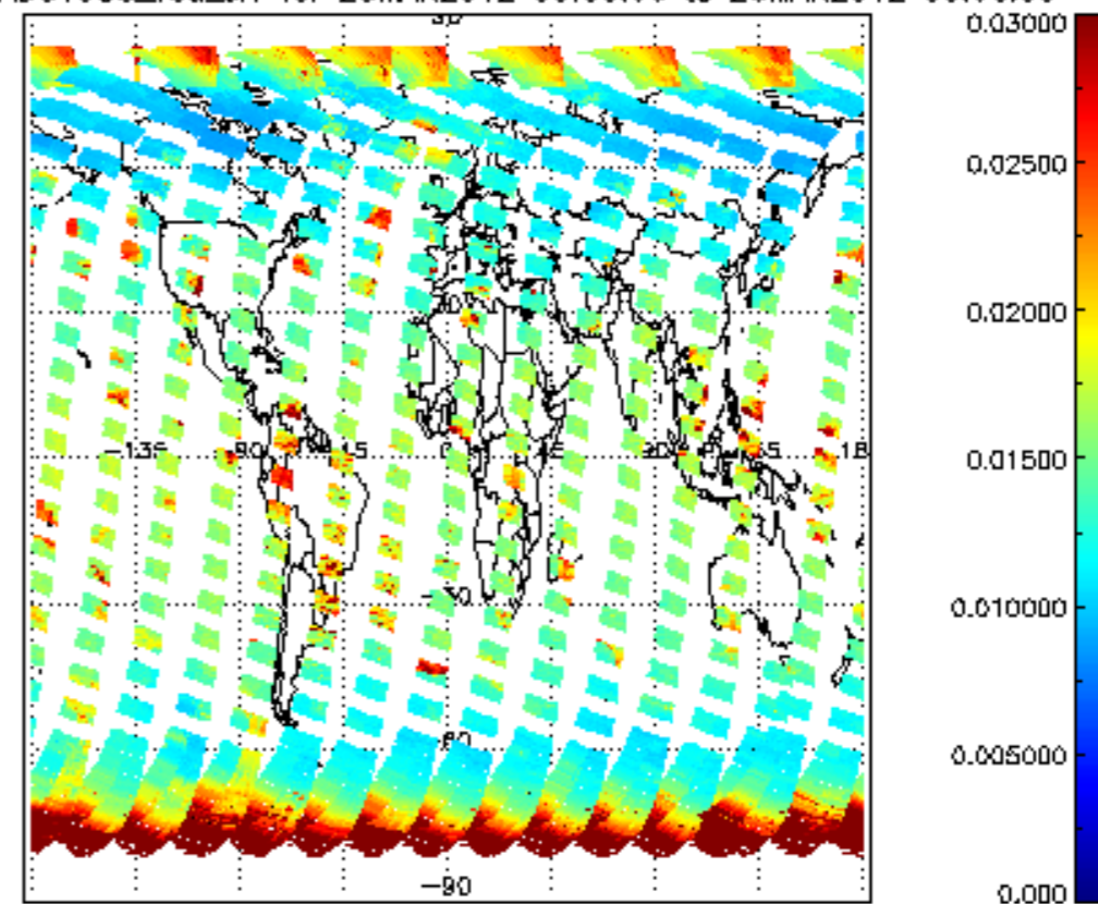
SCIOL2P_NADUV003_vcd_err for 25MAR2012 00:00:00 to 26MAR2012 00:00:00
