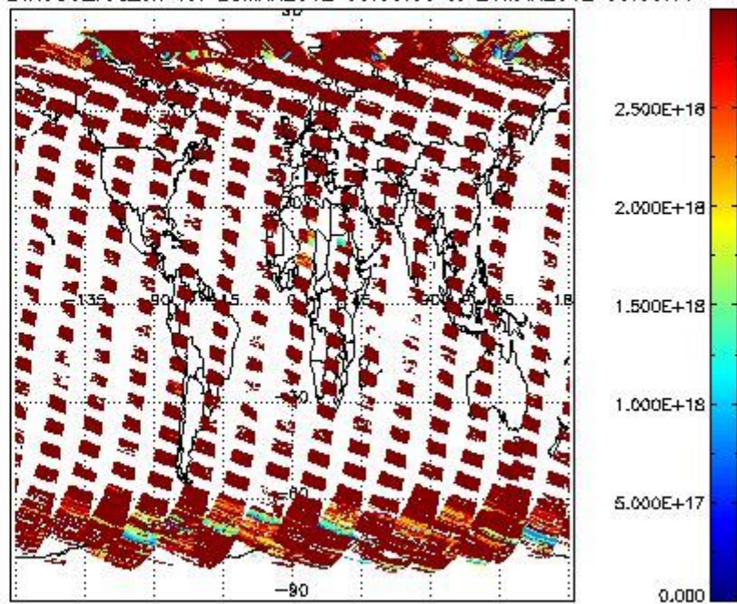
SCIOL2P_NADIR3CO_vcd_err for 25MAR2012 00:00:00 to 26MAR2012 00:00:00
