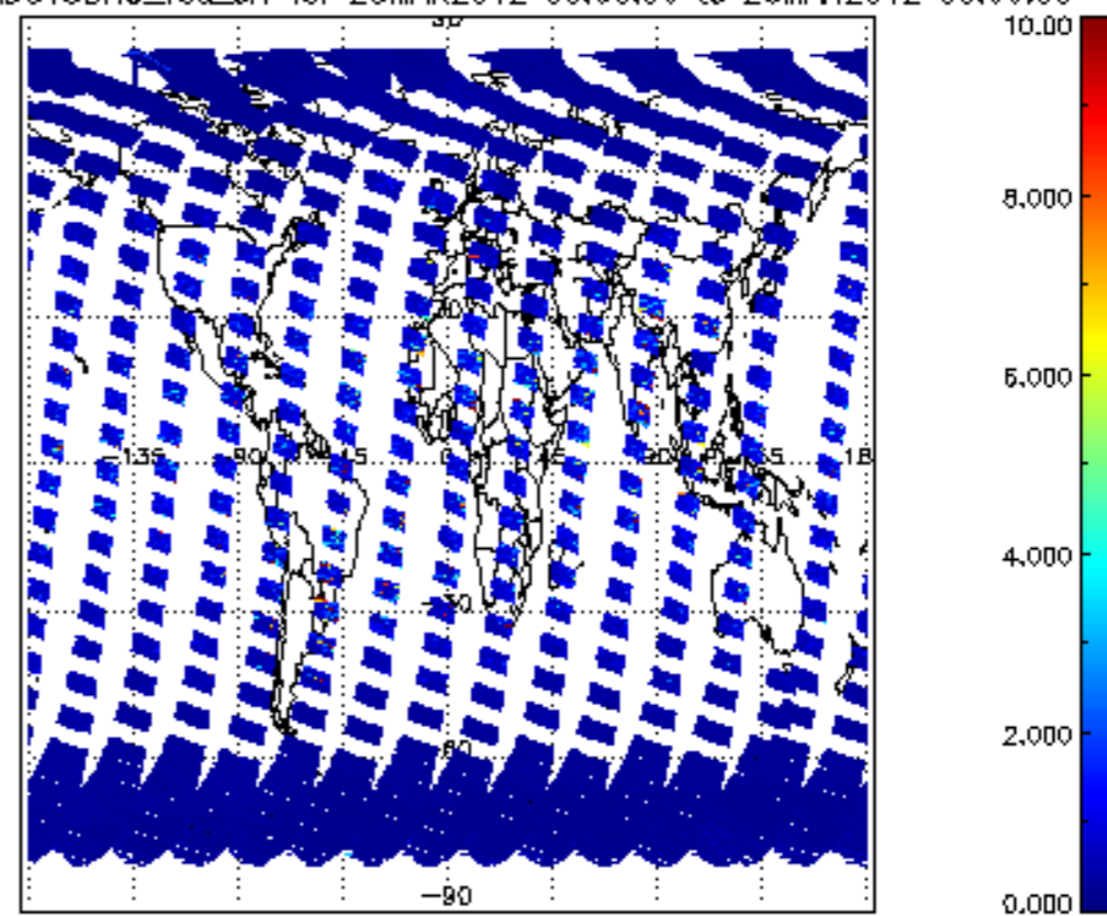
SCIOL2P_NADUV3BRO_vcd_err for 25MAR2012 00:00:00 to 26MAR2012 00:00:00
