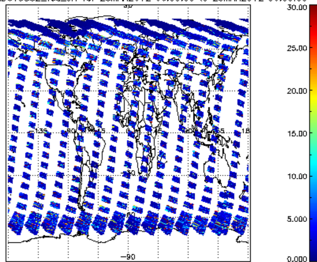
SCIOL2P_NADUV5S02_vcd_err for 25MAR2012 00:00:00 to 26MAR2012 00:00:00
