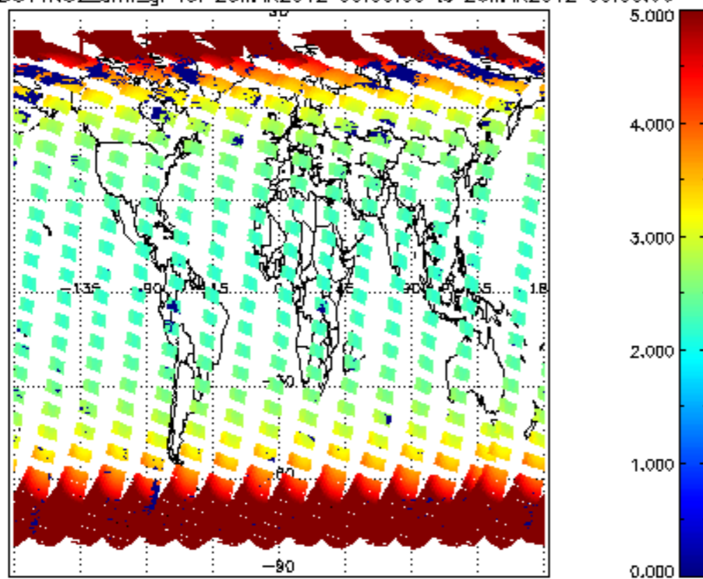
SCIOL2P_NADUV1NO2_amf_gr for 25MAR2012 00:00:00 to 26MAR2012 00:00:00
