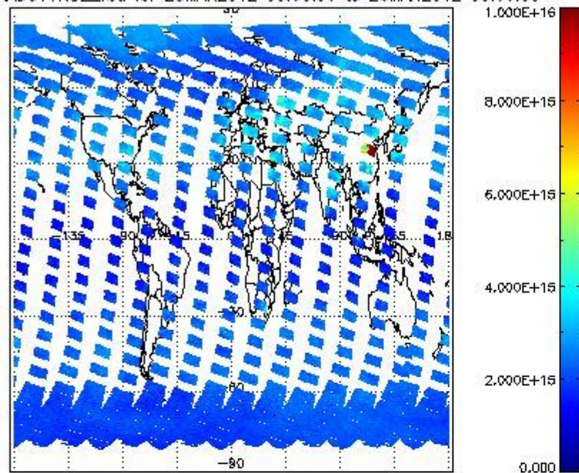
SCIOL2P_NADUV1NO2_vcd for 25MAR2012 00:00:00 to 26MAR2012 00:00:00
