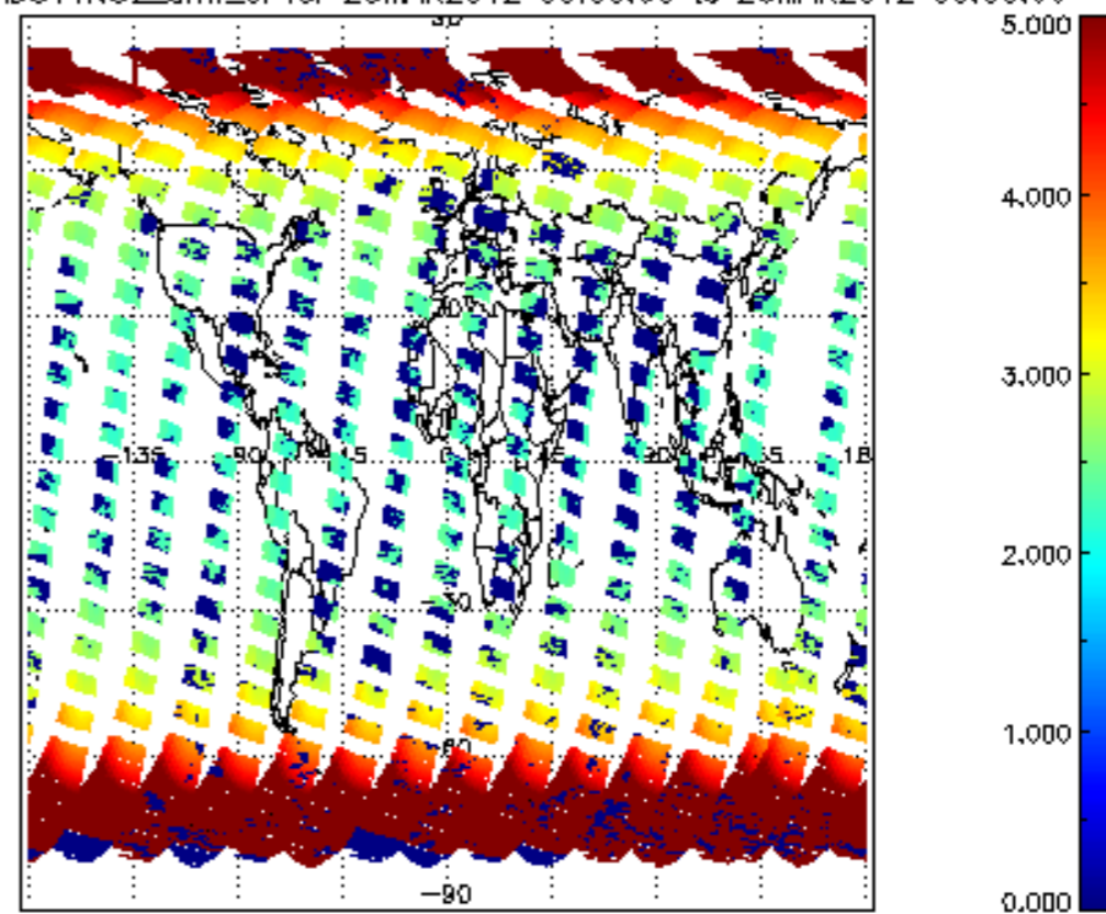
SCIOL2P_NADUV1NO2_amf_cl for 25MAR2012 00:00:00 to 26MAR2012 00:00:00
