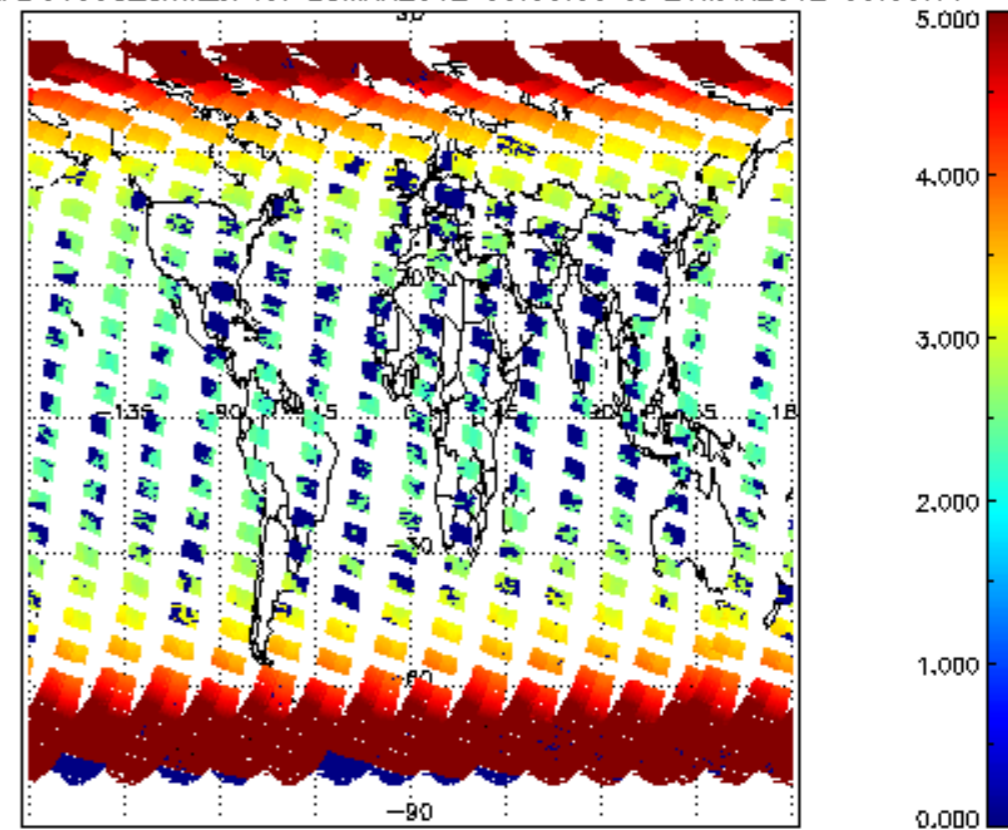
SCIOL2P_NADUV003_arnf_cl for 25MAR2012 00:00:00 to 26MAR2012 00:00:00
