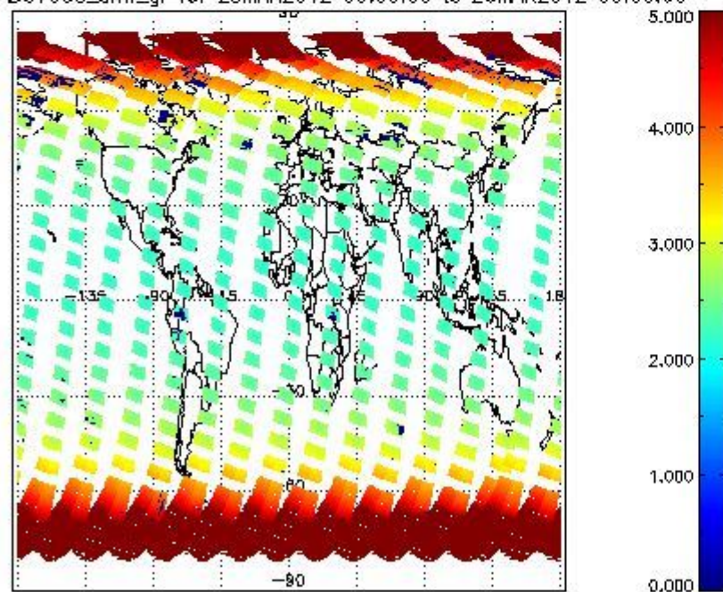
SCIOL2P_NADUV003_amf_gr for 25MAR2012 00:00:00 to 26MAR2012 00:00:00
