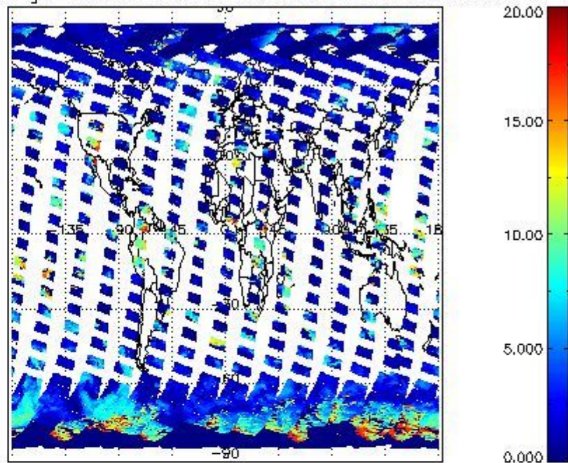
cL_top_height for 25MAR2012 00:00:00 to 26MAR2012 00:00:00
