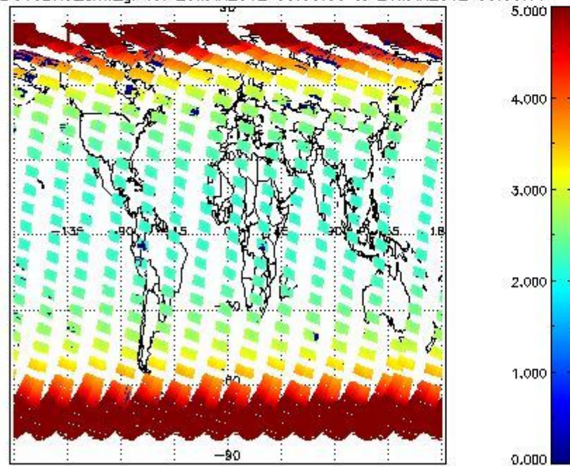
SCIOL2P_NADUV3BRO_amf_gr for 25MAR2012 00:00:00 to 26MAR2012 00:00:00
