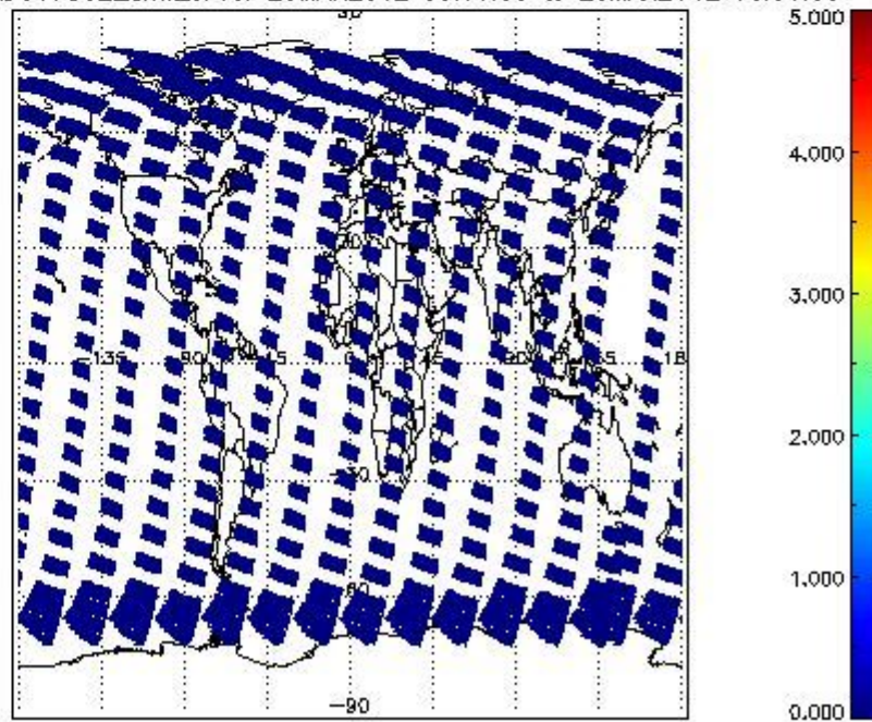
SCIOL2P_NADUV7S02_amf_cl for 25MAR2012 00:00:00 to 26MAR2012 00:00:00
