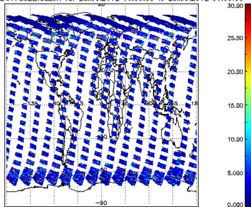
SCIOL2P_NADUV7S02_vcd_err for 25MAR2012 00:00:00 to 26MAR2012 00:00:00
