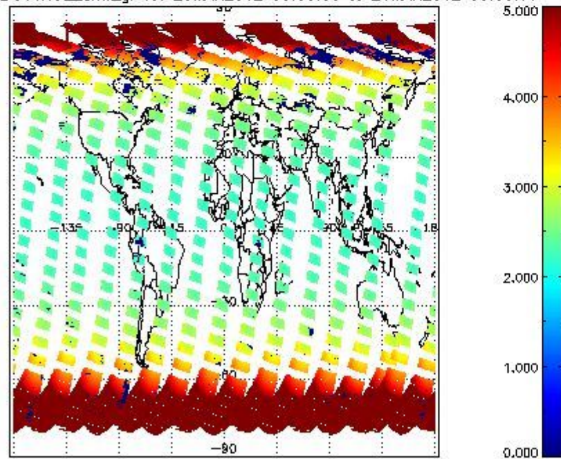
SCIOL2P_NADUV1NO2_amf_gr for 25MAR2012 00:00:00 to 26MAR2012 00:00:00
