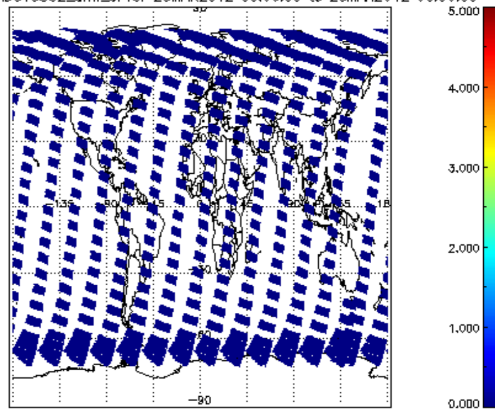
SCIOL2P_NADUV5S02_amf_cl for 25MAR2012 00:00:00 to 26MAR2012 00:00:00
