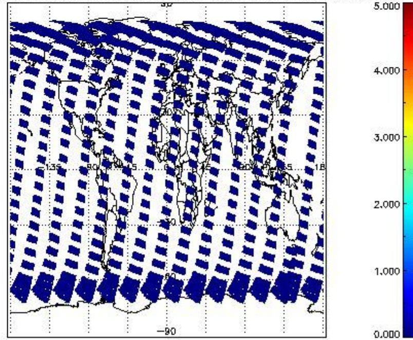
SCIOL2P_NADUV5SO2_amf_cl for 25MAR2012 00:00:00 to 26MAR2012 00:00:00
