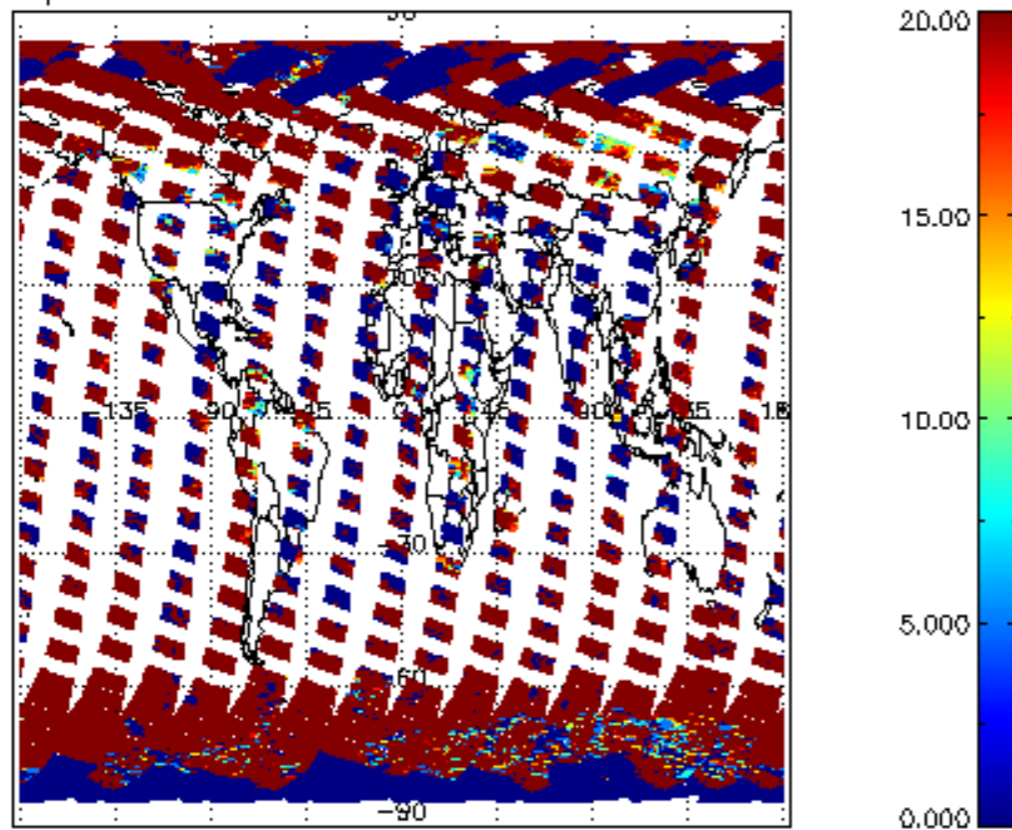
cL_opt_depth for 25MAR2012 00:00:00 to 26MAR2012 00:00:00
