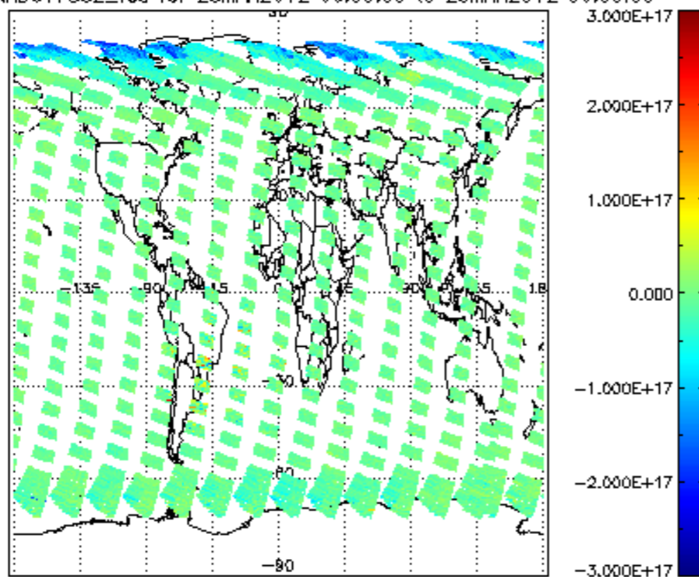
SCIOL2P_NADUV7S02_vcd for 25MAR2012 00:00:00 to 26MAR2012 00:00:00
