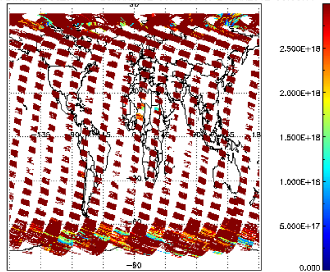
SCIOL2P_NADIR3CO_vcd_err for 25MAR2012 00:00:00 to 26MAR2012 00:00:00
