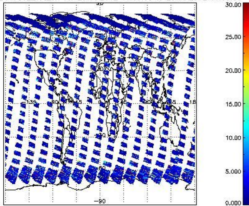
SCIOL2P_NADUV7S02_vcd_err for 25MAR2012 00:00:00 to 26MAR2012 00:00:00
