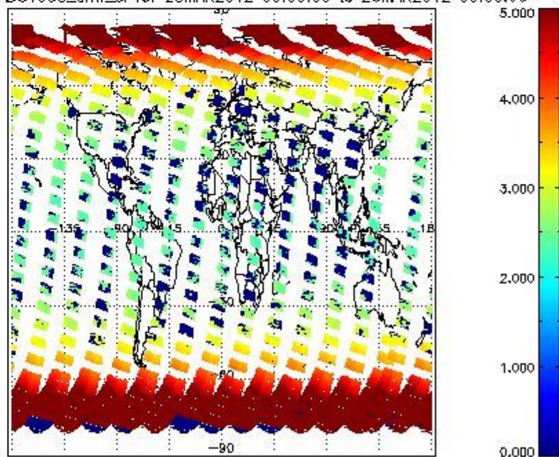
SCIOL2P_NADUV003_amf_cl for 25MAR2012 00:00:00 to 26MAR2012 00:00:00
