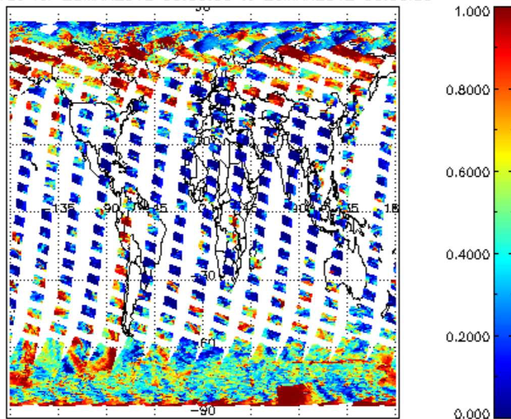
cL_frac for 25MAR2012 00:00:00 to 26MAR2012 00:00:00
