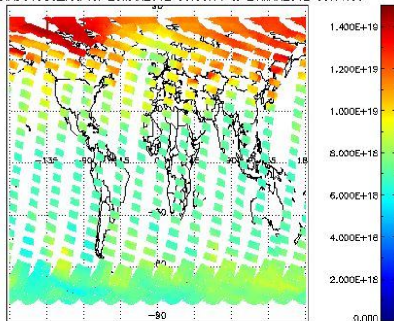
SCIOL2P_NADUV003_vcd for 25MAR2012 00:00:00 to 26MAR2012 00:00:00
