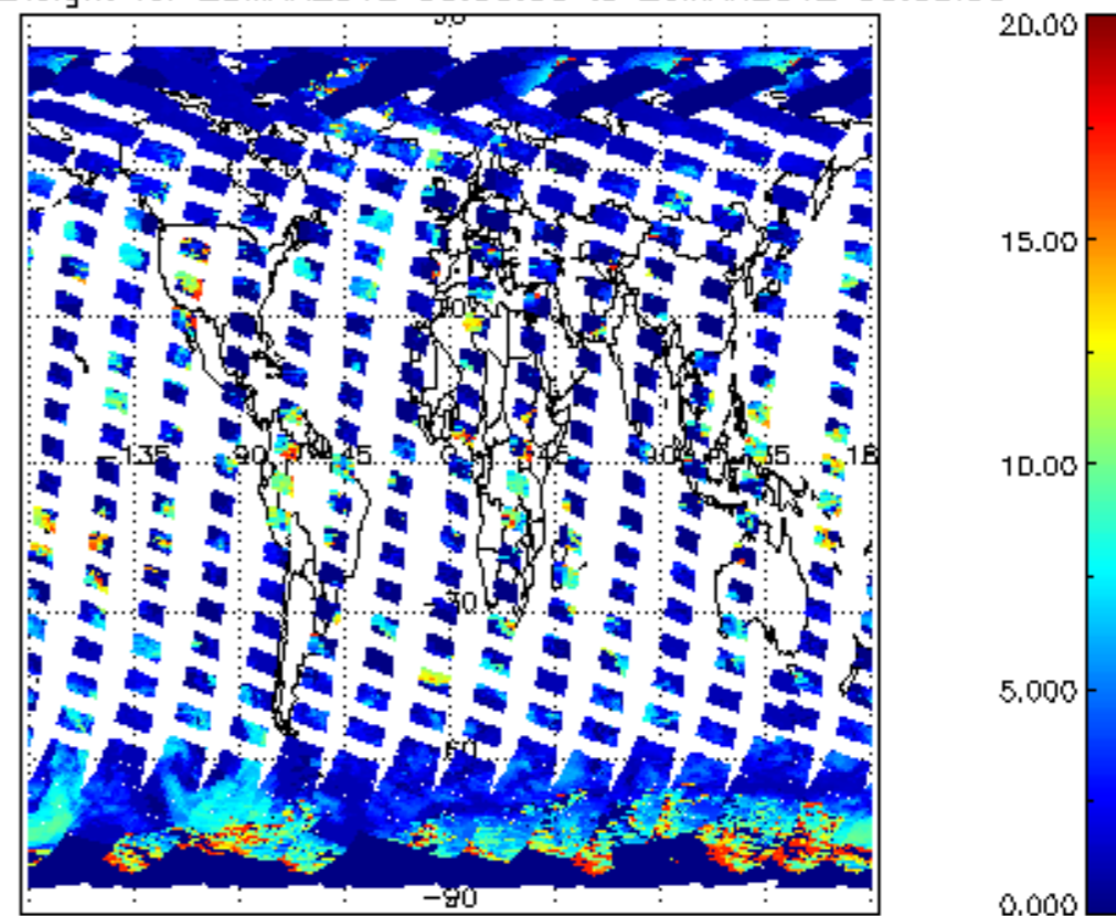
cL_top_height for 25MAR2012 00:00:00 to 26MAR2012 00:00:00
