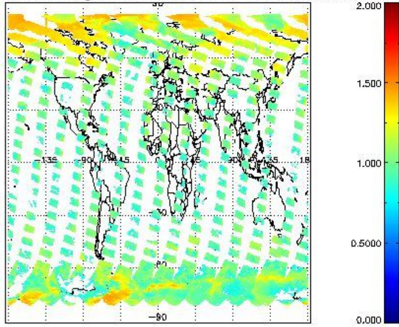
SCIOL2P_NADUV8H2O_arnf_gr for 25MAR2012 00:00:00 to 26MAR2012 00:00:00
