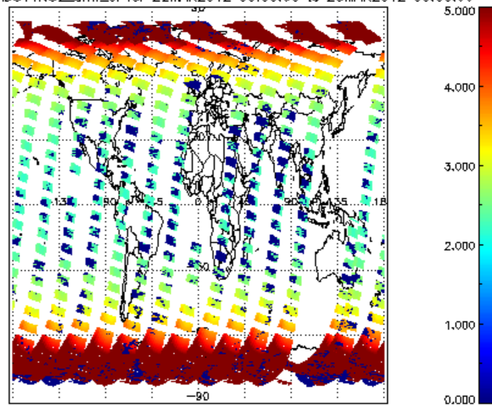
SCIOL2P_NADUV1NO2_amf_cl for 22MAR2012 00:00:00 to 23MAR2012 00:00:00
