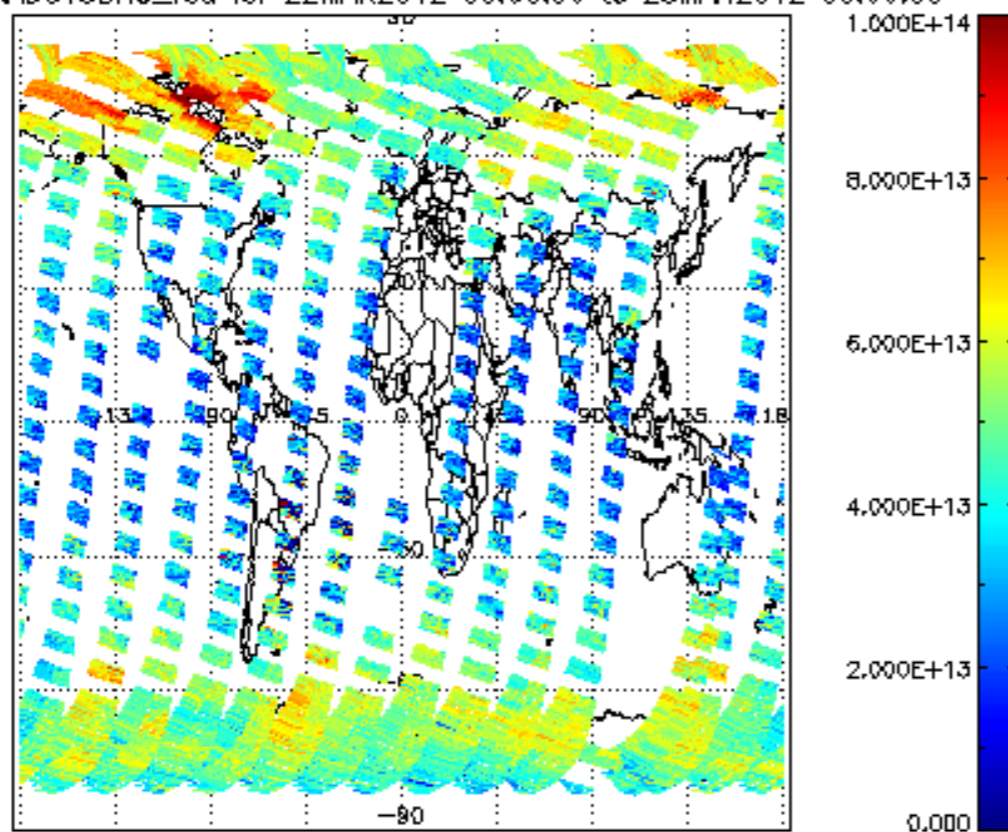
SCIOL2P_NADUV3BRO_vcd for 22MAR2012 00:00:00 to 23MAR2012 00:00:00
