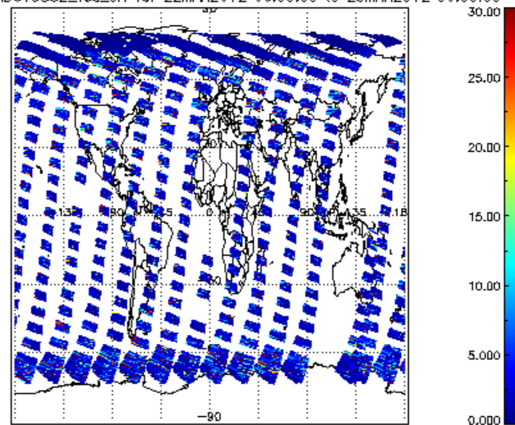
SCIOL2P_NADUV5S02_vcd_err for 22MAR2012 00:00:00 to 23MAR2012 00:00:00
