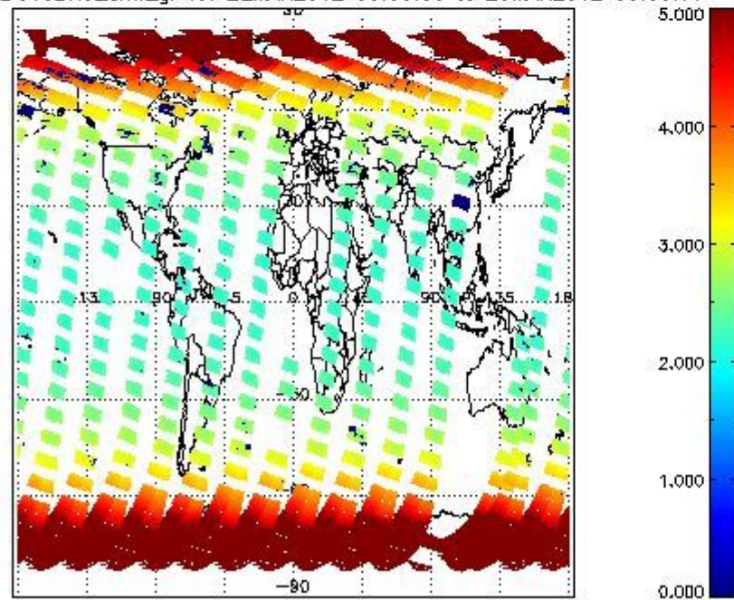
SCIOL2P_NADUV3BRO_amf_gr for 22MAR2012 00:00:00 to 23MAR2012 00:00:00
