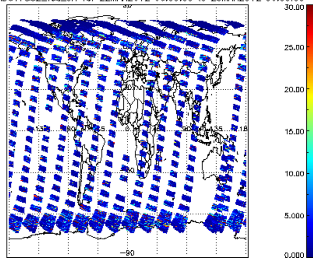
SCIOL2P_NADUV7S02_vcd_err for 22MAR2012 00:00:00 to 23MAR2012 00:00:00
