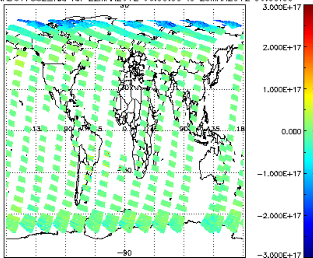
SCIOL2P_NADUV7S02_vcd for 22MAR2012 00:00:00 to 23MAR2012 00:00:00
