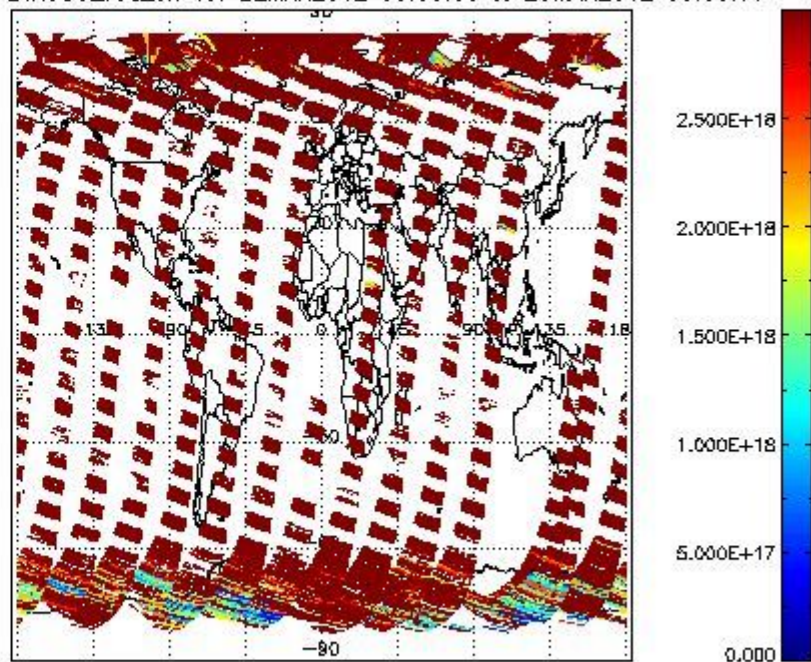
SCIDL2P_NADIR3CO_vcd_err for 22MAR2012 00:00:00 to 23MAR2012 00:00:00
