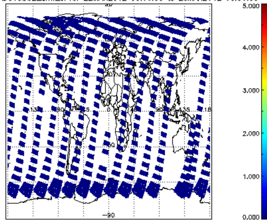
SCIOL2P_NADUV5S02_amf_cl for 22MAR2012 00:00:00 to 23MAR2012 00:00:00
