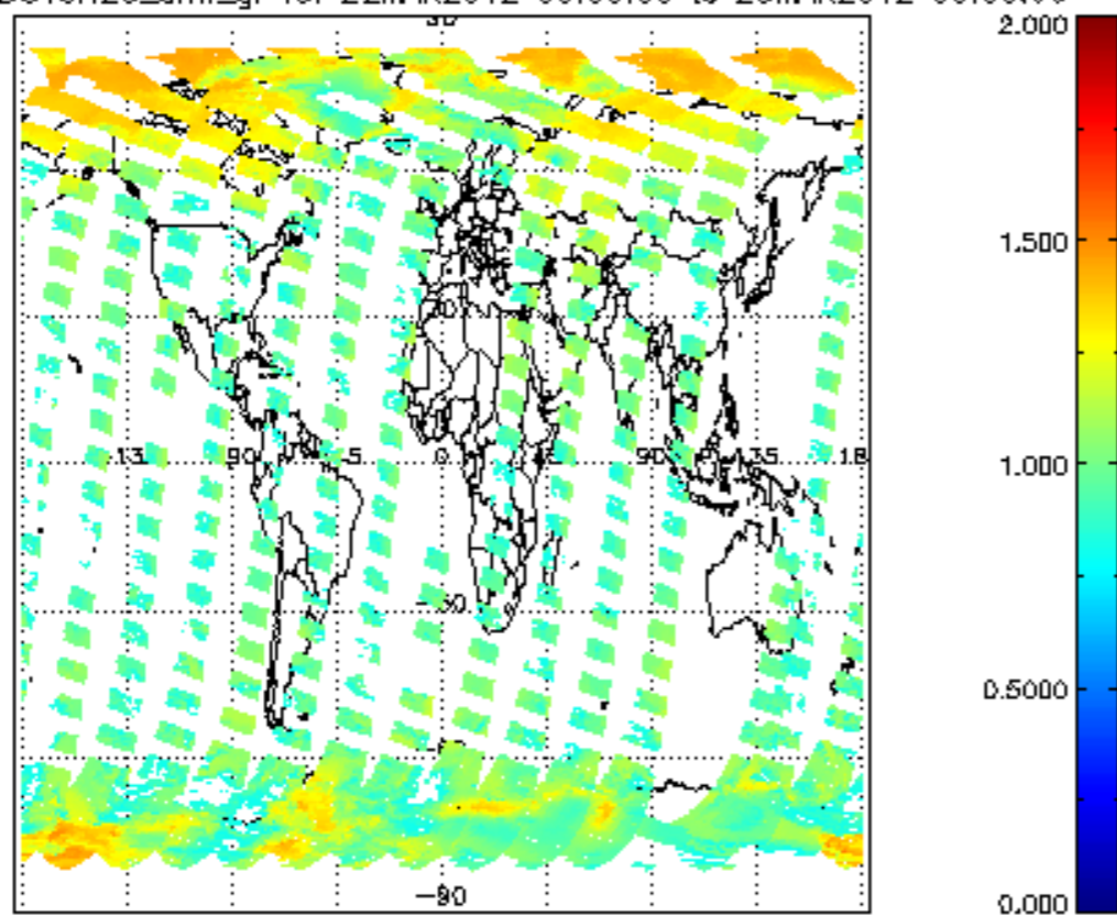
SCIOL2P_NADUV8H20_arnf_gr for 22MAR2012 00:00:00 to 23MAR2012 00:00:00
