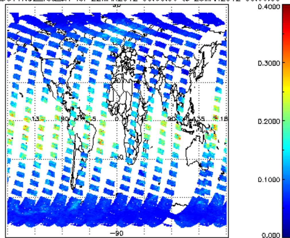
SCIOL2P_NADUV1NO2_vcd_err for 22MAR2012 00:00:00 to 23MAR2012 00:00:00
