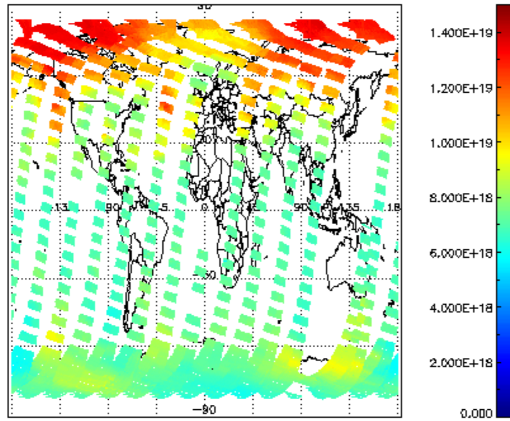
SCIOL2P_NADUV003_vcd for 22MAR2012 00:00:00 to 23MAR2012 00:00:00
