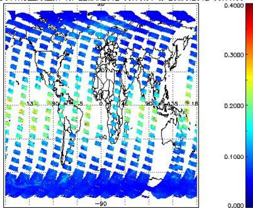
SCIOL2P_NADUV1NO2_vcd_err for 22MAR2012 00:00:00 to 23MAR2012 00:00:00
