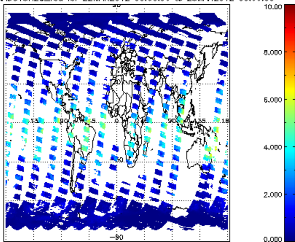
SCIOL2P_NADUV8H20_vcd for 22MAR2012 00:00:00 to 23MAR2012 00:00:00
