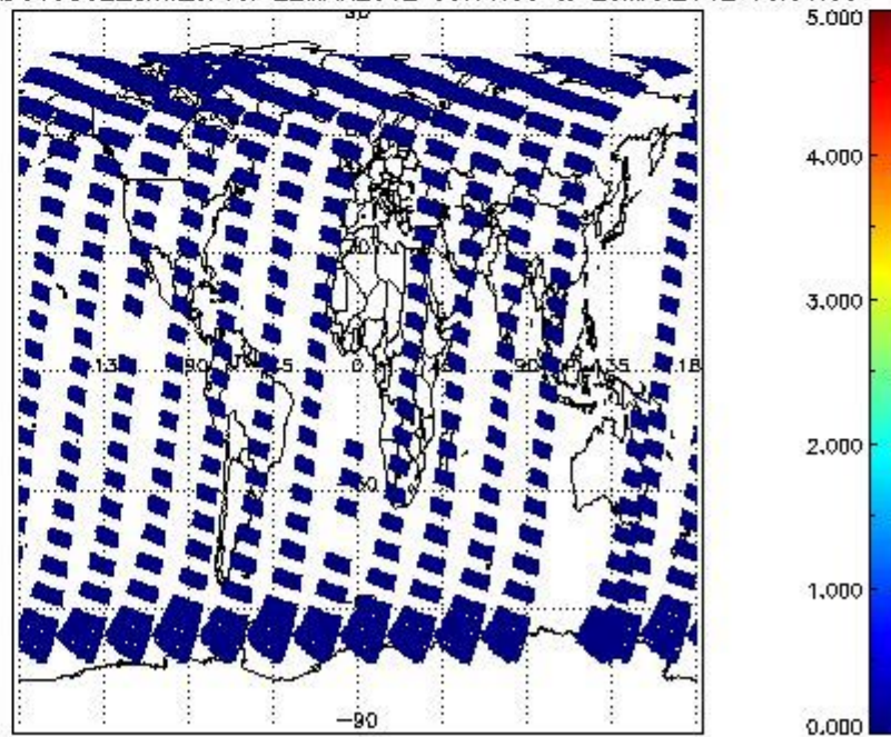
SCIOL2P_NADUV5SO2_amf_cl for 22MAR2012 00:00:00 to 23MAR2012 00:00:00
