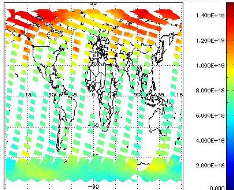
SCIOL2P_NADUV003_vcd for 22MAR2012 00:00:00 to 23MAR2012 00:00:00
