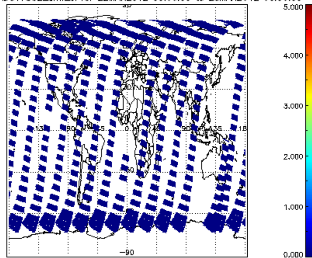
SCIOL2P_NADUV7S02_amf_cl for 22MAR2012 00:00:00 to 23MAR2012 00:00:00
