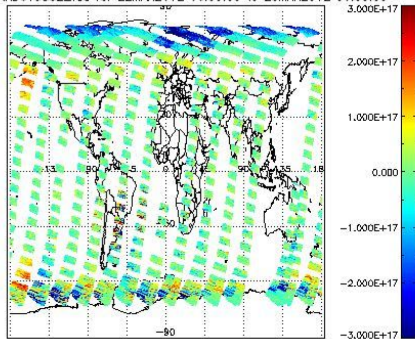
SCIOL2P_NADUV5SO2_vcd for 22MAR2012 00:00:00 to 23MAR2012 00:00:00
