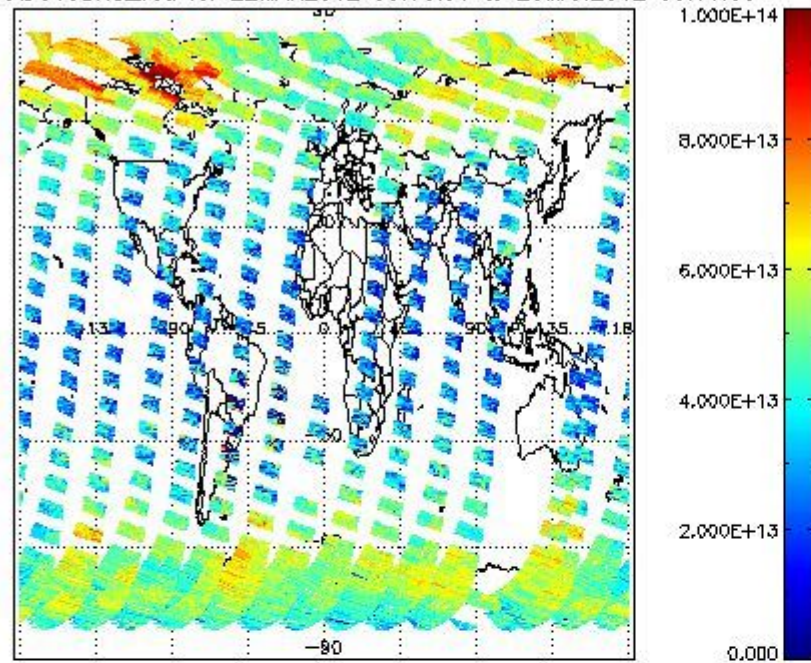
SCIOL2P_NADUV3BRO_vcd for 22MAR2012 00:00:00 to 23MAR2012 00:00:00
