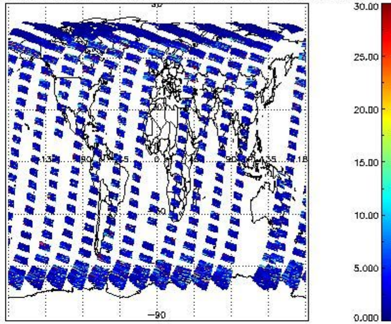
SCIOL2P_NADUV7S02_vcd_err for 22MAR2012 00:00:00 to 23MAR2012 00:00:00
