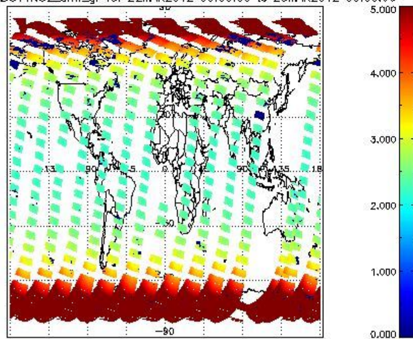
SCIOL2P_NADUV1NO2_amf_gr for 22MAR2012 00:00:00 to 23MAR2012 00:00:00
