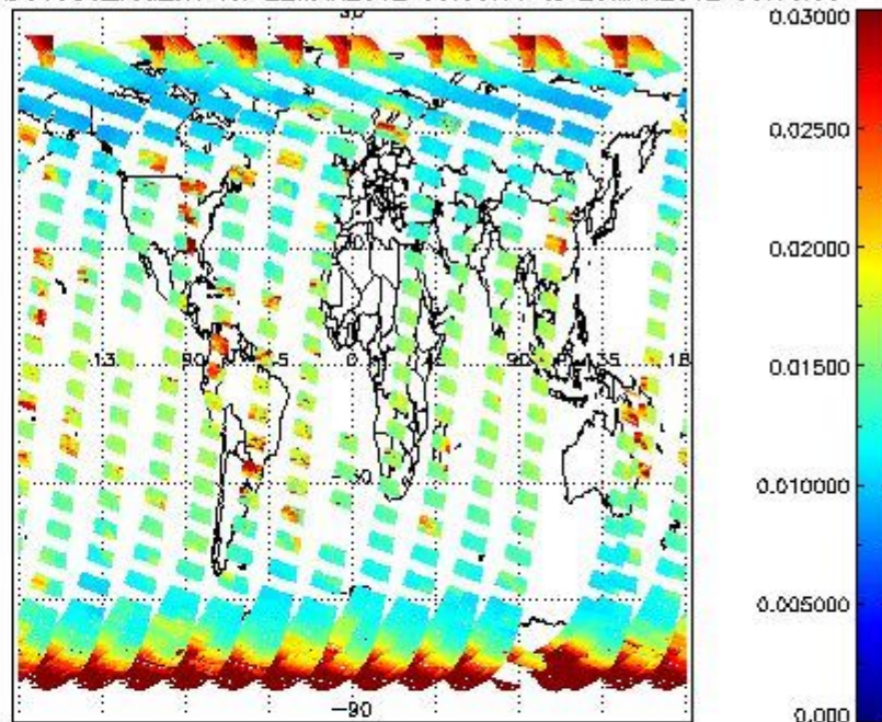
SCIOL2P_NADUV003_vcd_err for 22MAR2012 00:00:00 to 23MAR2012 00:00:00
