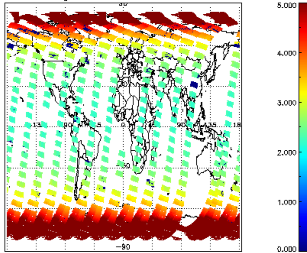
SCIOL2P_NADUV003_amf_gr for 22MAR2012 00:00:00 to 23MAR2012 00:00:00
