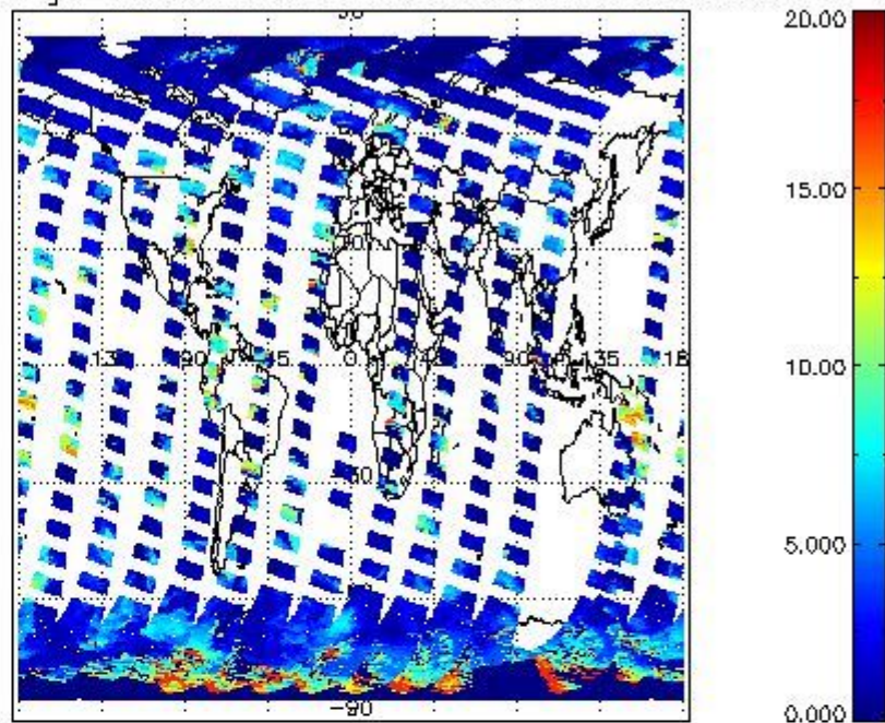
cL_top_height for 22MAR2012 00:00:00 to 23MAR2012 00:00:00
