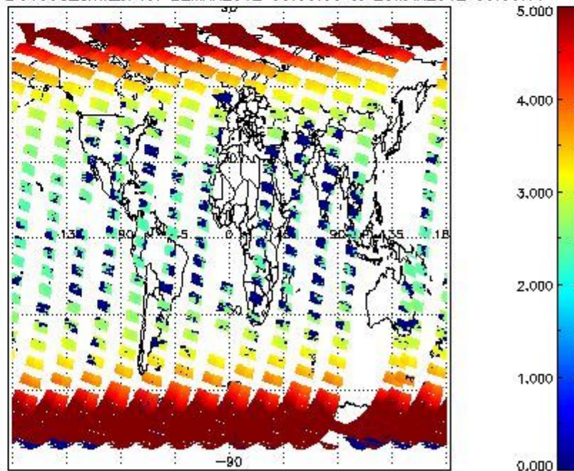
SCIOL2P_NADUV003_amf_cl for 22MAR2012 00:00:00 to 23MAR2012 00:00:00
