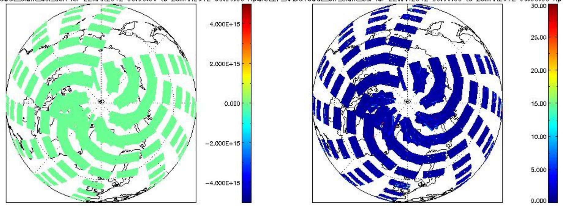
CIOL2P_NADUV6OCL_slant_col_den for 22MAR2012 00:00:00 to 23MAR2012 00:00:00 npCIOL2P_NADUV6OCL_err_slant_col for 22MAR2012 00:00:00 to 23MAR2012 00:00:00 np
