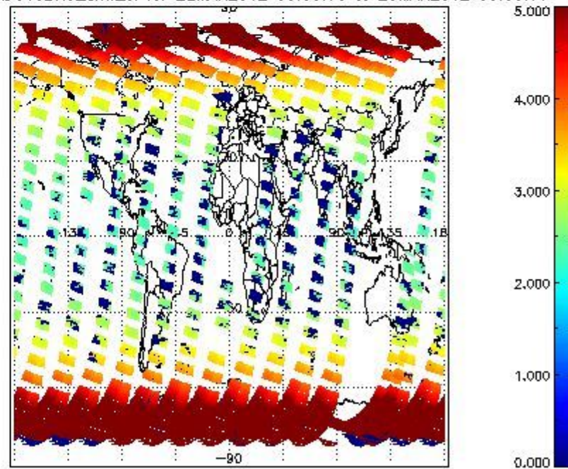
SCIOL2P_NADUV3BRO_amf_cl for 22MAR2012 00:00:00 to 23MAR2012 00:00:00
