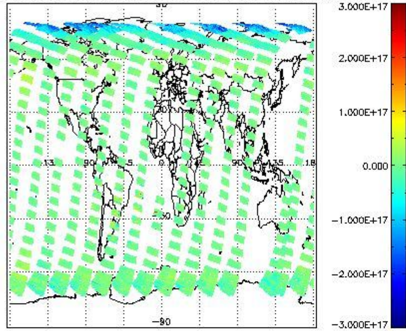
SCIOL2P_NADUV7S02_vcd for 22MAR2012 00:00:00 to 23MAR2012 00:00:00
