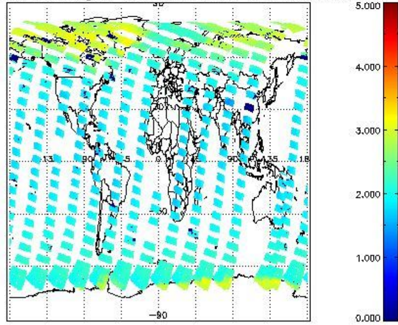
SCIOL2P_NADUV7S02_amf_gr for 22MAR2012 00:00:00 to 23MAR2012 00:00:00
