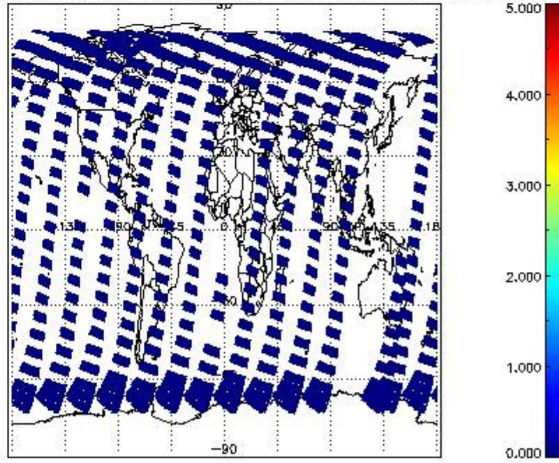
SCIOL2P_NADUV7S02_amf_cl for 22MAR2012 00:00:00 to 23MAR2012 00:00:00
