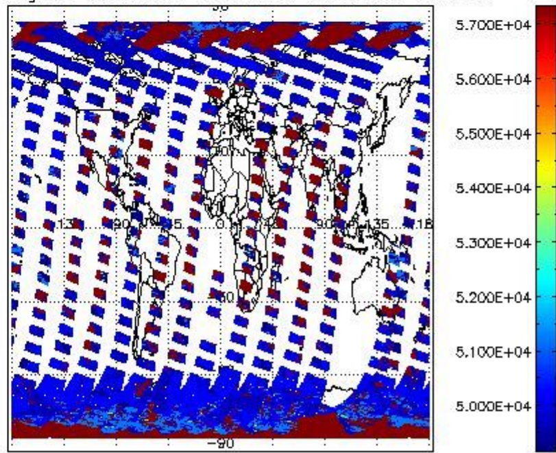
cloud_flags for 22MAR2012 00:00:00 to 23MAR2012 00:00:00
