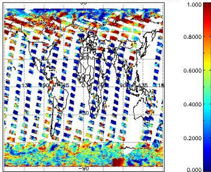
cL_frac for 22MAR2012 00:00:00 to 23MAR2012 00:00:00
