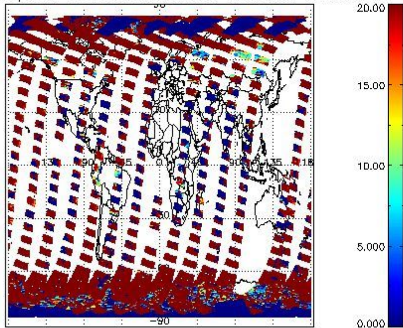
cL_opt_depth for 22MAR2012 00:00:00 to 23MAR2012 00:00:00
