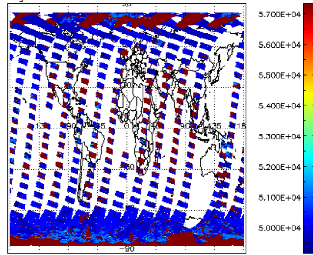
cloud_flags for 22MAR2012 00:00:00 to 23MAR2012 00:00:00
