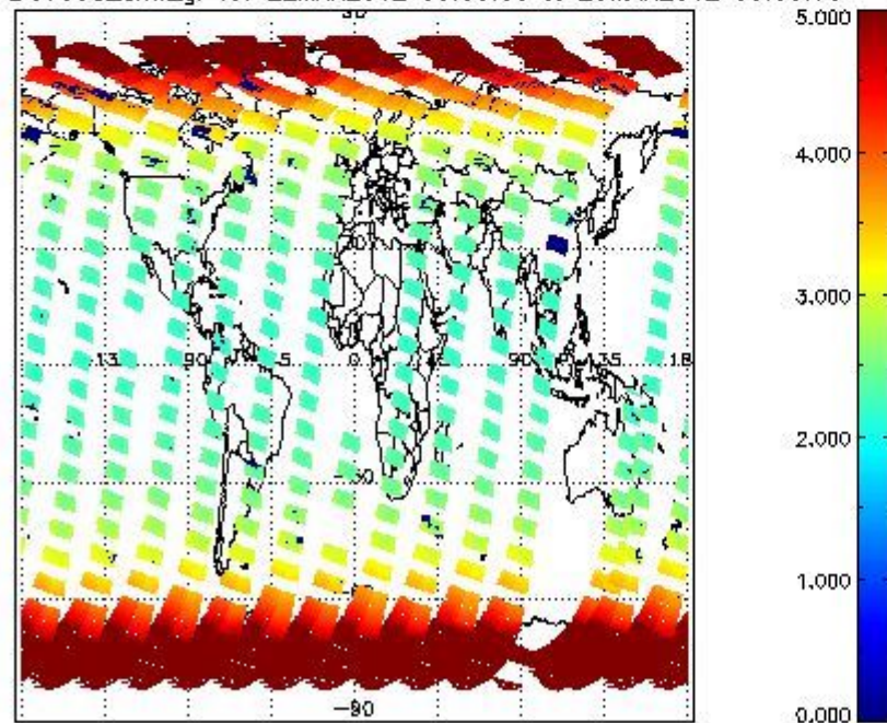
SCIOL2P_NADUV003_amf_gr for 22MAR2012 00:00:00 to 23MAR2012 00:00:00
