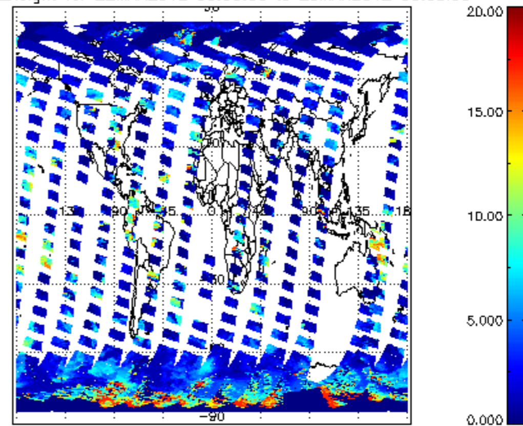
cL_top_height for 22MAR2012 00:00:00 to 23MAR2012 00:00:00
