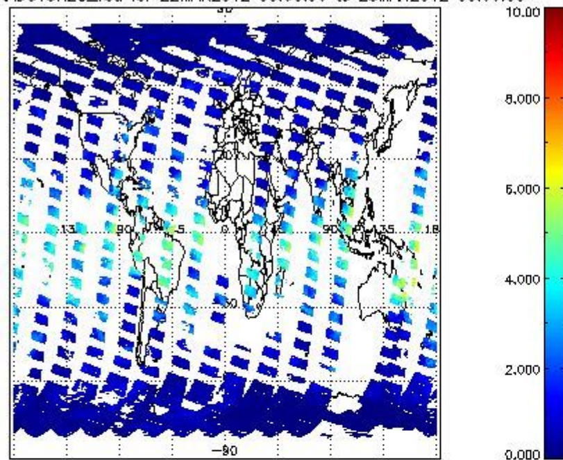
SCIOL2P_NADUV8H2O_vcd for 22MAR2012 00:00:00 to 23MAR2012 00:00:00
