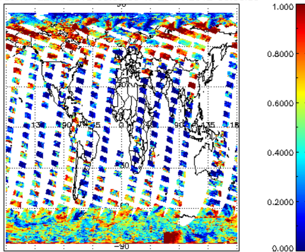
cL_frac for 22MAR2012 00:00:00 to 23MAR2012 00:00:00
