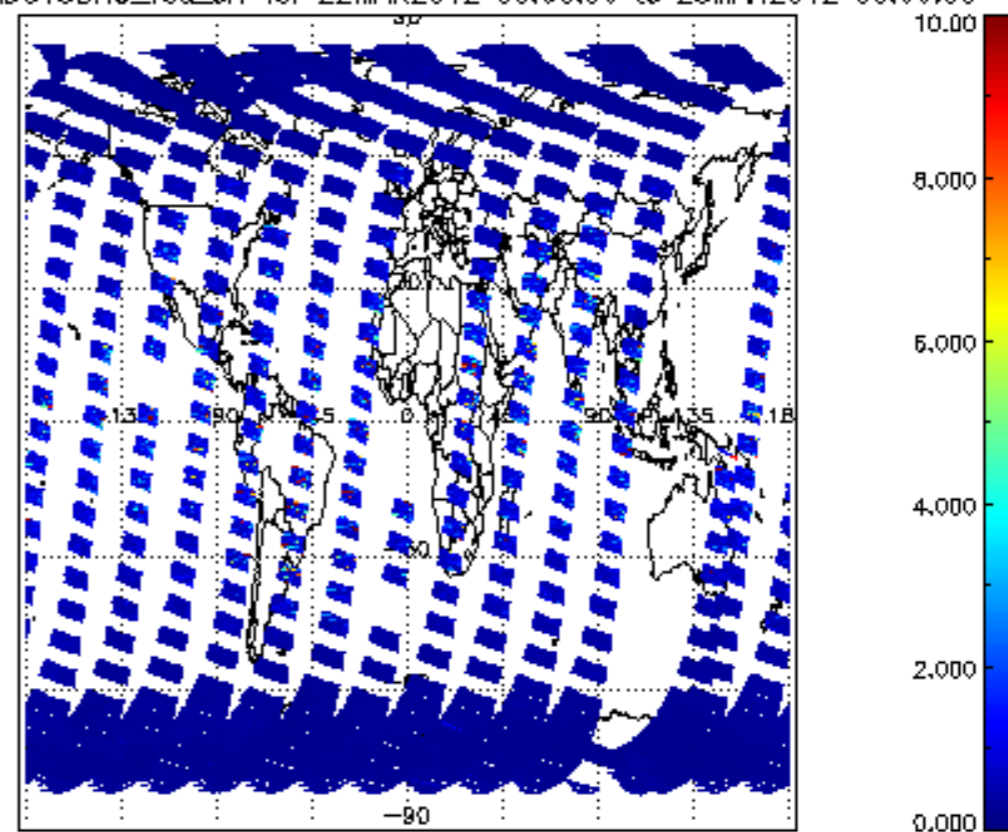
SCIOL2P_NADUV3BRO_vcd_err for 22MAR2012 00:00:00 to 23MAR2012 00:00:00
