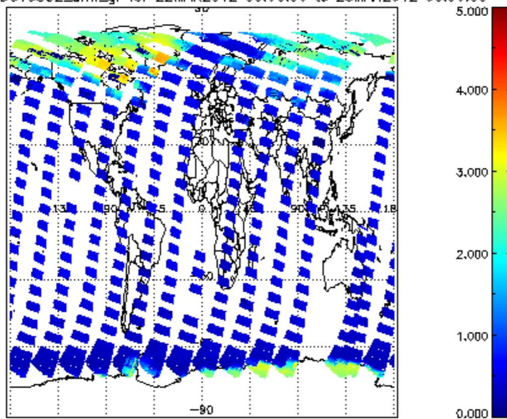
SCIOL2P_NADUV5S02_amf_gr for 22MAR2012 00:00:00 to 23MAR2012 00:00:00
