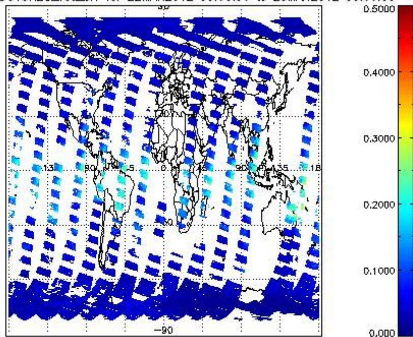
SCIOL2P_NADUV8H2O_vcd_err for 22MAR2012 00:00:00 to 23MAR2012 00:00:00
