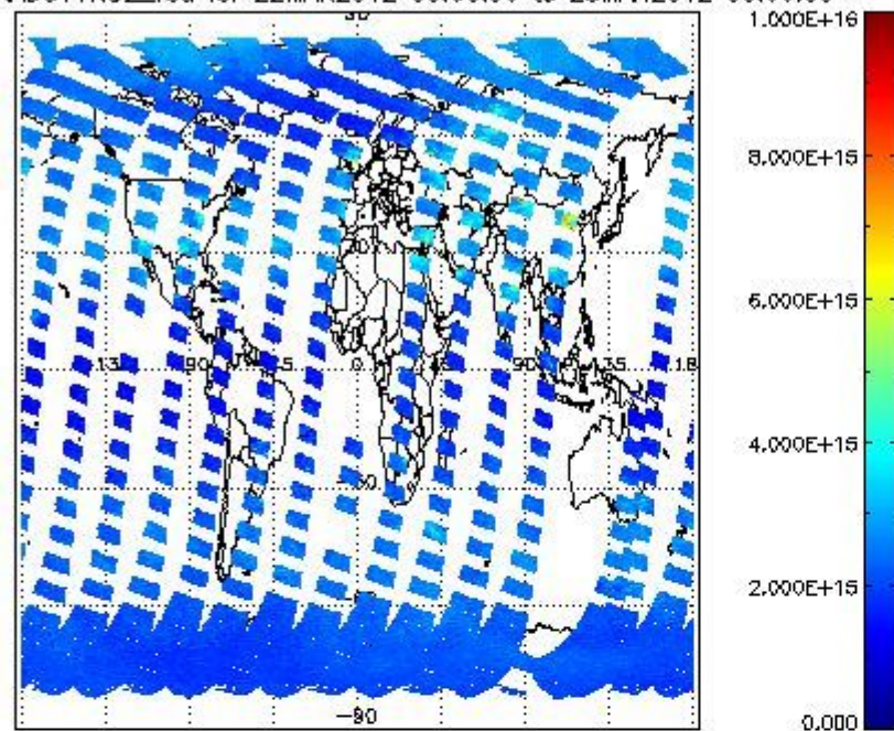
SCIOL2P_NADUV1NO2_vcd for 22MAR2012 00:00:00 to 23MAR2012 00:00:00
