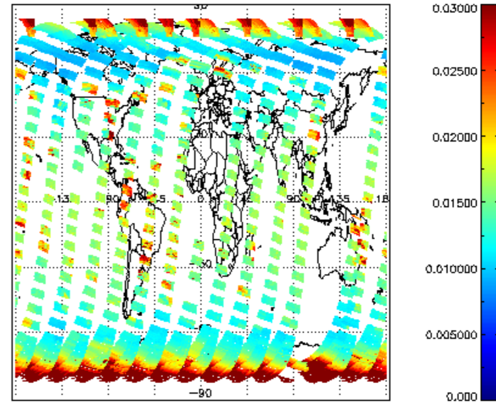
SCIOL2P_NADUV003_vcd_err for 22MAR2012 00:00:00 to 23MAR2012 00:00:00
