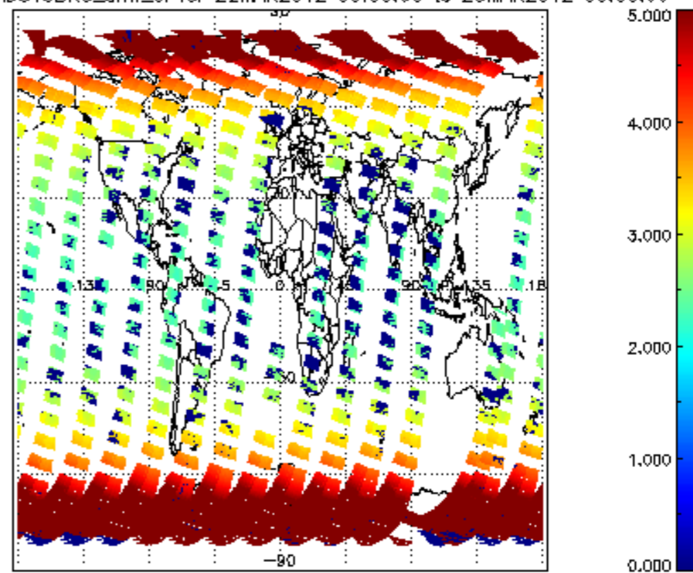
SCIOL2P_NADUV3BRO_amf_cl for 22MAR2012 00:00:00 to 23MAR2012 00:00:00
