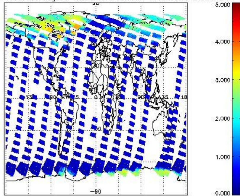
SCIOL2P_NADUV5SO2_amf_gr for 22MAR2012 00:00:00 to 23MAR2012 00:00:00
