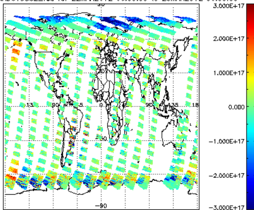
SCIOL2P_NADUV5S02_vcd for 22MAR2012 00:00:00 to 23MAR2012 00:00:00
