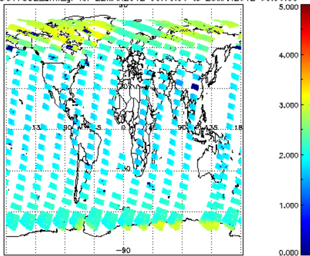
SCIOL2P_NADUV7S02_amf_gr for 22MAR2012 00:00:00 to 23MAR2012 00:00:00
