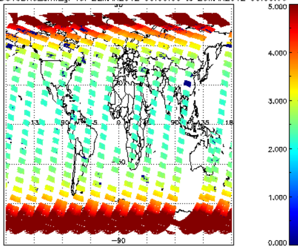
SCIOL2P_NADUV3BRO_amf_gr for 22MAR2012 00:00:00 to 23MAR2012 00:00:00
