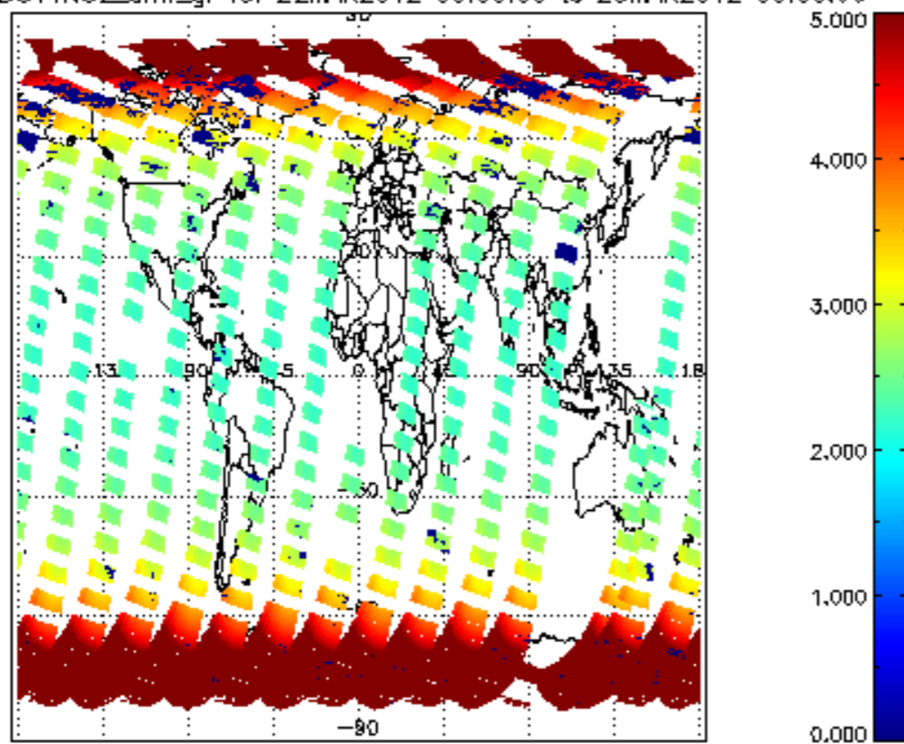
SCIOL2P_NADUV1NO2_amf_gr for 22MAR2012 00:00:00 to 23MAR2012 00:00:00
