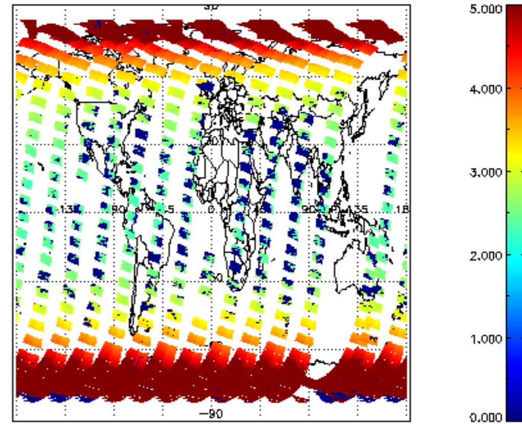
SCIOL2P_NADUV003_amf_cl for 22MAR2012 00:00:00 to 23MAR2012 00:00:00
