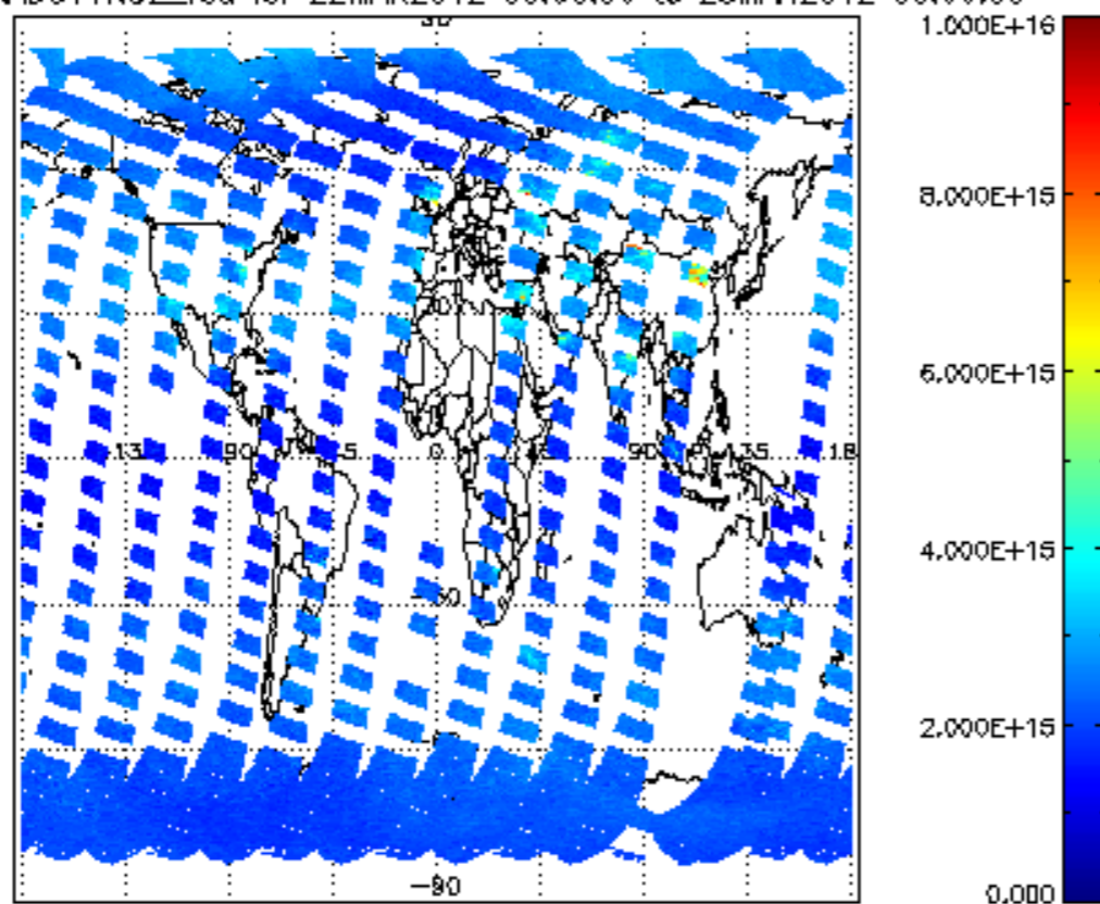
SCIOL2P_NADUV1NO2_vcd for 22MAR2012 00:00:00 to 23MAR2012 00:00:00
