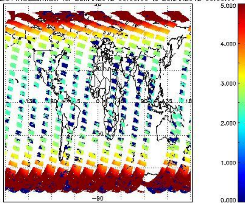
SCIOL2P_NADUV1NO2_amf_cl for 22MAR2012 00:00:00 to 23MAR2012 00:00:00
