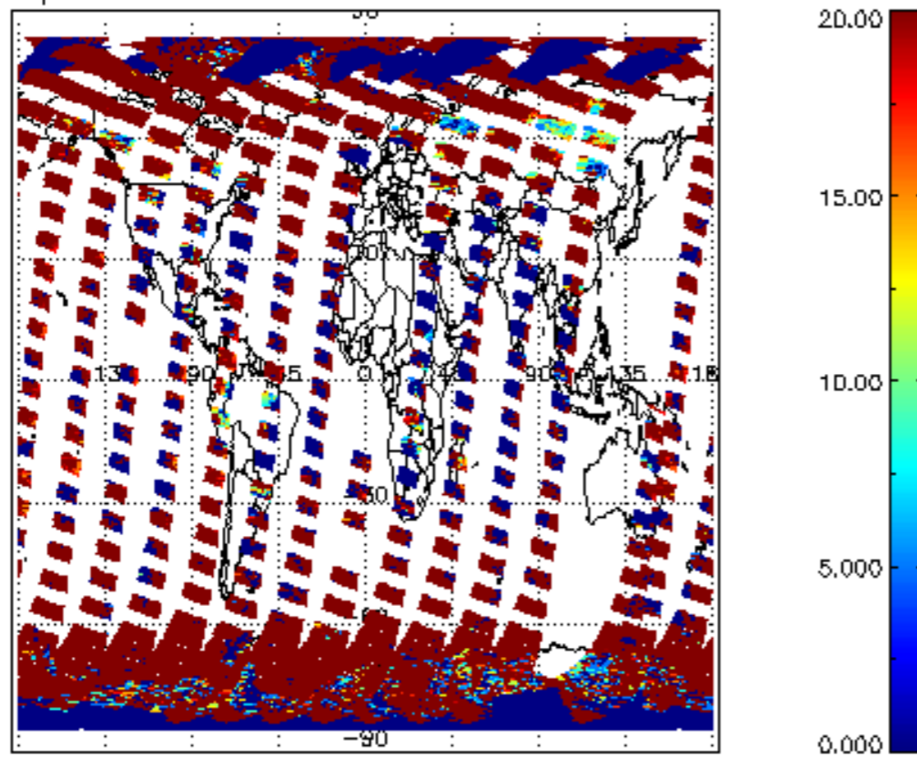
cL_opt_depth for 22MAR2012 00:00:00 to 23MAR2012 00:00:00
