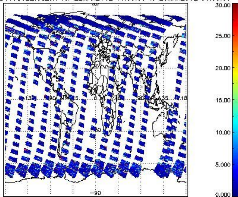
SCIOL2P_NADUV5SO2_vcd_err for 22MAR2012 00:00:00 to 23MAR2012 00:00:00
