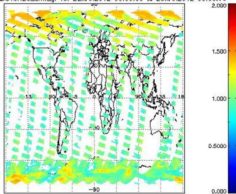
SCIOL2P_NADUV8H2O_amf_gr for 22MAR2012 00:00:00 to 23MAR2012 00:00:00
