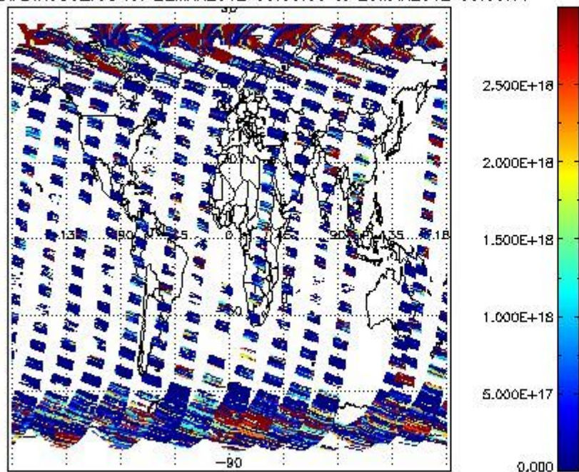
SCIDL2P_NADIR3CO_vcd for 22MAR2012 00:00:00 to 23MAR2012 00:00:00
