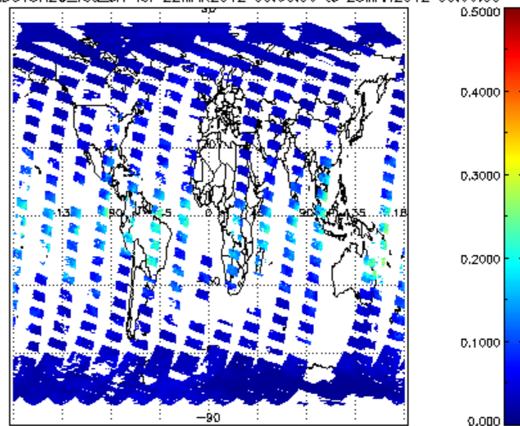
SCIOL2P_NADUV8H20_vcd_err for 22MAR2012 00:00:00 to 23MAR2012 00:00:00
