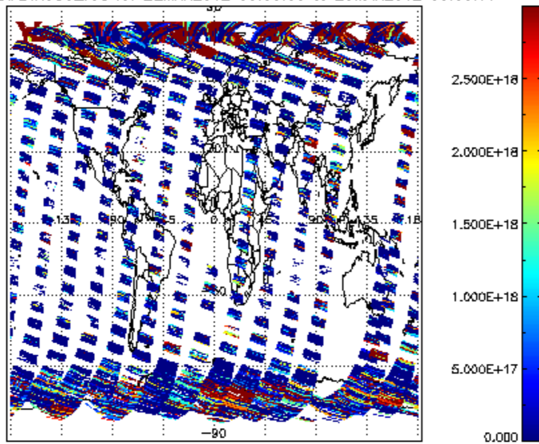
SCIOL2P_NADIR3CO_vcd for 22MAR2012 00:00:00 to 23MAR2012 00:00:00
