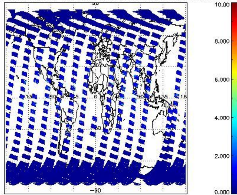
SCIOL2P_NADUV3BRO_vcd_err for 22MAR2012 00:00:00 to 23MAR2012 00:00:00
