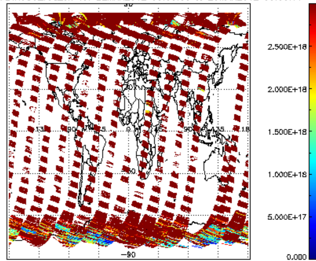
SCIOL2P_NADIR3CO_vcd_err for 22MAR2012 00:00:00 to 23MAR2012 00:00:00
