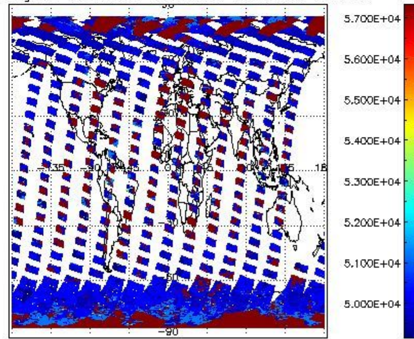
cloud_flags for 20MAR2012 00:00:00 to 21MAR2012 00:00:00
