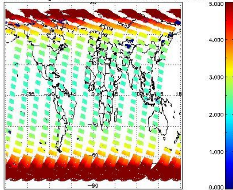
SCIOL2P_NADUV003_amf_gr for 20MAR2012 00:00:00 to 21MAR2012 00:00:00
