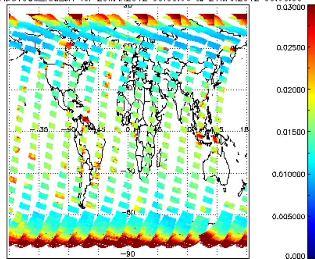
SCIOL2P_NADUV003_vcd_err for 20MAR2012 00:00:00 to 21MAR2012 00:00:00
