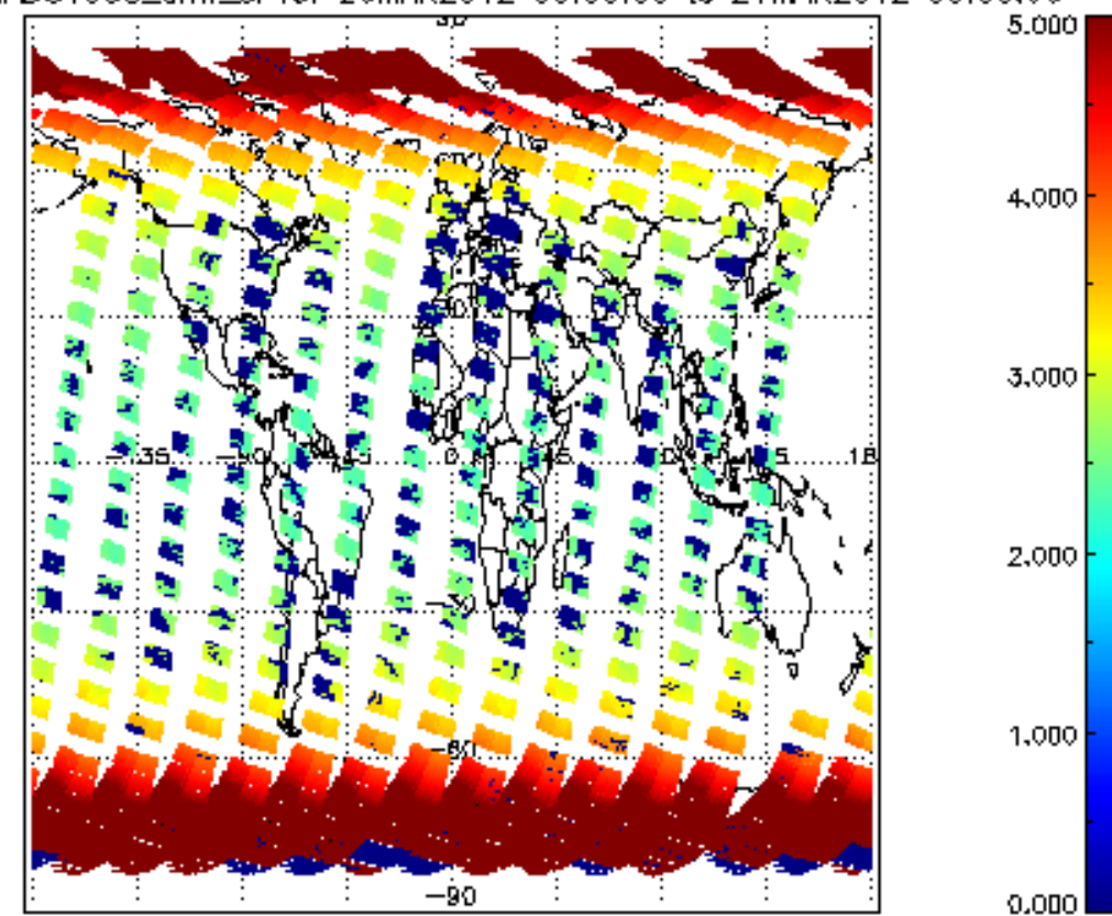
SCIOL2P_NADUV003_arnf_cl for 20MAR2012 00:00:00 to 21MAR2012 00:00:00
