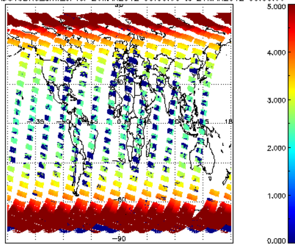
SCIOL2P_NADUV3BRO_amf_cl for 20MAR2012 00:00:00 to 21MAR2012 00:00:00
