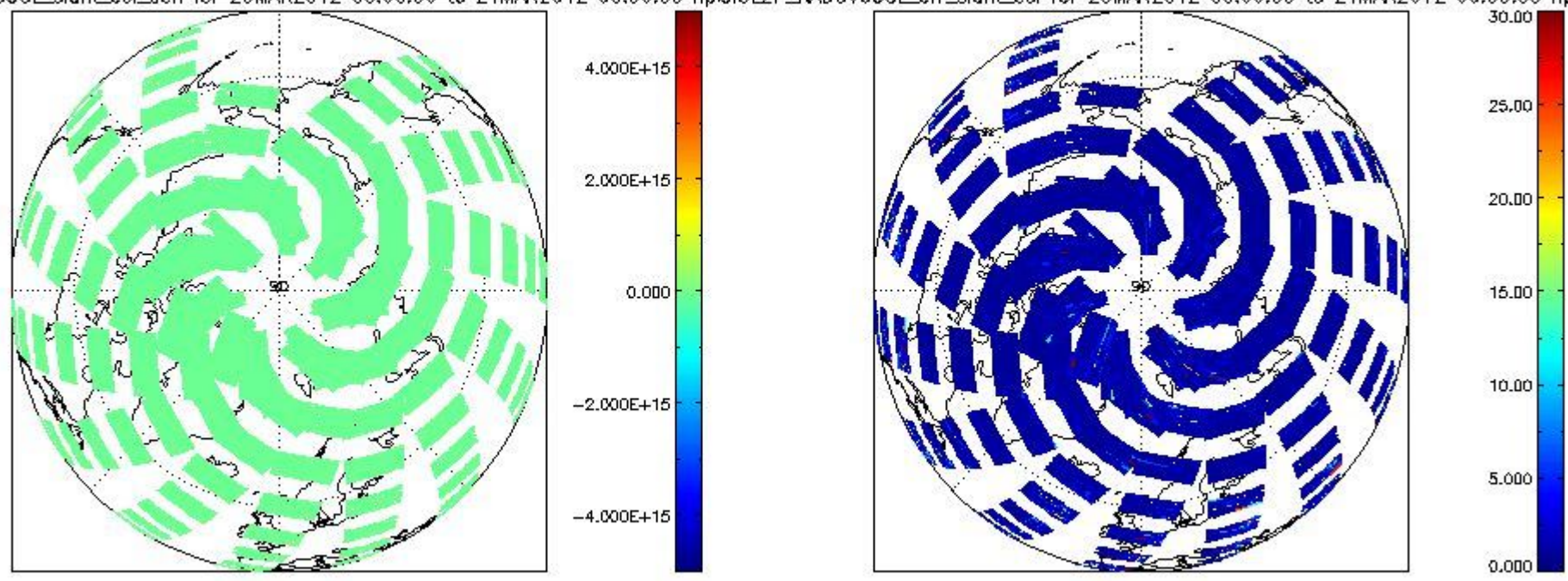
CIOL2P_NADUV6OCLslant_col_den for 20MAR2012 00:00:00 to 21MAR2012 00:00:00 npCIOL2P_NADUV6OCLerr_slant_col for 20MAR2012 00:00:00 to 21MAR2012 00:00:00 np
