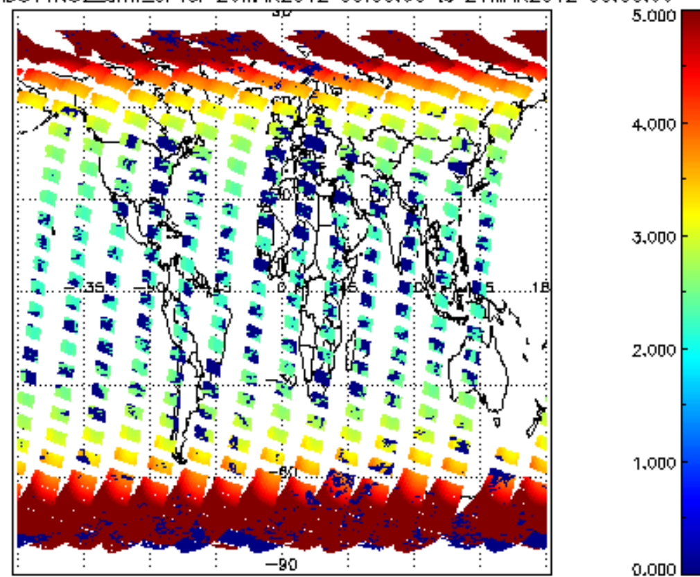
SCIOL2P_NADUV1NO2_amf_cl for 20MAR2012 00:00:00 to 21MAR2012 00:00:00
