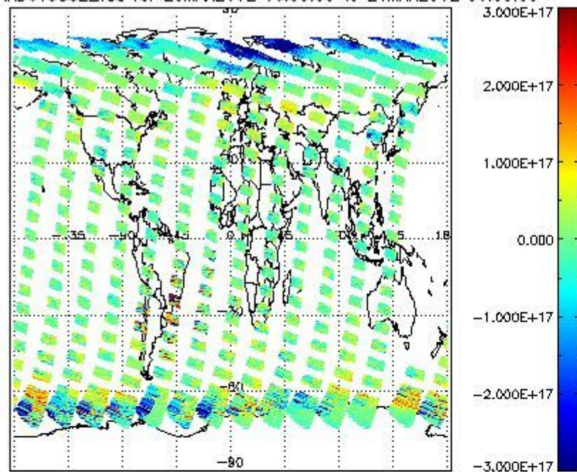
SCIOL2P_NADUV5SO2_vcd for 20MAR2012 00:00:00 to 21MAR2012 00:00:00
