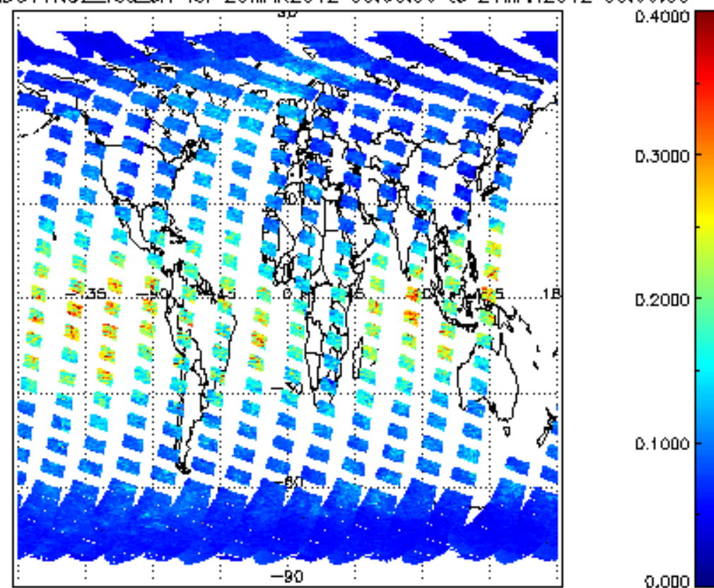
SCIOL2P_NADUV1NO2_vcdLerr for 20MAR2012 00:00:00 to 21MAR2012 00:00:00
