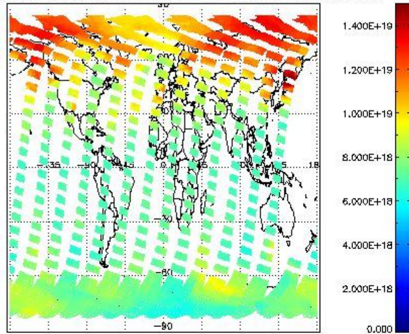
SCIOL2P_NADUV003_vcd for 20MAR2012 00:00:00 to 21MAR2012 00:00:00
