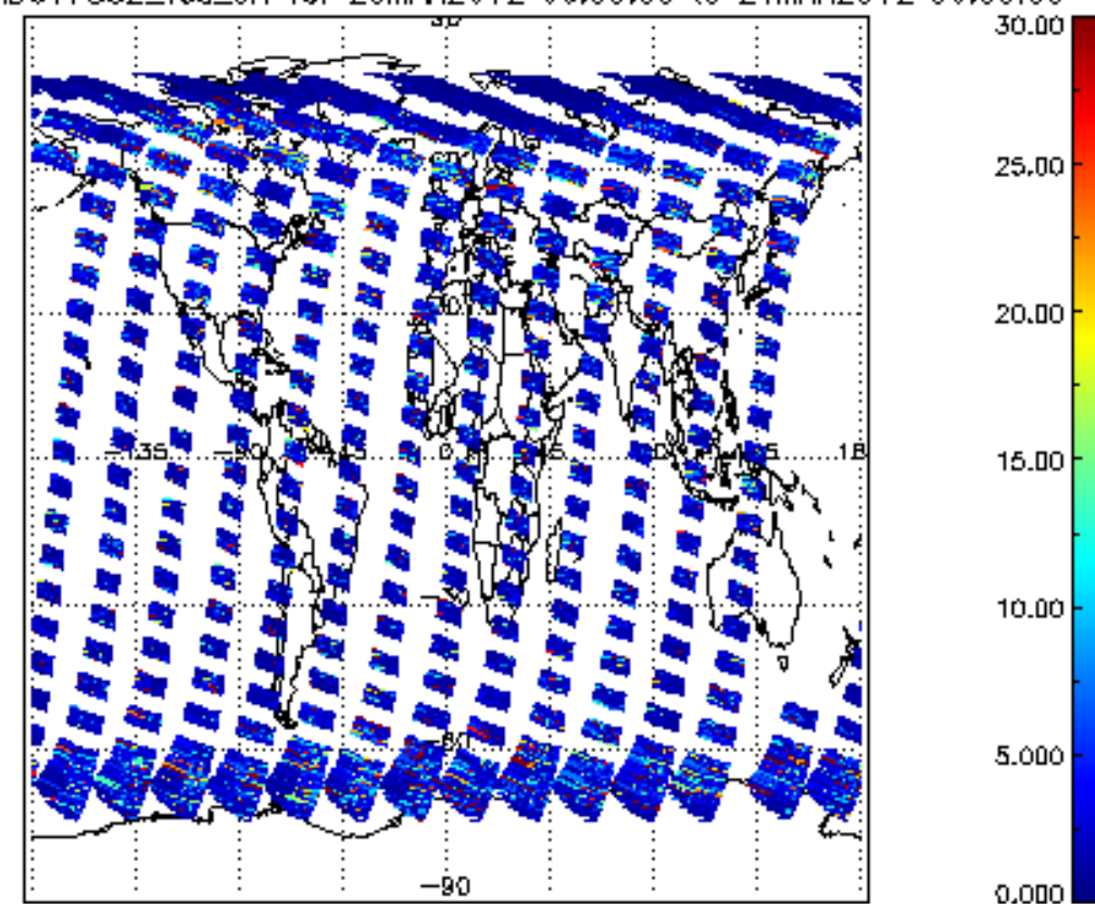
SCIOL2P_NADUV7S02_vcd_err for 20MAR2012 00:00:00 to 21MAR2012 00:00:00
