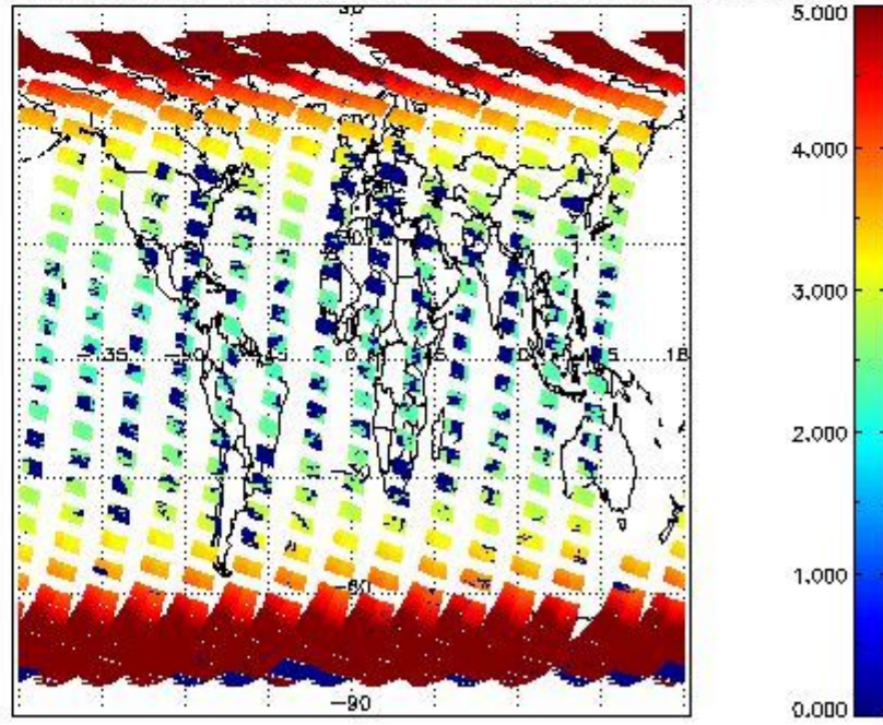
SCIOL2P_NADUV3BRO_amf_cl for 20MAR2012 00:00:00 to 21MAR2012 00:00:00
