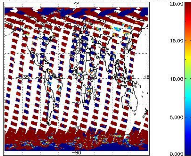
cL_opt_depth for 20MAR2012 00:00:00 to 21MAR2012 00:00:00
