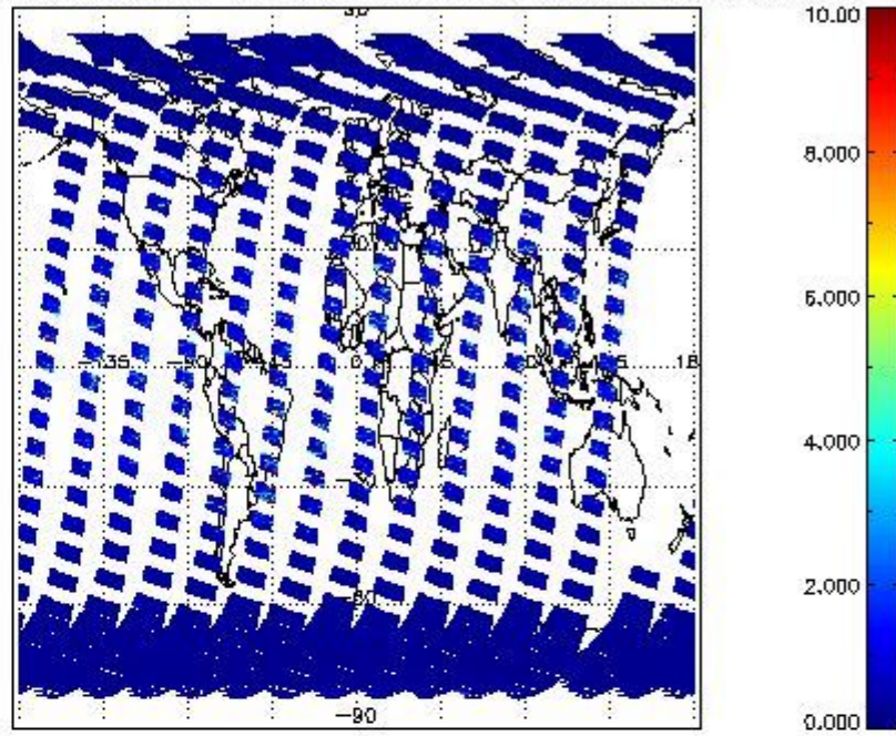
SCIOL2P_NADUV3BRO_vcd_err for 20MAR2012 00:00:00 to 21MAR2012 00:00:00
