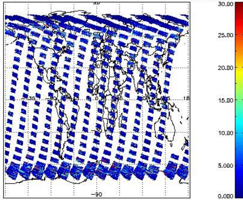
SCIOL2P_NADUV7S02_vcd_err for 20MAR2012 00:00:00 to 21MAR2012 00:00:00
