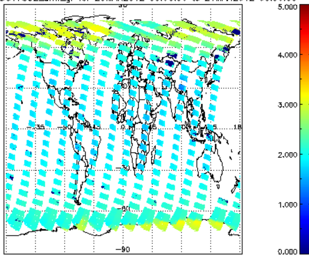
SCIOL2P_NADUV7S02_amf_gr for 20MAR2012 00:00:00 to 21MAR2012 00:00:00
