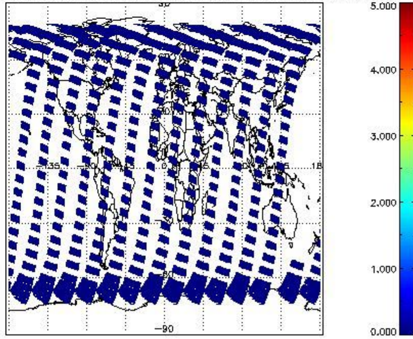
SCIOL2P_NADUV7S02_amf_cl for 20MAR2012 00:00:00 to 21MAR2012 00:00:00
