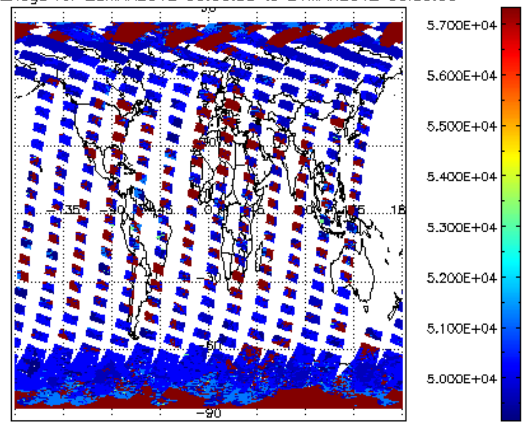
cloud_flags for 20MAR2012 00:00:00 to 21MAR2012 00:00:00
