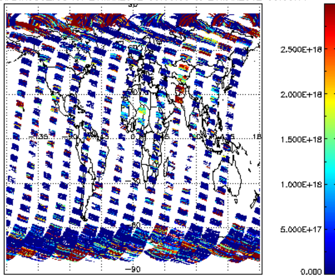
SCIOL2P_NADIR3CO_vcd for 20MAR2012 00:00:00 to 21MAR2012 00:00:00
