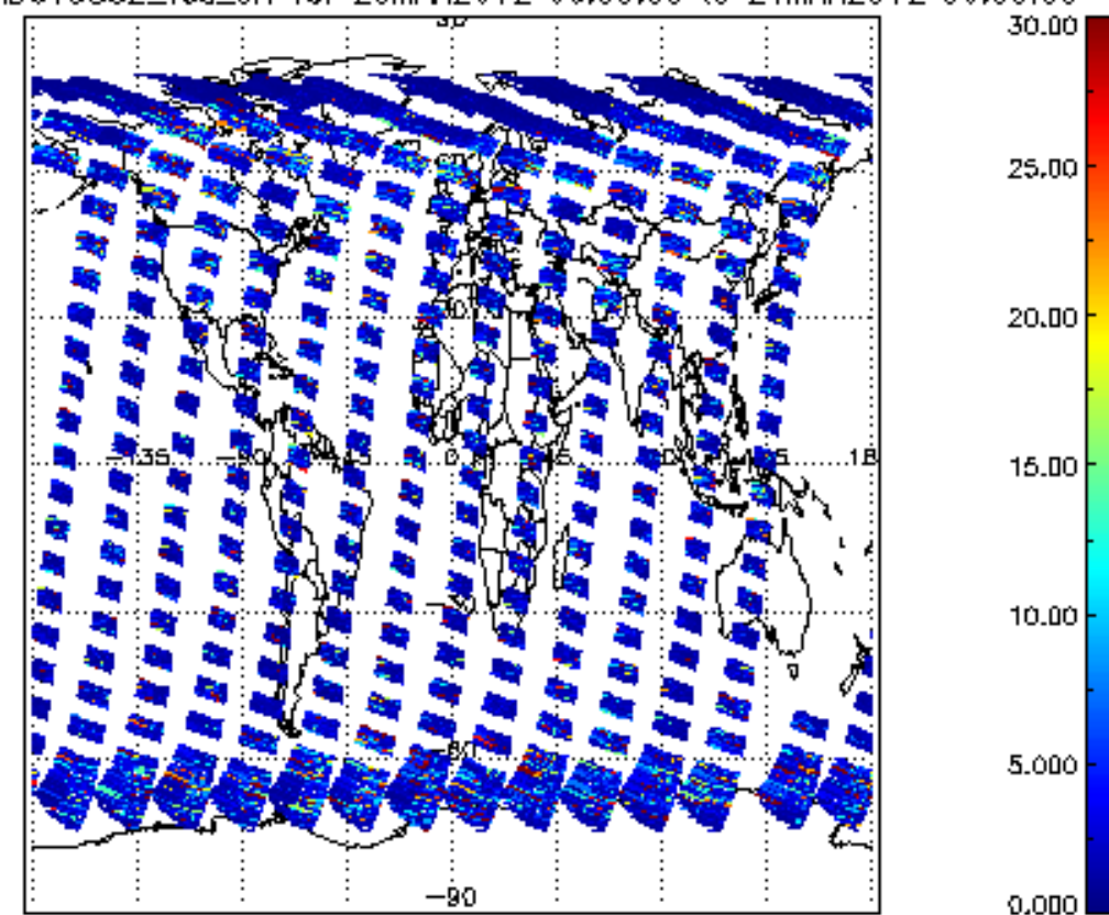
SCIOL2P_NADUV5S02_vcd_err for 20MAR2012 00:00:00 to 21MAR2012 00:00:00
