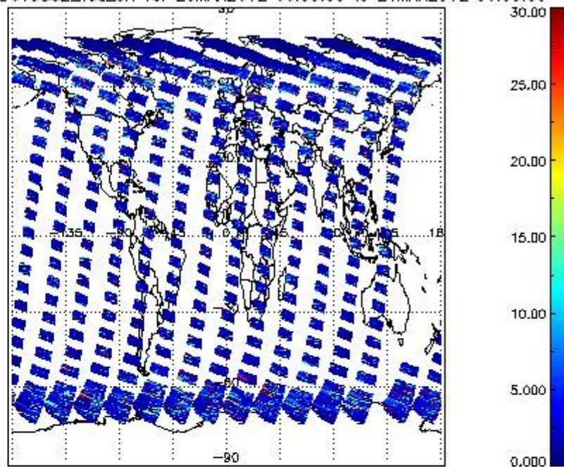
SCIOL2P_NADUV5SO2_vcd_err for 20MAR2012 00:00:00 to 21MAR2012 00:00:00
