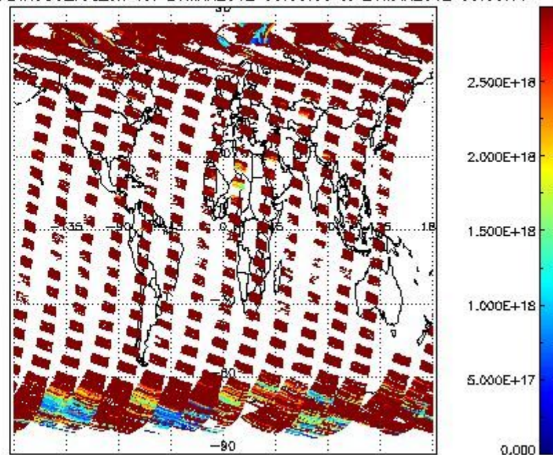
SCIDL2P_NADIR3CO_vcd_err for 20MAR2012 00:00:00 to 21MAR2012 00:00:00
