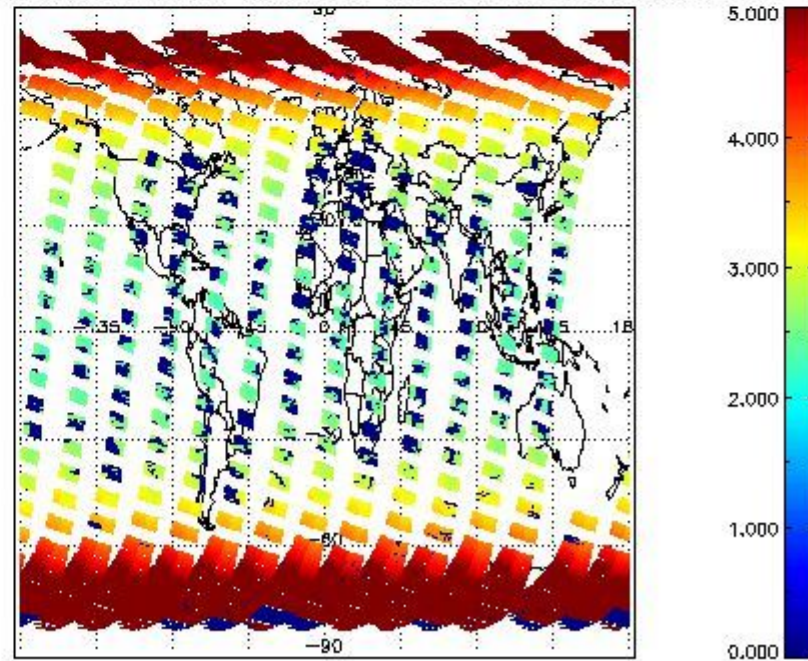
SCIOL2P_NADUV003_amf_cl for 20MAR2012 00:00:00 to 21MAR2012 00:00:00
