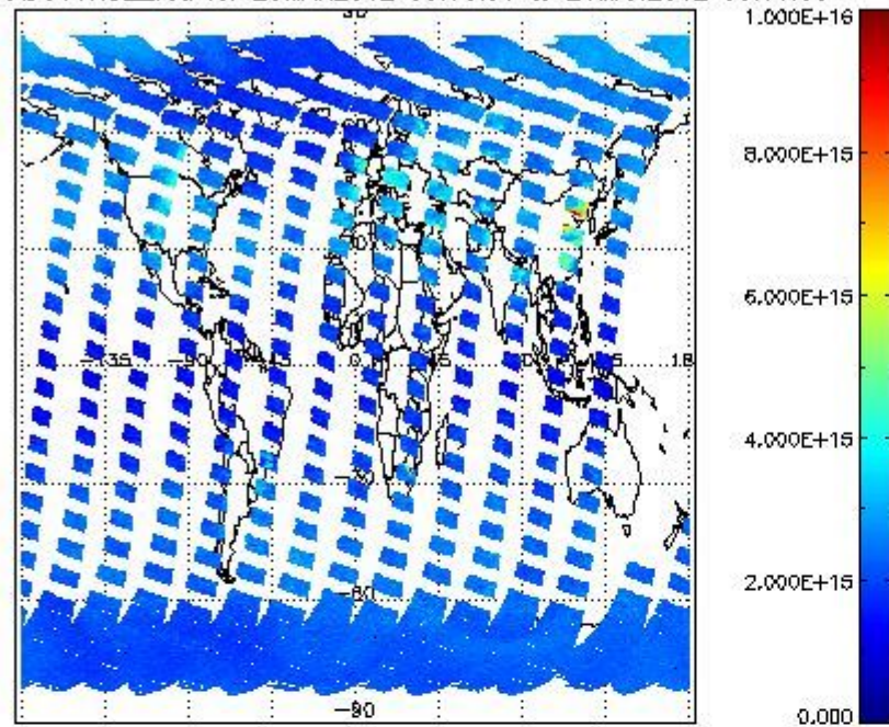
SCIOL2P_NADUV1NO2_vcd for 20MAR2012 00:00:00 to 21MAR2012 00:00:00
