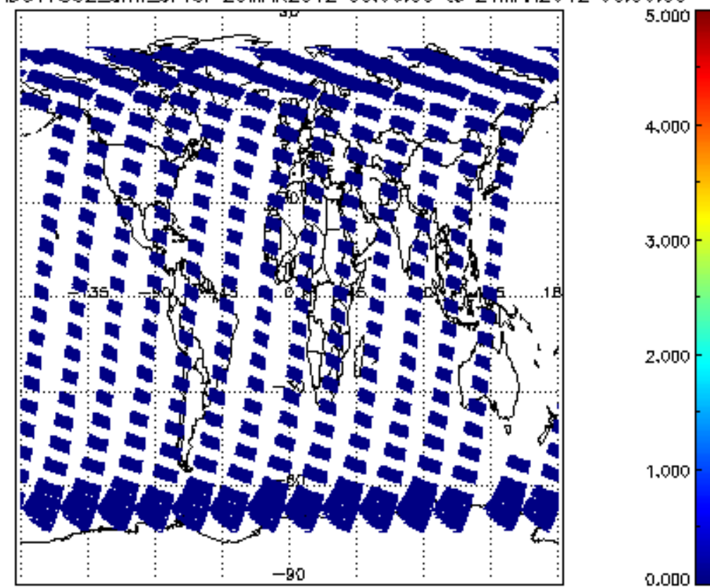
SCIOL2P_NADUV7S02_amf_cl for 20MAR2012 00:00:00 to 21MAR2012 00:00:00
