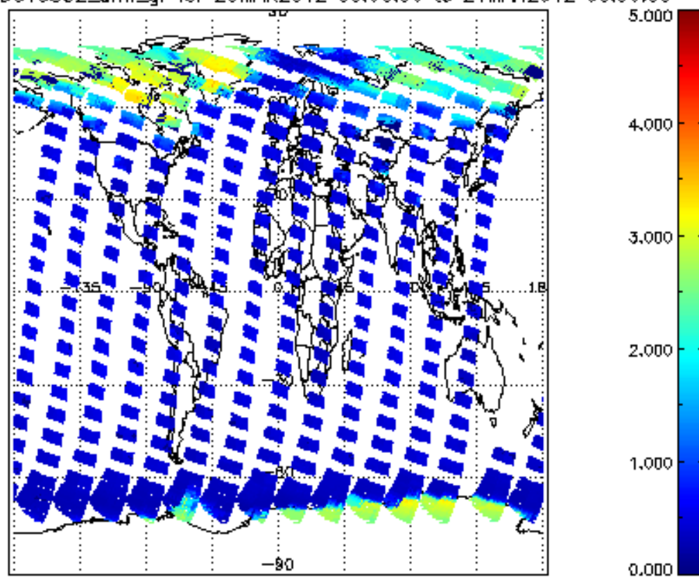
SCIOL2P_NADUV5S02_amf_gr for 20MAR2012 00:00:00 to 21MAR2012 00:00:00
