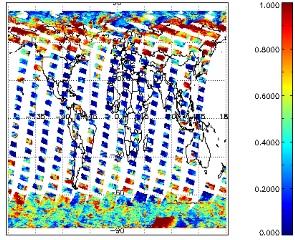
cL_frac for 20MAR2012 00:00:00 to 21MAR2012 00:00:00
