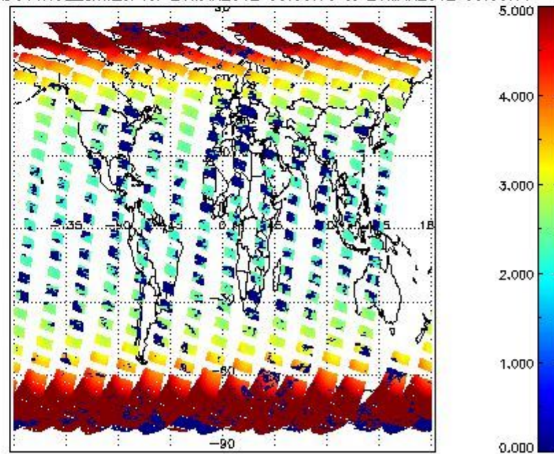
SCIOL2P_NADUV1NO2_amf_cl for 20MAR2012 00:00:00 to 21MAR2012 00:00:00
