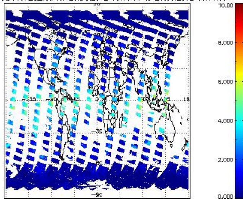
SCIOL2P_NADUV8H2O_vcd for 20MAR2012 00:00:00 to 21MAR2012 00:00:00
