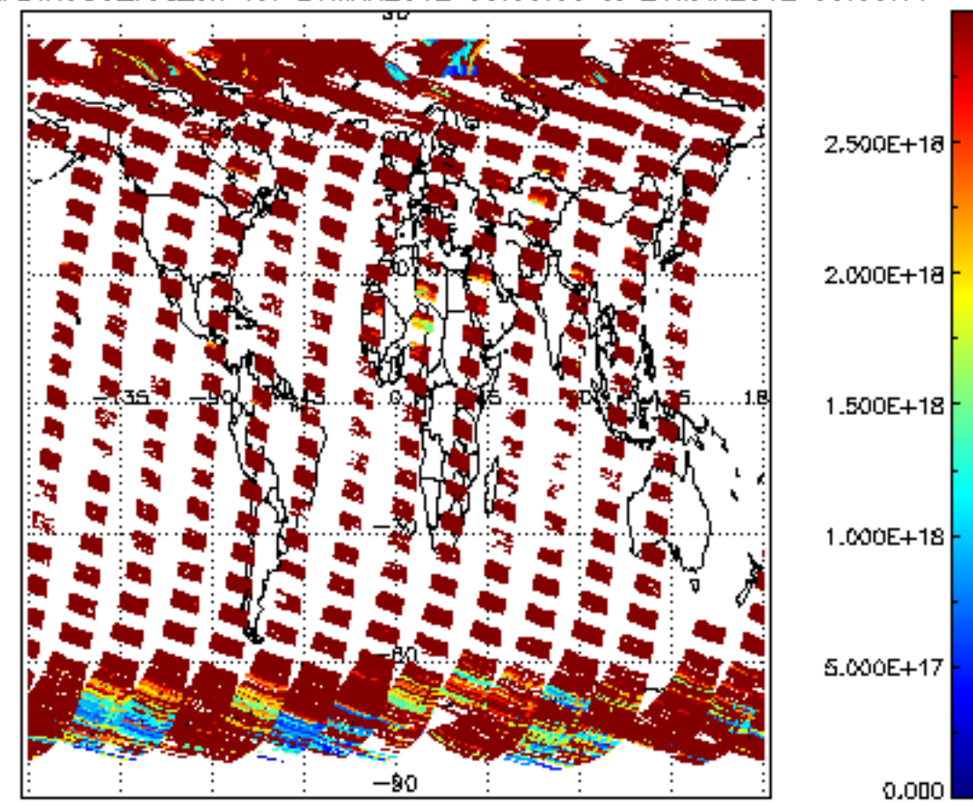
SCIOL2P_NADIR3CO_vcd_err for 20MAR2012 00:00:00 to 21MAR2012 00:00:00
