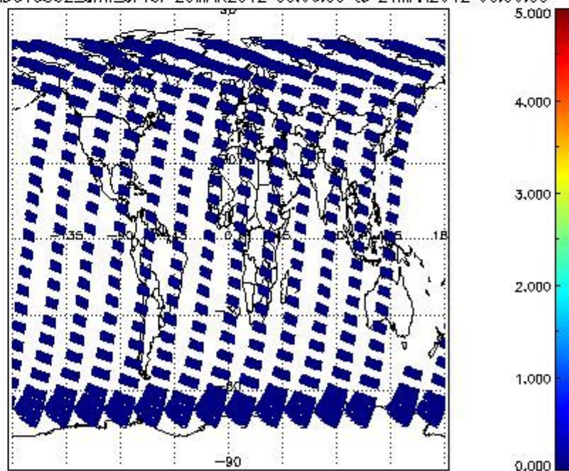
SCIOL2P_NADUV5SO2_amf_cl for 20MAR2012 00:00:00 to 21MAR2012 00:00:00
