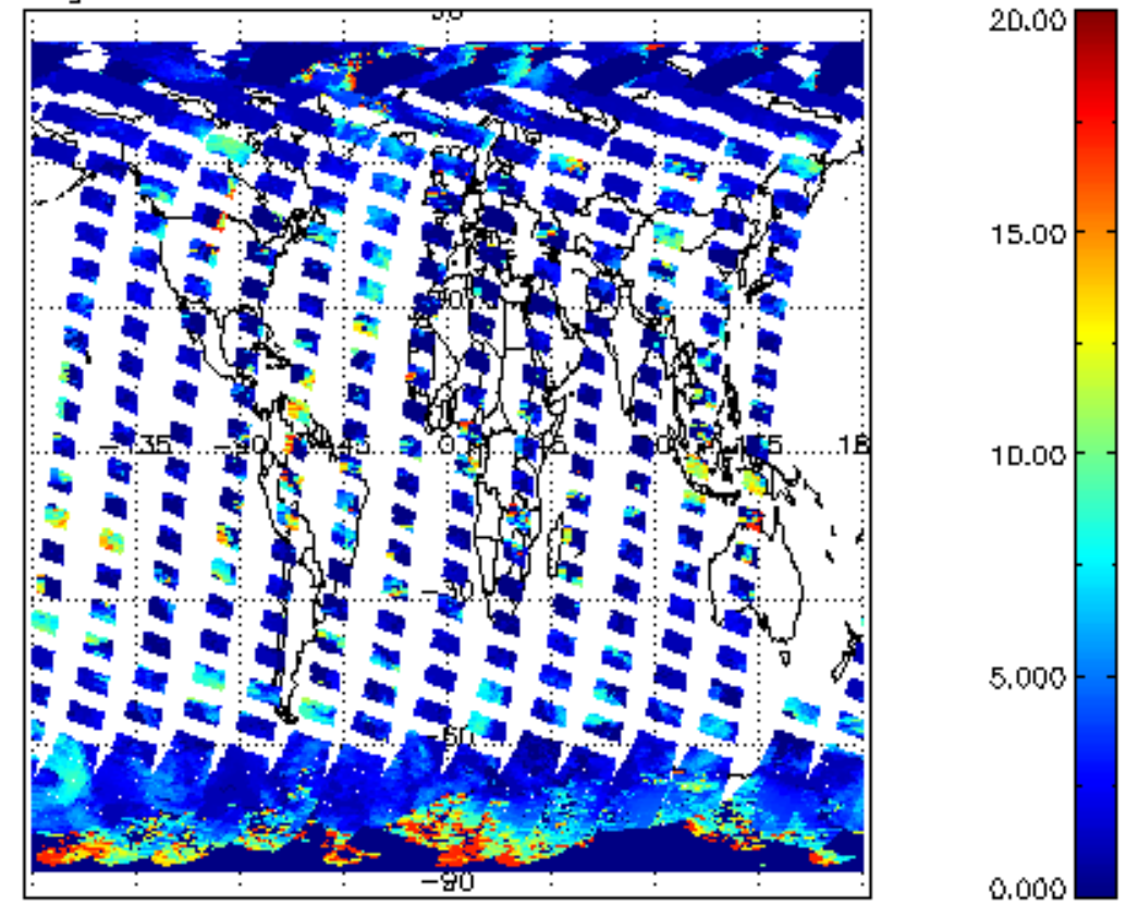
cL_top_height for 20MAR2012 00:00:00 to 21MAR2012 00:00:00
