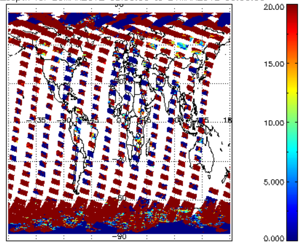
cL_opt_depth for 20MAR2012 00:00:00 to 21MAR2012 00:00:00
