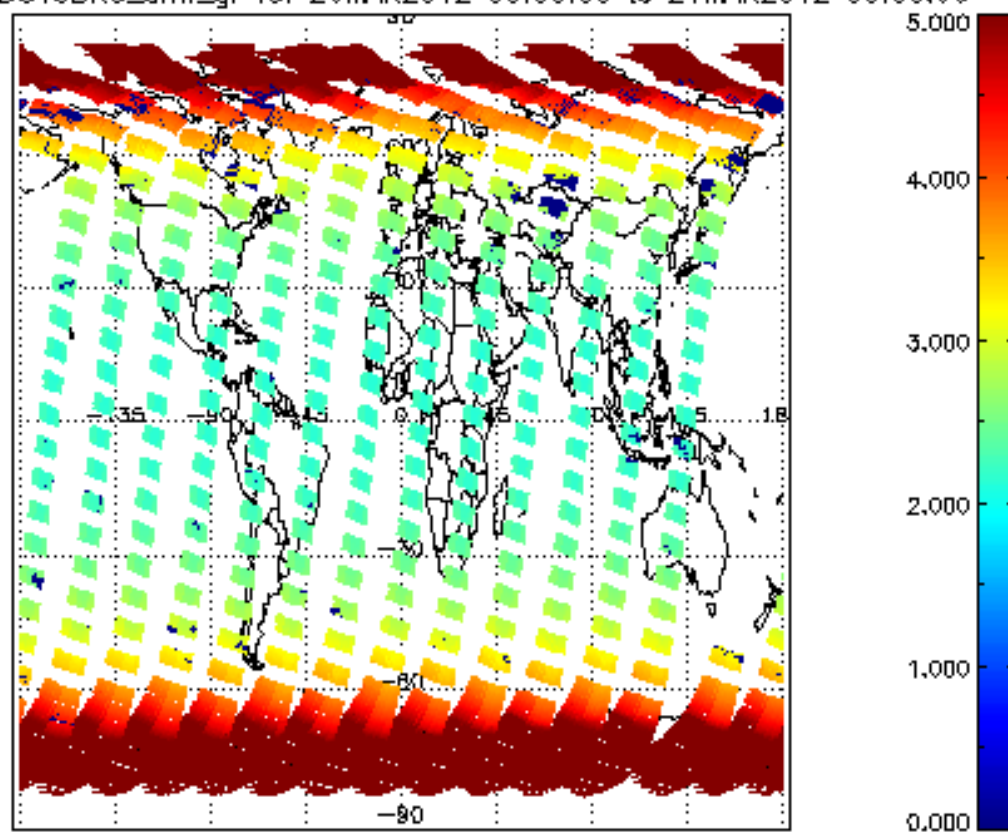
SCIOL2P_NADUV3BRO_amf_gr for 20MAR2012 00:00:00 to 21MAR2012 00:00:00
