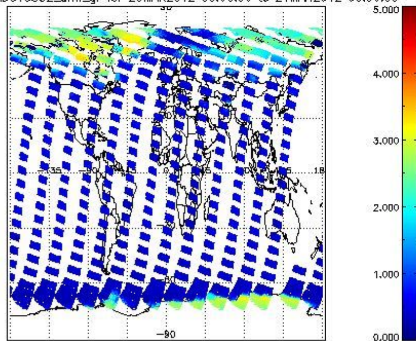
SCIOL2P_NADUV5SO2_amf_gr for 20MAR2012 00:00:00 to 21MAR2012 00:00:00
