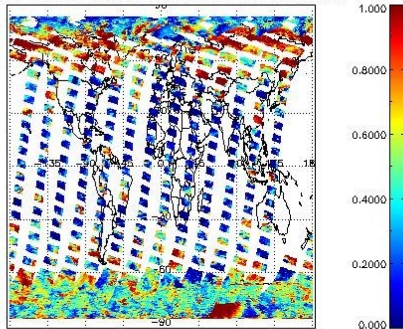
cL_frac for 20MAR2012 00:00:00 to 21MAR2012 00:00:00
