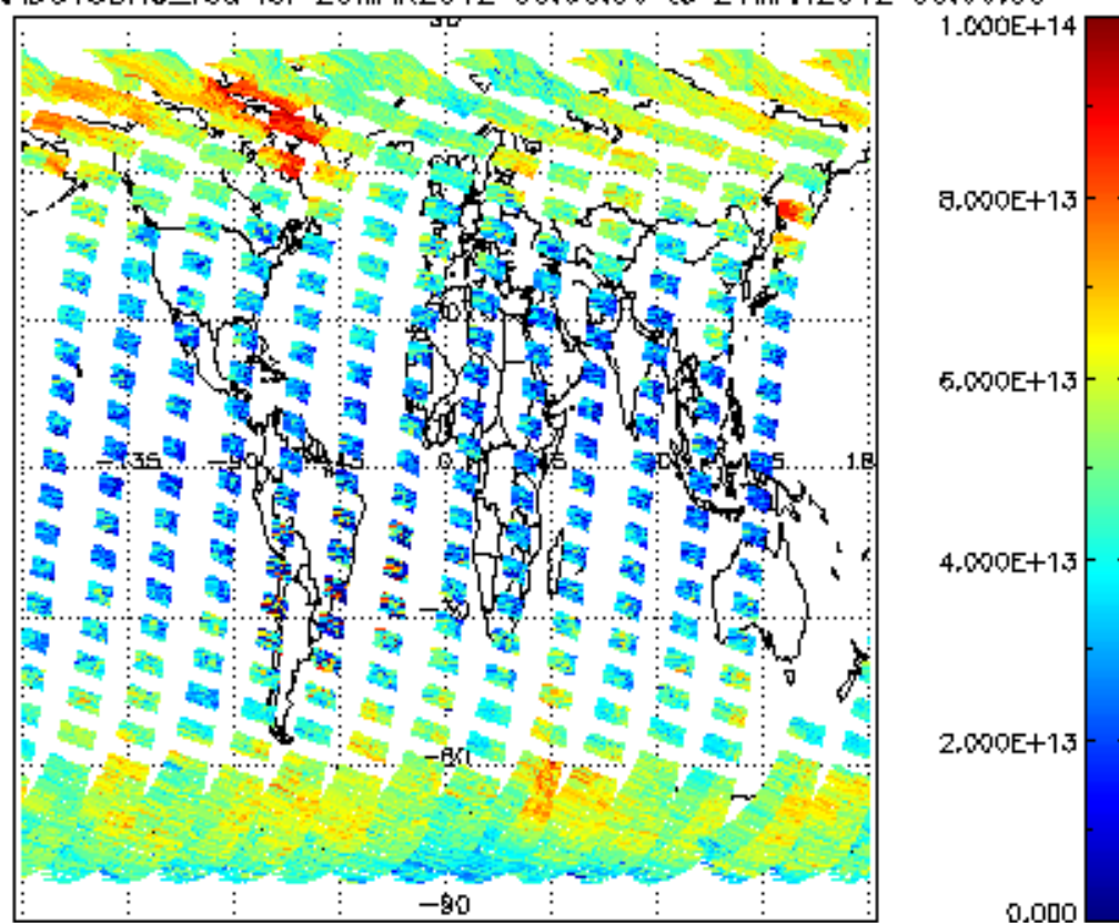
SCIOL2P_NADUV3BRO_vcd for 20MAR2012 00:00:00 to 21MAR2012 00:00:00
