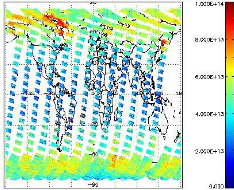
SCIOL2P_NADUV3BRO_vcd for 20MAR2012 00:00:00 to 21MAR2012 00:00:00
