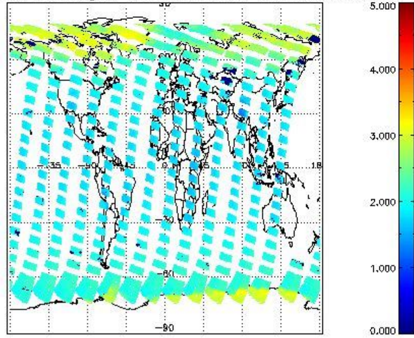
SCIOL2P_NADUV7S02_amf_gr for 20MAR2012 00:00:00 to 21MAR2012 00:00:00
