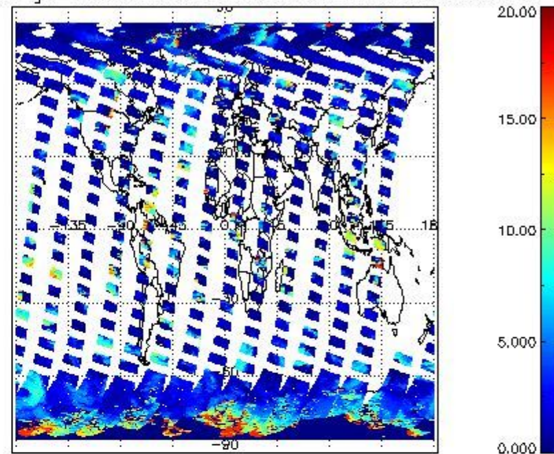
cL_top_height for 20MAR2012 00:00:00 to 21MAR2012 00:00:00
