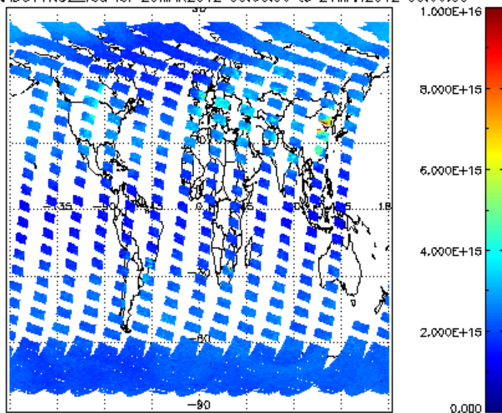
SCIOL2P_NADUV1NO2_vcd for 20MAR2012 00:00:00 to 21MAR2012 00:00:00
