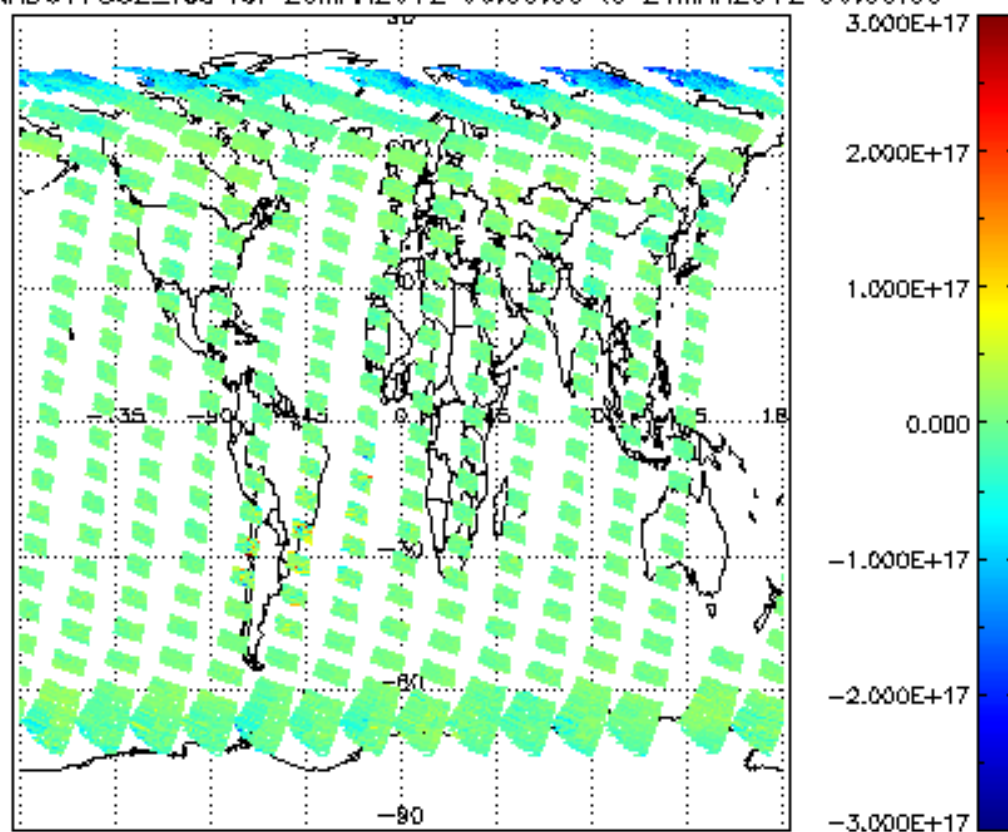
SCIOL2P_NADUV7S02_vcd for 20MAR2012 00:00:00 to 21MAR2012 00:00:00
