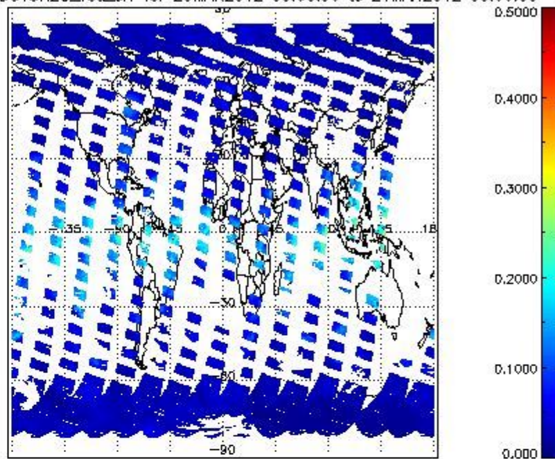
SCIOL2P_NADUV8H2O_vcd_err for 20MAR2012 00:00:00 to 21MAR2012 00:00:00
