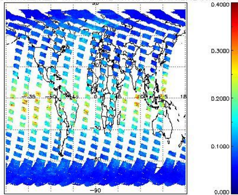
SCIOL2P_NADUV1NO2_vcd_err for 20MAR2012 00:00:00 to 21MAR2012 00:00:00
