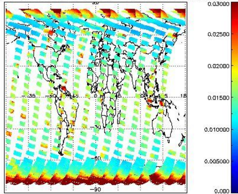
SCIOL2P_NADUV003_vcd_err for 20MAR2012 00:00:00 to 21MAR2012 00:00:00
