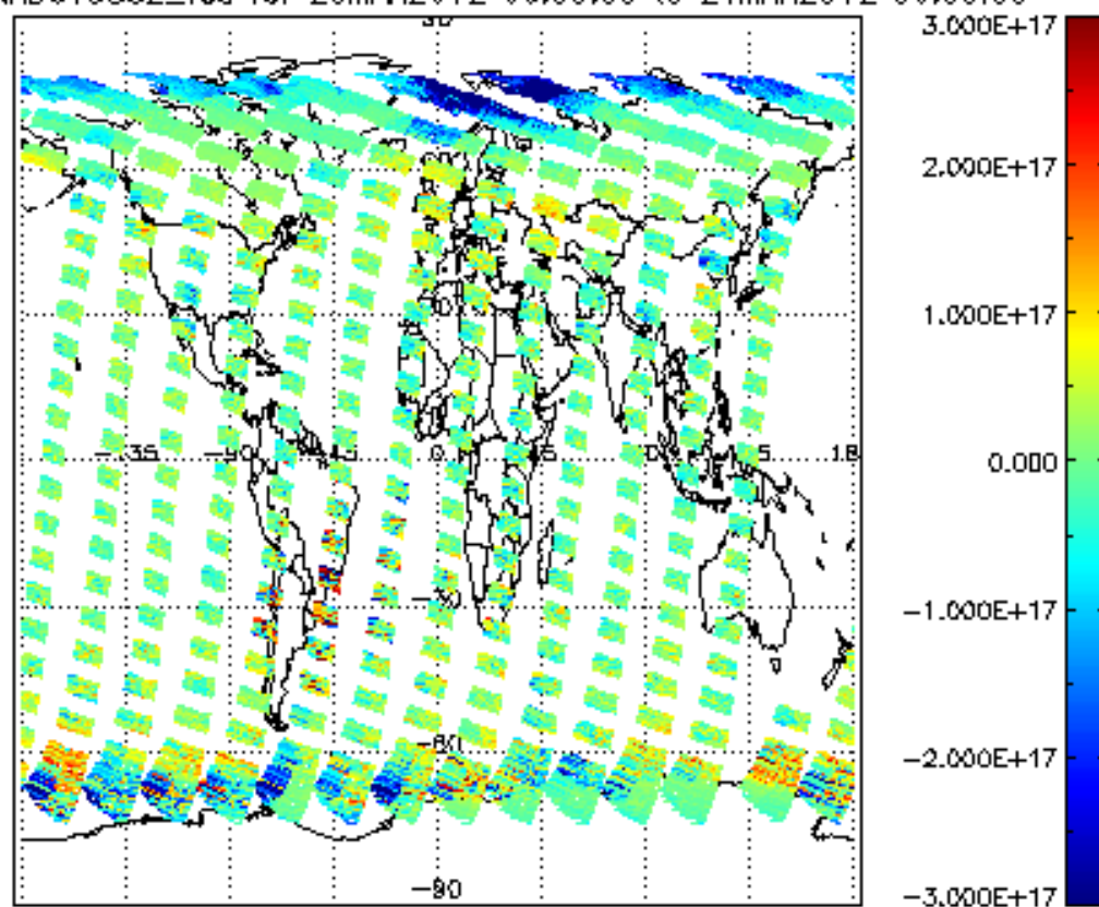
SCIOL2P_NADUV5S02_vcd for 20MAR2012 00:00:00 to 21MAR2012 00:00:00
