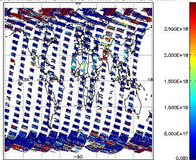
SCIDL2P_NADIR3CO_vcd for 20MAR2012 00:00:00 to 21MAR2012 00:00:00
