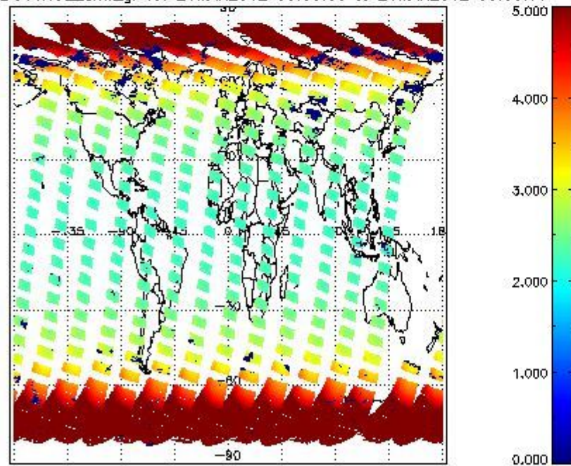
SCIOL2P_NADUV1NO2_amf_gr for 20MAR2012 00:00:00 to 21MAR2012 00:00:00
