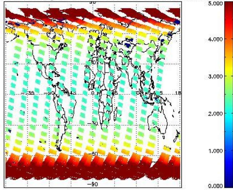
SCIOL2P_NADUV3BRO_amf_gr for 20MAR2012 00:00:00 to 21MAR2012 00:00:00
