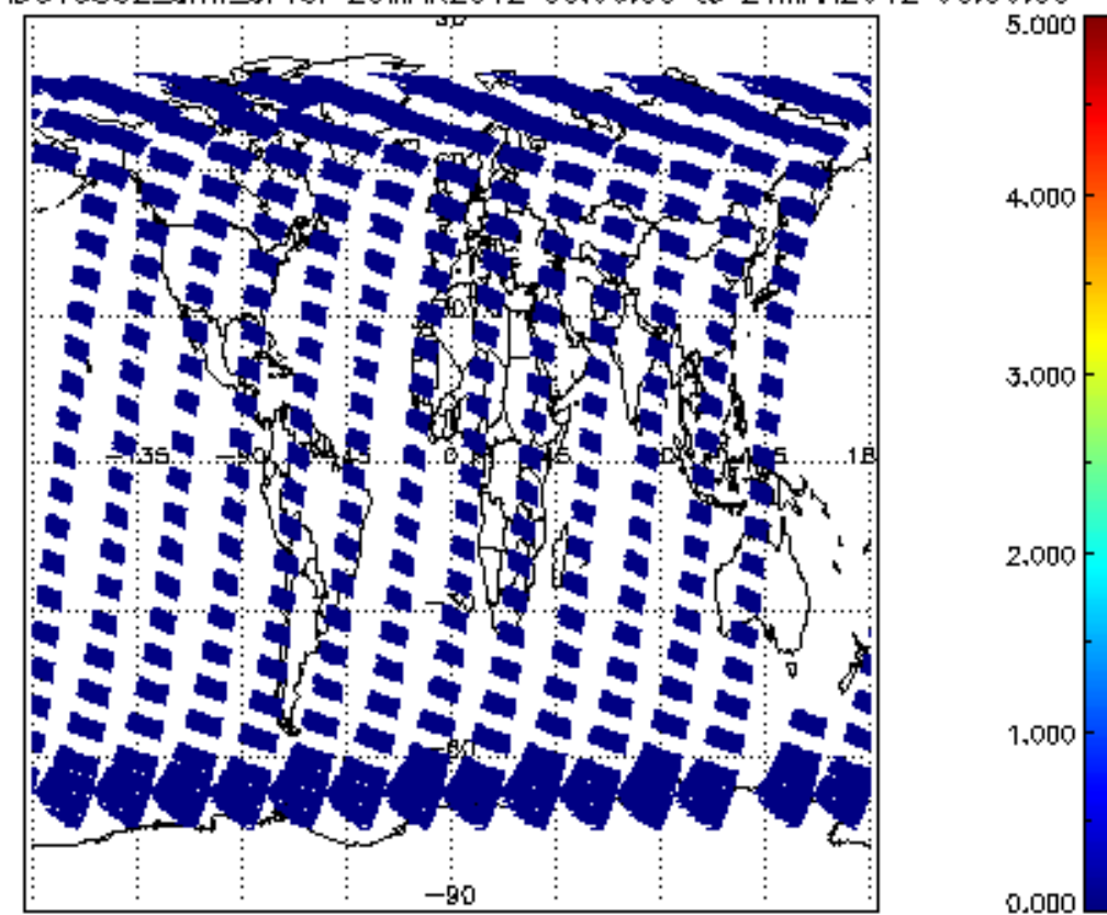
SCIOL2P_NADUV5S02_amf_cl for 20MAR2012 00:00:00 to 21MAR2012 00:00:00
