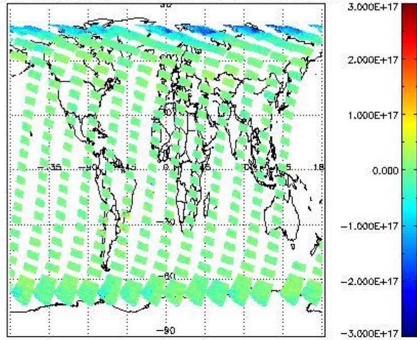
SCIOL2P_NADUV7S02_vcd for 20MAR2012 00:00:00 to 21MAR2012 00:00:00
