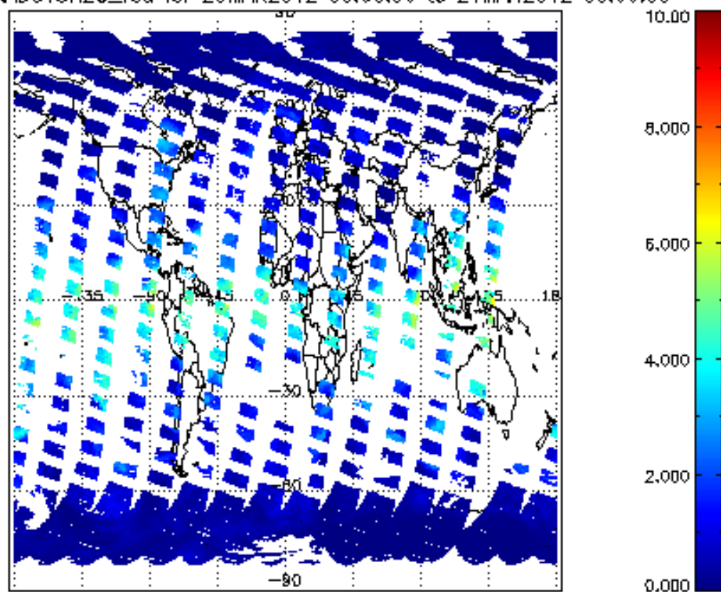
SCIOL2P_NADUV8H2O_vcd for 20MAR2012 00:00:00 to 21MAR2012 00:00:00
