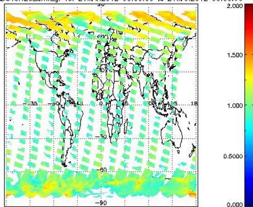
SCIOL2P_NADUV8H2O_arnf_gr for 20MAR2012 00:00:00 to 21MAR2012 00:00:00
