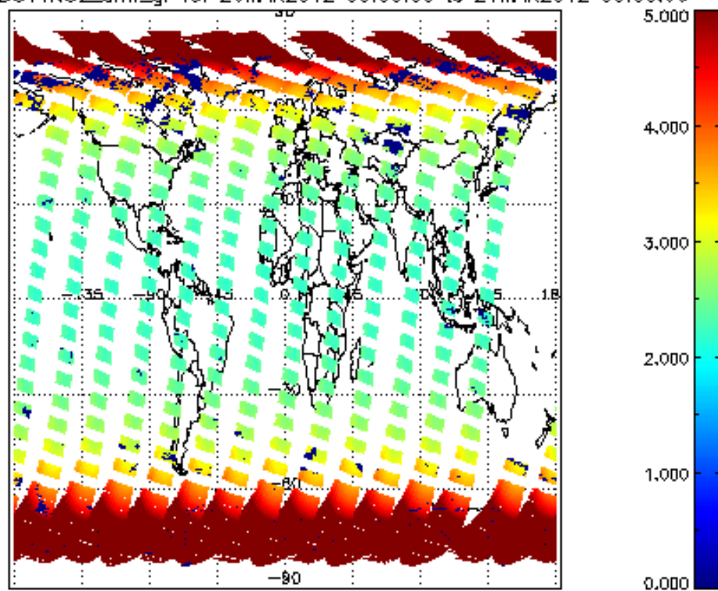
SCIOL2P_NADUV1NO2_amf_gr for 20MAR2012 00:00:00 to 21MAR2012 00:00:00
