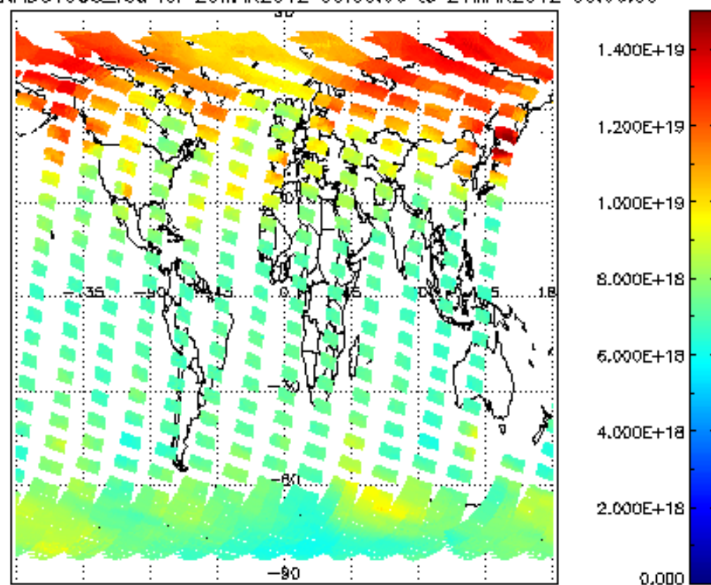
SCIOL2P_NADUV003_vcd for 20MAR2012 00:00:00 to 21MAR2012 00:00:00
