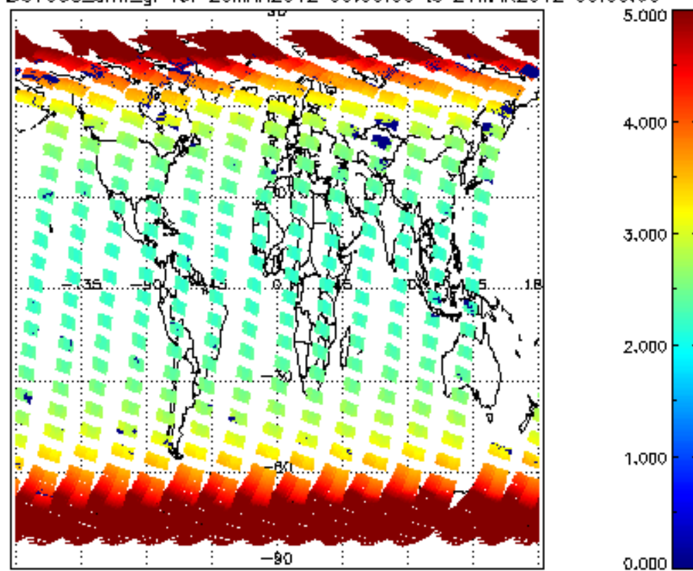
SCIOL2P_NADUV003_arnf_gr for 20MAR2012 00:00:00 to 21MAR2012 00:00:00
