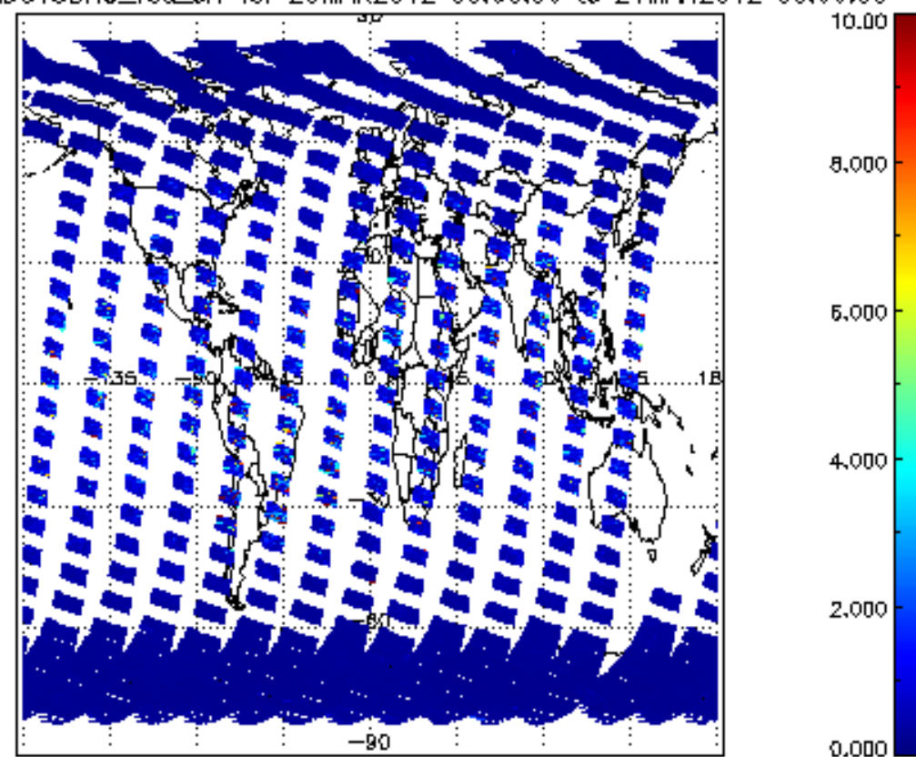
SCIOL2P_NADUV3BRO_vcd_Lerr for 20MAR2012 00:00:00 to 21MAR2012 00:00:00
