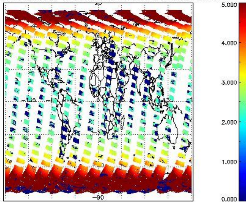
SCIOL2P_NADUV1NO2_amf_cl for 18MAR2012 00:00:00 to 19MAR2012 00:00:00
