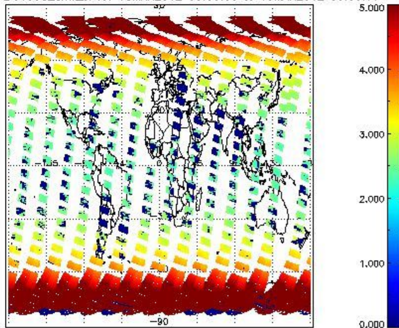
SCIOL2P_NADUV003_amf_cl for 18MAR2012 00:00:00 to 19MAR2012 00:00:00
