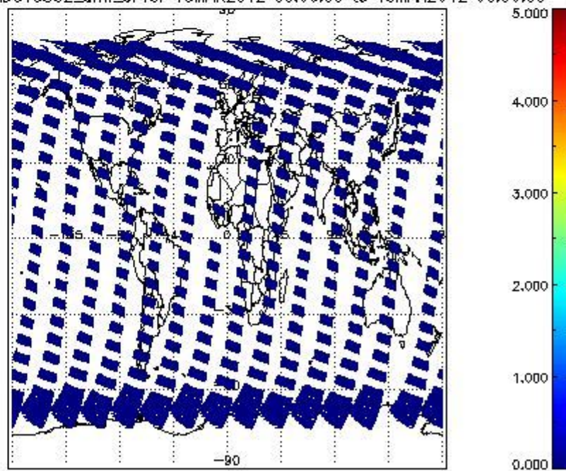
SCIOL2P_NADUV5S02_amf_cl for 18MAR2012 00:00:00 to 19MAR2012 00:00:00
