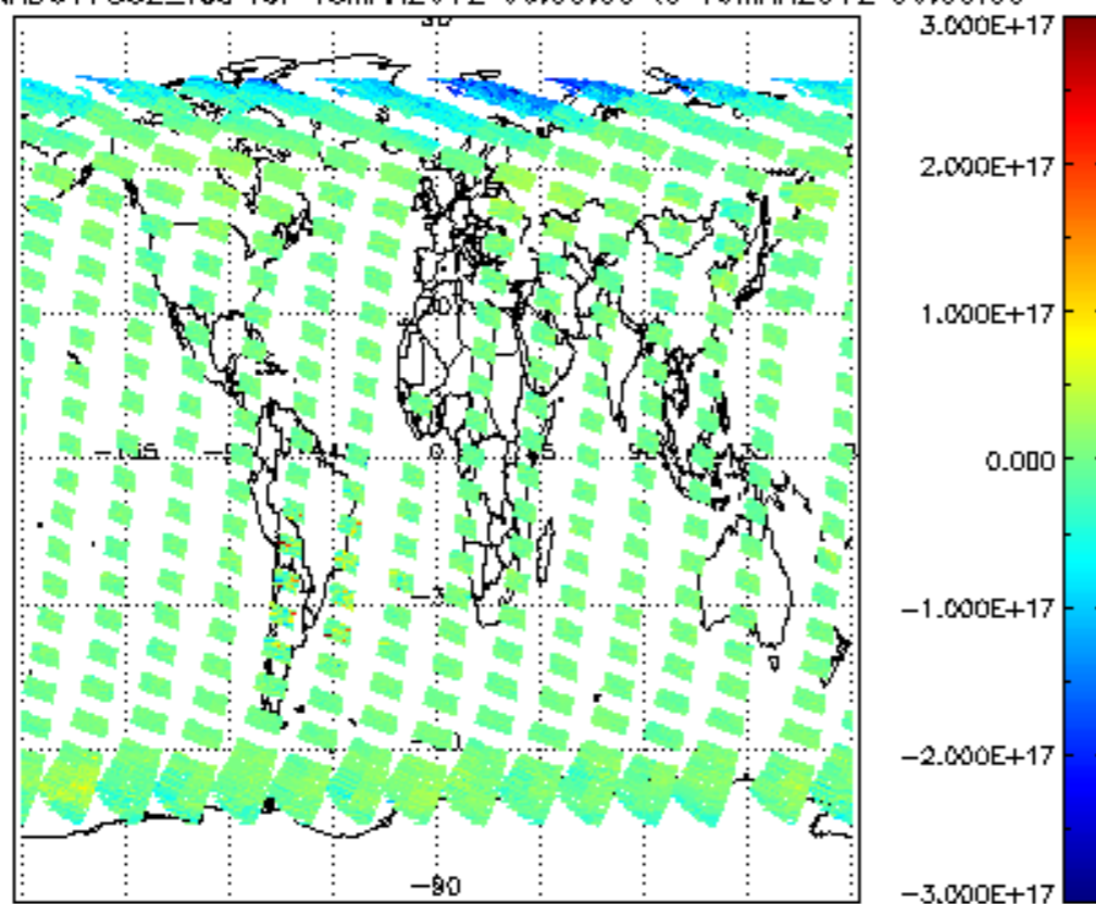
SCIOL2P_NADUV7S02_vcd for 18MAR2012 00:00:00 to 19MAR2012 00:00:00
