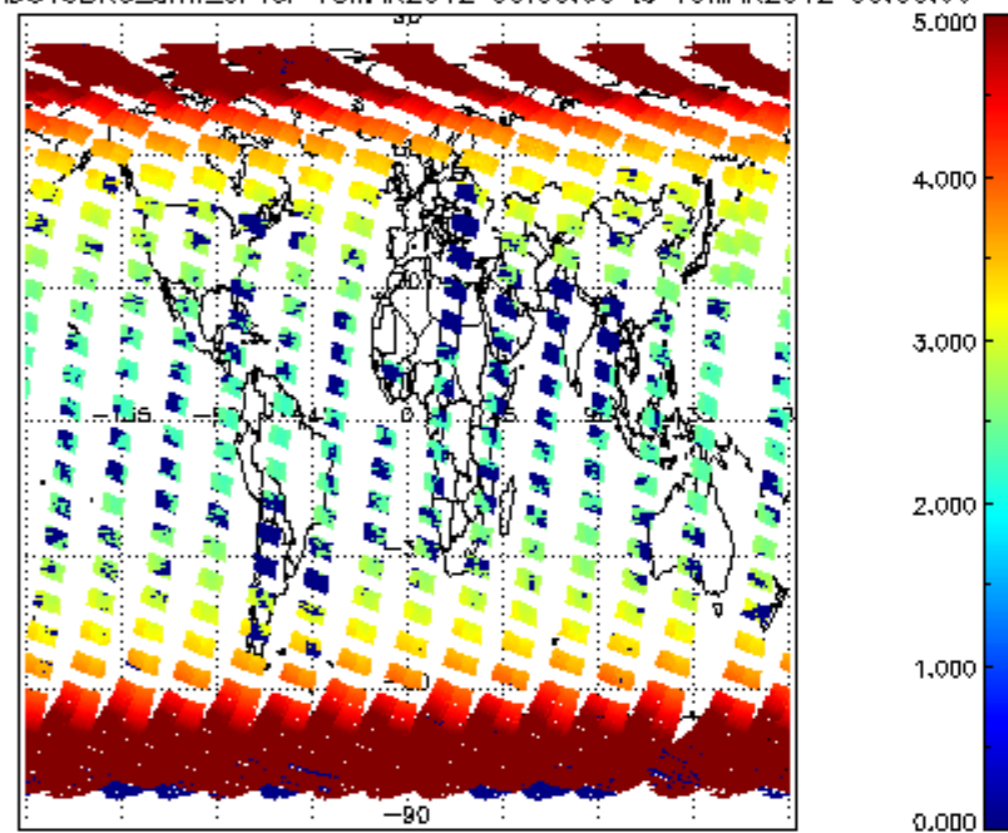
SCIOL2P_NADUV3BRO_amf_cl for 18MAR2012 00:00:00 to 19MAR2012 00:00:00
