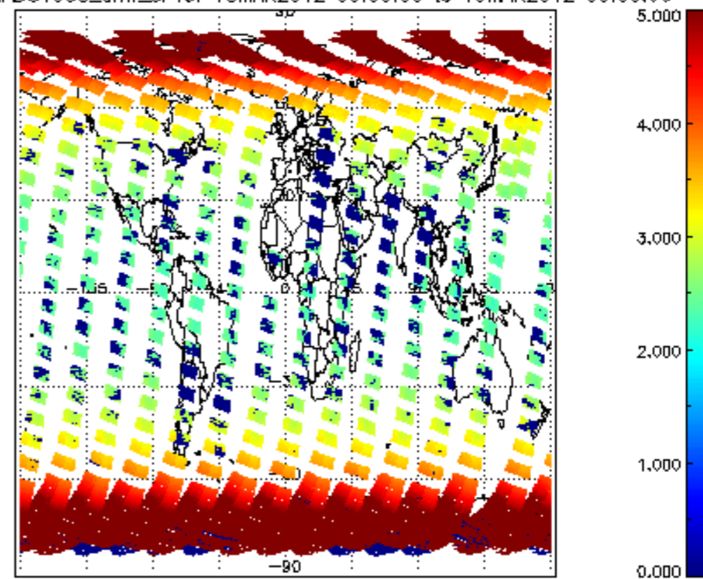
SCIOL2P_NADUV003_arnf_cl for 18MAR2012 00:00:00 to 19MAR2012 00:00:00
