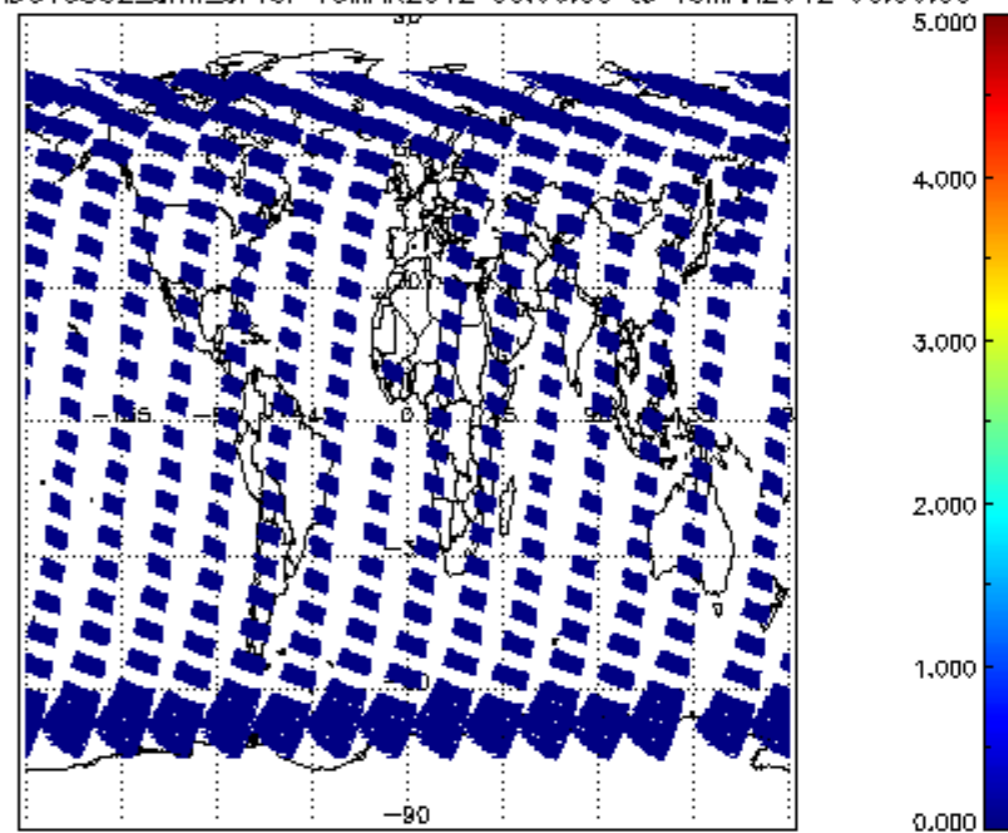
SCIOL2P_NADUV5S02_amf_cl for 18MAR2012 00:00:00 to 19MAR2012 00:00:00
