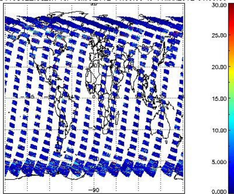
SCIOL2P_NADUV5S02_vcd_err for 18MAR2012 00:00:00 to 19MAR2012 00:00:00
