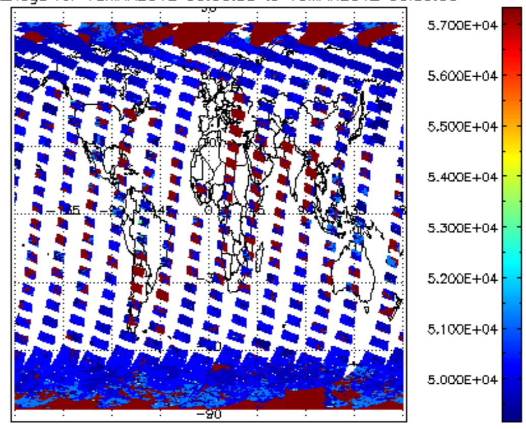
cloud_flags for 18MAR2012 00:00:00 to 19MAR2012 00:00:00
