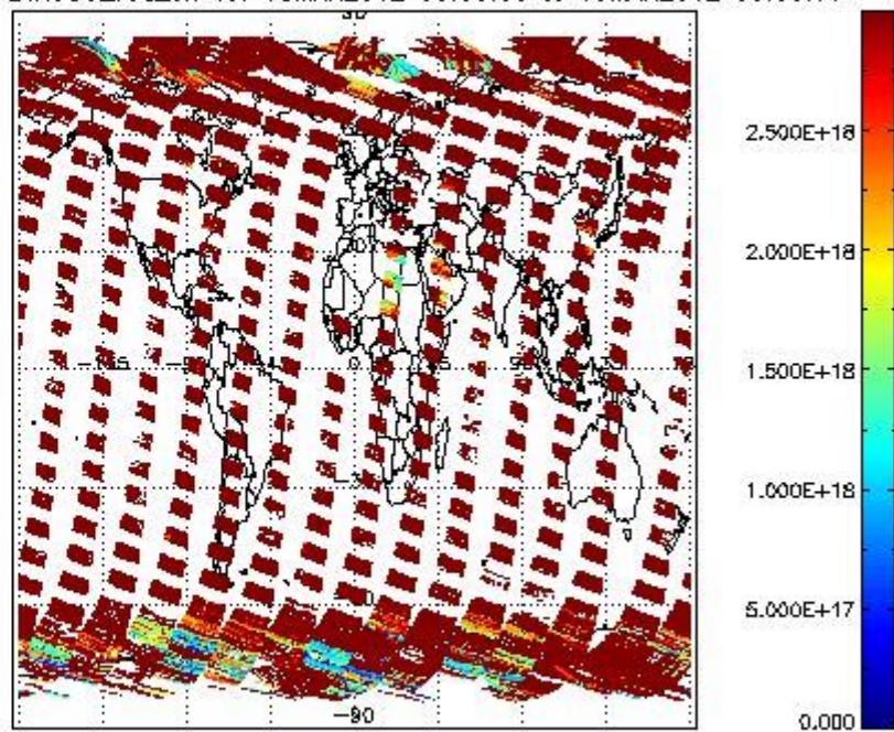
SCIDL2P_NADIR3CO_vcd_err for 18MAR2012 00:00:00 to 19MAR2012 00:00:00
