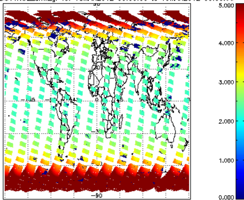
SCIOL2P_NADUV1NO2_amf_gr for 18MAR2012 00:00:00 to 19MAR2012 00:00:00
