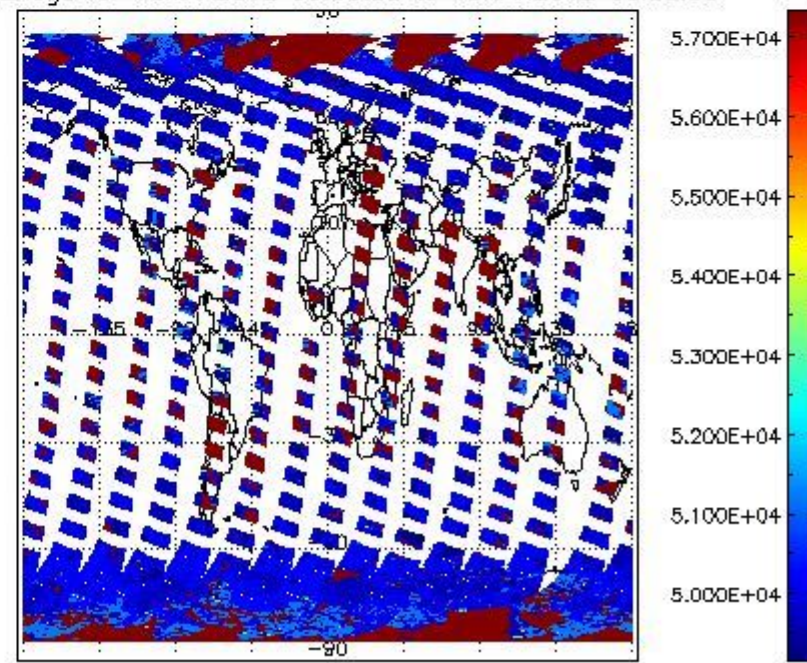
cloud_flags for 18MAR2012 00:00:00 to 19MAR2012 00:00:00
