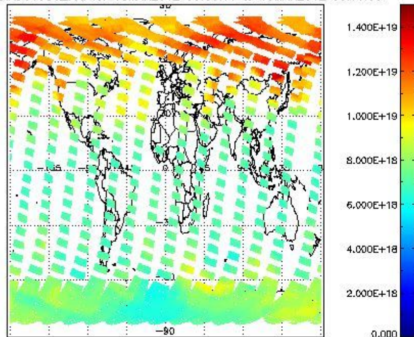
SCIOL2P_NADUV003_vcd for 18MAR2012 00:00:00 to 19MAR2012 00:00:00
