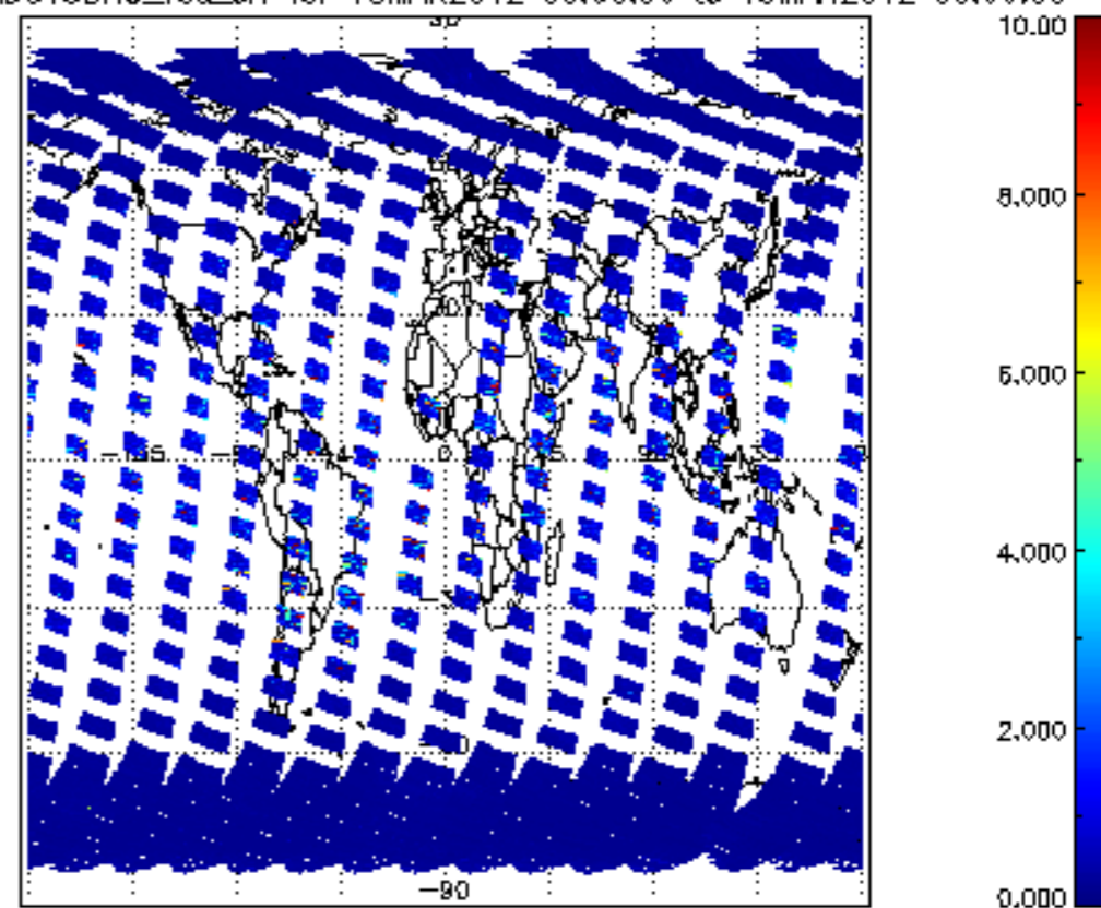
SCIOL2P_NADUV3BRO_vcd_err for 18MAR2012 00:00:00 to 19MAR2012 00:00:00
