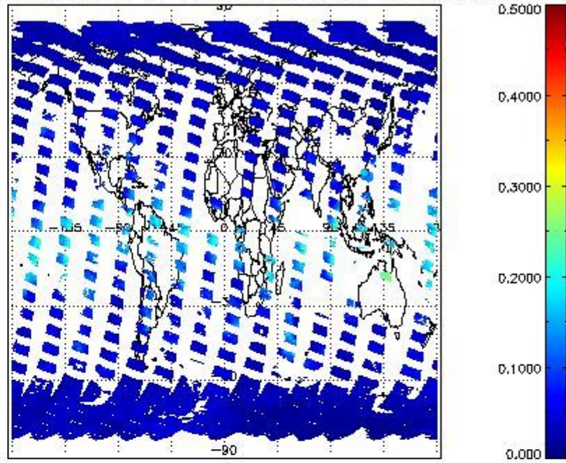
SCIOL2P_NADUV8H2O_vcd_err for 18MAR2012 00:00:00 to 19MAR2012 00:00:00
