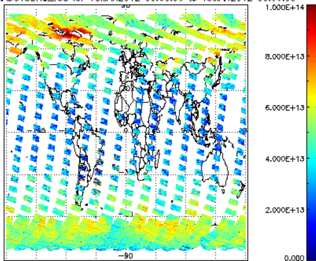
SCIOL2P_NADUV3BRO_vcd for 18MAR2012 00:00:00 to 19MAR2012 00:00:00
