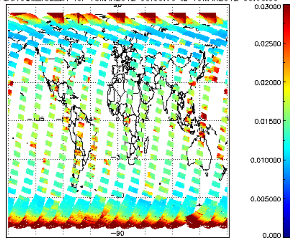
SCIOL2P_NADUV003_vcd_err for 18MAR2012 00:00:00 to 19MAR2012 00:00:00
