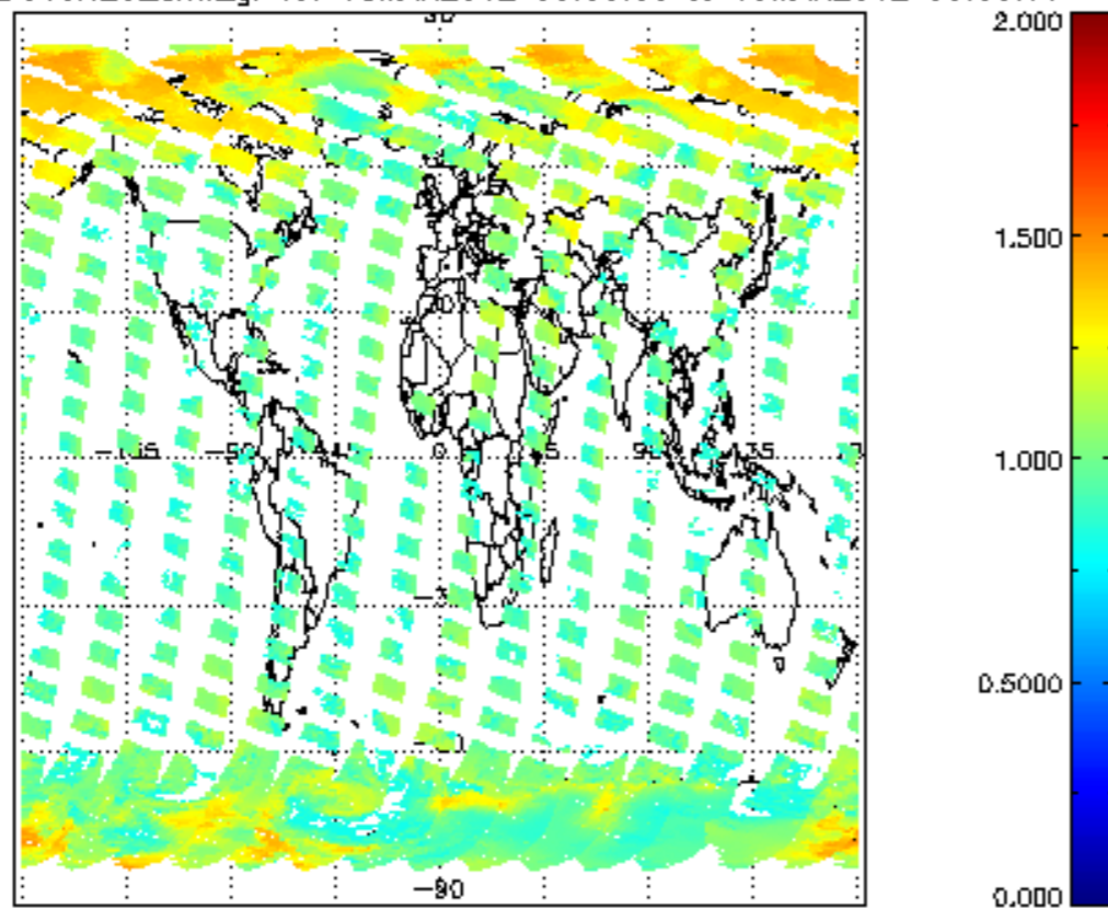
SCIOL2P_NADUV8H2O_arnf_gr for 18MAR2012 00:00:00 to 19MAR2012 00:00:00
