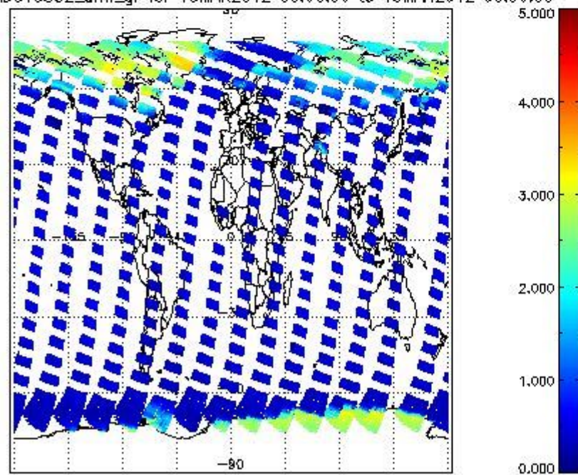
SCIOL2P_NADUV5S02_amf_gr for 18MAR2012 00:00:00 to 19MAR2012 00:00:00
