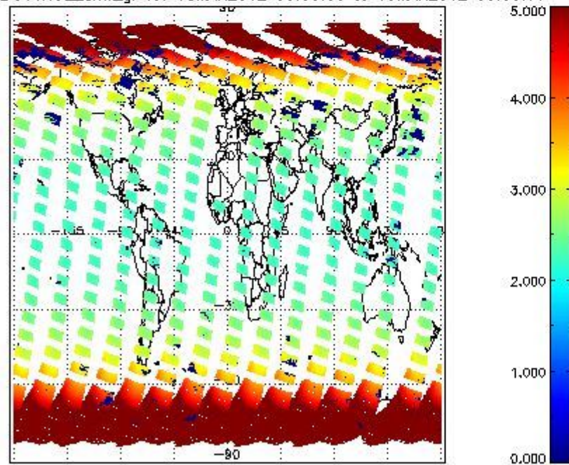
SCIOL2P_NADUV1NO2_amf_gr for 18MAR2012 00:00:00 to 19MAR2012 00:00:00
