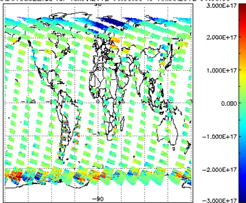
SCIOL2P_NADUV5S02_vcd for 18MAR2012 00:00:00 to 19MAR2012 00:00:00
