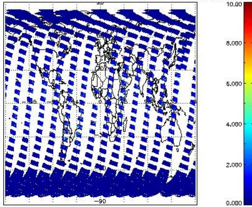
SCIOL2P_NADUV3BRO_vcd_err for 18MAR2012 00:00:00 to 19MAR2012 00:00:00
