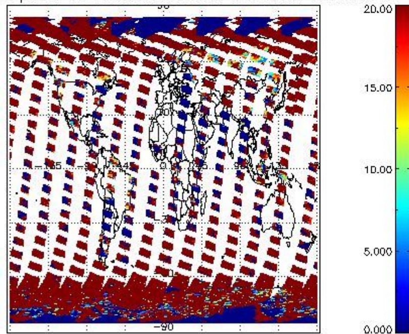
cL_opt_depth for 18MAR2012 00:00:00 to 19MAR2012 00:00:00
