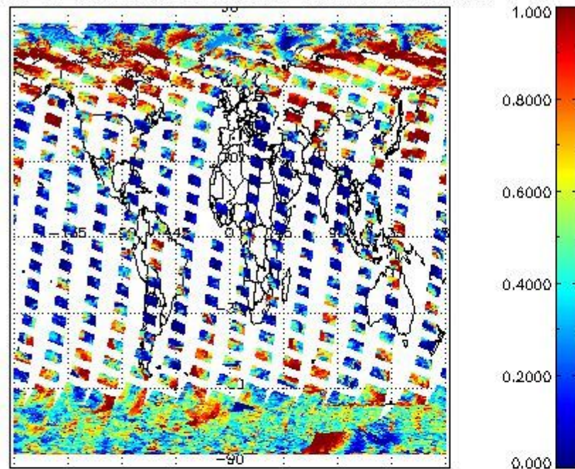
cL_frac for 18MAR2012 00:00:00 to 19MAR2012 00:00:00
