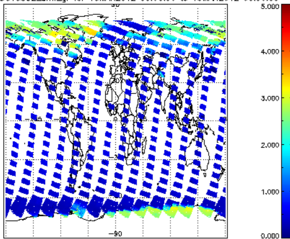
SCIOL2P_NADUV5S02_amf_gr for 18MAR2012 00:00:00 to 19MAR2012 00:00:00
