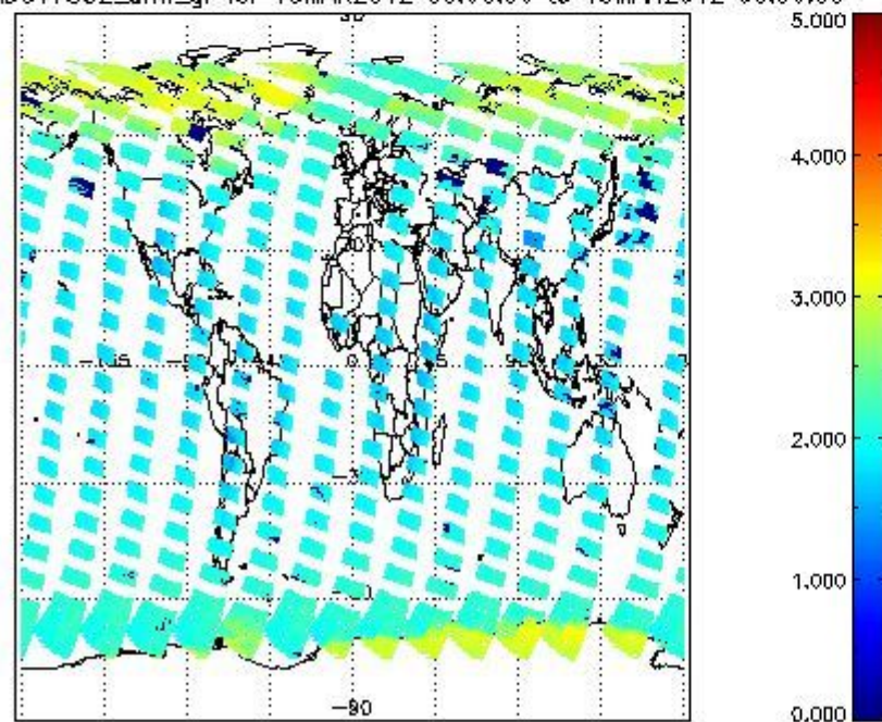
SCIOL2P_NADUV7S02_amf_gr for 18MAR2012 00:00:00 to 19MAR2012 00:00:00
