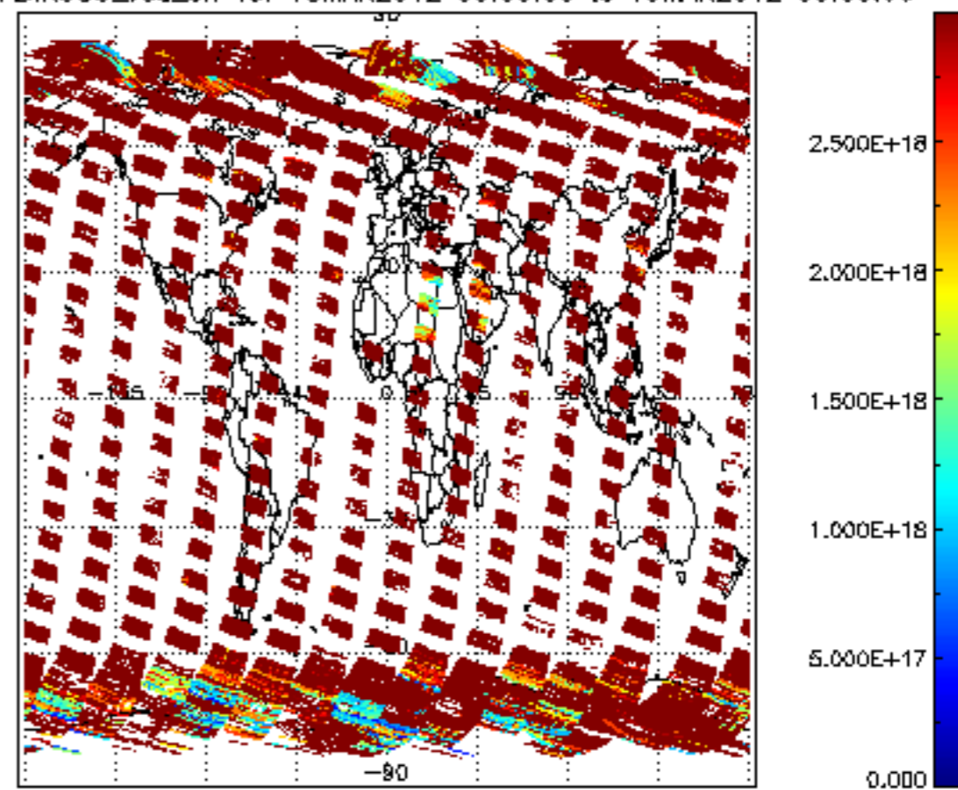
SCIOL2P_NADIR3CO_vcd_err for 18MAR2012 00:00:00 to 19MAR2012 00:00:00
