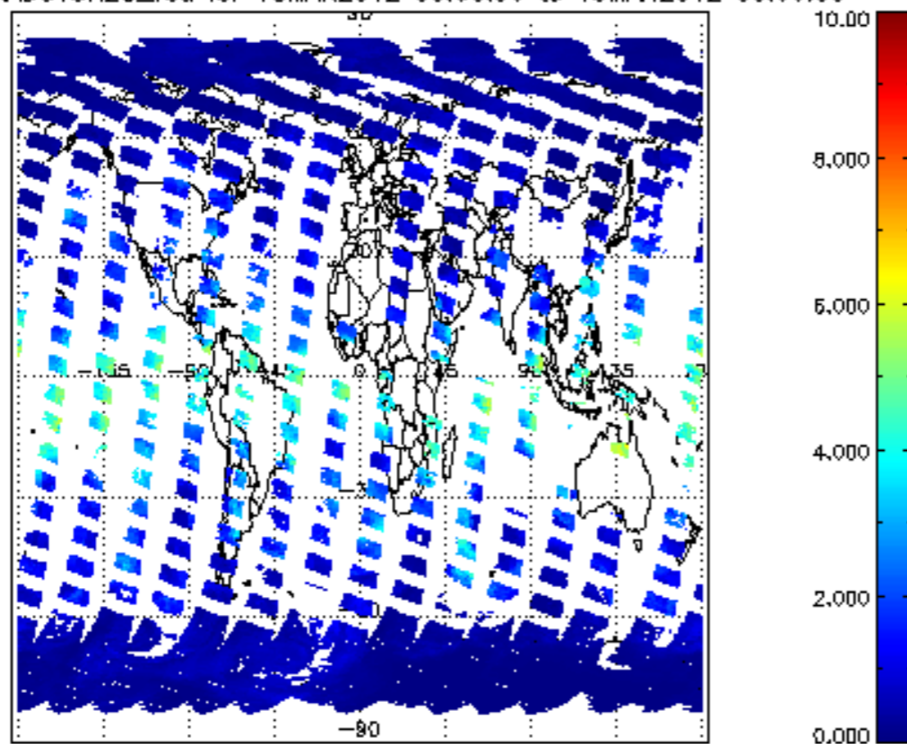
SCIOL2P_NADUV8H2O_vcd for 18MAR2012 00:00:00 to 19MAR2012 00:00:00
