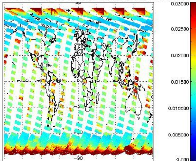
SCIOL2P_NADUV003_vcd_err for 18MAR2012 00:00:00 to 19MAR2012 00:00:00
