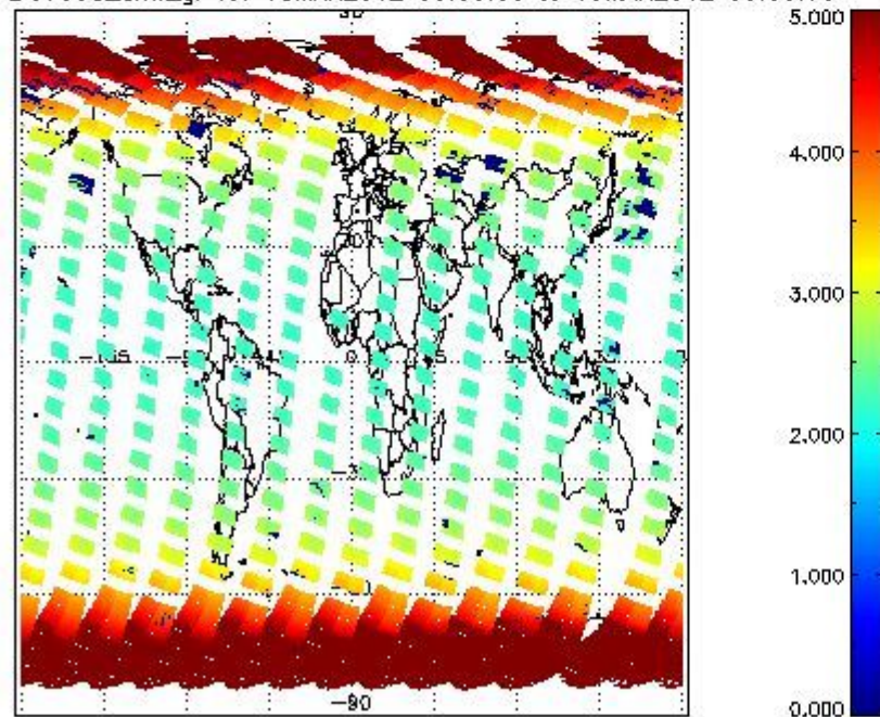
SCIOL2P_NADUV003_amf_gr for 18MAR2012 00:00:00 to 19MAR2012 00:00:00
