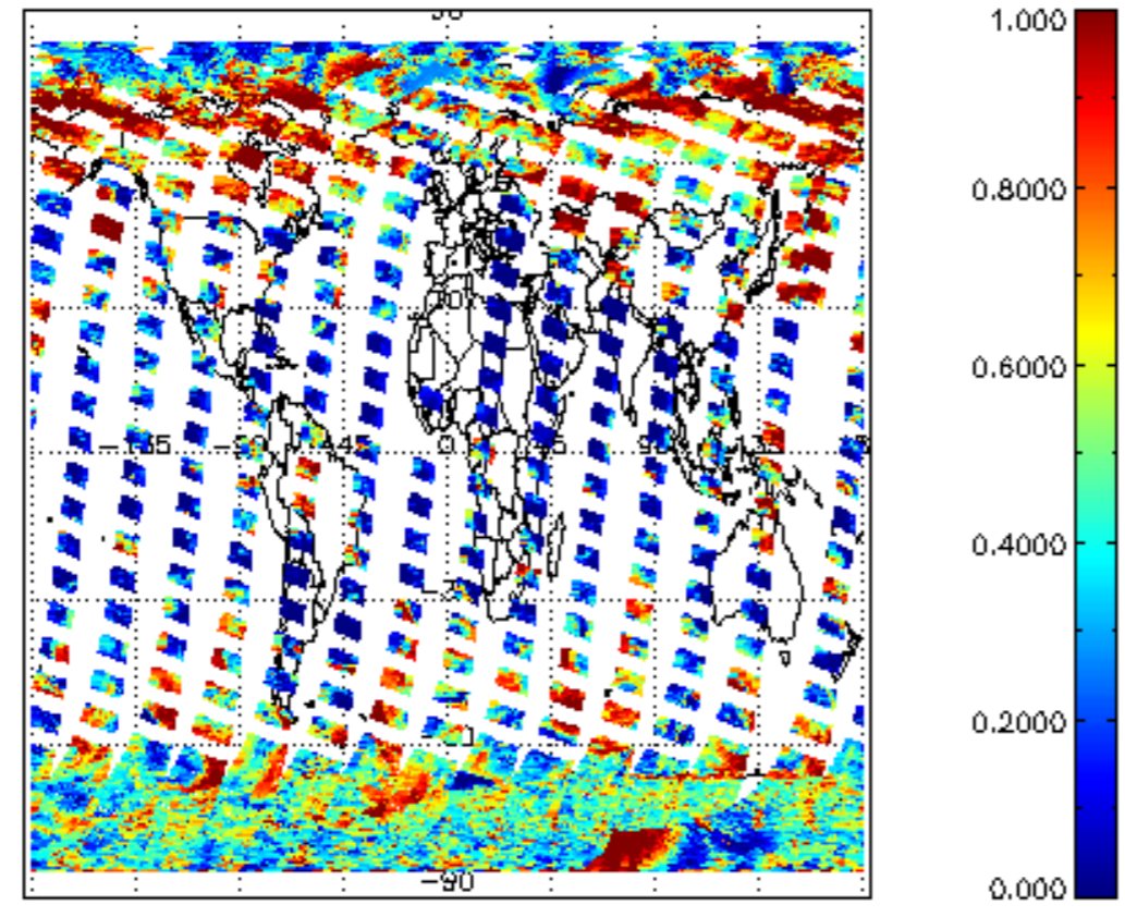
cL_frac for 18MAR2012 00:00:00 to 19MAR2012 00:00:00
