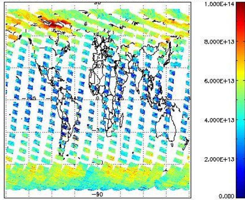
SCIOL2P_NADUV3BRO_vcd for 18MAR2012 00:00:00 to 19MAR2012 00:00:00
