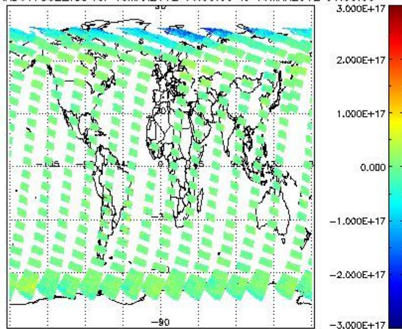
SCIOL2P_NADUV7S02_vcd for 18MAR2012 00:00:00 to 19MAR2012 00:00:00
