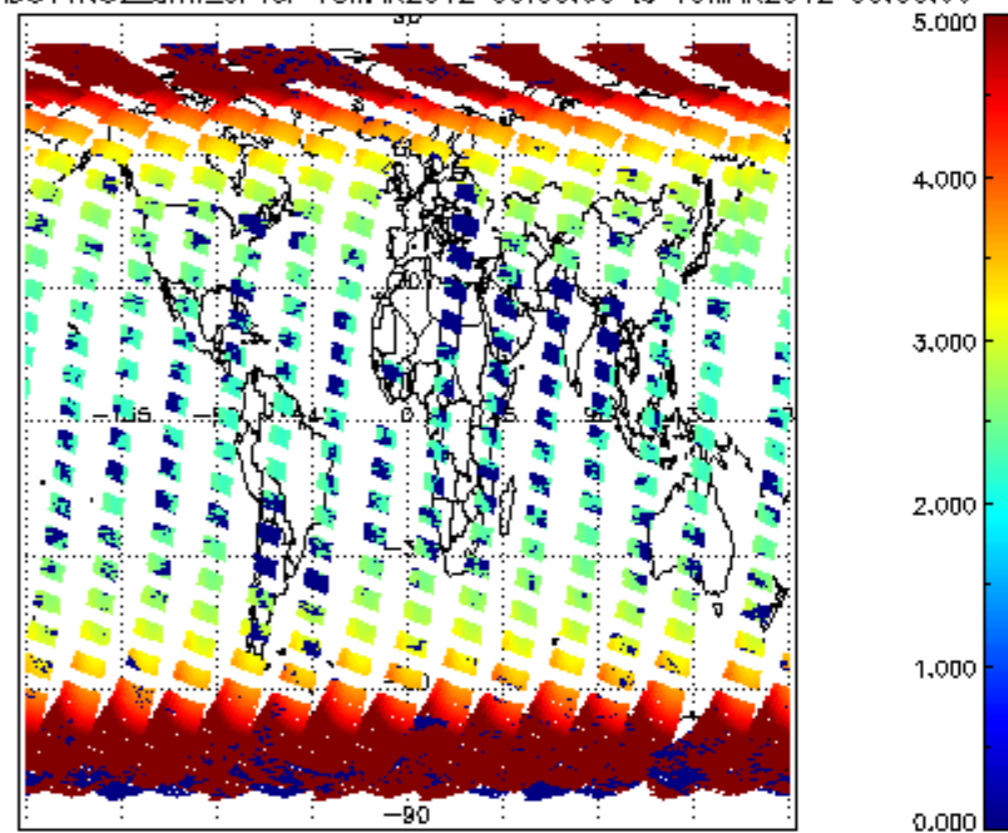
SCIOL2P_NADUV1NO2_amf_cl for 18MAR2012 00:00:00 to 19MAR2012 00:00:00
