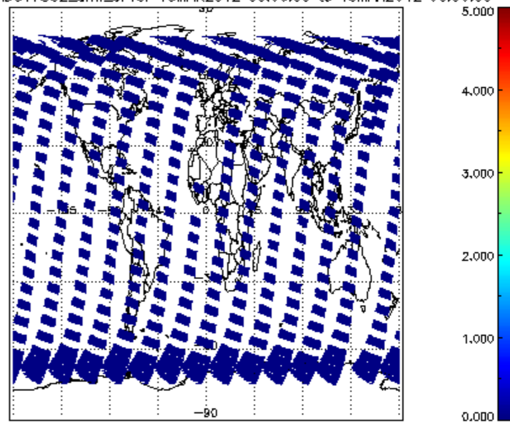
SCIOL2P_NADUV7S02_amf_cl for 18MAR2012 00:00:00 to 19MAR2012 00:00:00
