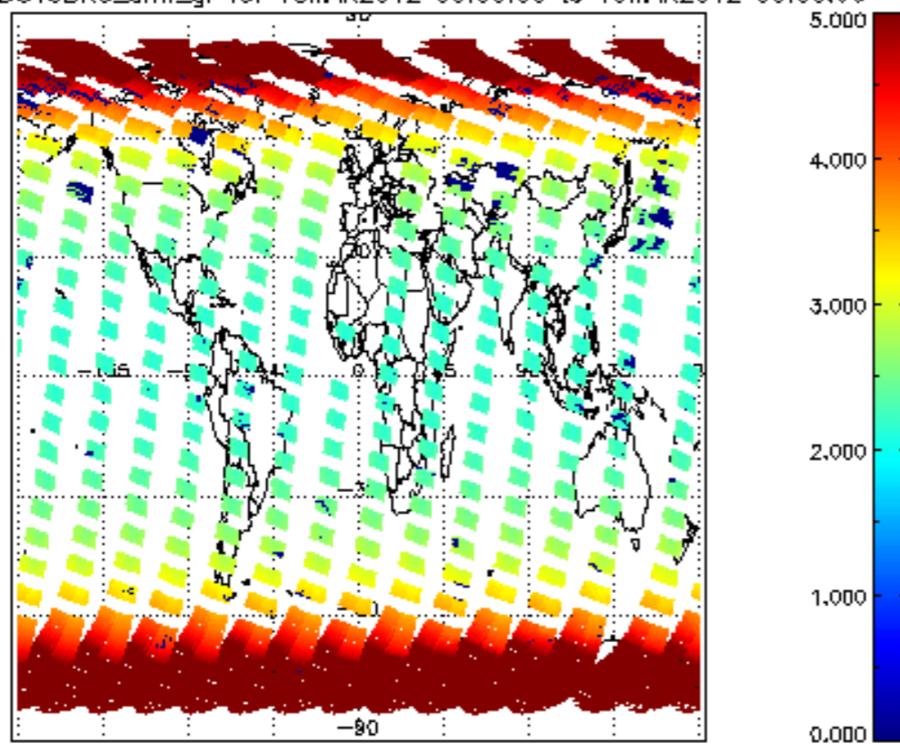
SCIOL2P_NADUV3BRO_amf_gr for 18MAR2012 00:00:00 to 19MAR2012 00:00:00
