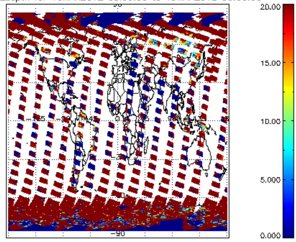
cL_opt_depth for 18MAR2012 00:00:00 to 19MAR2012 00:00:00
