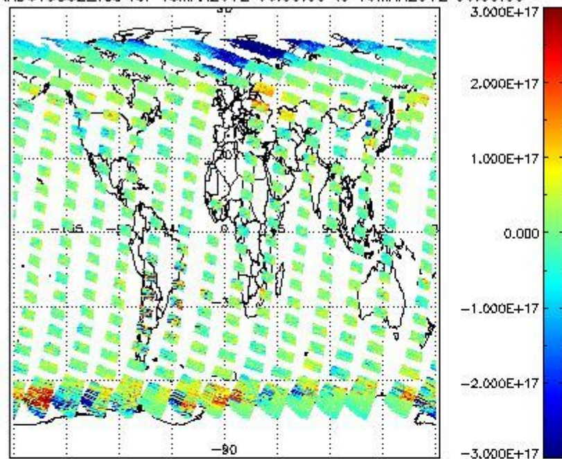
SCIOL2P_NADUV5S02_vcd for 18MAR2012 00:00:00 to 19MAR2012 00:00:00
