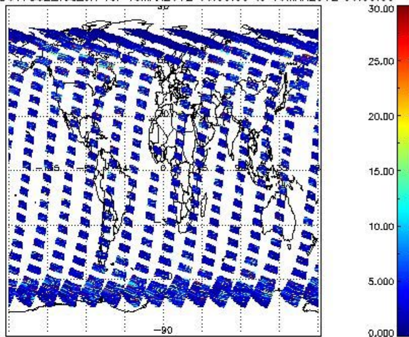
SCIOL2P_NADUV7S02_vcd_err for 18MAR2012 00:00:00 to 19MAR2012 00:00:00
