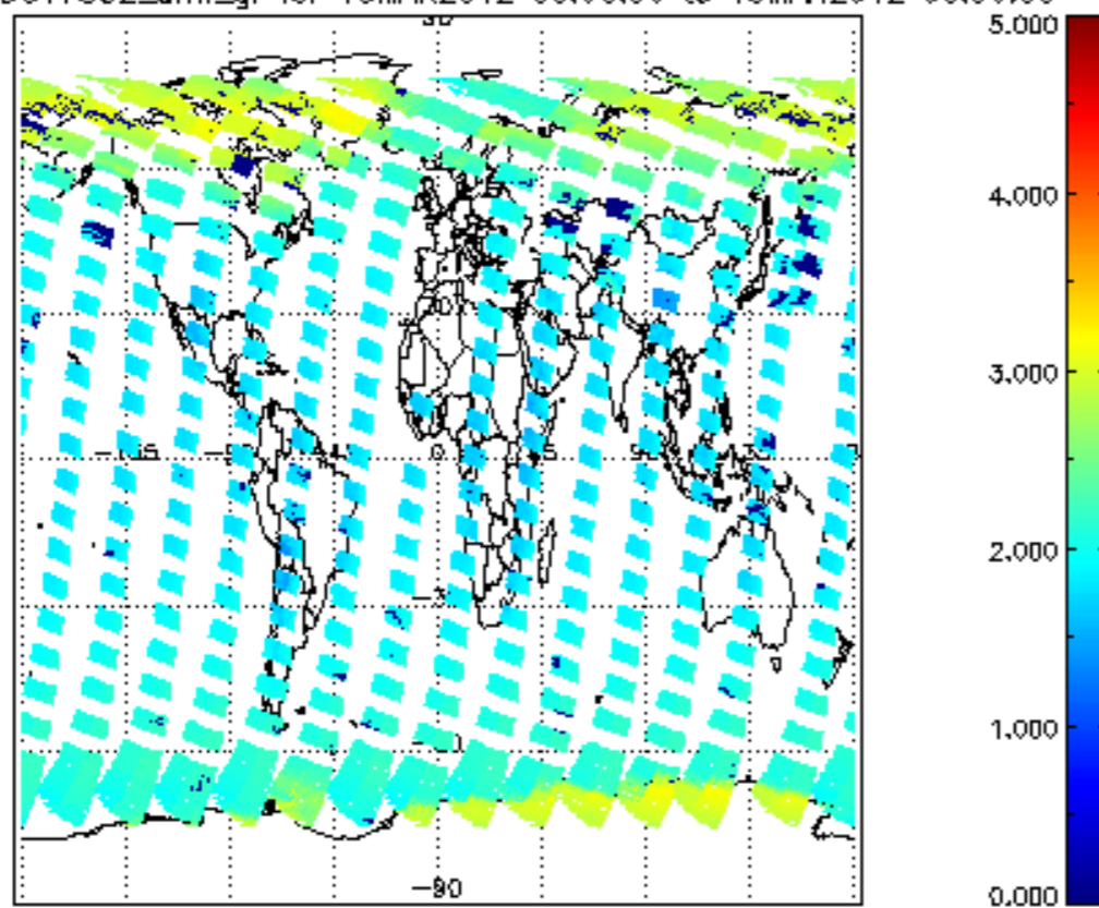
SCIOL2P_NADUV7S02_amf_gr for 18MAR2012 00:00:00 to 19MAR2012 00:00:00
