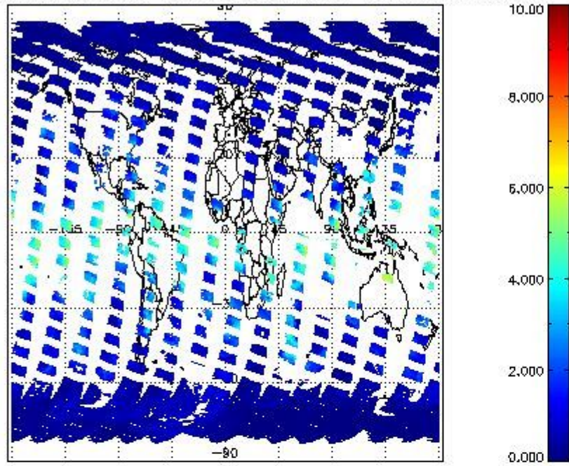
SCIOL2P_NADUV8H2O_vcd for 18MAR2012 00:00:00 to 19MAR2012 00:00:00
