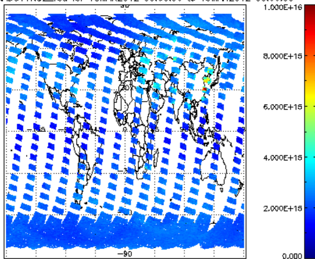
SCIOL2P_NADUV1NO2_vcd for 18MAR2012 00:00:00 to 19MAR2012 00:00:00
