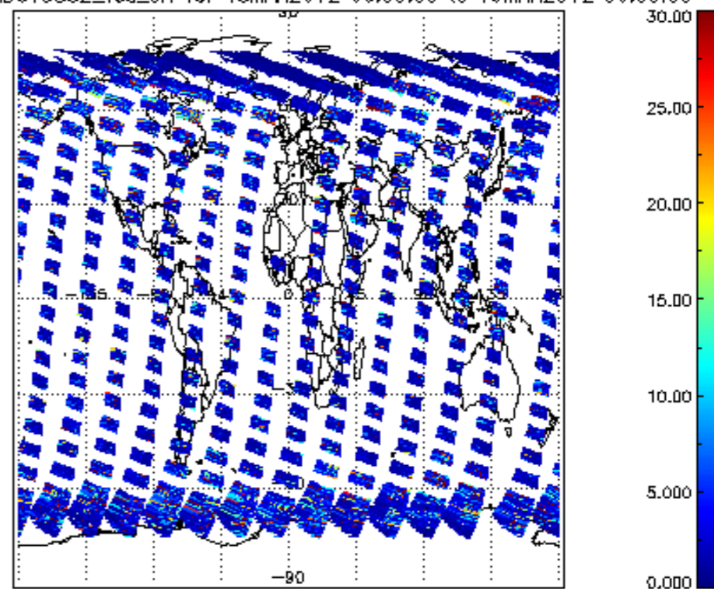
SCIOL2P_NADUV5S02_vcd_err for 18MAR2012 00:00:00 to 19MAR2012 00:00:00
