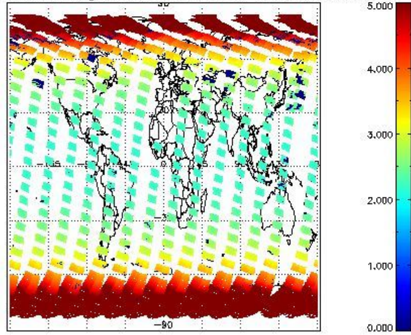
SCIOL2P_NADUV3BRO_amf_gr for 18MAR2012 00:00:00 to 19MAR2012 00:00:00
