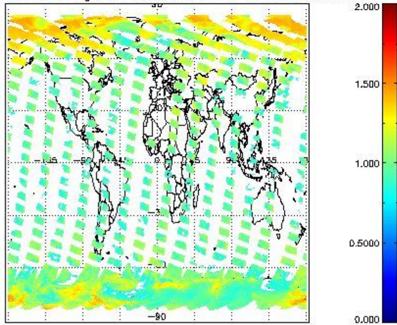
SCIOL2P_NADUV8H2O_arnf_gr for 18MAR2012 00:00:00 to 19MAR2012 00:00:00
