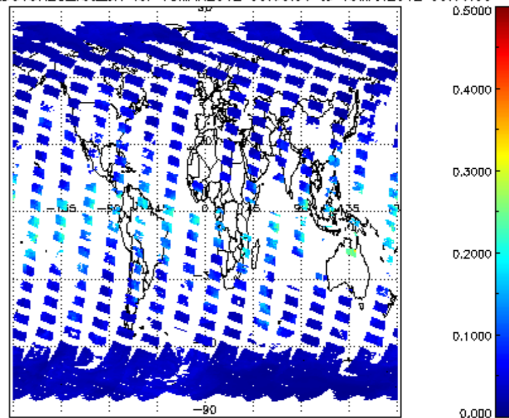
SCIOL2P_NADUV8H2O_vcd_Lerr for 18MAR2012 00:00:00 to 19MAR2012 00:00:00
