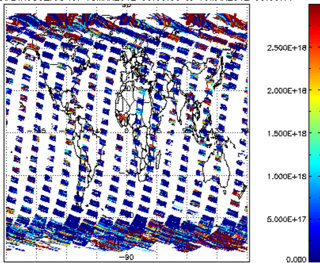
SCIOL2P_NADIR3CO_vcd for 18MAR2012 00:00:00 to 19MAR2012 00:00:00
