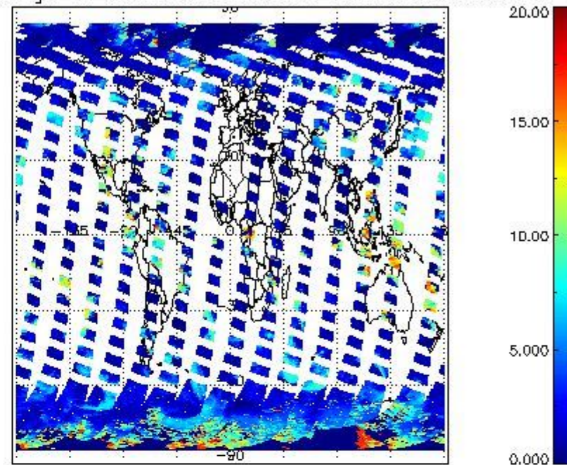
cL_top_height for 18MAR2012 00:00:00 to 19MAR2012 00:00:00
