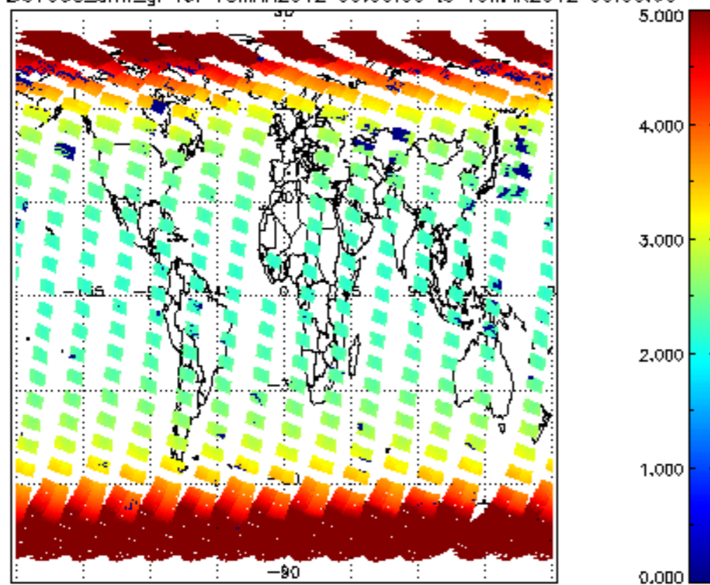
SCIOL2P_NADUV003_arnf_gr for 18MAR2012 00:00:00 to 19MAR2012 00:00:00
