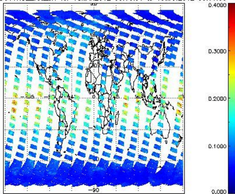
SCIOL2P_NADUV1NO2_vcd_err for 18MAR2012 00:00:00 to 19MAR2012 00:00:00
