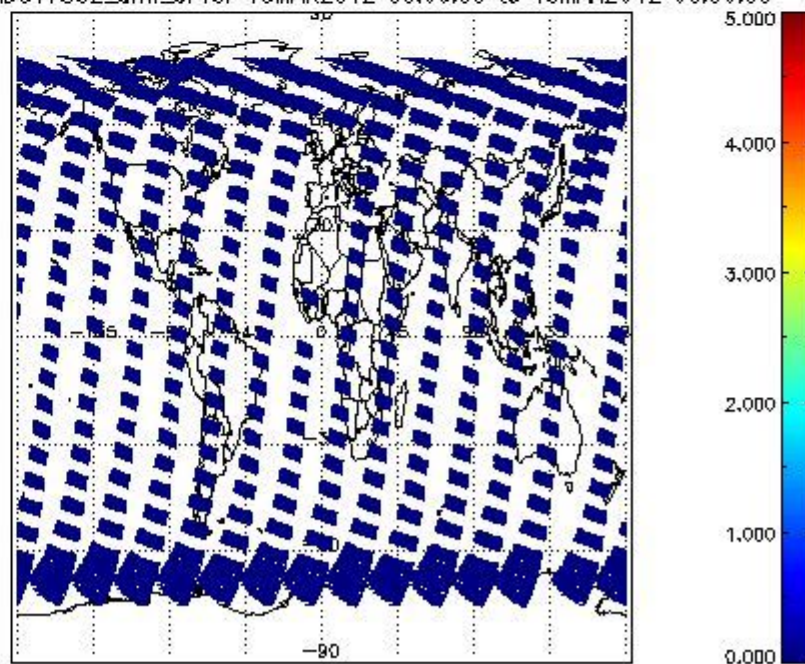
SCIOL2P_NADUV7S02_amf_cl for 18MAR2012 00:00:00 to 19MAR2012 00:00:00
