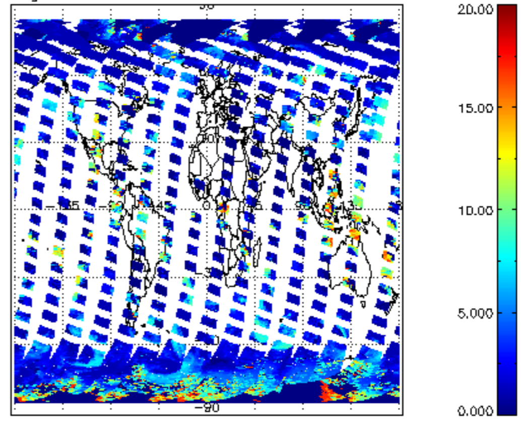
cL_top_height for 18MAR2012 00:00:00 to 19MAR2012 00:00:00
