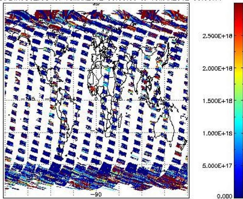
SCIDL2P_NADIR3CO_vcd for 18MAR2012 00:00:00 to 19MAR2012 00:00:00
