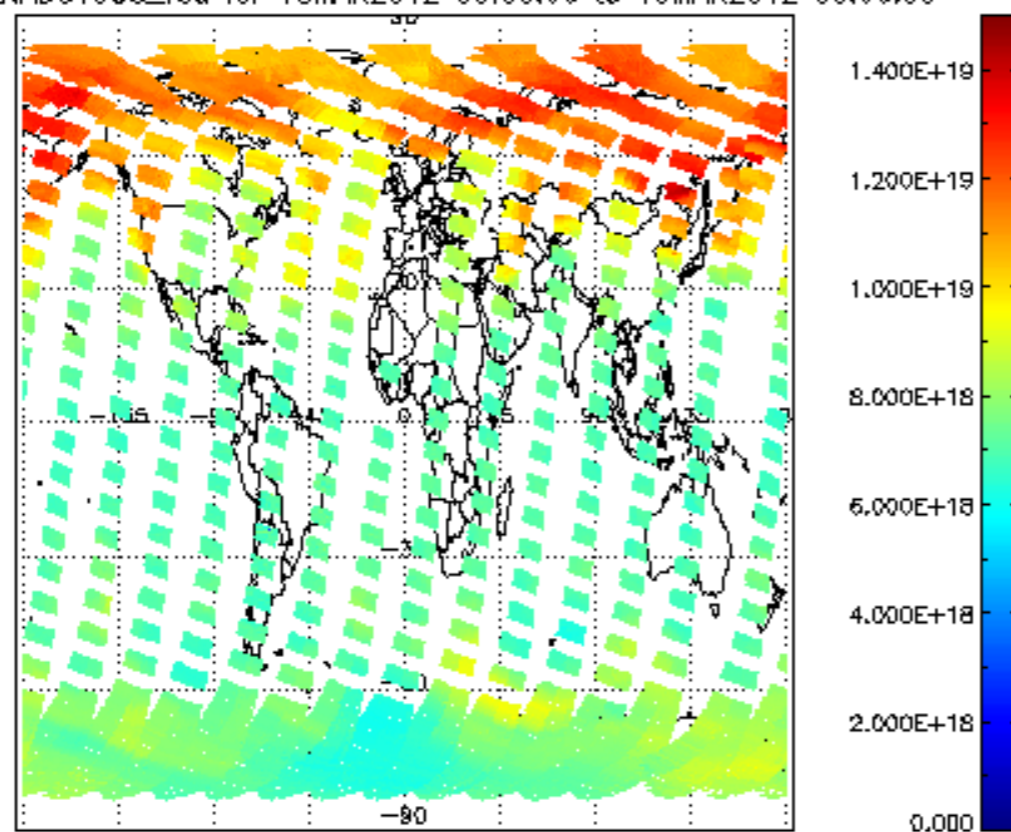
SCIOL2P_NADUV003_vcd for 18MAR2012 00:00:00 to 19MAR2012 00:00:00
