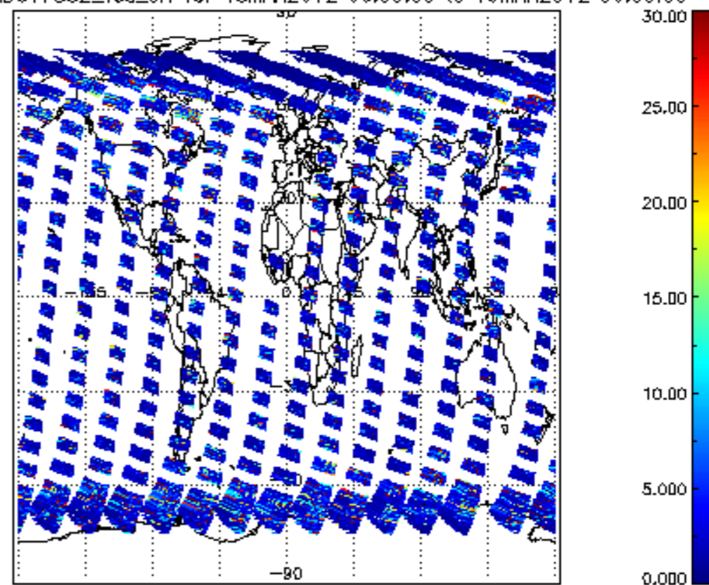
SCIOL2P_NADUV7S02_vcd_err for 18MAR2012 00:00:00 to 19MAR2012 00:00:00
