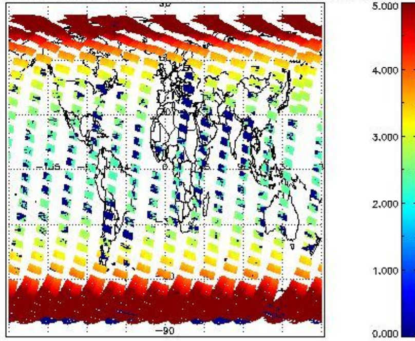
SCIOL2P_NADUV3BRO_amf_cl for 18MAR2012 00:00:00 to 19MAR2012 00:00:00
