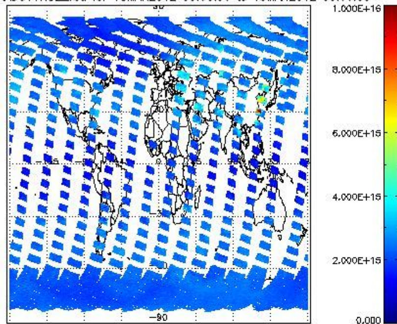
SCIOL2P_NADUV1NO2_vcd for 18MAR2012 00:00:00 to 19MAR2012 00:00:00
