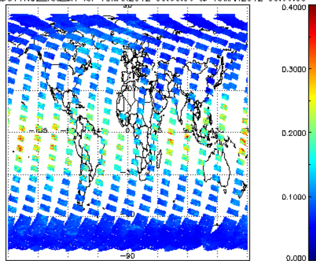
SCIOL2P_NADUV1NO2_vcd_err for 18MAR2012 00:00:00 to 19MAR2012 00:00:00
