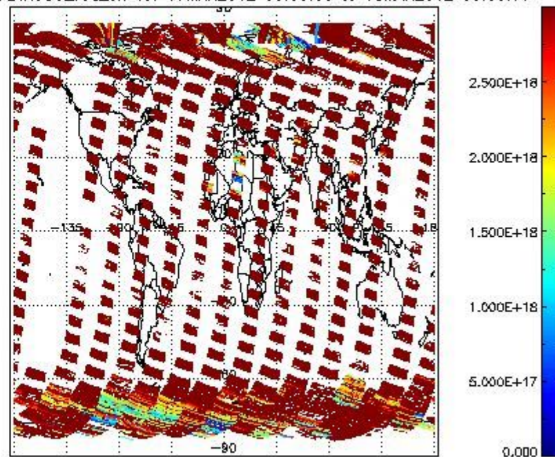
SCIOL2P_NADIR3CO_vcd_err for 17MAR2012 00:00:00 to 18MAR2012 00:00:00
