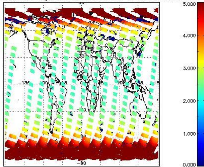
SCIOL2P_NADUV1NO2_amf_gr for 17MAR2012 00:00:00 to 18MAR2012 00:00:00
