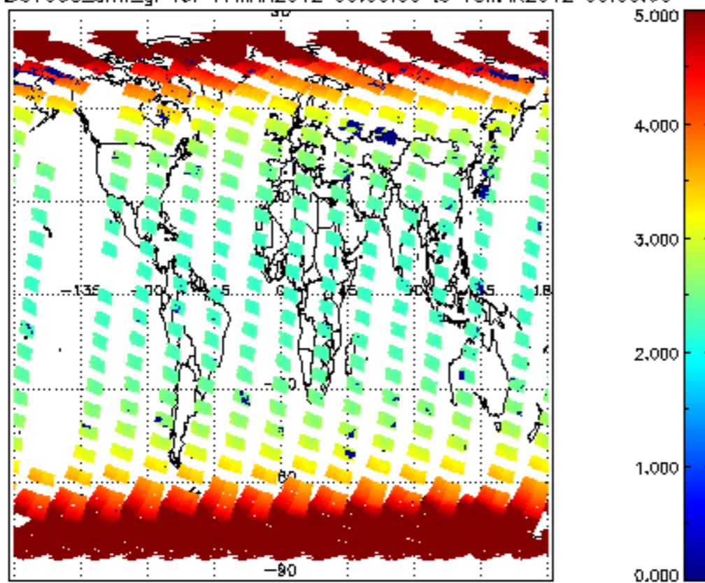
SCIOL2P_NADUV003_amf_gr for 17MAR2012 00:00:00 to 18MAR2012 00:00:00
