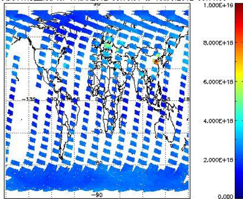
SCIOL2P_NADUV1NO2_vcd for 17MAR2012 00:00:00 to 18MAR2012 00:00:00
