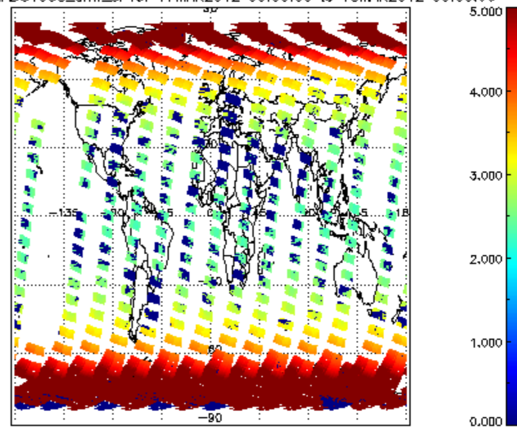
SCIOL2P_NADUV003_amf_cl for 17MAR2012 00:00:00 to 18MAR2012 00:00:00
