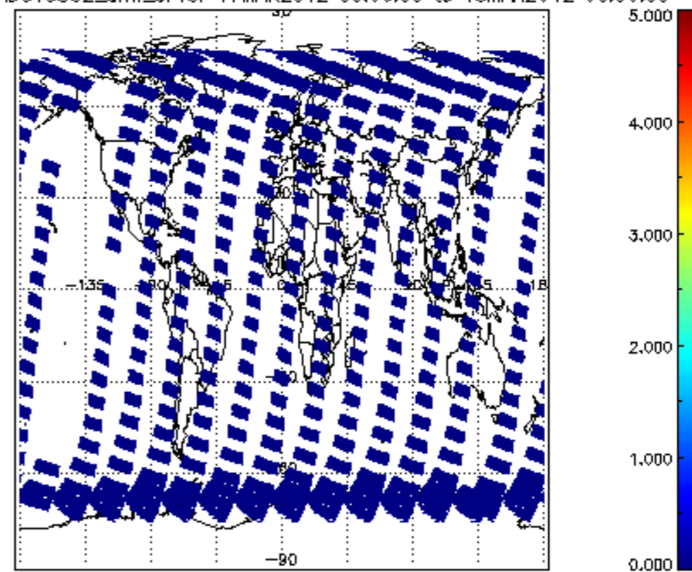
SCIOL2P_NADUV5S02_amf_cl for 17MAR2012 00:00:00 to 18MAR2012 00:00:00
