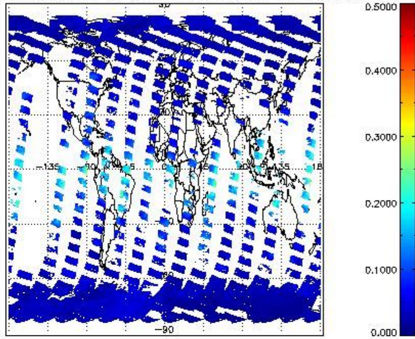
SCIOL2P_NADUV8H2O_vcd_err for 17MAR2012 00:00:00 to 18MAR2012 00:00:00
