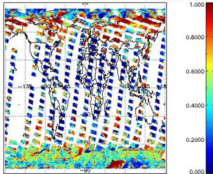
cL_frac for 17MAR2012 00:00:00 to 18MAR2012 00:00:00
