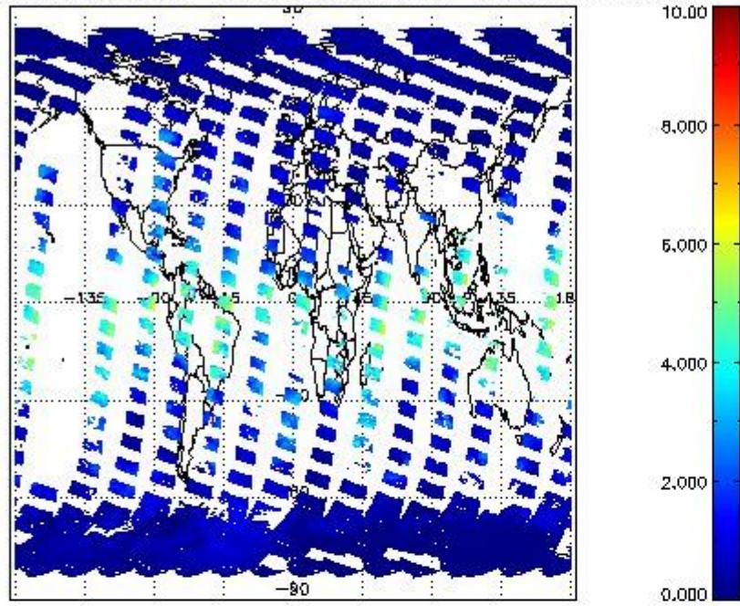
SCIOL2P_NADUV8H2O_vcd for 17MAR2012 00:00:00 to 18MAR2012 00:00:00
