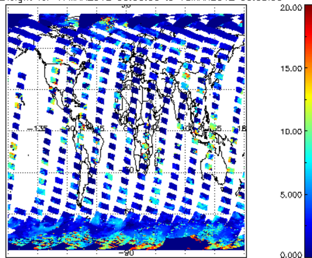
cL_top_height for 17MAR2012 00:00:00 to 18MAR2012 00:00:00
