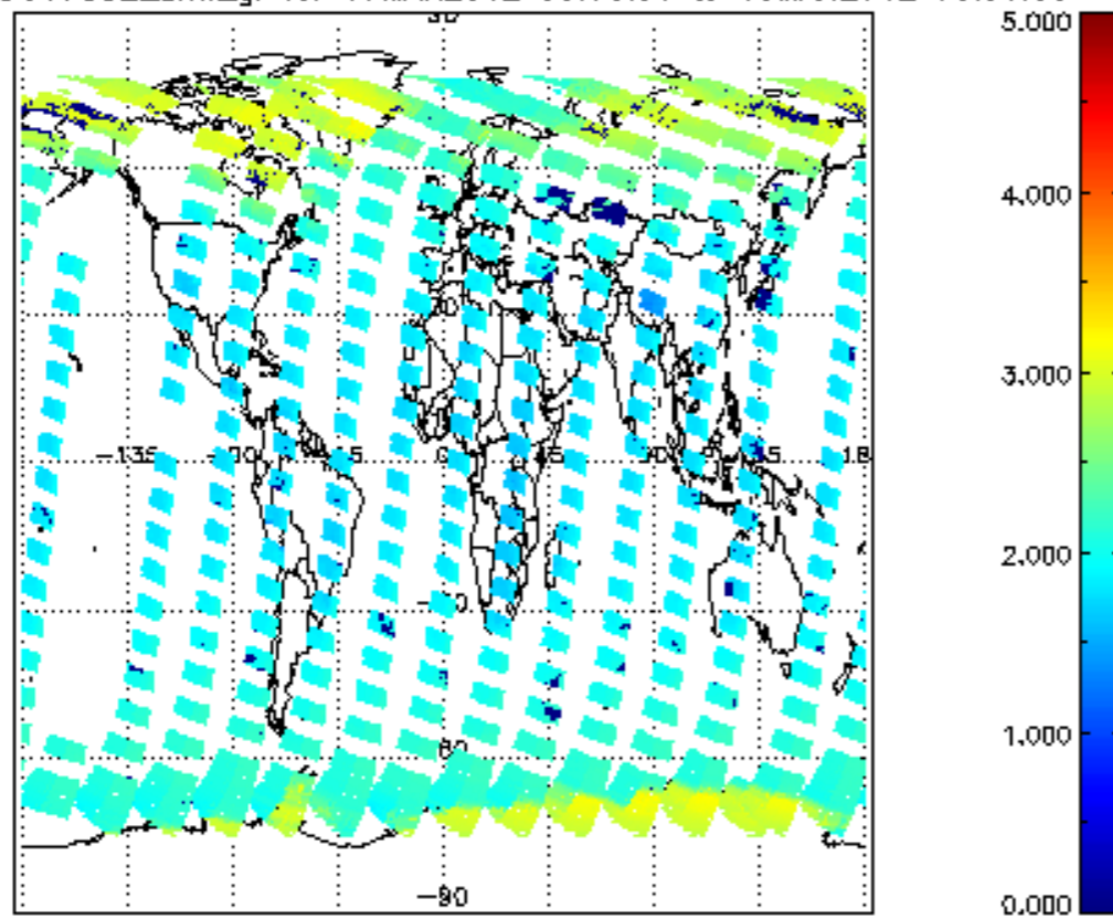
SCIOL2P_NADUV7S02_amf_gr for 17MAR2012 00:00:00 to 18MAR2012 00:00:00
