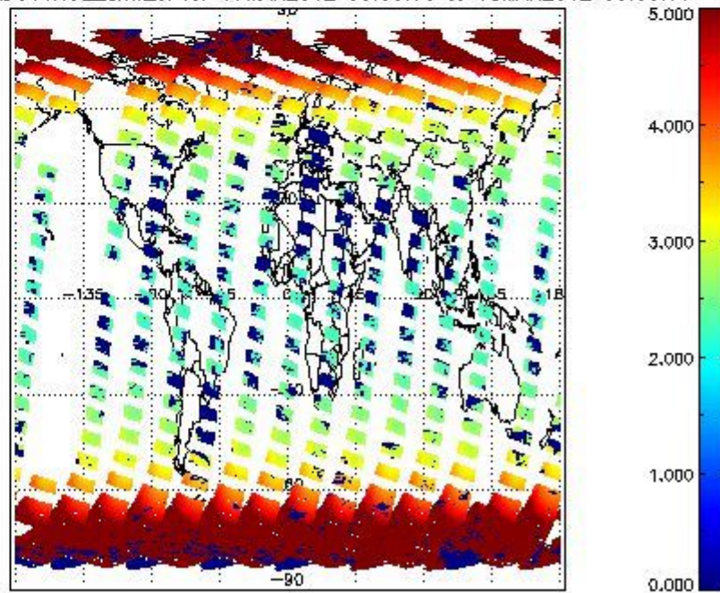
SCIOL2P_NADUV1NO2_amf_cl for 17MAR2012 00:00:00 to 18MAR2012 00:00:00
