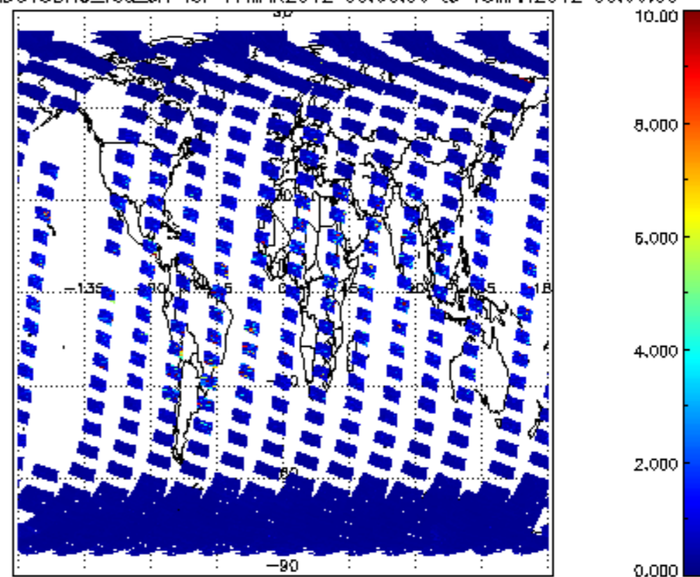
SCIOL2P_NADUV3BRO_vcd_err for 17MAR2012 00:00:00 to 18MAR2012 00:00:00
