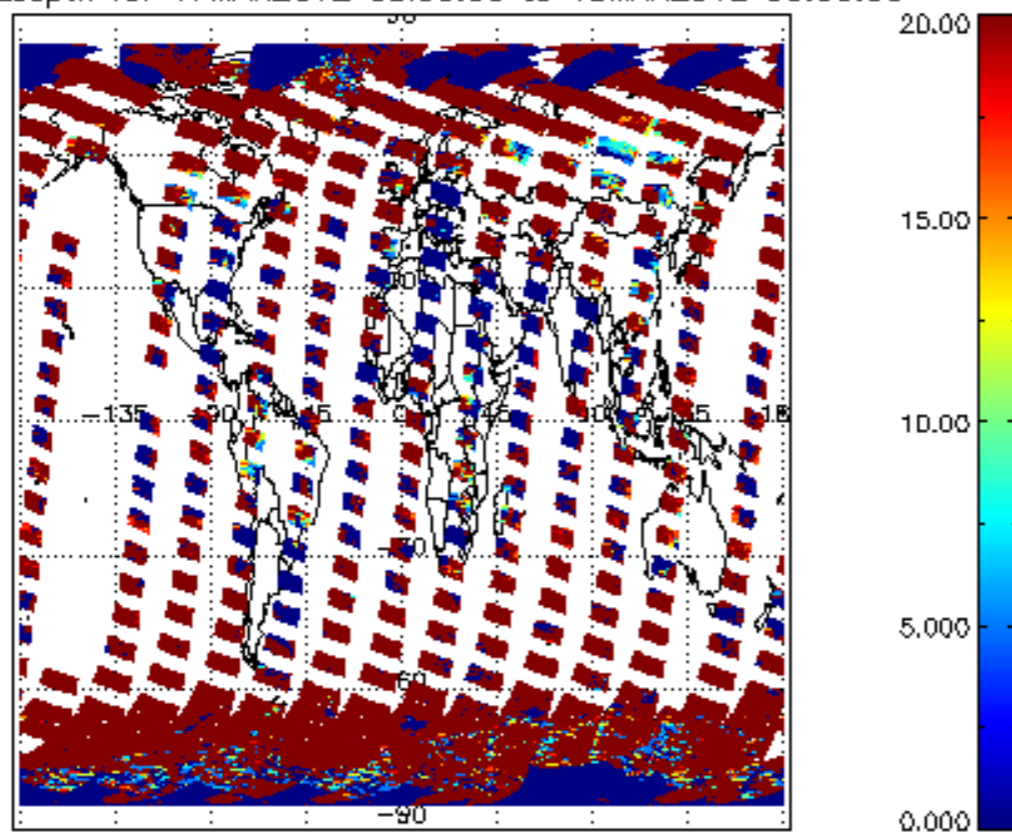
cL_opt_depth for 17MAR2012 00:00:00 to 18MAR2012 00:00:00
