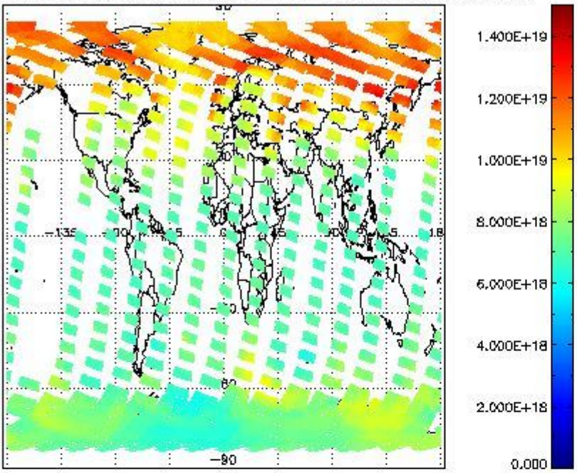
SCIOL2P_NADUV003_vcd for 17MAR2012 00:00:00 to 18MAR2012 00:00:00
