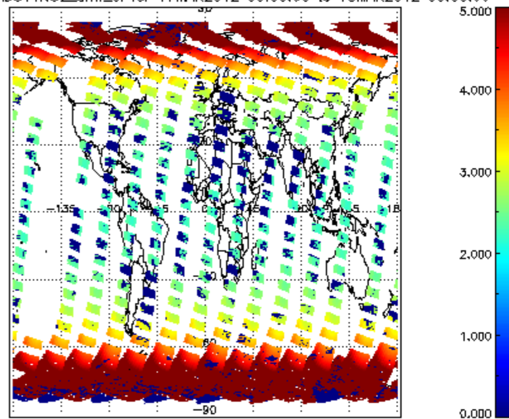
SCIOL2P_NADUV1NO2_amf_cl for 17MAR2012 00:00:00 to 18MAR2012 00:00:00
