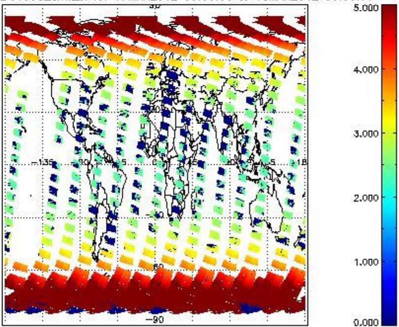
SCIOL2P_NADUV003_amf_cl for 17MAR2012 00:00:00 to 18MAR2012 00:00:00
