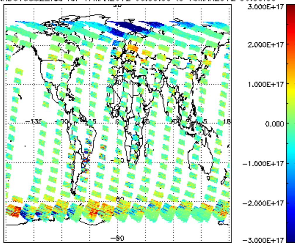
SCIOL2P_NADUV5S02_vcd for 17MAR2012 00:00:00 to 18MAR2012 00:00:00
