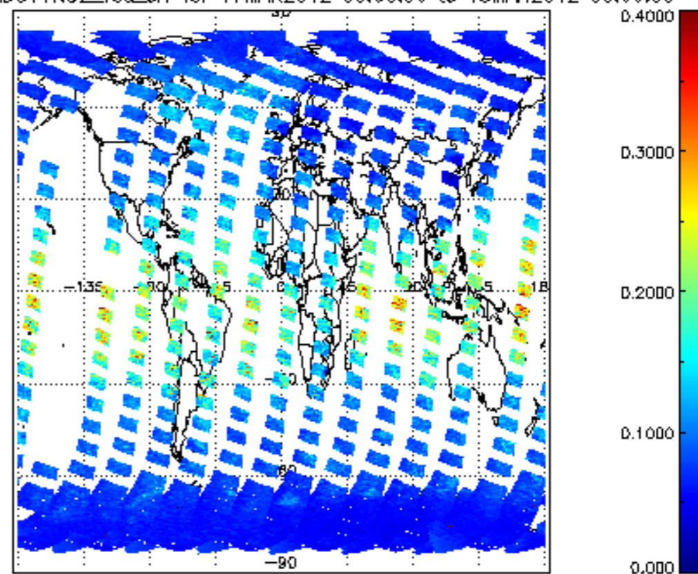
SCIOL2P_NADUV1NO2_vcdLerr for 17MAR2012 00:00:00 to 18MAR2012 00:00:00
