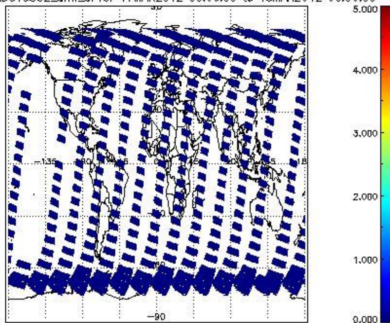
SCIOL2P_NADUV5SO2_amf_cl for 17MAR2012 00:00:00 to 18MAR2012 00:00:00
