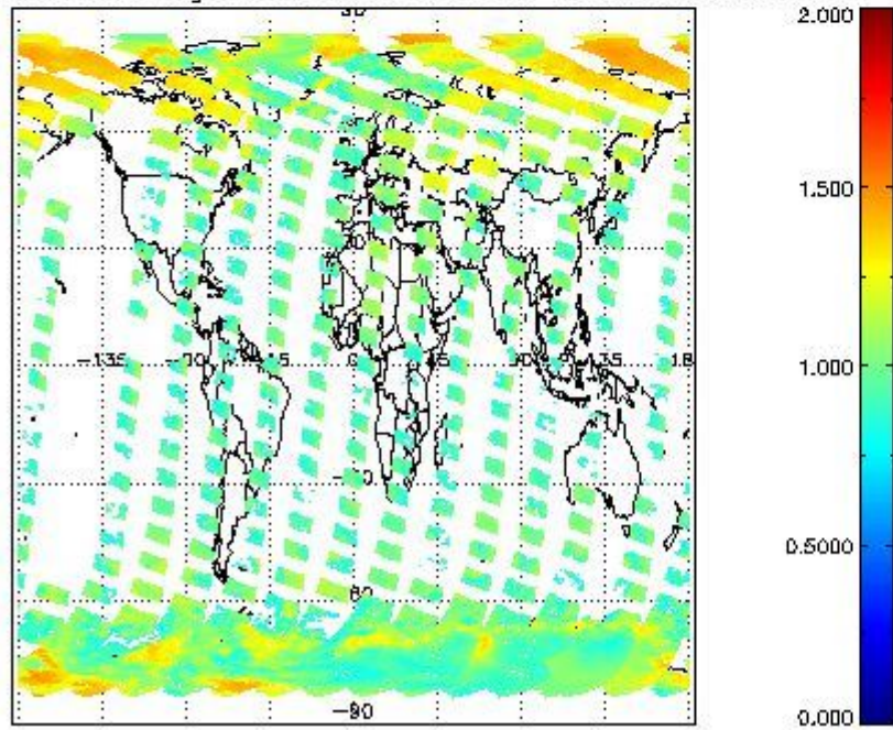
SCIOL2P_NADUV8H2O_arnf_gr for 17MAR2012 00:00:00 to 18MAR2012 00:00:00
