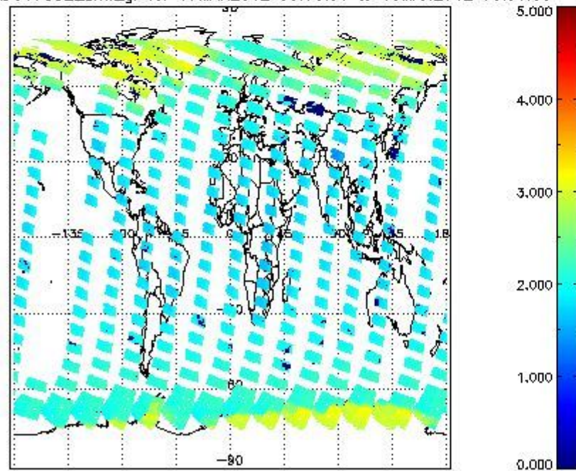
SCIOL2P_NADUV7S02_amf_gr for 17MAR2012 00:00:00 to 18MAR2012 00:00:00
