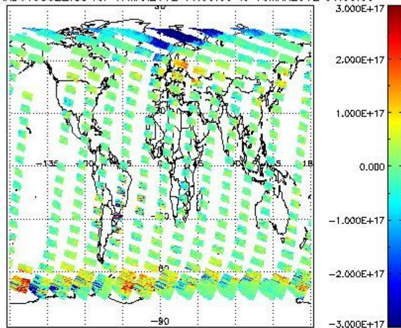
SCIOL2P_NADUV5SO2_vcd for 17MAR2012 00:00:00 to 18MAR2012 00:00:00
