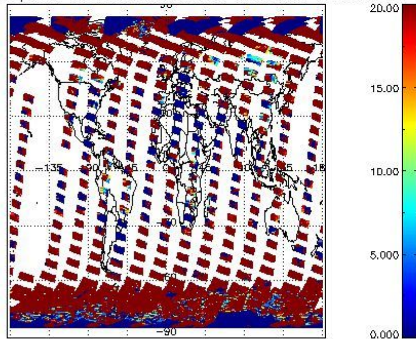
cL_opt_depth for 17MAR2012 00:00:00 to 18MAR2012 00:00:00
