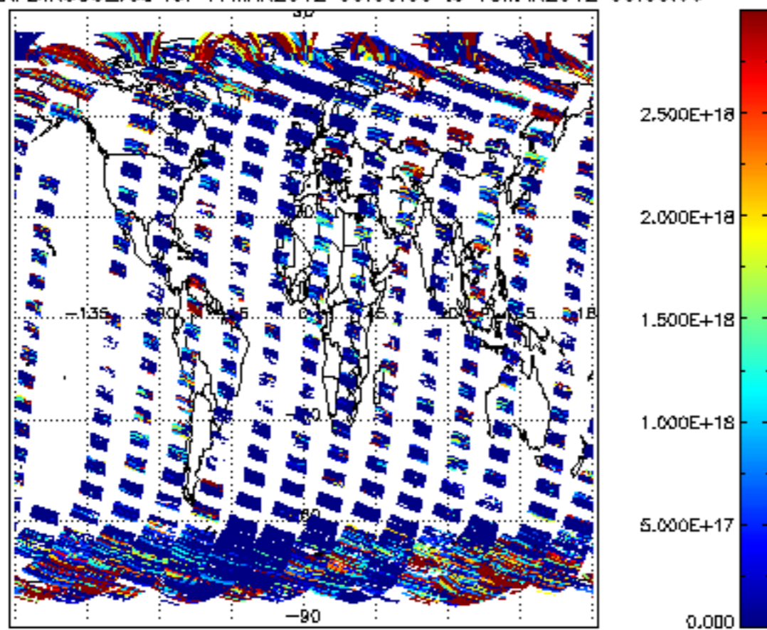
SCIOL2P_NADIR3CO_vcd for 17MAR2012 00:00:00 to 18MAR2012 00:00:00
