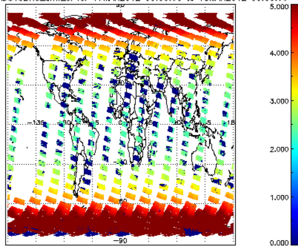
SCIOL2P_NADUV3BRO_amf_cl for 17MAR2012 00:00:00 to 18MAR2012 00:00:00
