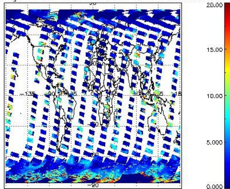
cL_top_height for 17MAR2012 00:00:00 to 18MAR2012 00:00:00
