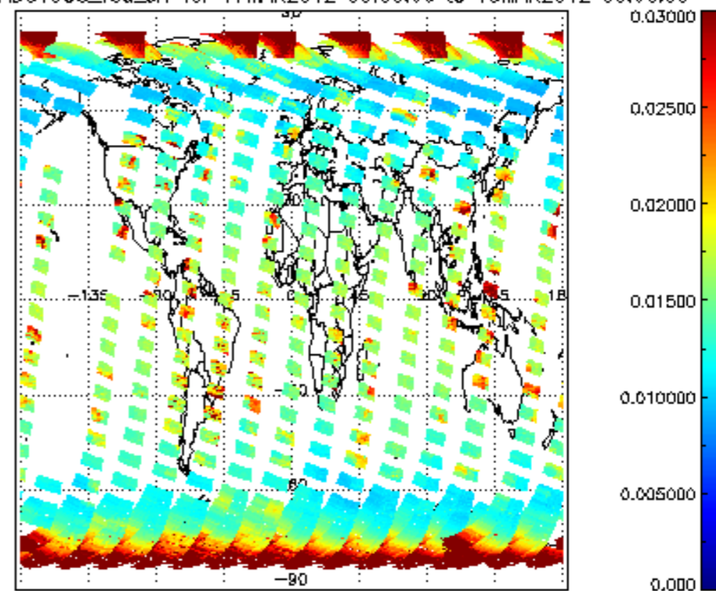
SCIOL2P_NADUV003_vcd_err for 17MAR2012 00:00:00 to 18MAR2012 00:00:00
