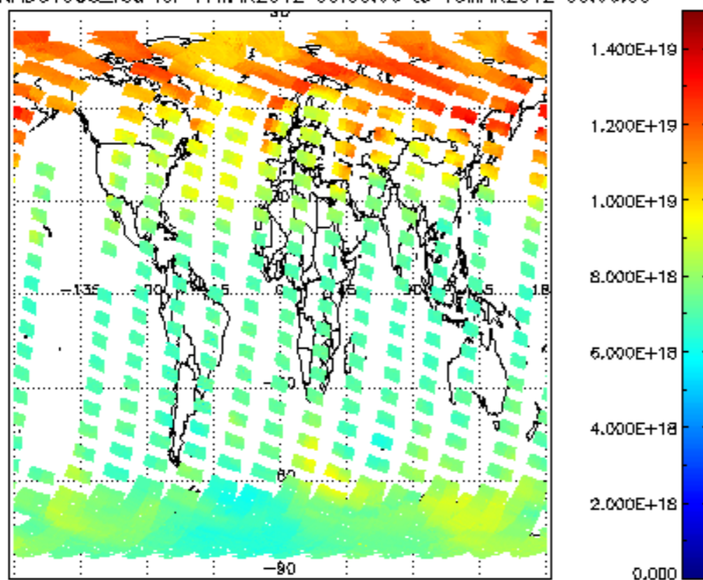
SCIOL2P_NADUV003_vcd for 17MAR2012 00:00:00 to 18MAR2012 00:00:00
