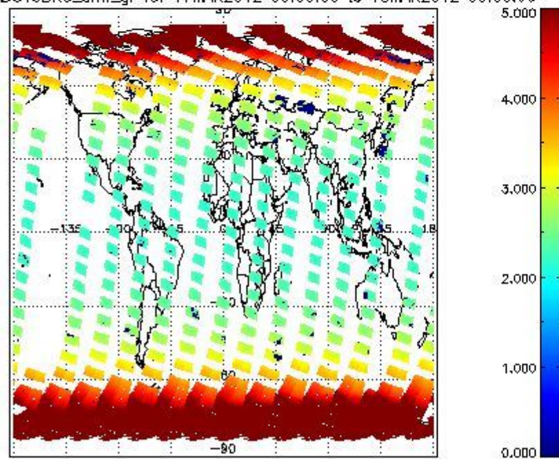
SCIOL2P_NADUV3BRO_amf_gr for 17MAR2012 00:00:00 to 18MAR2012 00:00:00
