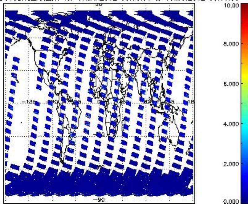
SCIOL2P_NADUV3BRO_vcd_err for 17MAR2012 00:00:00 to 18MAR2012 00:00:00
