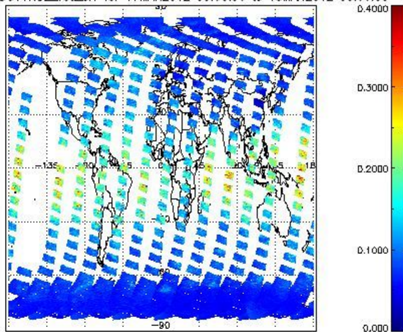
SCIOL2P_NADUV1NO2_vcd_err for 17MAR2012 00:00:00 to 18MAR2012 00:00:00
