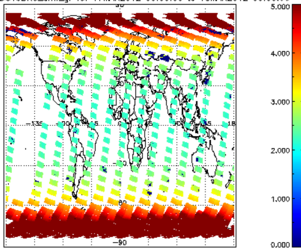
SCIOL2P_NADUV3BRO_amf_gr for 17MAR2012 00:00:00 to 18MAR2012 00:00:00
