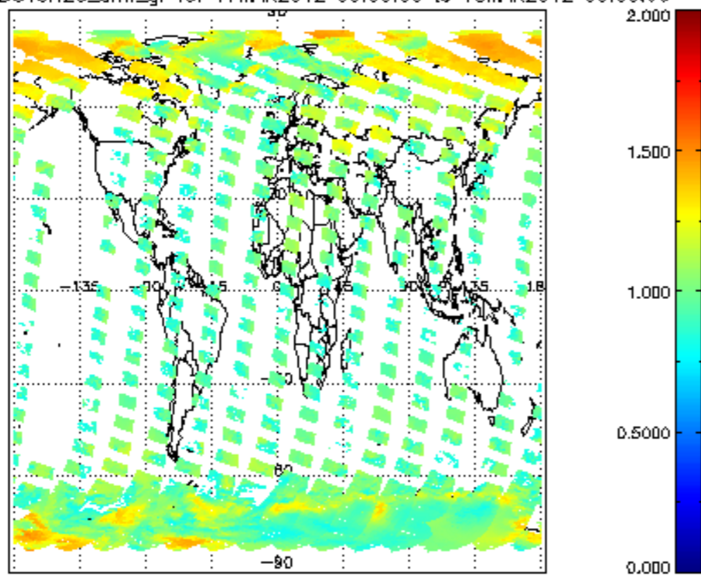
SCIOL2P_NADUV8H20_arnf_gr for 17MAR2012 00:00:00 to 18MAR2012 00:00:00
