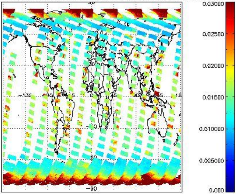
SCIOL2P_NADUV003_vcd_err for 17MAR2012 00:00:00 to 18MAR2012 00:00:00
