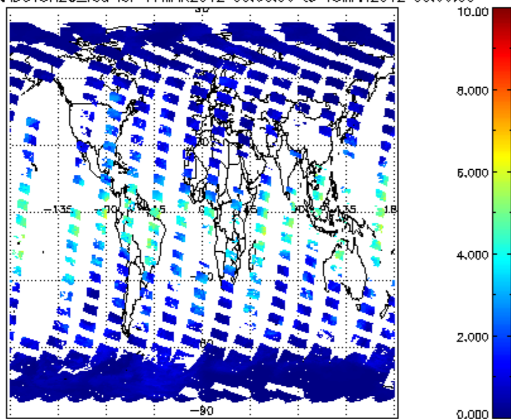
SCIOL2P_NADUV8H20_vcd for 17MAR2012 00:00:00 to 18MAR2012 00:00:00
