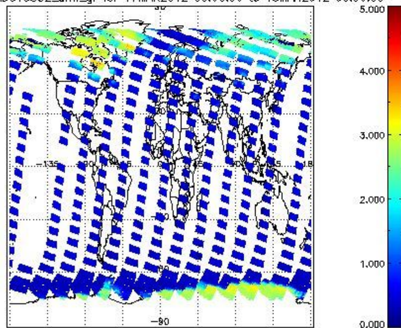
SCIOL2P_NADUV5SO2_amf_gr for 17MAR2012 00:00:00 to 18MAR2012 00:00:00
