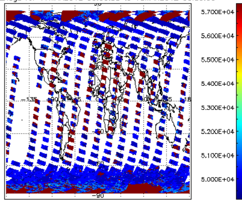
cloud_flags for 17MAR2012 00:00:00 to 18MAR2012 00:00:00
