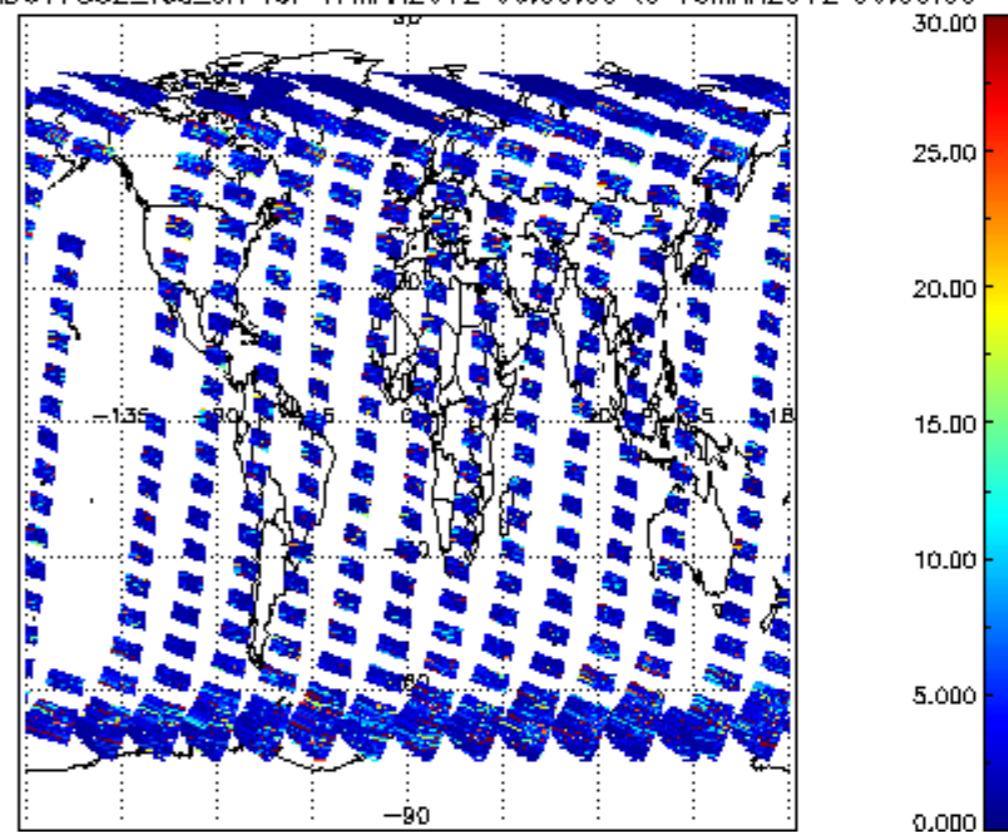
SCIOL2P_NADUV7S02_vcd_err for 17MAR2012 00:00:00 to 18MAR2012 00:00:00
