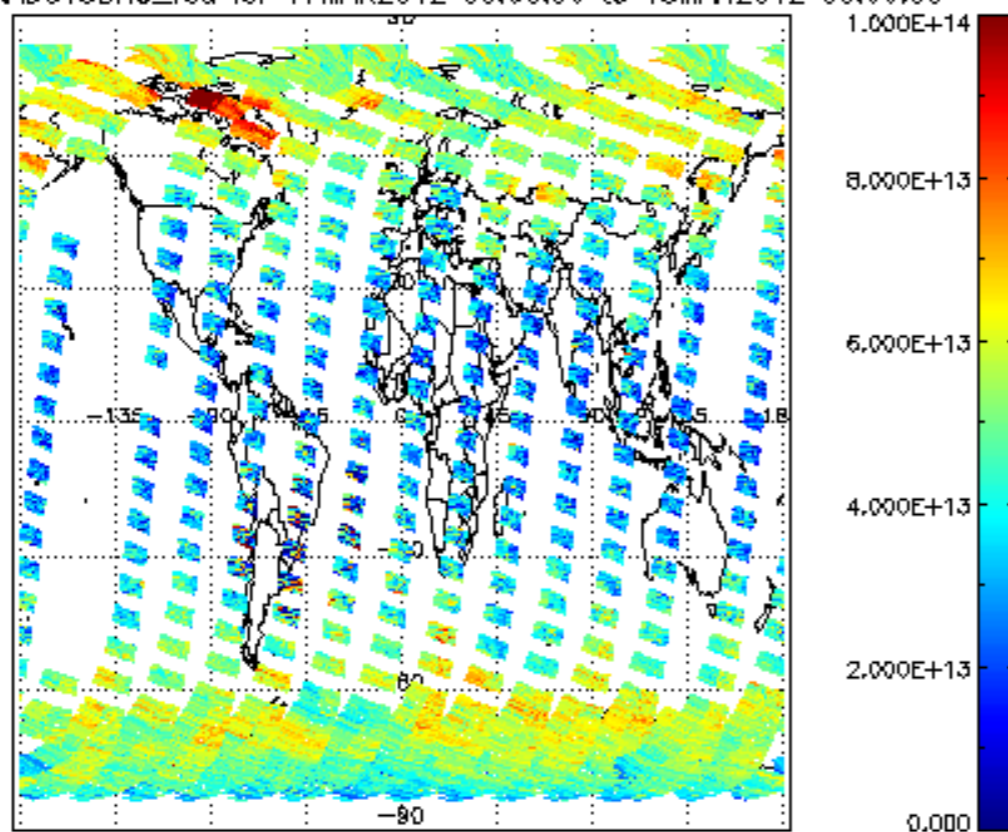
SCIOL2P_NADUV3BRO_vcd for 17MAR2012 00:00:00 to 18MAR2012 00:00:00
