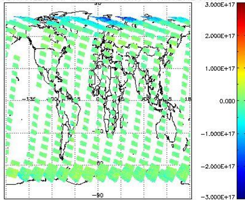
SCIOL2P_NADUV7S02_vcd for 17MAR2012 00:00:00 to 18MAR2012 00:00:00
