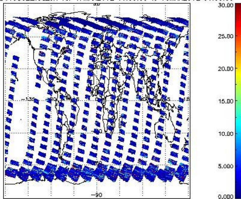
SCIOL2P_NADUV5SO2_vcd_err for 17MAR2012 00:00:00 to 18MAR2012 00:00:00
