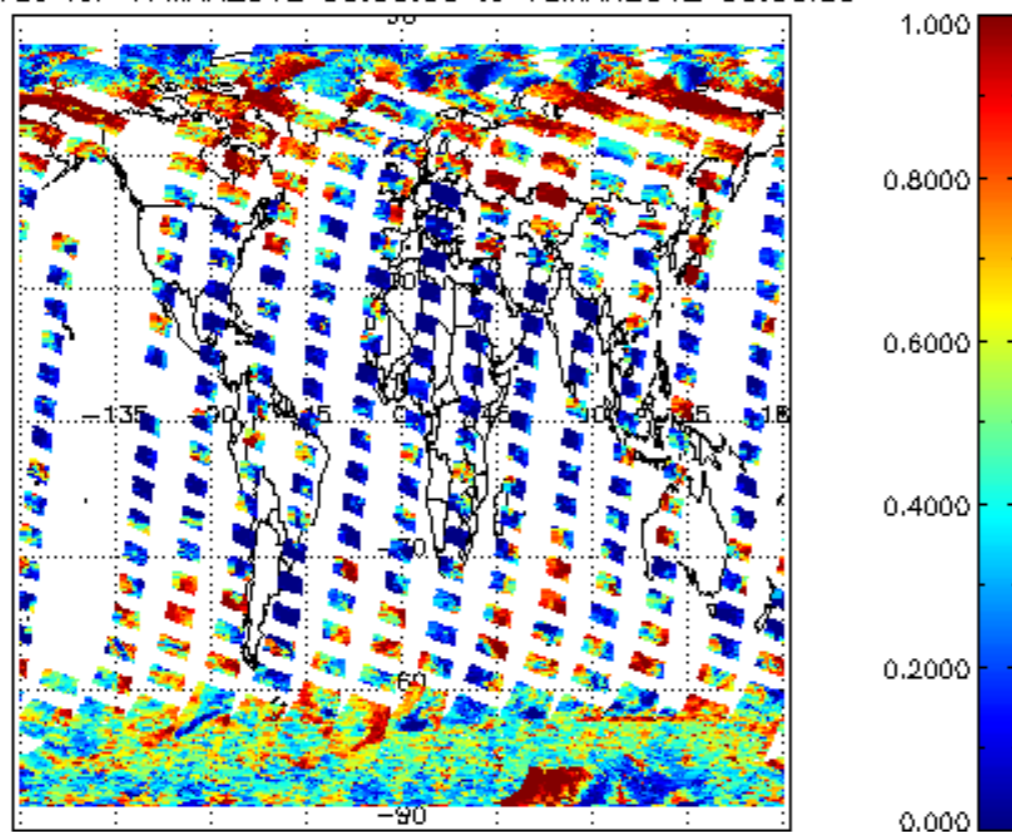
cL_frac for 17MAR2012 00:00:00 to 18MAR2012 00:00:00
