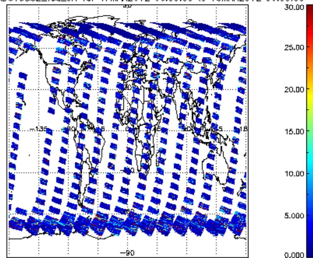
SCIOL2P_NADUV5S02_vcd_err for 17MAR2012 00:00:00 to 18MAR2012 00:00:00
