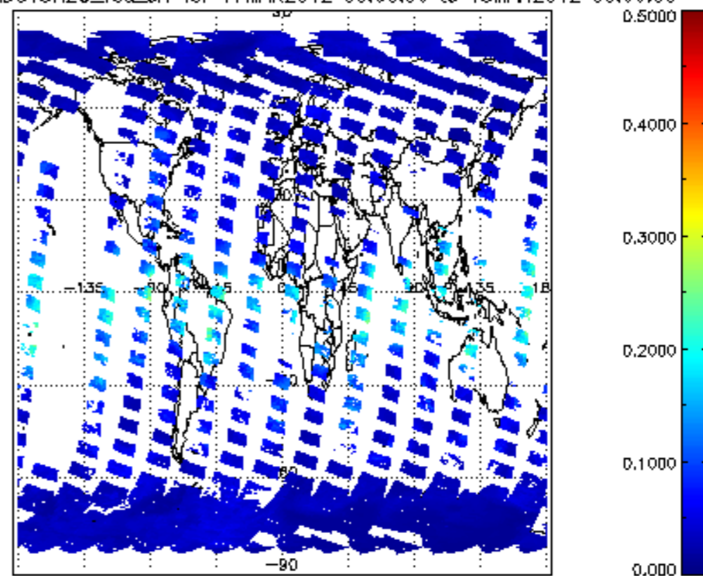
SCIOL2P_NADUV8H20_vcd_Lerr for 17MAR2012 00:00:00 to 18MAR2012 00:00:00
