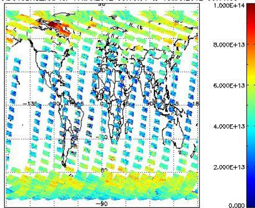
SCIOL2P_NADUV3BRO_vcd for 17MAR2012 00:00:00 to 18MAR2012 00:00:00
