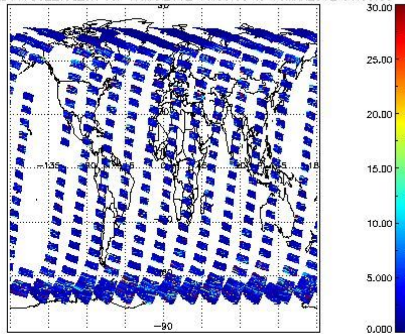
SCIOL2P_NADUV7S02_vcd_err for 17MAR2012 00:00:00 to 18MAR2012 00:00:00
