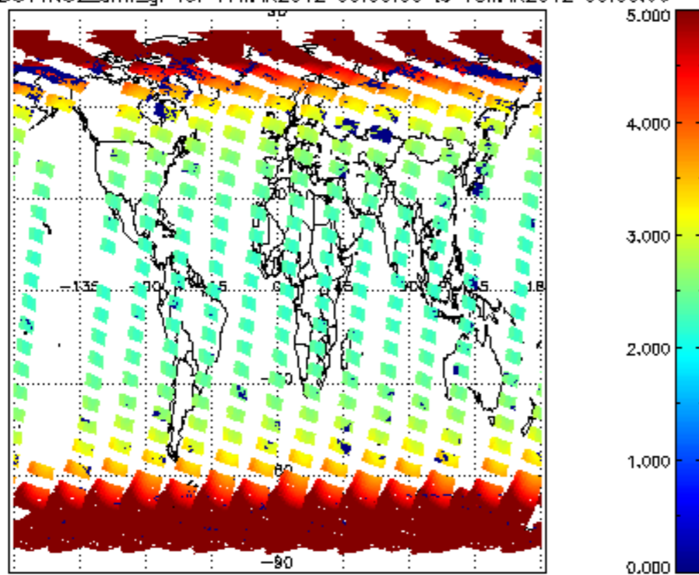
SCIOL2P_NADUV1NO2_amf_gr for 17MAR2012 00:00:00 to 18MAR2012 00:00:00
