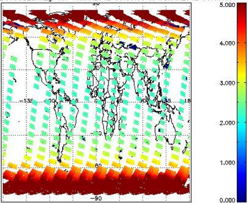
SCIOL2P_NADUV003_amf_gr for 17MAR2012 00:00:00 to 18MAR2012 00:00:00
