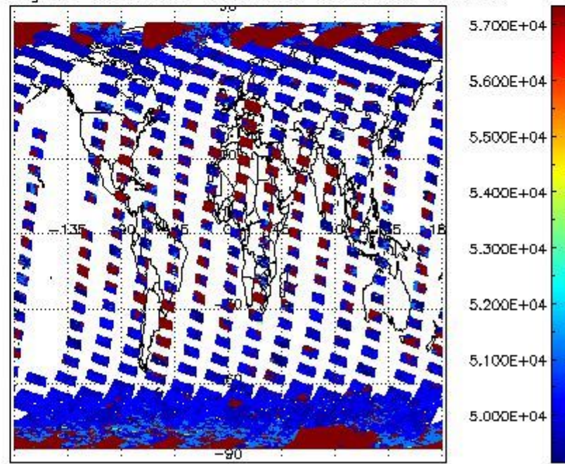
cloud_flags for 17MAR2012 00:00:00 to 18MAR2012 00:00:00
