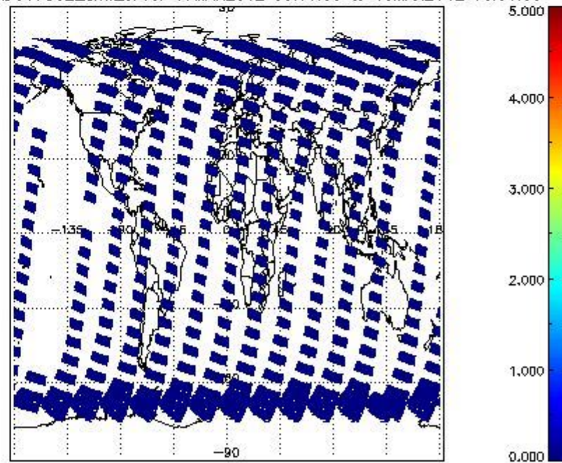
SCIOL2P_NADUV7S02_amf_cl for 17MAR2012 00:00:00 to 18MAR2012 00:00:00
