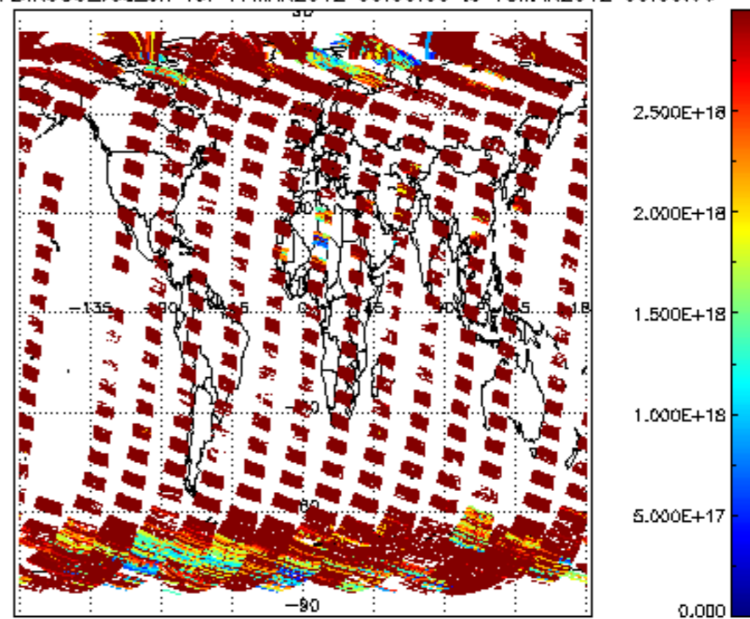
SCIOL2P_NADIR3CO_vcd_err for 17MAR2012 00:00:00 to 18MAR2012 00:00:00
