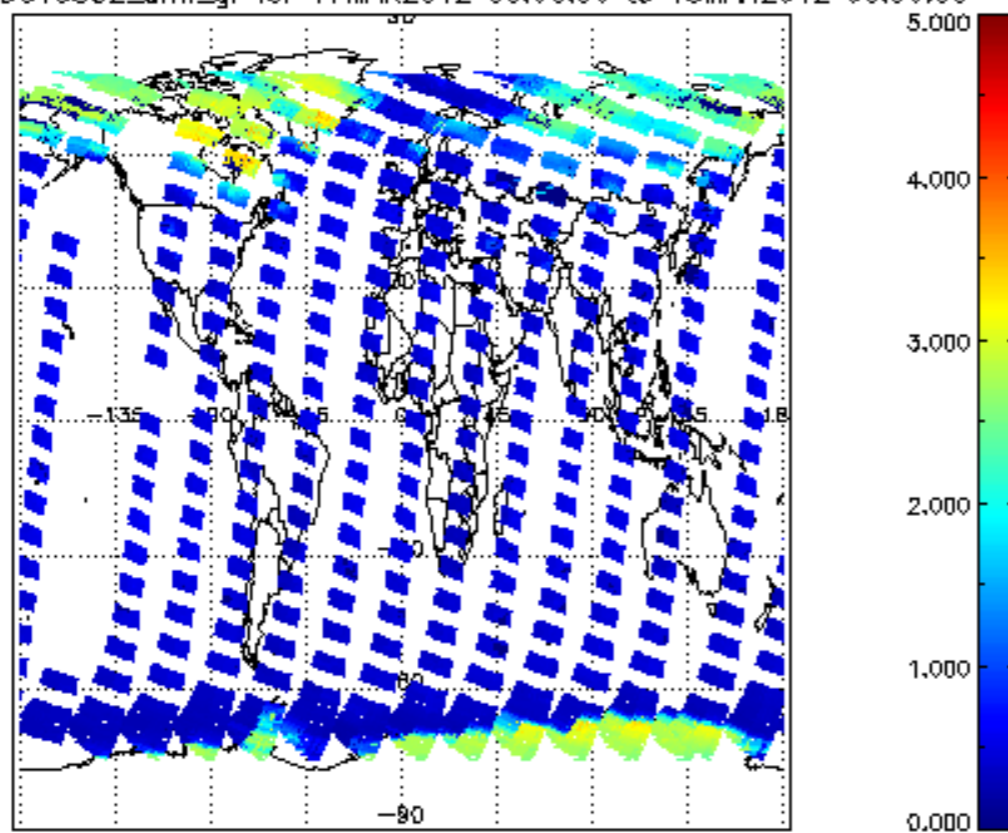
SCIOL2P_NADUV5S02_amf_gr for 17MAR2012 00:00:00 to 18MAR2012 00:00:00
