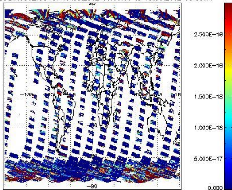
SCIOL2P_NADIR3CO_vcd for 17MAR2012 00:00:00 to 18MAR2012 00:00:00
