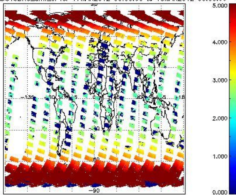
SCIOL2P_NADUV3BRO_amf_cl for 17MAR2012 00:00:00 to 18MAR2012 00:00:00
