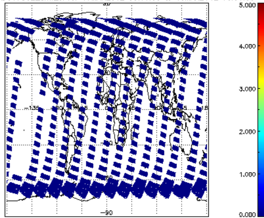
SCIOL2P_NADUV7S02_amf_cl for 17MAR2012 00:00:00 to 18MAR2012 00:00:00
