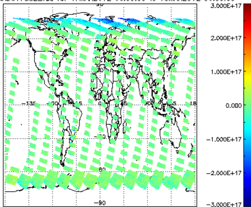
SCIOL2P_NADUV7S02_vcd for 17MAR2012 00:00:00 to 18MAR2012 00:00:00
