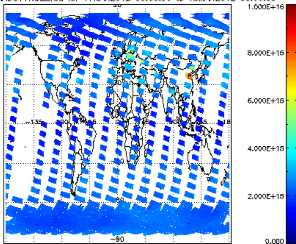
SCIOL2P_NADUV1NO2_vcd for 17MAR2012 00:00:00 to 18MAR2012 00:00:00
