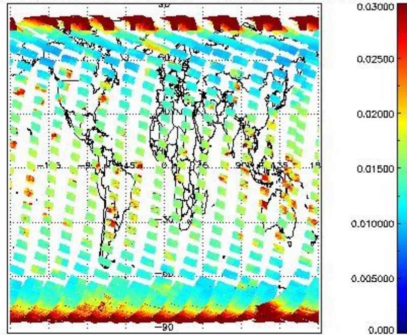
SCIOL2P_NADUV003_vcd_err for 13MAR2012 00:00:00 to 14MAR2012 00:00:00
