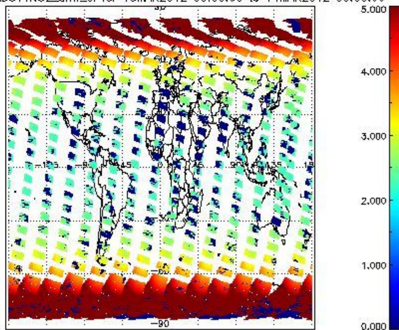
SCIOL2P_NADUV1NO2_amf_cl for 13MAR2012 00:00:00 to 14MAR2012 00:00:00
