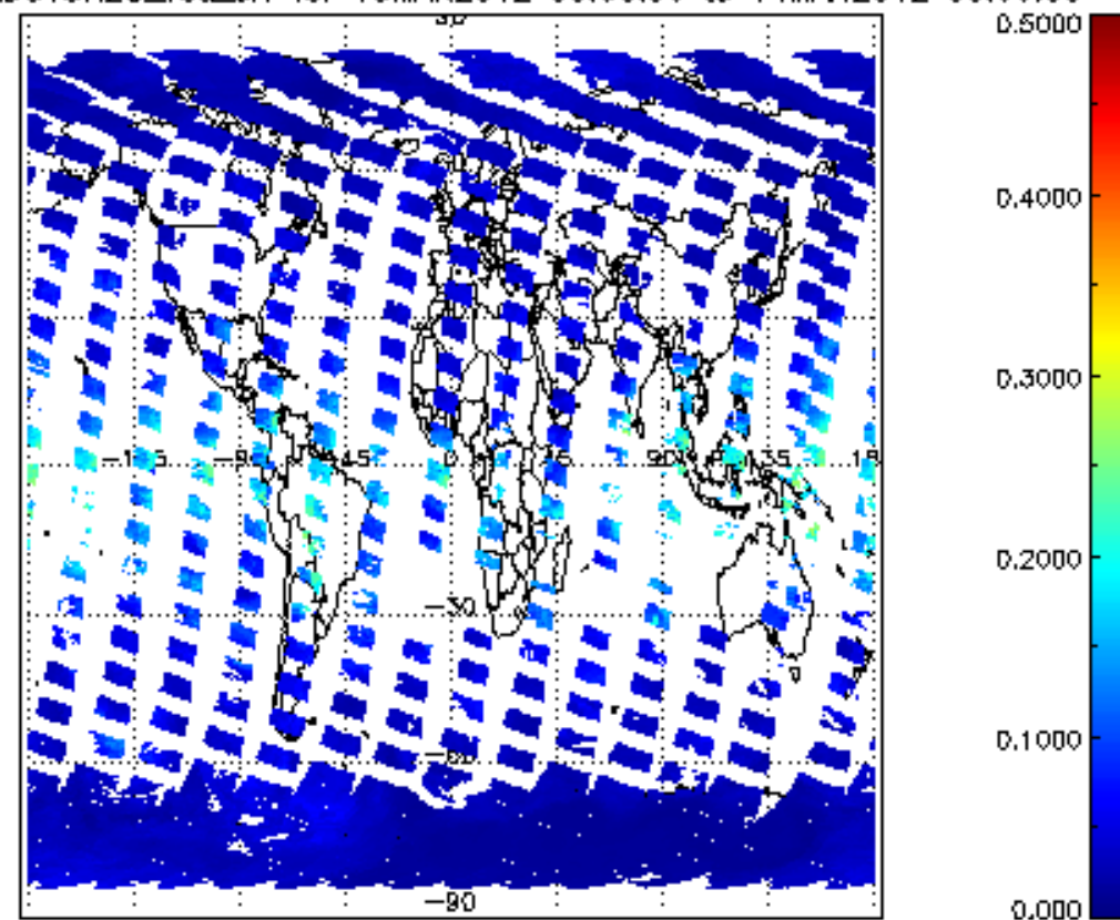
SCIOL2P_NADUV8H2O_vcd_err for 13MAR2012 00:00:00 to 14MAR2012 00:00:00
