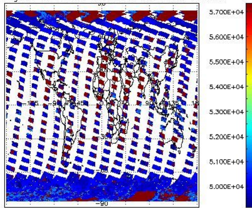
cloud_flags for 13MAR2012 00:00:00 to 14MAR2012 00:00:00
