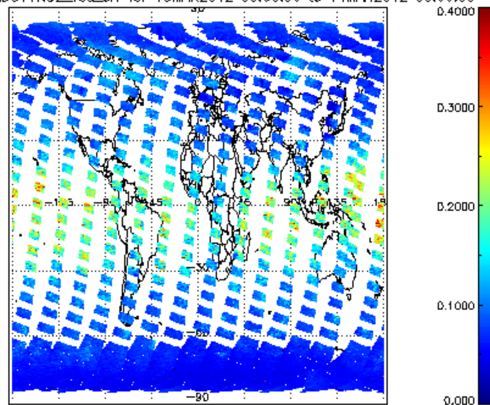
SCIOL2P_NADUV1NO2_vcd_err for 13MAR2012 00:00:00 to 14MAR2012 00:00:00
