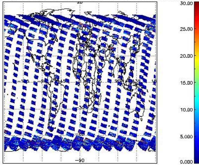
SCIOL2P_NADUV7S02_vcd_err for 13MAR2012 00:00:00 to 14MAR2012 00:00:00
