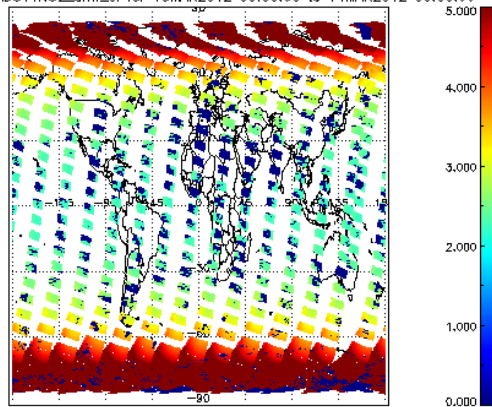
SCIOL2P_NADUV1NO2_amf_cl for 13MAR2012 00:00:00 to 14MAR2012 00:00:00
