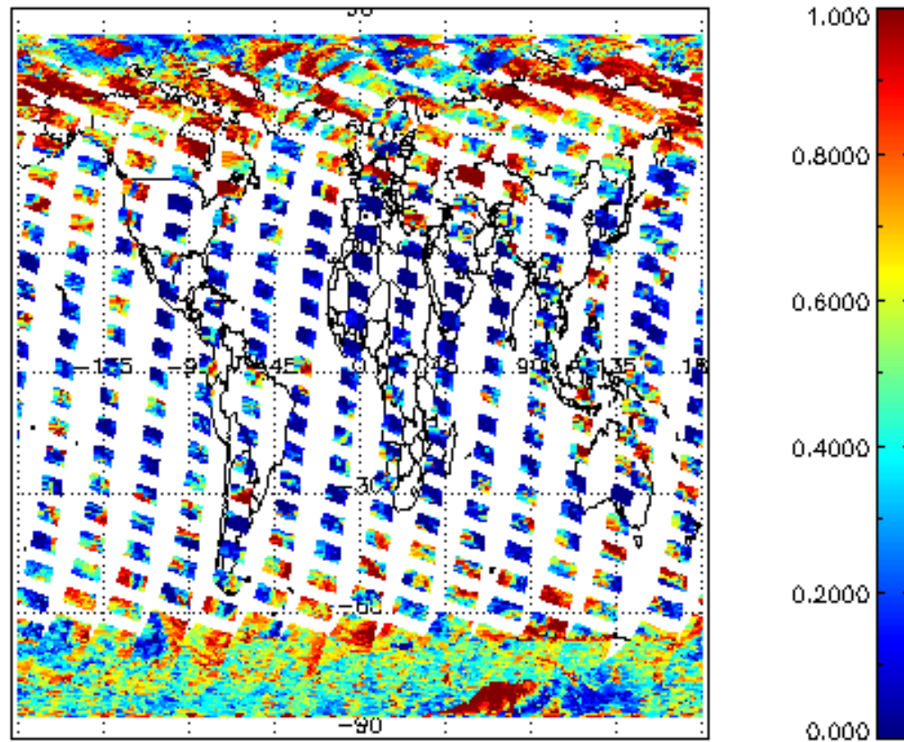
cL_frac for 13MAR2012 00:00:00 to 14MAR2012 00:00:00
