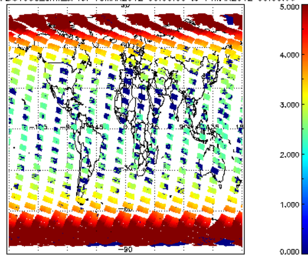
SCIOL2P_NADUV003_arnf_cl for 13MAR2012 00:00:00 to 14MAR2012 00:00:00
