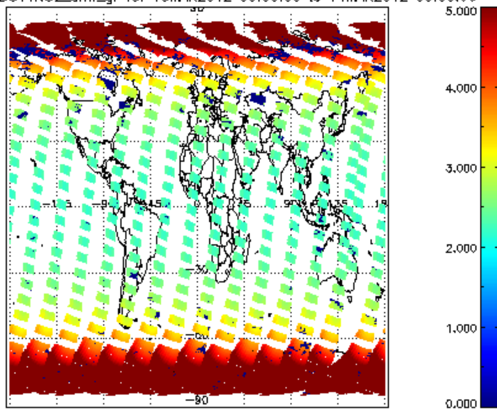
SCIOL2P_NADUV1NO2_amf_gr for 13MAR2012 00:00:00 to 14MAR2012 00:00:00
