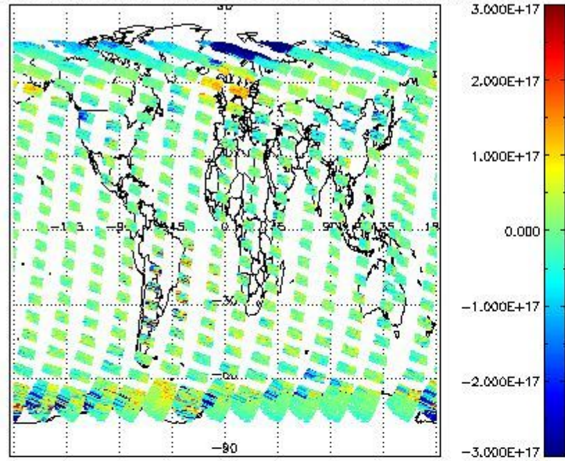
SCIOL2P_NADUV5SO2_vcd for 13MAR2012 00:00:00 to 14MAR2012 00:00:00
