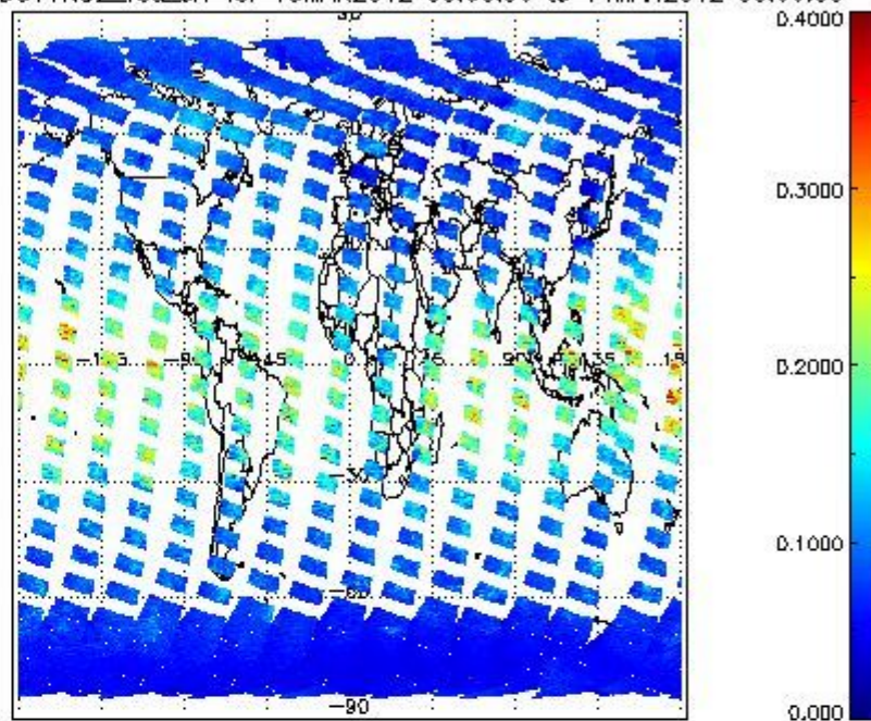
SCIOL2P_NADUV1NO2_vcd_err for 13MAR2012 00:00:00 to 14MAR2012 00:00:00
