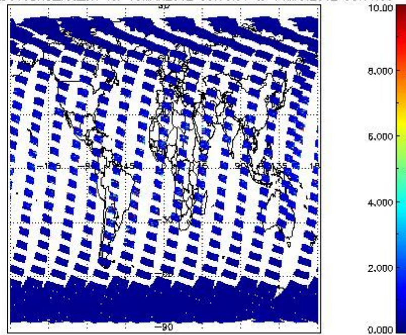
SCIOL2P_NADUV3BRO_vcd_err for 13MAR2012 00:00:00 to 14MAR2012 00:00:00
