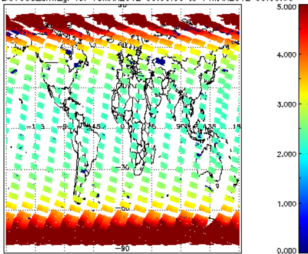
SCIOL2P_NADUV003_arnf_gr for 13MAR2012 00:00:00 to 14MAR2012 00:00:00
