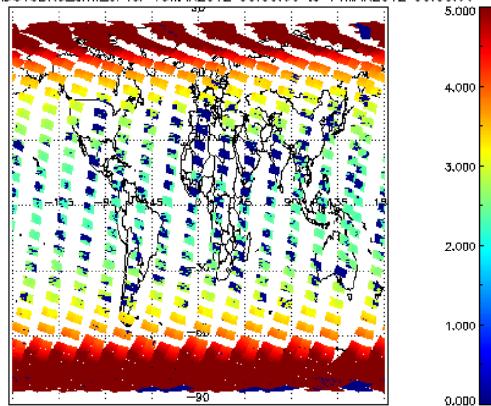
SCIOL2P_NADUV3BRO_arnf_cl for 13MAR2012 00:00:00 to 14MAR2012 00:00:00
