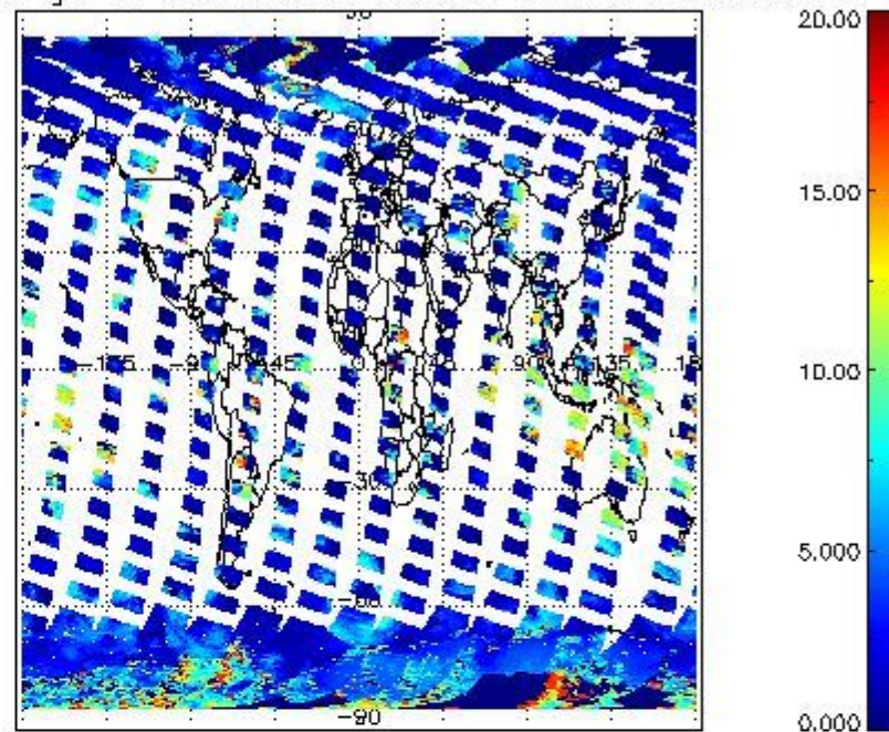
cL_top_height for 13MAR2012 00:00:00 to 14MAR2012 00:00:00
