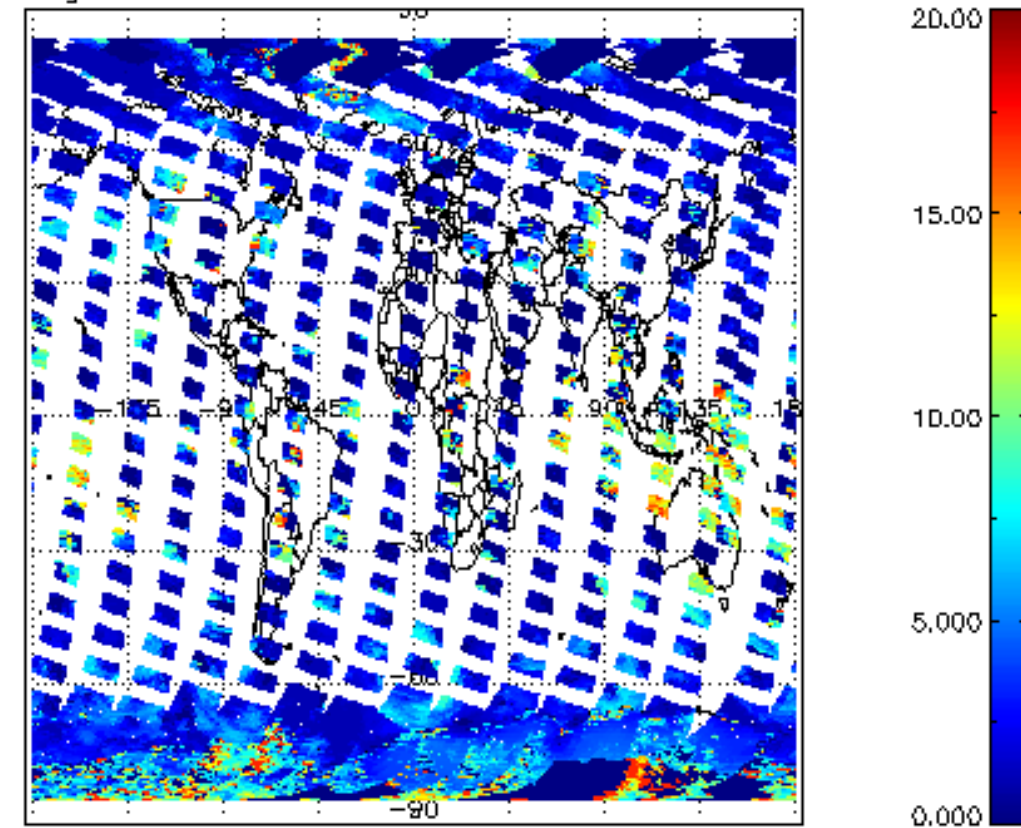
cL_top_height for 13MAR2012 00:00:00 to 14MAR2012 00:00:00
