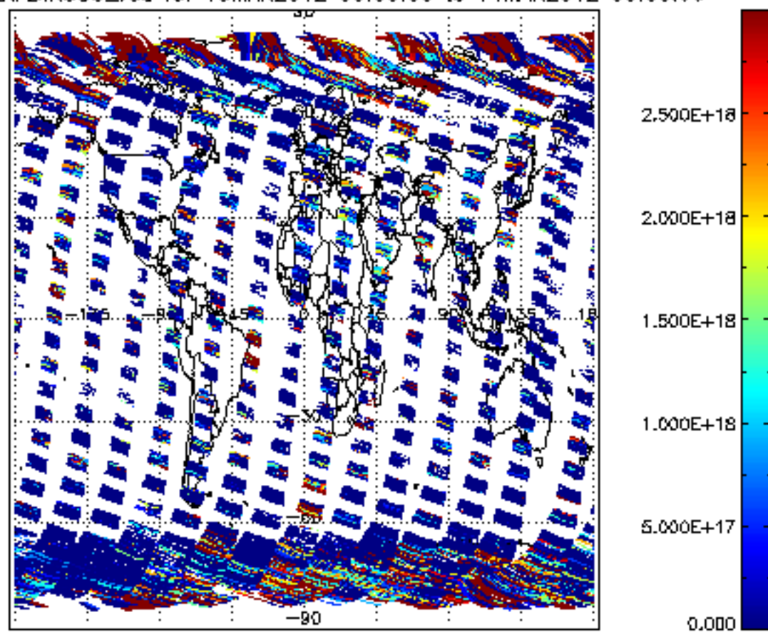
SCIOL2P_NADIR3CO_vcd for 13MAR2012 00:00:00 to 14MAR2012 00:00:00
