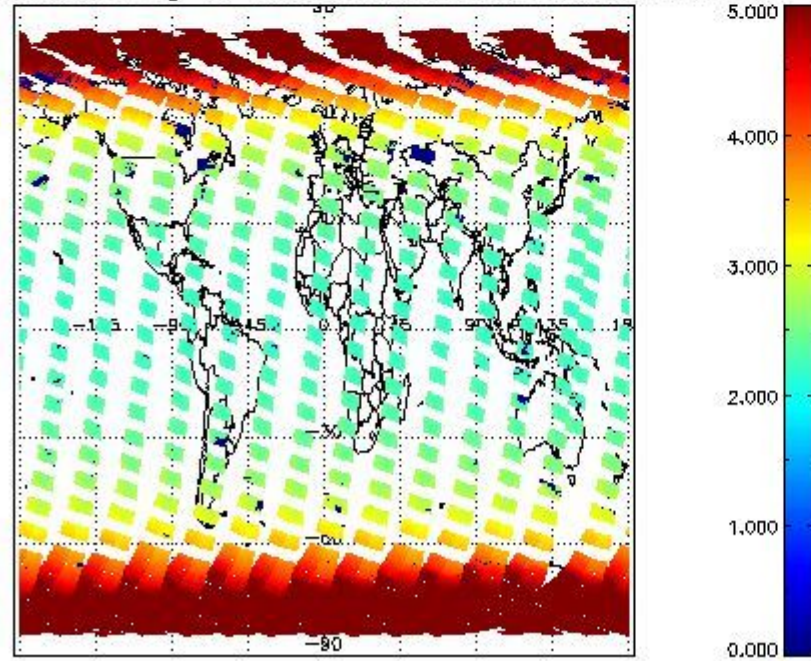
SCIOL2P_NADUV003_amf_gr for 13MAR2012 00:00:00 to 14MAR2012 00:00:00
