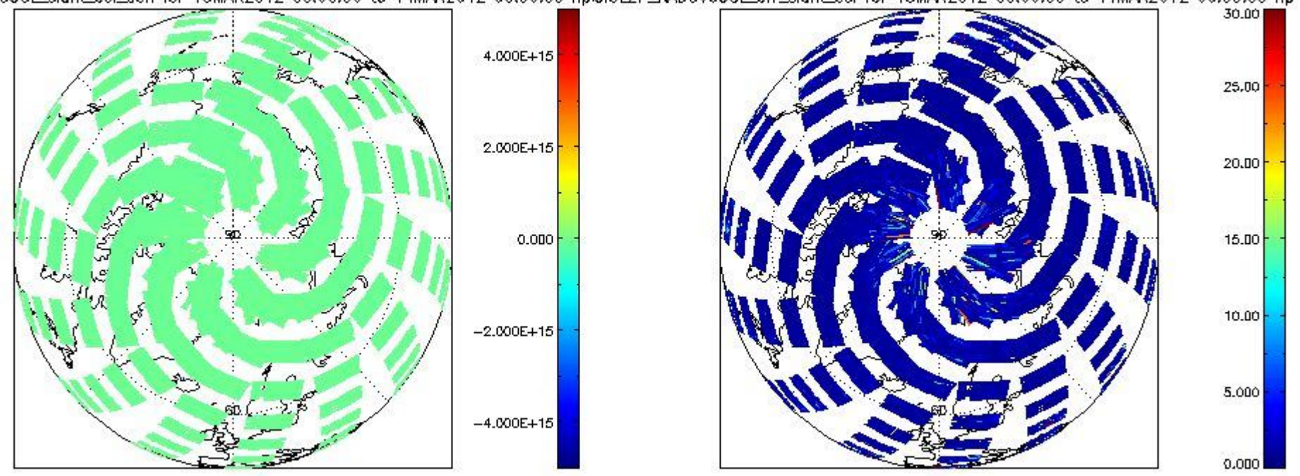
CIOL2P_NADUV6OCL_slant_col_den for 13MAR2012 00:00:00 to 14MAR2012 00:00:00 npCIOL2P_NADUV6OCL_err_slant_col for 13MAR2012 00:00:00 to 14MAR2012 00:00:00 np
