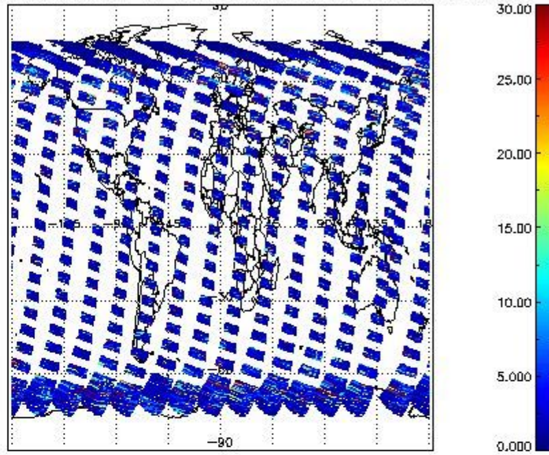
SCIOL2P_NADUV5SO2_vcd_err for 13MAR2012 00:00:00 to 14MAR2012 00:00:00
