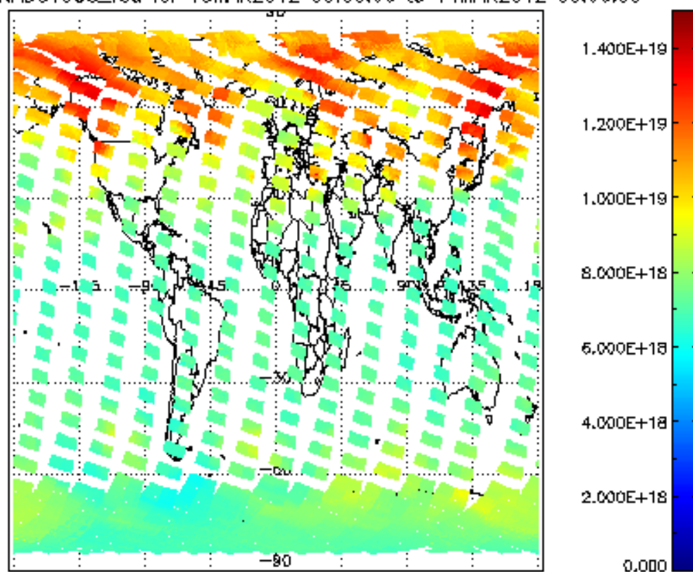
SCIOL2P_NADUV003_vcd for 13MAR2012 00:00:00 to 14MAR2012 00:00:00
