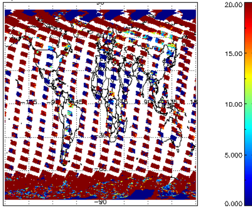
cL_opt_depth for 13MAR2012 00:00:00 to 14MAR2012 00:00:00
