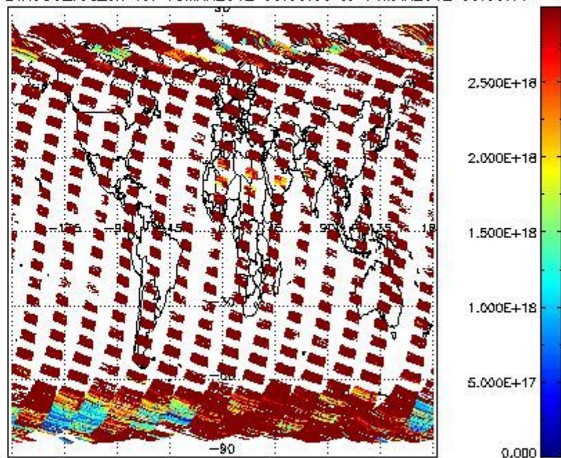
SCIO2P_NADIR3CO_vcd_err for 13MAR2012 00:00:00 to 14MAR2012 00:00:00
