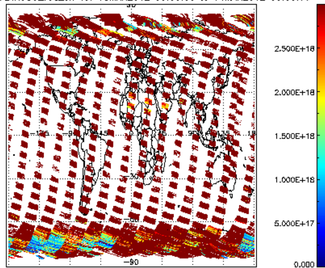
SCIOL2P_NADIR3CO_vcd_err for 13MAR2012 00:00:00 to 14MAR2012 00:00:00
