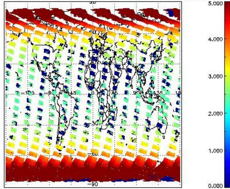
SCIOL2P_NADUV003_amf_cl for 13MAR2012 00:00:00 to 14MAR2012 00:00:00
