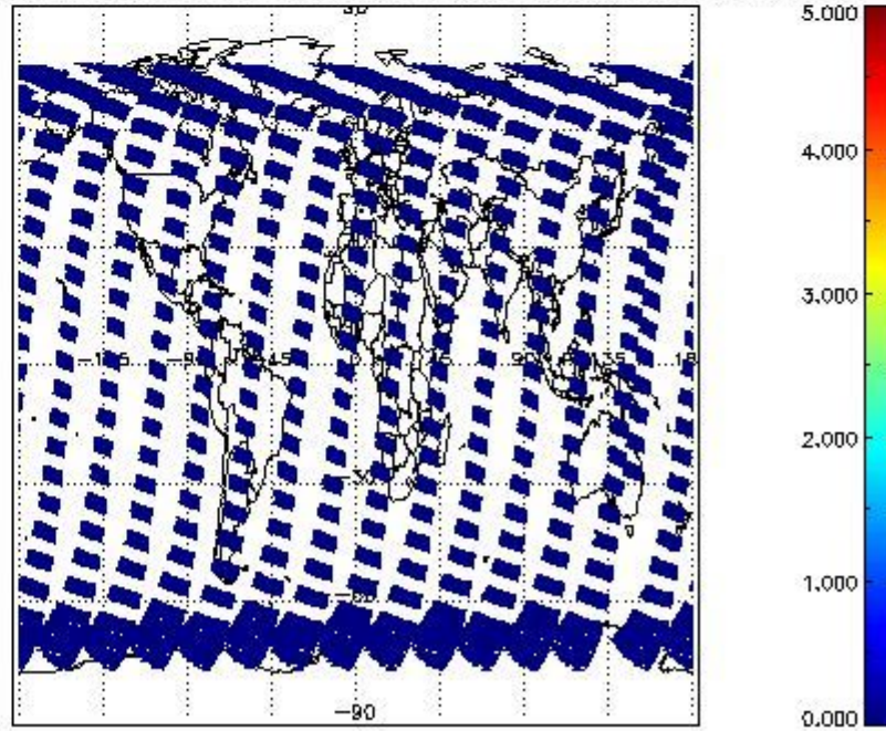
SCIOL2P_NADUV7S02_amf_cl for 13MAR2012 00:00:00 to 14MAR2012 00:00:00
