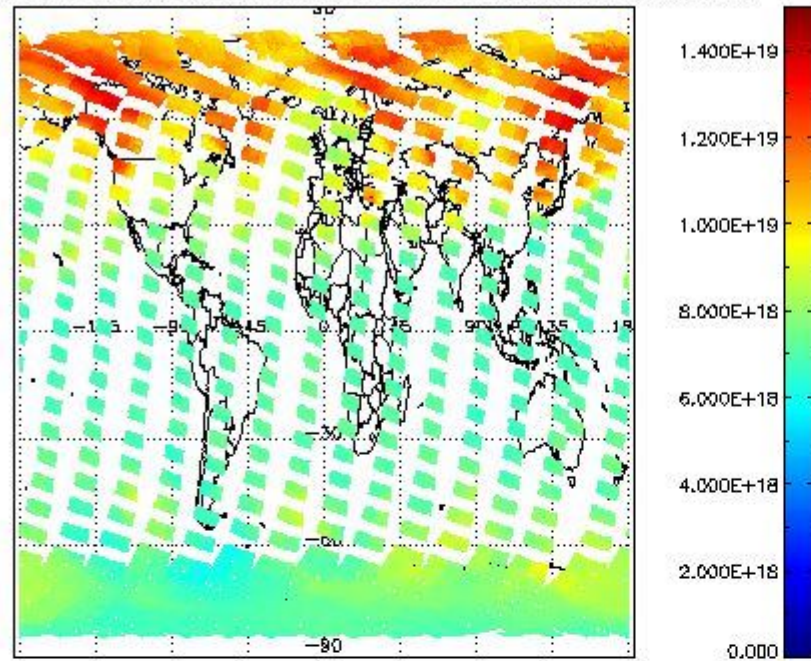
SCIOL2P_NADUV003_vcd for 13MAR2012 00:00:00 to 14MAR2012 00:00:00
