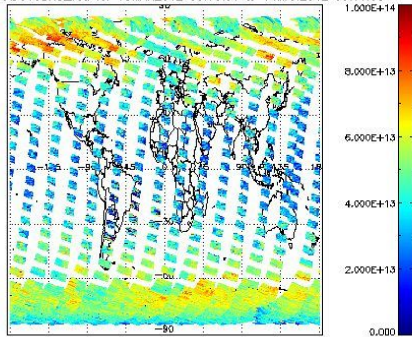
SCIOL2P_NADUV3BRO_vcd for 13MAR2012 00:00:00 to 14MAR2012 00:00:00
