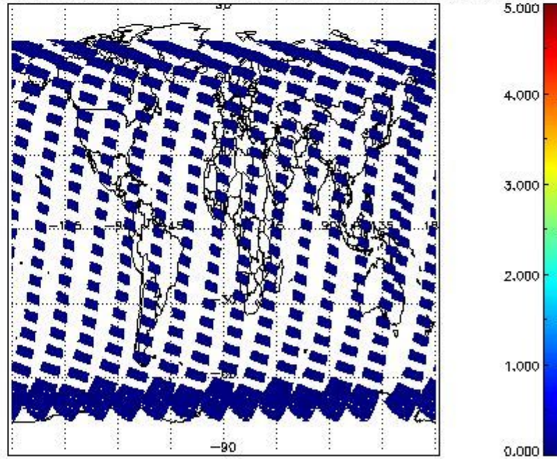
SCIOL2P_NADUV5SO2_amf_cl for 13MAR2012 00:00:00 to 14MAR2012 00:00:00
