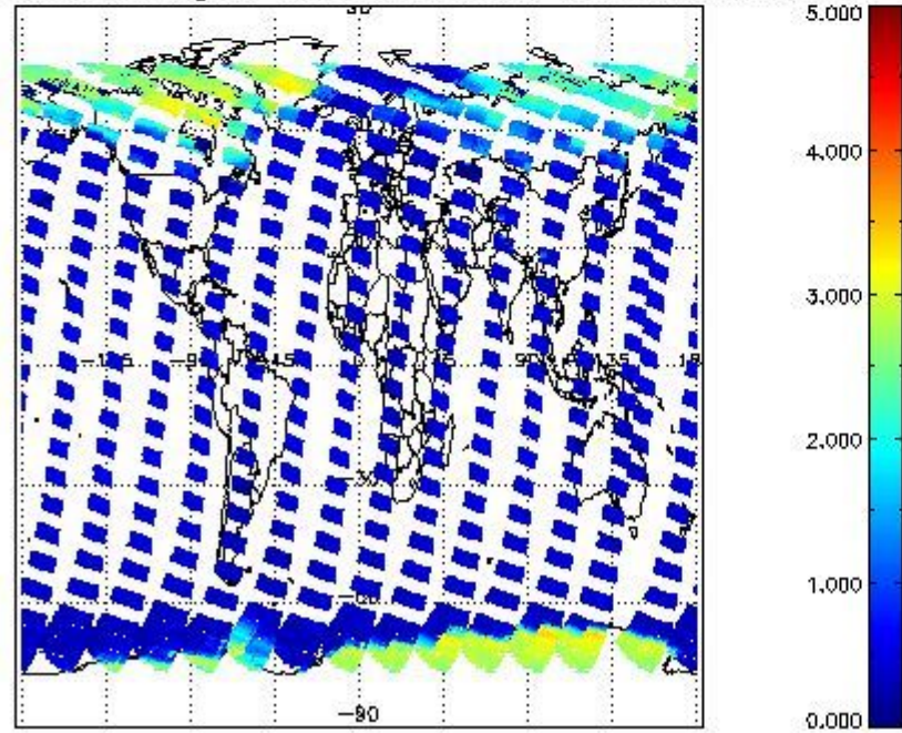
SCIOL2P_NADUV5SO2_amf_gr for 13MAR2012 00:00:00 to 14MAR2012 00:00:00
