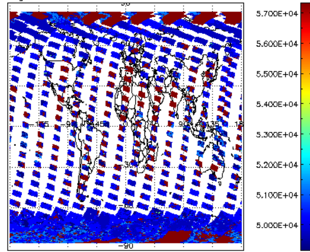
cloud_flags for 13MAR2012 00:00:00 to 14MAR2012 00:00:00
