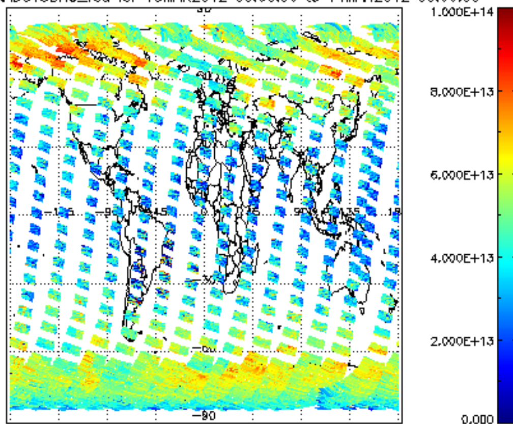
SCIOL2P_NADUV3BRO_vcd for 13MAR2012 00:00:00 to 14MAR2012 00:00:00
