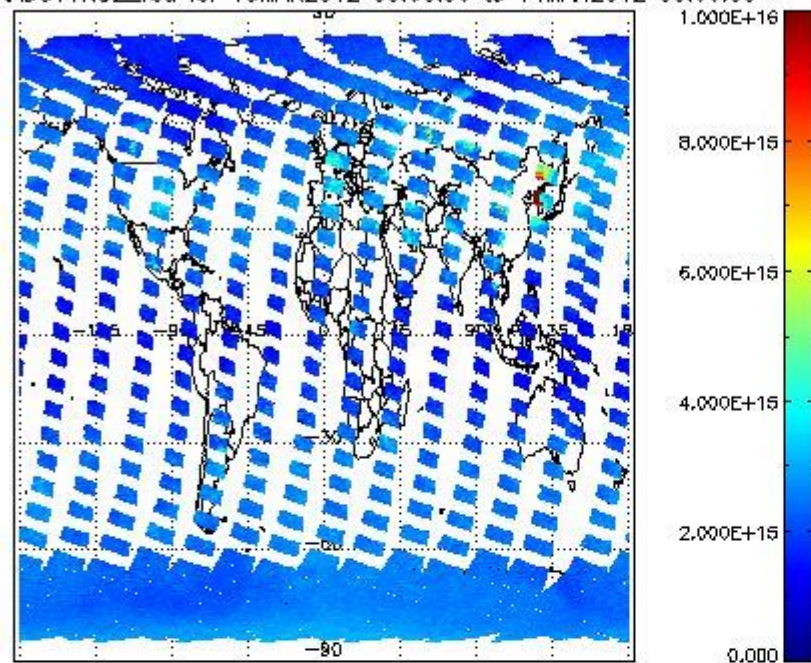
SCIOL2P_NADUV1NO2_vcd for 13MAR2012 00:00:00 to 14MAR2012 00:00:00
