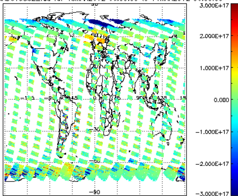
SCIOL2P_NADUV5S02_vcd for 13MAR2012 00:00:00 to 14MAR2012 00:00:00
