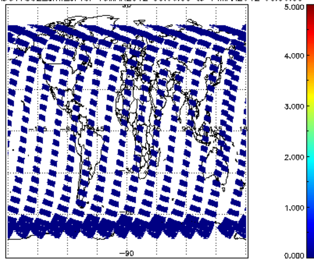
SCIOL2P_NADUV7S02_amf_cl for 13MAR2012 00:00:00 to 14MAR2012 00:00:00
