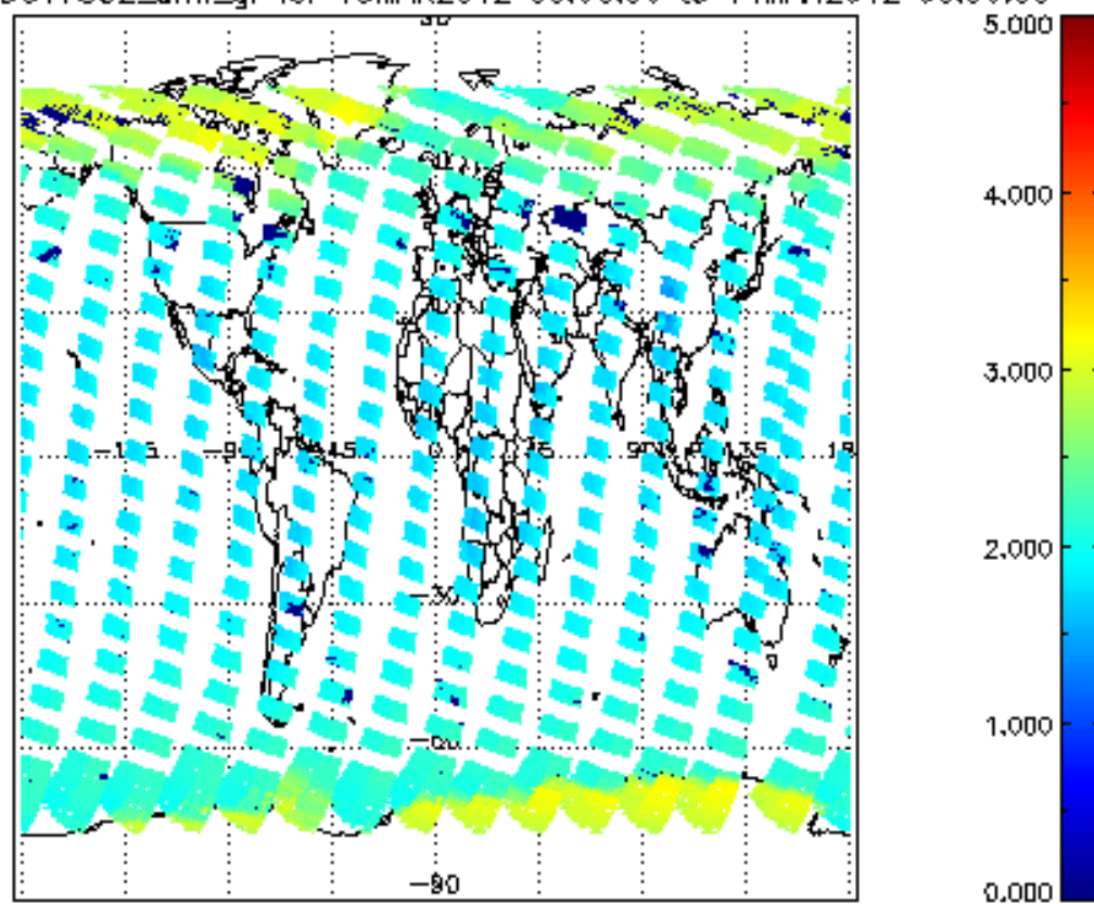
SCIOL2P_NADUV7S02_amf_gr for 13MAR2012 00:00:00 to 14MAR2012 00:00:00
