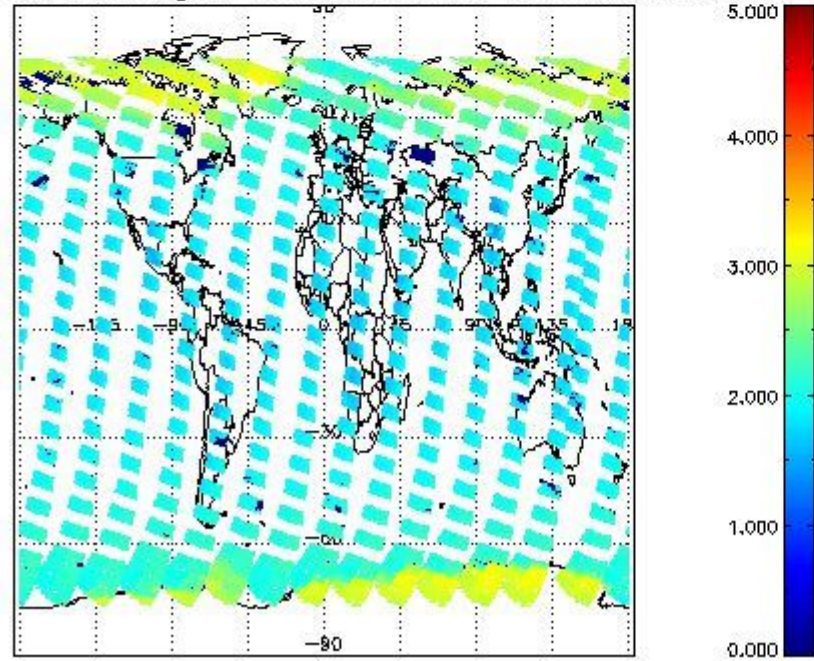
SCIOL2P_NADUV7S02_amf_gr for 13MAR2012 00:00:00 to 14MAR2012 00:00:00
