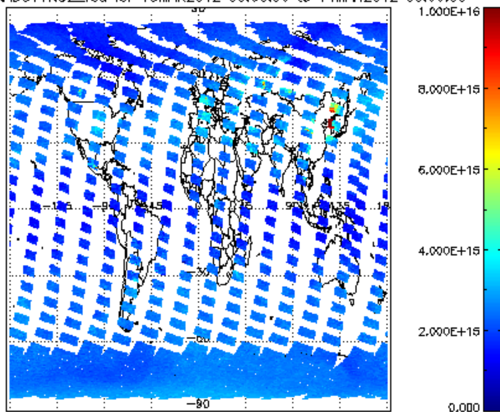
SCIOL2P_NADUV1NO2_vcd for 13MAR2012 00:00:00 to 14MAR2012 00:00:00
