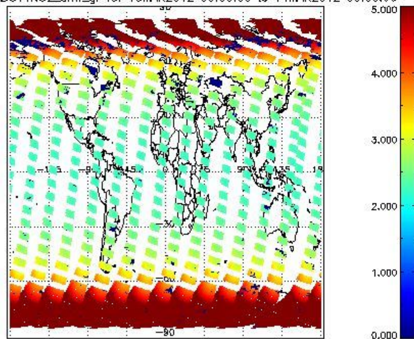
SCIOL2P_NADUV1NO2_amf_gr for 13MAR2012 00:00:00 to 14MAR2012 00:00:00
