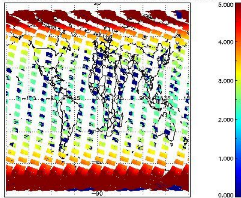
SCIOL2P_NADUV3BRO_amf_cl for 13MAR2012 00:00:00 to 14MAR2012 00:00:00
