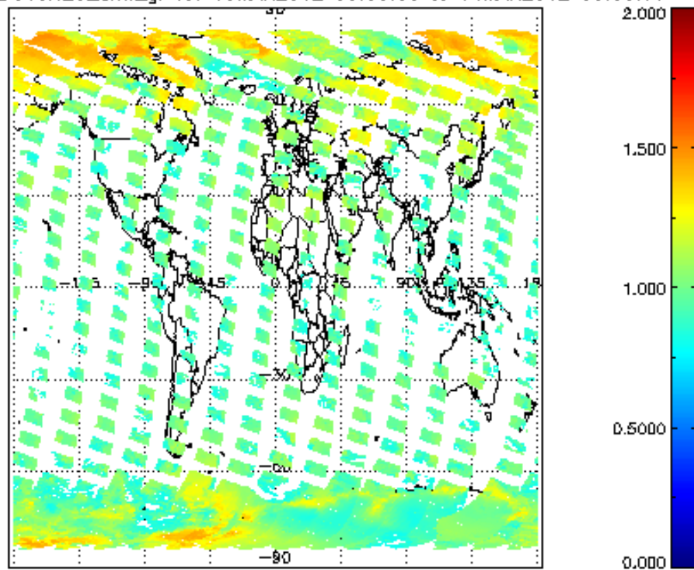
SCIOL2P_NADUV8H2O_arnf_gr for 13MAR2012 00:00:00 to 14MAR2012 00:00:00
