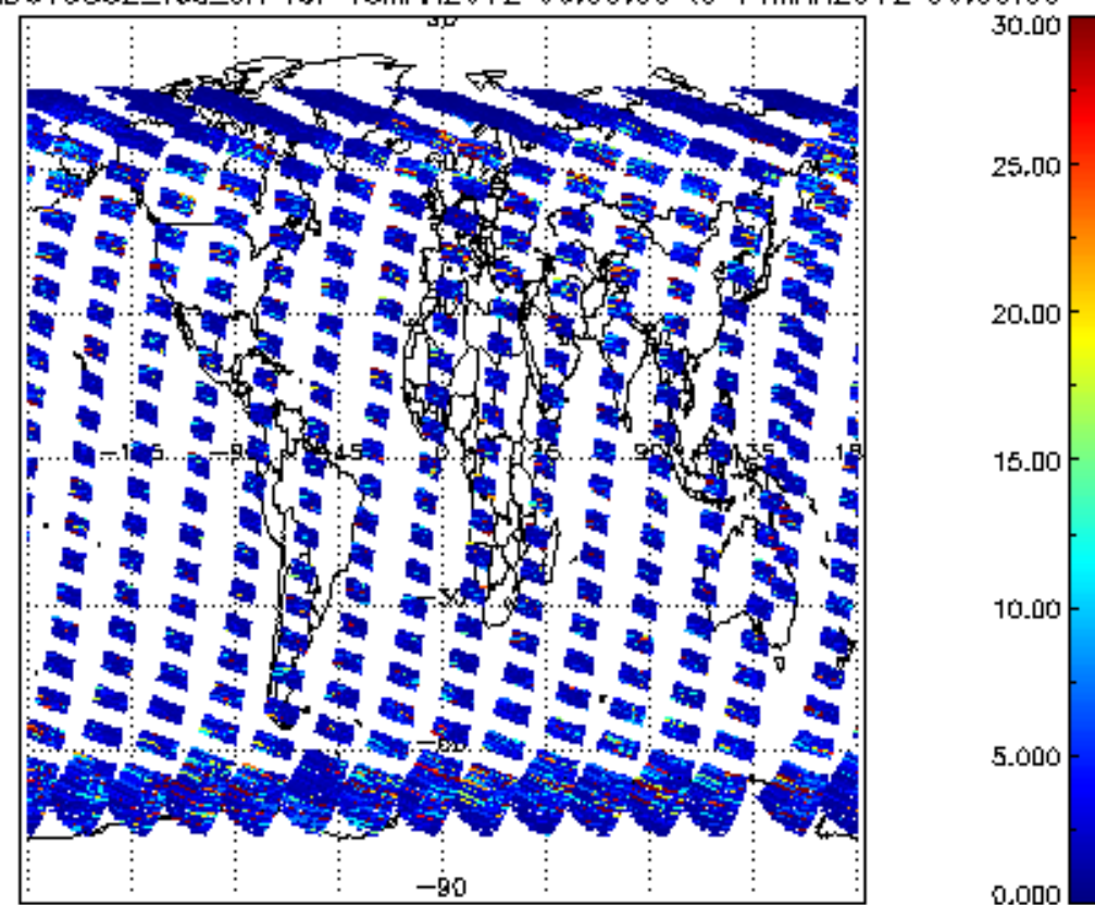
SCIOL2P_NADUV5S02_vcd_err for 13MAR2012 00:00:00 to 14MAR2012 00:00:00
