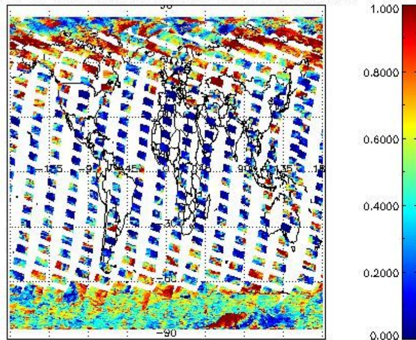
cL_frac for 13MAR2012 00:00:00 to 14MAR2012 00:00:00
