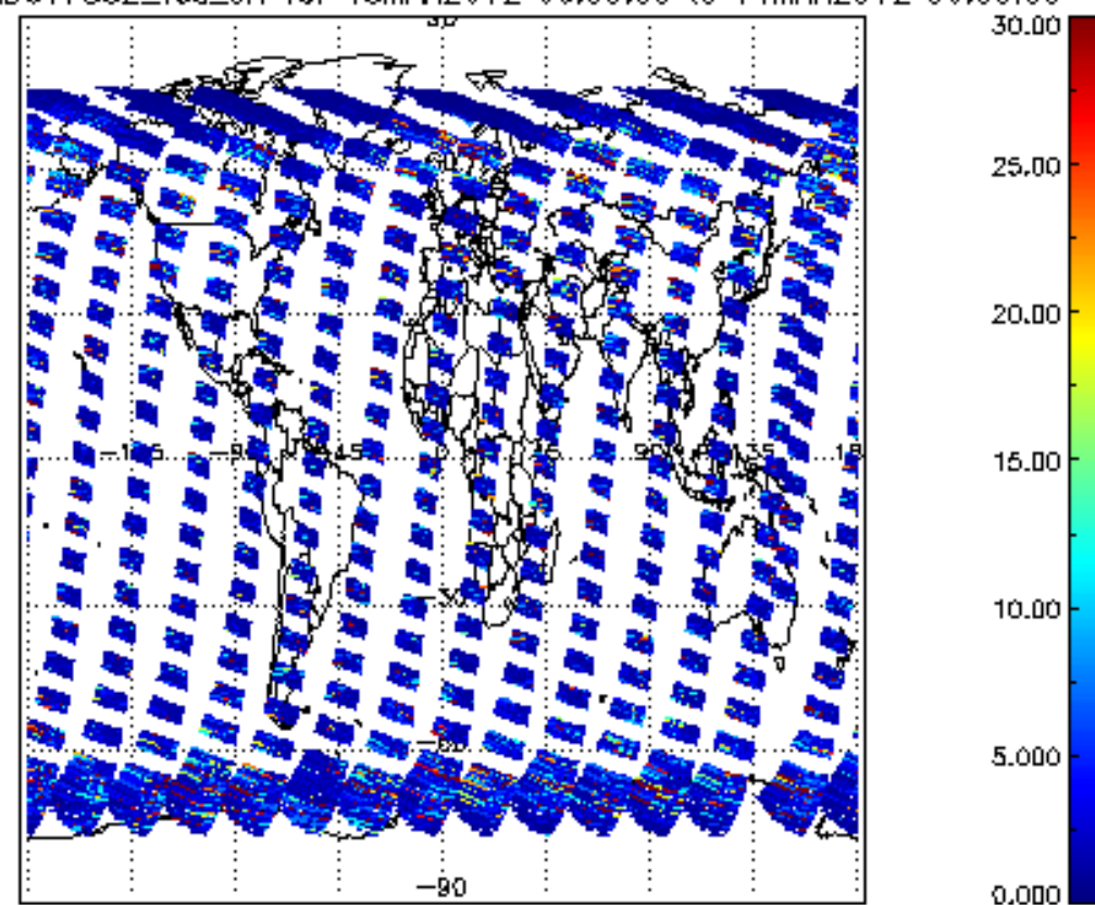
SCIOL2P_NADUV7S02_vcd_err for 13MAR2012 00:00:00 to 14MAR2012 00:00:00
