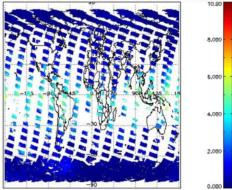
SCIOL2P_NADUV8H2O_vcd for 13MAR2012 00:00:00 to 14MAR2012 00:00:00
