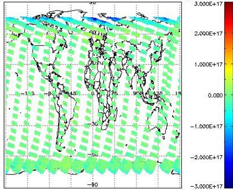
SCIOL2P_NADUV7S02_vcd for 13MAR2012 00:00:00 to 14MAR2012 00:00:00
