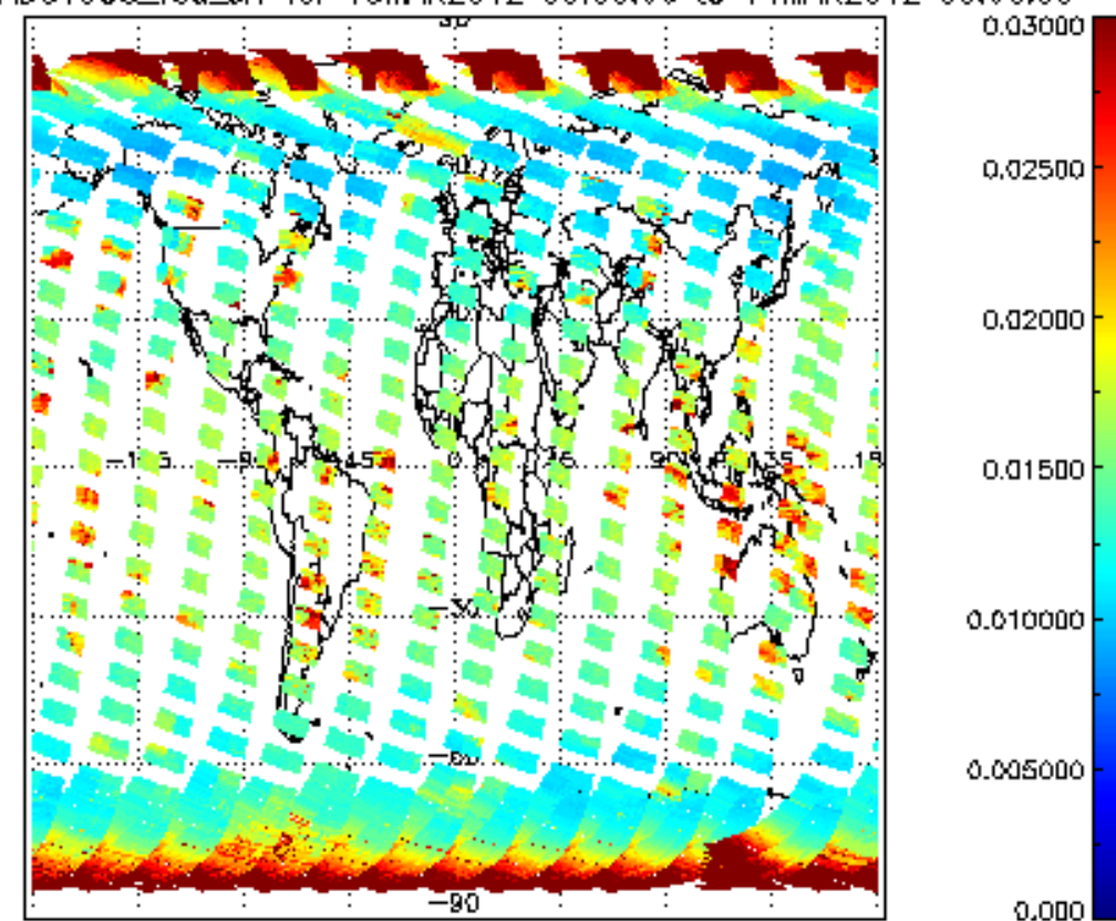
SCIOL2P_NADUV003_vcd_err for 13MAR2012 00:00:00 to 14MAR2012 00:00:00
