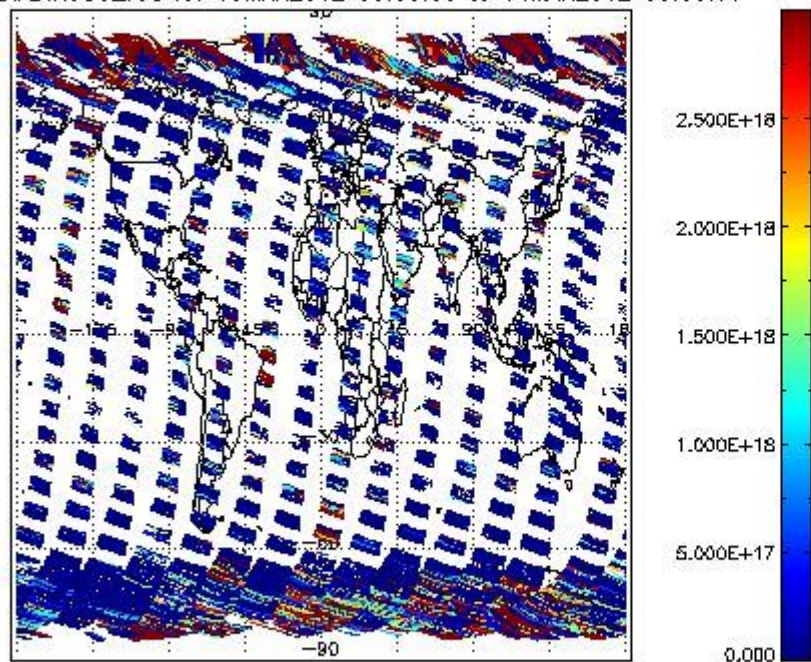
SCIO2P_NADIR3CO_vcd for 13MAR2012 00:00:00 to 14MAR2012 00:00:00
