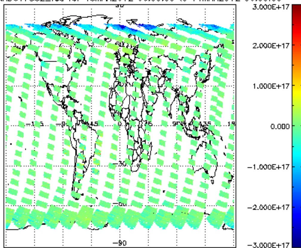
SCIOL2P_NADUV7S02_vcd for 13MAR2012 00:00:00 to 14MAR2012 00:00:00
