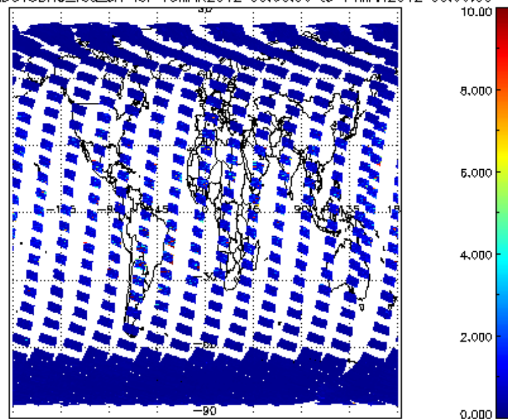
SCIOL2P_NADUV3BRO_vcd_Lerr for 13MAR2012 00:00:00 to 14MAR2012 00:00:00
