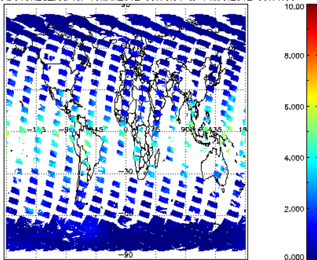
SCIOL2P_NADUV8H2O_vcd for 13MAR2012 00:00:00 to 14MAR2012 00:00:00
