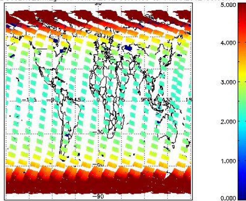
SCIOL2P_NADUV3BRO_amf_gr for 13MAR2012 00:00:00 to 14MAR2012 00:00:00
