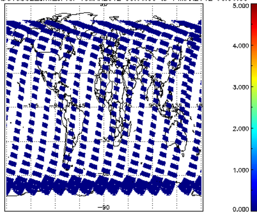
SCIOL2P_NADUV5S02_amf_cl for 13MAR2012 00:00:00 to 14MAR2012 00:00:00
