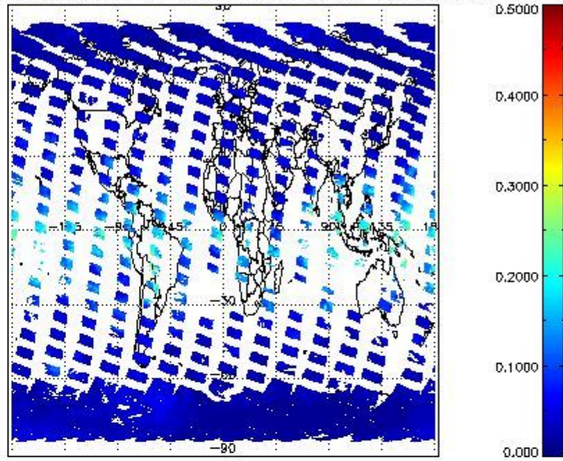
SCIOL2P_NADUV8H2O_vcd_err for 13MAR2012 00:00:00 to 14MAR2012 00:00:00
