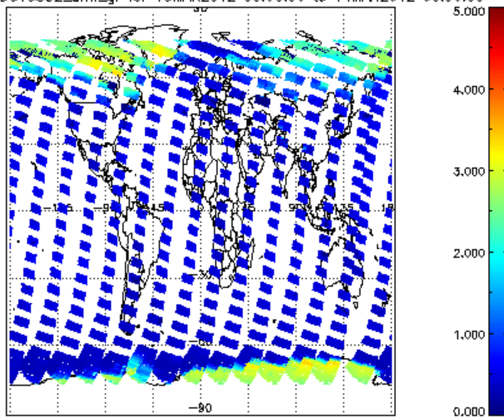
SCIOL2P_NADUV5S02_amf_gr for 13MAR2012 00:00:00 to 14MAR2012 00:00:00
