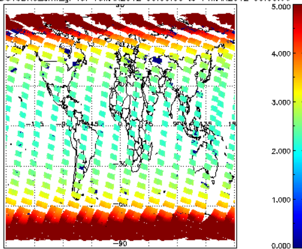
SCIOL2P_NADUV3BRO_arnf_gr for 13MAR2012 00:00:00 to 14MAR2012 00:00:00
