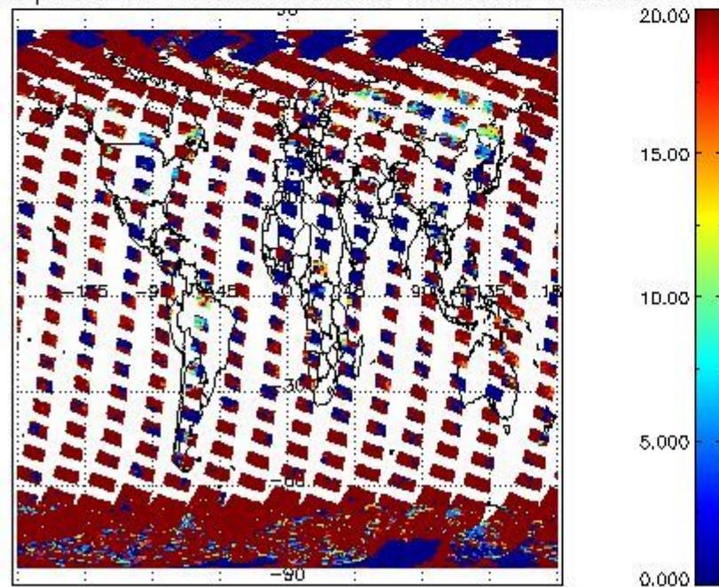
cL_opt_depth for 13MAR2012 00:00:00 to 14MAR2012 00:00:00
