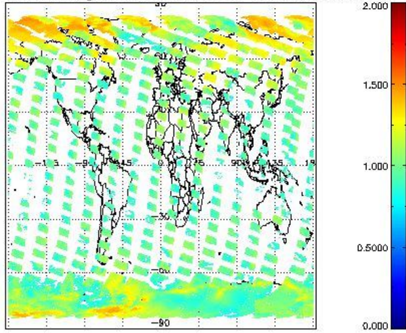
SCIOL2P_NADUV8H2O_amf_gr for 13MAR2012 00:00:00 to 14MAR2012 00:00:00
