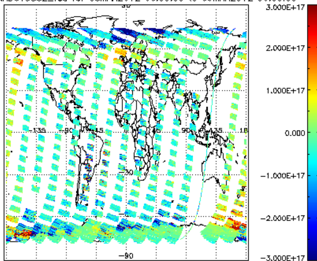
SCIOL2P_NADUV5S02_vcd for 08MAR2012 00:00:00 to 09MAR2012 00:00:00
