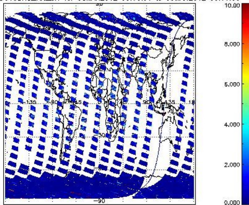
SCIOL2P_NADUV3BRO_vcd_err for 08MAR2012 00:00:00 to 09MAR2012 00:00:00
