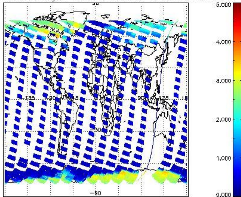
SCIOL2P_NADUV5S02_amf_gr for 08MAR2012 00:00:00 to 09MAR2012 00:00:00
