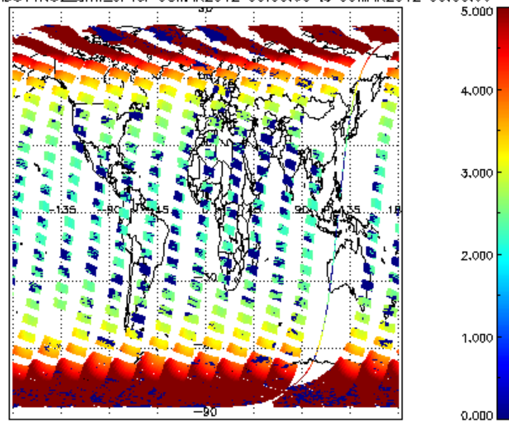
SCIOL2P_NADUV1NO2_amf_cl for 08MAR2012 00:00:00 to 09MAR2012 00:00:00
