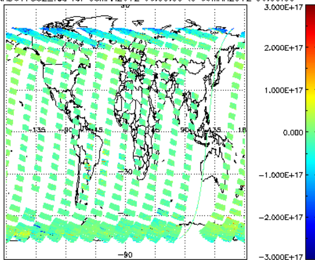
SCIOL2P_NADUV7S02_vcd for 08MAR2012 00:00:00 to 09MAR2012 00:00:00
