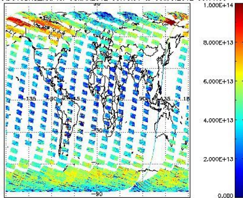
SCIOL2P_NADUV3BRO_vcd for 08MAR2012 00:00:00 to 09MAR2012 00:00:00
