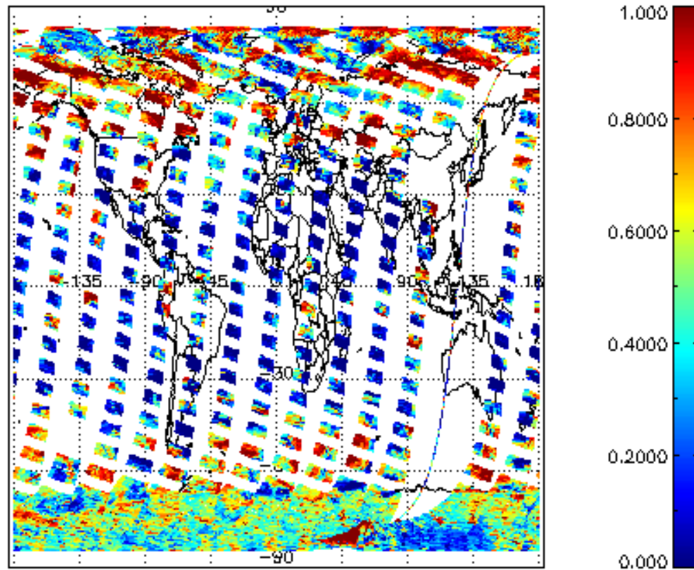
cL_frac for 08MAR2012 00:00:00 to 09MAR2012 00:00:00
