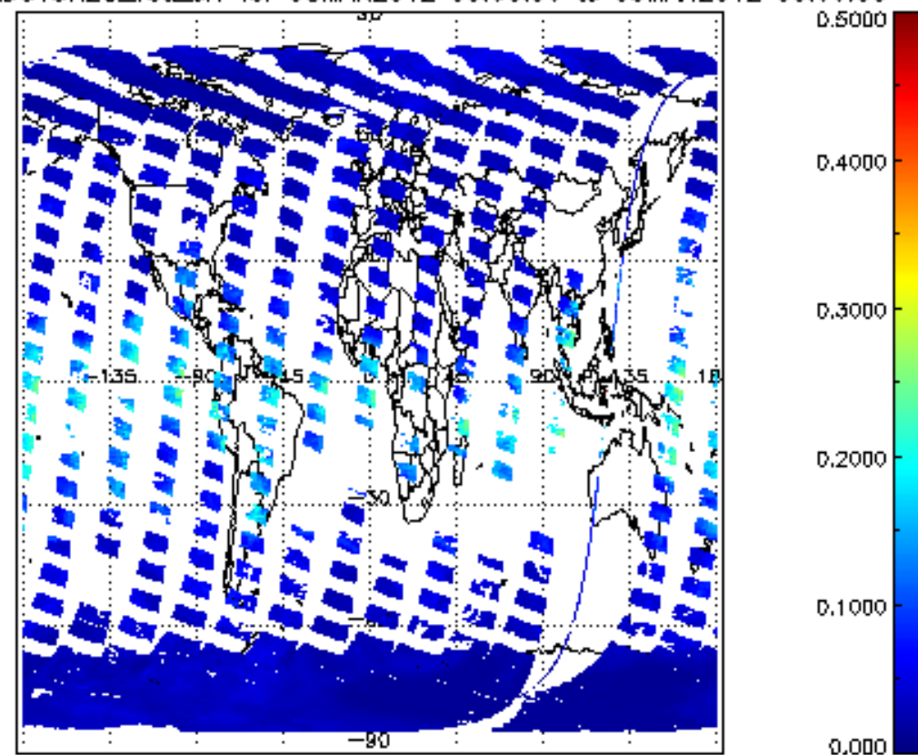
SCIOL2P_NADUV8H20_vcd_Lerr for 08MAR2012 00:00:00 to 09MAR2012 00:00:00
