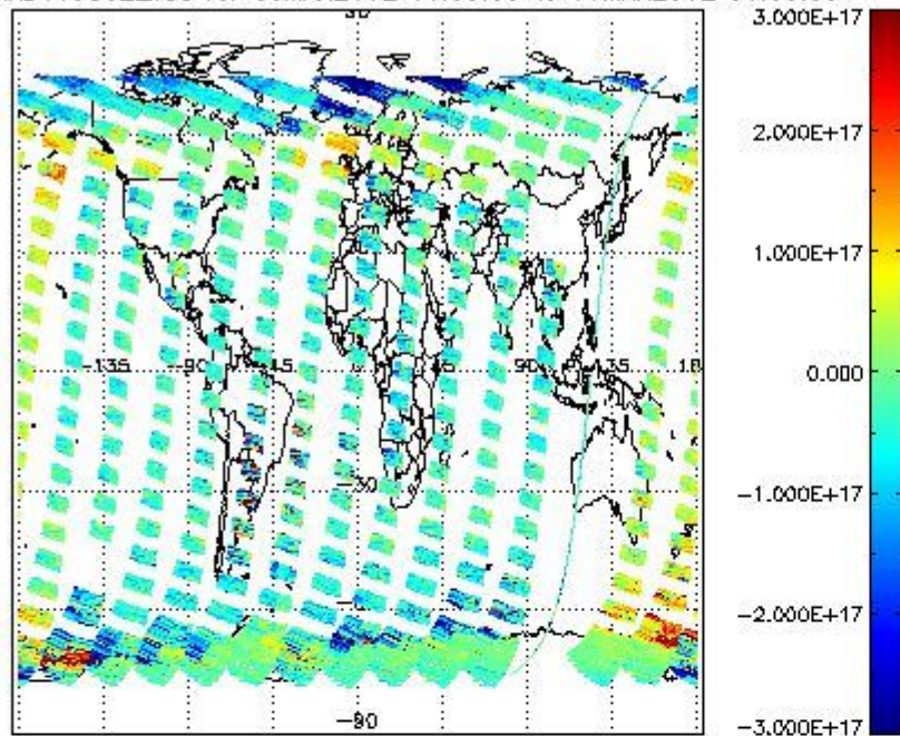
SCIOL2P_NADUV5S02_vcd for 08MAR2012 00:00:00 to 09MAR2012 00:00:00
