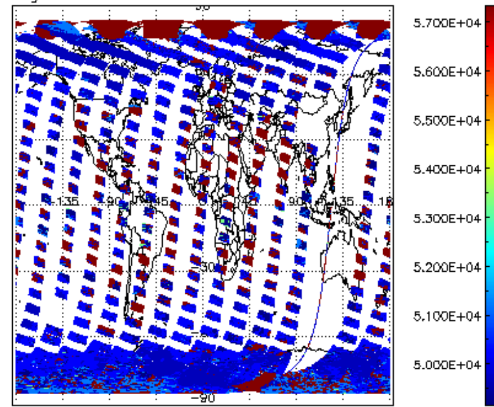
cloud_flags for 08MAR2012 00:00:00 to 09MAR2012 00:00:00
