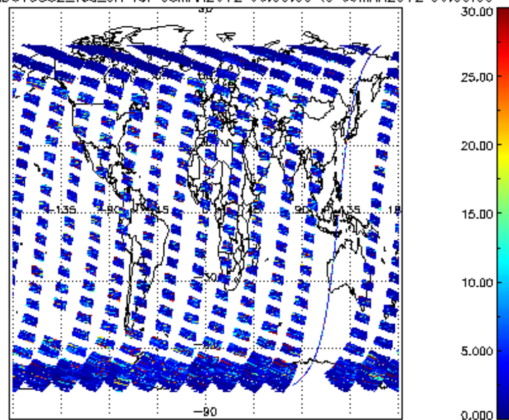
SCIOL2P_NADUV5S02_vcd_err for 08MAR2012 00:00:00 to 09MAR2012 00:00:00
