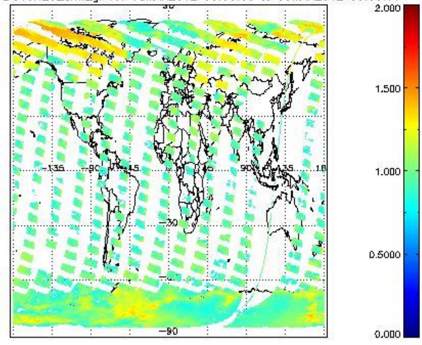
SCIOL2P_NADUV8H2O_arnf_gr for 08MAR2012 00:00:00 to 09MAR2012 00:00:00
