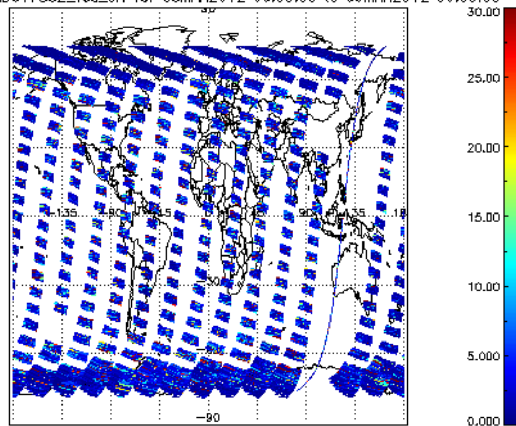
SCIOL2P_NADUV7S02_vcd_err for 08MAR2012 00:00:00 to 09MAR2012 00:00:00
