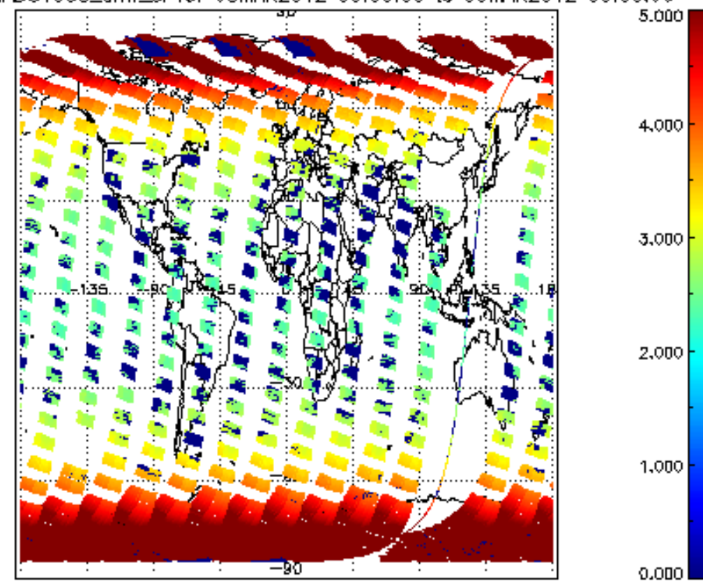
SCIOL2P_NADUV003_arnf_cl for 08MAR2012 00:00:00 to 09MAR2012 00:00:00
