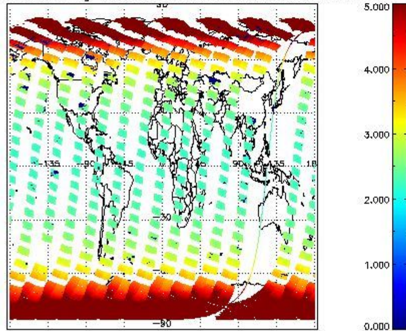
SCIOL2P_NADUV003_amf_gr for 08MAR2012 00:00:00 to 09MAR2012 00:00:00
