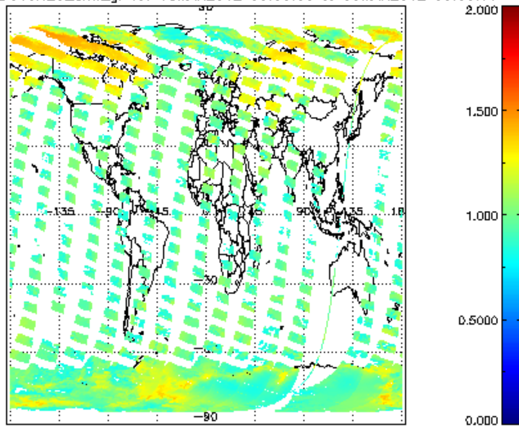
SCIOL2P_NADUV8H20_arnf_gr for 08MAR2012 00:00:00 to 09MAR2012 00:00:00
