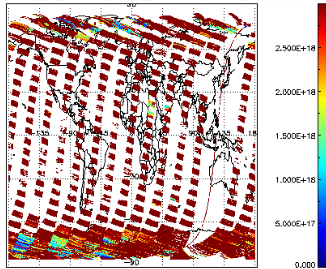
SCIOL2P_NADIR3CO_vcd_err for 08MAR2012 00:00:00 to 09MAR2012 00:00:00
