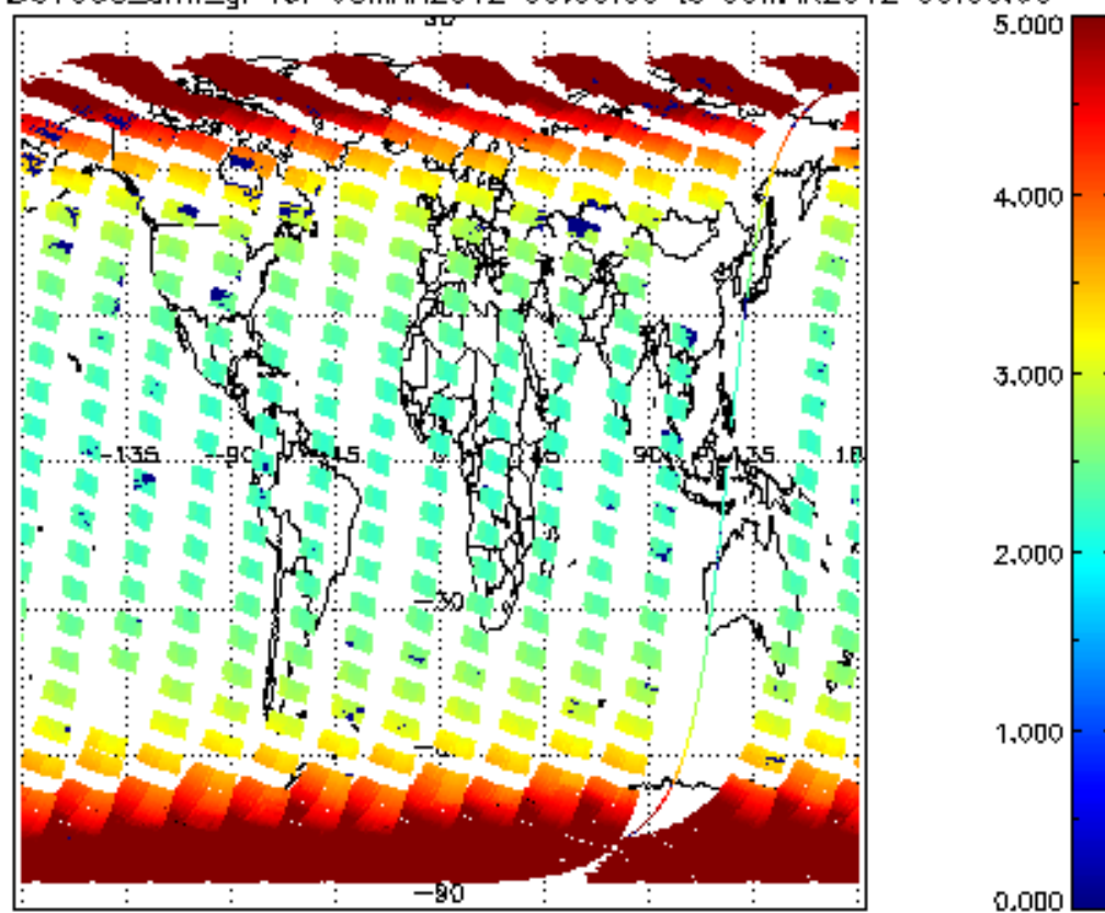
SCIOL2P_NADUV003_arnf_gr for 08MAR2012 00:00:00 to 09MAR2012 00:00:00
