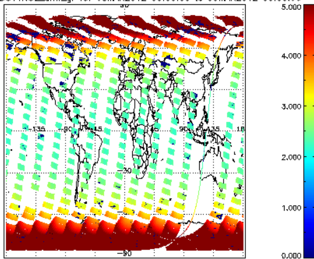
SCIOL2P_NADUV1NO2_amf_gr for 08MAR2012 00:00:00 to 09MAR2012 00:00:00
