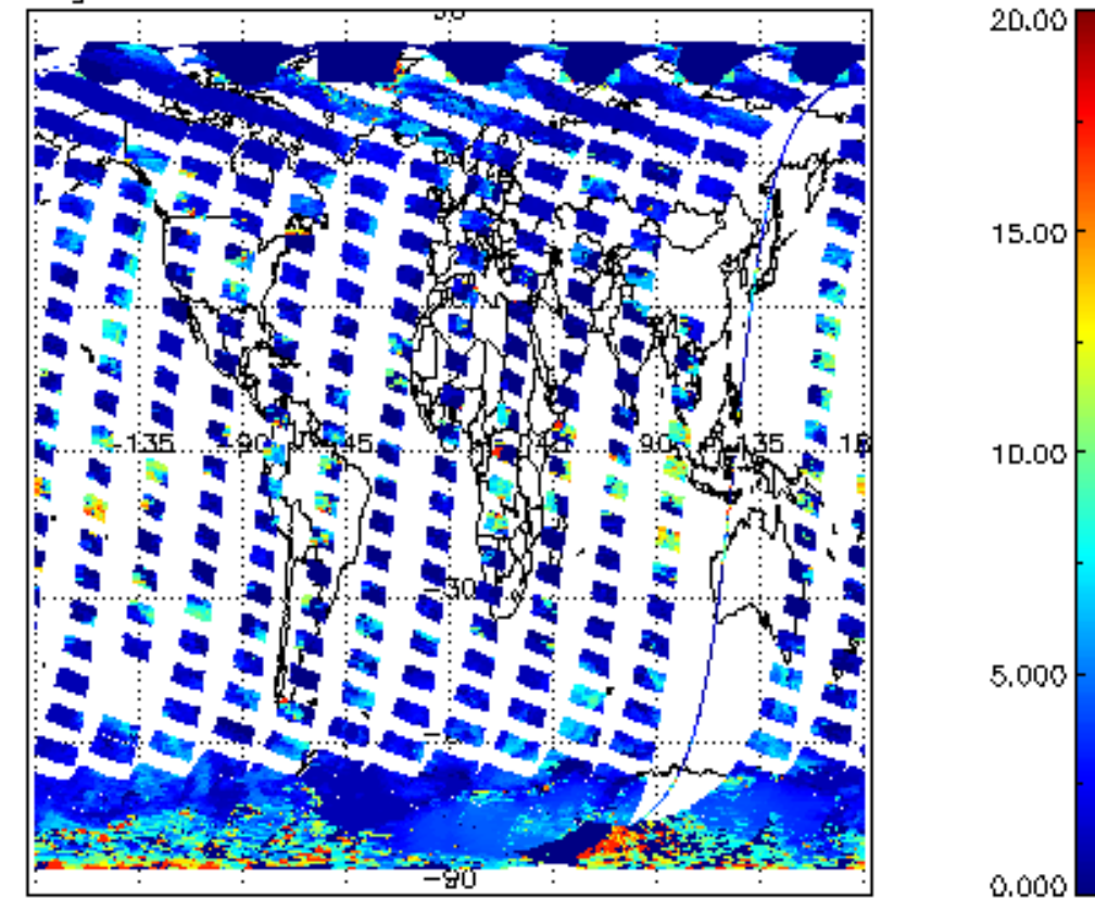
cL_top_height for 08MAR2012 00:00:00 to 09MAR2012 00:00:00
