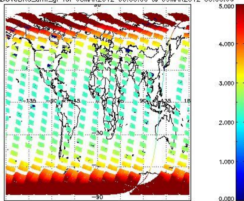
SCIOL2P_NADUV3BRO_amf_gr for 08MAR2012 00:00:00 to 09MAR2012 00:00:00
