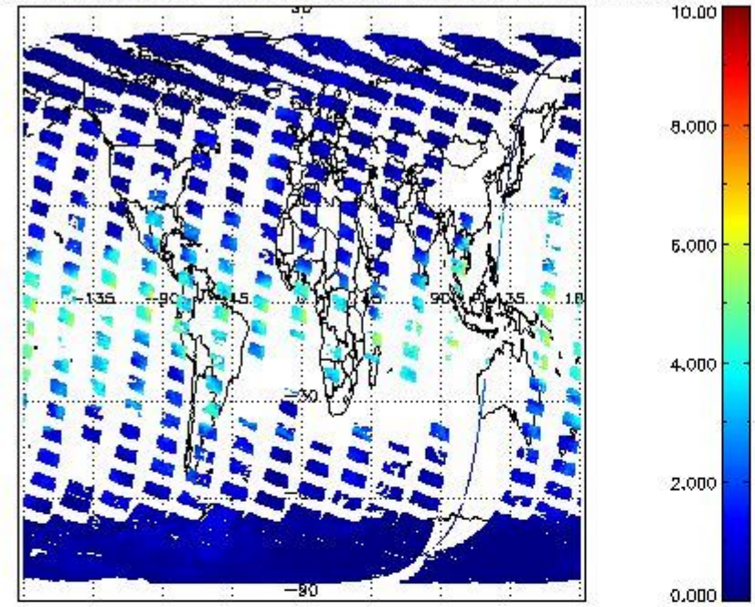
SCIOL2P_NADUV8H2O_vcd for 08MAR2012 00:00:00 to 09MAR2012 00:00:00
