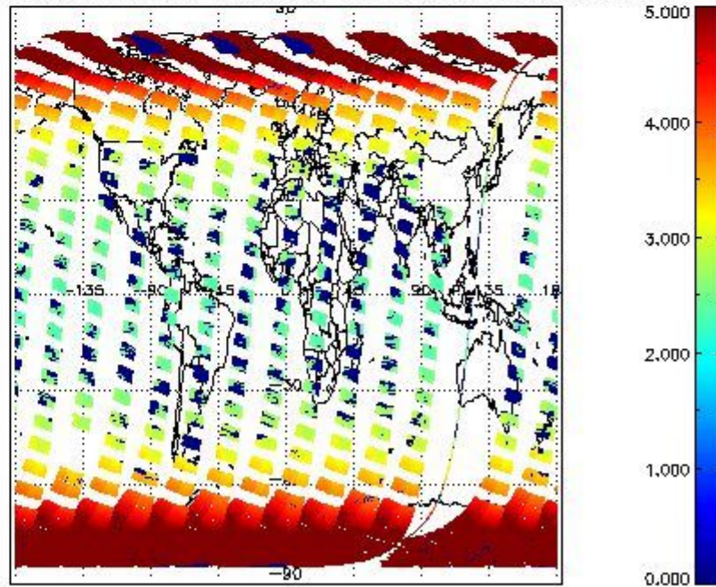
SCIOL2P_NADUV003_amf_cl for 08MAR2012 00:00:00 to 09MAR2012 00:00:00
