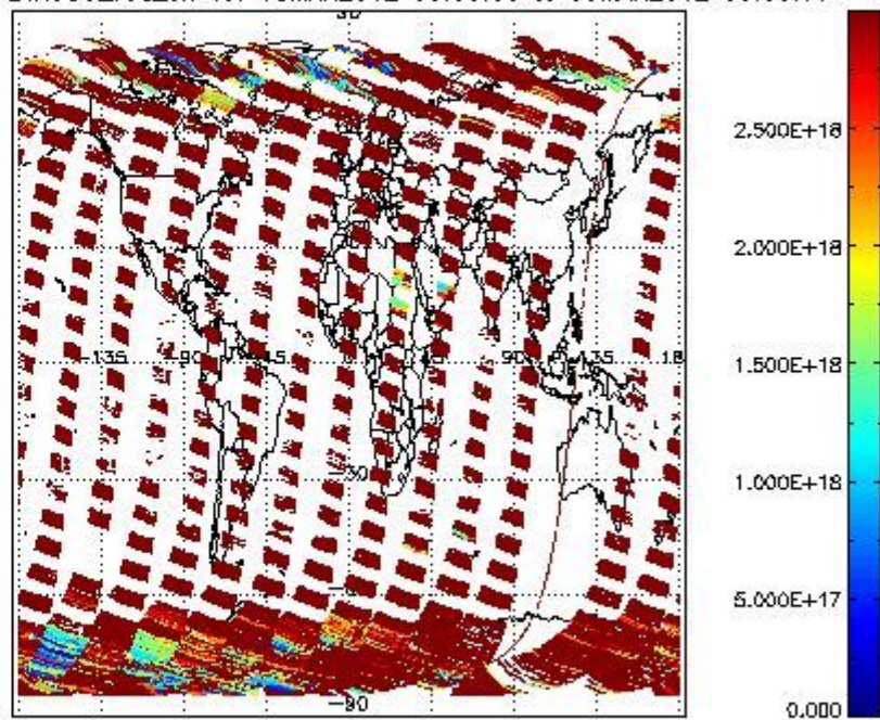
SCIOL2P_NADIR3CO_vcd_err for 08MAR2012 00:00:00 to 09MAR2012 00:00:00
