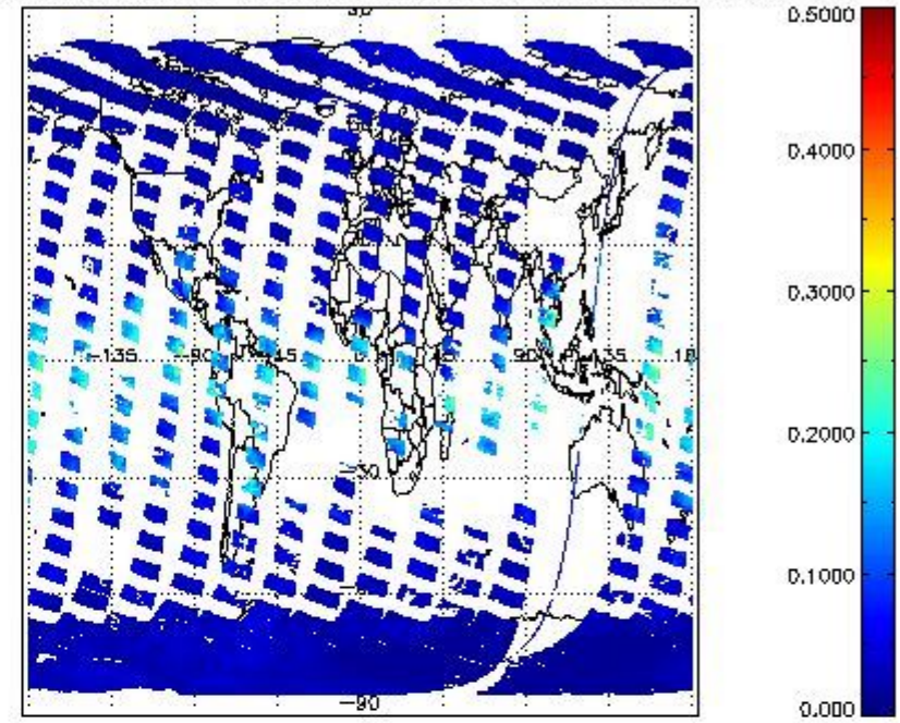
SCIOL2P_NADUV8H2O_vcd_err for 08MAR2012 00:00:00 to 09MAR2012 00:00:00
