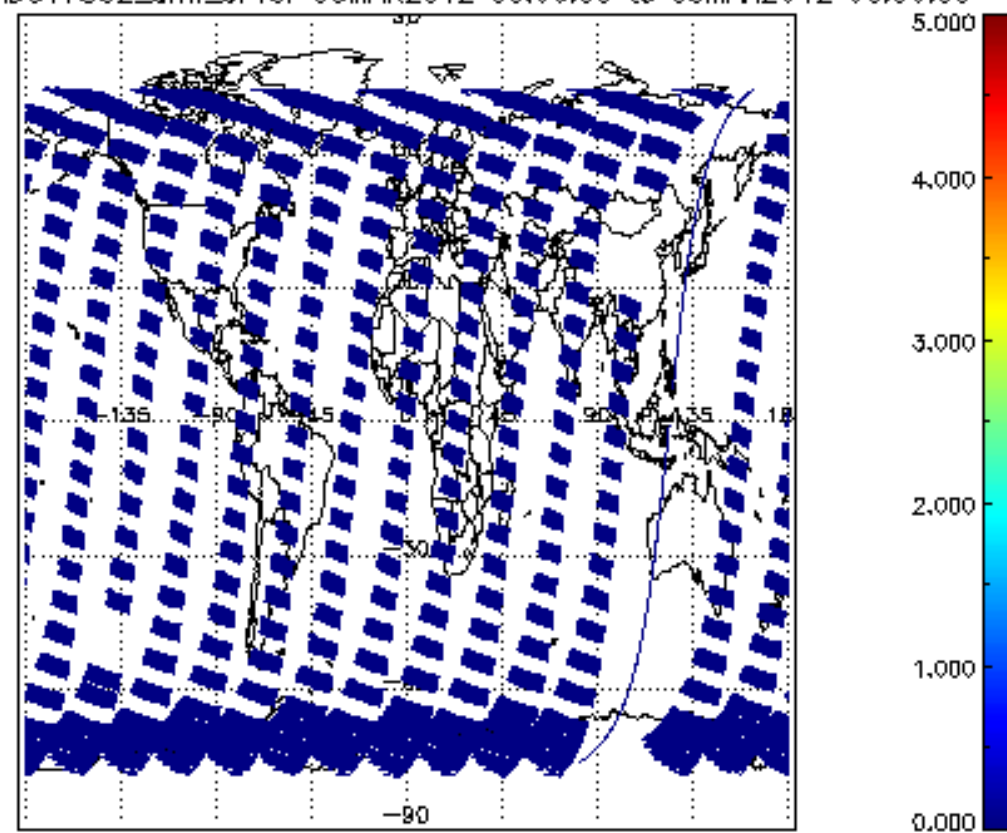
SCIOL2P_NADUV7S02_amf_cl for 08MAR2012 00:00:00 to 09MAR2012 00:00:00
