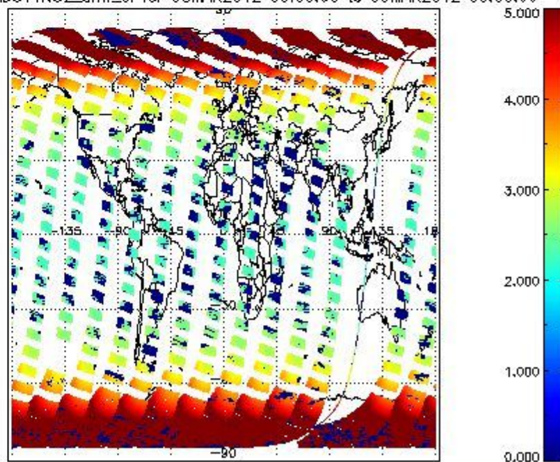
SCIOL2P_NADUV1NO2_amf_cl for 08MAR2012 00:00:00 to 09MAR2012 00:00:00
