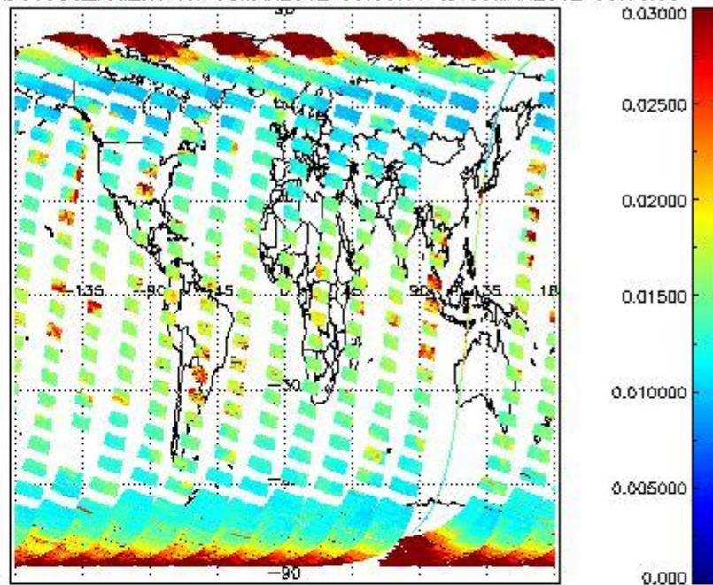
SCIOL2P_NADUV003_vcd_err for 08MAR2012 00:00:00 to 09MAR2012 00:00:00
