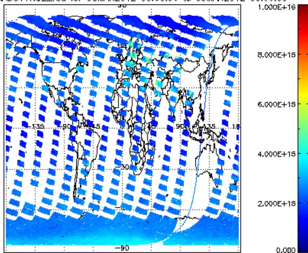
SCIOL2P_NADUV1NO2_vcd for 08MAR2012 00:00:00 to 09MAR2012 00:00:00
