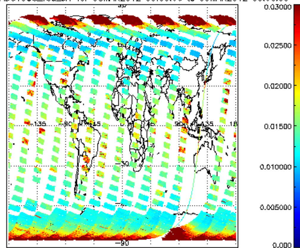
SCIOL2P_NADUV003_vcd_err for 08MAR2012 00:00:00 to 09MAR2012 00:00:00
