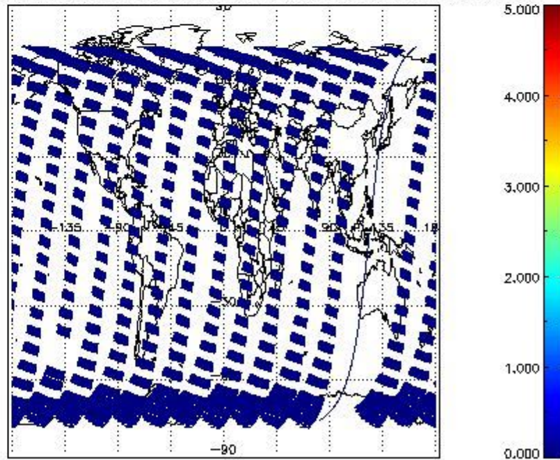
SCIOL2P_NADUV7S02_amf_cl for 08MAR2012 00:00:00 to 09MAR2012 00:00:00
