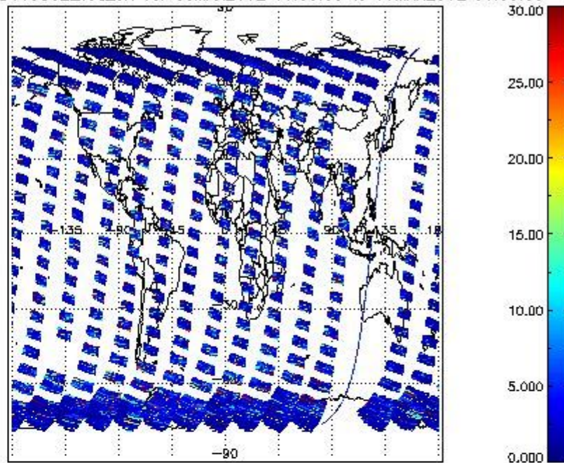
SCIOL2P_NADUV5S02_vcd_err for 08MAR2012 00:00:00 to 09MAR2012 00:00:00
