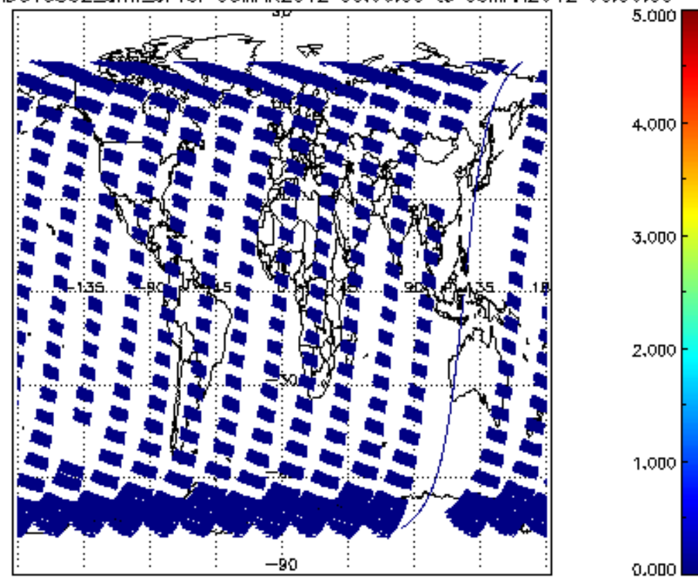
SCIOL2P_NADUV5S02_amf_cl for 08MAR2012 00:00:00 to 09MAR2012 00:00:00
