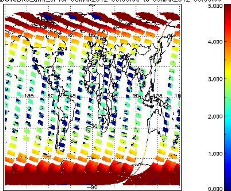
SCIOL2P_NADUV3BRO_amf_cl for 08MAR2012 00:00:00 to 09MAR2012 00:00:00
