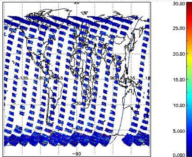
SCIOL2P_NADUV7S02_vcd_err for 08MAR2012 00:00:00 to 09MAR2012 00:00:00
