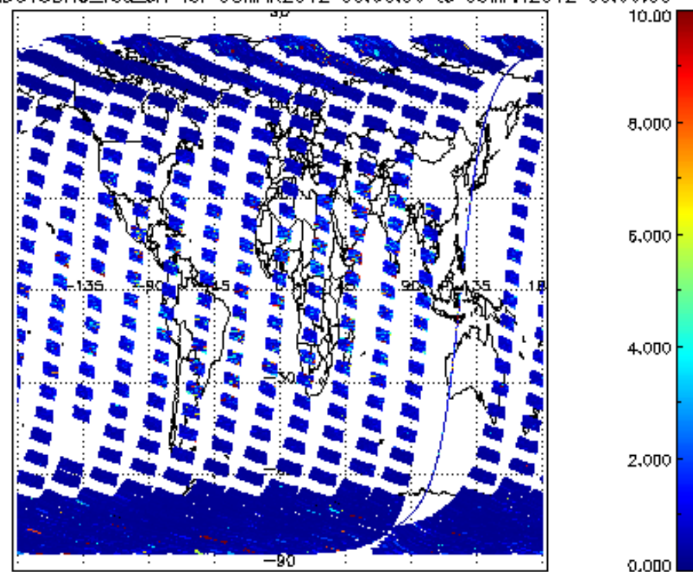
SCIOL2P_NADUV3BRO_vcd_err for 08MAR2012 00:00:00 to 09MAR2012 00:00:00
