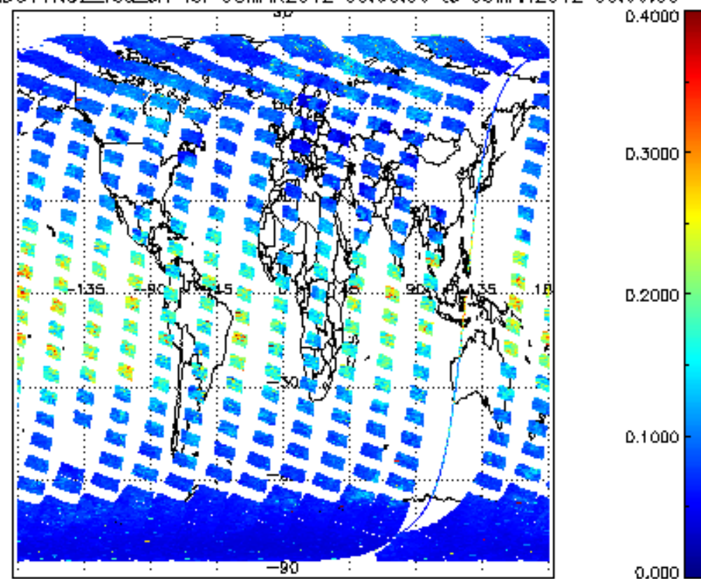
SCIOL2P_NADUV1NO2_vcd_err for 08MAR2012 00:00:00 to 09MAR2012 00:00:00
