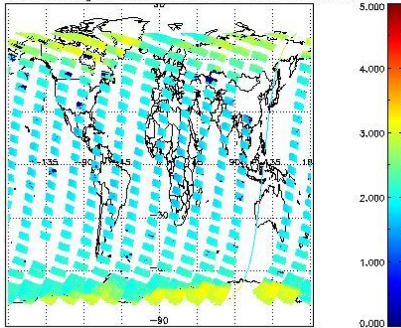
SCIOL2P_NADUV7S02_amf_gr for 08MAR2012 00:00:00 to 09MAR2012 00:00:00
