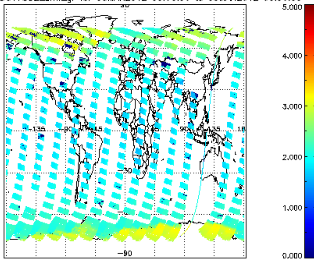
SCIOL2P_NADUV7S02_amf_gr for 08MAR2012 00:00:00 to 09MAR2012 00:00:00
