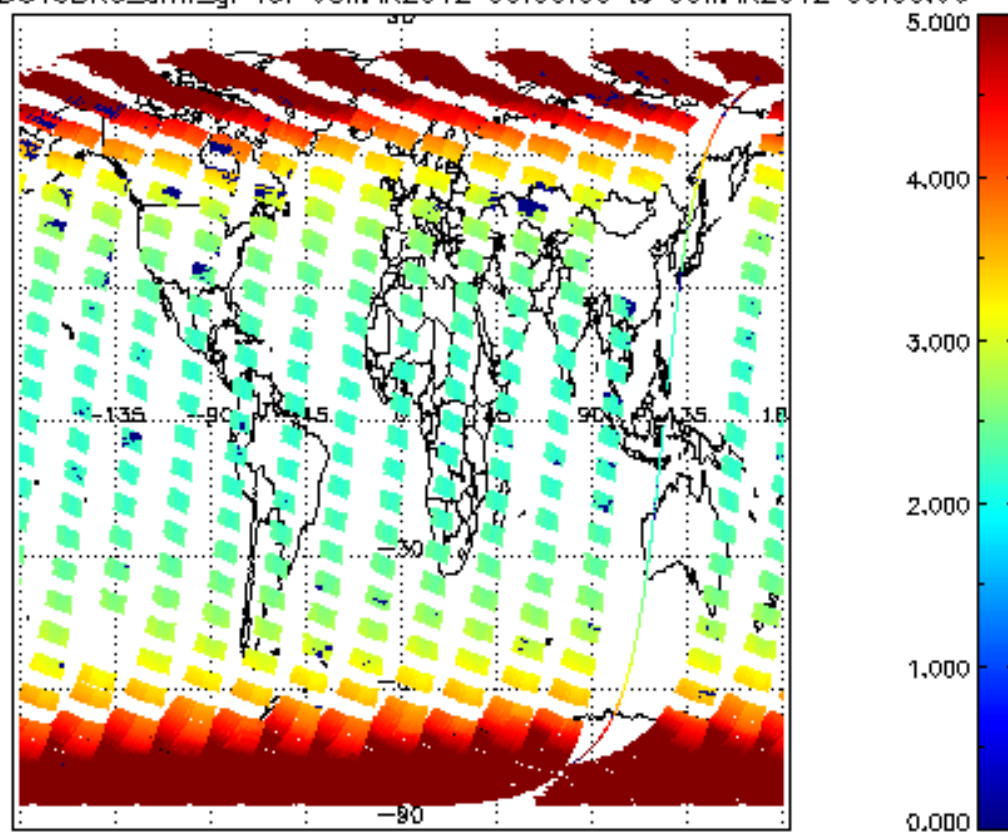
SCIOL2P_NADUV3BRO_amf_gr for 08MAR2012 00:00:00 to 09MAR2012 00:00:00
