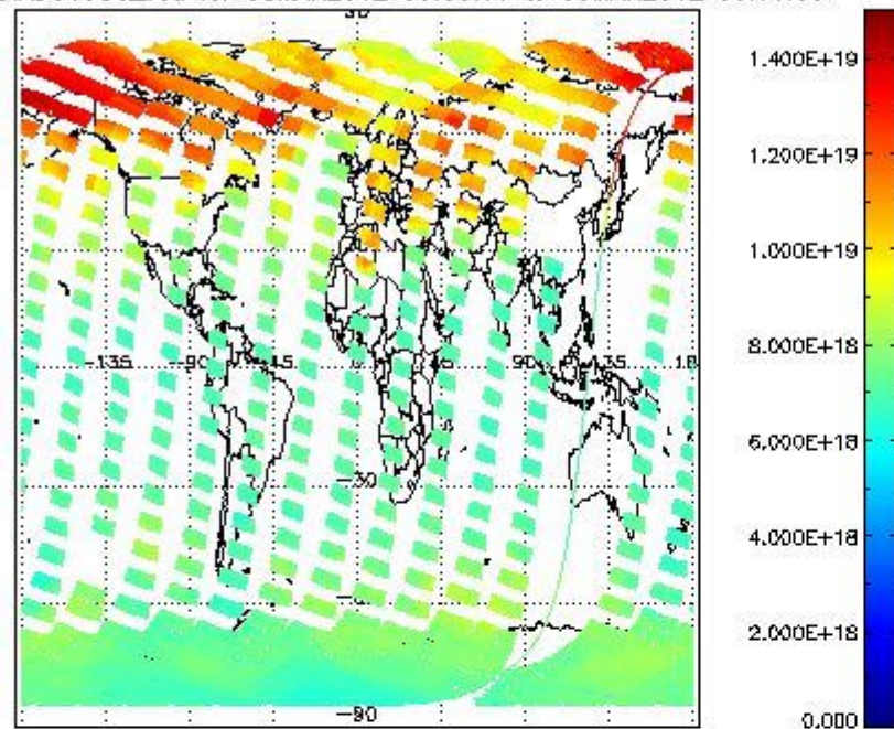
SCIOL2P_NADUV003_vcd for 08MAR2012 00:00:00 to 09MAR2012 00:00:00
