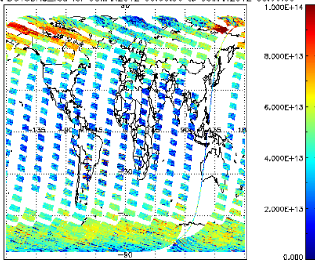
SCIOL2P_NADUV3BRO_vcd for 08MAR2012 00:00:00 to 09MAR2012 00:00:00
