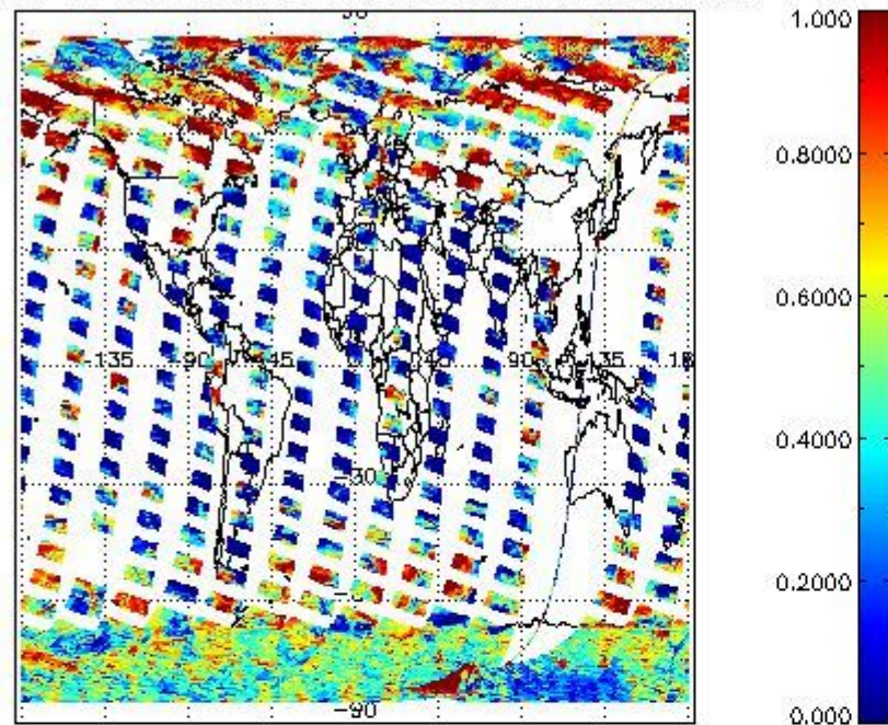
cL_frac for 08MAR2012 00:00:00 to 09MAR2012 00:00:00
