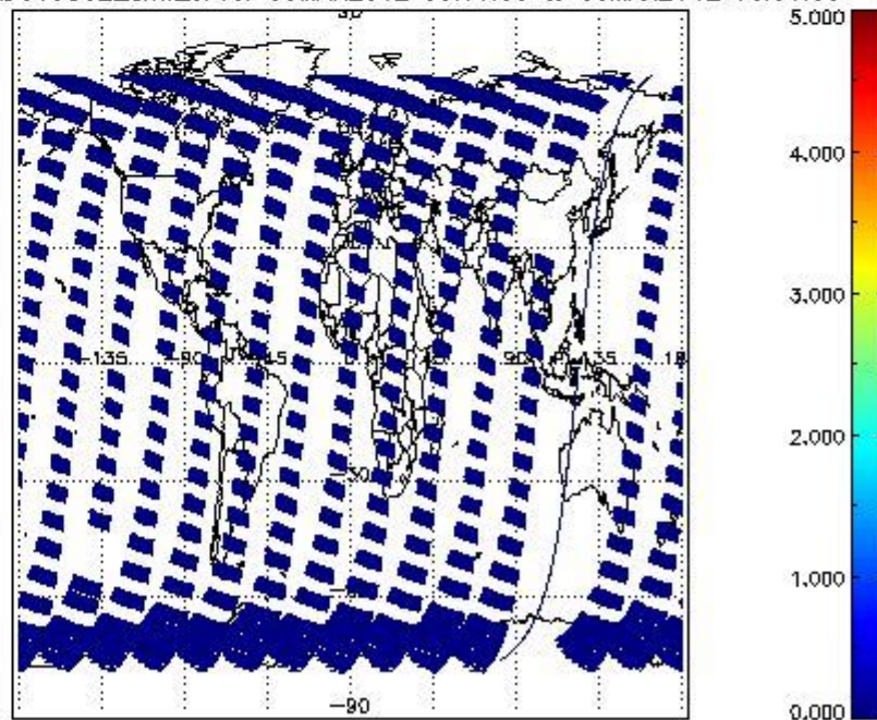
SCIOL2P_NADUV5S02_amf_cl for 08MAR2012 00:00:00 to 09MAR2012 00:00:00
