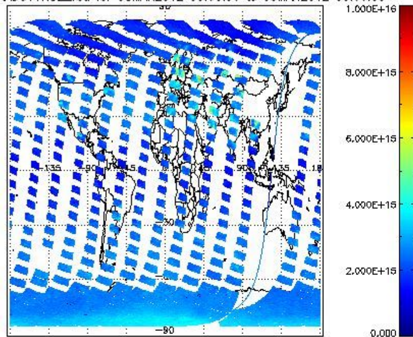
SCIOL2P_NADUV1NO2_vcd for 08MAR2012 00:00:00 to 09MAR2012 00:00:00
