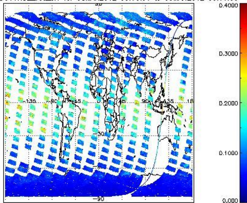
SCIOL2P_NADUV1NO2_vcd_err for 08MAR2012 00:00:00 to 09MAR2012 00:00:00
