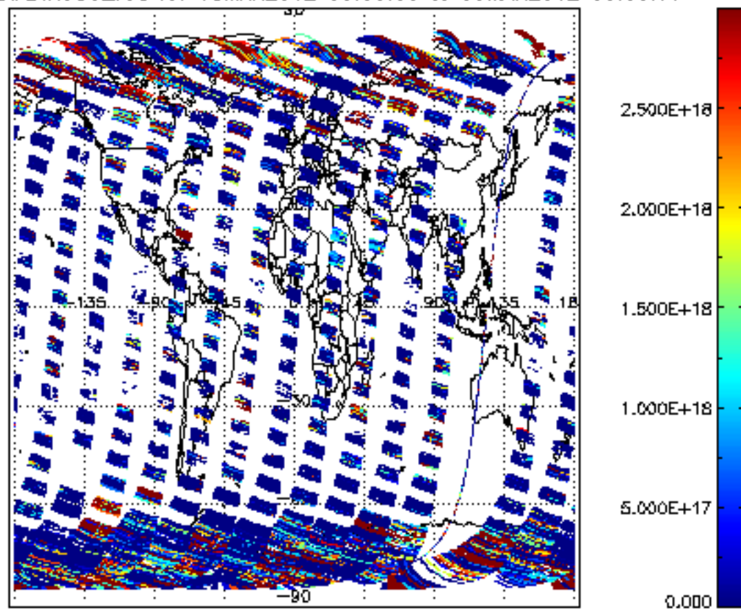
SCIOL2P_NADIR3CO_vcd for 08MAR2012 00:00:00 to 09MAR2012 00:00:00
