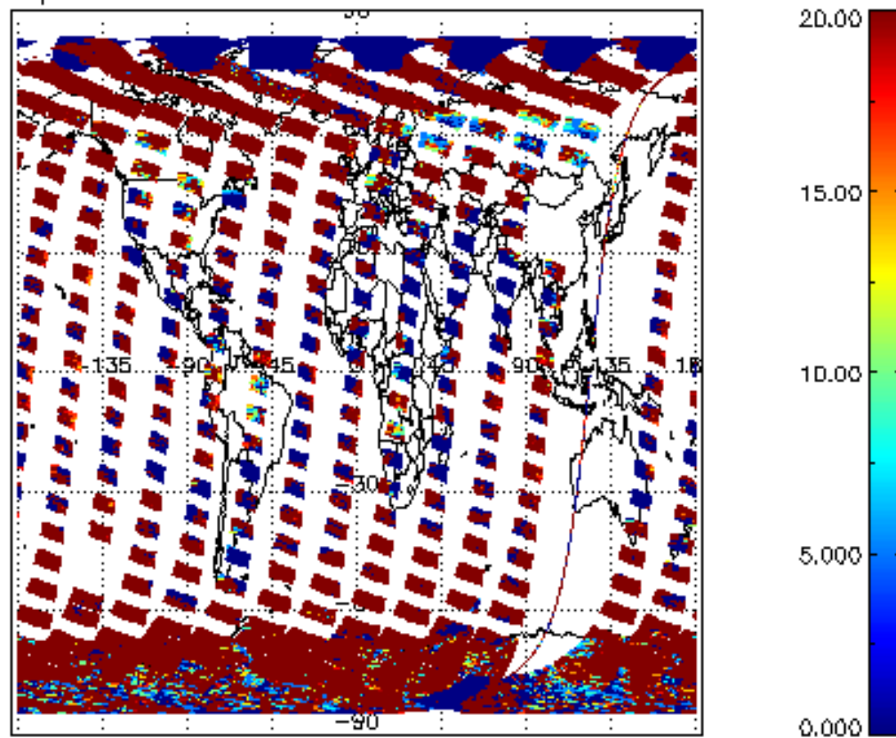
cL_opt_depth for 08MAR2012 00:00:00 to 09MAR2012 00:00:00
