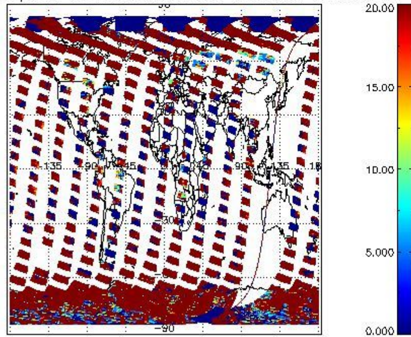
cL_opt_depth for 08MAR2012 00:00:00 to 09MAR2012 00:00:00
