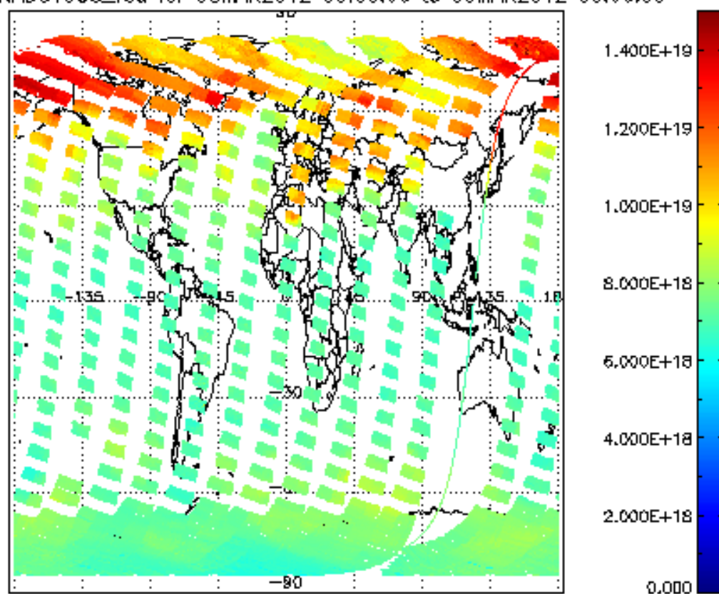
SCIOL2P_NADUV003_vcd for 08MAR2012 00:00:00 to 09MAR2012 00:00:00
