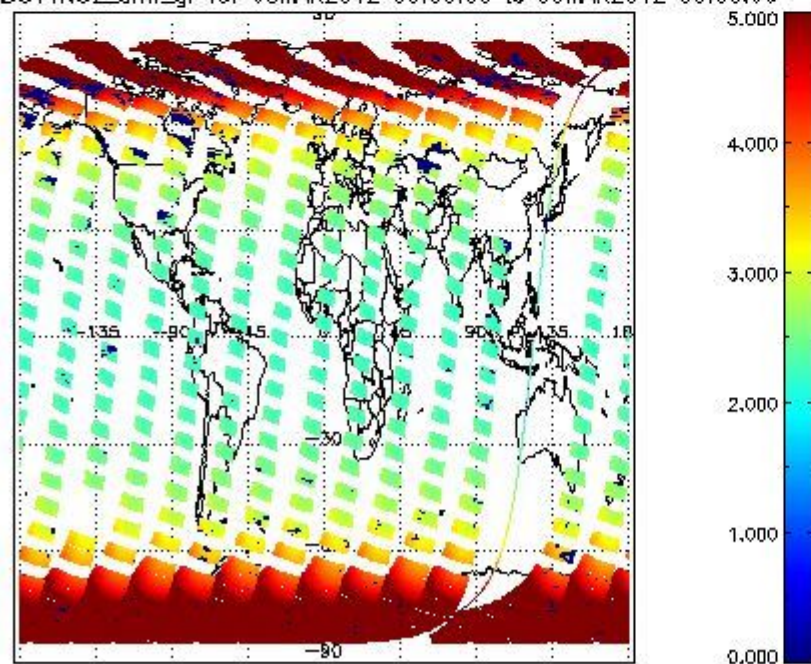
SCIOL2P_NADUV1NO2_amf_gr for 08MAR2012 00:00:00 to 09MAR2012 00:00:00
