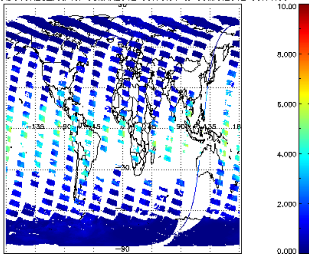
SCIOL2P_NADUV8H20_vcd for 08MAR2012 00:00:00 to 09MAR2012 00:00:00
