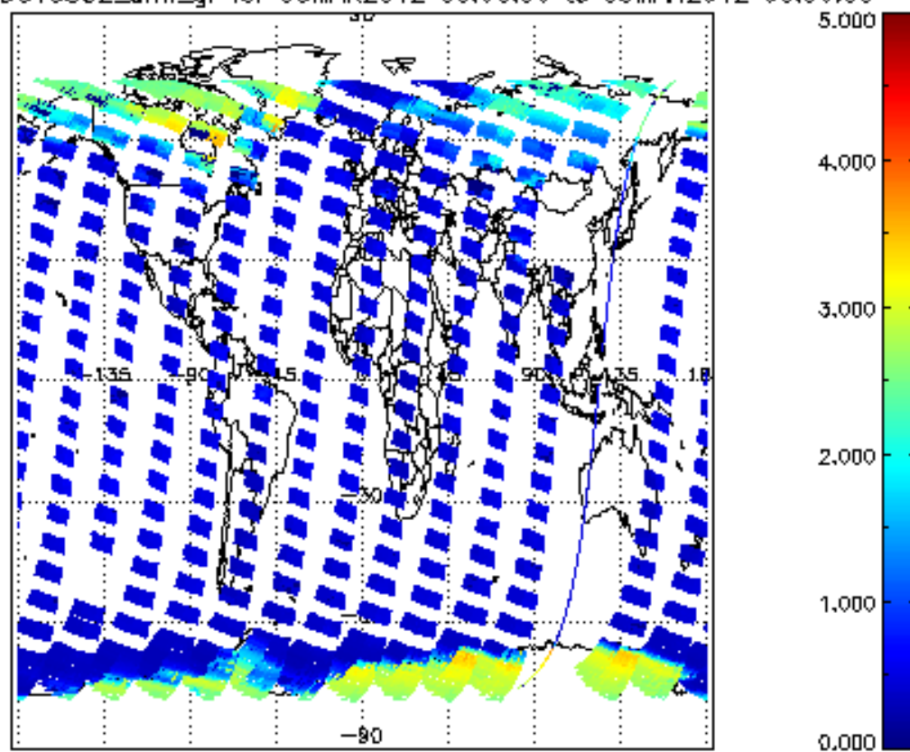
SCIOL2P_NADUV5S02_amf_gr for 08MAR2012 00:00:00 to 09MAR2012 00:00:00
