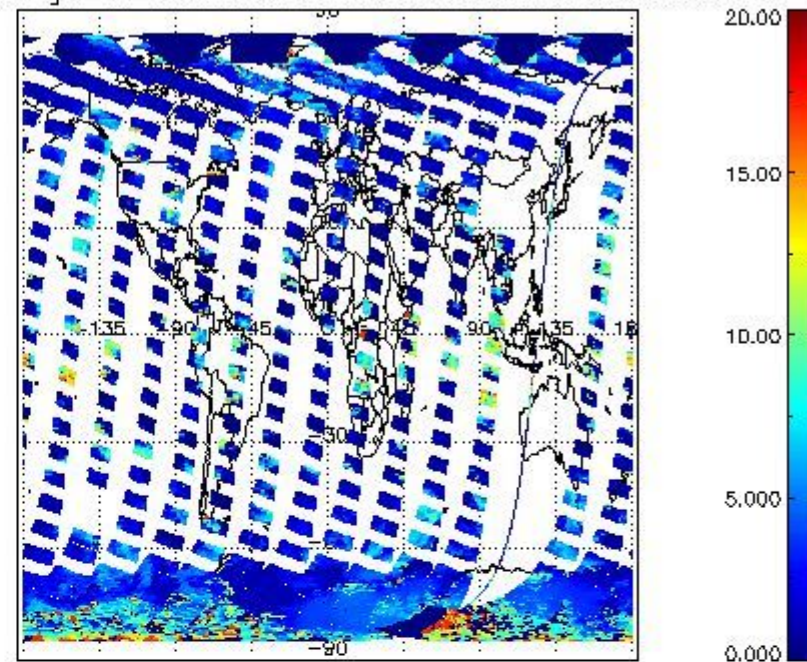
cL_top_height for 08MAR2012 00:00:00 to 09MAR2012 00:00:00
