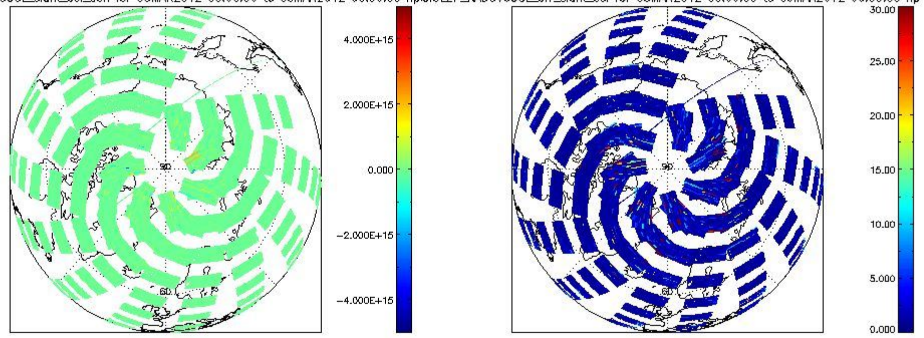
CIOL2P_NADUV6OCL_slant_col_den for 08MAR2012 00:00:00 to 09MAR2012 00:00:00 np CIOL2P_NADUV6OCL_err_slant_col for 08MAR2012 00:00:00 to 09MAR2012 00:00:00 np
