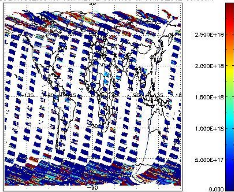
SCIOL2P_NADIR3CO_vcd for 08MAR2012 00:00:00 to 09MAR2012 00:00:00
