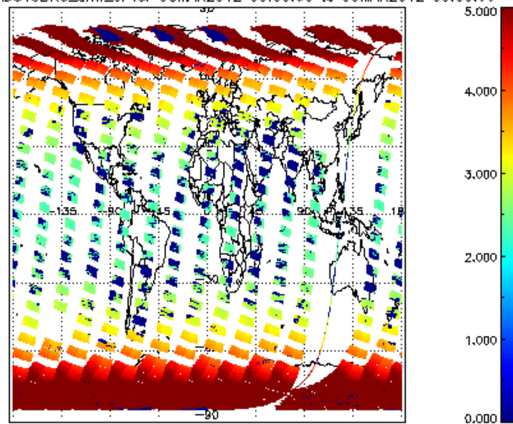
SCIOL2P_NADUV3BRO_amf_cl for 08MAR2012 00:00:00 to 09MAR2012 00:00:00
