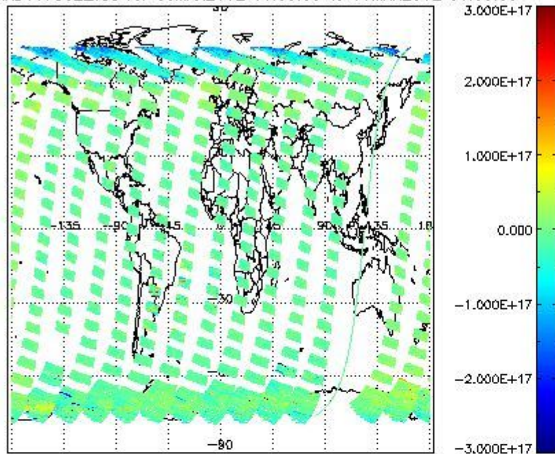
SCIOL2P_NADUV7S02_vcd for 08MAR2012 00:00:00 to 09MAR2012 00:00:00
