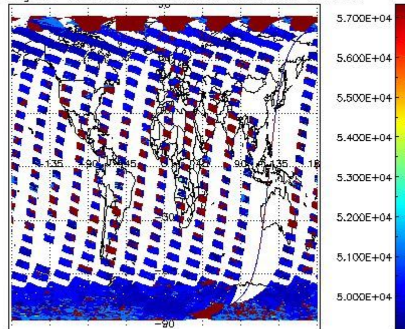
cloud_flags for 08MAR2012 00:00:00 to 09MAR2012 00:00:00
