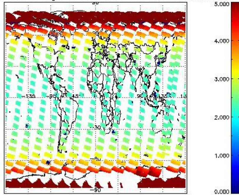
SCIOL2P_NADUV3BRO_amf_gr for 05MAR2012 00:00:00 to 06MAR2012 00:00:00
