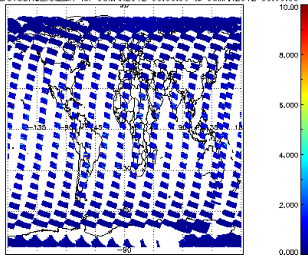
SCIOL2P_NADUV3BRO_vcd_err for 05MAR2012 00:00:00 to 06MAR2012 00:00:00
