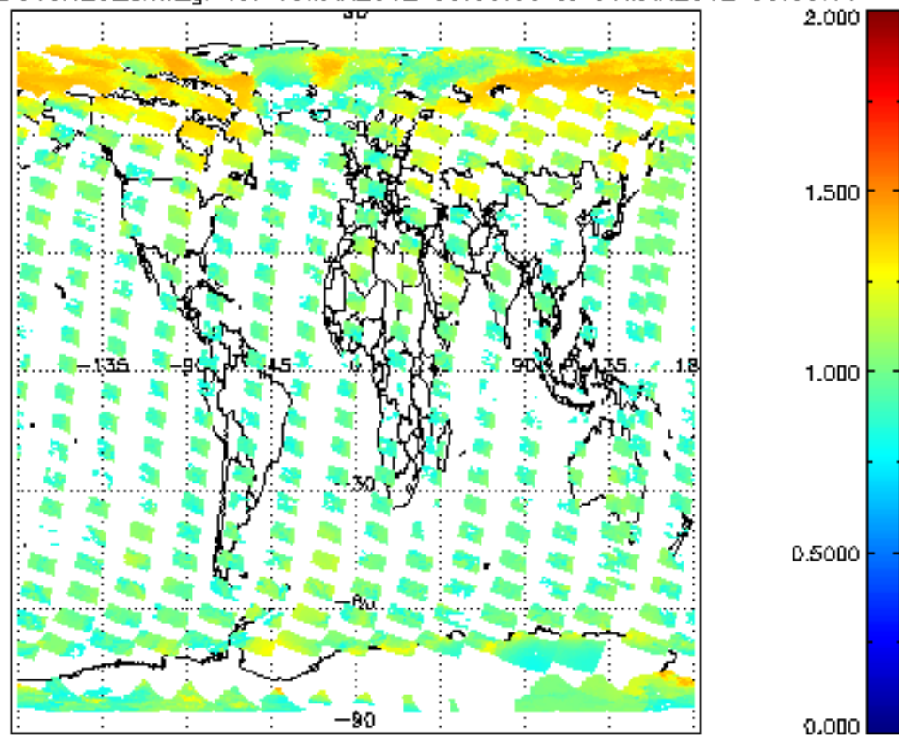
SCIOL2P_NADUV8H20_arnf_gr for 05MAR2012 00:00:00 to 06MAR2012 00:00:00
