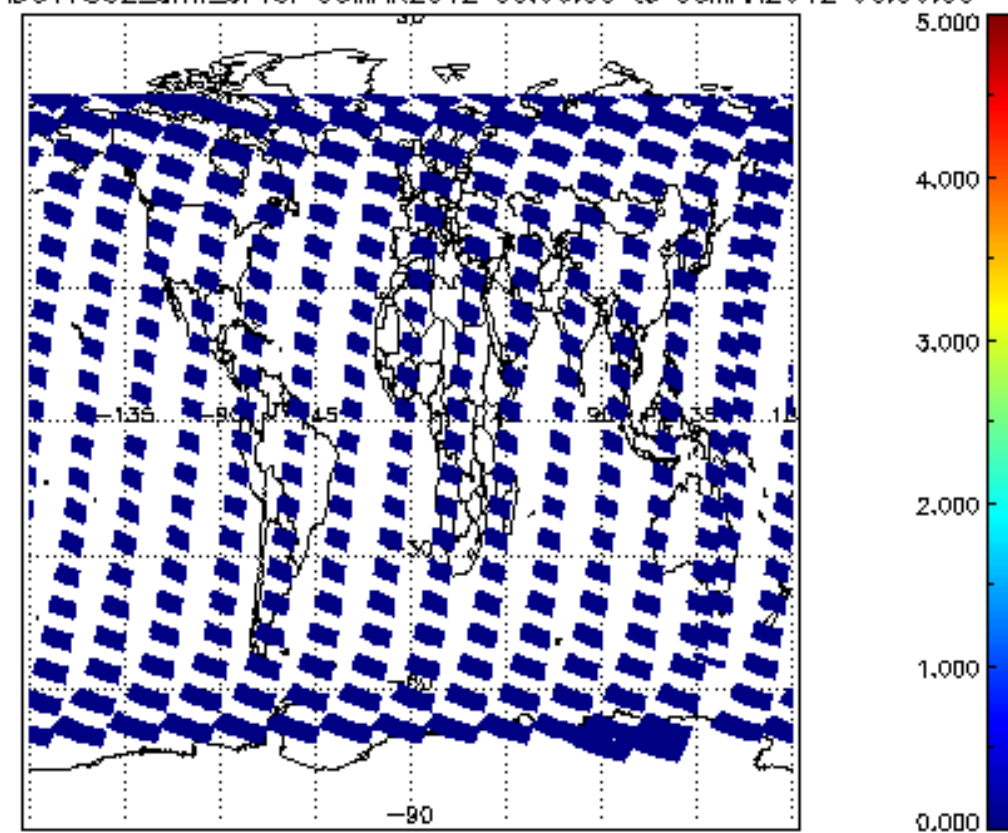
SCIOL2P_NADUV7S02_amf_cl for 05MAR2012 00:00:00 to 06MAR2012 00:00:00
