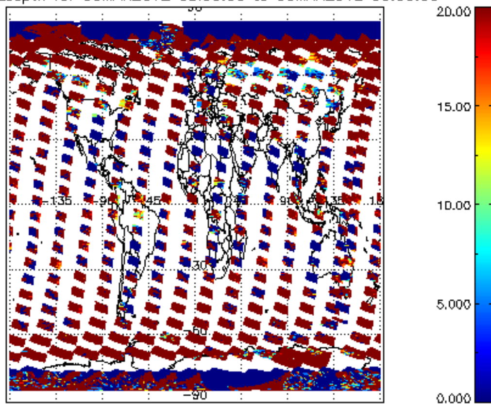
cL_opt_depth for 05MAR2012 00:00:00 to 06MAR2012 00:00:00
