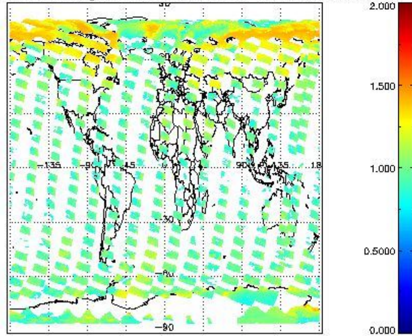
SCIOL2P_NADUV8H2O_arnf_gr for 05MAR2012 00:00:00 to 06MAR2012 00:00:00
