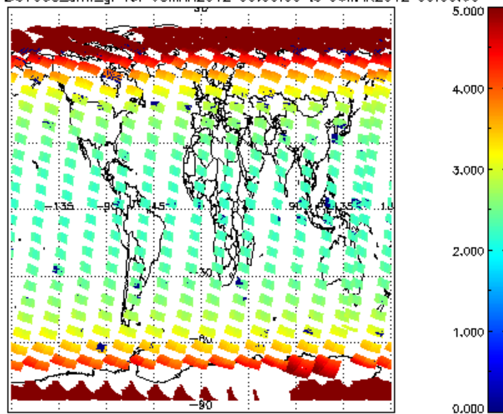
SCIOL2P_NADUV003_arnf_gr for 05MAR2012 00:00:00 to 06MAR2012 00:00:00
