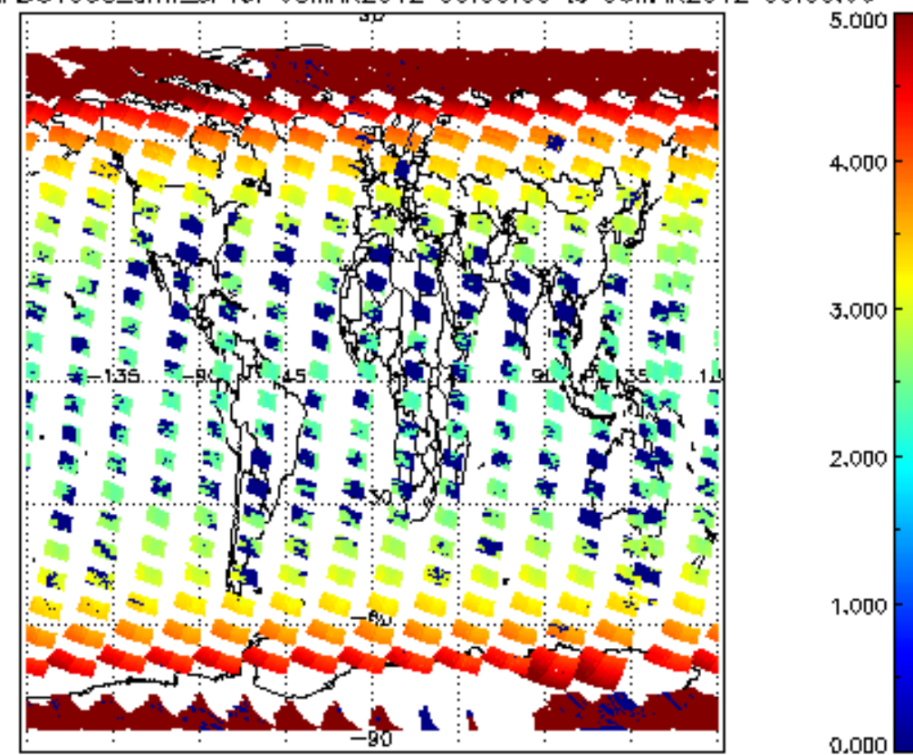
SCIOL2P_NADUV003_arnf_cl for 05MAR2012 00:00:00 to 06MAR2012 00:00:00
