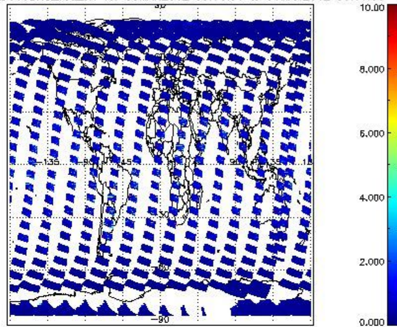
SCIOL2P_NADUV3BRO_vcd_err for 05MAR2012 00:00:00 to 06MAR2012 00:00:00
