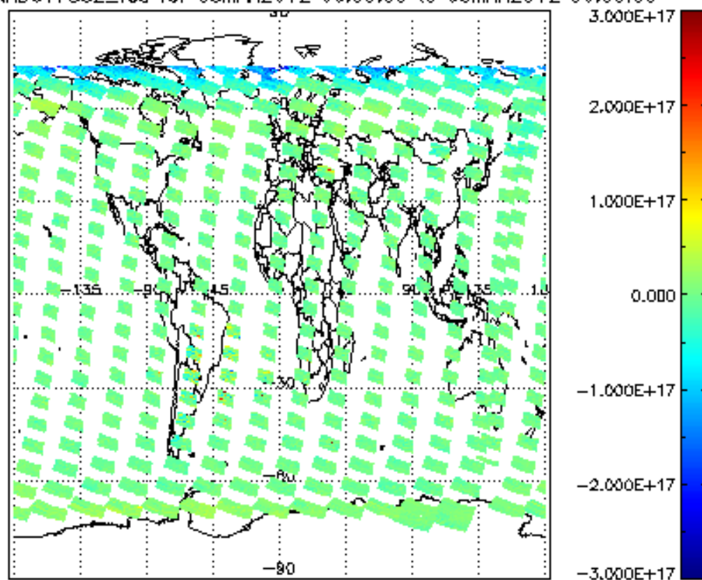
SCIOL2P_NADUV7S02_vcd for 05MAR2012 00:00:00 to 06MAR2012 00:00:00
