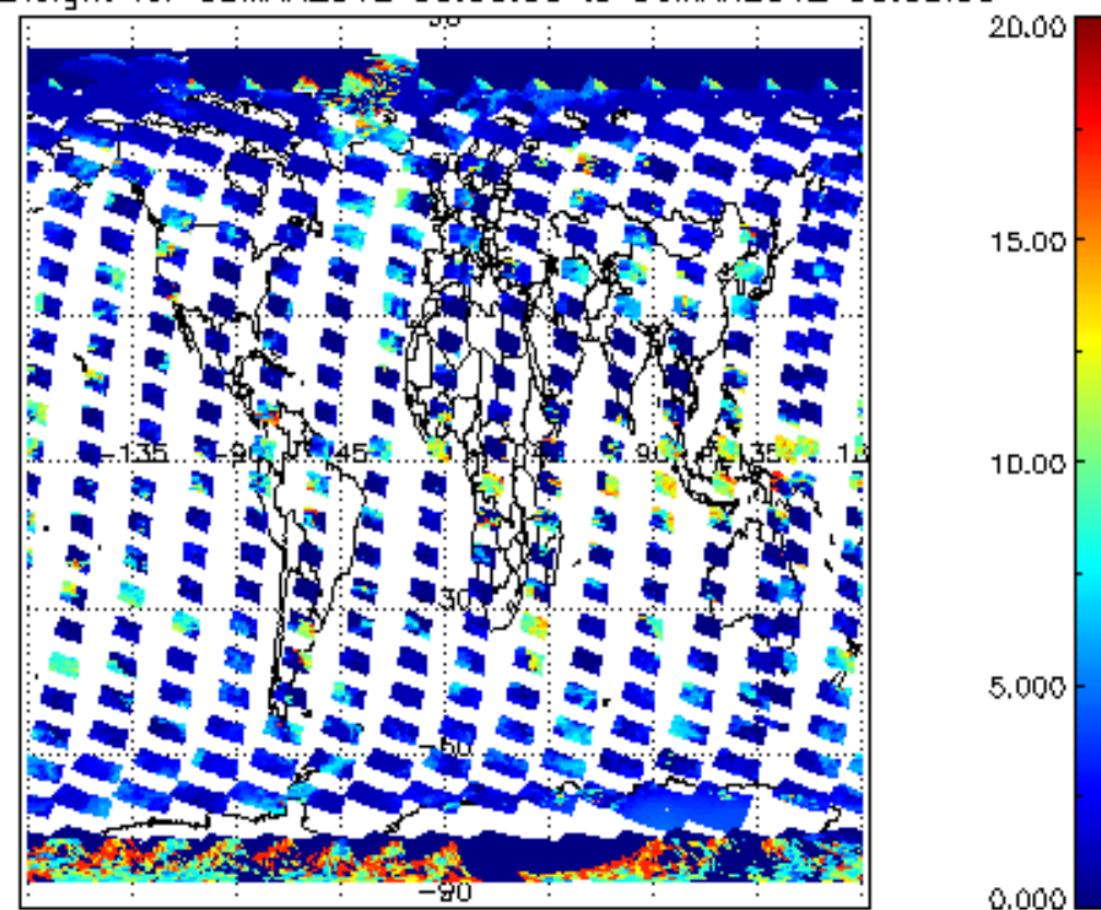
cL_top_height for 05MAR2012 00:00:00 to 06MAR2012 00:00:00
