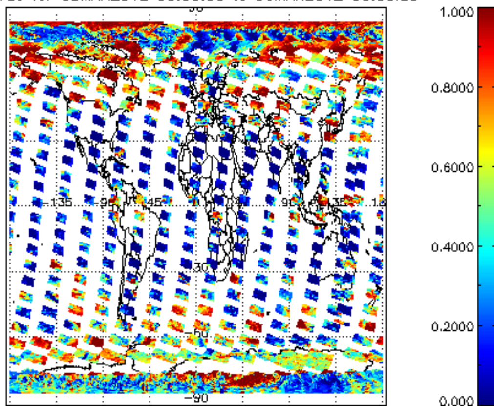
cL_frac for 05MAR2012 00:00:00 to 06MAR2012 00:00:00
