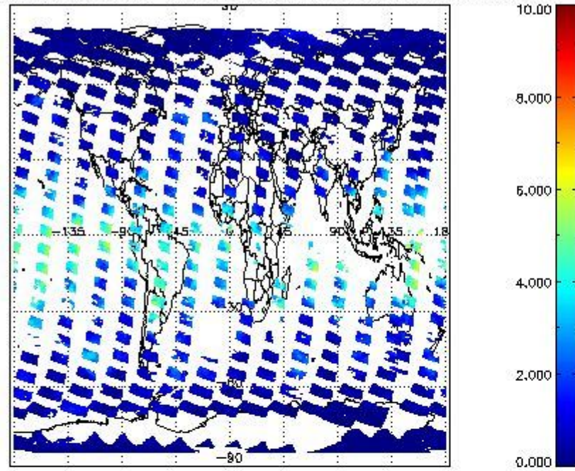
SCIOL2P_NADUV8H2O_vcd for 05MAR2012 00:00:00 to 06MAR2012 00:00:00
