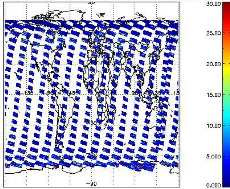
SCIOL2P_NADUV5SO2_vcd_err for 05MAR2012 00:00:00 to 06MAR2012 00:00:00
