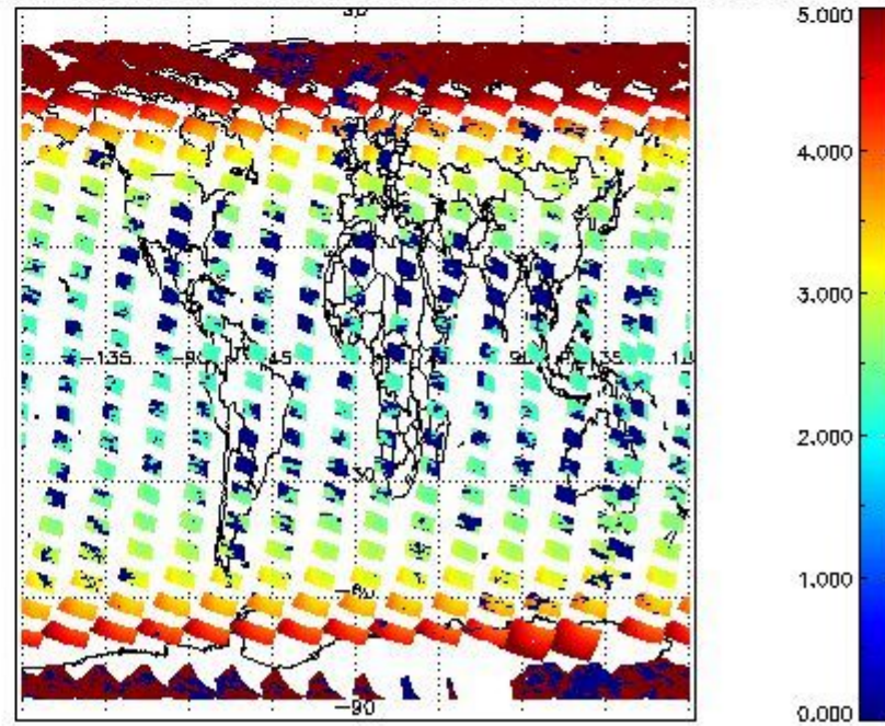
SCIOL2P_NADUV1NO2_amf_cl for 05MAR2012 00:00:00 to 06MAR2012 00:00:00
