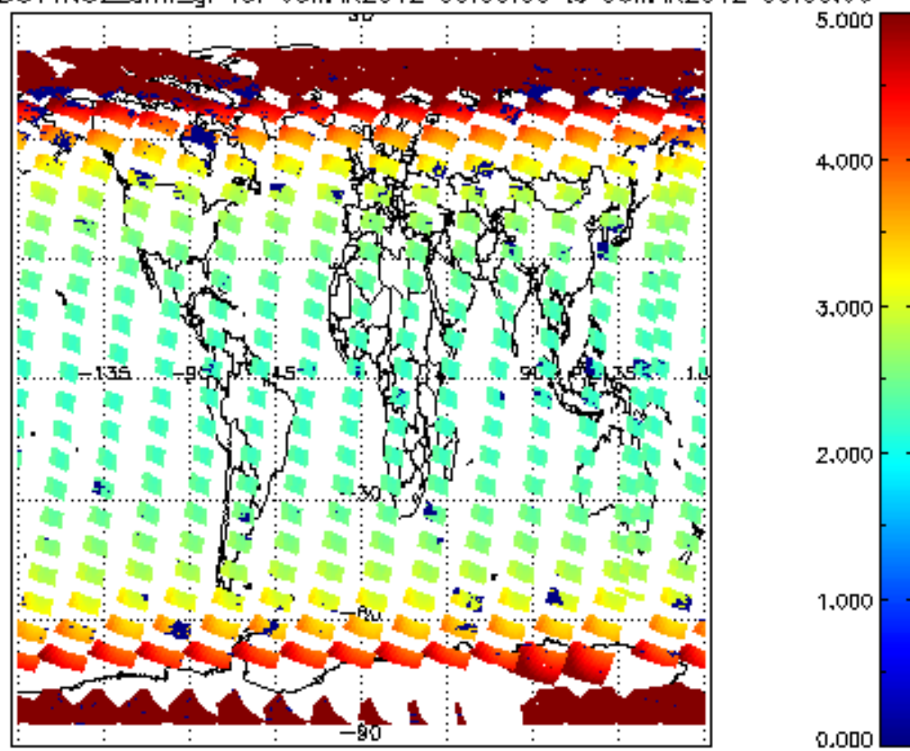
SCIOL2P_NADUV1NO2_amf_gr for 05MAR2012 00:00:00 to 06MAR2012 00:00:00
