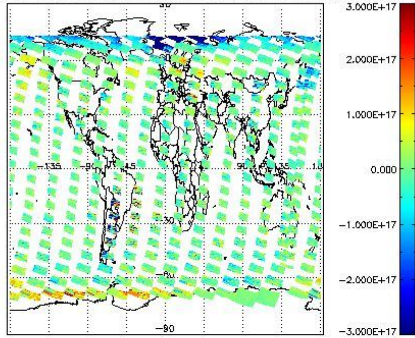
SCIOL2P_NADUV5SO2_vcd for 05MAR2012 00:00:00 to 06MAR2012 00:00:00
