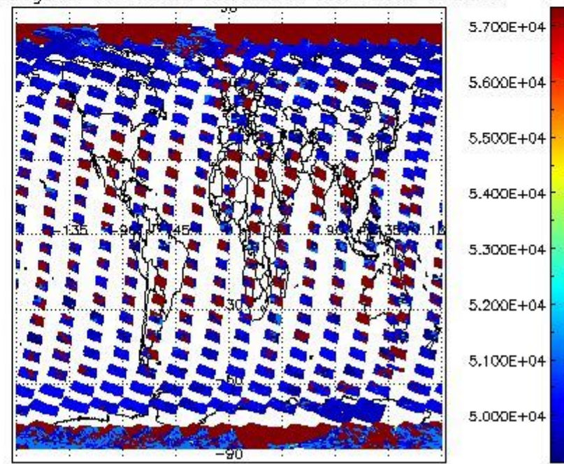
cloud_flags for 05MAR2012 00:00:00 to 06MAR2012 00:00:00
