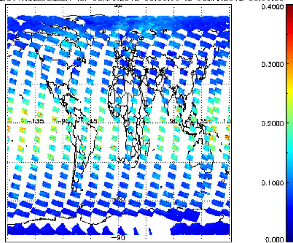
SCIOL2P_NADUV1NO2_vcd_err for 05MAR2012 00:00:00 to 06MAR2012 00:00:00
