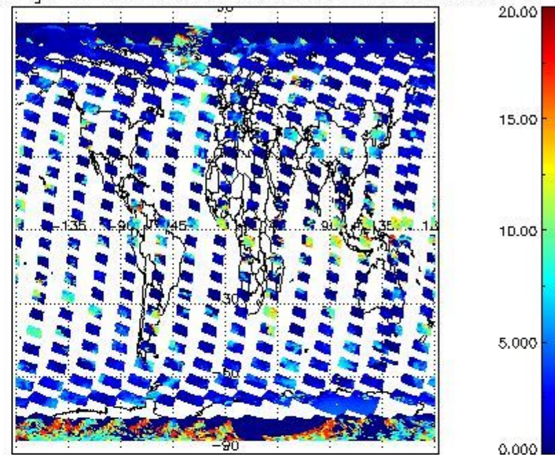
cL_top_height for 05MAR2012 00:00:00 to 06MAR2012 00:00:00
