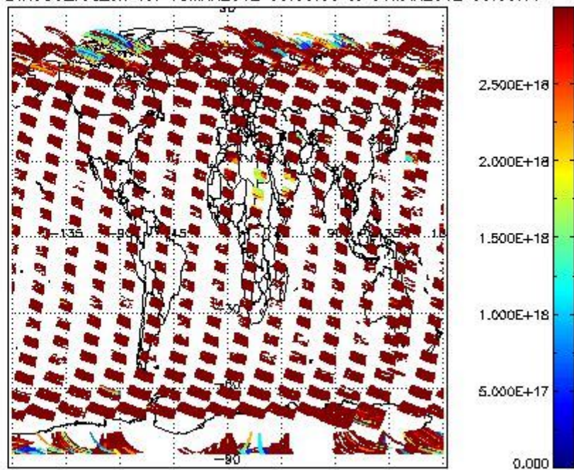
SCIDL2P_NADIR3CO_vcd_err for 05MAR2012 00:00:00 to 06MAR2012 00:00:00
