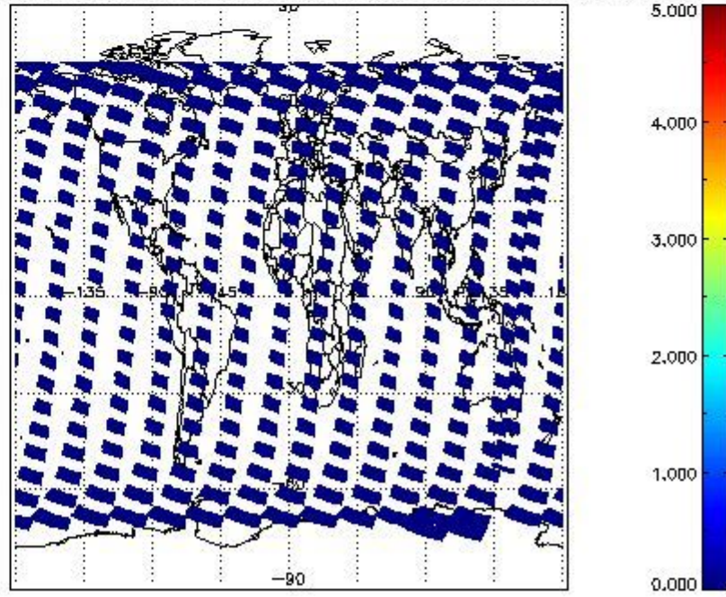
SCIOL2P_NADUV5SO2_amf_cl for 05MAR2012 00:00:00 to 06MAR2012 00:00:00
