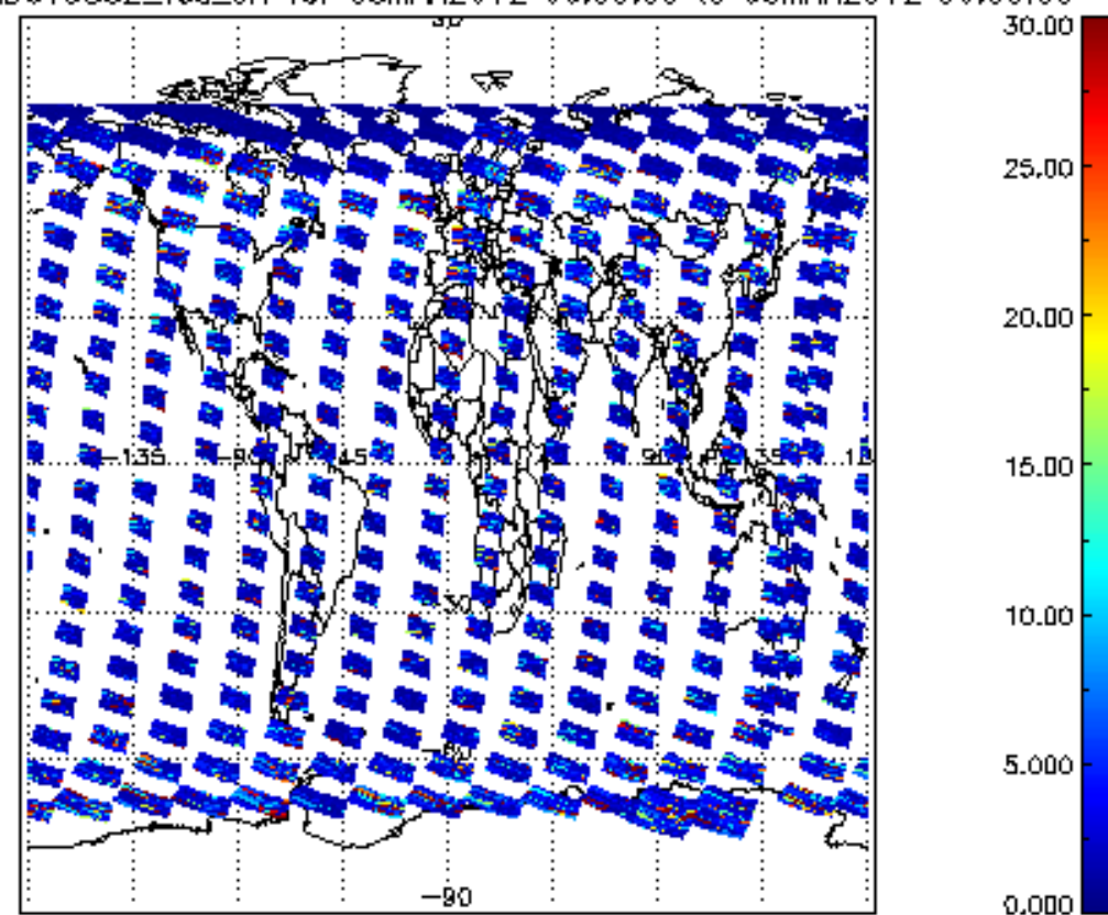
SCIOL2P_NADUV5S02_vcd_err for 05MAR2012 00:00:00 to 06MAR2012 00:00:00
