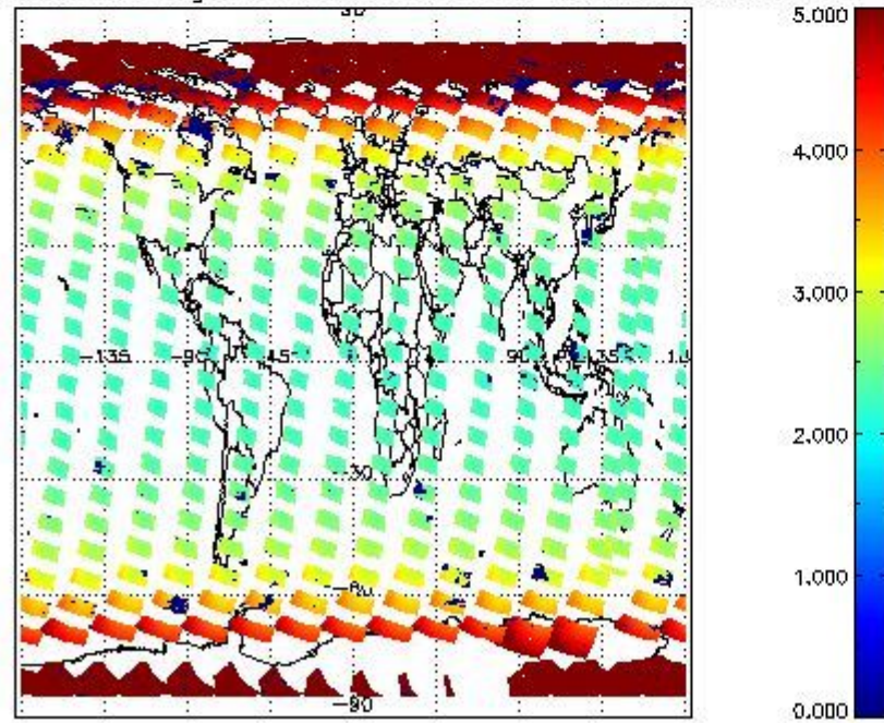
SCIOL2P_NADUV1NO2_amf_gr for 05MAR2012 00:00:00 to 06MAR2012 00:00:00
