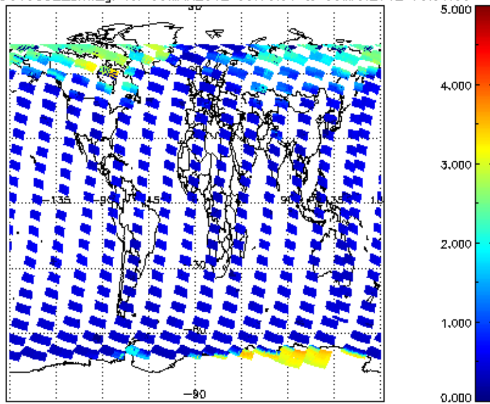
SCIOL2P_NADUV5S02_amf_gr for 05MAR2012 00:00:00 to 06MAR2012 00:00:00
