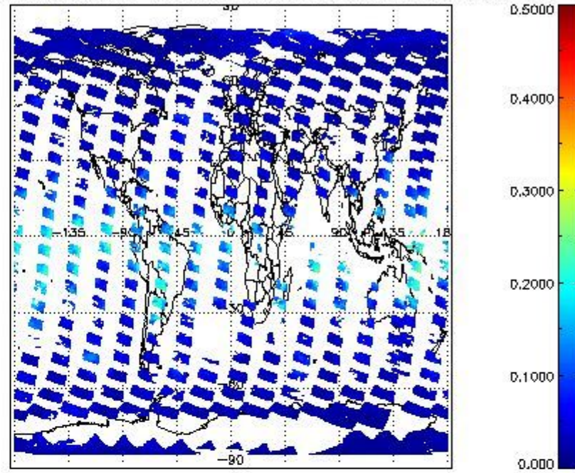
SCIOL2P_NADUV8H2O_vcd_err for 05MAR2012 00:00:00 to 06MAR2012 00:00:00
