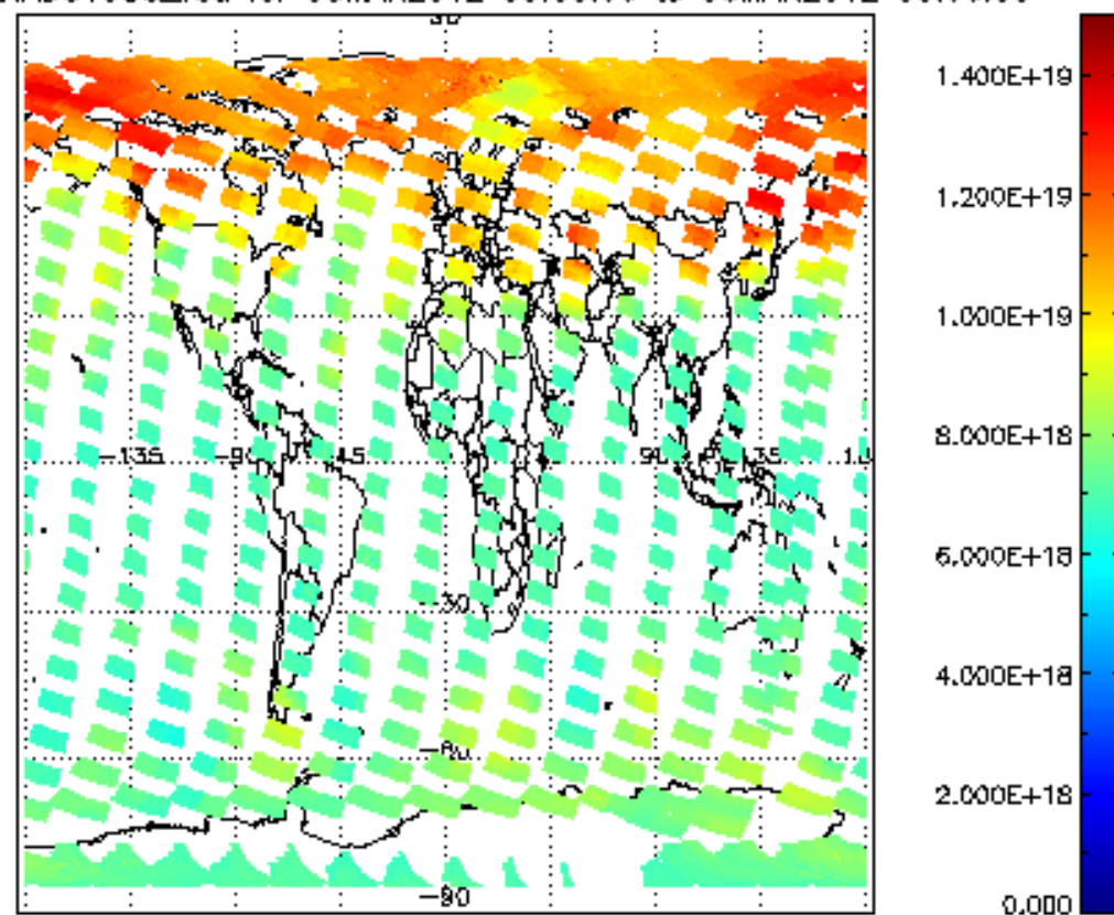
SCIOL2P_NADUV003_vcd for 05MAR2012 00:00:00 to 06MAR2012 00:00:00
