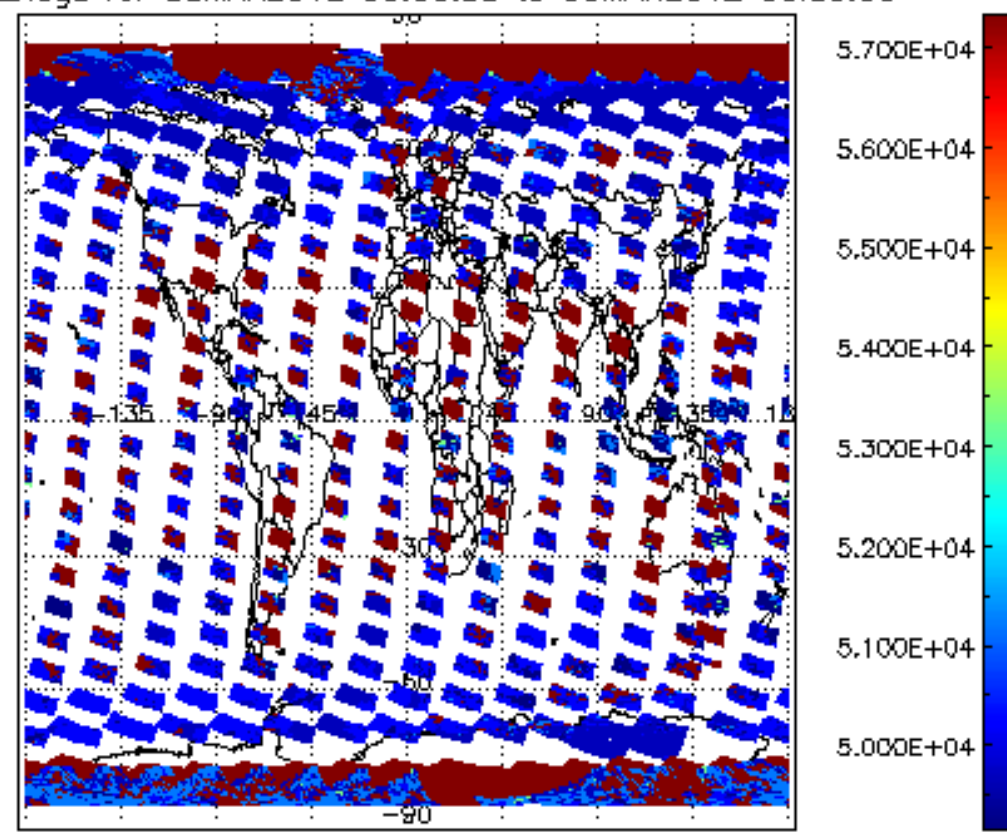
cloud_flags for 05MAR2012 00:00:00 to 06MAR2012 00:00:00
