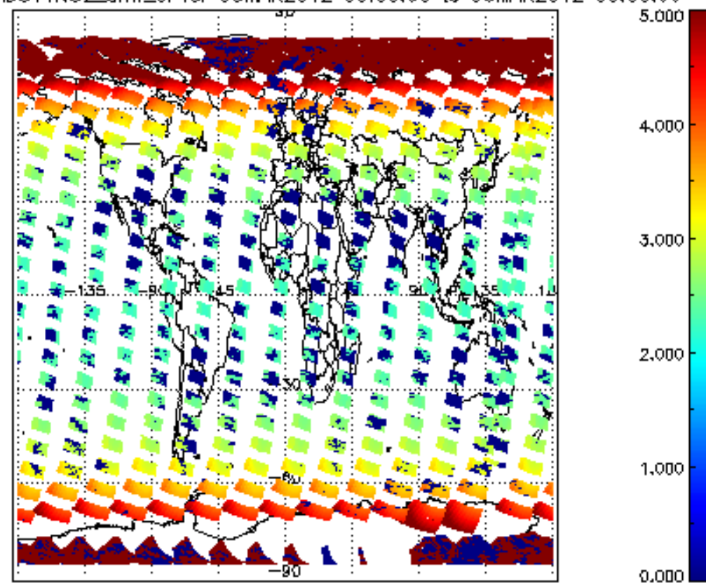
SCIOL2P_NADUV1NO2_amf_cl for 05MAR2012 00:00:00 to 06MAR2012 00:00:00
