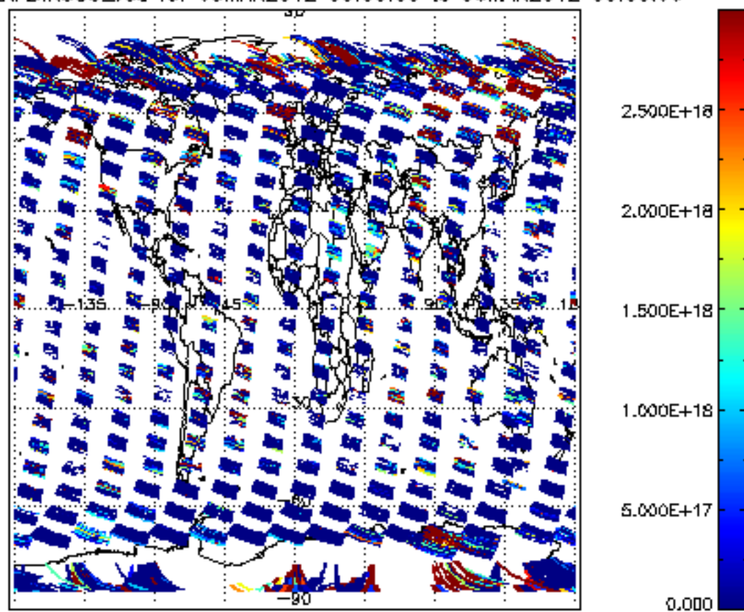
SCIOL2P_NADIR3CO_vcd for 05MAR2012 00:00:00 to 06MAR2012 00:00:00
