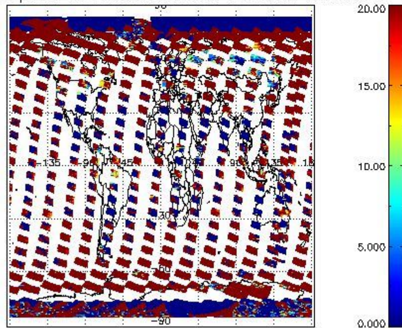
cL_opt_depth for 05MAR2012 00:00:00 to 06MAR2012 00:00:00
