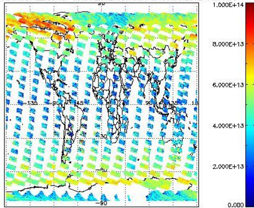
SCIOL2P_NADUV3BRO_vcd for 05MAR2012 00:00:00 to 06MAR2012 00:00:00
