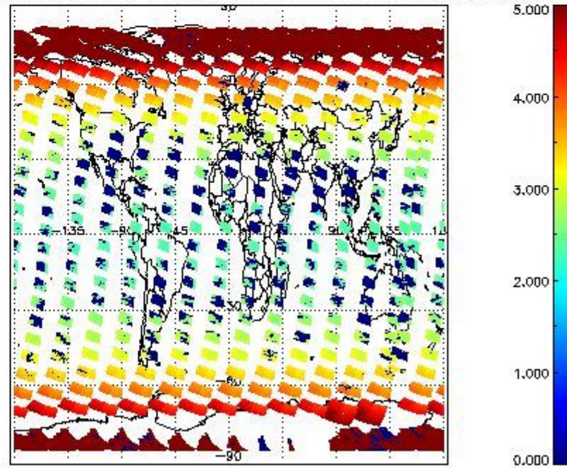
SCIOL2P_NADUV3BRO_amf_cl for 05MAR2012 00:00:00 to 06MAR2012 00:00:00
