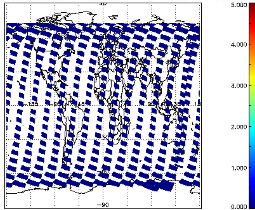
SCIOL2P_NADUV5S02_amf_cl for 05MAR2012 00:00:00 to 06MAR2012 00:00:00
