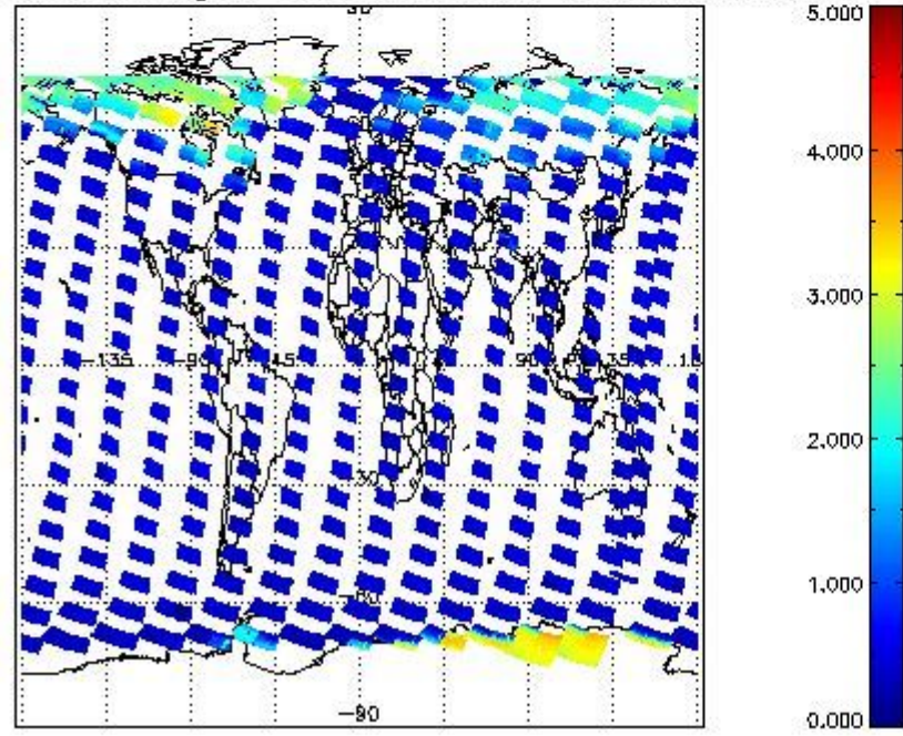
SCIOL2P_NADUV5SO2_amf_gr for 05MAR2012 00:00:00 to 06MAR2012 00:00:00
