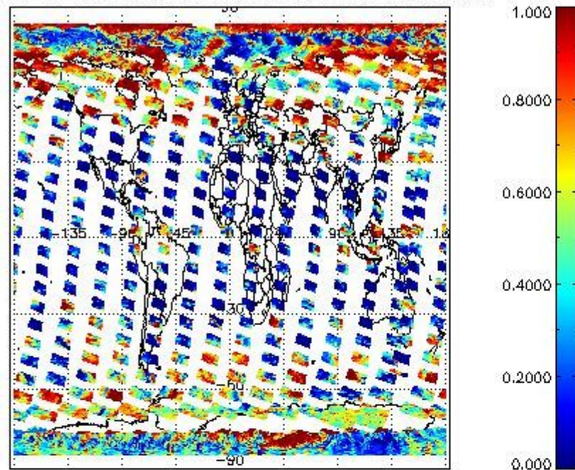
cL_frac for 05MAR2012 00:00:00 to 06MAR2012 00:00:00
