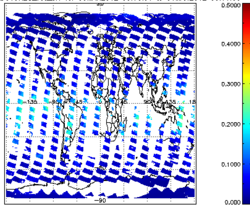
SCIOL2P_NADUV8H20_vcd_err for 05MAR2012 00:00:00 to 06MAR2012 00:00:00
