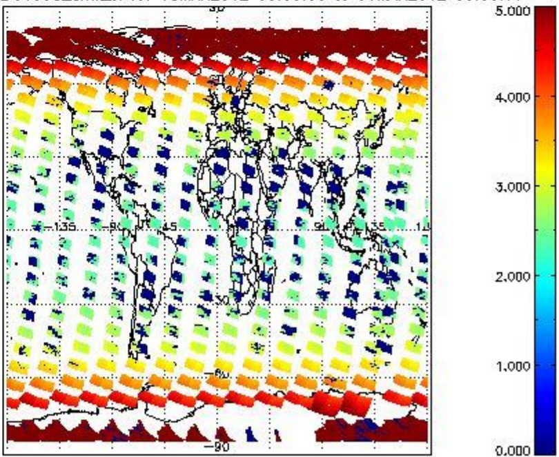
SCIOL2P_NADUV003_amf_cl for 05MAR2012 00:00:00 to 06MAR2012 00:00:00
