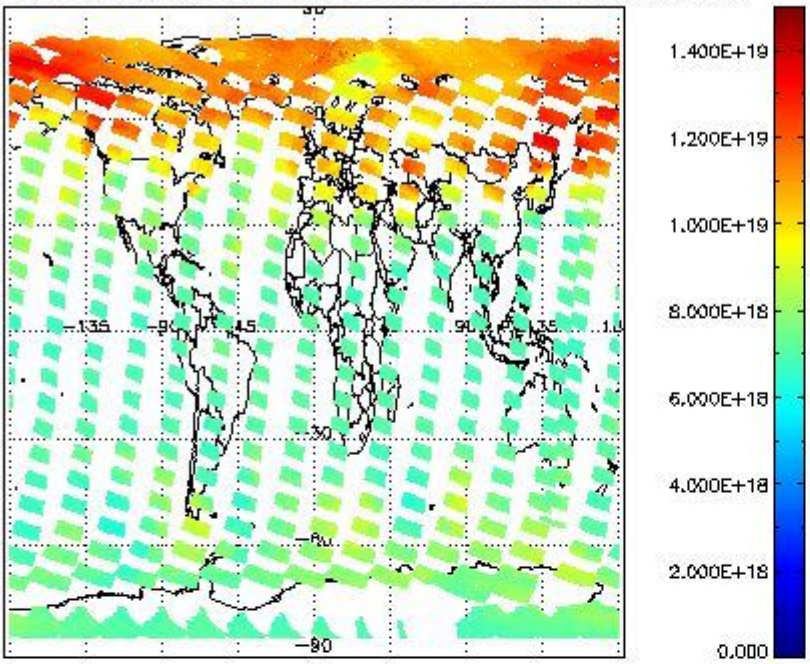
SCIOL2P_NADUV003_vcd for 05MAR2012 00:00:00 to 06MAR2012 00:00:00
