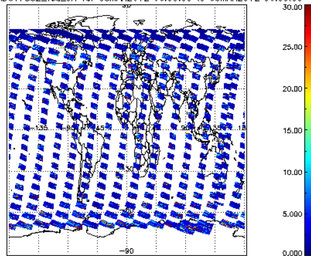
SCIOL2P_NADUV7S02_vcd_err for 05MAR2012 00:00:00 to 06MAR2012 00:00:00
