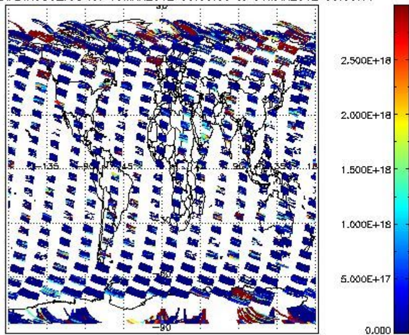
SCIDL2P_NADIR3CO_vcd for 05MAR2012 00:00:00 to 06MAR2012 00:00:00
