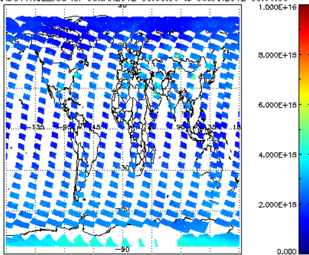
SCIOL2P_NADUV1NO2_vcd for 05MAR2012 00:00:00 to 06MAR2012 00:00:00
