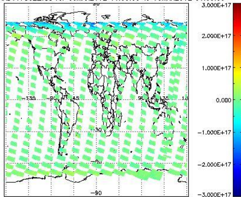
SCIOL2P_NADUV7S02_vcd for 05MAR2012 00:00:00 to 06MAR2012 00:00:00
