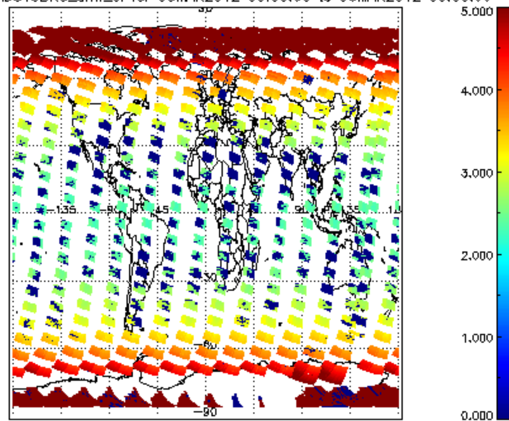
SCIOL2P_NADUV3BRO_amf_cl for 05MAR2012 00:00:00 to 06MAR2012 00:00:00
