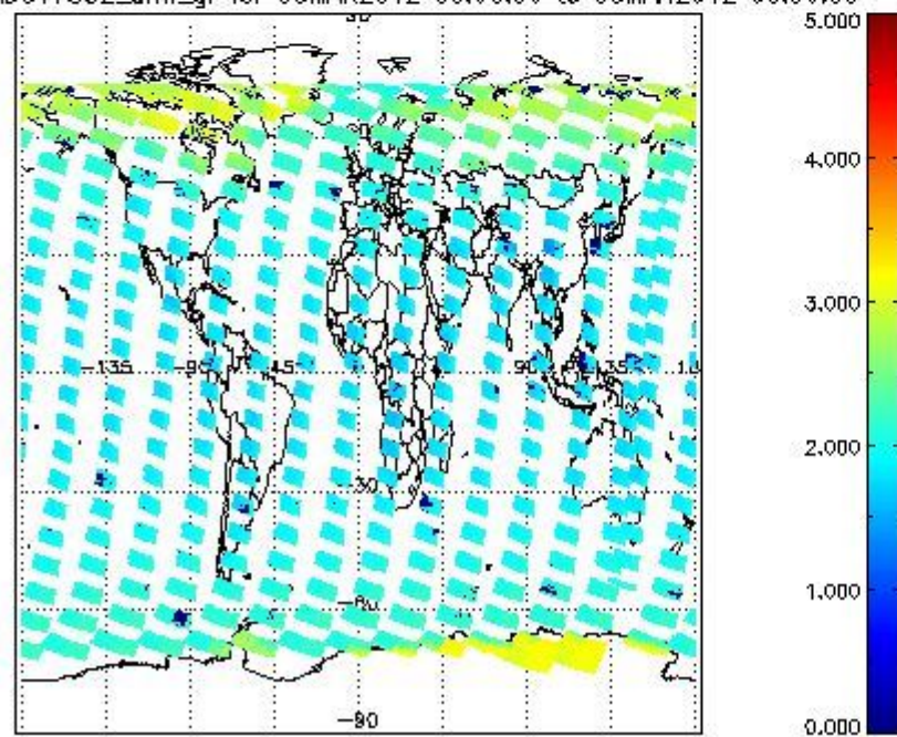
SCIOL2P_NADUV7S02_amf_gr for 05MAR2012 00:00:00 to 06MAR2012 00:00:00
