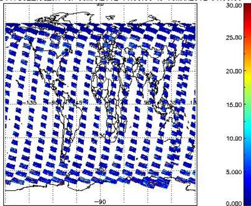
SCIOL2P_NADUV7S02_vcd_err for 05MAR2012 00:00:00 to 06MAR2012 00:00:00
