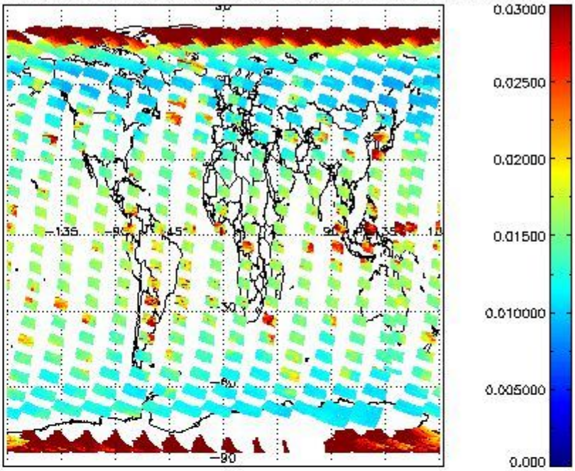
SCIOL2P_NADUV003_vcd_err for 05MAR2012 00:00:00 to 06MAR2012 00:00:00
