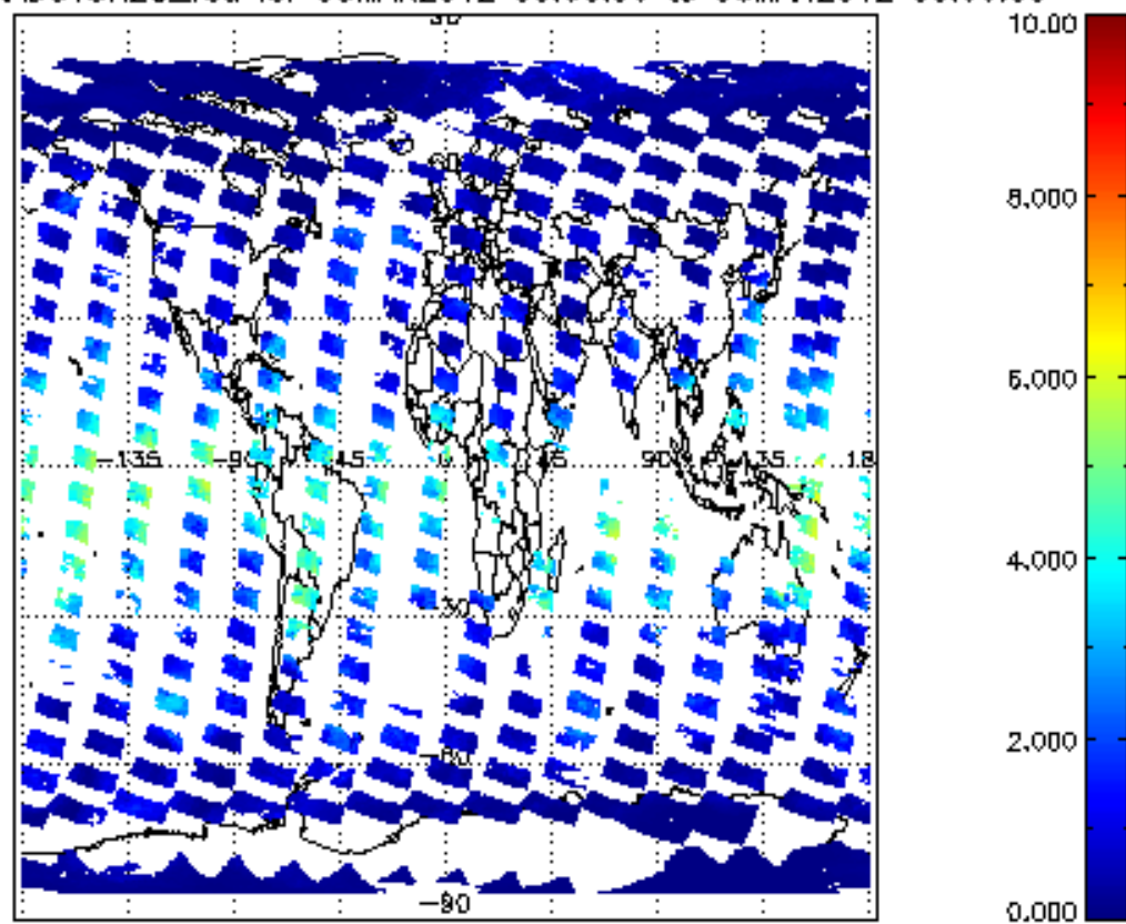
SCIOL2P_NADUV8H20_vcd for 05MAR2012 00:00:00 to 06MAR2012 00:00:00
