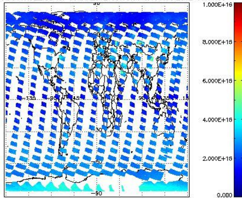
SCIOL2P_NADUV1NO2_vcd for 05MAR2012 00:00:00 to 06MAR2012 00:00:00
