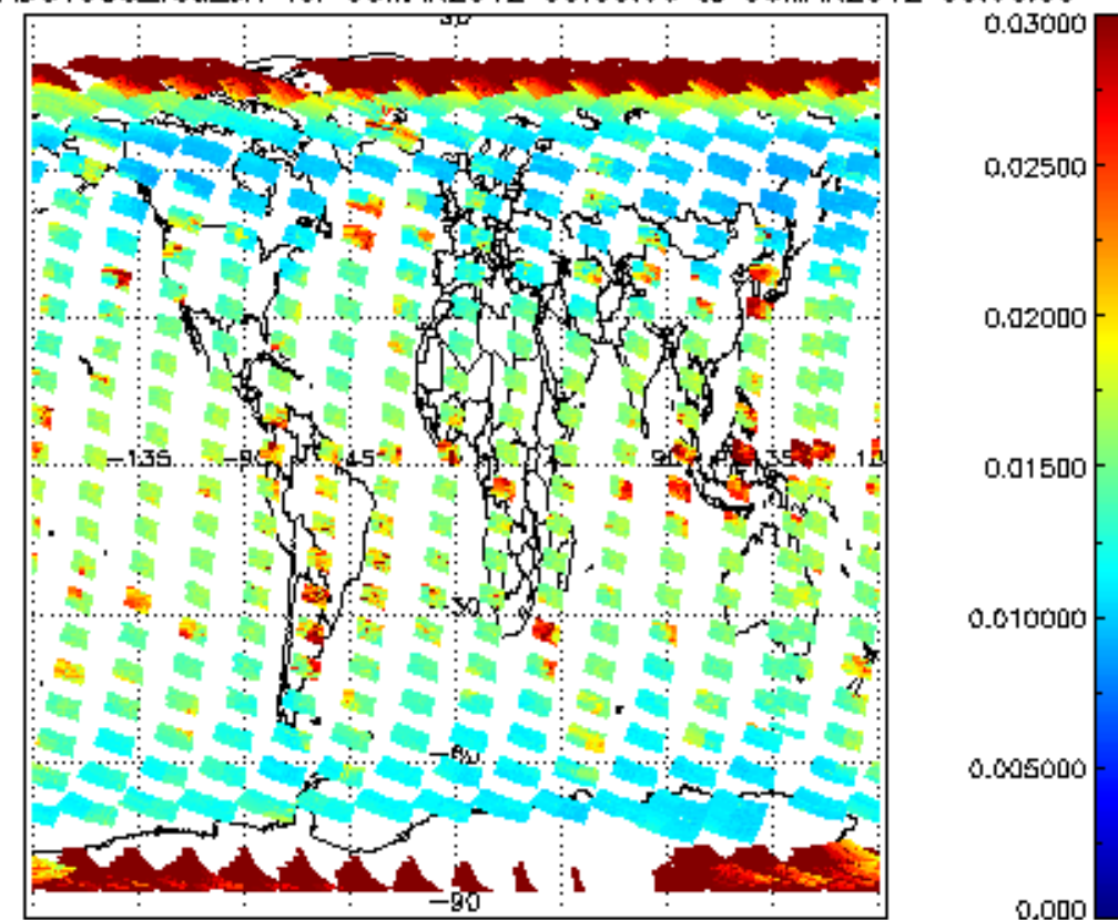
SCIOL2P_NADUV003_vcd_err for 05MAR2012 00:00:00 to 06MAR2012 00:00:00
