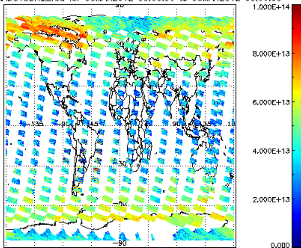
SCIOL2P_NADUV3BRO_vcd for 05MAR2012 00:00:00 to 06MAR2012 00:00:00
