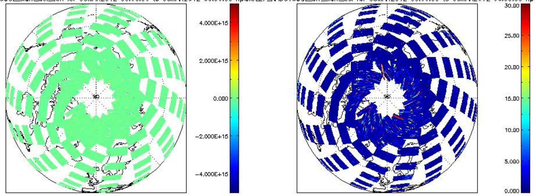
CIOL2P_NADUV6OCL_slant_col_den for 05MAR2012 00:00:00 to 06MAR2012 00:00:00 np CIOL2P_NADUV6OCL_err_slant_col for 05MAR2012 00:00:00 to 06MAR2012 00:00:00 np
