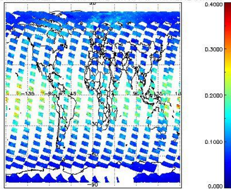
SCIOL2P_NADUV1NO2_vcd_err for 05MAR2012 00:00:00 to 06MAR2012 00:00:00
