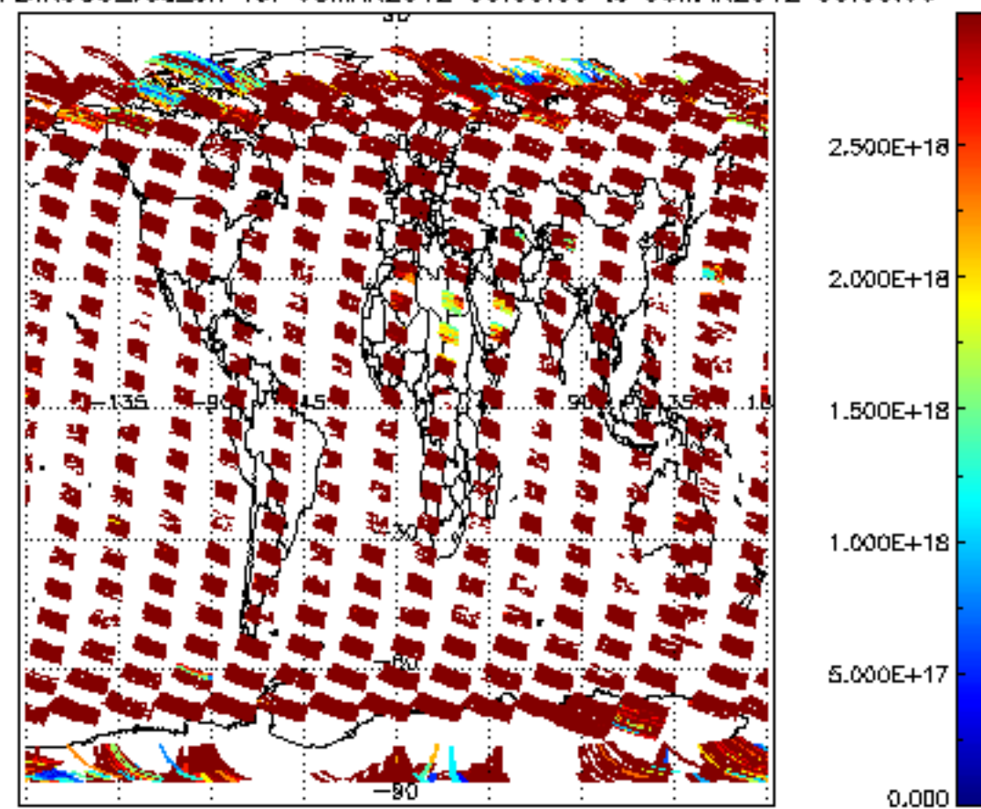
SCIOL2P_NADIR3CO_vcd_err for 05MAR2012 00:00:00 to 06MAR2012 00:00:00
