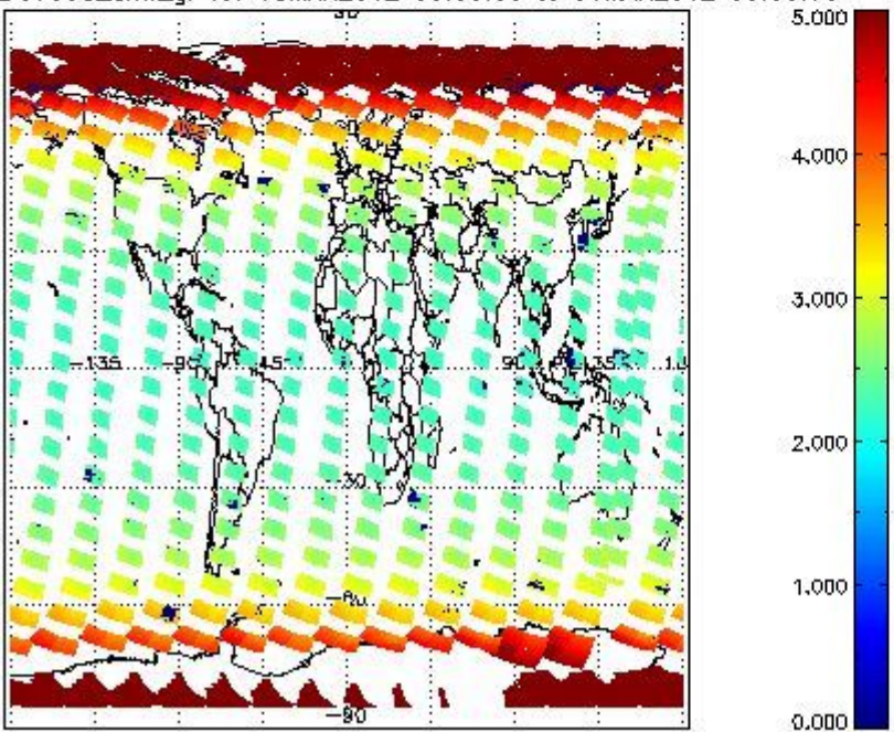
SCIOL2P_NADUV003_amf_gr for 05MAR2012 00:00:00 to 06MAR2012 00:00:00
