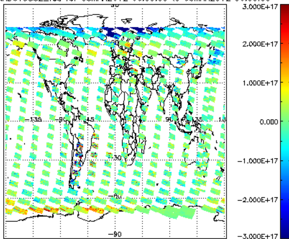
SCIOL2P_NADUV5S02_vcd for 05MAR2012 00:00:00 to 06MAR2012 00:00:00
