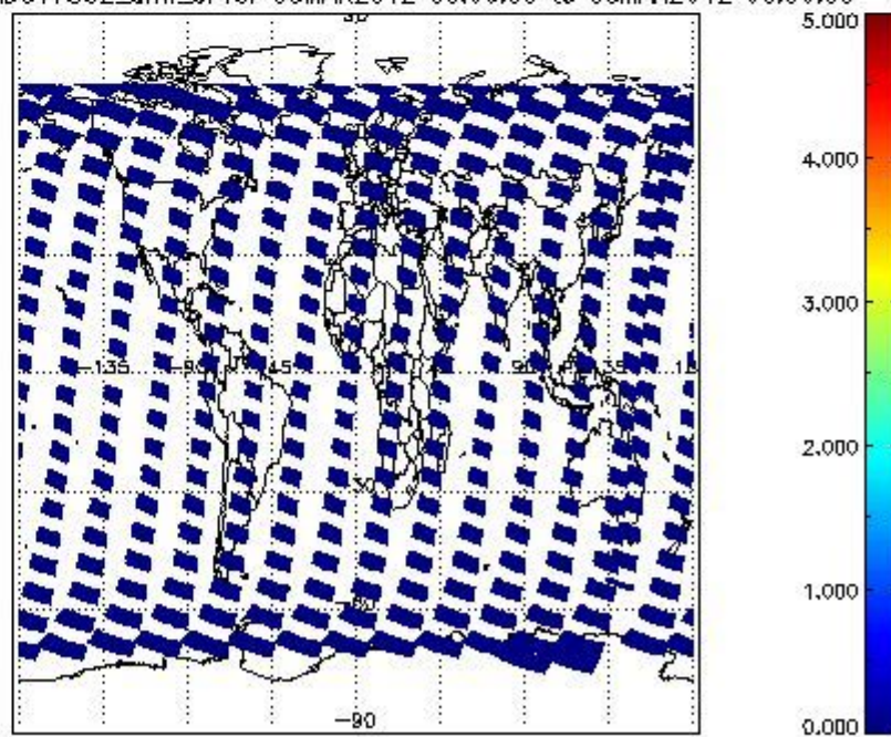
SCIOL2P_NADUV7S02_amf_cl for 05MAR2012 00:00:00 to 06MAR2012 00:00:00
