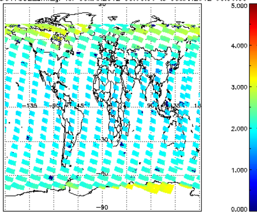
SCIOL2P_NADUV7S02_amf_gr for 05MAR2012 00:00:00 to 06MAR2012 00:00:00
