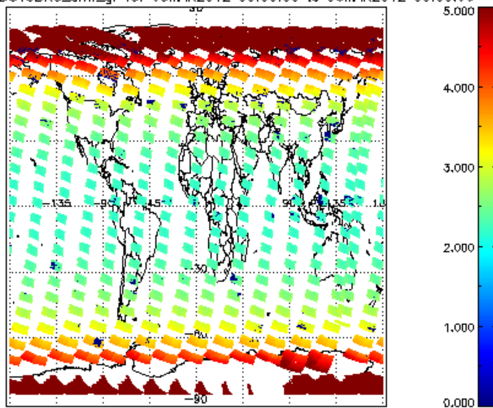
SCIOL2P_NADUV3BRO_amf_gr for 05MAR2012 00:00:00 to 06MAR2012 00:00:00
