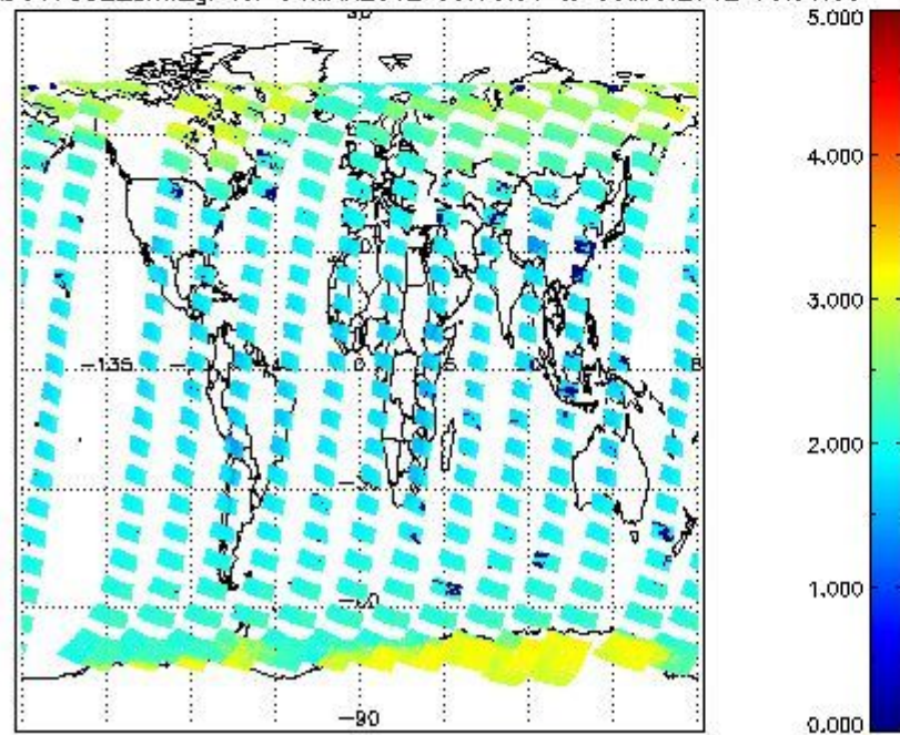
SCIOL2P_NADUV7S02_amf_gr for 04MAR2012 00:00:00 to 05MAR2012 00:00:00
