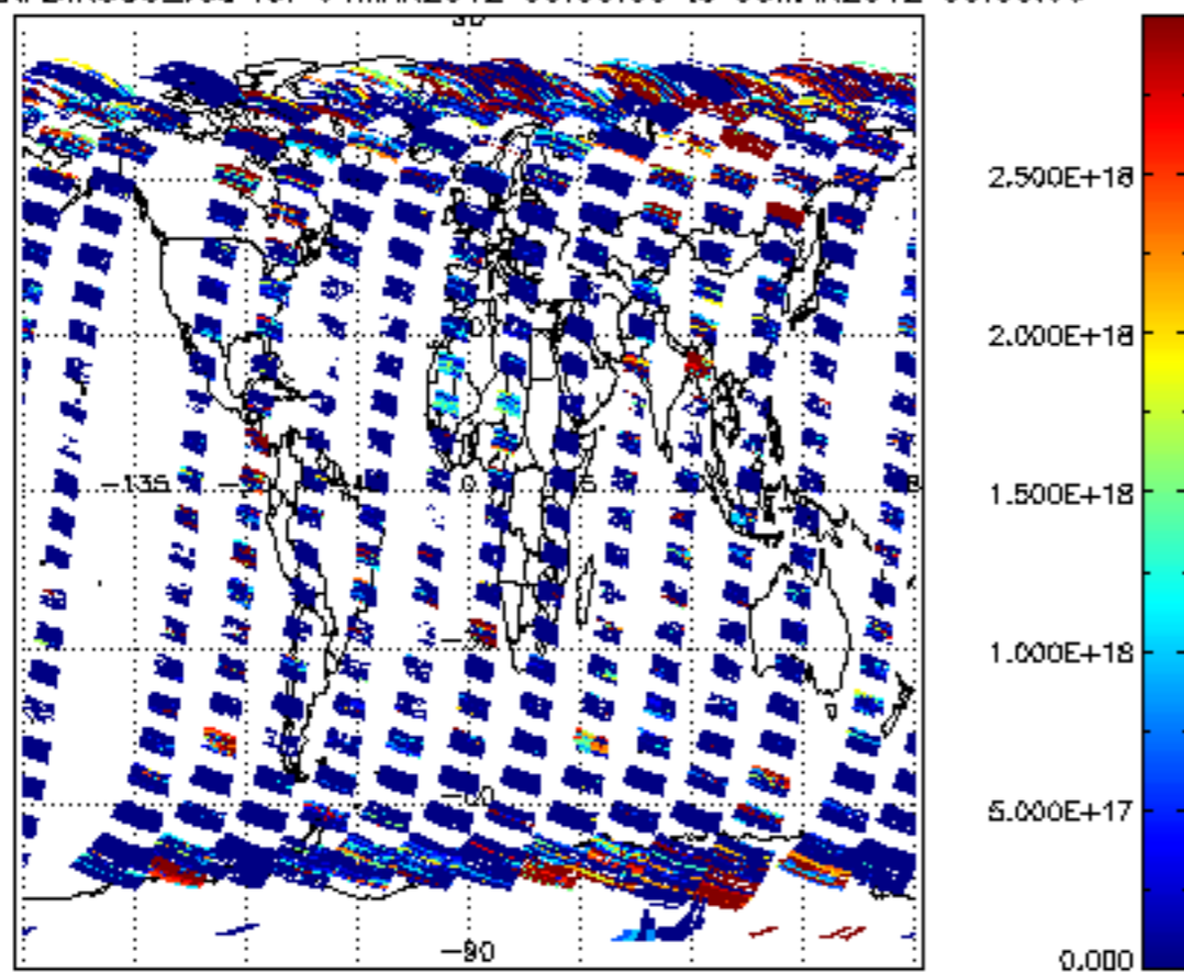
SCIOL2P_NADIR3CO_vcd for 04MAR2012 00:00:00 to 05MAR2012 00:00:00
