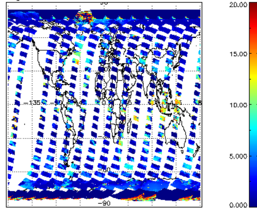
cL_top_height for 04MAR2012 00:00:00 to 05MAR2012 00:00:00
