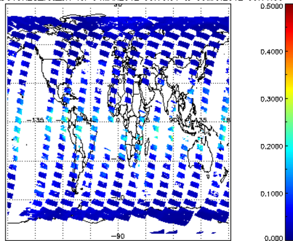
SCIOL2P_NADUV8H20_vcd_Lerr for 04MAR2012 00:00:00 to 05MAR2012 00:00:00
