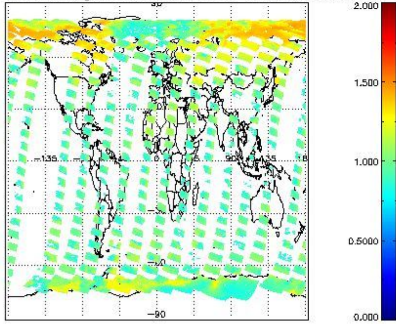
SCIOL2P_NADUV8H2O_arnf_gr for 04MAR2012 00:00:00 to 05MAR2012 00:00:00
