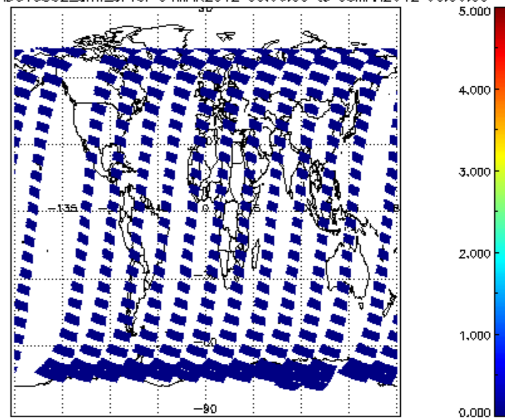
SCIOL2P_NADUV5S02_amf_cl for 04MAR2012 00:00:00 to 05MAR2012 00:00:00
