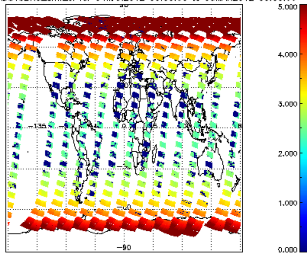
SCIOL2P_NADUV3BRO_arnf_cl for 04MAR2012 00:00:00 to 05MAR2012 00:00:00
