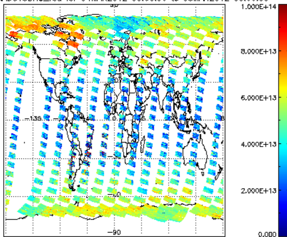
SCIOL2P_NADUV3BRO_vcd for 04MAR2012 00:00:00 to 05MAR2012 00:00:00
