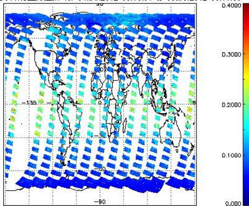
SCIOL2P_NADUV1NO2_vcd_err for 04MAR2012 00:00:00 to 05MAR2012 00:00:00
