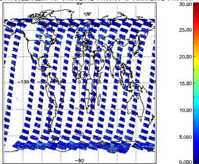
SCIOL2P_NADUV7S02_vcd_err for 04MAR2012 00:00:00 to 05MAR2012 00:00:00
