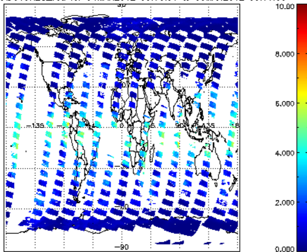
SCIOL2P_NADUV8H20_vcd for 04MAR2012 00:00:00 to 05MAR2012 00:00:00
