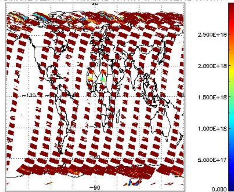
SCIDL2P_NADIR3CO_vcd_err for 04MAR2012 00:00:00 to 05MAR2012 00:00:00
