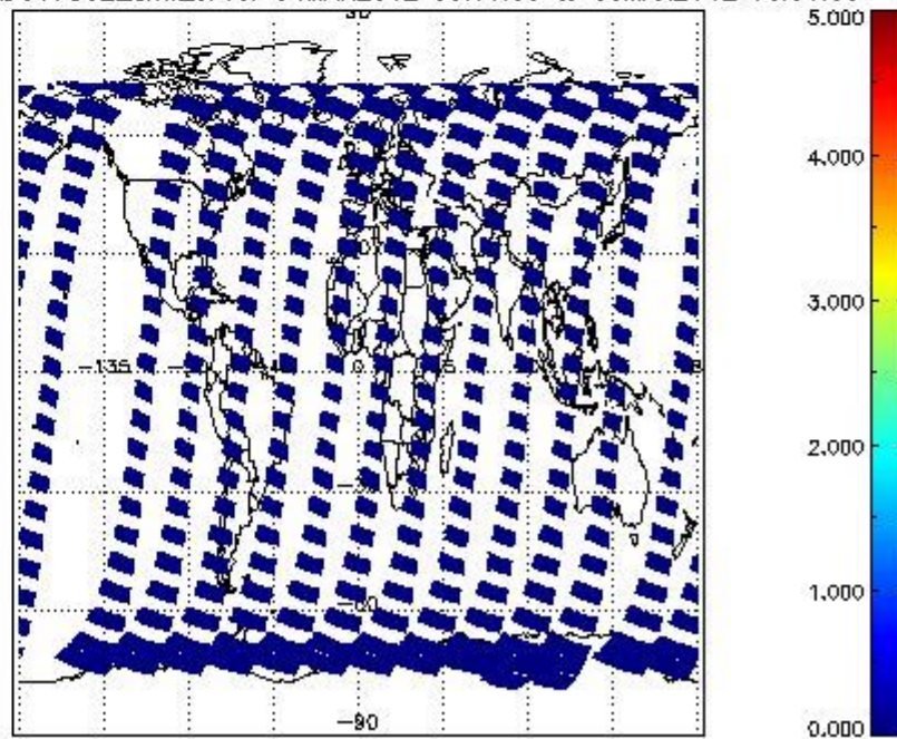
SCIOL2P_NADUV7S02_amf_cl for 04MAR2012 00:00:00 to 05MAR2012 00:00:00
