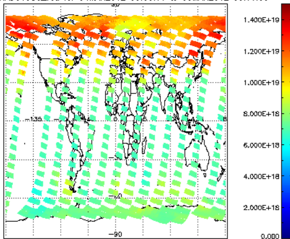
SCIOL2P_NADUV003_vcd for 04MAR2012 00:00:00 to 05MAR2012 00:00:00
