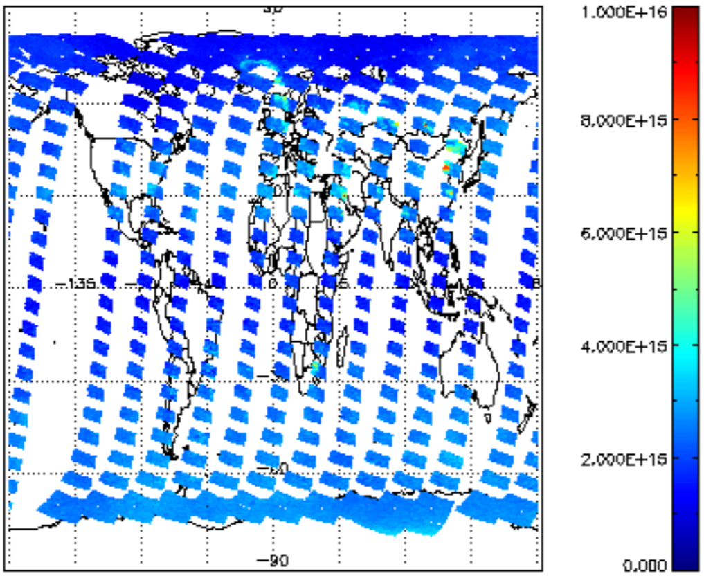
SCIOL2P_NADUV1NO2_vcd for 04MAR2012 00:00:00 to 05MAR2012 00:00:00
