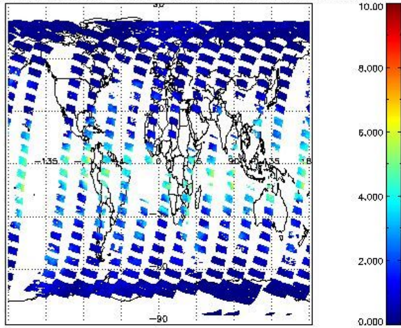
SCIOL2P_NADUV8H2O_vcd for 04MAR2012 00:00:00 to 05MAR2012 00:00:00
