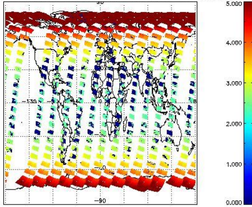
SCIOL2P_NADUV3BRO_amf_cl for 04MAR2012 00:00:00 to 05MAR2012 00:00:00
