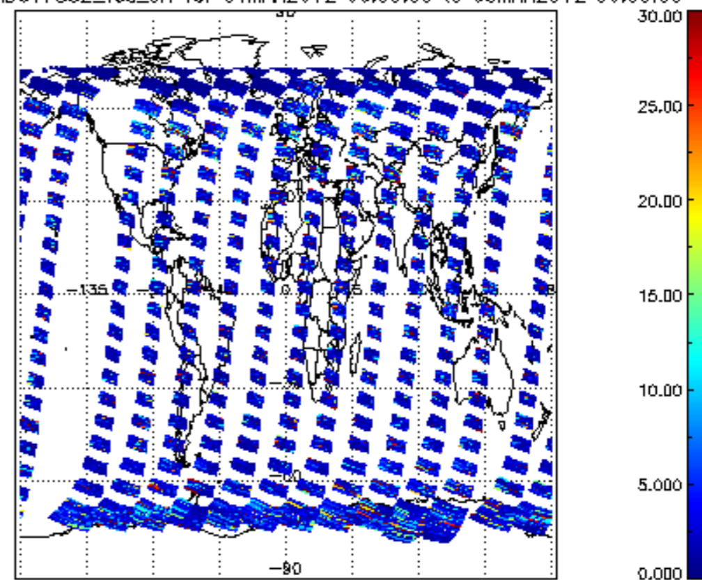
SCIOL2P_NADUV7S02_vcd_err for 04MAR2012 00:00:00 to 05MAR2012 00:00:00
