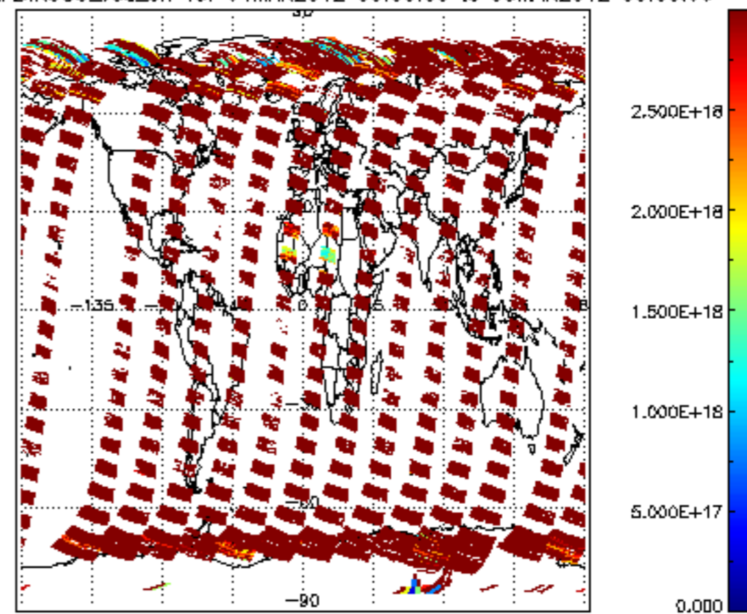
SCIOL2P_NADIR3CO_vcd_err for 04MAR2012 00:00:00 to 05MAR2012 00:00:00
