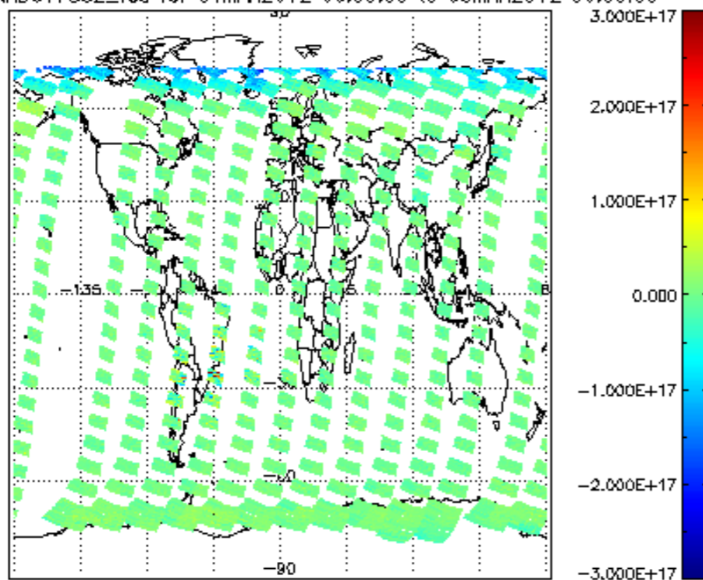
SCIOL2P_NADUV7S02_vcd for 04MAR2012 00:00:00 to 05MAR2012 00:00:00
