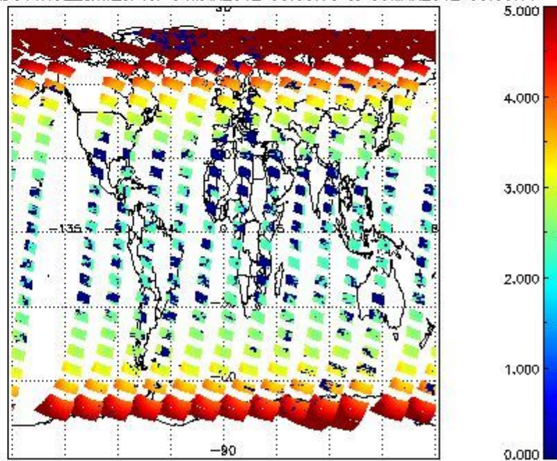
SCIOL2P_NADUV1NO2_amf_cl for 04MAR2012 00:00:00 to 05MAR2012 00:00:00
