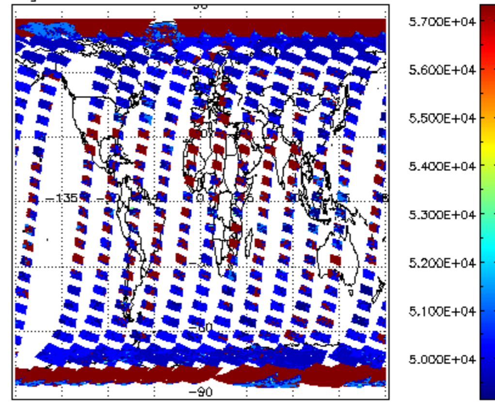
cloud_flags for 04MAR2012 00:00:00 to 05MAR2012 00:00:00
