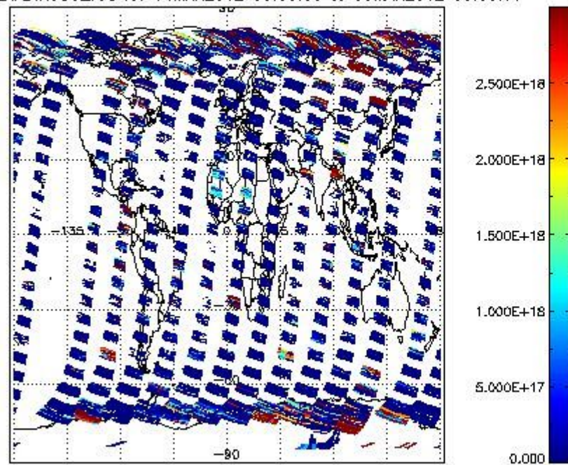
SCIDL2P_NADIR3CO_vcd for 04MAR2012 00:00:00 to 05MAR2012 00:00:00
