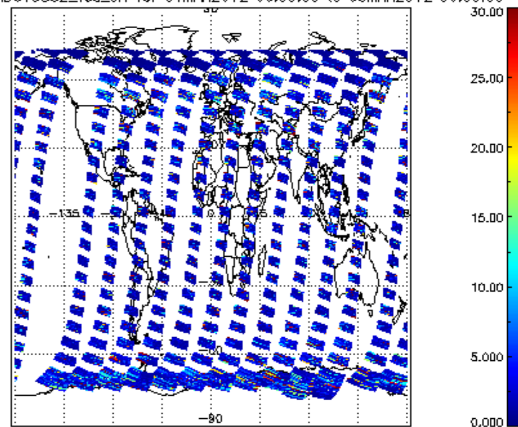
SCIOL2P_NADUV5S02_vcd_err for 04MAR2012 00:00:00 to 05MAR2012 00:00:00
