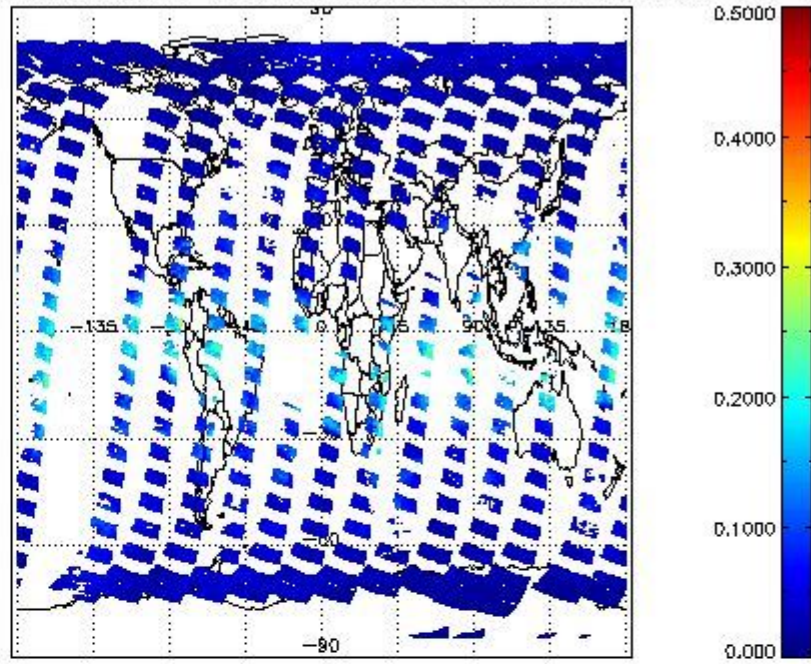
SCIOL2P_NADUV8H2O_vcd_err for 04MAR2012 00:00:00 to 05MAR2012 00:00:00
