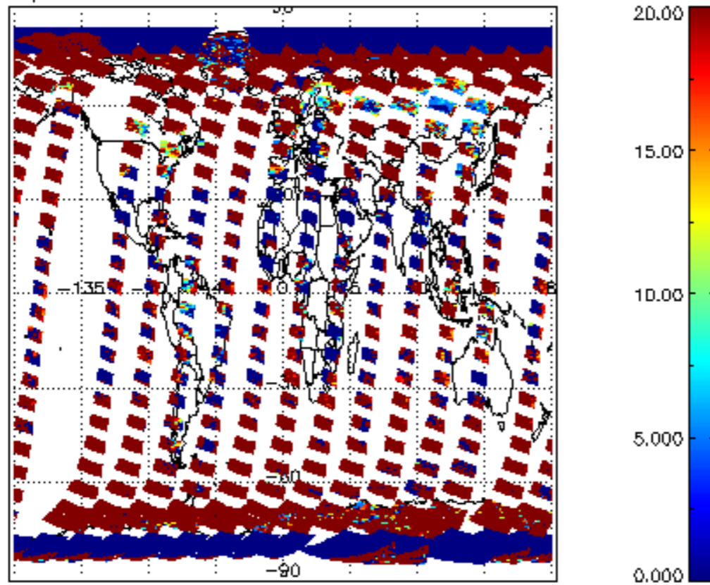
cL_opt_depth for 04MAR2012 00:00:00 to 05MAR2012 00:00:00
