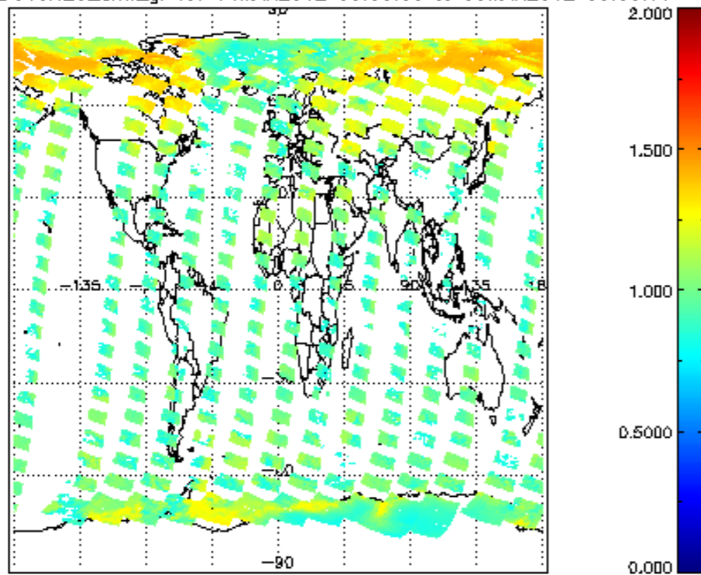
SCIOL2P_NADUV8H20_arnf_gr for 04MAR2012 00:00:00 to 05MAR2012 00:00:00
