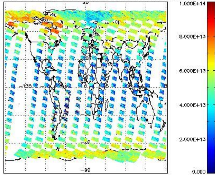
SCIOL2P_NADUV3BRO_vcd for 04MAR2012 00:00:00 to 05MAR2012 00:00:00
