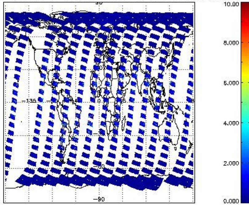
SCIOL2P_NADUV3BRO_vcd_err for 04MAR2012 00:00:00 to 05MAR2012 00:00:00
