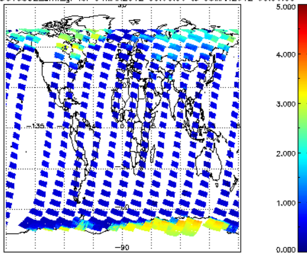
SCIOL2P_NADUV5S02_amf_gr for 04MAR2012 00:00:00 to 05MAR2012 00:00:00
