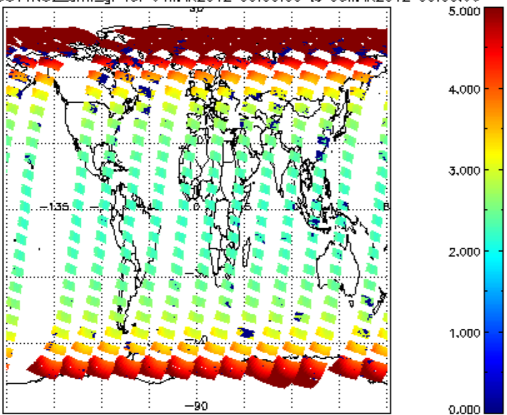
SCIOL2P_NADUV1NO2_amf_gr for 04MAR2012 00:00:00 to 05MAR2012 00:00:00
