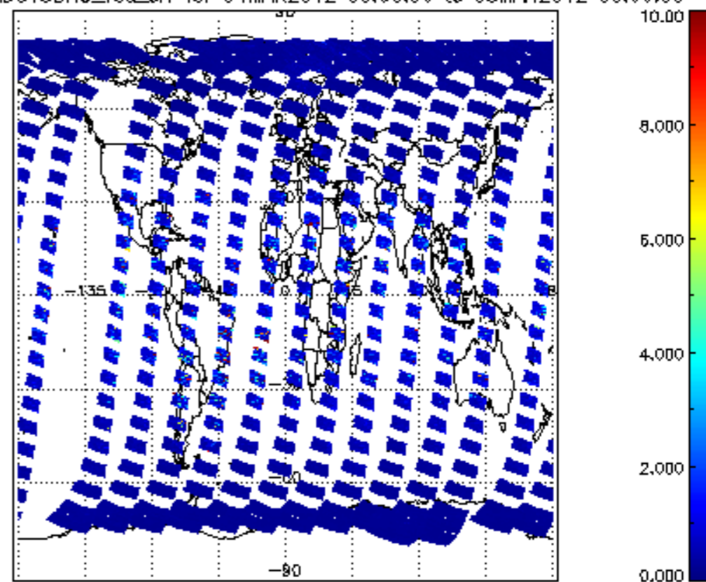
SCIOL2P_NADUV3BRO_vcd_err for 04MAR2012 00:00:00 to 05MAR2012 00:00:00
