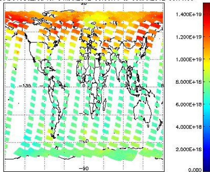
SCIOL2P_NADUV003_vcd for 04MAR2012 00:00:00 to 05MAR2012 00:00:00
