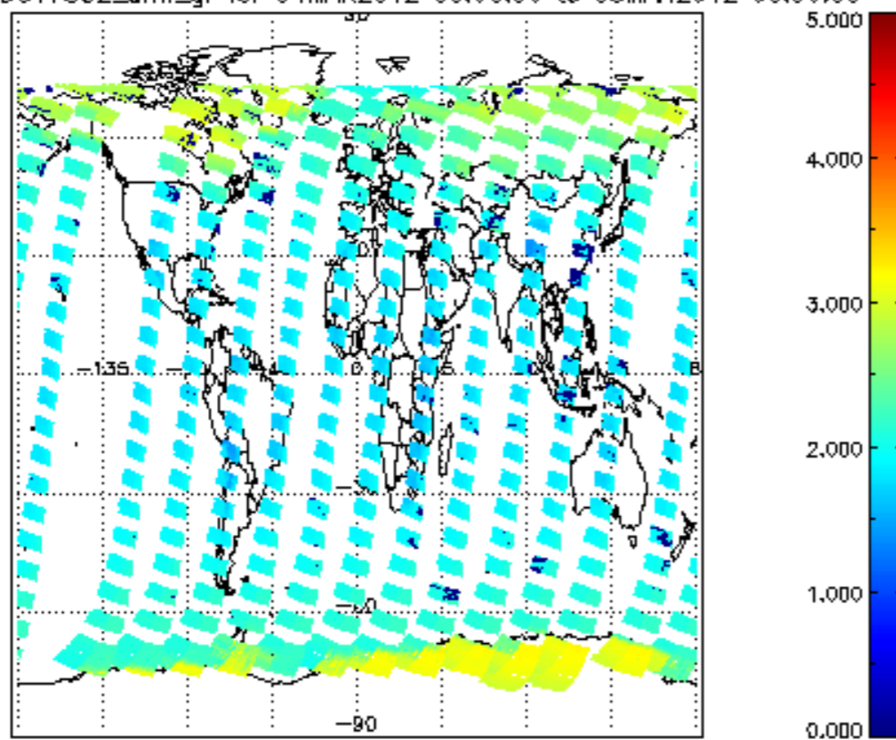
SCIOL2P_NADUV7S02_amf_gr for 04MAR2012 00:00:00 to 05MAR2012 00:00:00
