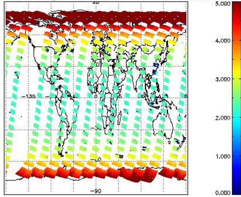
SCIOL2P_NADUV3BRO_amf_gr for 04MAR2012 00:00:00 to 05MAR2012 00:00:00
