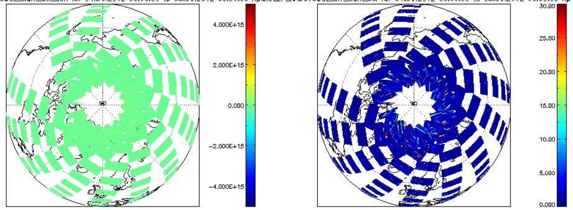
CIOL2P_NADUV6OCLslant_col_den for 04MAR2012 00:00:00 to 05MAR2012 00:00:00 npCIOL2P_NADUV6OCLerr_slant_col for 04MAR2012 00:00:00 to 05MAR2012 00:00:00 np
