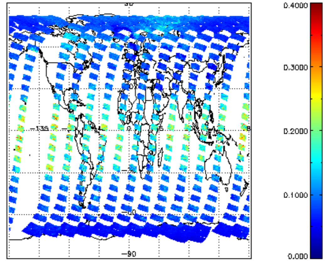
SCIOL2P_NADUV1NO2_vcd_err for 04MAR2012 00:00:00 to 05MAR2012 00:00:00
