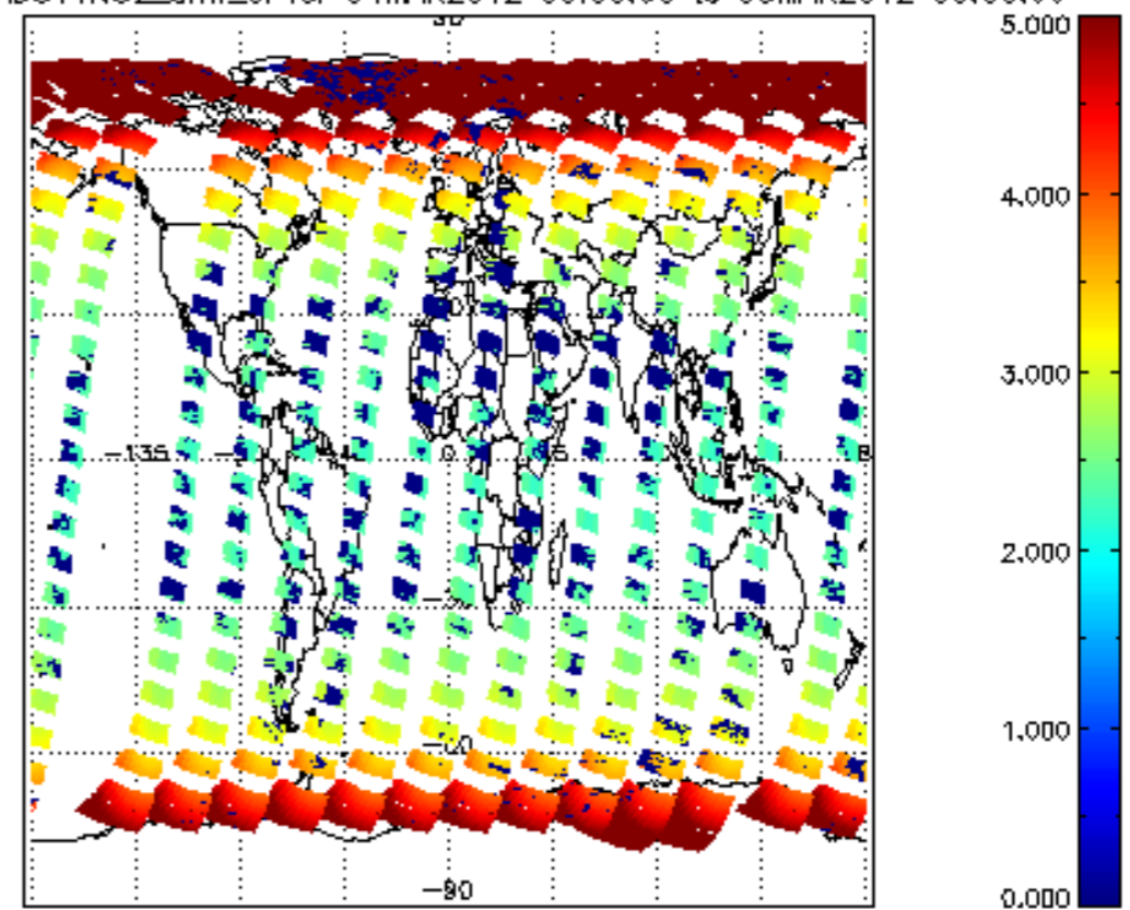
SCIOL2P_NADUV1NO2_amf_cl for 04MAR2012 00:00:00 to 05MAR2012 00:00:00
