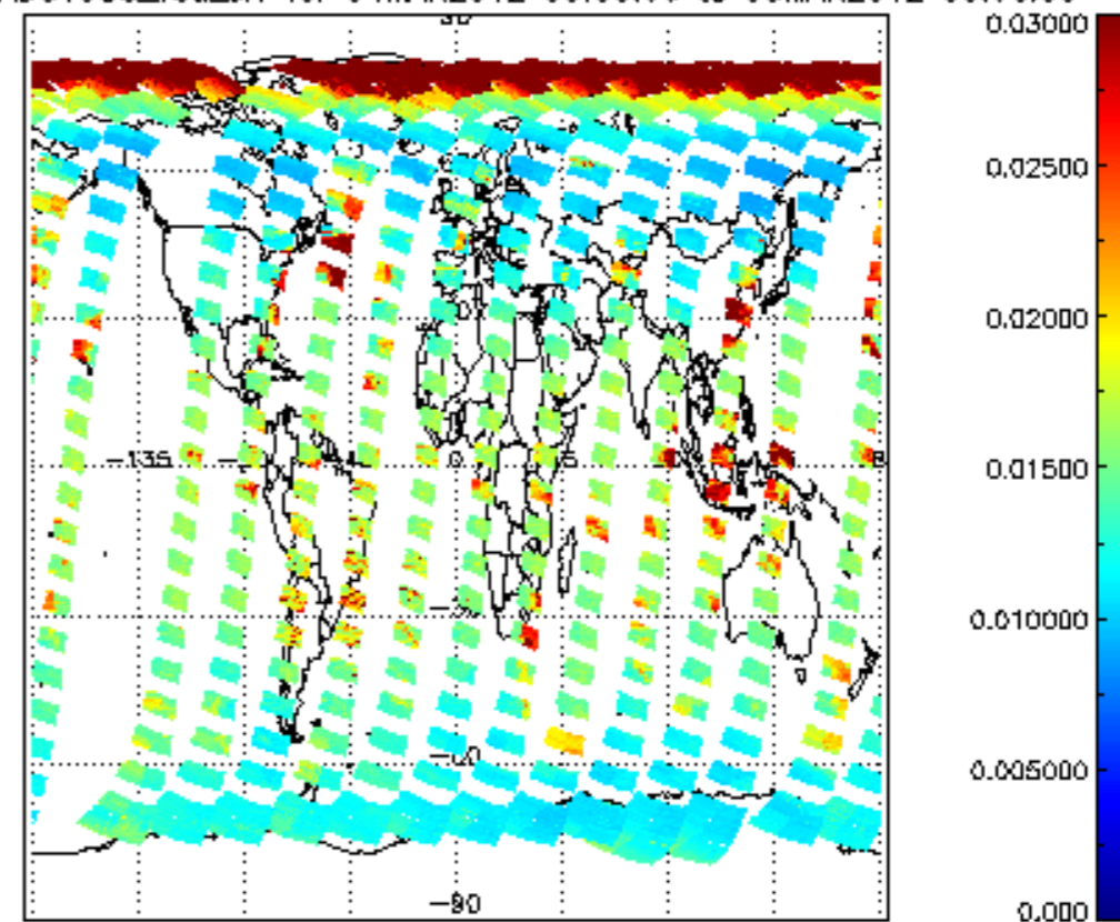
SCIOL2P_NADUV003_vcd_err for 04MAR2012 00:00:00 to 05MAR2012 00:00:00
