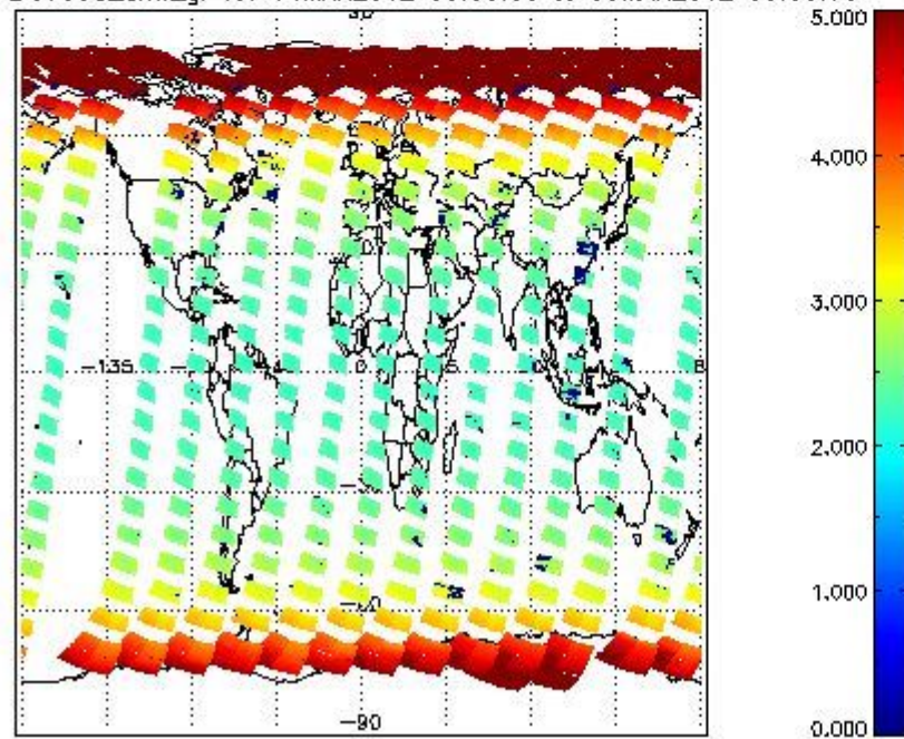
SCIOL2P_NADUV003_amf_gr for 04MAR2012 00:00:00 to 05MAR2012 00:00:00
