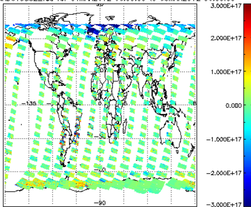
SCIOL2P_NADUV5S02_vcd for 04MAR2012 00:00:00 to 05MAR2012 00:00:00
