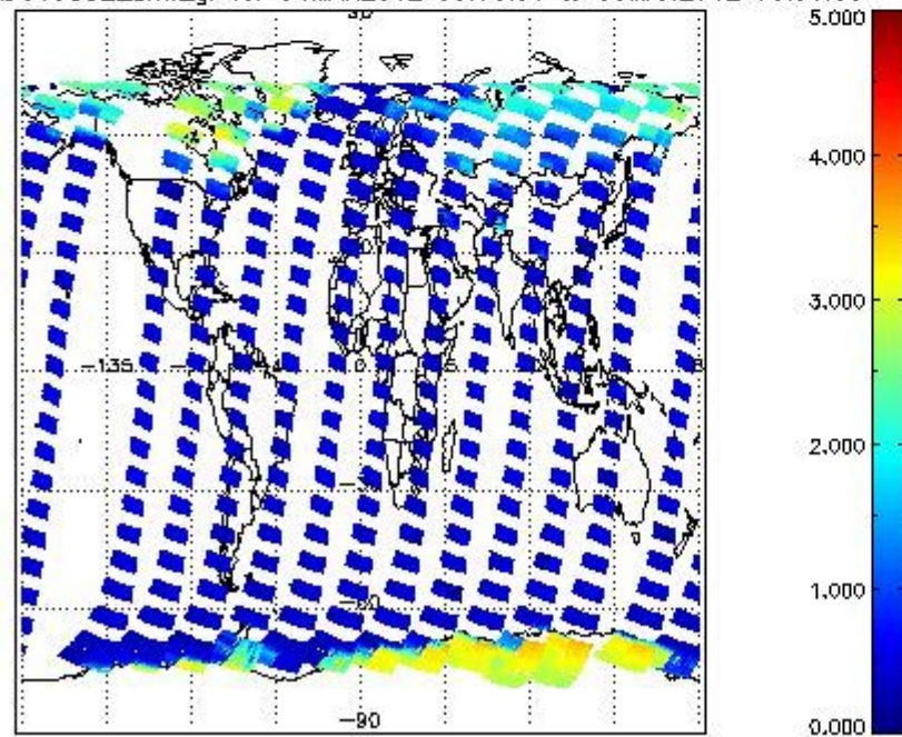
SCIOL2P_NADUV5S02_amf_gr for 04MAR2012 00:00:00 to 05MAR2012 00:00:00
