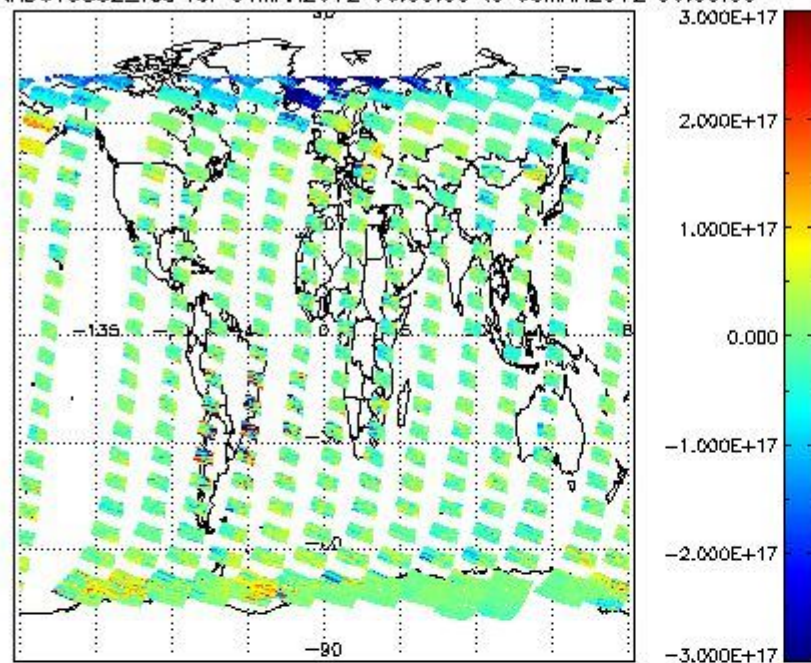
SCIOL2P_NADUV5S02_vcd for 04MAR2012 00:00:00 to 05MAR2012 00:00:00
