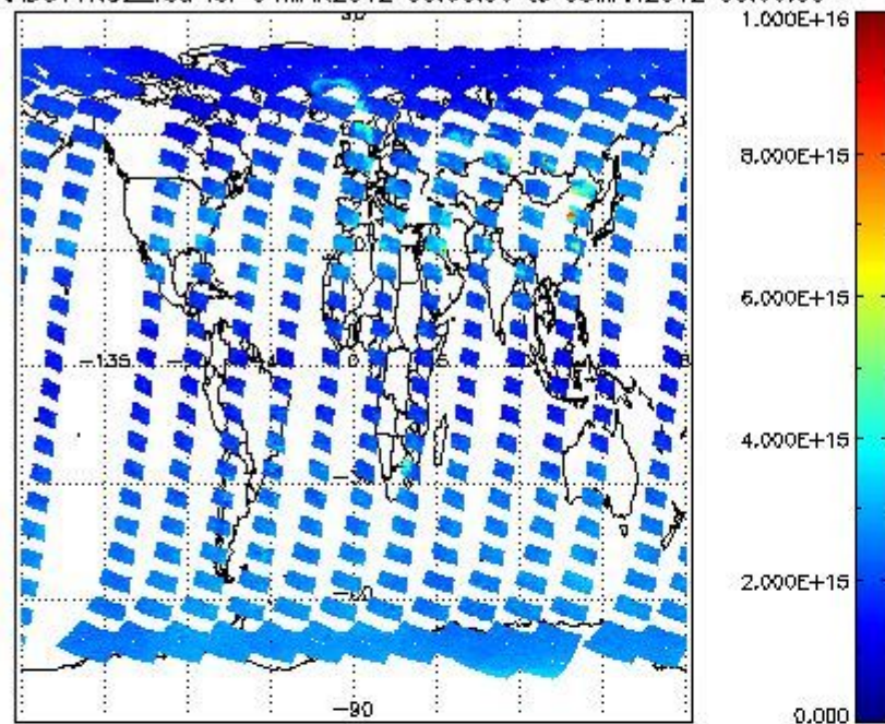
SCIOL2P_NADUV1NO2_vcd for 04MAR2012 00:00:00 to 05MAR2012 00:00:00
