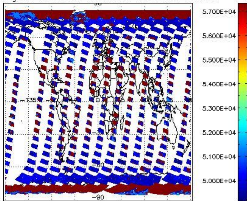
cloud_flags for 04MAR2012 00:00:00 to 05MAR2012 00:00:00
