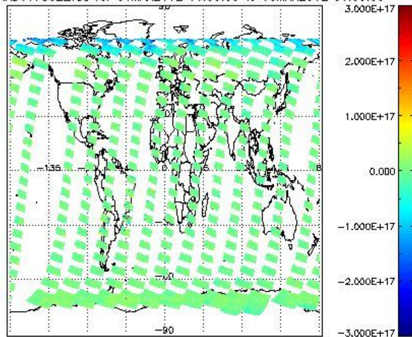
SCIOL2P_NADUV7S02_vcd for 04MAR2012 00:00:00 to 05MAR2012 00:00:00
