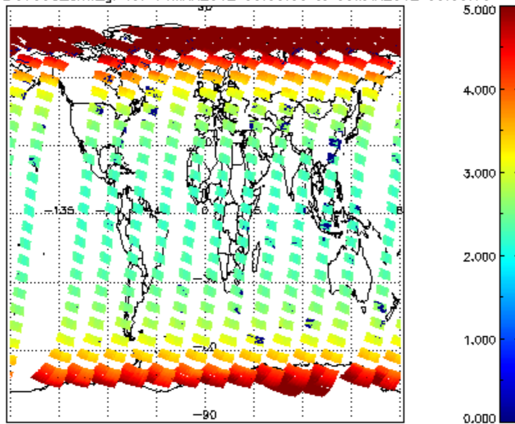
SCIOL2P_NADUV003_amf_gr for 04MAR2012 00:00:00 to 05MAR2012 00:00:00
