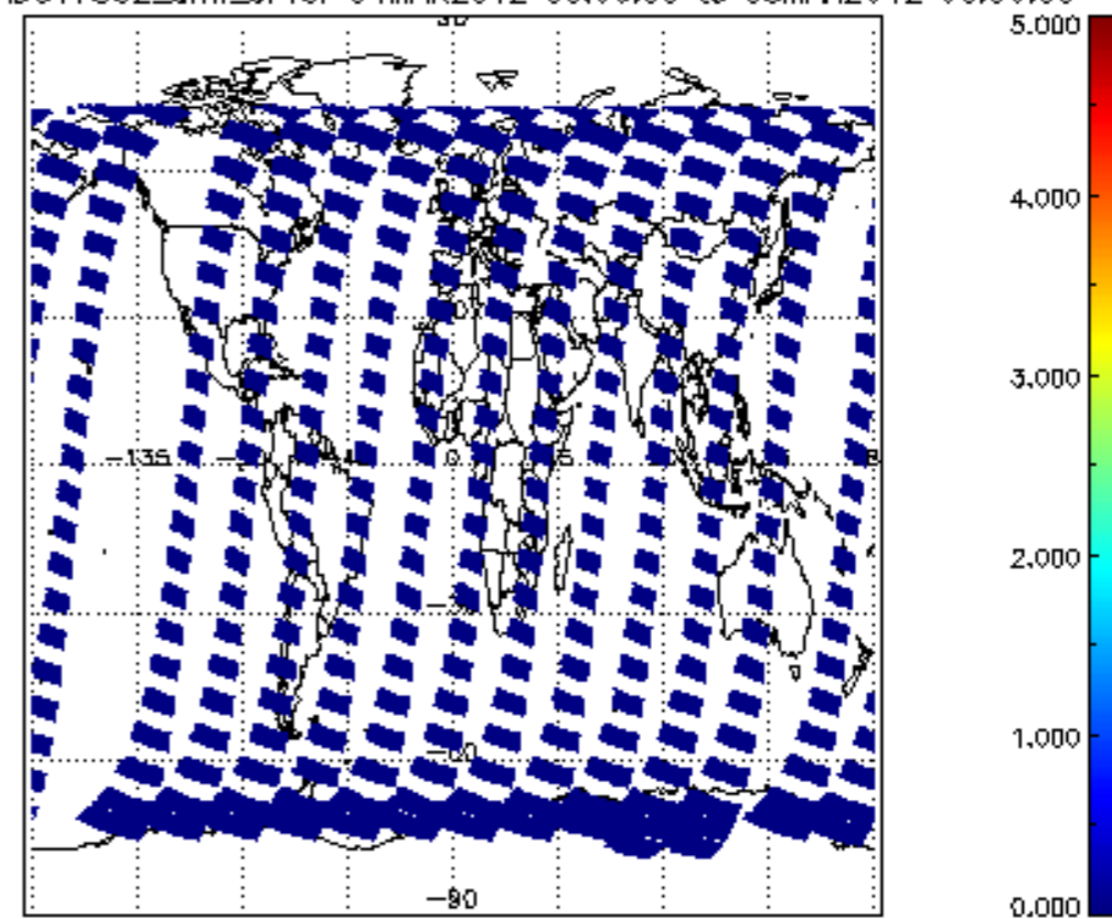
SCIOL2P_NADUV7S02_amf_cl for 04MAR2012 00:00:00 to 05MAR2012 00:00:00
