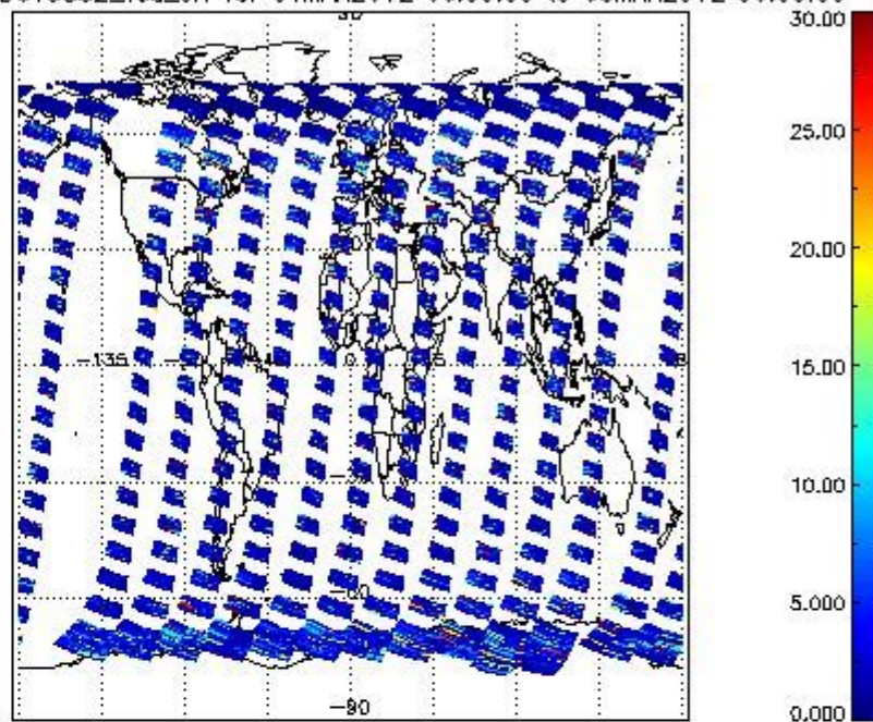
SCIOL2P_NADUV5S02_vcd_err for 04MAR2012 00:00:00 to 05MAR2012 00:00:00
