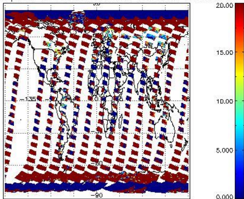
cL_opt_depth for 04MAR2012 00:00:00 to 05MAR2012 00:00:00
