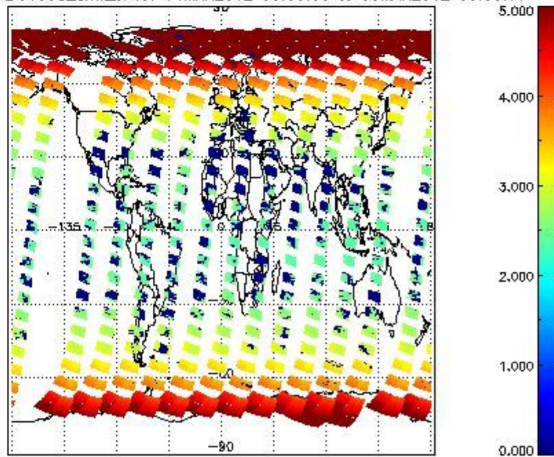
SCIOL2P_NADUV003_amf_cl for 04MAR2012 00:00:00 to 05MAR2012 00:00:00
