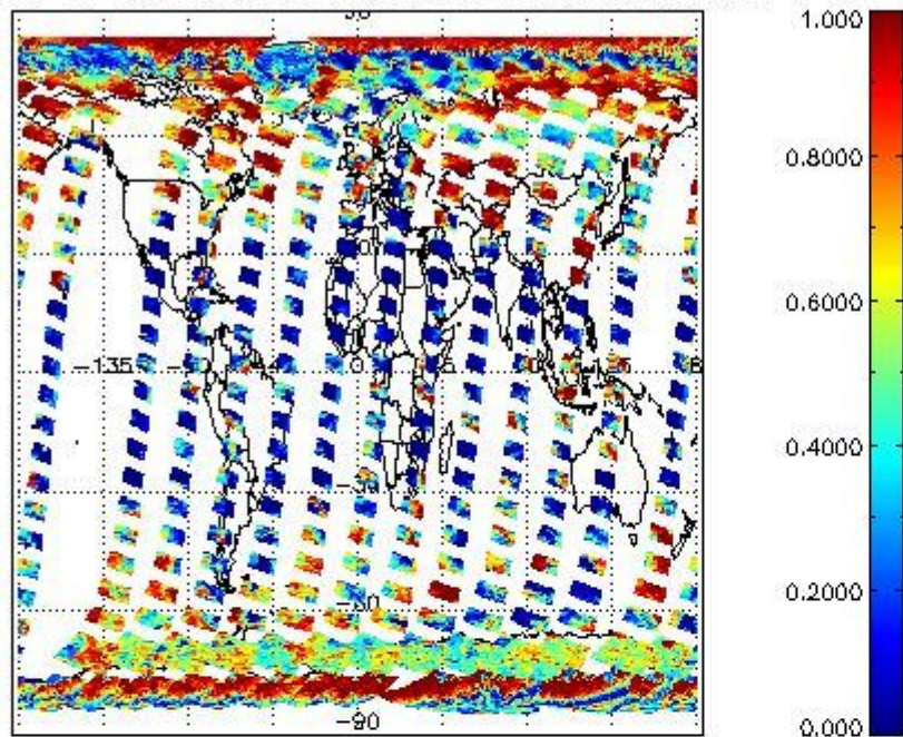
cL_frac for 04MAR2012 00:00:00 to 05MAR2012 00:00:00
