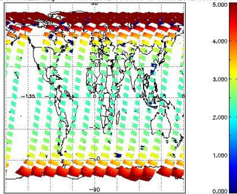
SCIOL2P_NADUV1NO2_amf_gr for 04MAR2012 00:00:00 to 05MAR2012 00:00:00
