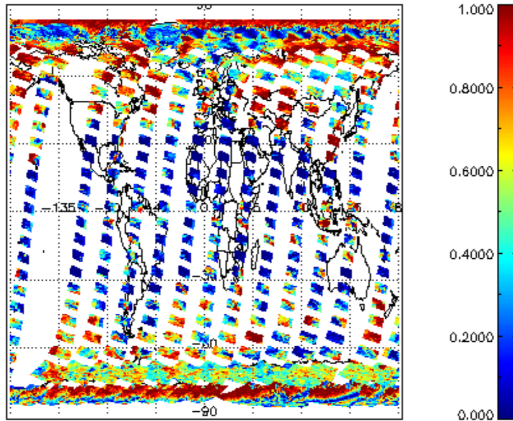
cL_frac for 04MAR2012 00:00:00 to 05MAR2012 00:00:00
