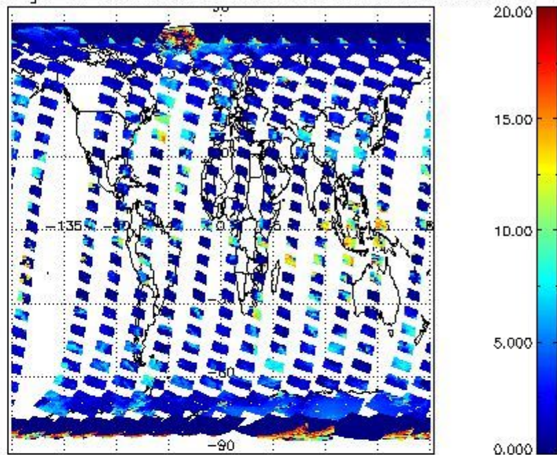
cL_top_height for 04MAR2012 00:00:00 to 05MAR2012 00:00:00
