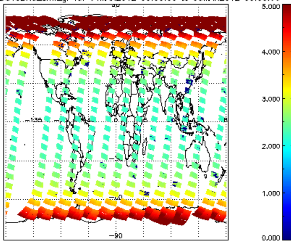
SCIOL2P_NADUV3BRO_arnf_gr for 04MAR2012 00:00:00 to 05MAR2012 00:00:00
