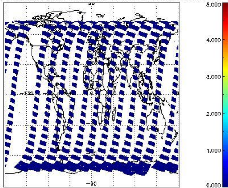
SCIOL2P_NADUV5S02_amf_cl for 04MAR2012 00:00:00 to 05MAR2012 00:00:00
