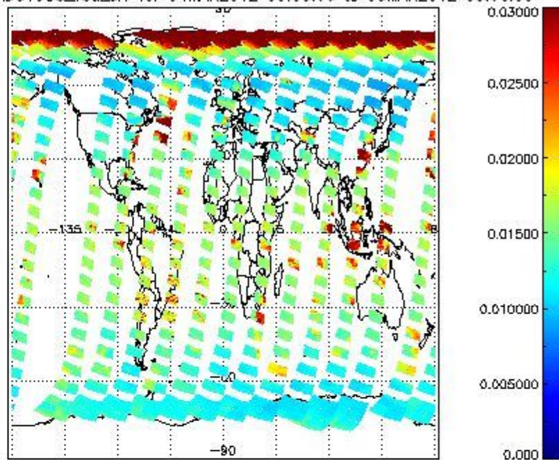
SCIOL2P_NADUV003_vcd_err for 04MAR2012 00:00:00 to 05MAR2012 00:00:00
