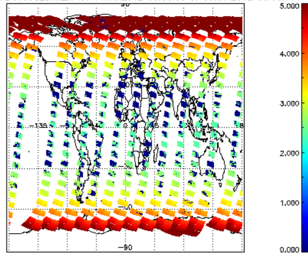
SCIOL2P_NADUV003_amf_cl for 04MAR2012 00:00:00 to 05MAR2012 00:00:00
