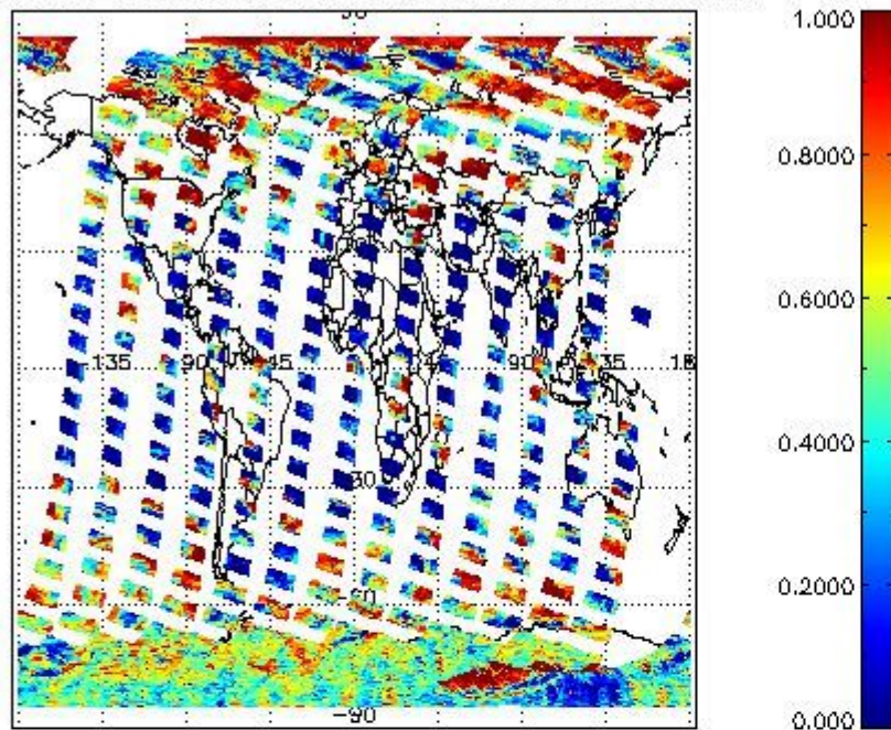
cLfrac for 29FEB2012 00:00:00 to 01MAR2012 00:00:00
