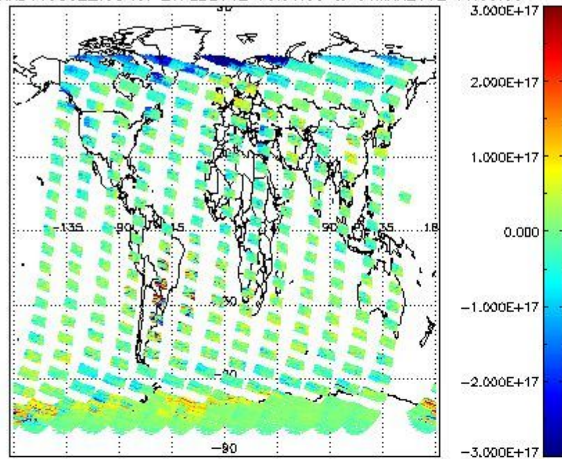
SCIOL2P_NADUV5S02_vcd for 29FEB2012 00:00:00 to 01MAR2012 00:00:00
