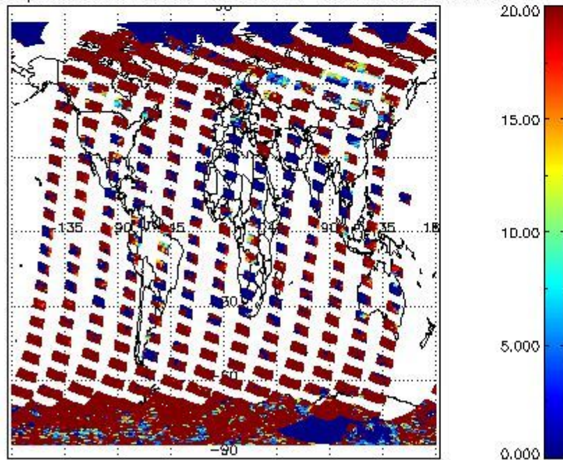
cL_opt_depth for 29FEB2012 00:00:00 to 01MAR2012 00:00:00
