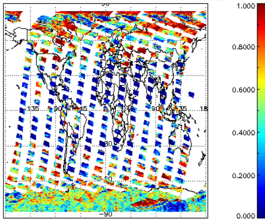
cL_frac for 29FEB2012 00:00:00 to 01MAR2012 00:00:00
