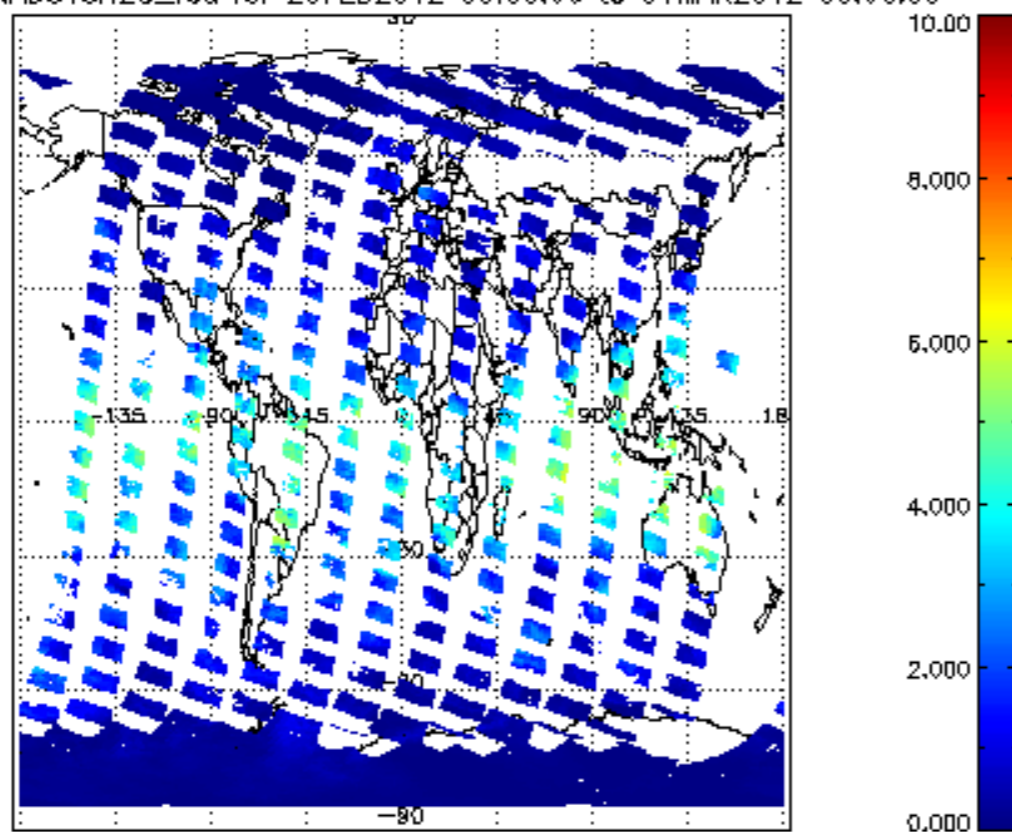
SCIOL2P_NADUV8H2O_vcd for 29FEB2012 00:00:00 to 01MAR2012 00:00:00
