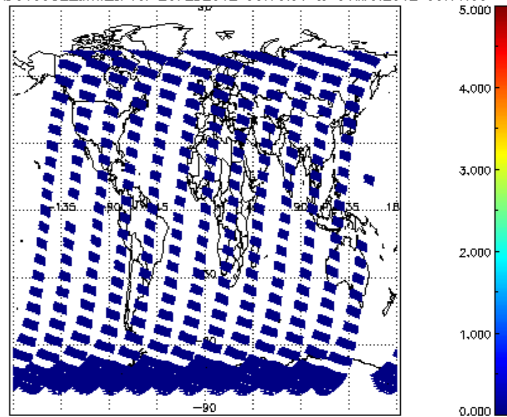
SCIOL2P_NADUV5S02_amf_cl for 29FEB2012 00:00:00 to 01MAR2012 00:00:00
