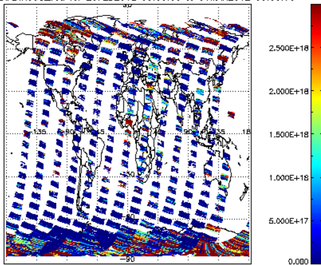
SCIOL2P_NADIR3CO_vcd for 29FEB2012 00:00:00 to 01MAR2012 00:00:00
