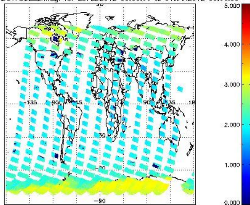
SCIOL2P_NADUV7S02_amf_gr for 29FEB2012 00:00:00 to 01MAR2012 00:00:00
