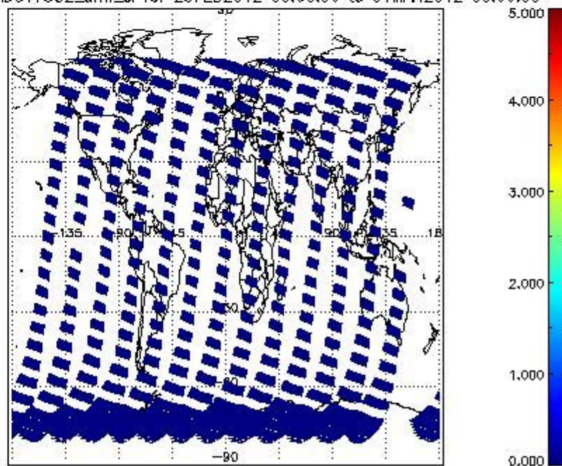
SCIOL2P_NADUV7S02_amf_cl for 29FEB2012 00:00:00 to 01MAR2012 00:00:00
