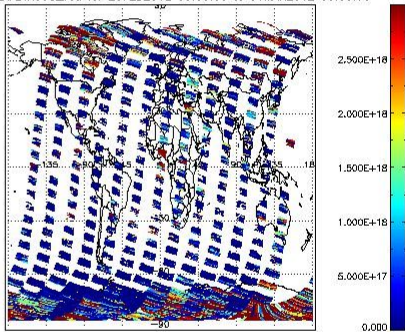
SCIDL2P_NADIR3CO_vcd for 29FEB2012 00:00:00 to 01MAR2012 00:00:00
