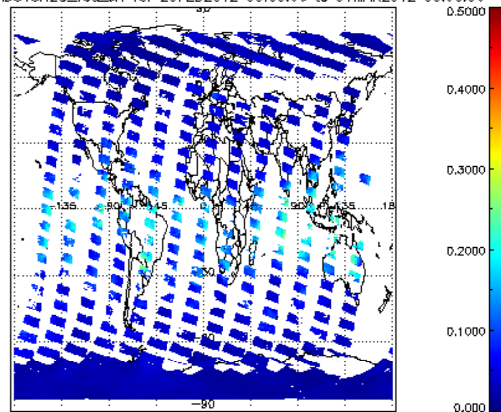
SCIOL2P_NADUV8H2O_vcd_err for 29FEB2012 00:00:00 to 01MAR2012 00:00:00
