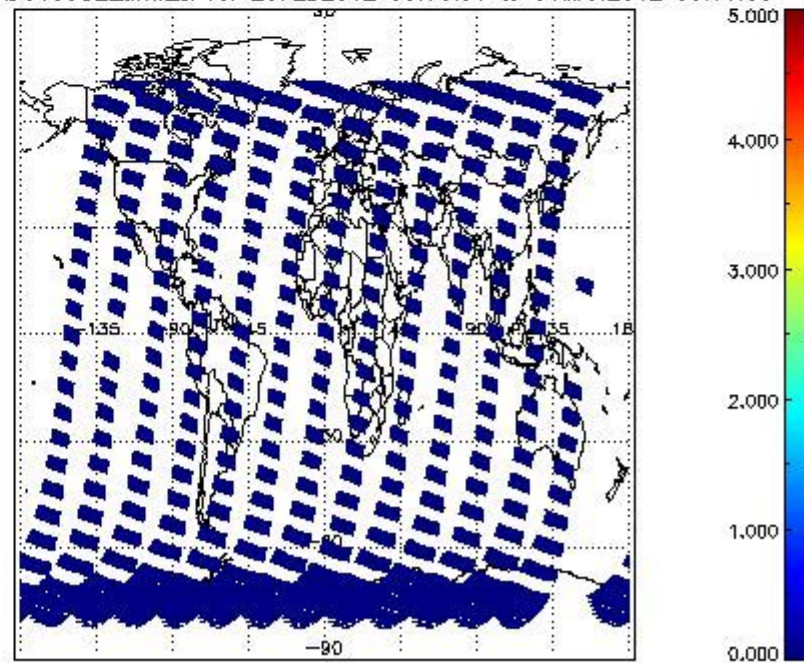
SCIOL2P_NADUV5S02_amf_cl for 29FEB2012 00:00:00 to 01MAR2012 00:00:00
