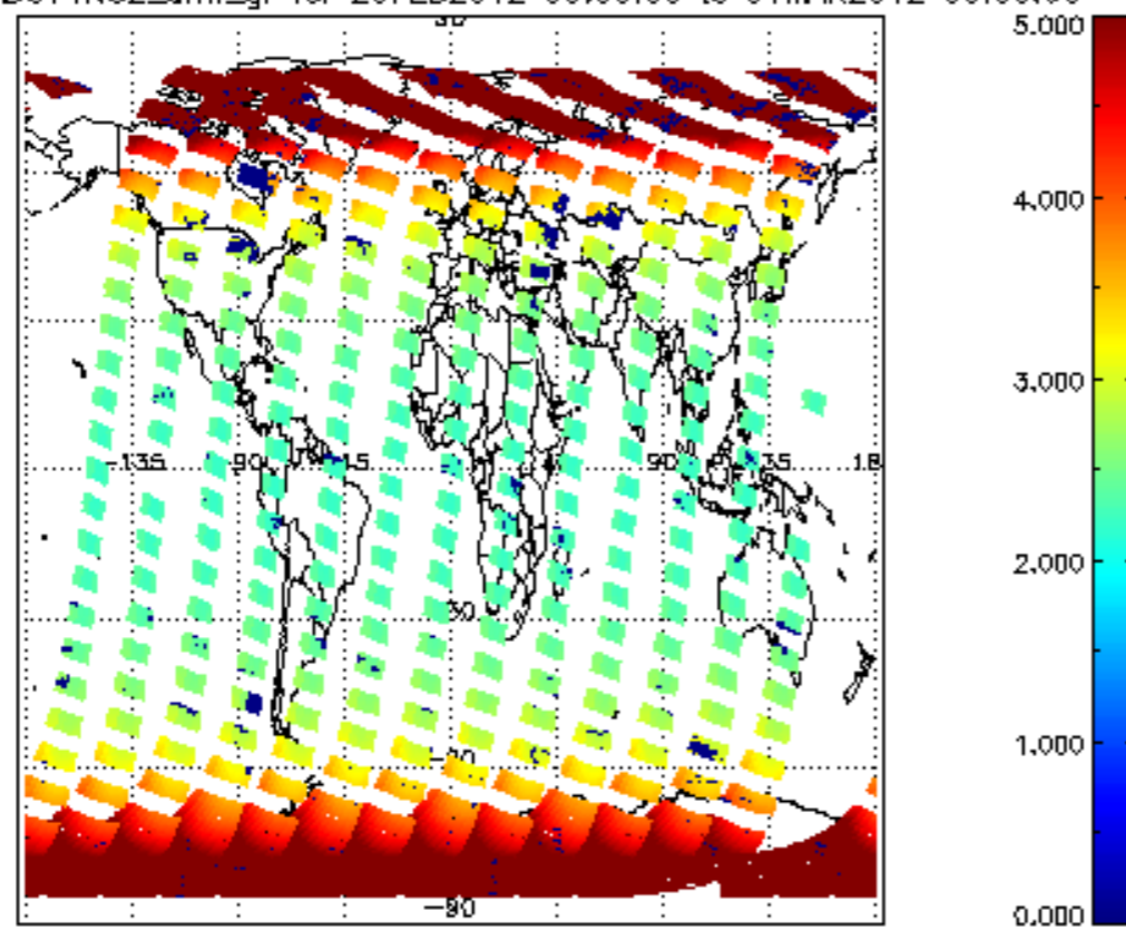
SCIOL2P_NADUV1NO2_amf_gr for 29FEB2012 00:00:00 to 01MAR2012 00:00:00
