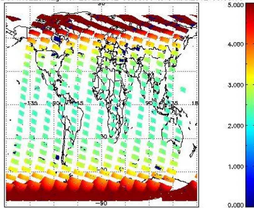
SCIOL2P_NADUV1N02_amf_gr for 29FEB2012 00:00:00 to 01MAR2012 00:00:00
