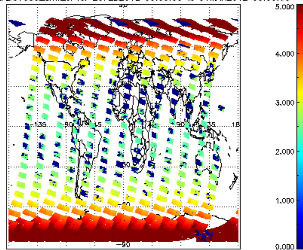
SCIOL2P_NADUV003_amf_cl for 29FEB2012 00:00:00 to 01MAR2012 00:00:00
