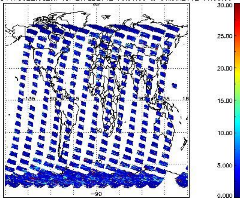
SCIOL2P_NADUV7S02_vcd_err for 29FEB2012 00:00:00 to 01MAR2012 00:00:00
