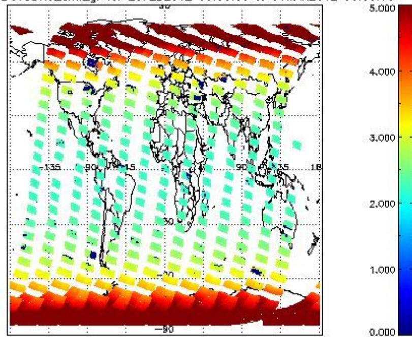
SCIOL2P_NADUV3BRO_amf_gr for 29FEB2012 00:00:00 to 01MAR2012 00:00:00
