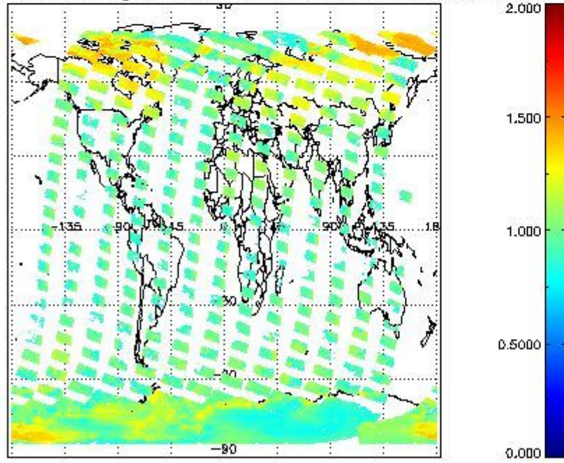
SCIOL2P_NADUV8H2O_amf_gr for 29FEB2012 00:00:00 to 01MAR2012 00:00:00
