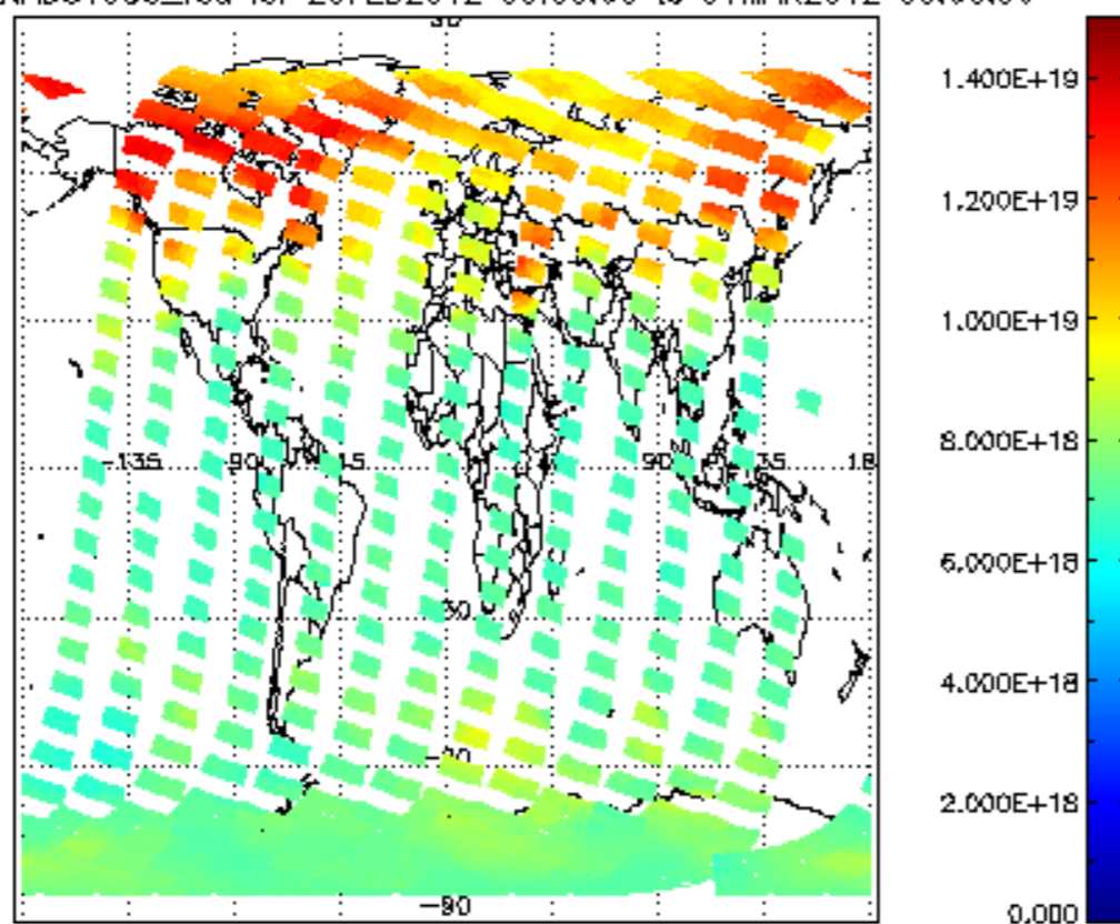
SCIOL2P_NADUV003_vcd for 29FEB2012 00:00:00 to 01MAR2012 00:00:00
