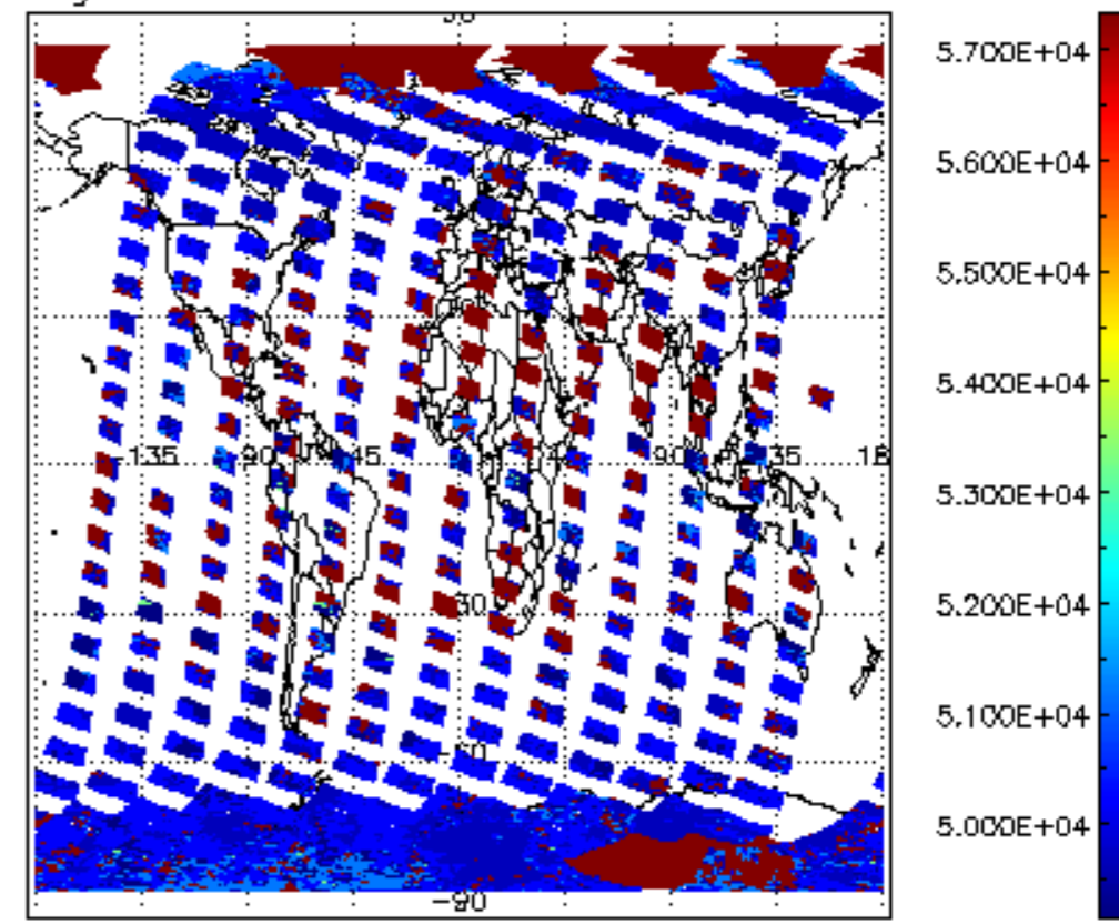
cloud_flags for 29FEB2012 00:00:00 to 01MAR2012 00:00:00
