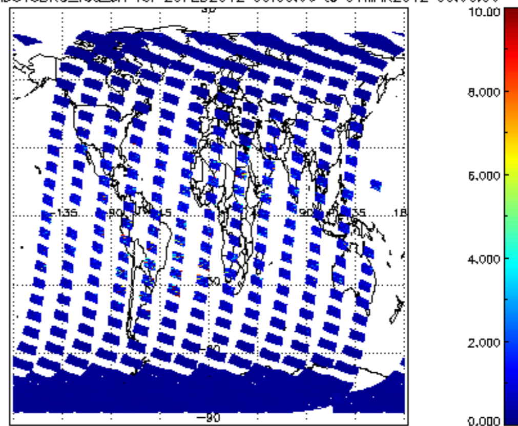
SCIOL2P_NADUV3BRO_vcd_err for 29FEB2012 00:00:00 to 01MAR2012 00:00:00
