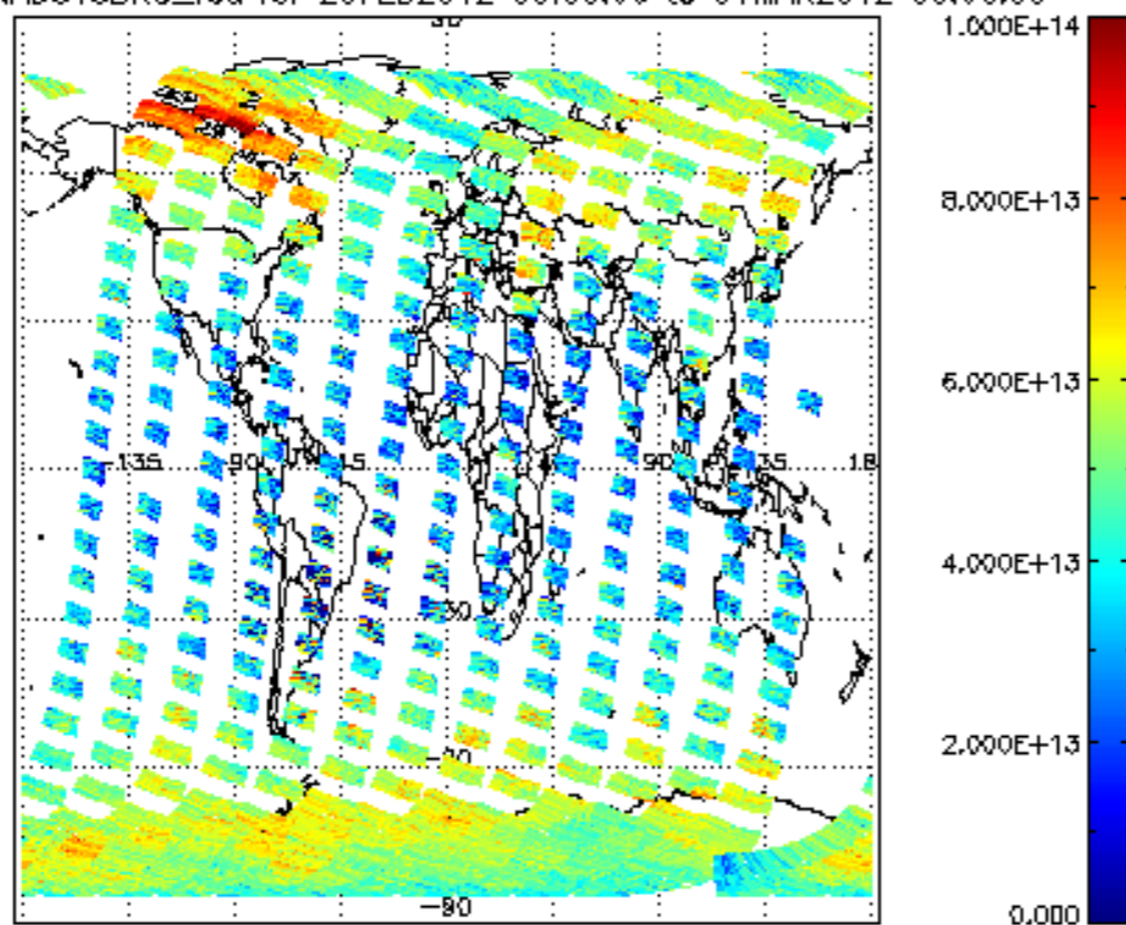
SCIOL2P_NADUV3BRO_vcd for 29FEB2012 00:00:00 to 01MAR2012 00:00:00
