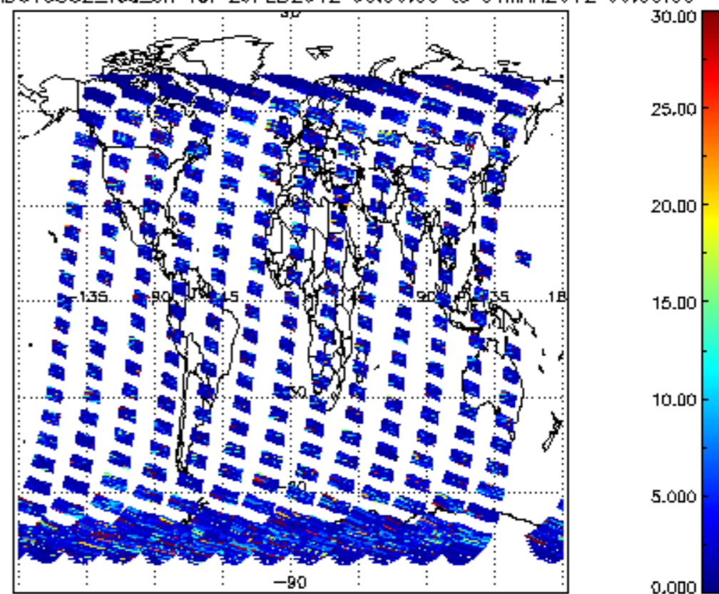
SCIOL2P_NADUV5S02_vcd_err for 29FEB2012 00:00:00 to 01MAR2012 00:00:00
