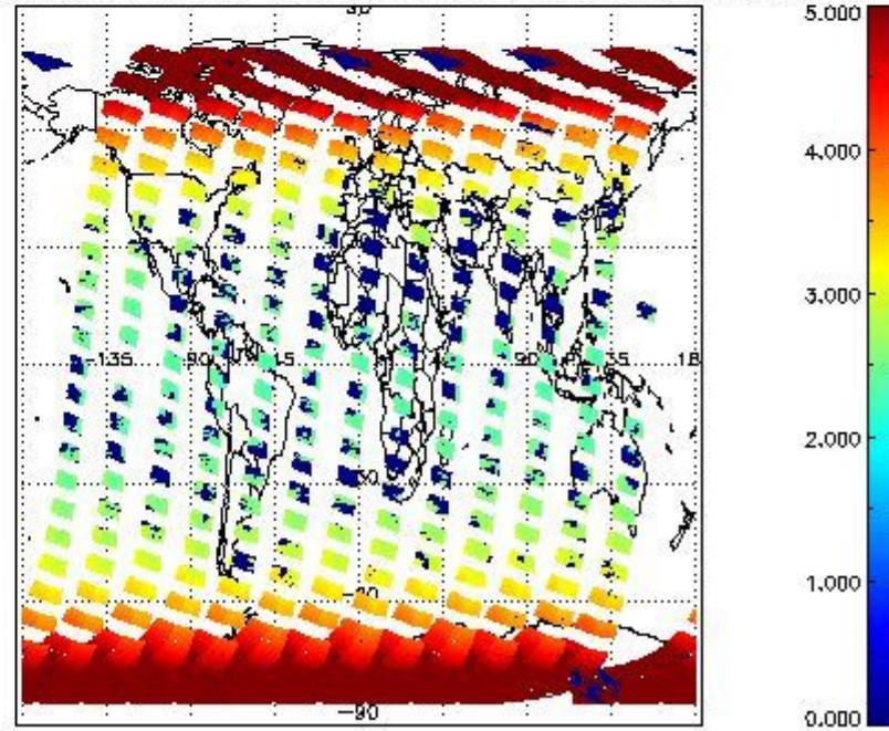
SCIOL2P_NADUV003_amf_cl for 29FEB2012 00:00:00 to 01MAR2012 00:00:00
