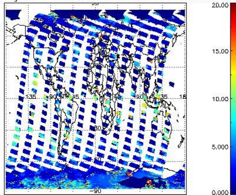
cL_top_height for 29FEB2012 00:00:00 to 01MAR2012 00:00:00
