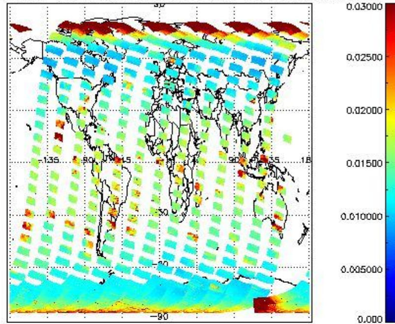
SCIOL2P_NADUV003_vcd_Lerr for 29FEB2012 00:00:00 to 01MAR2012 00:00:00
