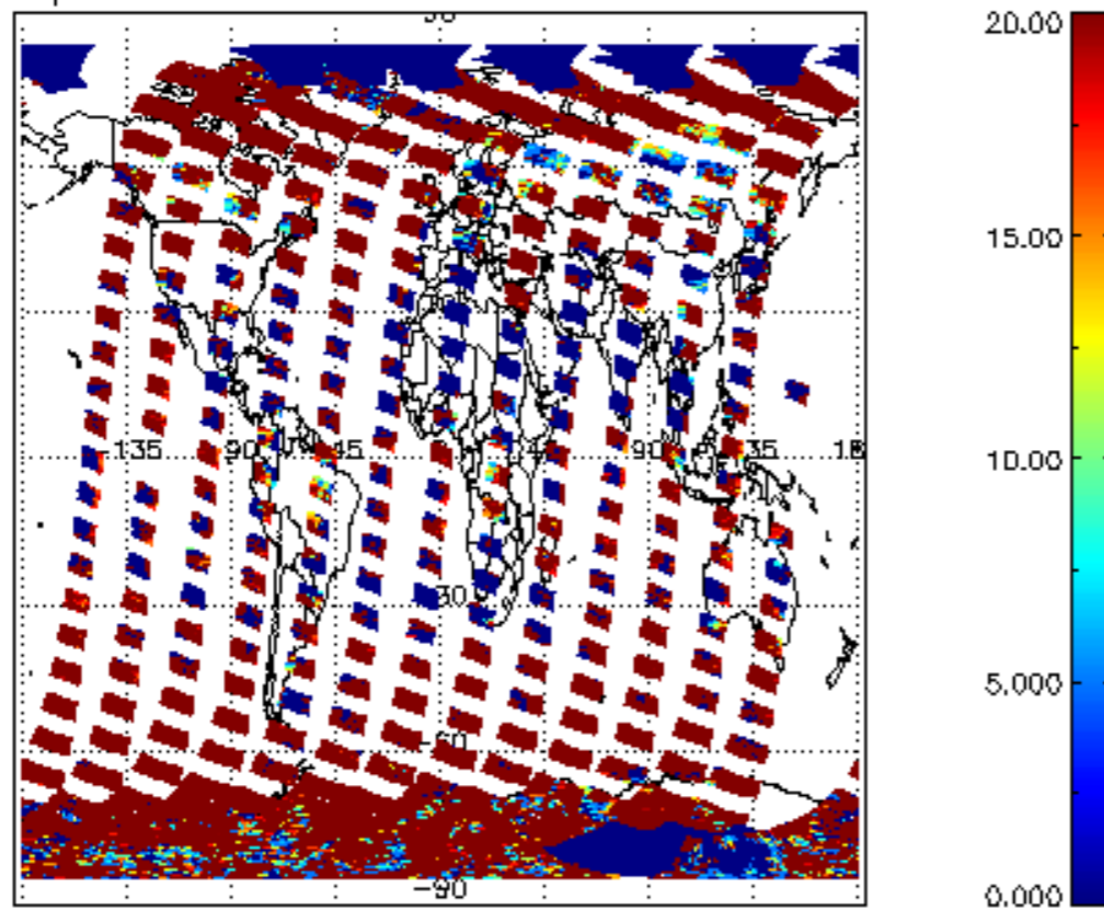
cL_opt_depth for 29FEB2012 00:00:00 to 01MAR2012 00:00:00
