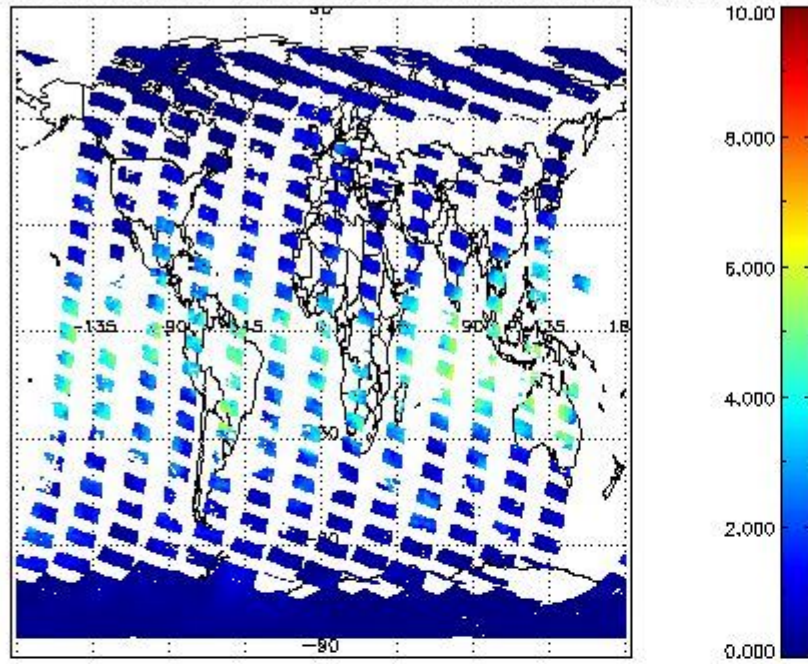
SCIOL2P_NADUV8H2O_vcd for 29FEB2012 00:00:00 to 01MAR2012 00:00:00
