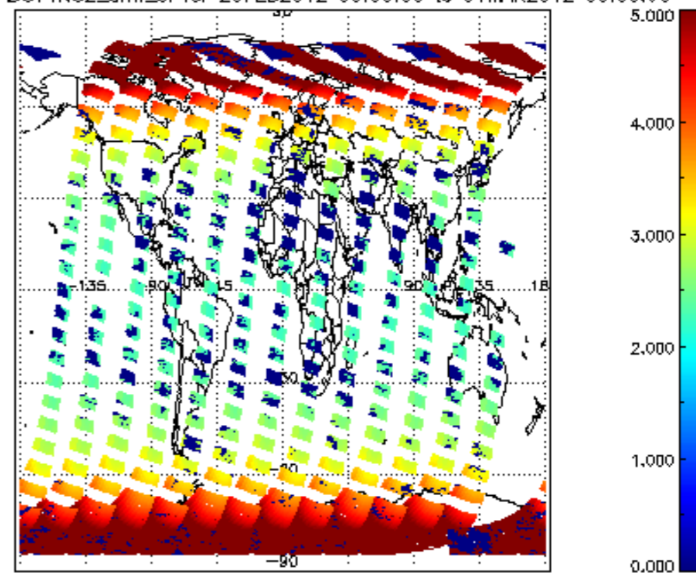
SCIOL2P_NADUV1NO2_amf_cl for 29FEB2012 00:00:00 to 01MAR2012 00:00:00
