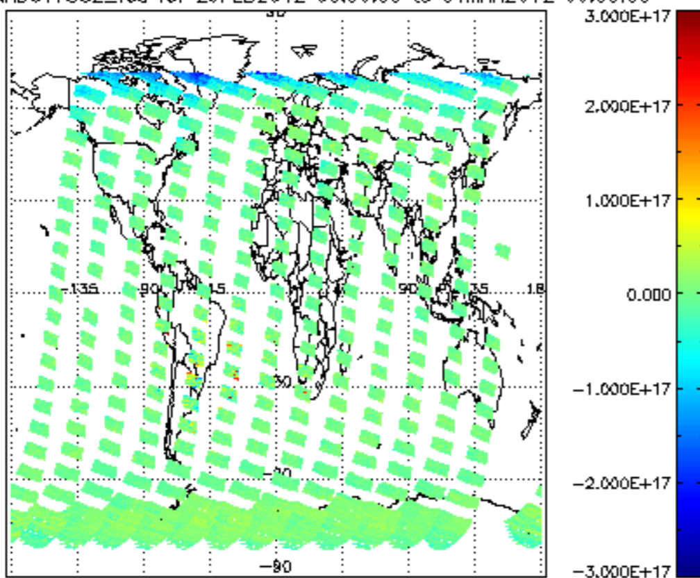
SCIOL2P_NADUV7S02_vcd for 29FEB2012 00:00:00 to 01MAR2012 00:00:00
