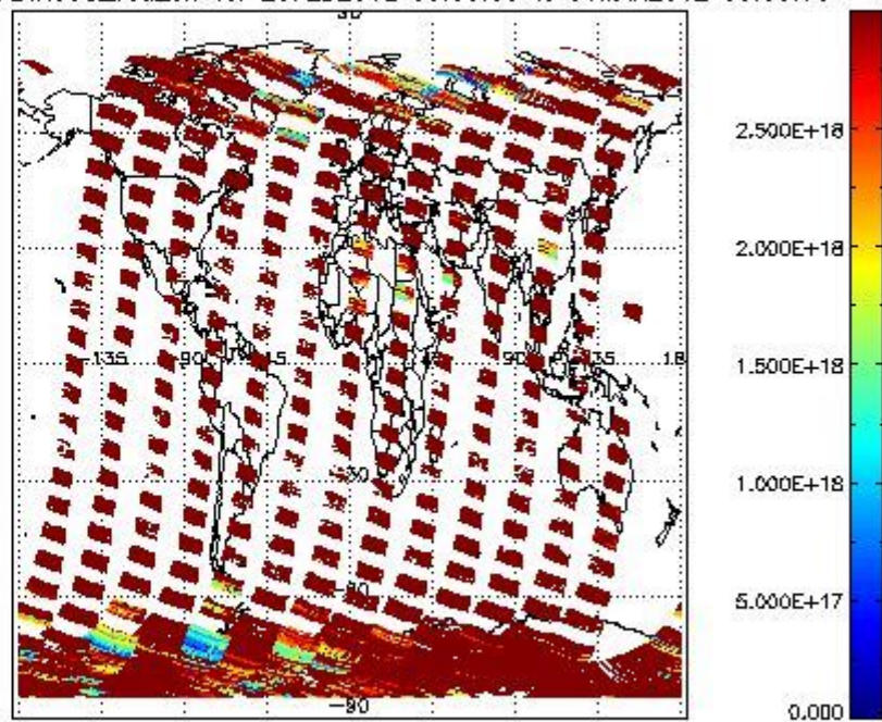
SCIDL2P_NADIR3CO_vcd_err for 29FEB2012 00:00:00 to 01MAR2012 00:00:00
