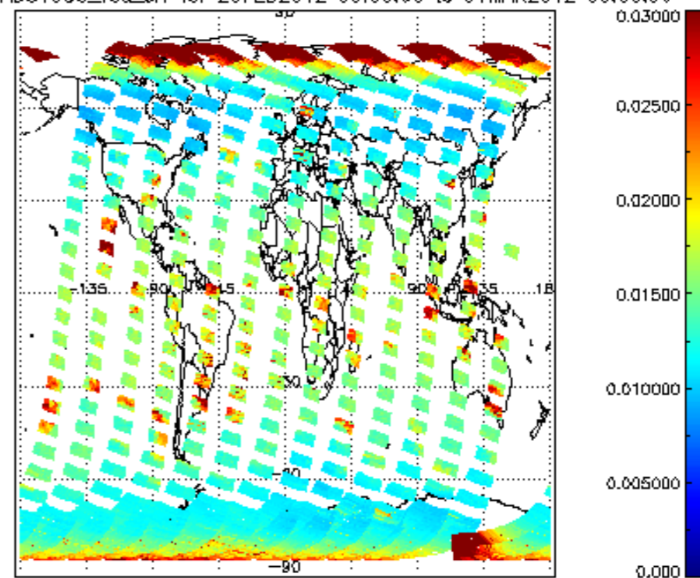
SCIOL2P_NADUV003_vcd_Lerr for 29FEB2012 00:00:00 to 01MAR2012 00:00:00
