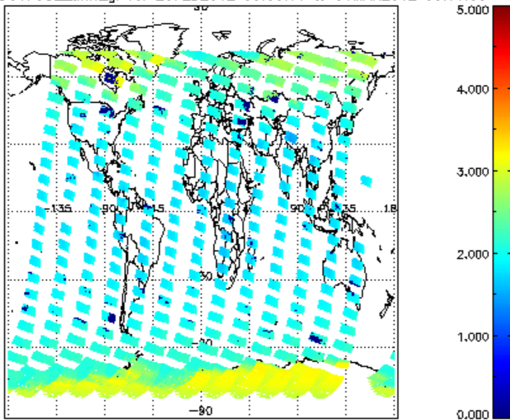
SCIOL2P_NADUV7S02_amf_gr for 29FEB2012 00:00:00 to 01MAR2012 00:00:00
