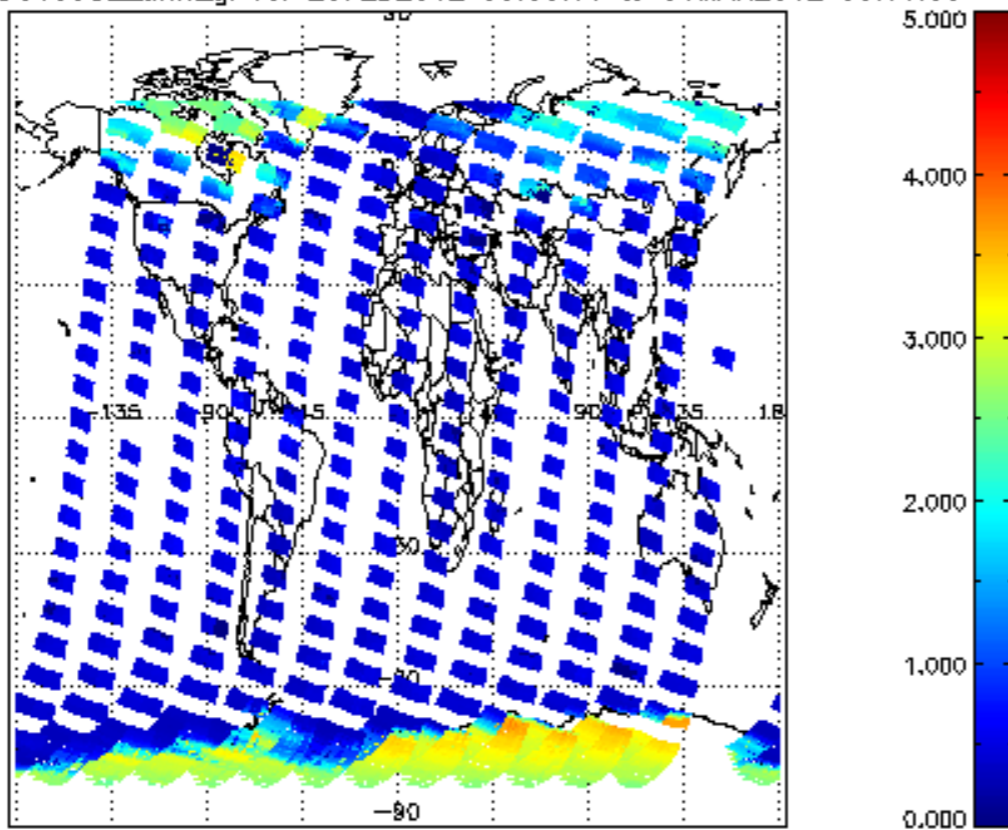
SCIOL2P_NADUV5S02_amf_gr for 29FEB2012 00:00:00 to 01MAR2012 00:00:00
