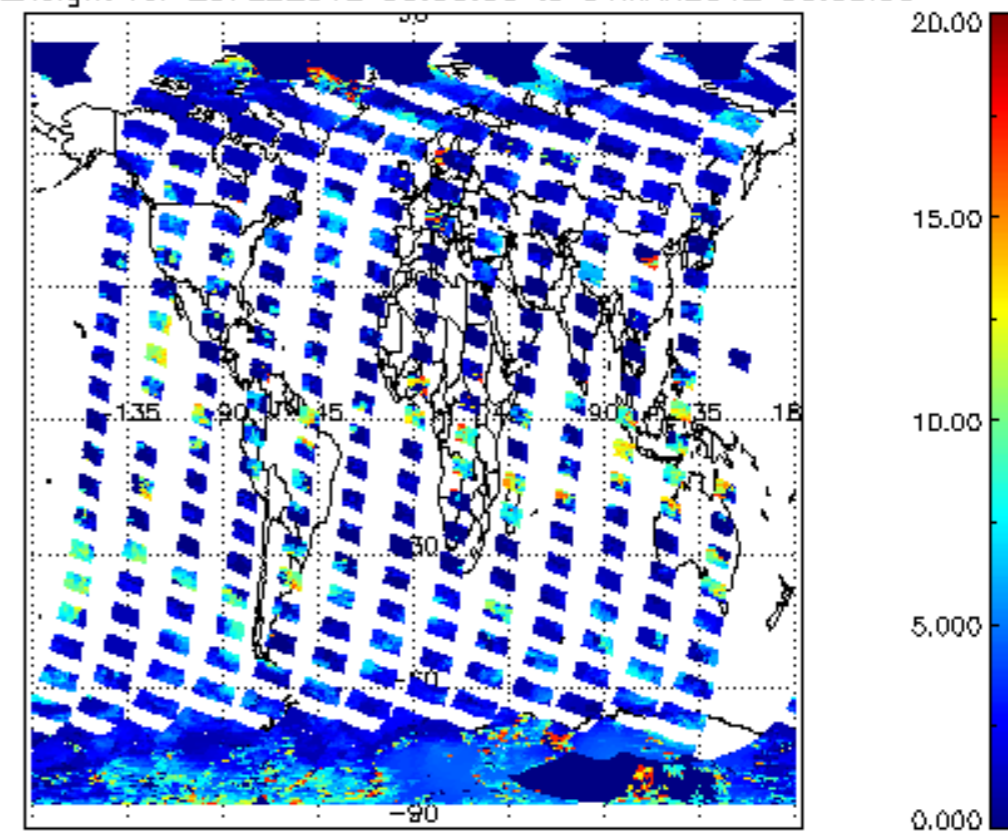
cL_top_height for 29FEB2012 00:00:00 to 01MAR2012 00:00:00
