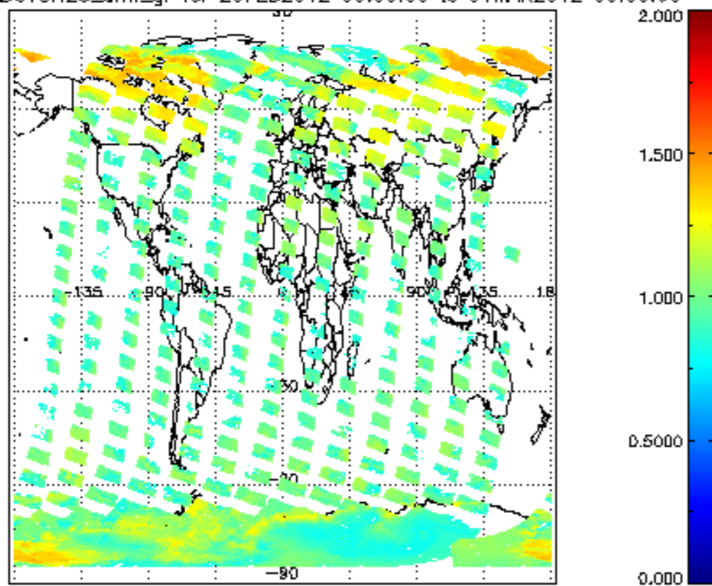
SCIOL2P_NADUV8H2O_amf_gr for 29FEB2012 00:00:00 to 01MAR2012 00:00:00
