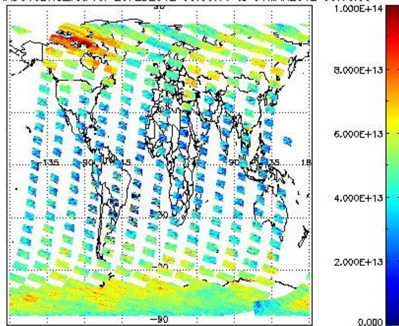
SCIOL2P_NADUV3BRO_vcd for 29FEB2012 00:00:00 to 01MAR2012 00:00:00
