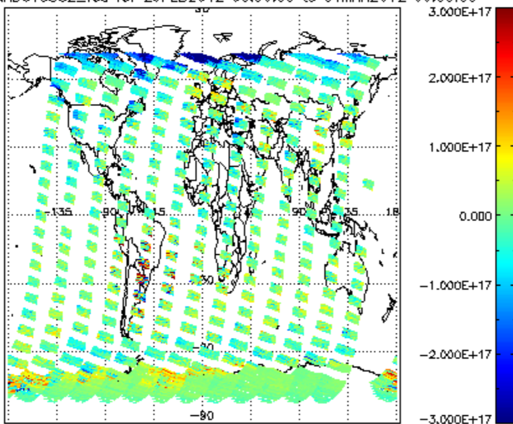
SCIOL2P_NADUV5S02_vcd for 29FEB2012 00:00:00 to 01MAR2012 00:00:00
