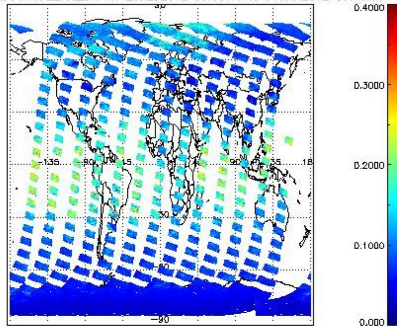
SCIOL2P_NADUV1N02_vcd_err for 29FEB2012 00:00:00 to 01MAR2012 00:00:00
