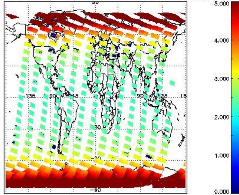
SCIOL2P_NADUV003_amf_gr for 29FEB2012 00:00:00 to 01MAR2012 00:00:00
