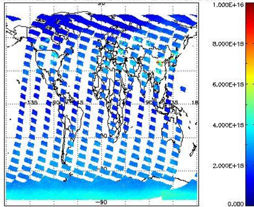
SCIOL2P_NADUV1N02_vcd for 29FEB2012 00:00:00 to 01MAR2012 00:00:00
