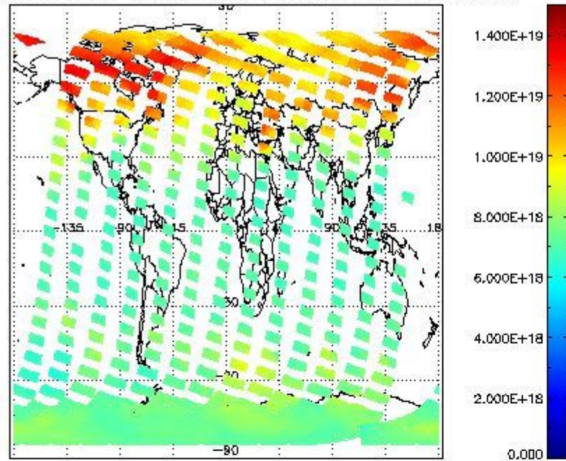
SCIOL2P_NADUV003_vcd for 29FEB2012 00:00:00 to 01MAR2012 00:00:00
