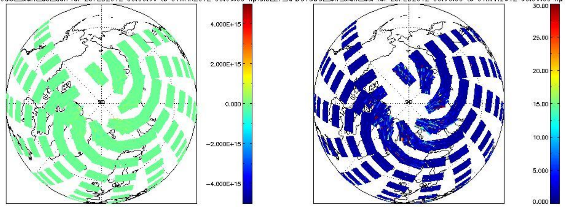
CIOL2P_NADUV60CLslant_col_den for 29FEB2012 00:00:00 to 01MAR2012 00:00:00 np; CIOL2P_NADUV60CLerr_slant_col for 29FEB2012 00:00:00 to 01MAR2012 00:00:00 np
