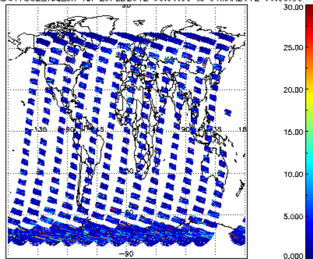
SCIOL2P_NADUV7S02_vcd_err for 29FEB2012 00:00:00 to 01MAR2012 00:00:00
