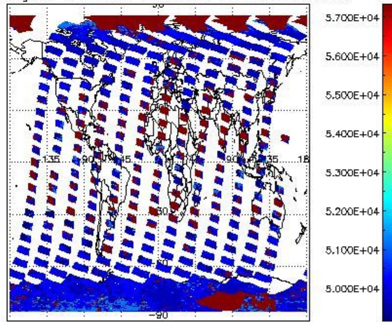
cloud_flags for 29FEB2012 00:00:00 to 01MAR2012 00:00:00
