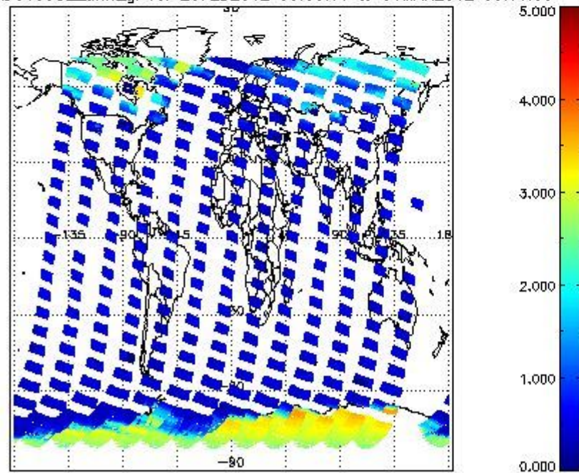
SCIOL2P_NADUV5S02_amf_gr for 29FEB2012 00:00:00 to 01MAR2012 00:00:00
