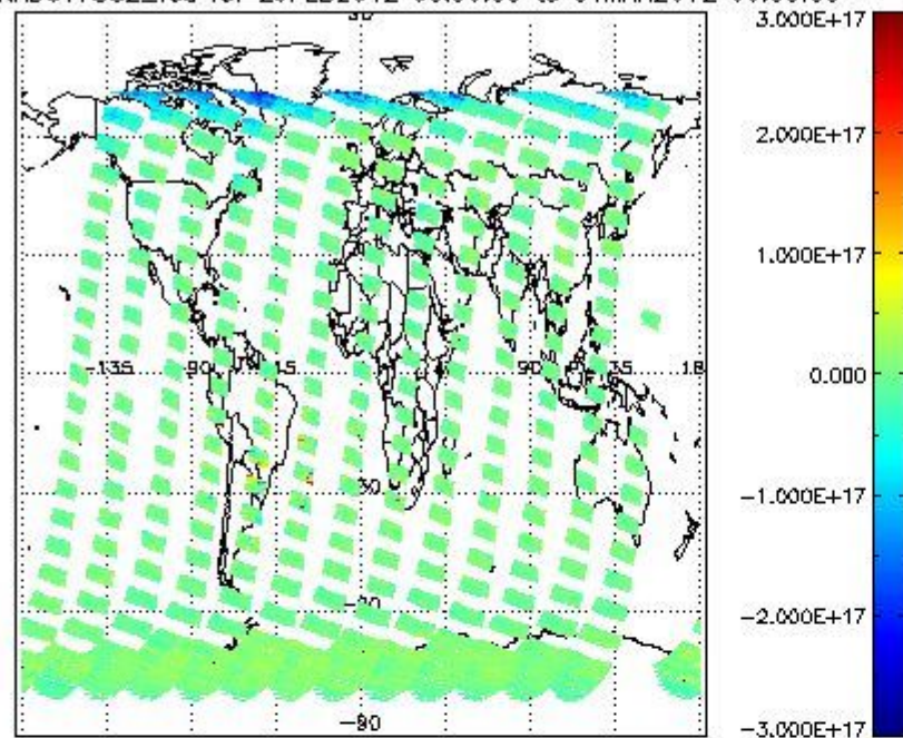
SCIOL2P_NADUV7S02_vcd for 29FEB2012 00:00:00 to 01MAR2012 00:00:00
