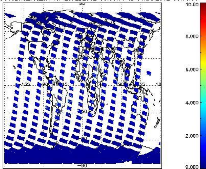
SCIOL2P_NADUV3BRO_vcd_err for 29FEB2012 00:00:00 to 01MAR2012 00:00:00
