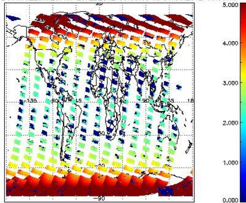
SCIOL2P_NADUV1N02_amf_cl for 29FEB2012 00:00:00 to 01MAR2012 00:00:00
