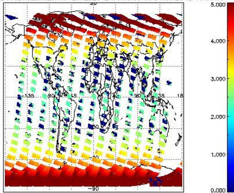
SCIOL2P_NADUV3BRO_amf_cl for 29FEB2012 00:00:00 to 01MAR2012 00:00:00
