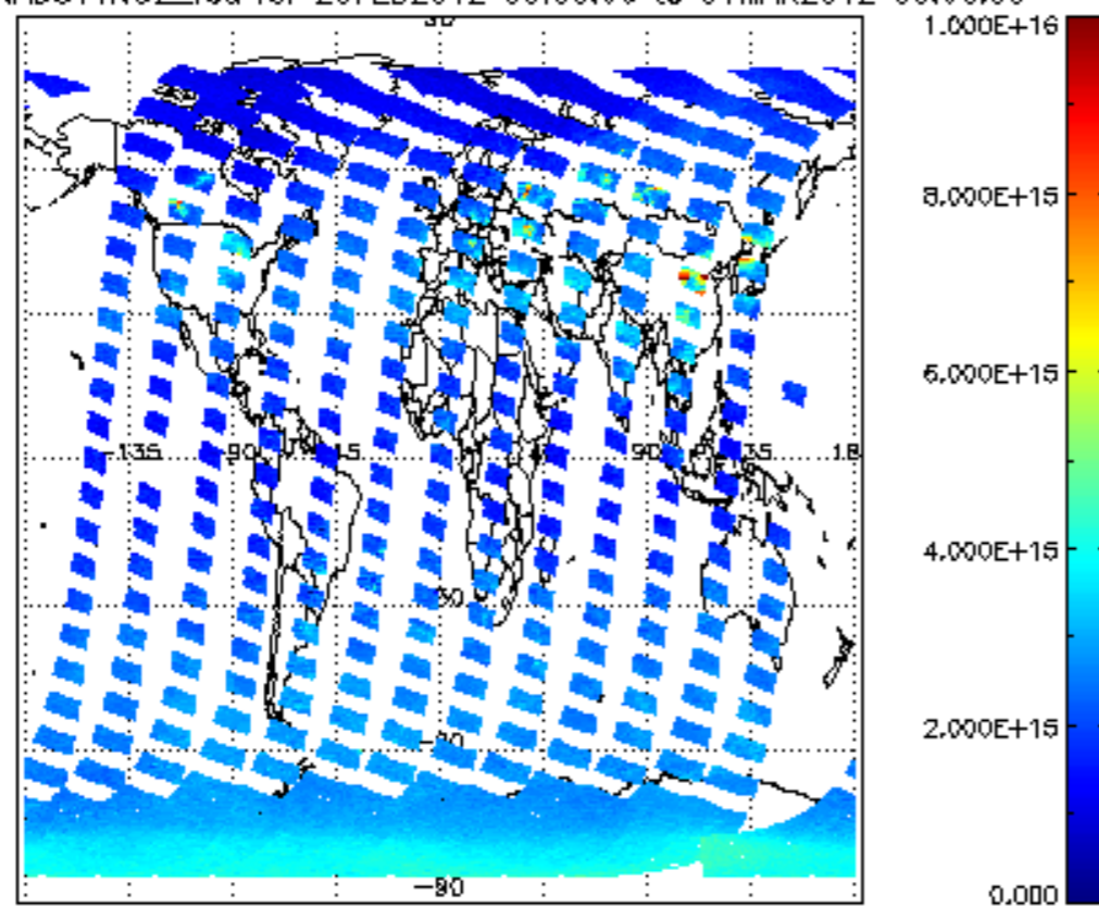
SCIOL2P_NADUV1NO2_vcd for 29FEB2012 00:00:00 to 01MAR2012 00:00:00
