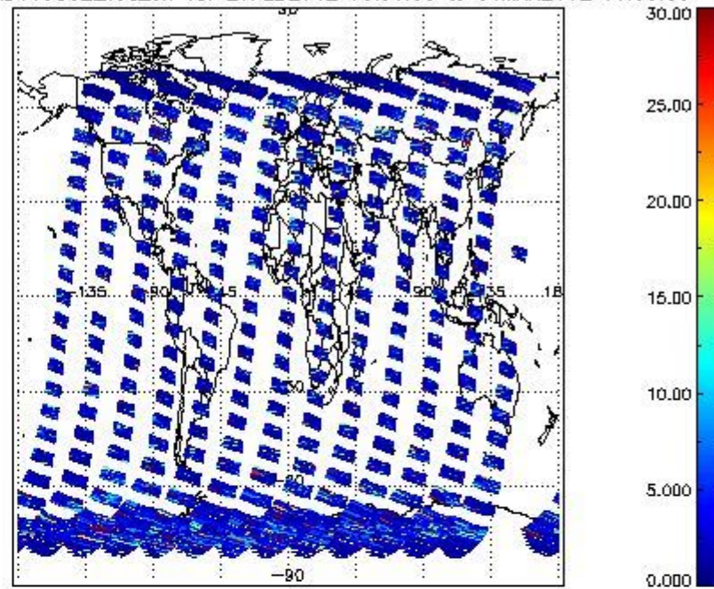
SCIOL2P_NADUV5S02_vcd_err for 29FEB2012 00:00:00 to 01MAR2012 00:00:00
