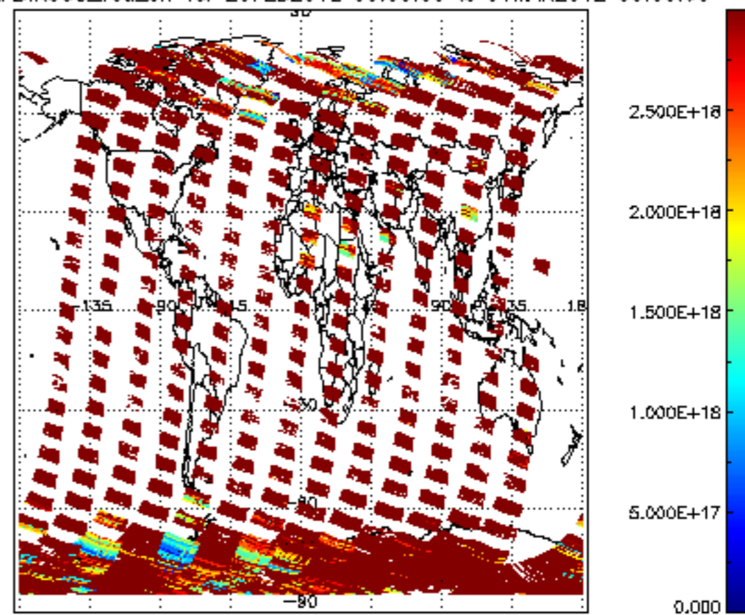
SCIOL2P_NADIR3CO_vcd_err for 29FEB2012 00:00:00 to 01MAR2012 00:00:00
