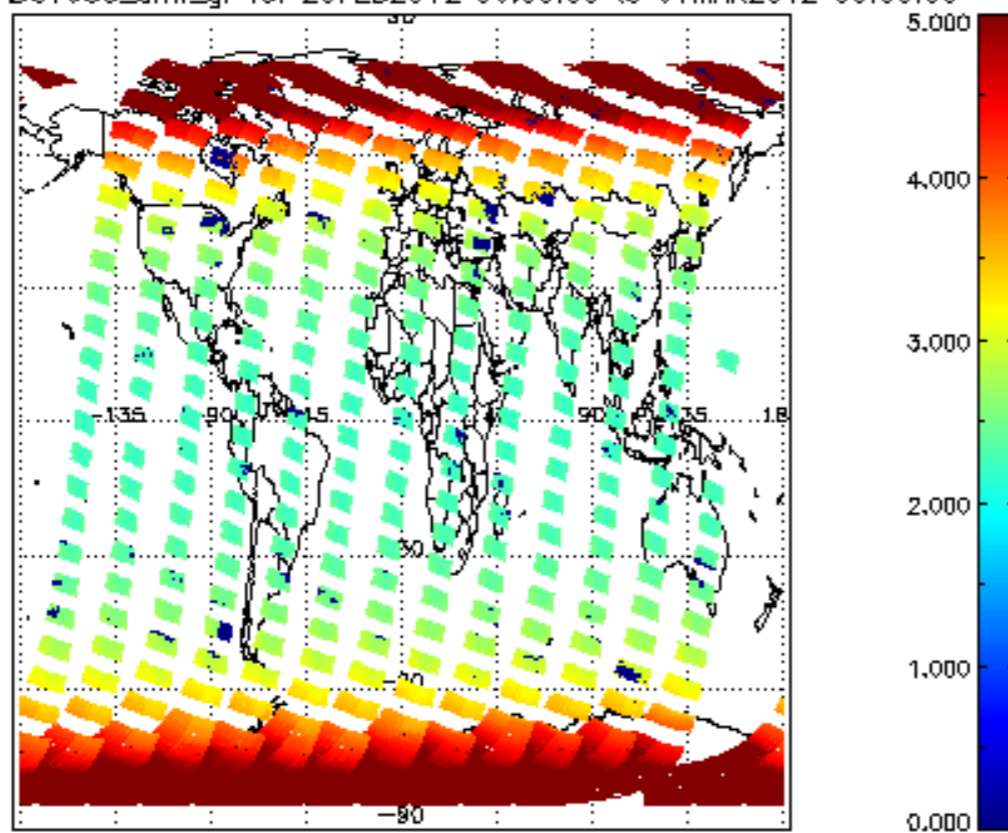
SCIOL2P_NADUV003_amf_gr for 29FEB2012 00:00:00 to 01MAR2012 00:00:00
