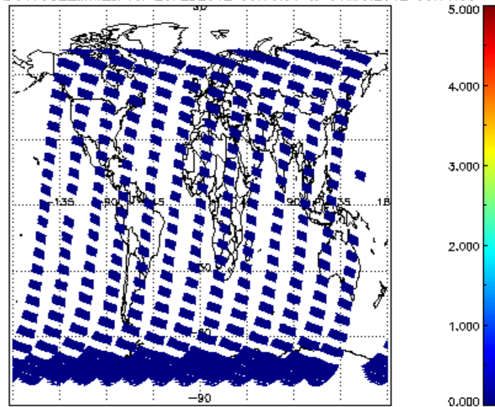
SCIOL2P_NADUV7S02_amf_cl for 29FEB2012 00:00:00 to 01MAR2012 00:00:00
