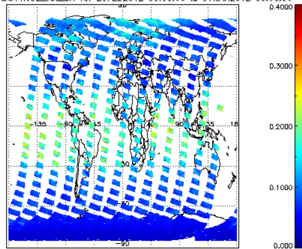
SCIOL2P_NADUV1NO2_vcd_err for 29FEB2012 00:00:00 to 01MAR2012 00:00:00
