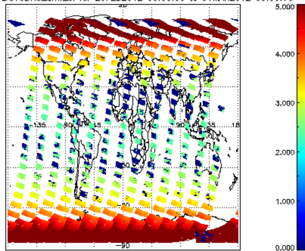
SCIOL2P_NADUV3BRO_amf_cl for 29FEB2012 00:00:00 to 01MAR2012 00:00:00
