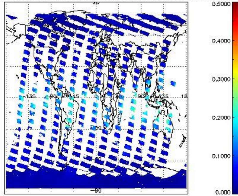
SCIOL2P_NADUV8H2O_vcd_err for 29FEB2012 00:00:00 to 01MAR2012 00:00:00
