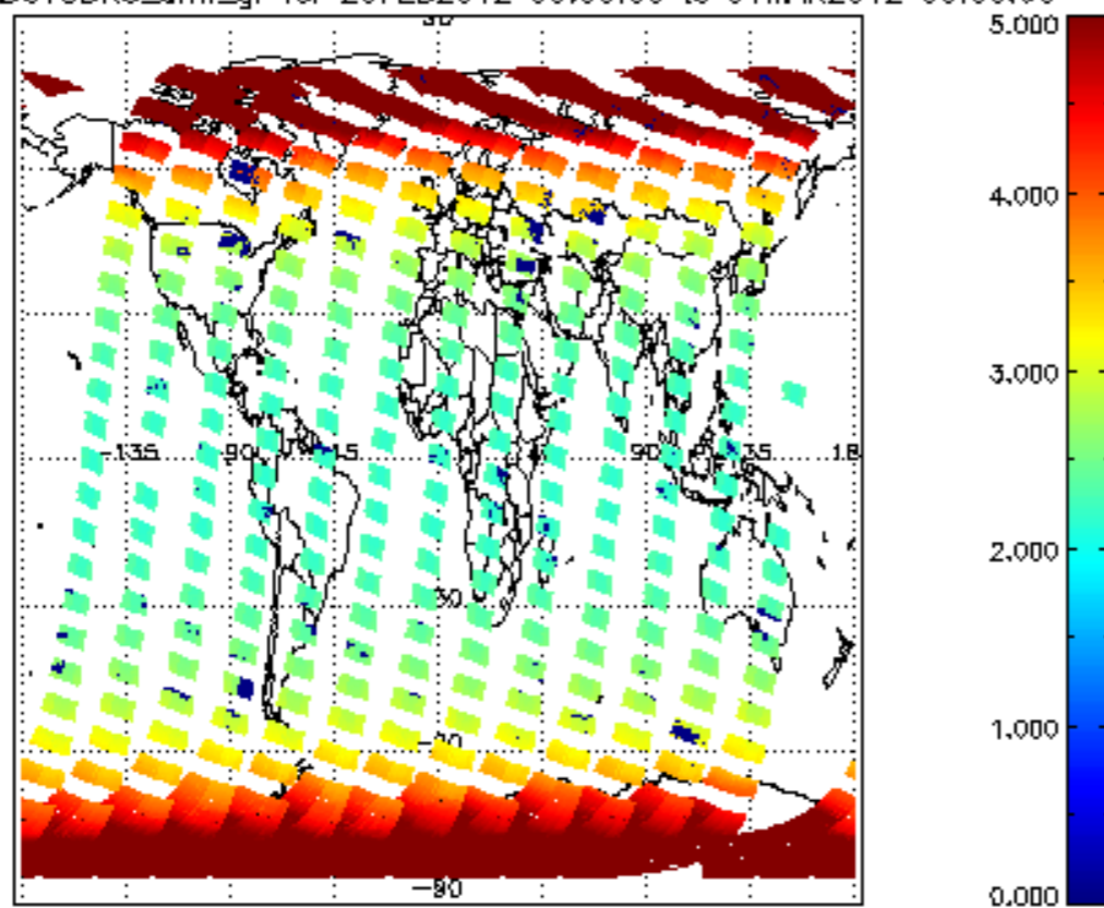
SCIOL2P_NADUV3BRO_amf_gr for 29FEB2012 00:00:00 to 01MAR2012 00:00:00
