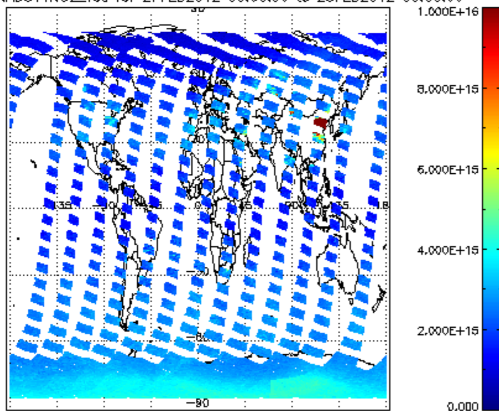
SCIOL2P_NADUV1N02_vcd for 27FEB2012 00:00:00 to 28FEB2012 00:00:00
