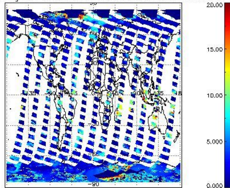
cL_top_height for 27FEB2012 00:00:00 to 28FEB2012 00:00:00
