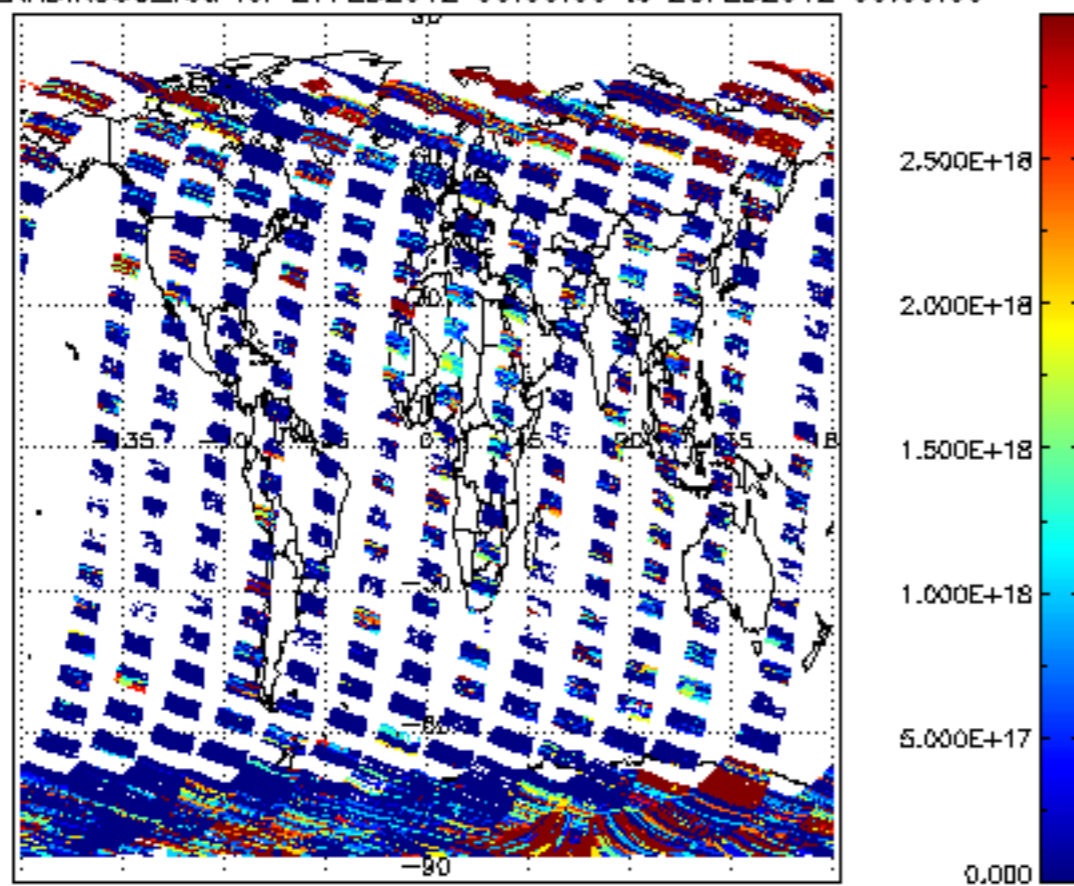
SCIOL2P_NADIR3CO_vcd for 27FEB2012 00:00:00 to 28FEB2012 00:00:00
