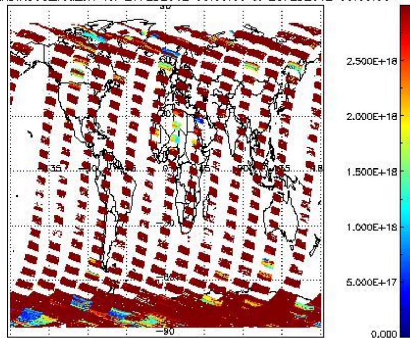
SCIDL2P_NADIR3CO_vcd_err for 27FEB2012 00:00:00 to 28FEB2012 00:00:00
