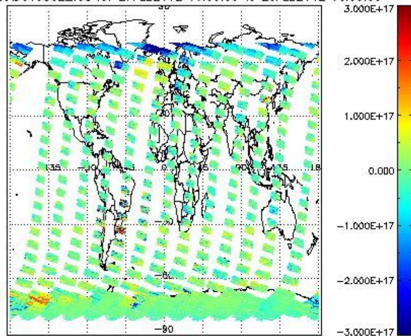
SCIOL2P_NADUV5SO2_vcd for 27FEB2012 00:00:00 to 28FEB2012 00:00:00
