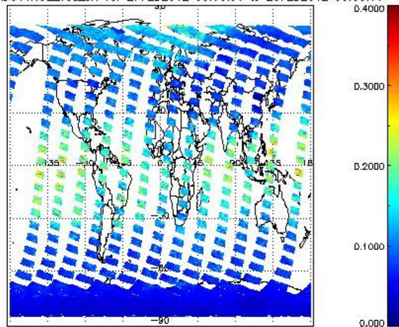
SCIOL2P_NADUV1N02_vcd_err for 27FEB2012 00:00:00 to 28FEB2012 00:00:00
