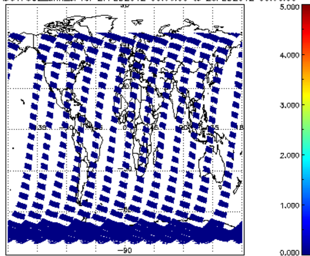
SCIOL2P_NADUV7S02_amf_cl for 27FEB2012 00:00:00 to 28FEB2012 00:00:00
