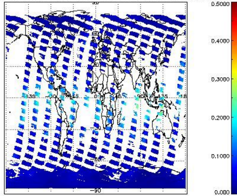
SCIOL2P_NADUV8H2O_vcd_err for 27FEB2012 00:00:00 to 28FEB2012 00:00:00
