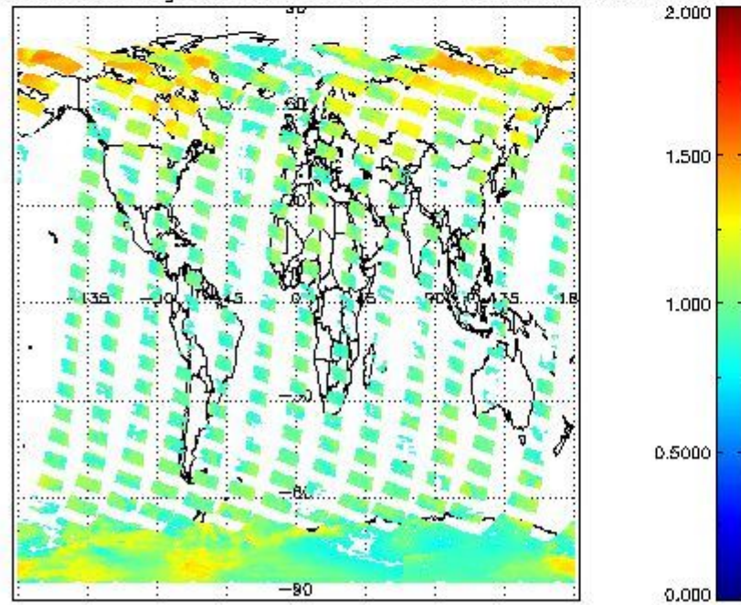
SCIOL2P_NADUV8H2O_amf_gr for 27FEB2012 00:00:00 to 28FEB2012 00:00:00
