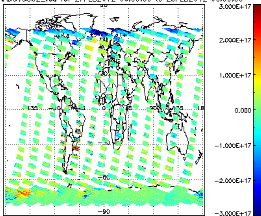
SCIOL2P_NADUV5S02_vcd for 27FEB2012 00:00:00 to 28FEB2012 00:00:00
