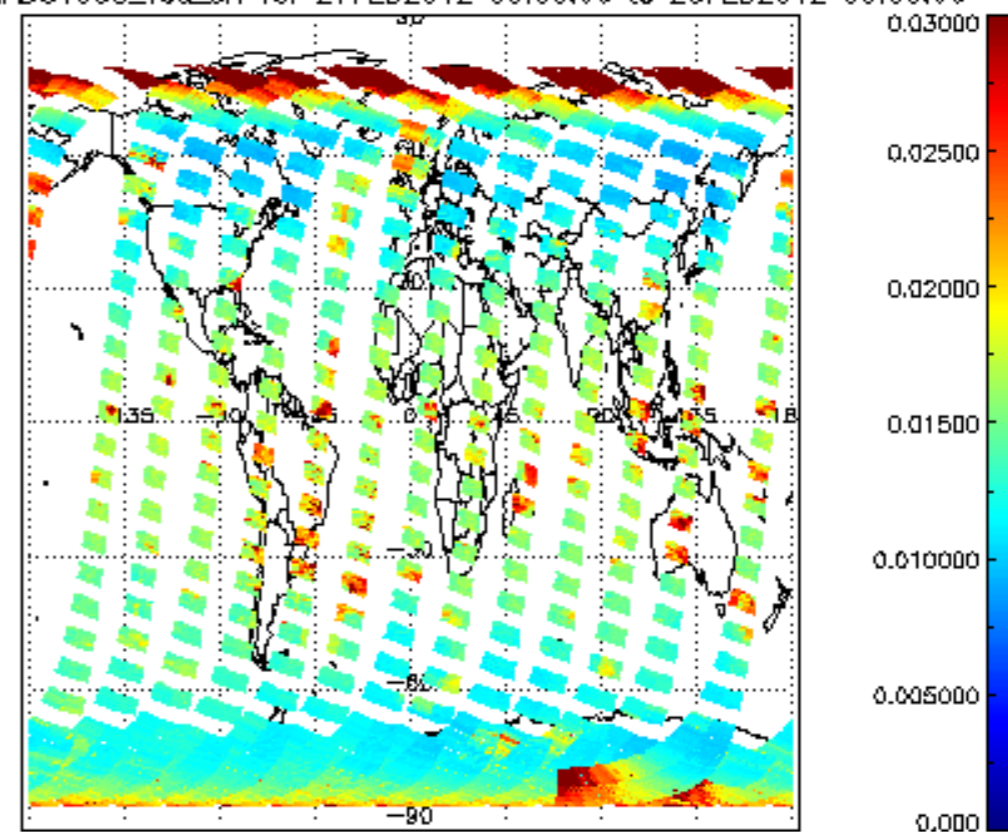
SCIOL2P_NADUV003_vcd_err for 27FEB2012 00:00:00 to 28FEB2012 00:00:00
