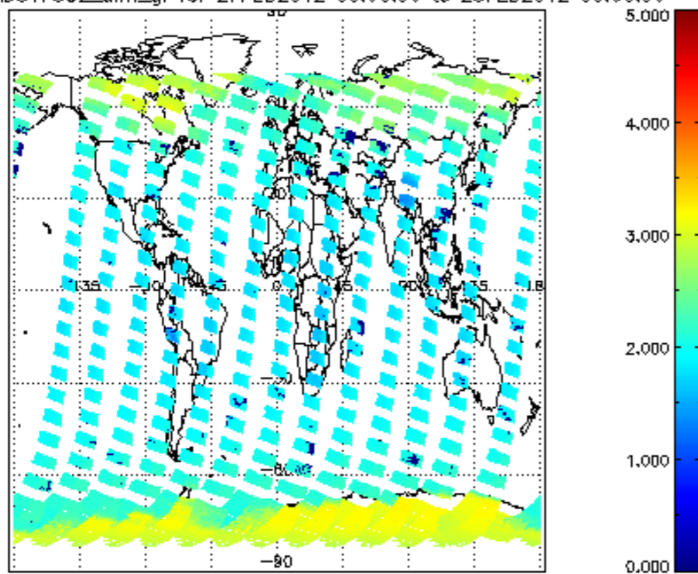
SCIOL2P_NADUV7S02_amf_gr for 27FEB2012 00:00:00 to 28FEB2012 00:00:00
