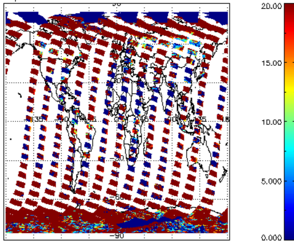
cl_opt_depth for 27FEB2012 00:00:00 to 28FEB2012 00:00:00
