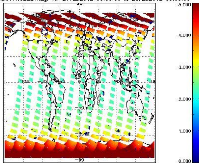
SCIOL2P_NADUV1N02_amf_gr for 27FEB2012 00:00:00 to 28FEB2012 00:00:00
