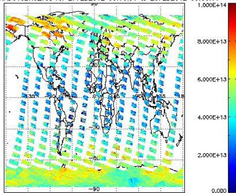
SCIOL2P_NADUV3BRO_vcd for 27FEB2012 00:00:00 to 28FEB2012 00:00:00
