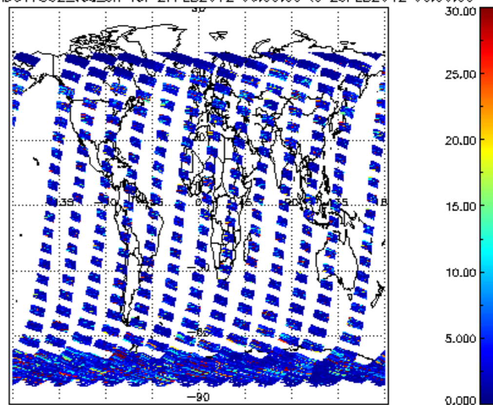
SCIOL2P_NADUV7S02_vcd_err for 27FEB2012 00:00:00 to 28FEB2012 00:00:00
