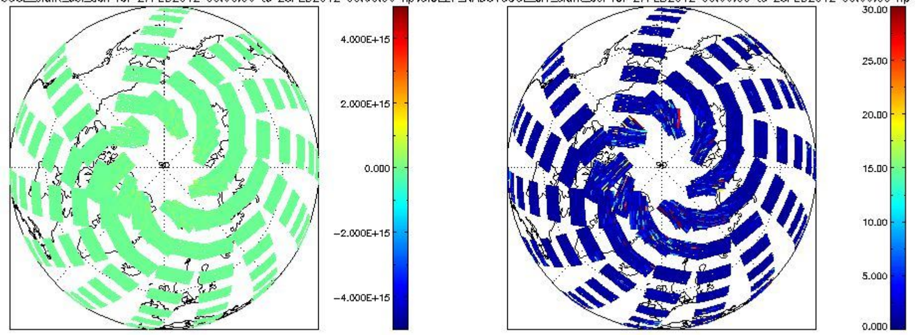
CIOL2P_NADUV6OCL_slant_col_den for 27FEB2012 00:00:00 to 28FEB2012 00:00:00 np; CIOL2P_NADUV6OCL_err_slant_col for 27FEB2012 00:00:00 to 28FEB2012 00:00:00 np
