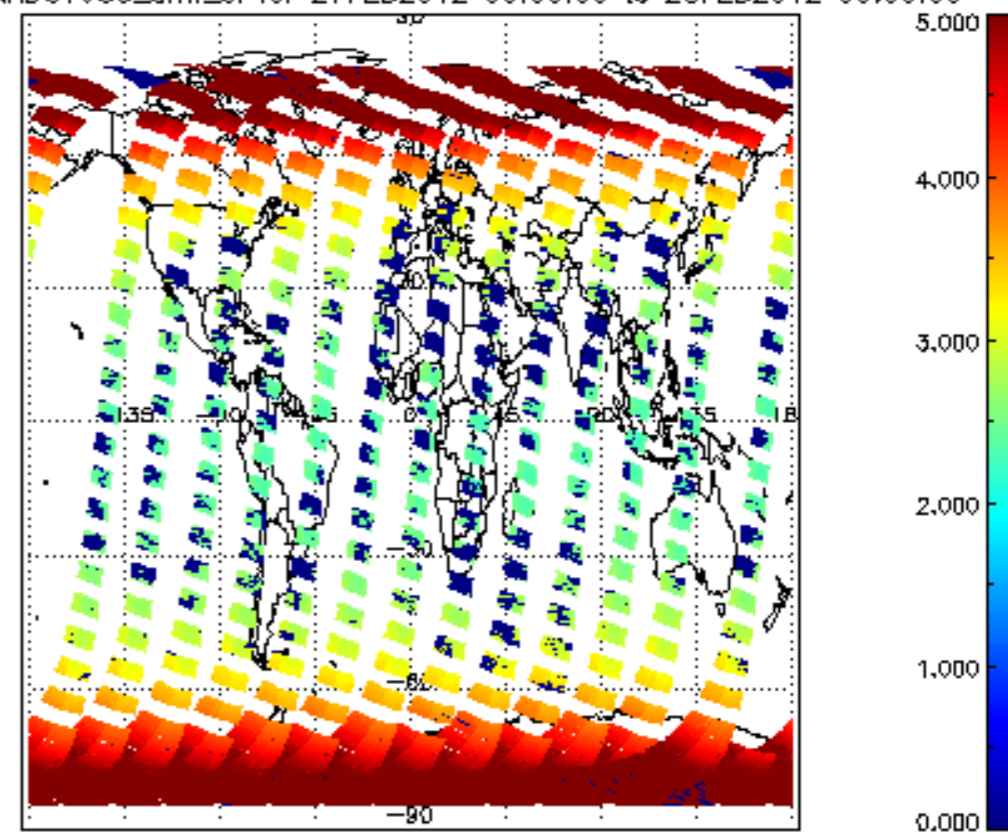
SCIOL2P_NADUV003_amf_cl for 27FEB2012 00:00:00 to 28FEB2012 00:00:00
