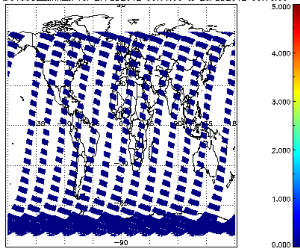
SCIOL2P_NADUV5S02_amf_cl for 27FEB2012 00:00:00 to 28FEB2012 00:00:00
