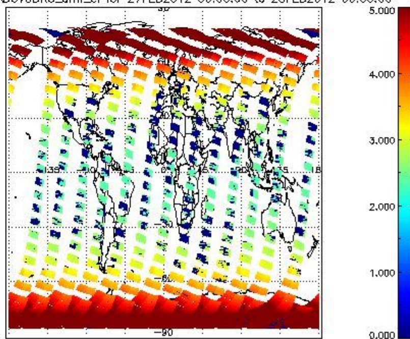
SCIOL2P_NADUV3BRO_amf_cl for 27FEB2012 00:00:00 to 28FEB2012 00:00:00
