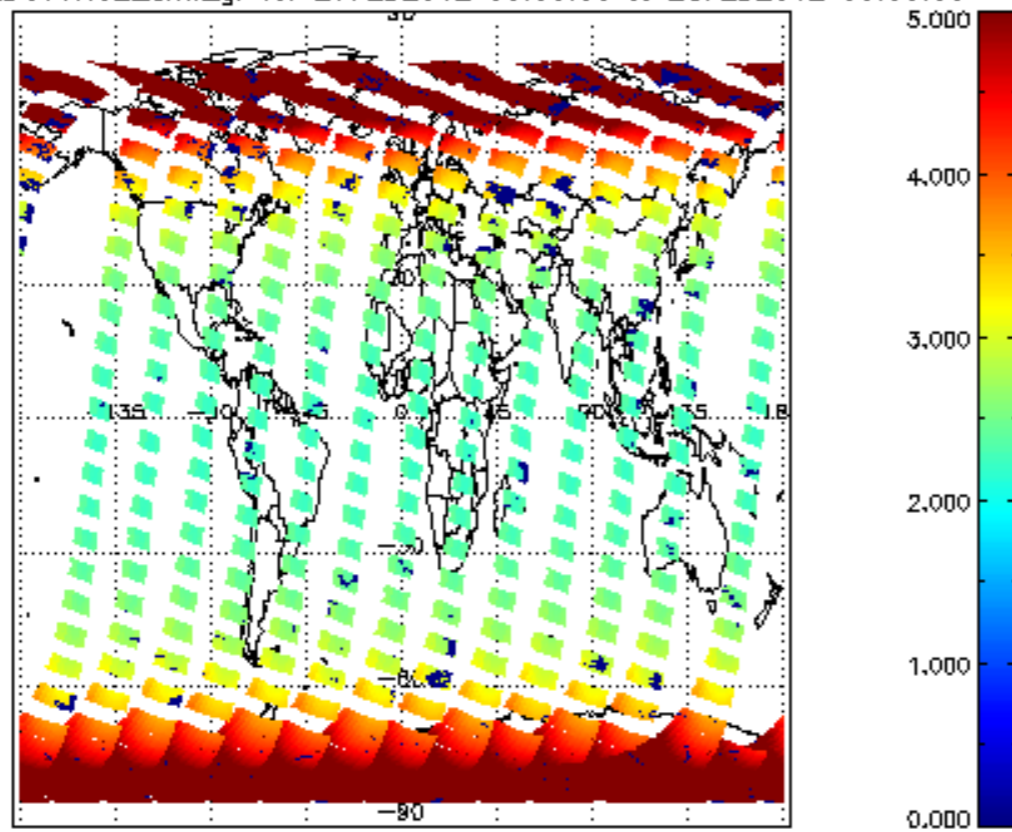
SCIOL2P_NADUV1N02_amf_gr for 27FEB2012 00:00:00 to 28FEB2012 00:00:00
