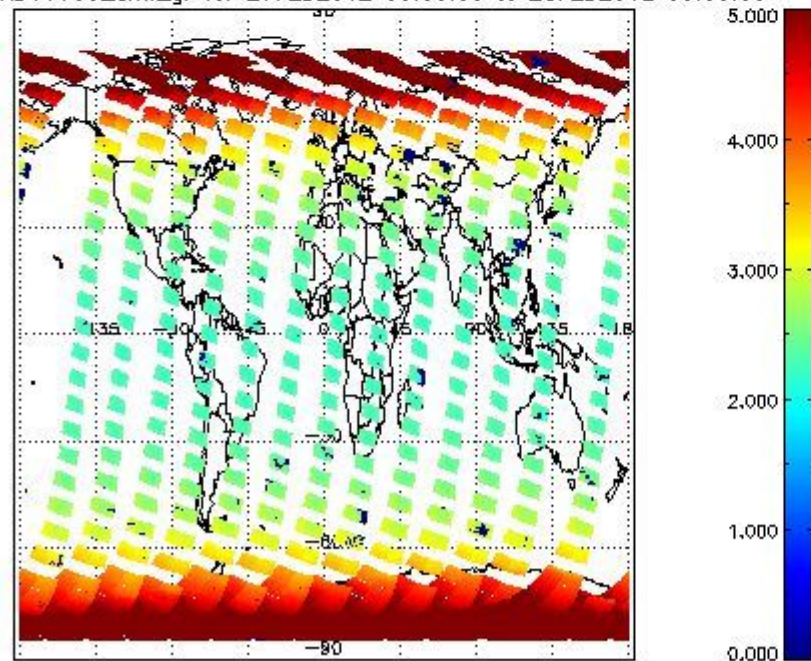
SCIOL2P_NADUV003_amf_gr for 27FEB2012 00:00:00 to 28FEB2012 00:00:00
