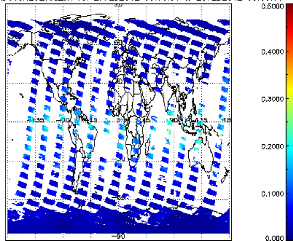
SCIOL2P_NADUV8H20_vcd_err for 27FEB2012 00:00:00 to 28FEB2012 00:00:00
