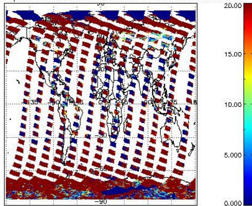
cL_opt_depth for 27FEB2012 00:00:00 to 28FEB2012 00:00:00
