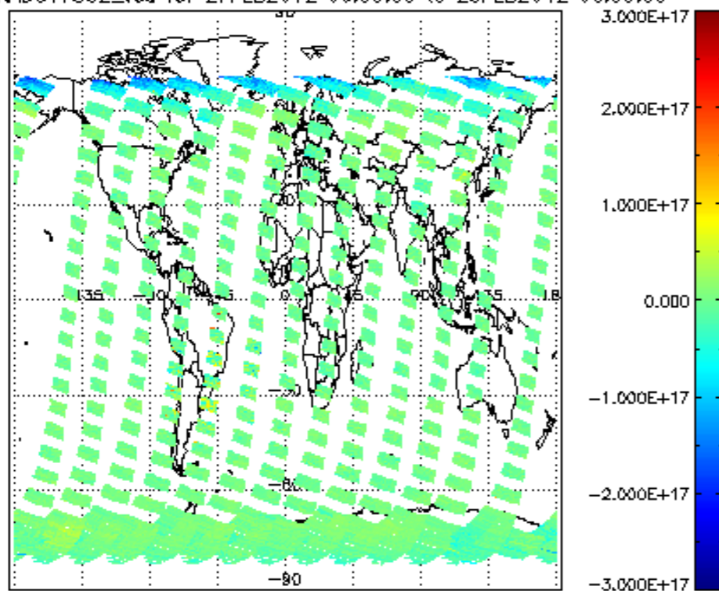
SCIOL2P_NADUV7S02_vcd for 27FEB2012 00:00:00 to 28FEB2012 00:00:00
