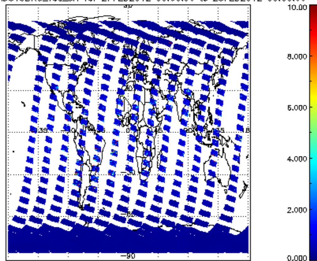
SCIOL2P_NADUV3BRO_vcd_err for 27FEB2012 00:00:00 to 28FEB2012 00:00:00
