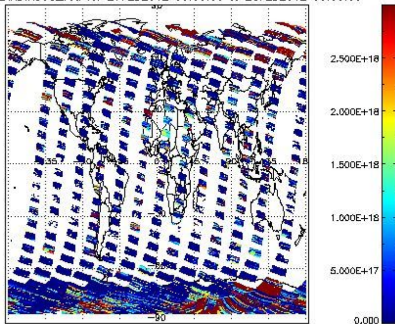
SCIDL2P_NADIR3CO_vcd for 27FEB2012 00:00:00 to 28FEB2012 00:00:00
