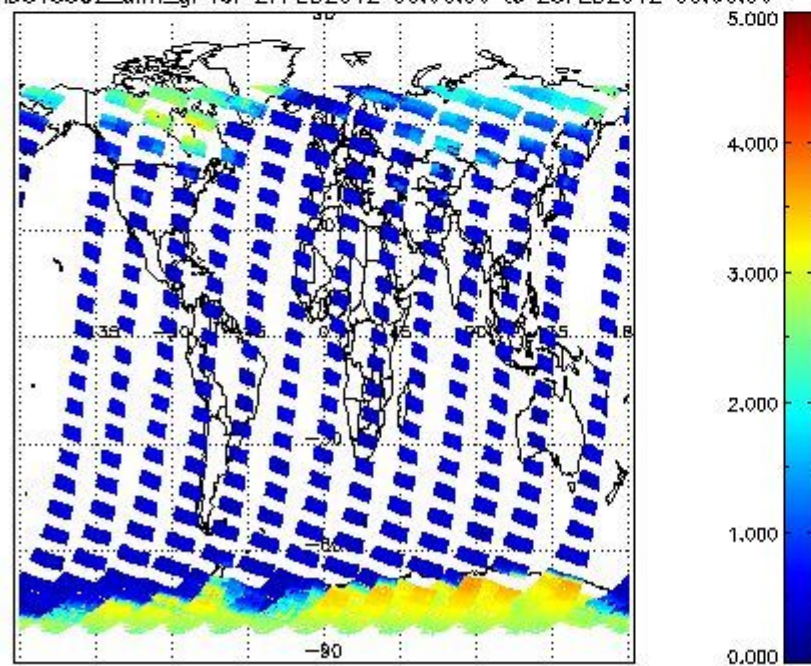
SCIOL2P_NADUV5SO2_amf_gr for 27FEB2012 00:00:00 to 28FEB2012 00:00:00
