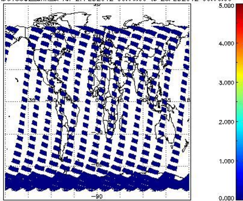
SCIOL2P_NADUV5SO2_amf_cl for 27FEB2012 00:00:00 to 28FEB2012 00:00:00
