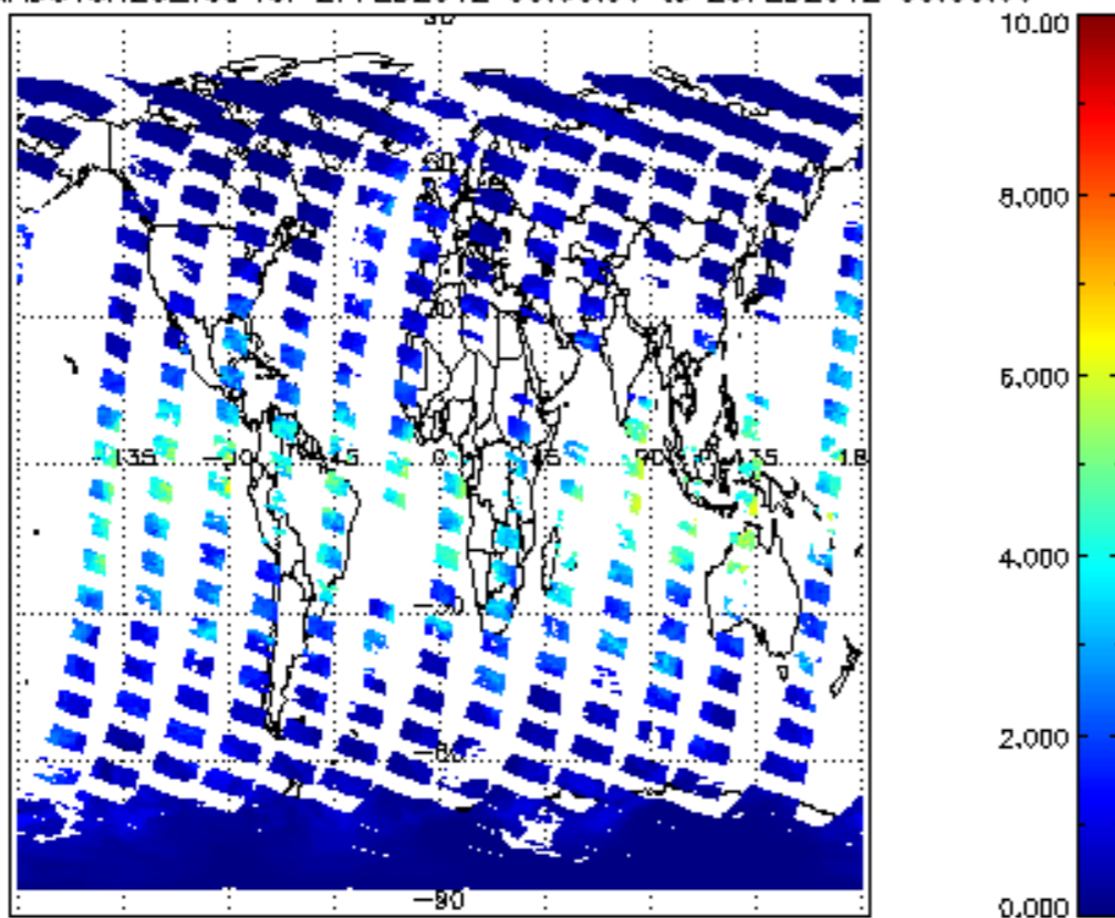
SCIOL2P_NADUV8H20_vcd for 27FEB2012 00:00:00 to 28FEB2012 00:00:00
