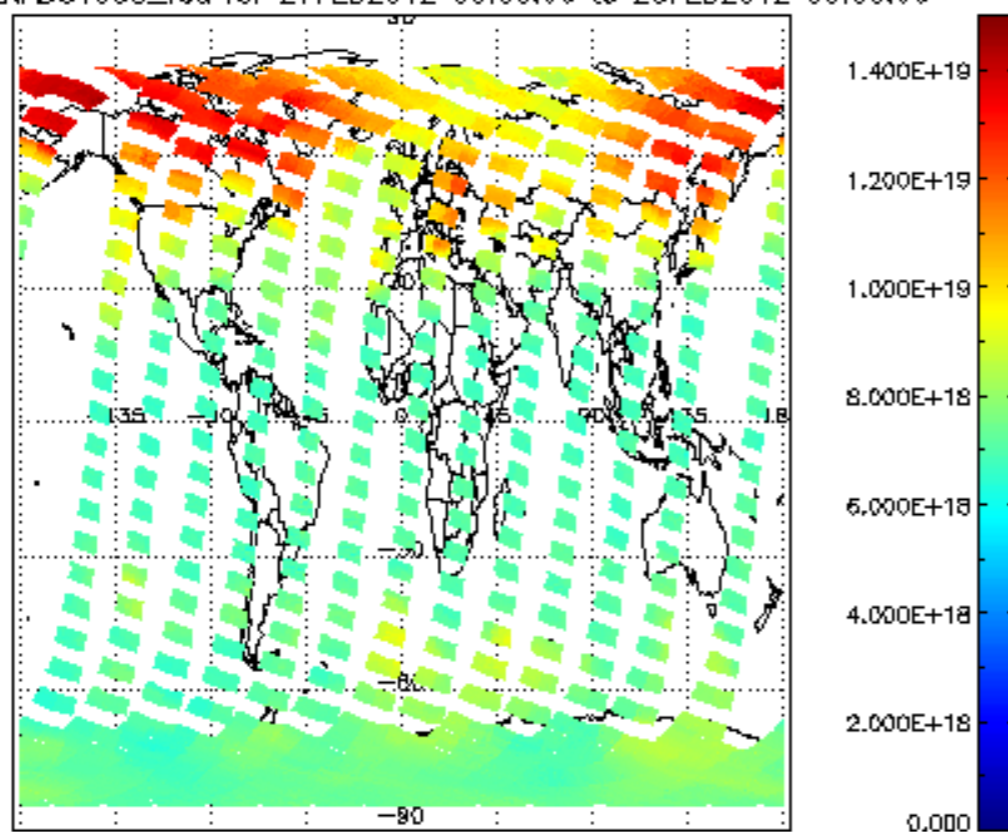
SCIOL2P_NADUV003_vcd for 27FEB2012 00:00:00 to 28FEB2012 00:00:00
