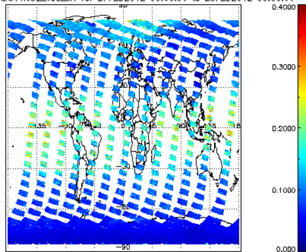
SCIOL2P_NADUV1N02_vcd_err for 27FEB2012 00:00:00 to 28FEB2012 00:00:00
