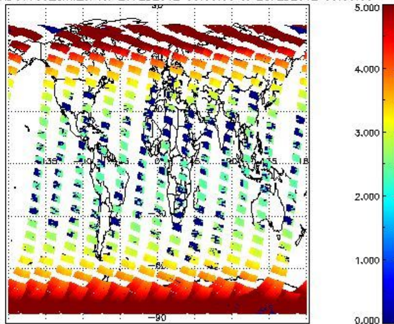
SCIOL2P_NADUV003_amf_cl for 27FEB2012 00:00:00 to 28FEB2012 00:00:00
