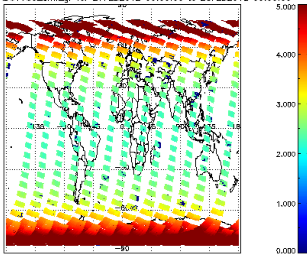
SCIOL2P_NADUV003_amf_gr for 27FEB2012 00:00:00 to 28FEB2012 00:00:00
