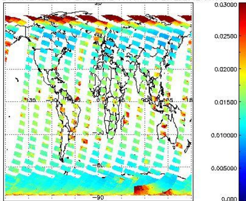
SCIOL2P_NADUV003_vcd_err for 27FEB2012 00:00:00 to 28FEB2012 00:00:00
