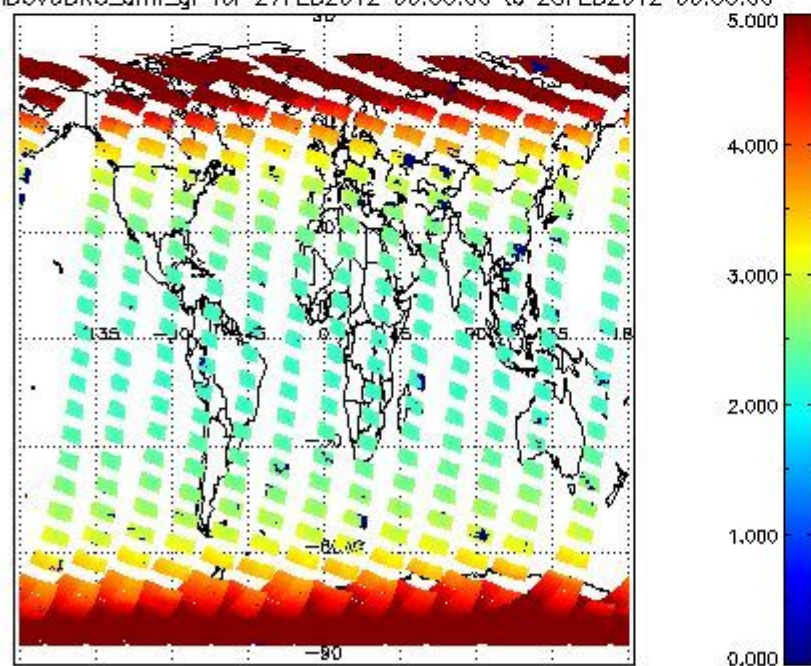
SCIOL2P_NADUV3BRO_amf_gr for 27FEB2012 00:00:00 to 28FEB2012 00:00:00
