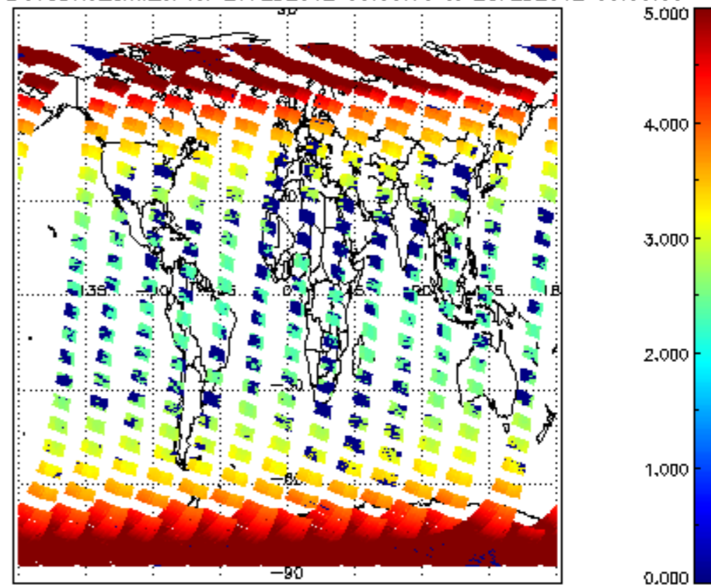
SCIOL2P_NADUV3BRO_amf_cl for 27FEB2012 00:00:00 to 28FEB2012 00:00:00
