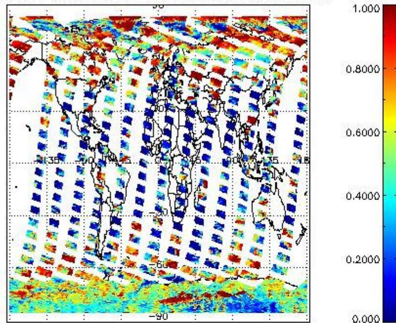
cL_frac for 27FEB2012 00:00:00 to 28FEB2012 00:00:00
