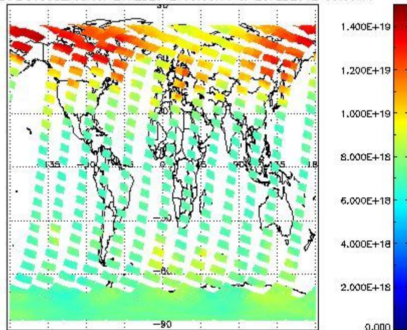
SCIOL2P_NADUV003_vcd for 27FEB2012 00:00:00 to 28FEB2012 00:00:00
