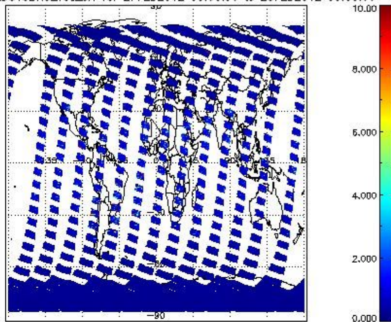
SCIOL2P_NADUV3BRO_vcd_err for 27FEB2012 00:00:00 to 28FEB2012 00:00:00
