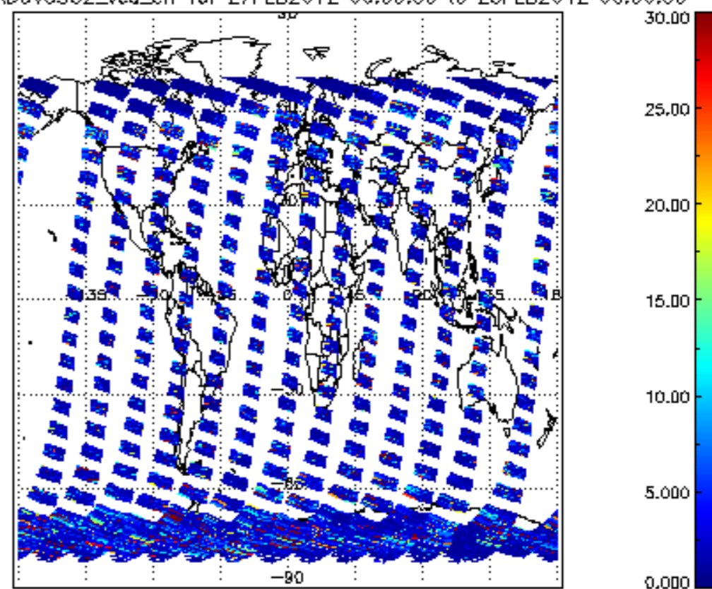
SCIOL2P_NADUV5S02_vcd_err for 27FEB2012 00:00:00 to 28FEB2012 00:00:00
