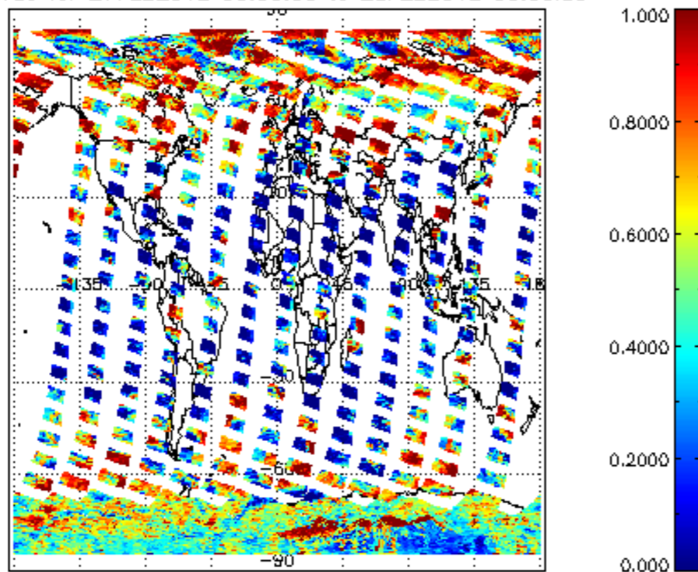
cl_frac for 27FEB2012 00:00:00 to 28FEB2012 00:00:00
