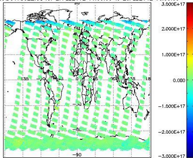
SCIOL2P_NADUV7S02_vcd for 27FEB2012 00:00:00 to 28FEB2012 00:00:00
