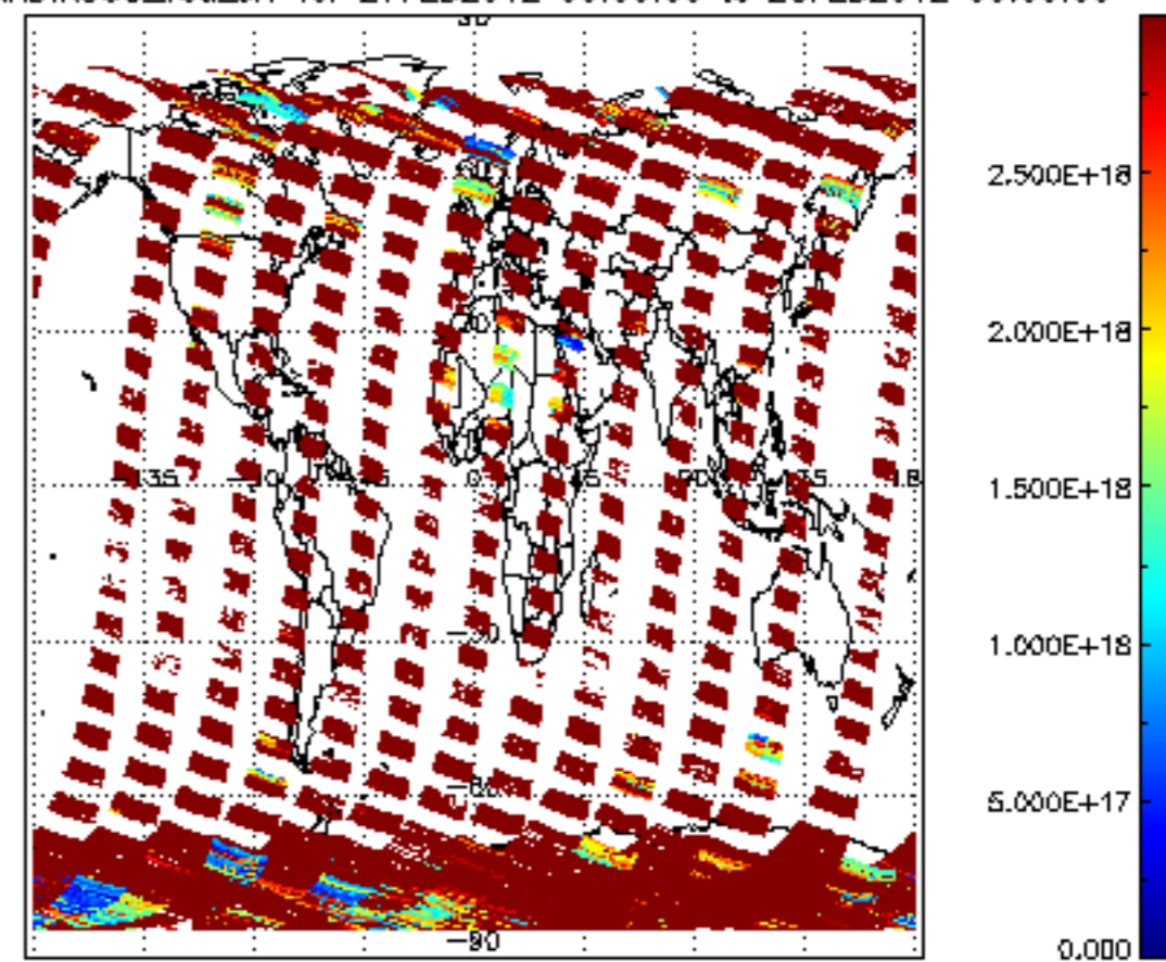
SCIOL2P_NADIR3CO_vcd_err for 27FEB2012 00:00:00 to 28FEB2012 00:00:00
