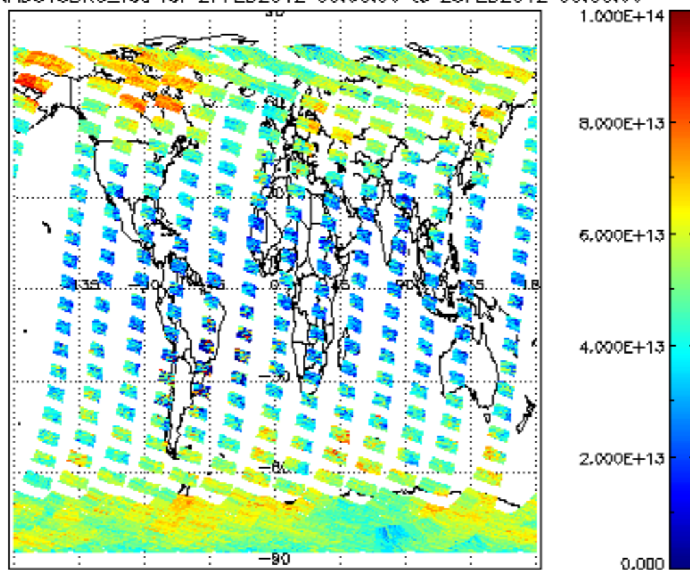
SCIOL2P_NADUV3BRO_vcd for 27FEB2012 00:00:00 to 28FEB2012 00:00:00
