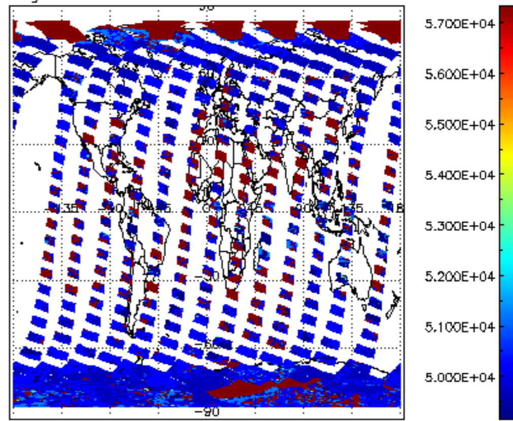
cloud_flags for 27FEB2012 00:00:00 to 28FEB2012 00:00:00
