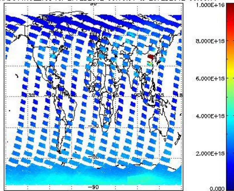
SCIOL2P_NADUV1N02_vcd for 27FEB2012 00:00:00 to 28FEB2012 00:00:00
