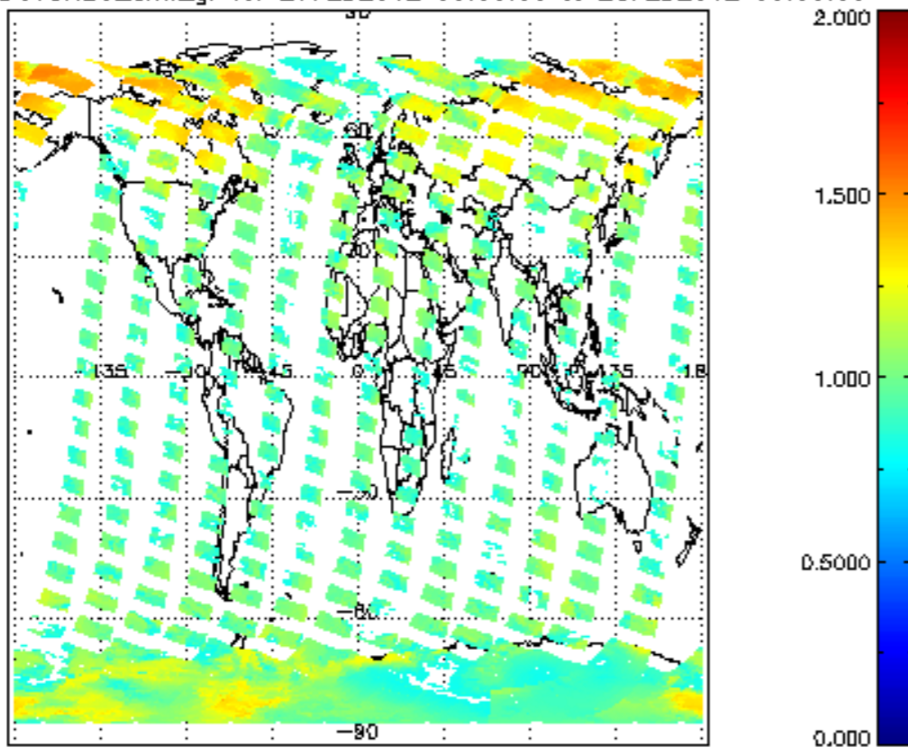
SCIOL2P_NADUV8H20_amf_gr for 27FEB2012 00:00:00 to 28FEB2012 00:00:00
