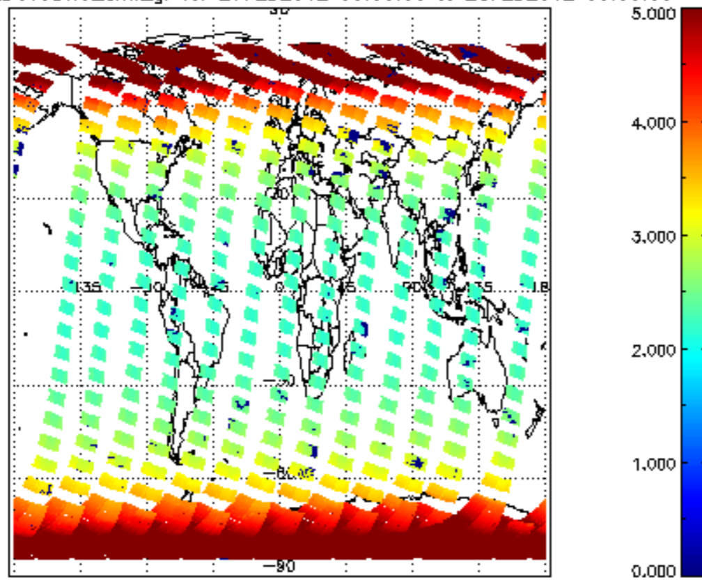
SCIOL2P_NADUV3BRO_amf_gr for 27FEB2012 00:00:00 to 28FEB2012 00:00:00
