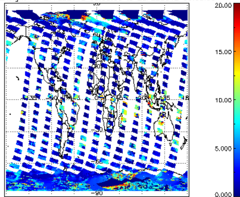
cl_top_height for 27FEB2012 00:00:00 to 28FEB2012 00:00:00
