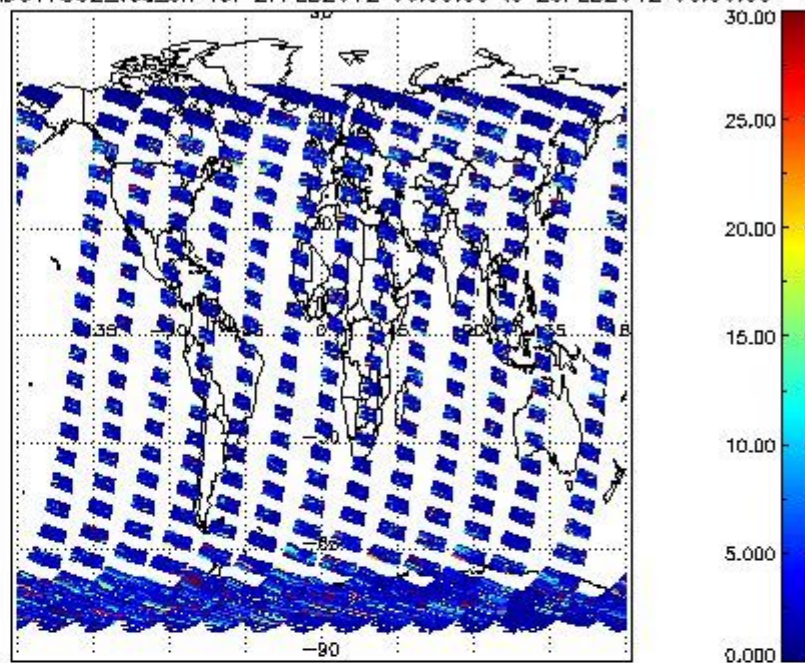
SCIOL2P_NADUV7S02_vcd_err for 27FEB2012 00:00:00 to 28FEB2012 00:00:00
