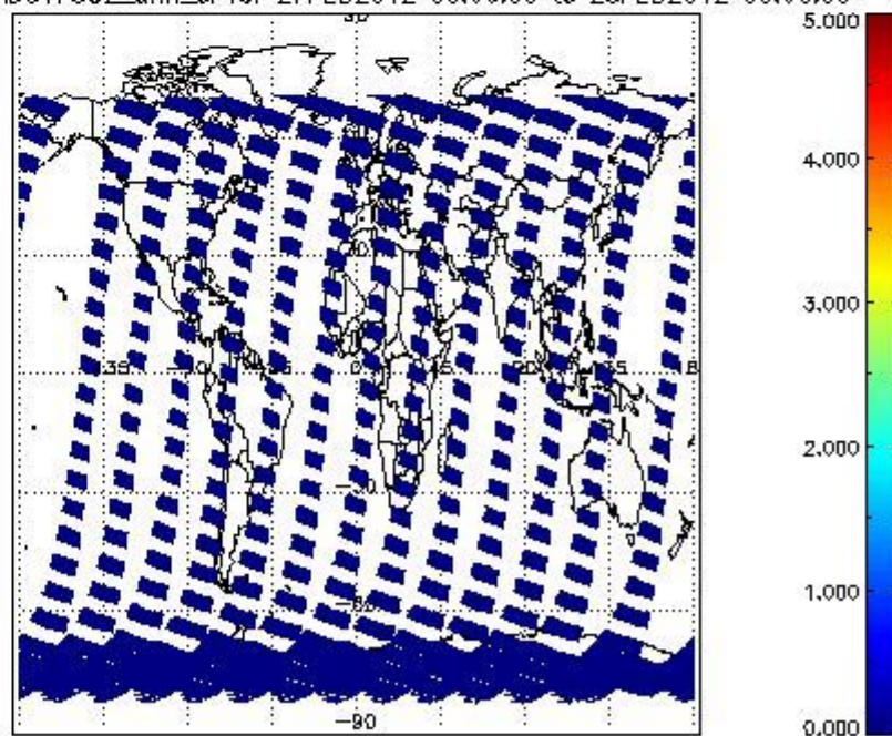
SCIOL2P_NADUV7S02_amf_cl for 27FEB2012 00:00:00 to 28FEB2012 00:00:00
