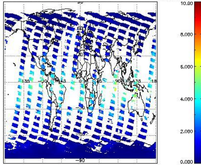
SCIOL2P_NADUV8H2O_vcd for 27FEB2012 00:00:00 to 28FEB2012 00:00:00
