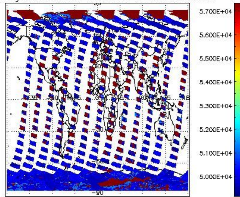
cloud_flags for 27FEB2012 00:00:00 to 28FEB2012 00:00:00
