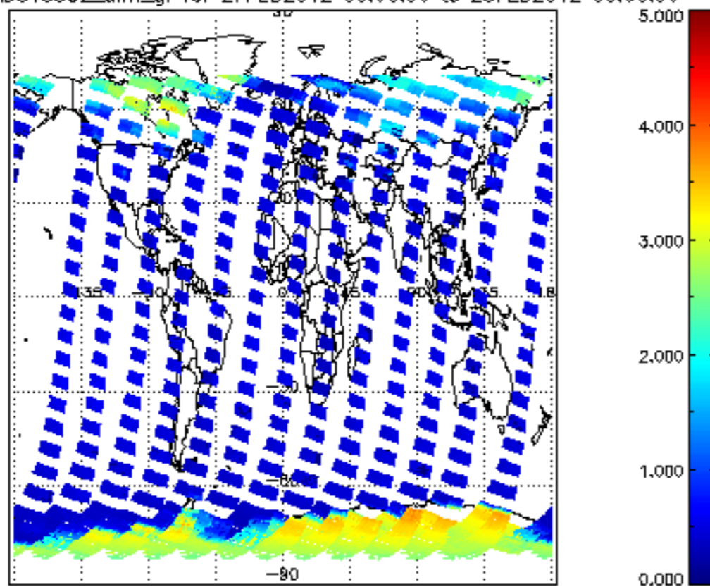
SCIOL2P_NADUV5S02_amf_gr for 27FEB2012 00:00:00 to 28FEB2012 00:00:00
