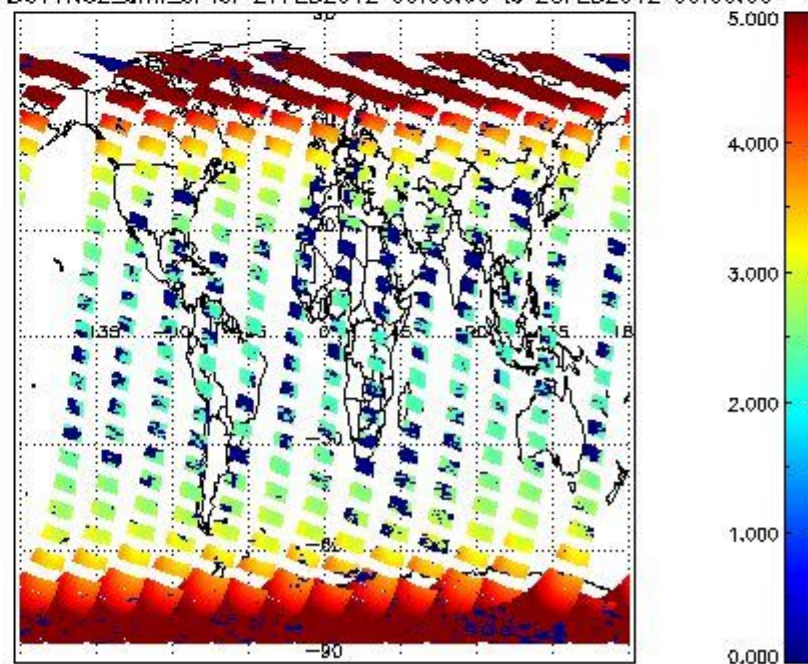
SCIOL2P_NADUV1N02_amf_cl for 27FEB2012 00:00:00 to 28FEB2012 00:00:00
