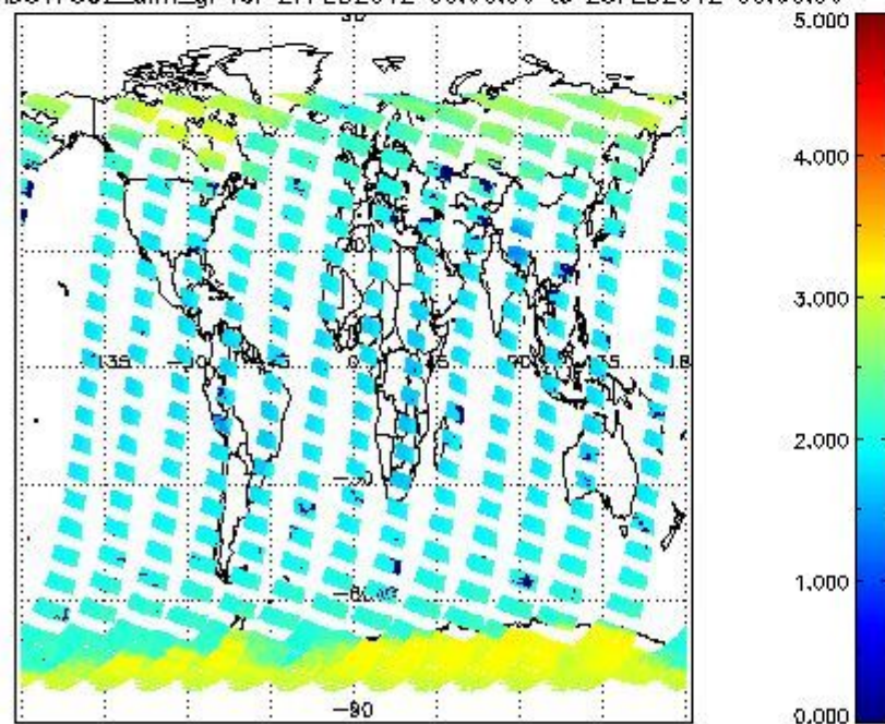
SCIOL2P_NADUV7S02_amf_gr for 27FEB2012 00:00:00 to 28FEB2012 00:00:00
