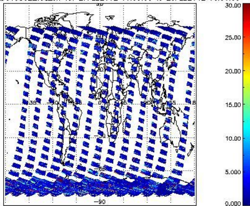
SCIOL2P_NADUV5SO2_vcd_err for 27FEB2012 00:00:00 to 28FEB2012 00:00:00
