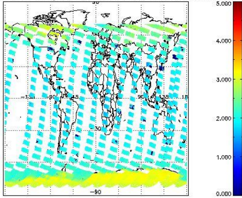
SCIOL2P_NADUV7S02_amf_gr for 26FEB2012 00:00:00 to 27FEB2012 00:00:00
