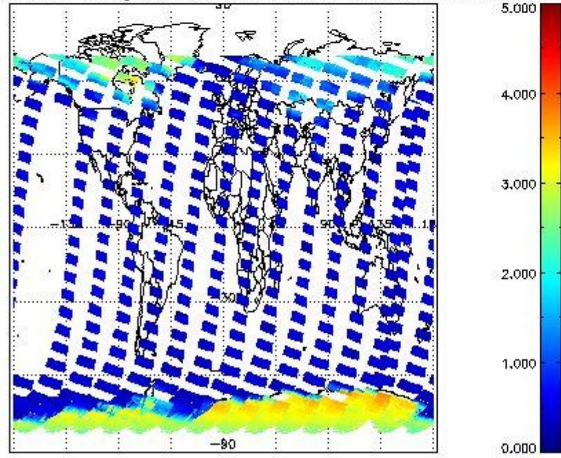
SCIOL2P_NADUV5SO2_amf_gr for 26FEB2012 00:00:00 to 27FEB2012 00:00:00
