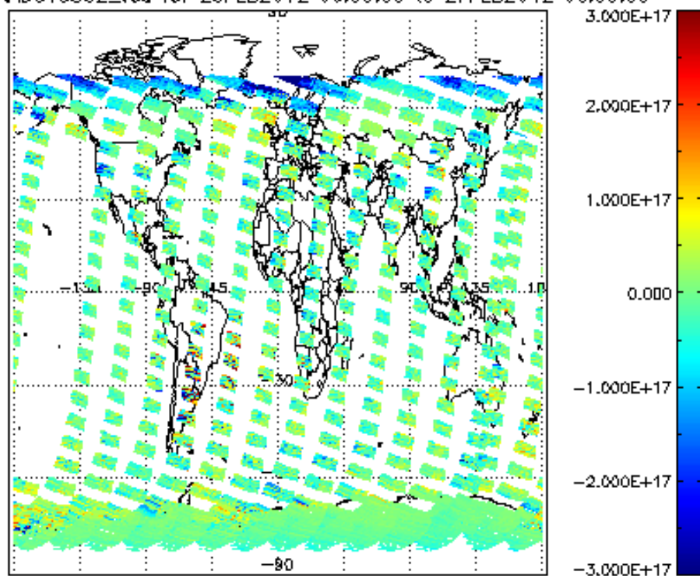
SCIOL2P_NADUV5S02_vcd for 26FEB2012 00:00:00 to 27FEB2012 00:00:00
