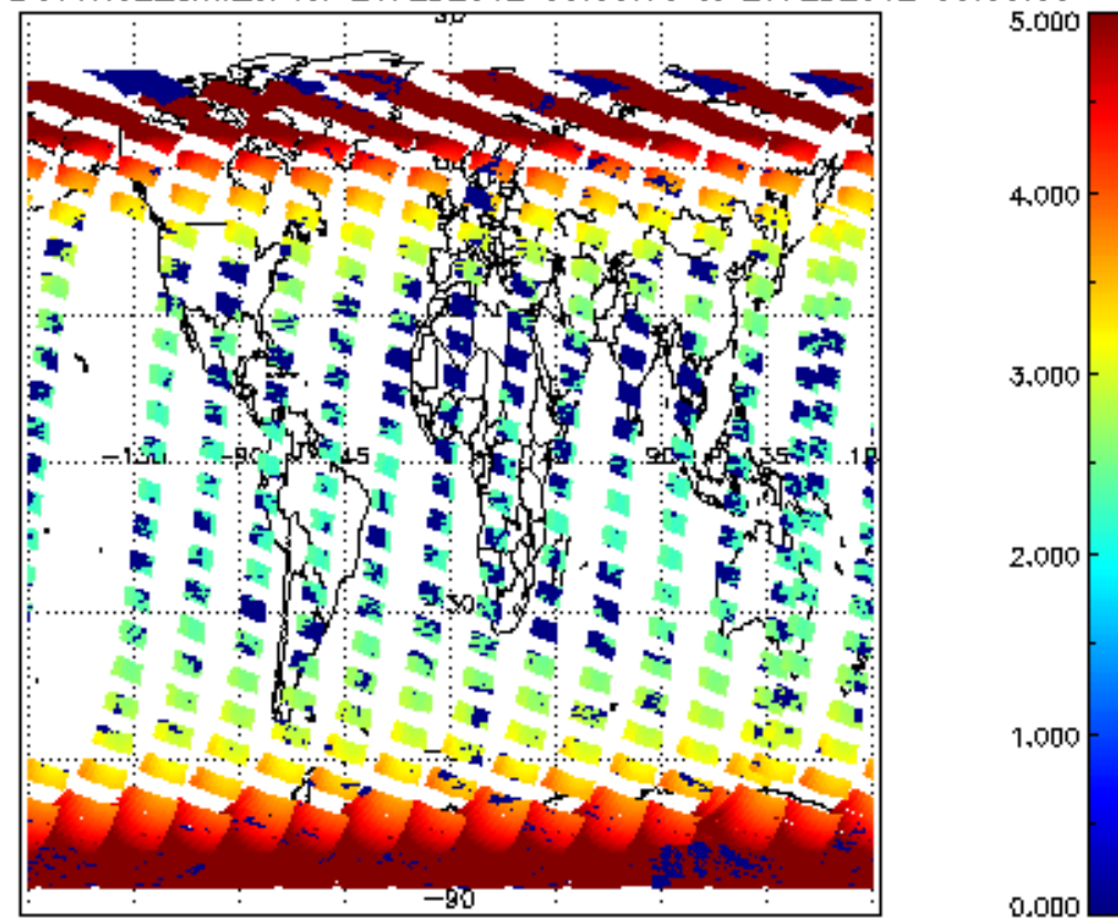
SCIOL2P_NADUV1N02_amf_cl for 26FEB2012 00:00:00 to 27FEB2012 00:00:00
