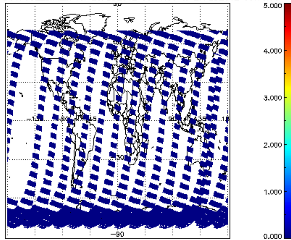
SCIOL2P_NADUV7S02_amf_cl for 26FEB2012 00:00:00 to 27FEB2012 00:00:00
