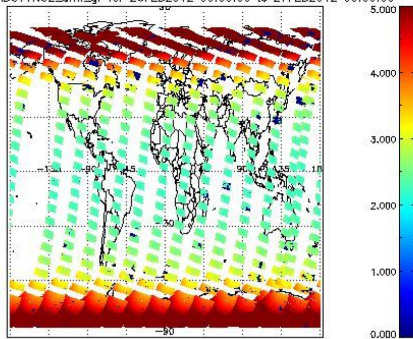
SCIOL2P_NADUV1N02_amf_gr for 26FEB2012 00:00:00 to 27FEB2012 00:00:00
