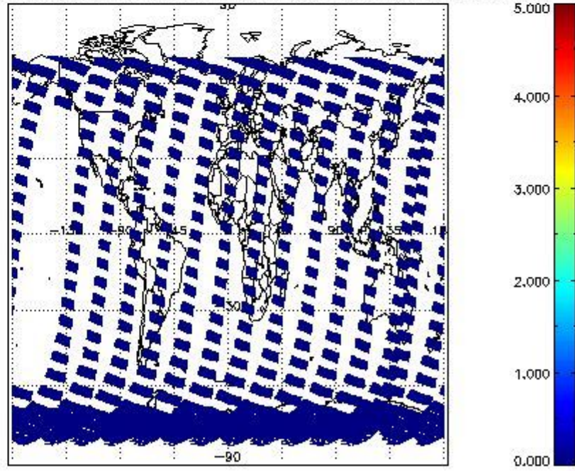
SCIOL2P_NADUV7S02_amf_cl for 26FEB2012 00:00:00 to 27FEB2012 00:00:00
