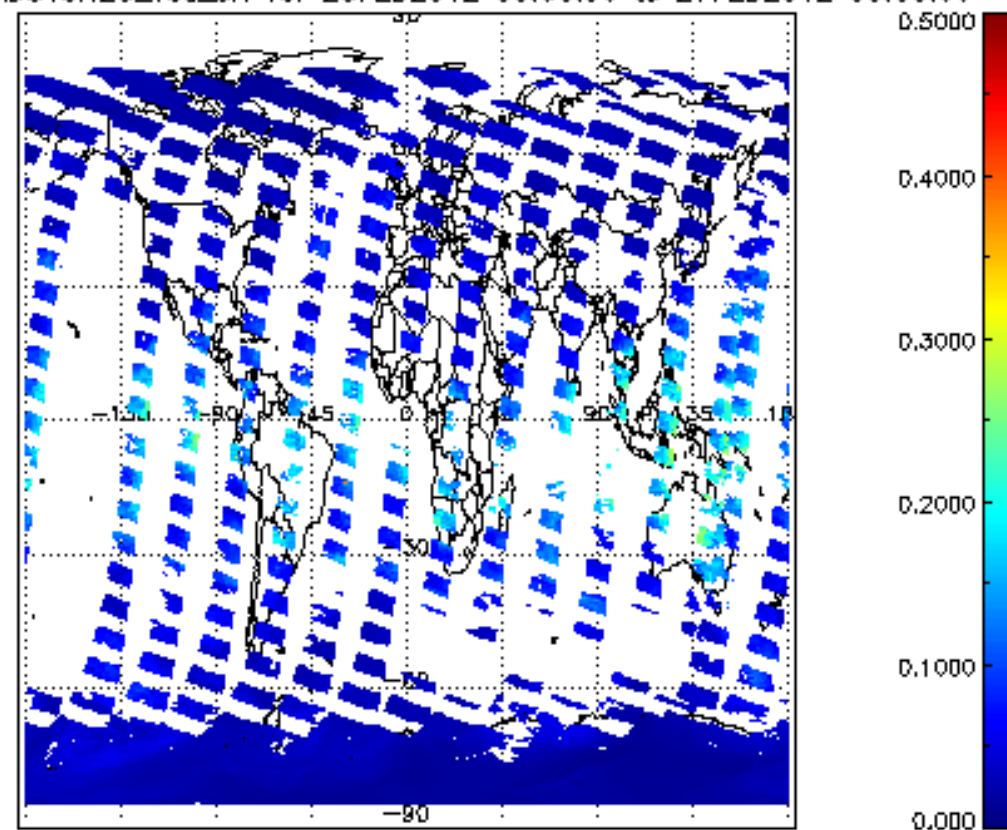
SCIOL2P_NADUV8H2O_vcd_err for 26FEB2012 00:00:00 to 27FEB2012 00:00:00
