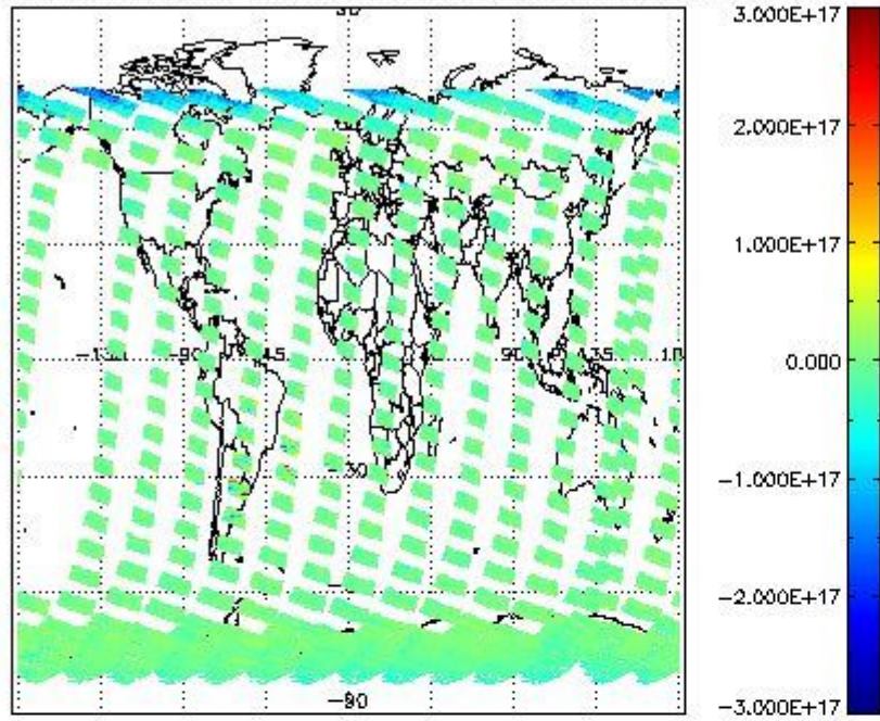
SCIOL2P_NADUV7S02_vcd for 26FEB2012 00:00:00 to 27FEB2012 00:00:00
