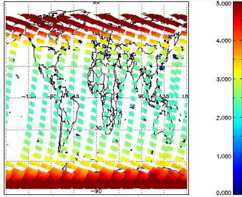
SCIOL2P_NADUV3BRO_amf_gr for 26FEB2012 00:00:00 to 27FEB2012 00:00:00
