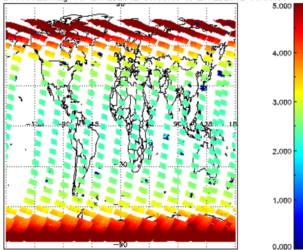
SCIOL2P_NADUV003_amf_gr for 26FEB2012 00:00:00 to 27FEB2012 00:00:00
