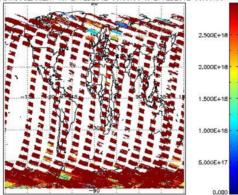
SCIOL2P_NADIR3CO_vcd_err for 26FEB2012 00:00:00 to 27FEB2012 00:00:00
