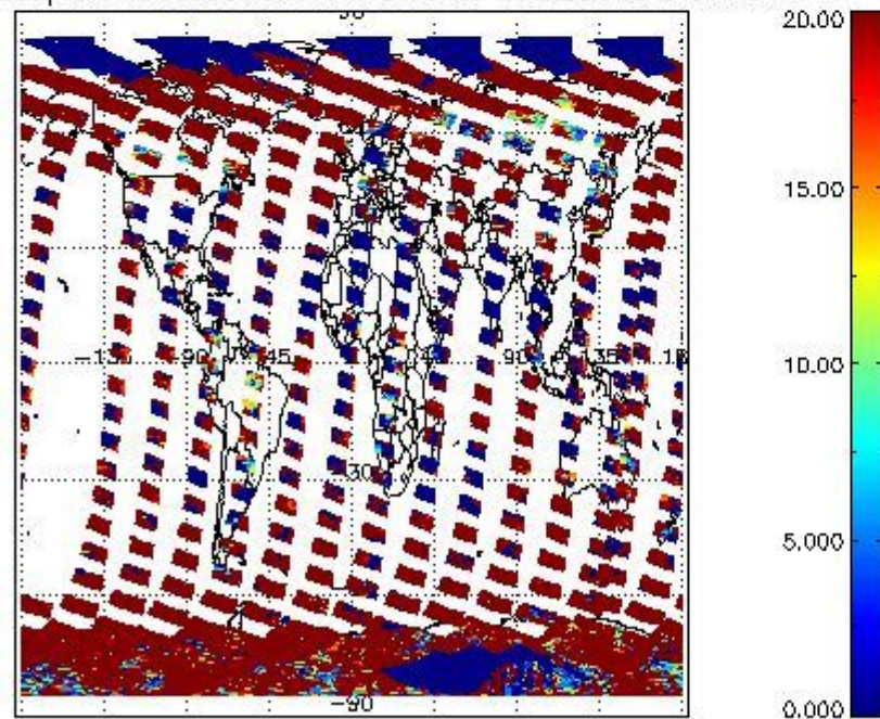
cL_opt_depth for 26FEB2012 00:00:00 to 27FEB2012 00:00:00
