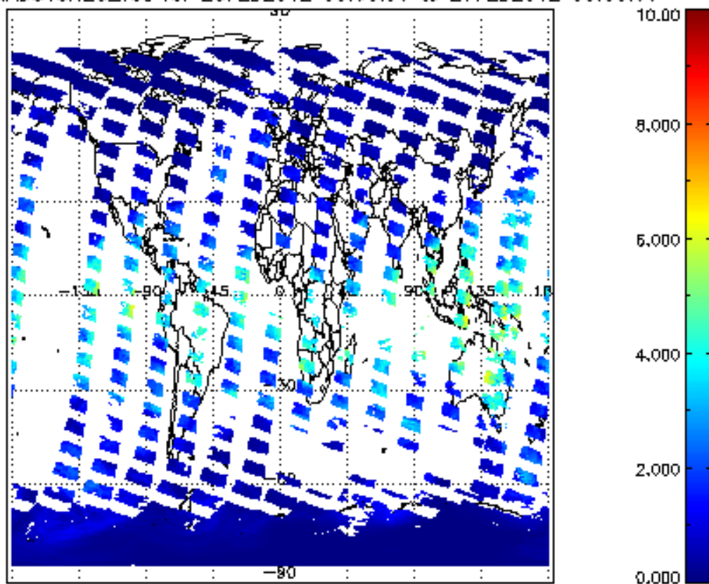
SCIOL2P_NADUV8H2O_vcd for 26FEB2012 00:00:00 to 27FEB2012 00:00:00
