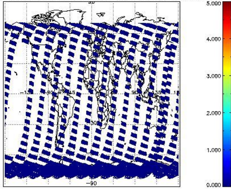
SCIOL2P_NADUV5SO2_amf_cl for 26FEB2012 00:00:00 to 27FEB2012 00:00:00
