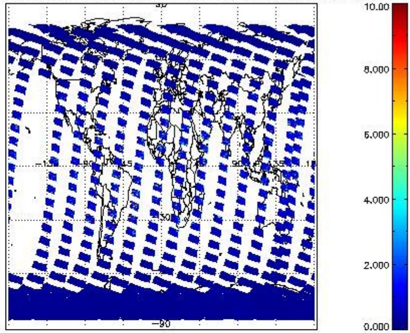
SCIOL2P_NADUV3BRO_vcd_err for 26FEB2012 00:00:00 to 27FEB2012 00:00:00
