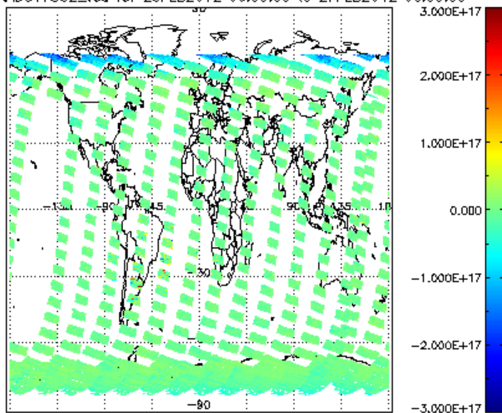
SCIOL2P_NADUV7S02_vcd for 26FEB2012 00:00:00 to 27FEB2012 00:00:00
