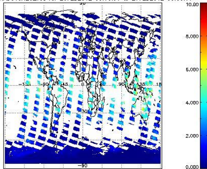
SCIOL2P_NADUV8H2O_vcd for 26FEB2012 00:00:00 to 27FEB2012 00:00:00
