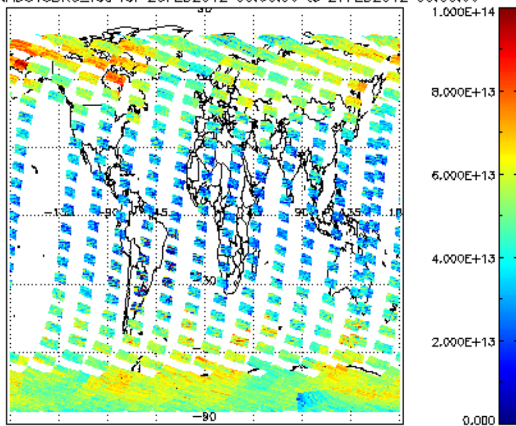
SCIOL2P_NADUV3BRO_vcd for 26FEB2012 00:00:00 to 27FEB2012 00:00:00
