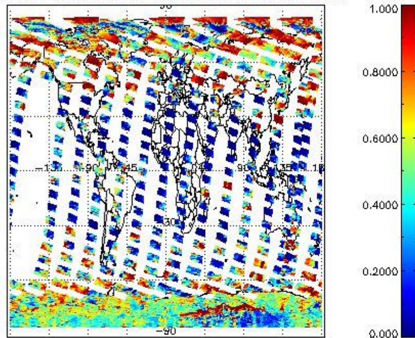
cL_frac for 26FEB2012 00:00:00 to 27FEB2012 00:00:00
