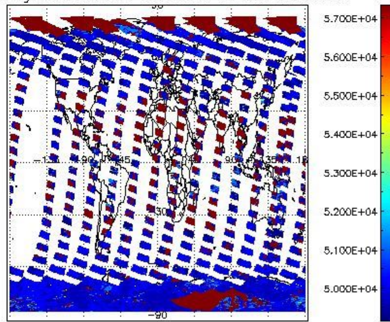
cloud_flags for 26FEB2012 00:00:00 to 27FEB2012 00:00:00
