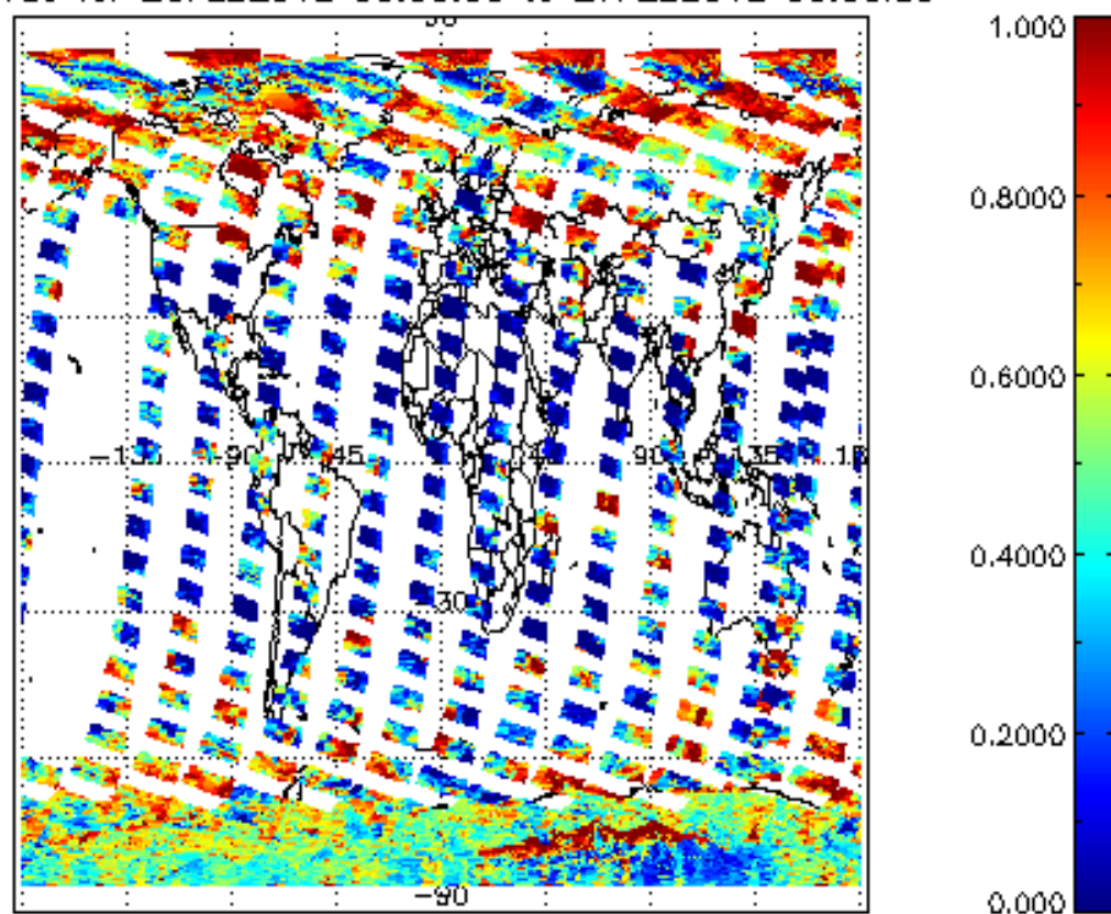
cl_frac for 26FEB2012 00:00:00 to 27FEB2012 00:00:00
