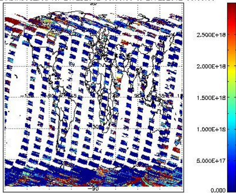
SCIOL2P_NADIR3CO_vcd for 26FEB2012 00:00:00 to 27FEB2012 00:00:00
