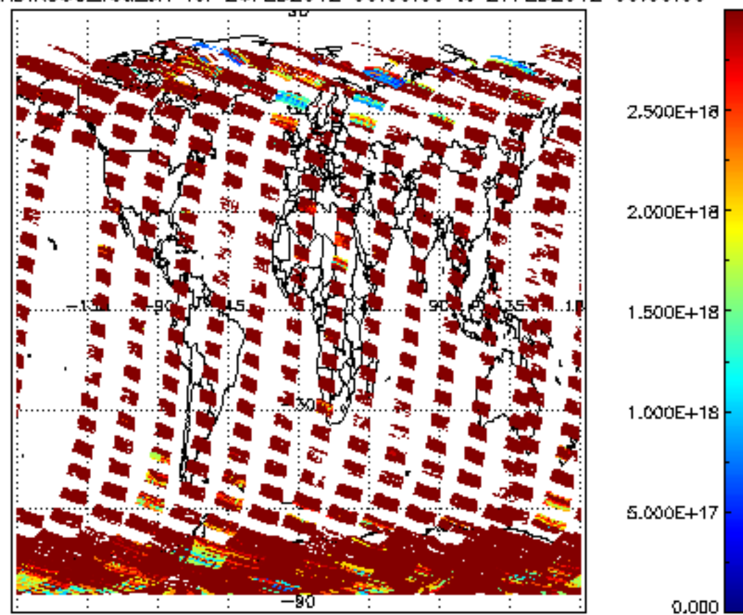
SCIOL2P_NADIR3CO_vcd_err for 26FEB2012 00:00:00 to 27FEB2012 00:00:00
