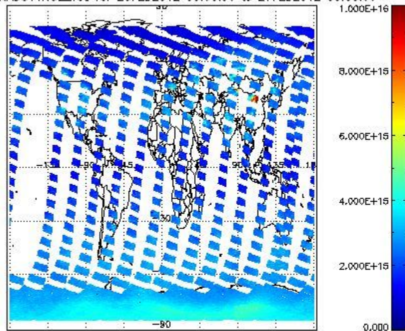
SCIOL2P_NADUV1N02_vcd for 26FEB2012 00:00:00 to 27FEB2012 00:00:00
