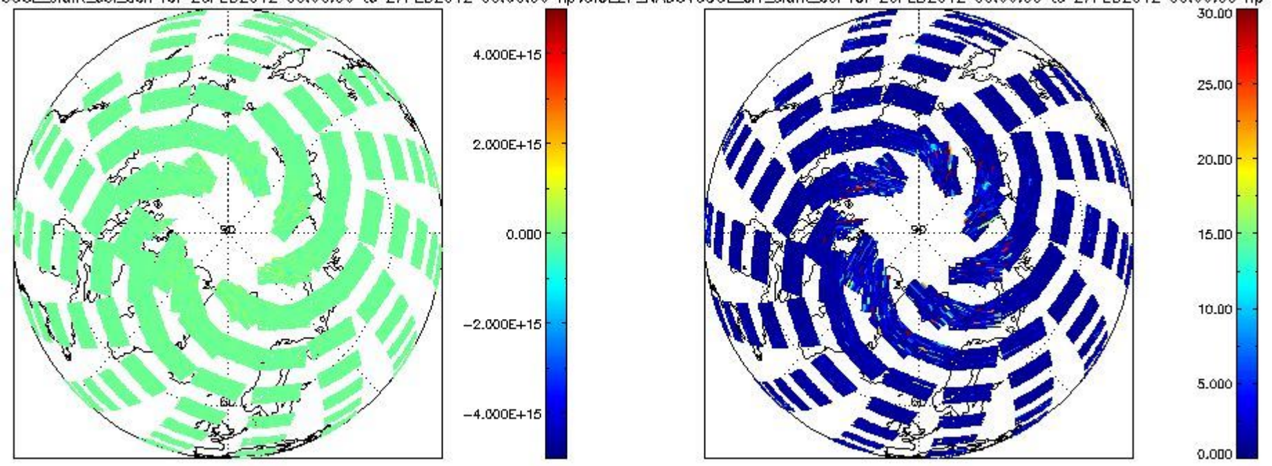
CIOL2P_NADUV6OCL_slant_col_den for 26FEB2012 00:00:00 to 27FEB2012 00:00:00 np; CIOL2P_NADUV6OCL_slant_col for 26FEB2012 00:00:00 to 27FEB2012 00:00:00 np
