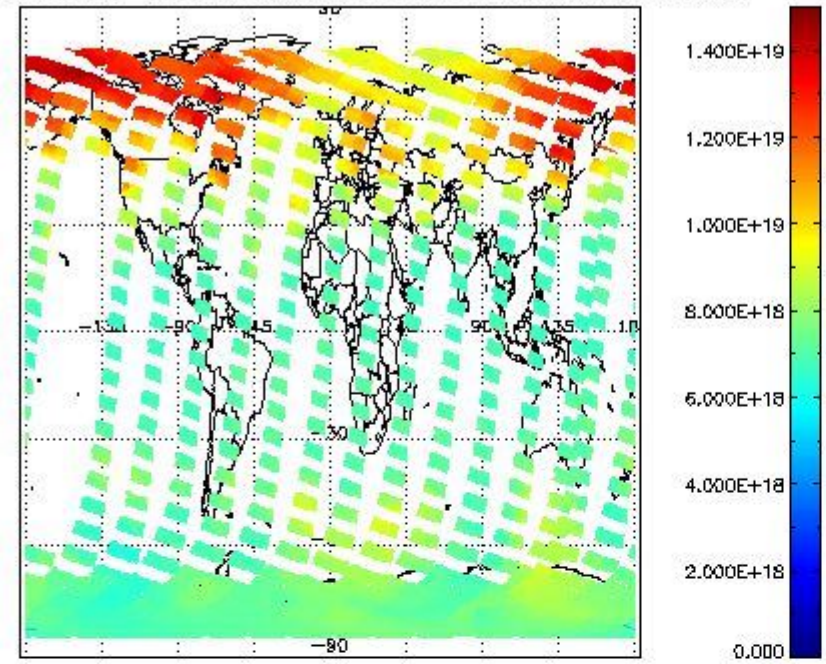
SCIOL2P_NADUV003_vcd for 26FEB2012 00:00:00 to 27FEB2012 00:00:00
