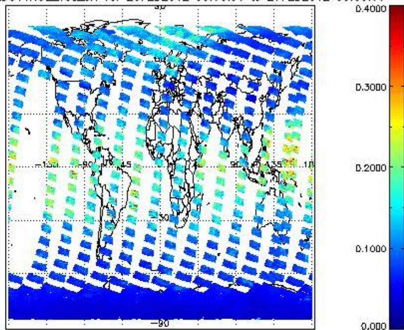
SCIOL2P_NADUV1N02_vcd_err for 26FEB2012 00:00:00 to 27FEB2012 00:00:00
