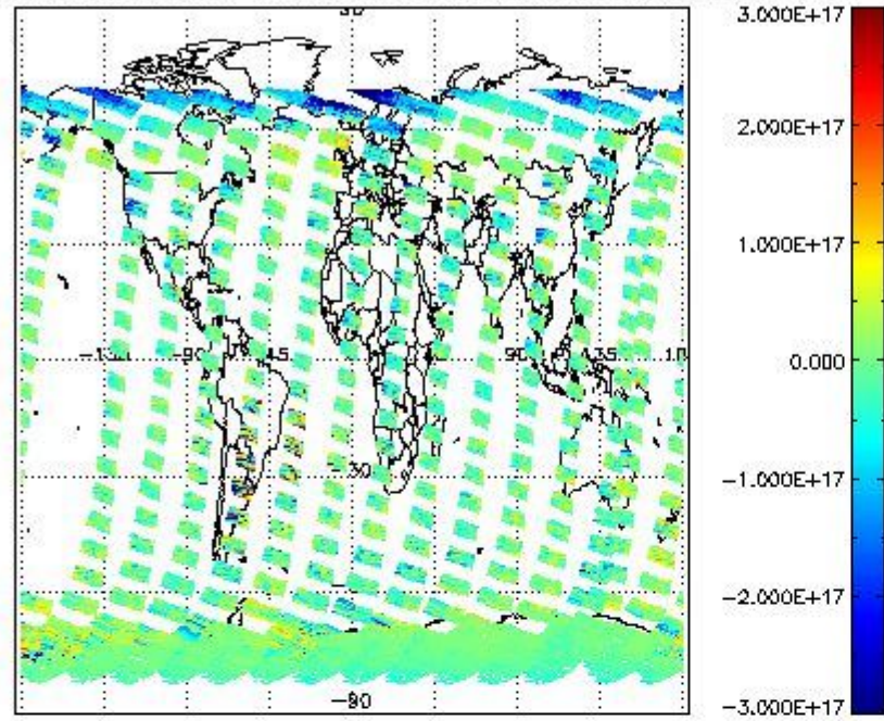
SCIOL2P_NADUV5SO2_vcd for 26FEB2012 00:00:00 to 27FEB2012 00:00:00
