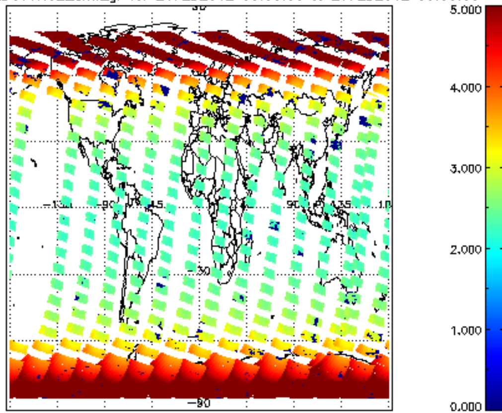
SCIOL2P_NADUV1N02_amf_gr for 26FEB2012 00:00:00 to 27FEB2012 00:00:00
