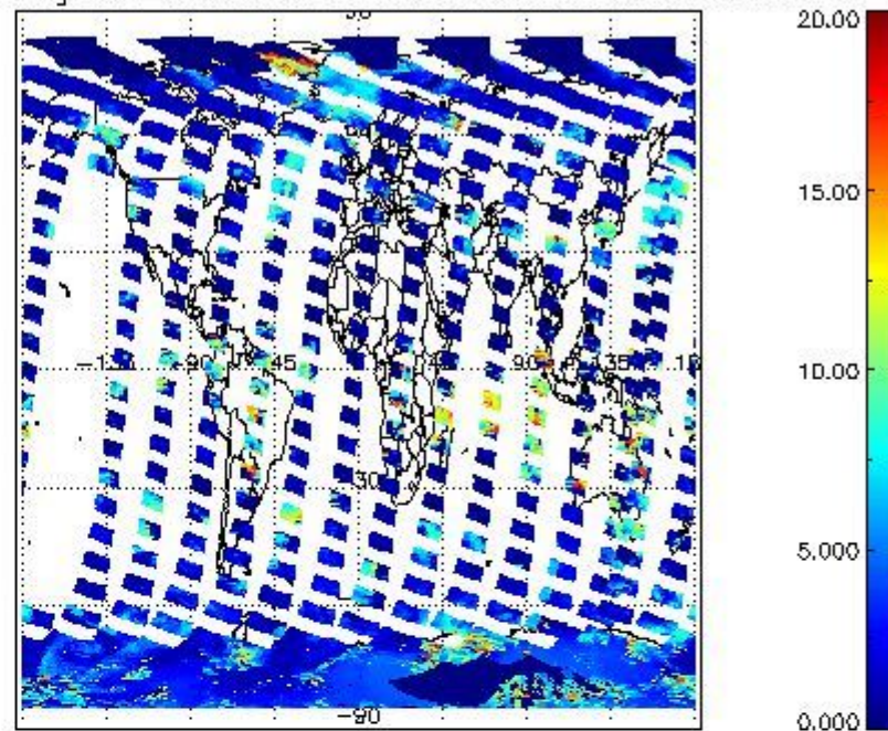
cL_top_height for 26FEB2012 00:00:00 to 27FEB2012 00:00:00
