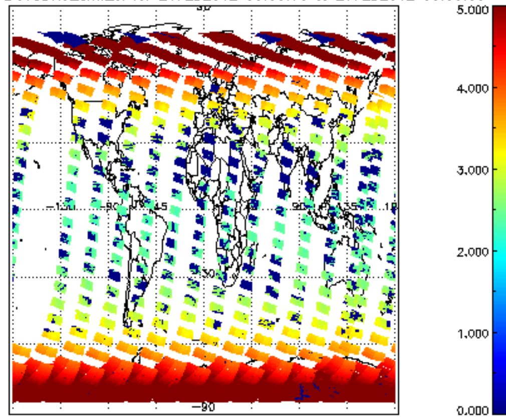
SCIOL2P_NADUV3BRO_amf_cl for 26FEB2012 00:00:00 to 27FEB2012 00:00:00
