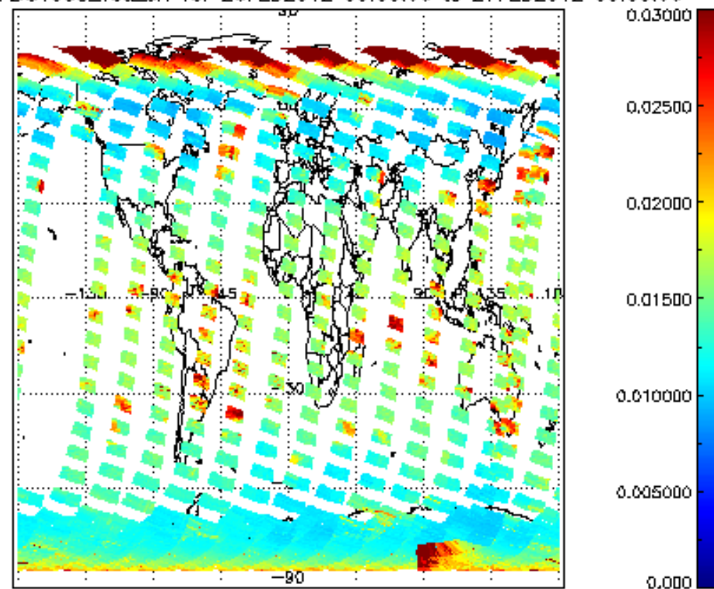
SCIOL2P_NADUV003_vcd_err for 26FEB2012 00:00:00 to 27FEB2012 00:00:00
