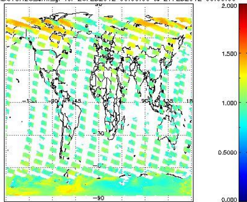
SCIOL2P_NADUV8H2O_amf_gr for 26FEB2012 00:00:00 to 27FEB2012 00:00:00
