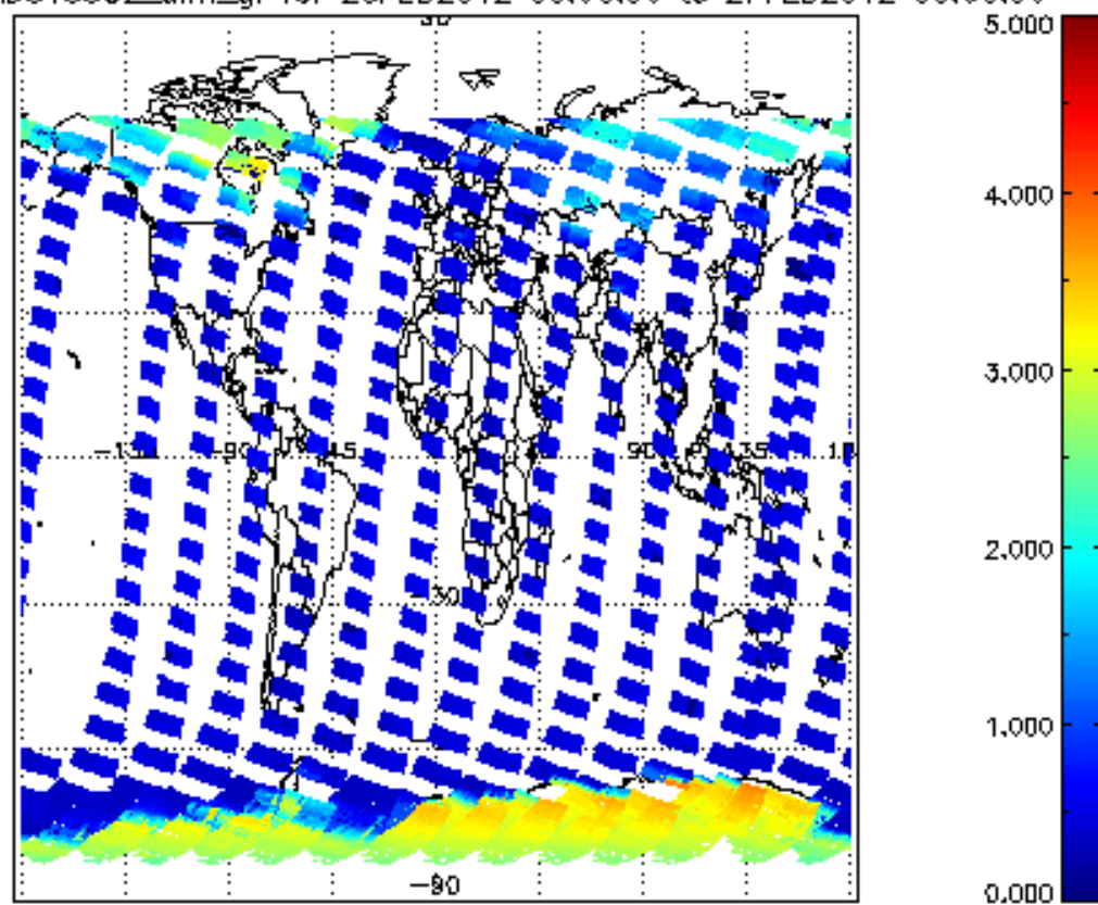
SCIOL2P_NADUV5S02_amf_gr for 26FEB2012 00:00:00 to 27FEB2012 00:00:00
