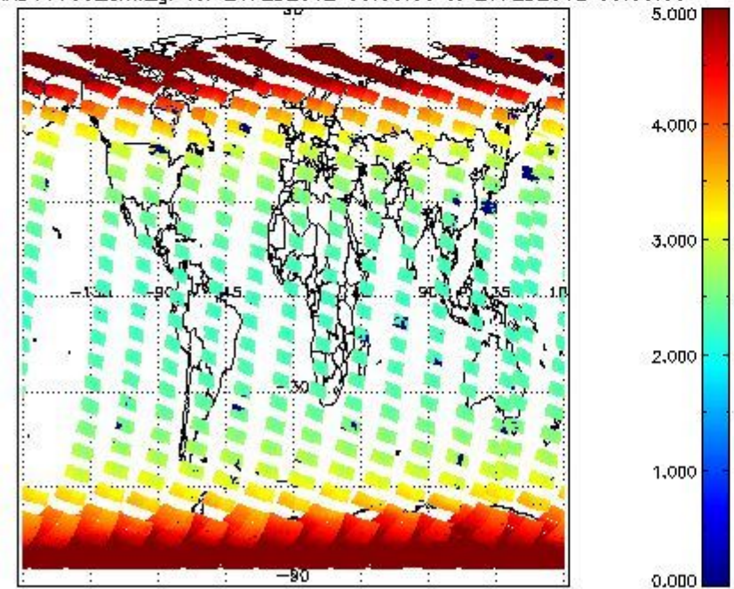
SCIOL2P_NADUV003_amf_gr for 26FEB2012 00:00:00 to 27FEB2012 00:00:00
