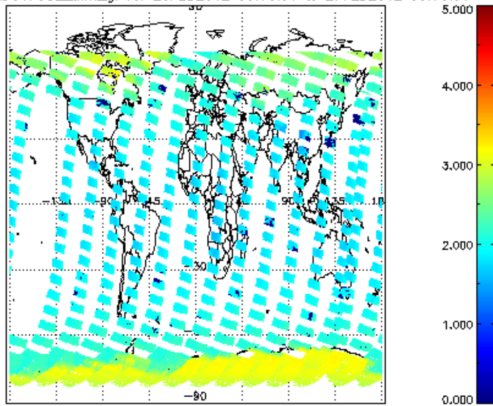
SCIOL2P_NADUV7S02_amf_gr for 26FEB2012 00:00:00 to 27FEB2012 00:00:00
