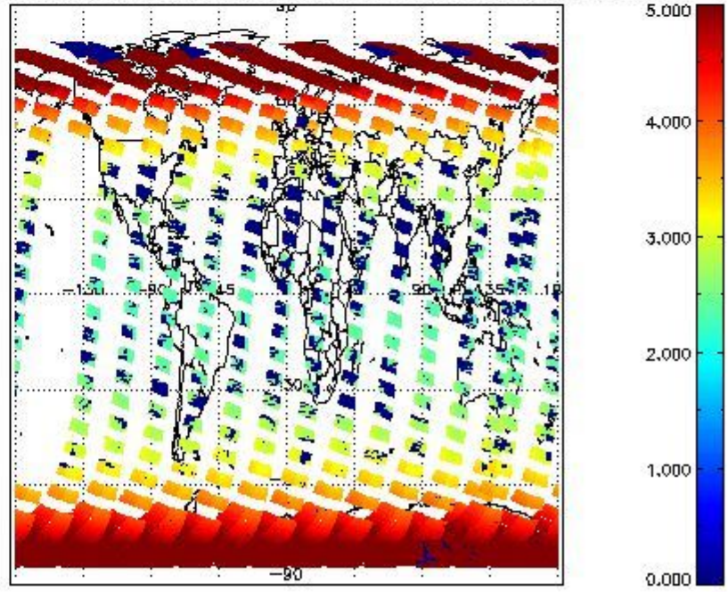
SCIOL2P_NADUV3BRO_amf_cl for 26FEB2012 00:00:00 to 27FEB2012 00:00:00
