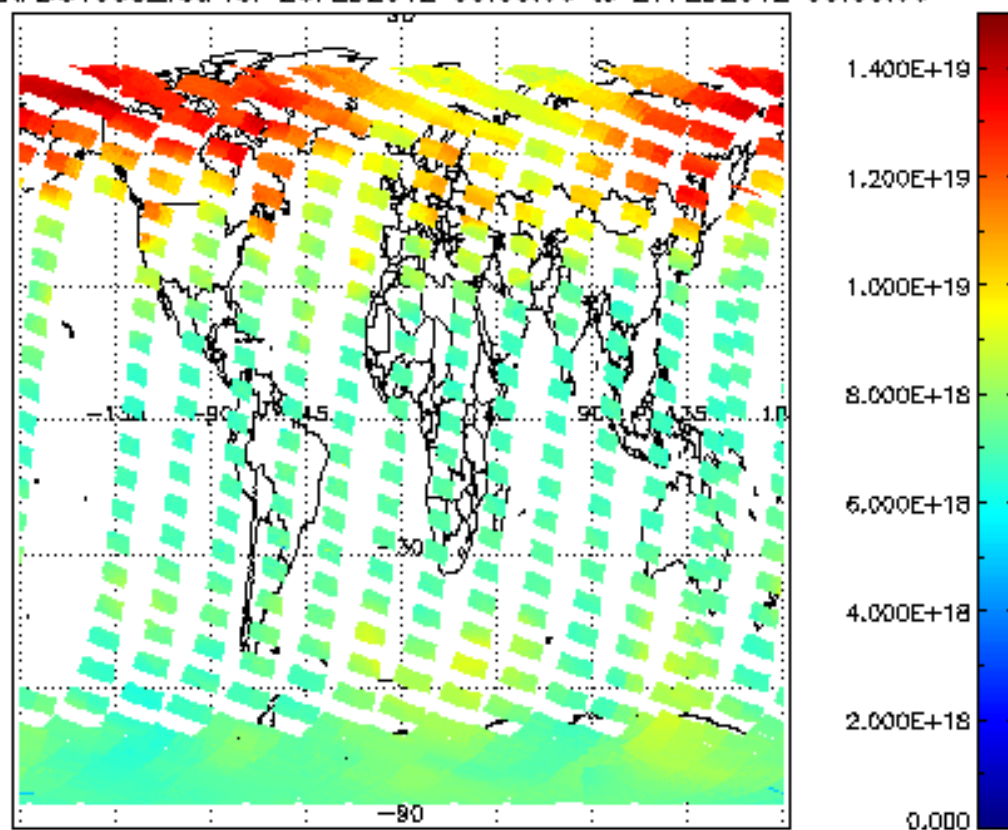
SCIOL2P_NADUV003_vcd for 26FEB2012 00:00:00 to 27FEB2012 00:00:00
