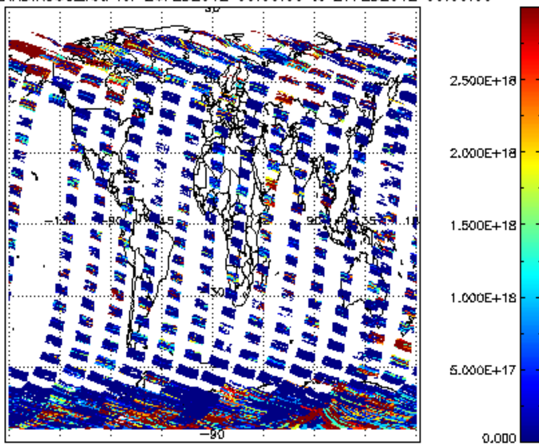
SCIOL2P_NADIR3CO_vcd for 26FEB2012 00:00:00 to 27FEB2012 00:00:00
