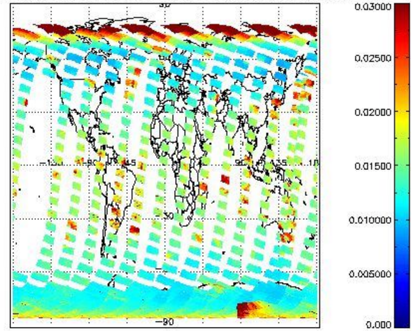
SCIOL2P_NADUV003_vcd_err for 26FEB2012 00:00:00 to 27FEB2012 00:00:00
