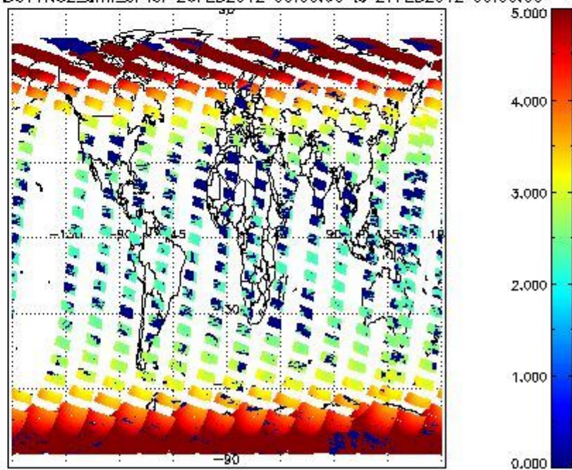
SCIOL2P_NADUV1N02_amf_cl for 26FEB2012 00:00:00 to 27FEB2012 00:00:00
