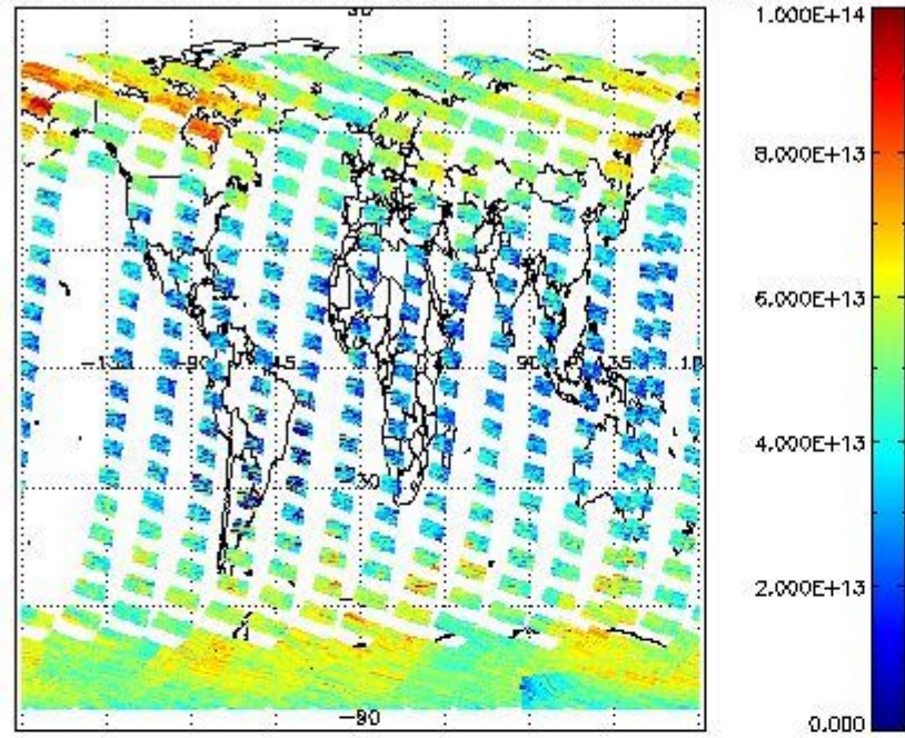
SCIOL2P_NADUV3BRO_vcd for 26FEB2012 00:00:00 to 27FEB2012 00:00:00
