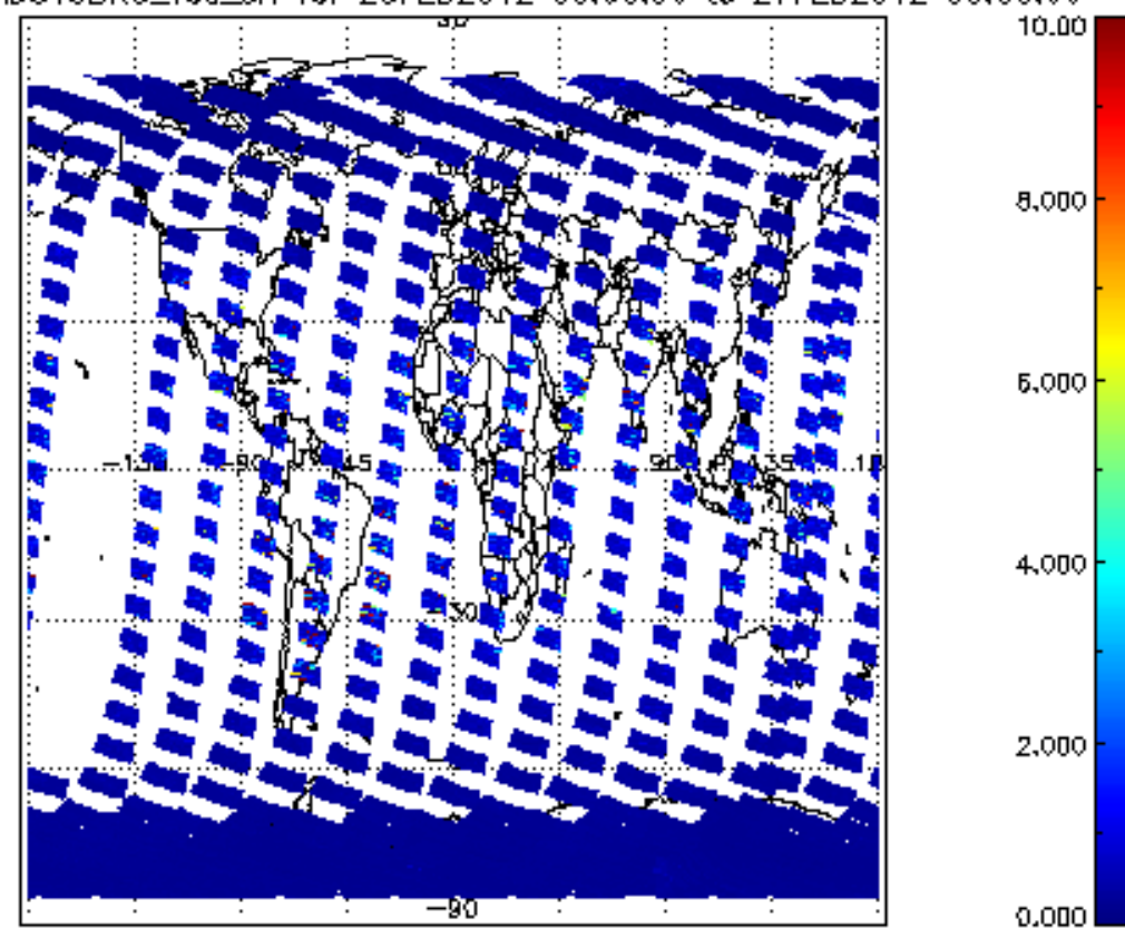
SCIOL2P_NADUV3BRO_vcd_err for 26FEB2012 00:00:00 to 27FEB2012 00:00:00
