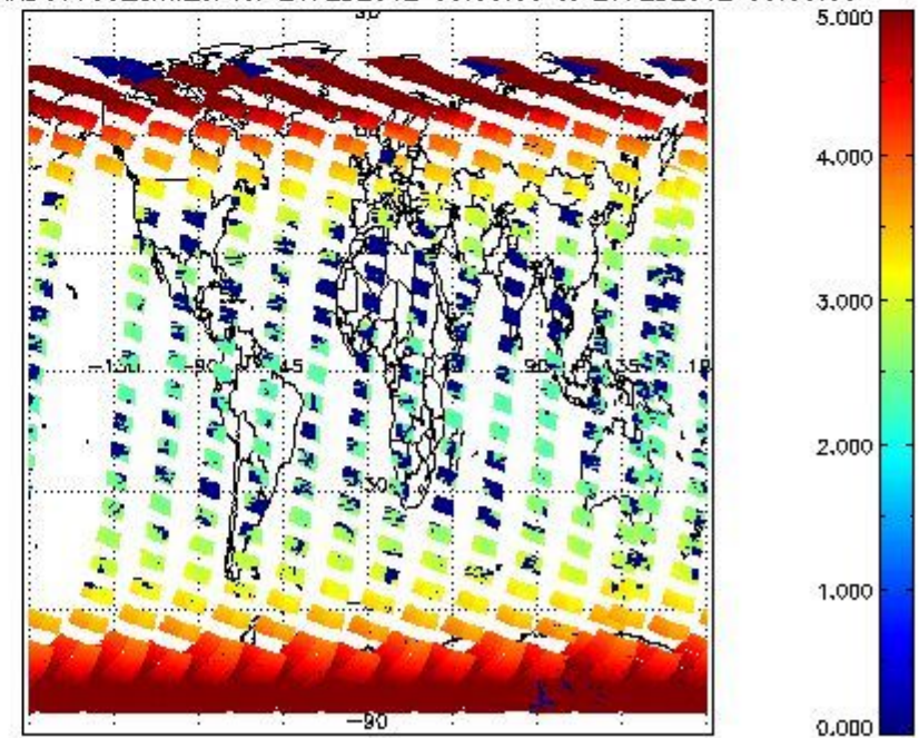
SCIOL2P_NADUV003_amf_cl for 26FEB2012 00:00:00 to 27FEB2012 00:00:00
