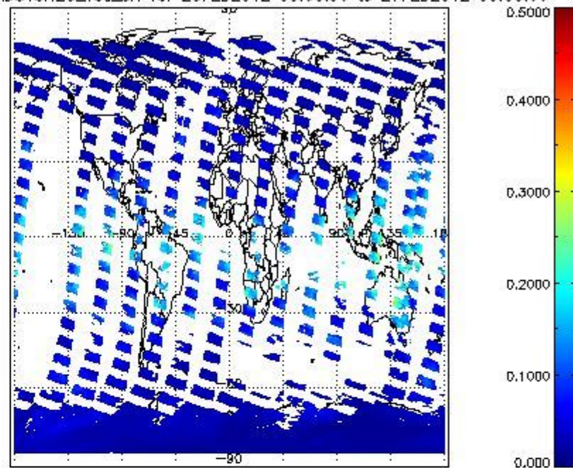
SCIOL2P_NADUV8H2O_vcd_err for 26FEB2012 00:00:00 to 27FEB2012 00:00:00
