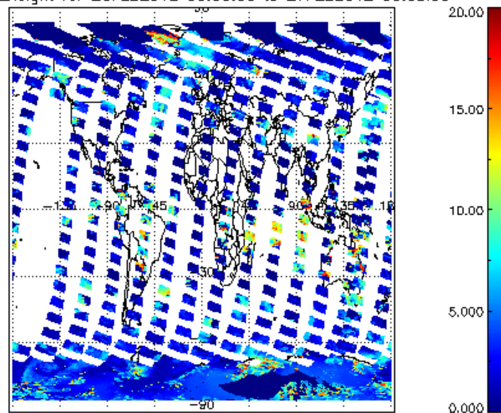
cl_top_height for 26FEB2012 00:00:00 to 27FEB2012 00:00:00
