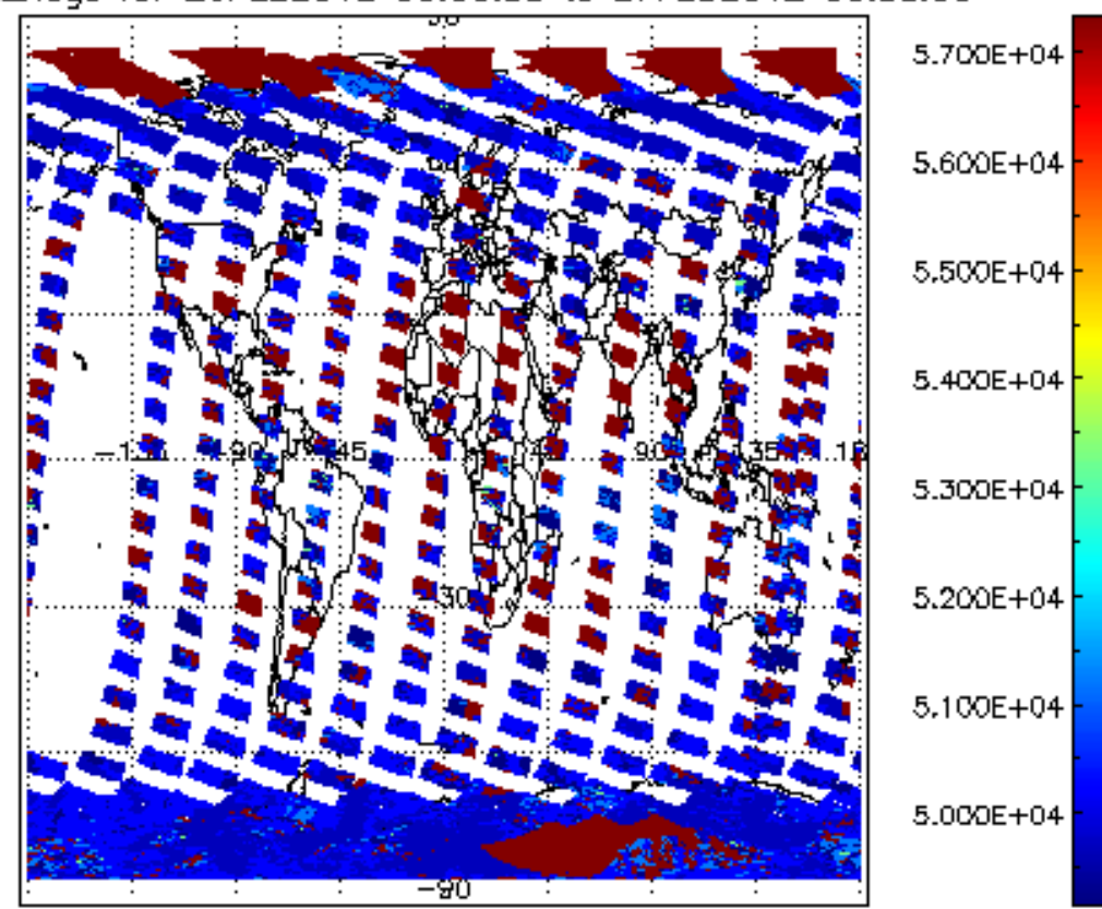
cloud_flags for 26FEB2012 00:00:00 to 27FEB2012 00:00:00
