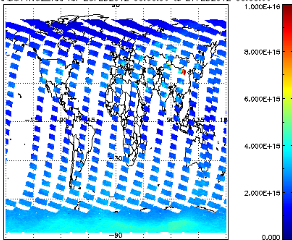
SCIOL2P_NADUV1N02_vcd for 26FEB2012 00:00:00 to 27FEB2012 00:00:00
