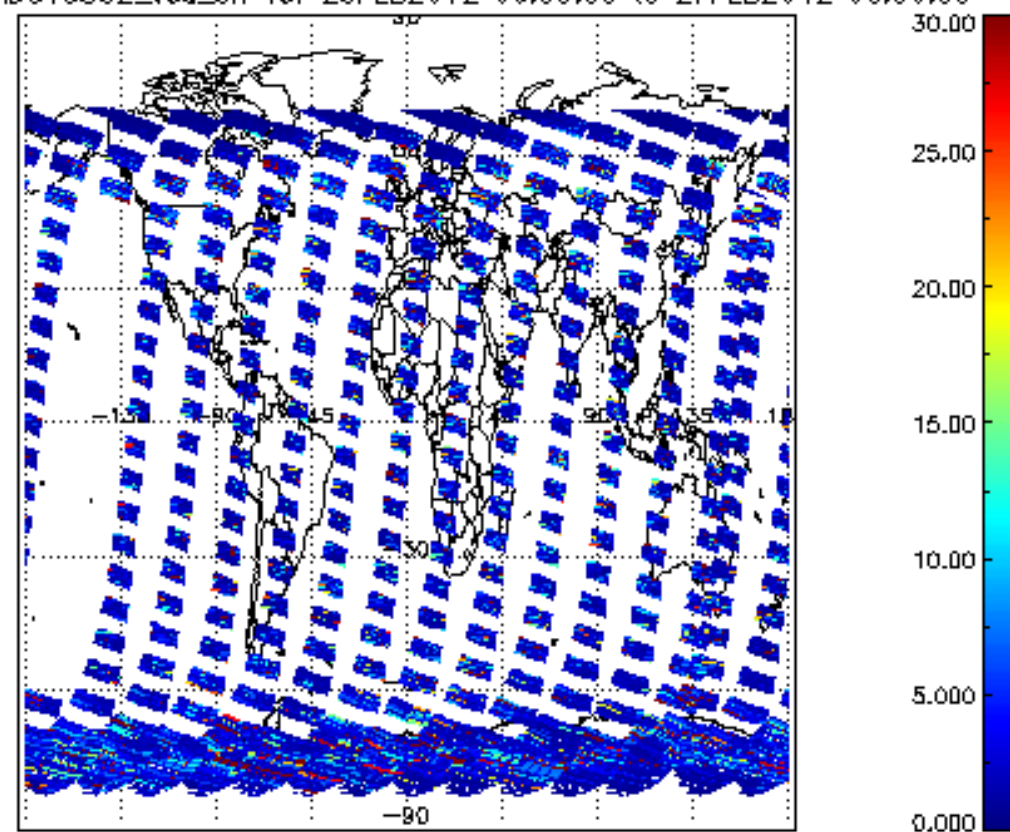
SCIOL2P_NADUV5S02_vcd_err for 26FEB2012 00:00:00 to 27FEB2012 00:00:00
