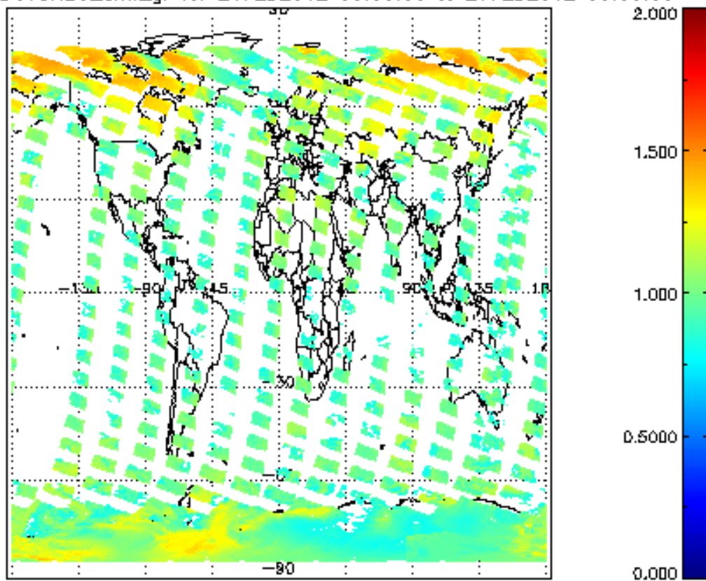
SCIOL2P_NADUV8H2O_amf_gr for 26FEB2012 00:00:00 to 27FEB2012 00:00:00
