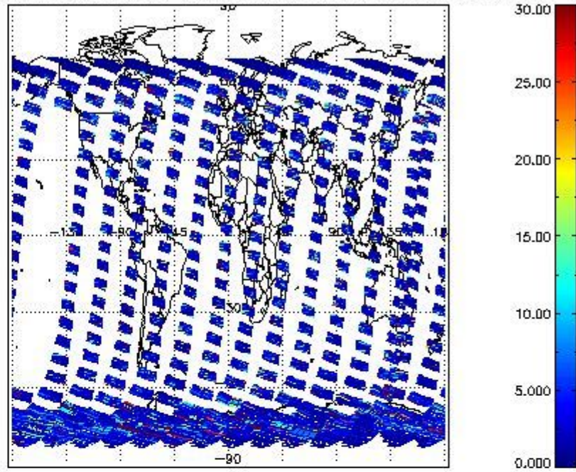
SCIOL2P_NADUV7S02_vcd_err for 26FEB2012 00:00:00 to 27FEB2012 00:00:00
