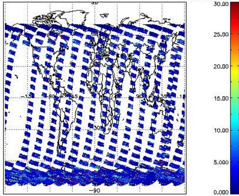
SCIOL2P_NADUV5SO2_vcd_err for 26FEB2012 00:00:00 to 27FEB2012 00:00:00
