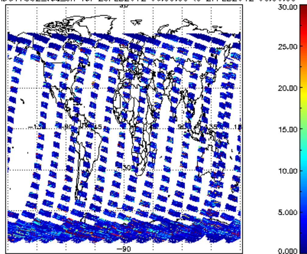
SCIOL2P_NADUV7S02_vcd_err for 26FEB2012 00:00:00 to 27FEB2012 00:00:00
