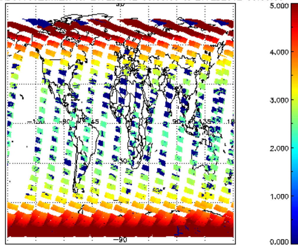
SCIOL2P_NADUV003_amf_cl for 26FEB2012 00:00:00 to 27FEB2012 00:00:00
