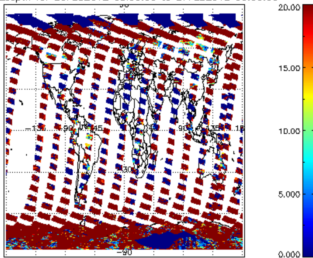
cl_opt_depth for 26FEB2012 00:00:00 to 27FEB2012 00:00:00
