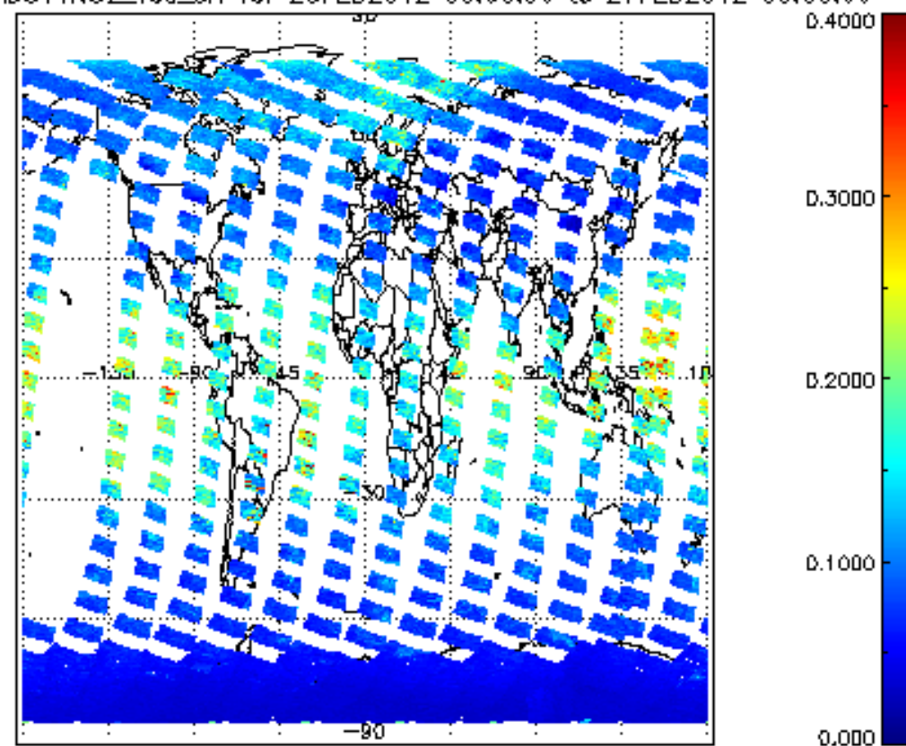
SCIOL2P_NADUV1N02_vcd_err for 26FEB2012 00:00:00 to 27FEB2012 00:00:00
