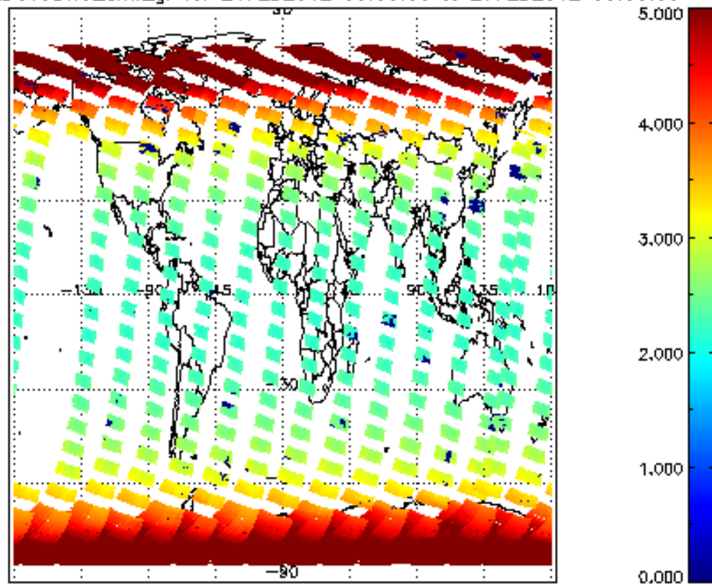
SCIOL2P_NADUV3BRO_amf_gr for 26FEB2012 00:00:00 to 27FEB2012 00:00:00
