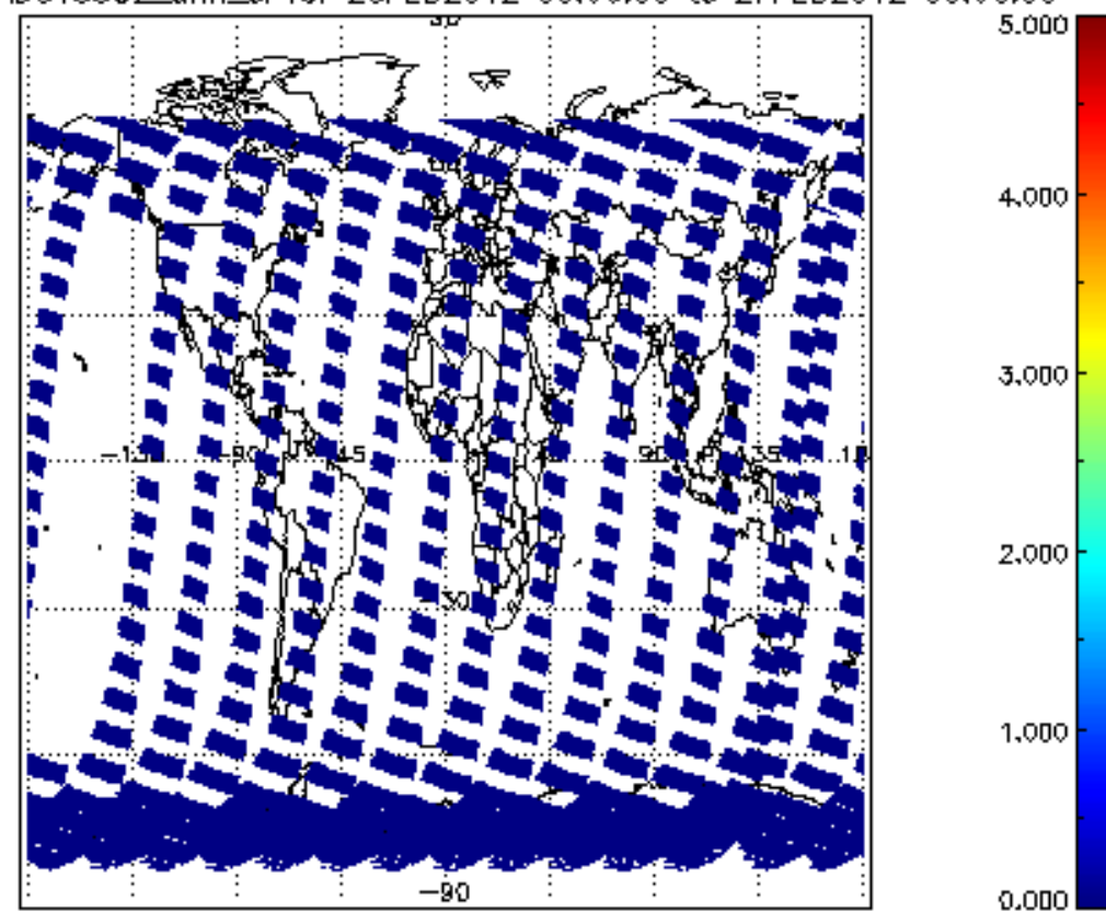
SCIOL2P_NADUV5S02_amf_cl for 26FEB2012 00:00:00 to 27FEB2012 00:00:00
