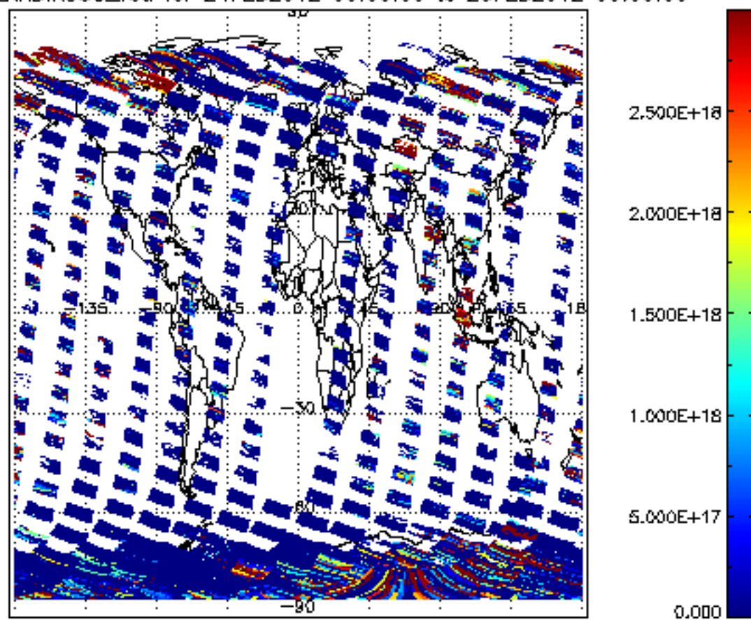
SCIOL2P_NADIR3CO_vcd for 24FEB2012 00:00:00 to 25FEB2012 00:00:00
