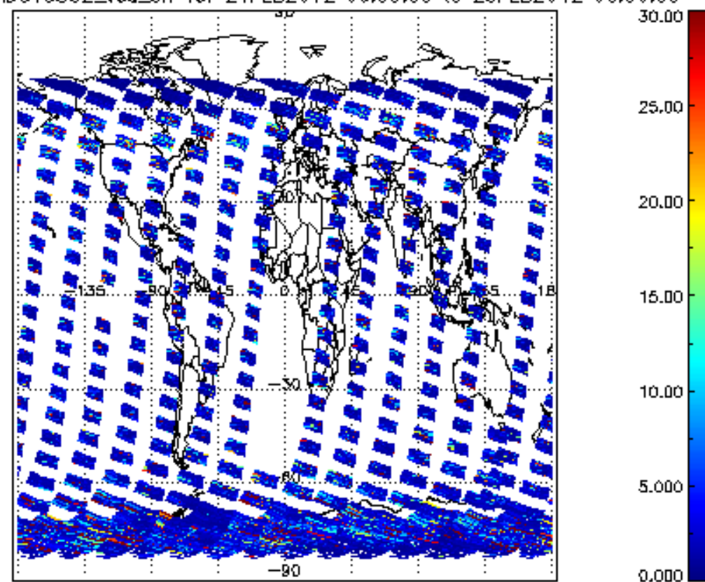
SCIOL2P_NADUV5S02_vcd_err for 24FEB2012 00:00:00 to 25FEB2012 00:00:00
