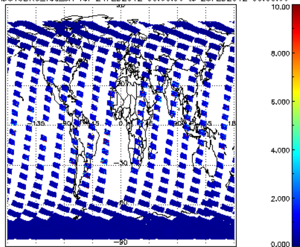
SCIOL2P_NADUV3BRO_vcd_err for 24FEB2012 00:00:00 to 25FEB2012 00:00:00
