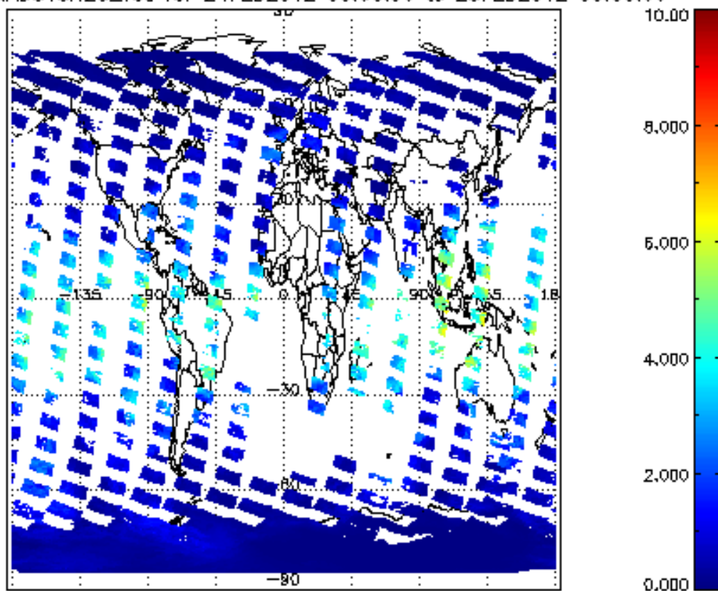
SCIOL2P_NADUV8H20_vcd for 24FEB2012 00:00:00 to 25FEB2012 00:00:00
