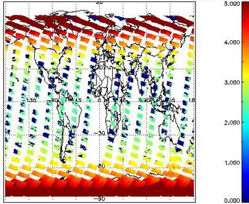
SCIOL2P_NADUV3BRO_amf_cl for 24FEB2012 00:00:00 to 25FEB2012 00:00:00
