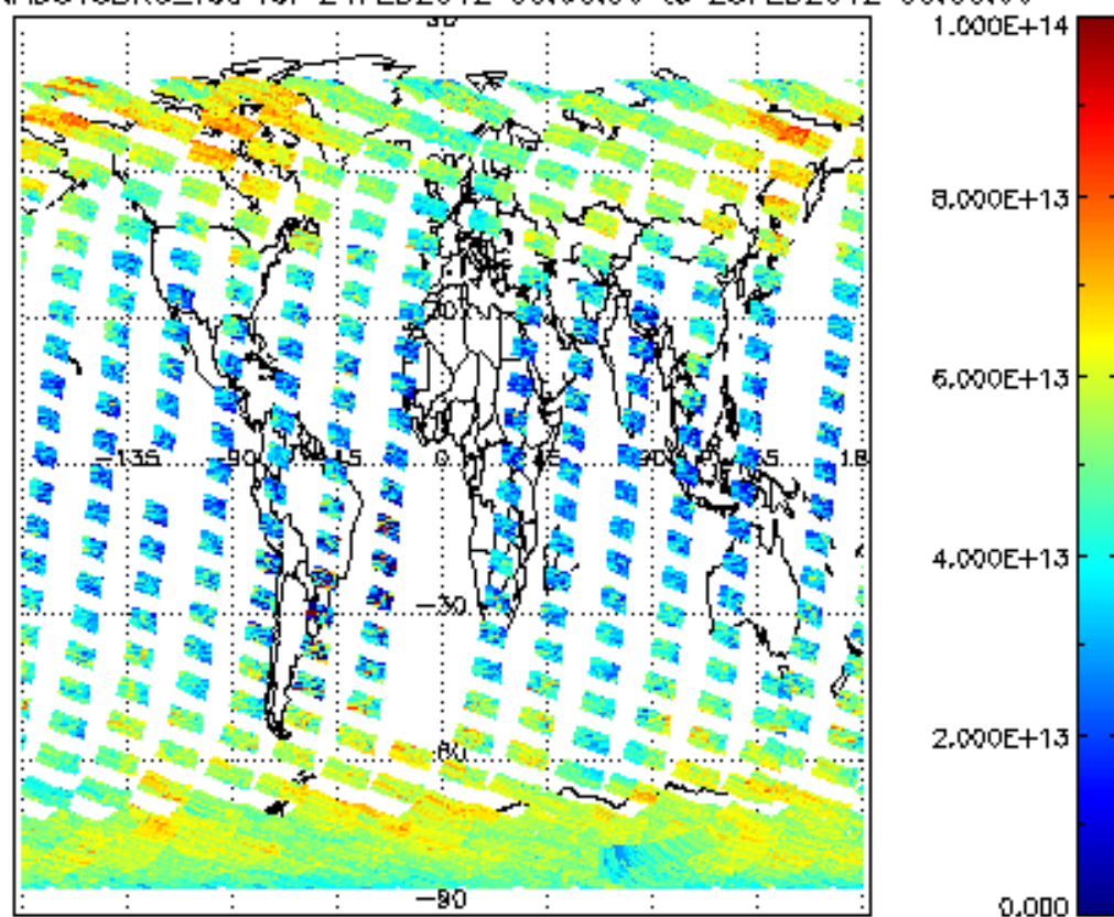
SCIOL2P_NADUV3BRO_vcd for 24FEB2012 00:00:00 to 25FEB2012 00:00:00
