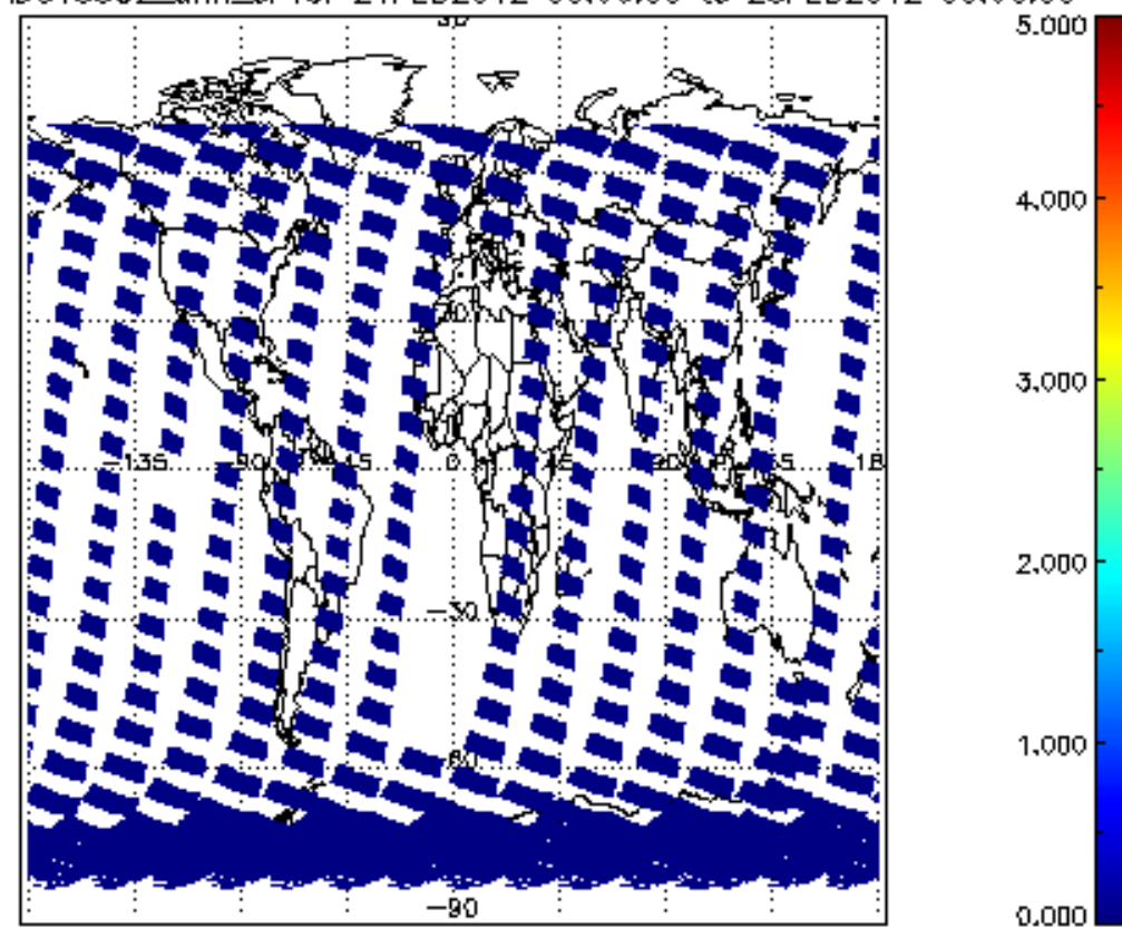
SCIOL2P_NADUV5S02_amf_cl for 24FEB2012 00:00:00 to 25FEB2012 00:00:00
