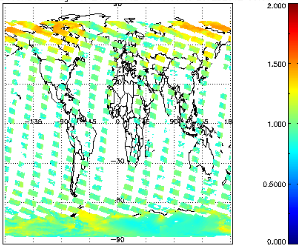
SCIOL2P_NADUV8H20_amf_gr for 24FEB2012 00:00:00 to 25FEB2012 00:00:00
