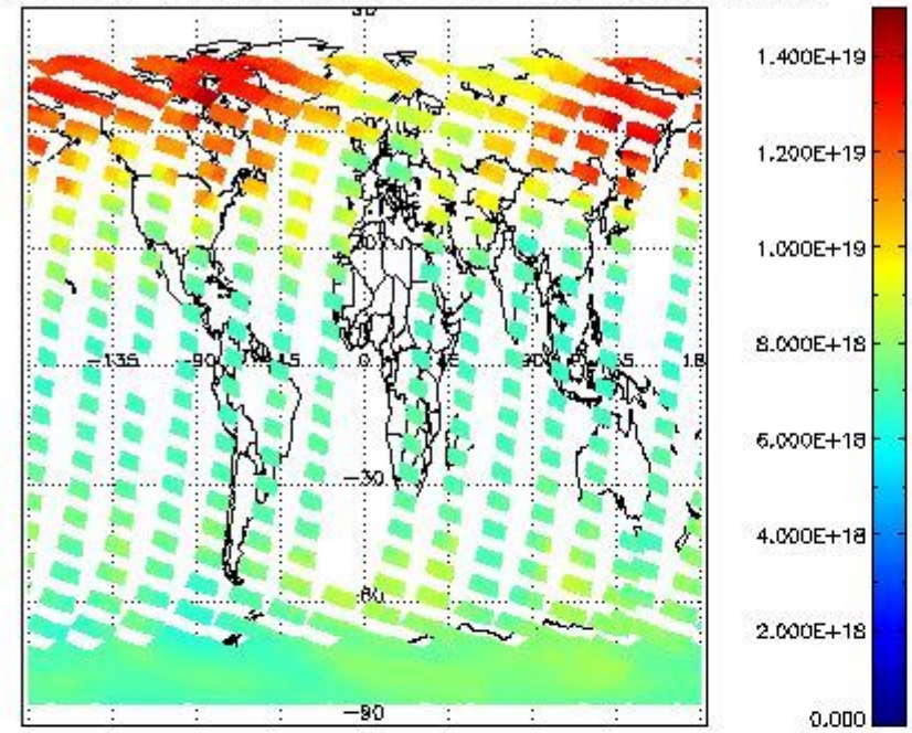
SCIOL2P_NADUV003_vcd for 24FEB2012 00:00:00 to 25FEB2012 00:00:00
