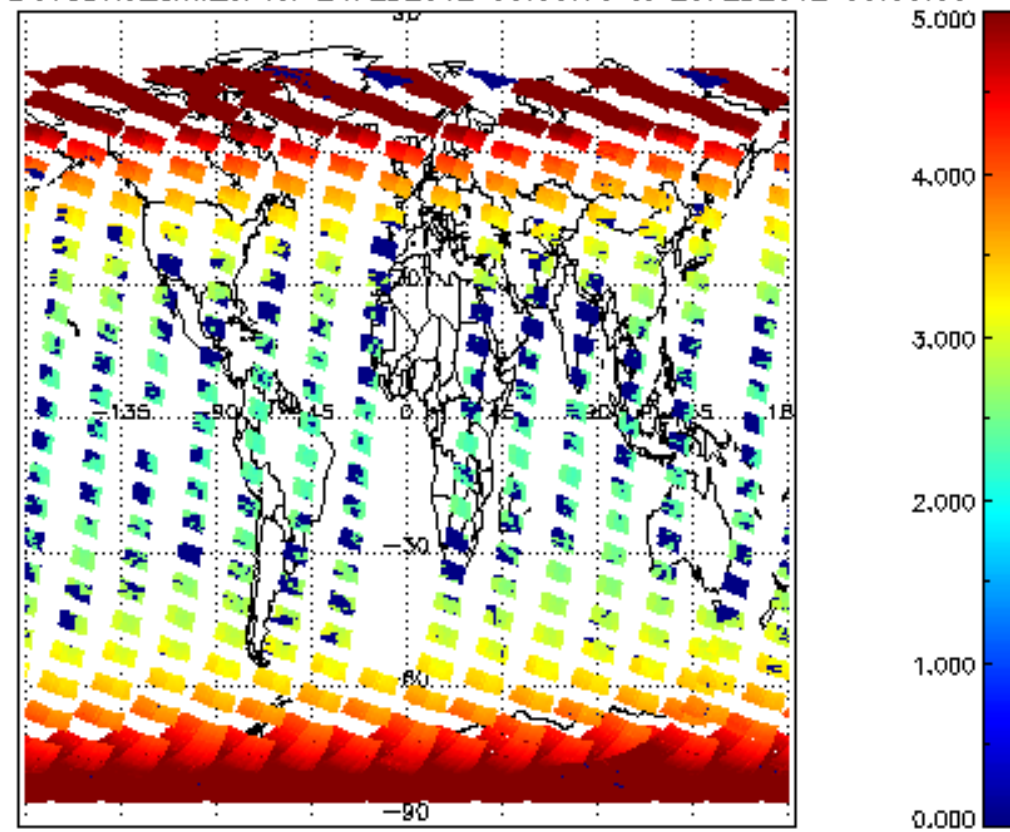
SCIOL2P_NADUV3BRO_amf_cl for 24FEB2012 00:00:00 to 25FEB2012 00:00:00
