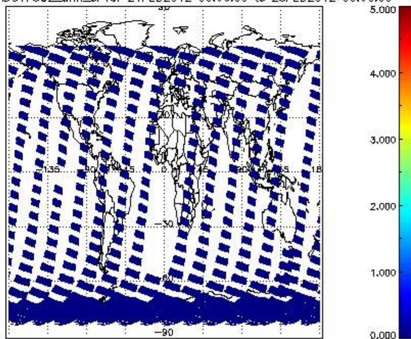
SCIOL2P_NADUV7S02_amf_cl for 24FEB2012 00:00:00 to 25FEB2012 00:00:00
