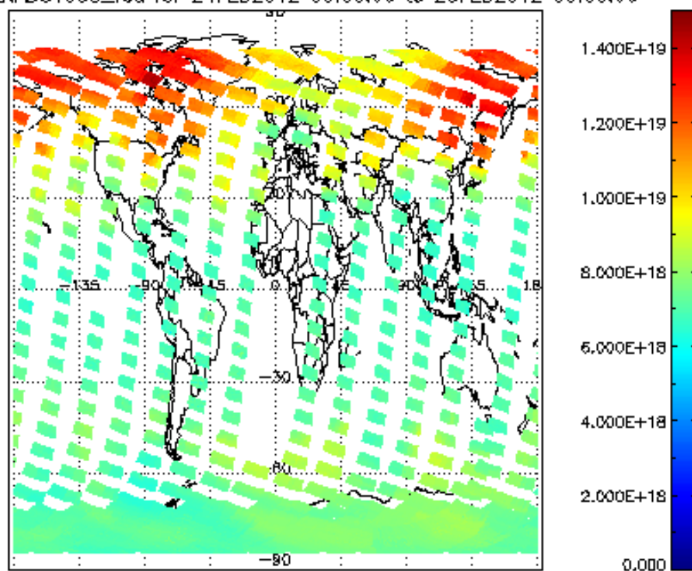
SCIOL2P_NADUV003_vcd for 24FEB2012 00:00:00 to 25FEB2012 00:00:00
