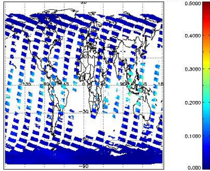
SCIOL2P_NADUV8H2O_vcd_err for 24FEB2012 00:00:00 to 25FEB2012 00:00:00
