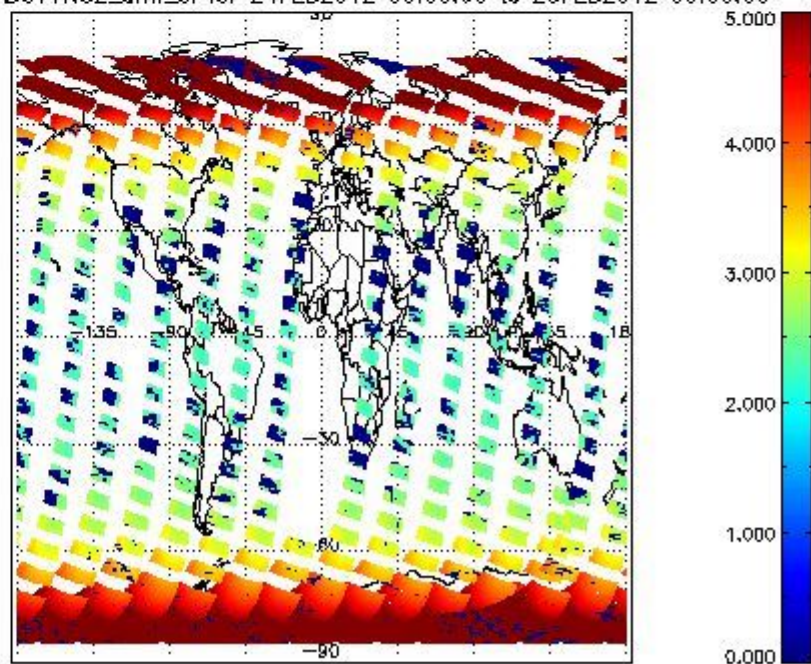
SCIOL2P_NADUV1N02_amf_cl for 24FEB2012 00:00:00 to 25FEB2012 00:00:00
