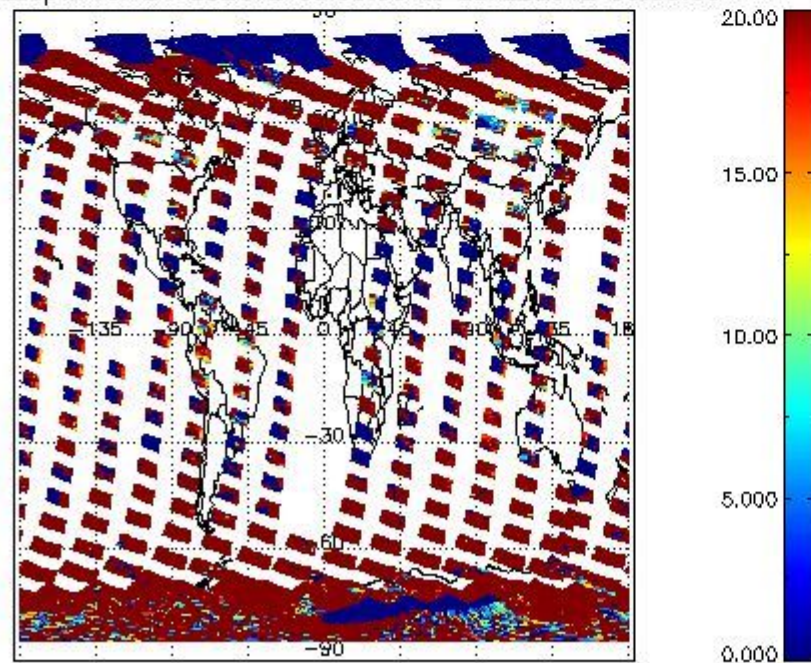
cL_opt_depth for 24FEB2012 00:00:00 to 25FEB2012 00:00:00
