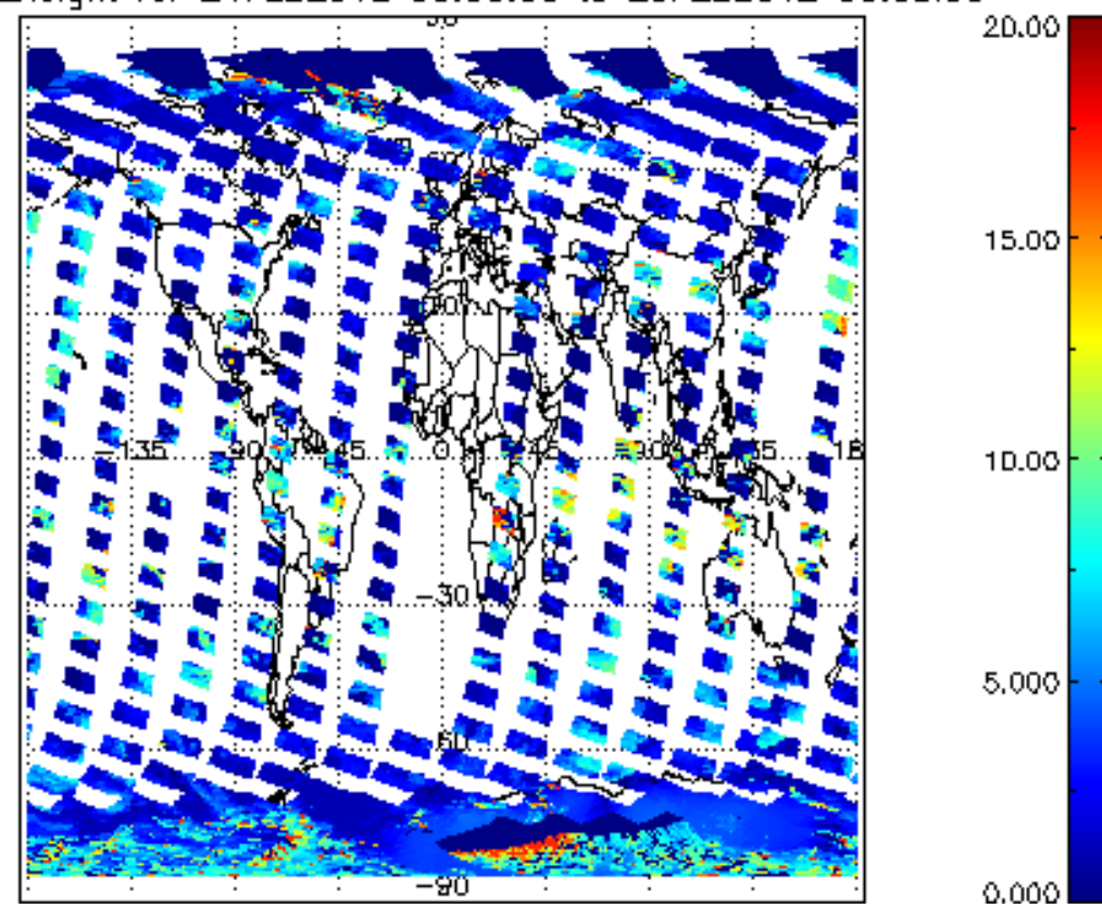
cl_top_height for 24FEB2012 00:00:00 to 25FEB2012 00:00:00
