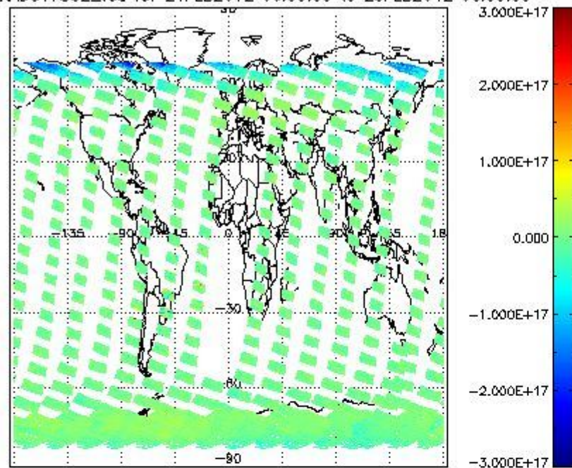
SCIOL2P_NADUV7S02_vcd for 24FEB2012 00:00:00 to 25FEB2012 00:00:00
