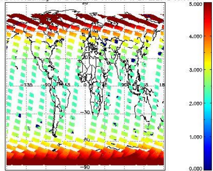
SCIOL2P_NADUV003_amf_gr for 24FEB2012 00:00:00 to 25FEB2012 00:00:00
