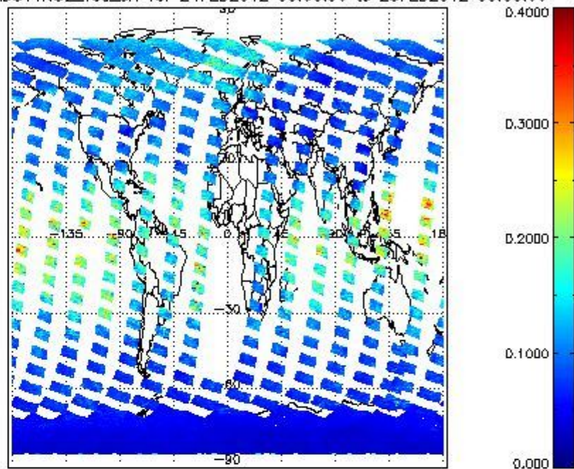
SCIOL2P_NADUV1N02_vcd_err for 24FEB2012 00:00:00 to 25FEB2012 00:00:00
