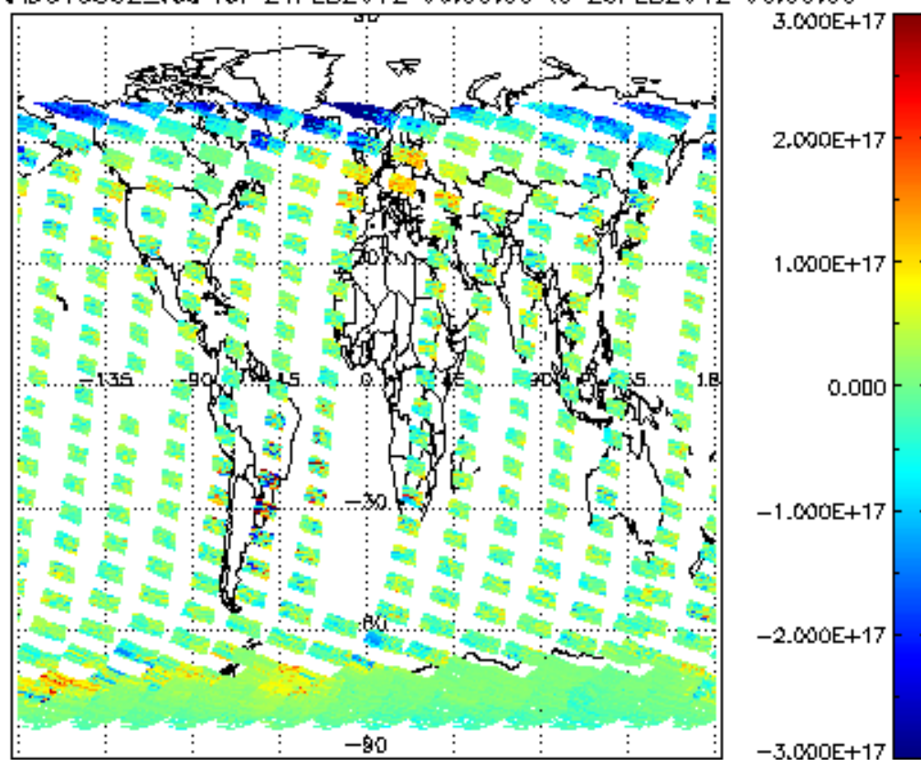
SCIOL2P_NADUV5S02_vcd for 24FEB2012 00:00:00 to 25FEB2012 00:00:00
