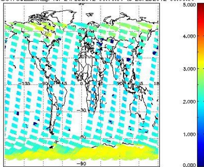
SCIOL2P_NADUV7S02_amf_gr for 24FEB2012 00:00:00 to 25FEB2012 00:00:00
