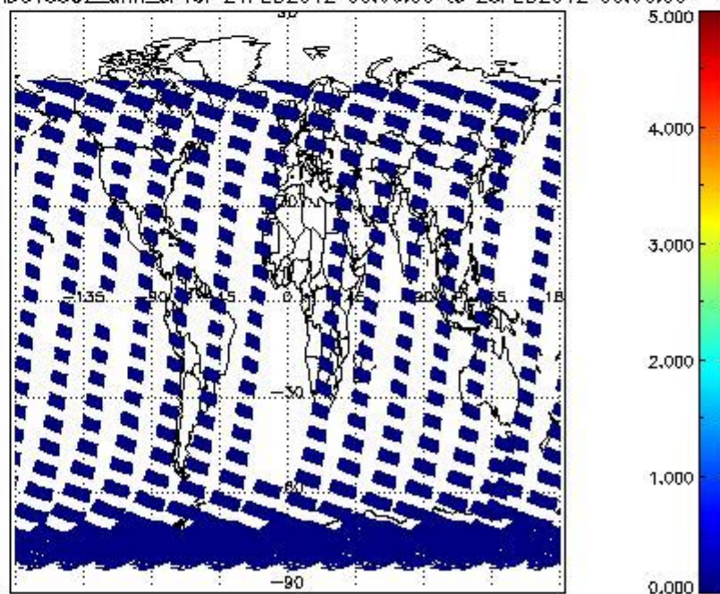
SCIOL2P_NADUV5S02_amf_cl for 24FEB2012 00:00:00 to 25FEB2012 00:00:00
