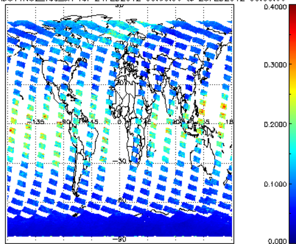
SCIOL2P_NADUV1N02_vcd_err for 24FEB2012 00:00:00 to 25FEB2012 00:00:00
