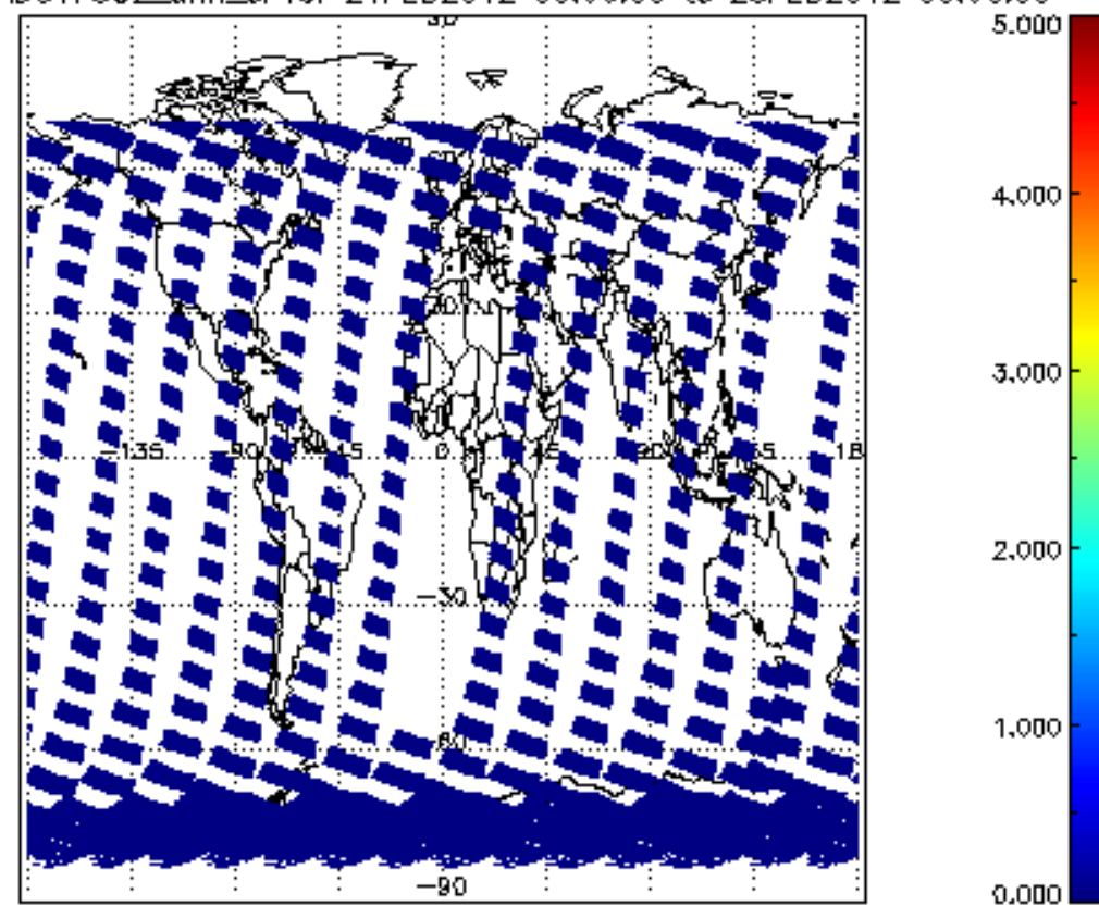
SCIOL2P_NADUV7S02_amf_cl for 24FEB2012 00:00:00 to 25FEB2012 00:00:00
