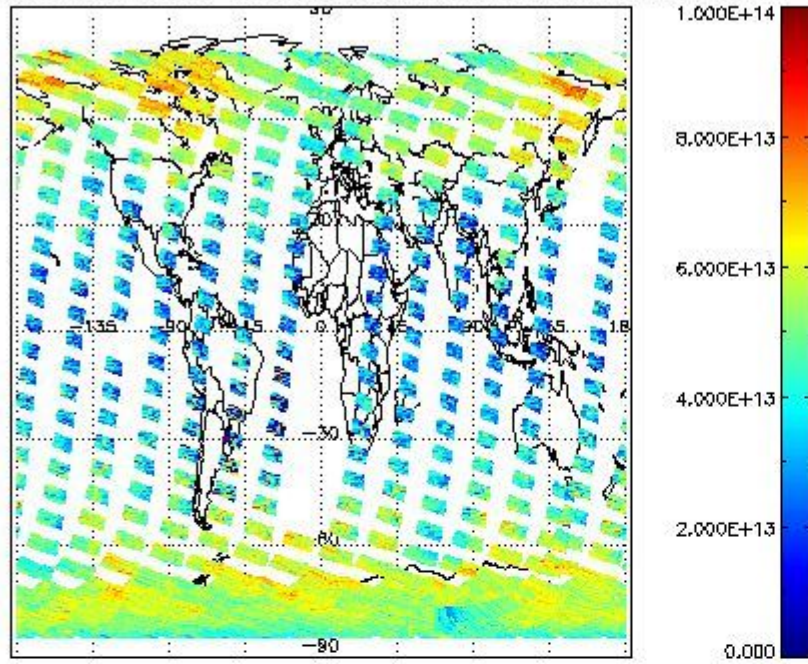
SCIOL2P_NADUV3BRO_vcd for 24FEB2012 00:00:00 to 25FEB2012 00:00:00
