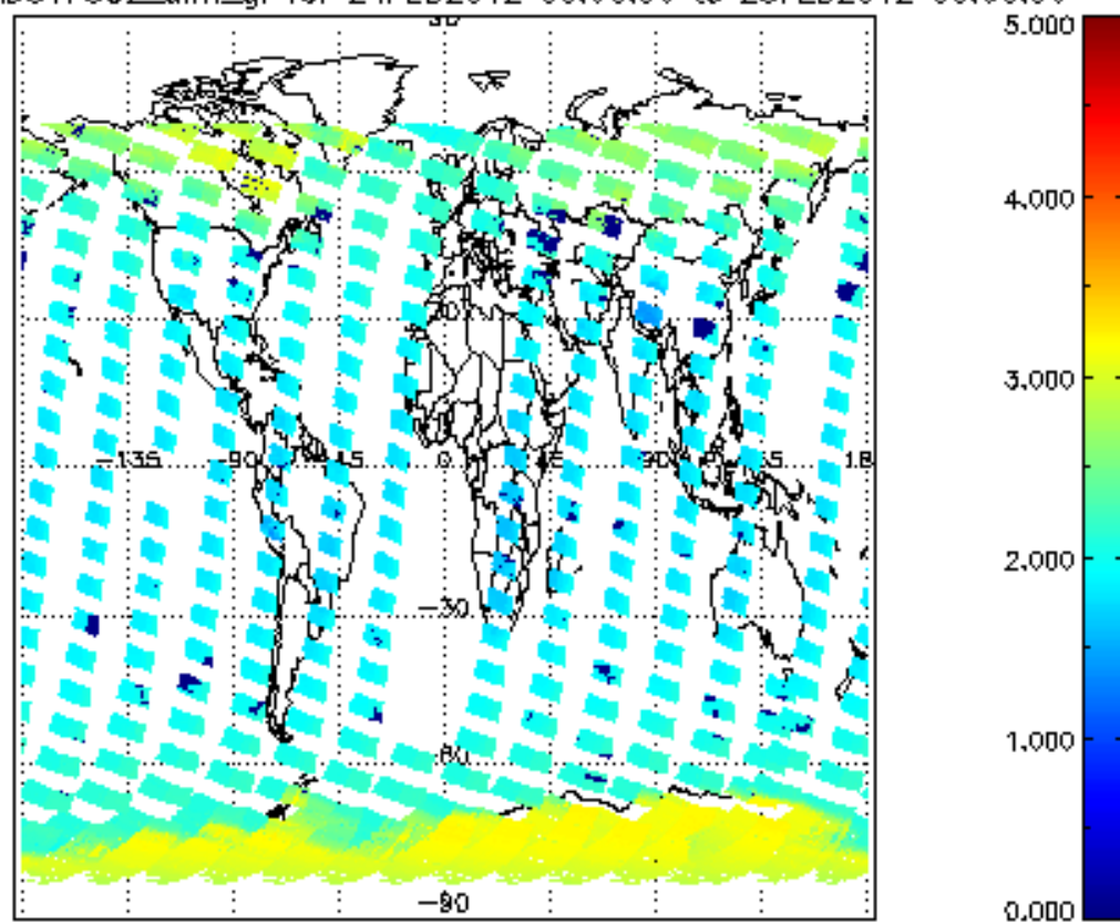
SCIOL2P_NADUV7S02_amf_gr for 24FEB2012 00:00:00 to 25FEB2012 00:00:00
