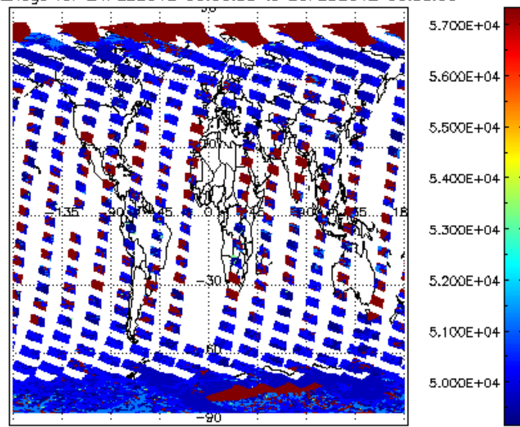
cloud_flags for 24FEB2012 00:00:00 to 25FEB2012 00:00:00
