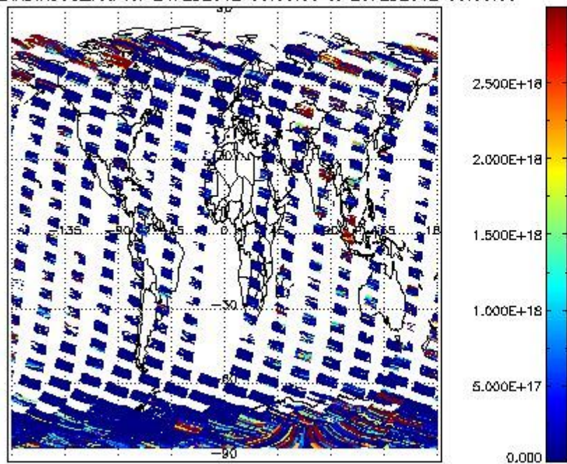
SCIO2P_NADIR3CO_vcd for 24FEB2012 00:00:00 to 25FEB2012 00:00:00
