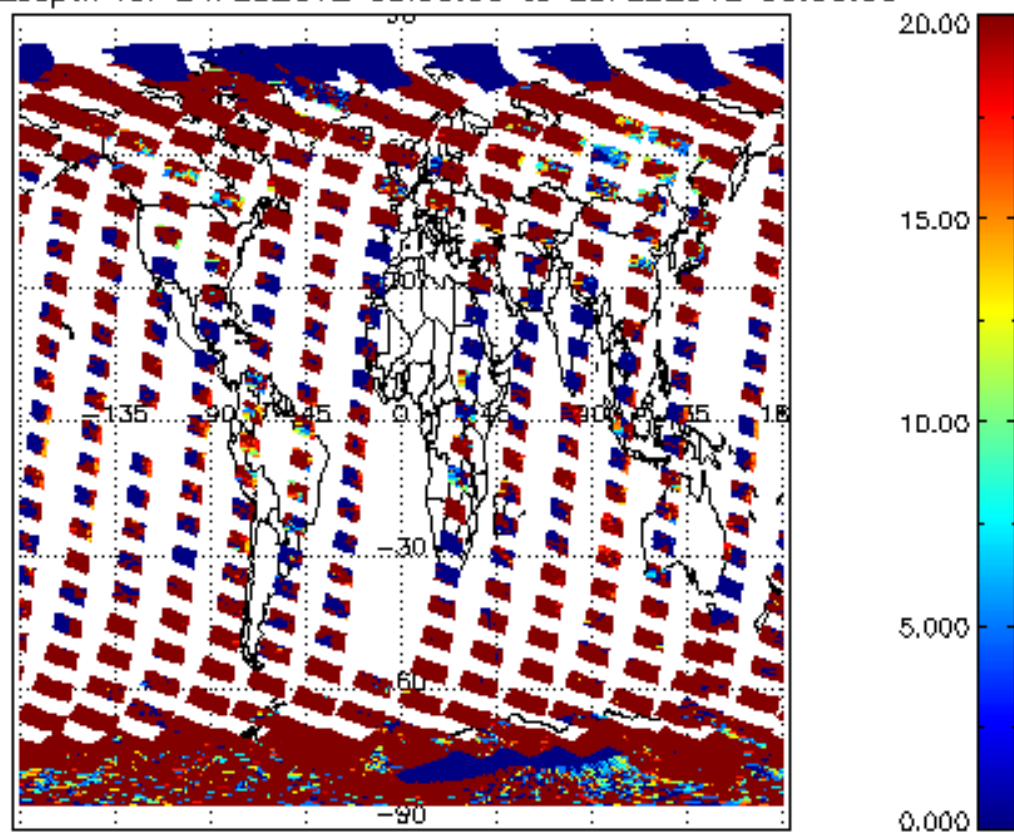
cl_opt_depth for 24FEB2012 00:00:00 to 25FEB2012 00:00:00
