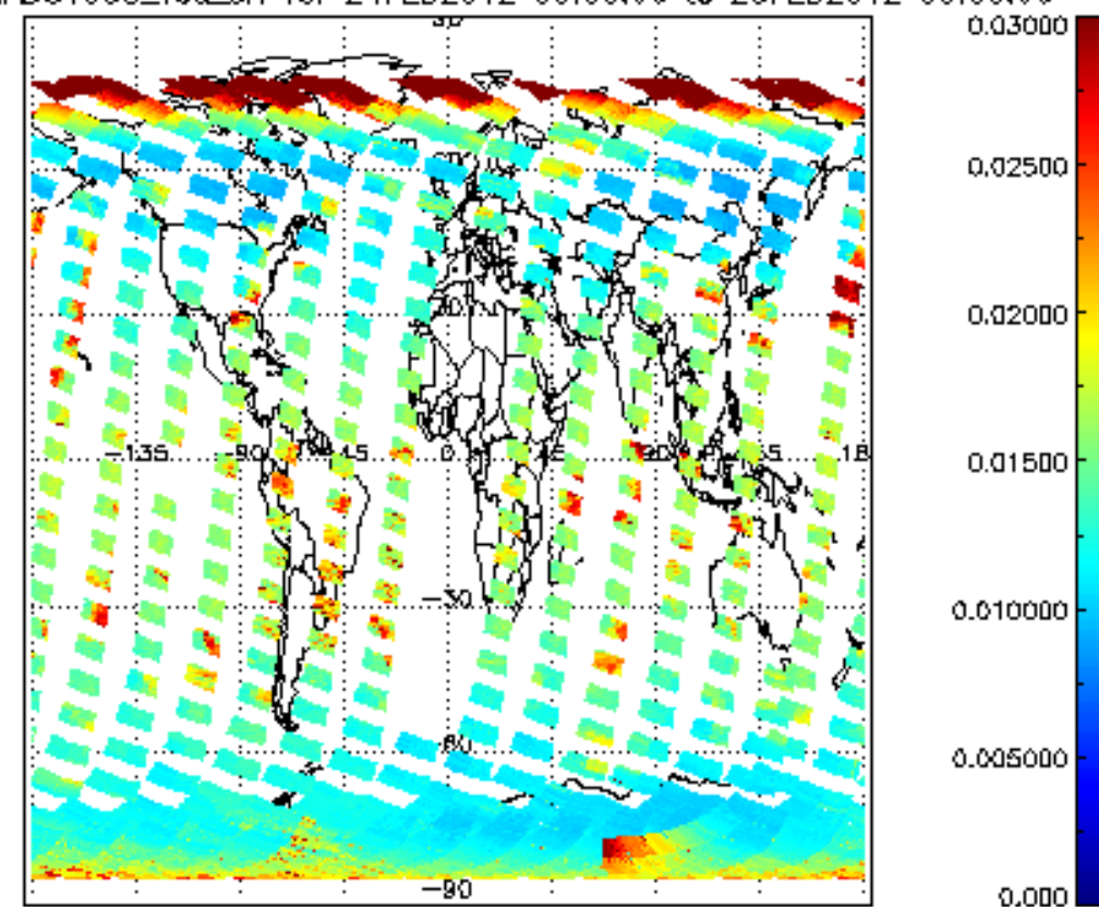
SCIOL2P_NADUV003_vcd_err for 24FEB2012 00:00:00 to 25FEB2012 00:00:00
