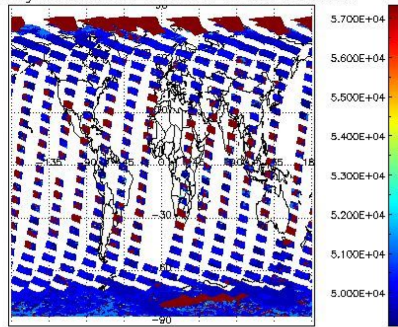
cloud_flags for 24FEB2012 00:00:00 to 25FEB2012 00:00:00
