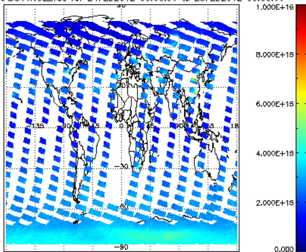
SCIOL2P_NADUV1N02_vcd for 24FEB2012 00:00:00 to 25FEB2012 00:00:00
