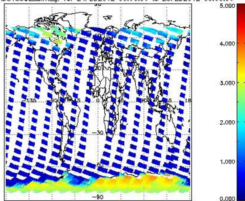
SCIOL2P_NADUV5S02_amf_gr for 24FEB2012 00:00:00 to 25FEB2012 00:00:00
