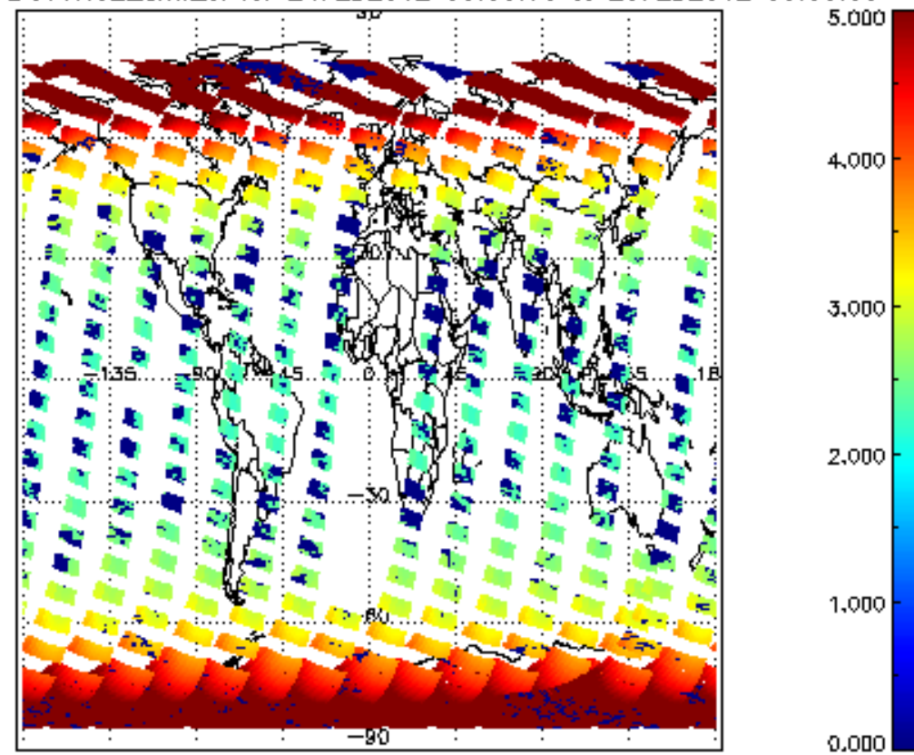
SCIOL2P_NADUV1N02_amf_cl for 24FEB2012 00:00:00 to 25FEB2012 00:00:00
