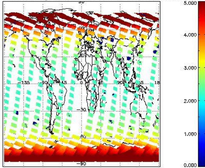
SCIOL2P_NADUV3BRO_amf_gr for 24FEB2012 00:00:00 to 25FEB2012 00:00:00
