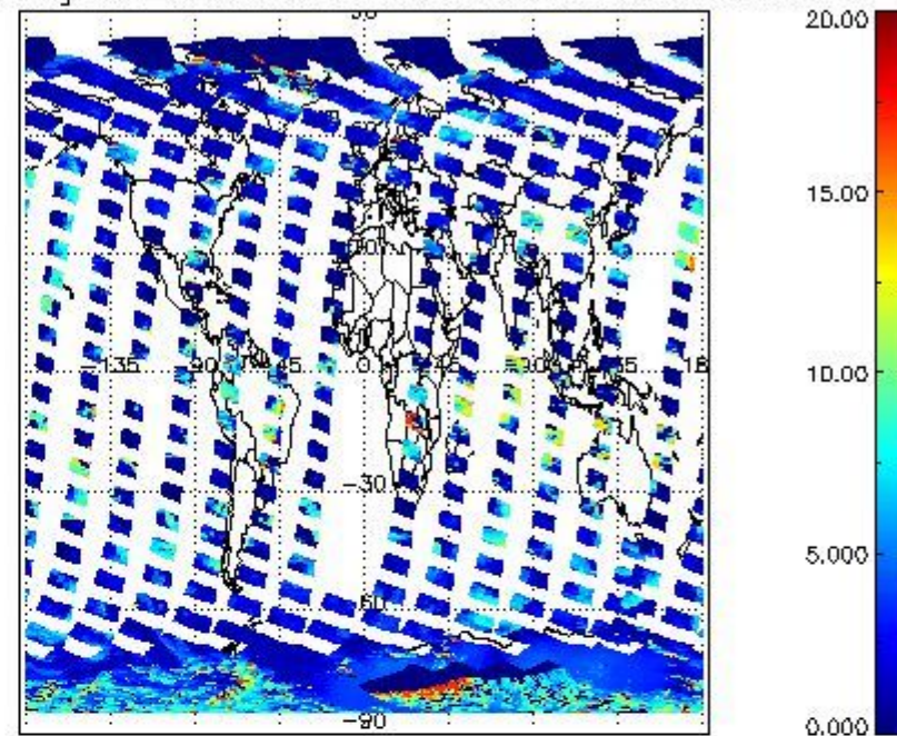
cL_top_height for 24FEB2012 00:00:00 to 25FEB2012 00:00:00
