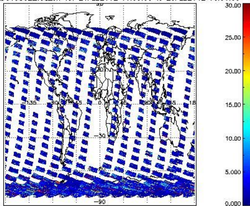
SCIOL2P_NADUV5S02_vcd_err for 24FEB2012 00:00:00 to 25FEB2012 00:00:00
