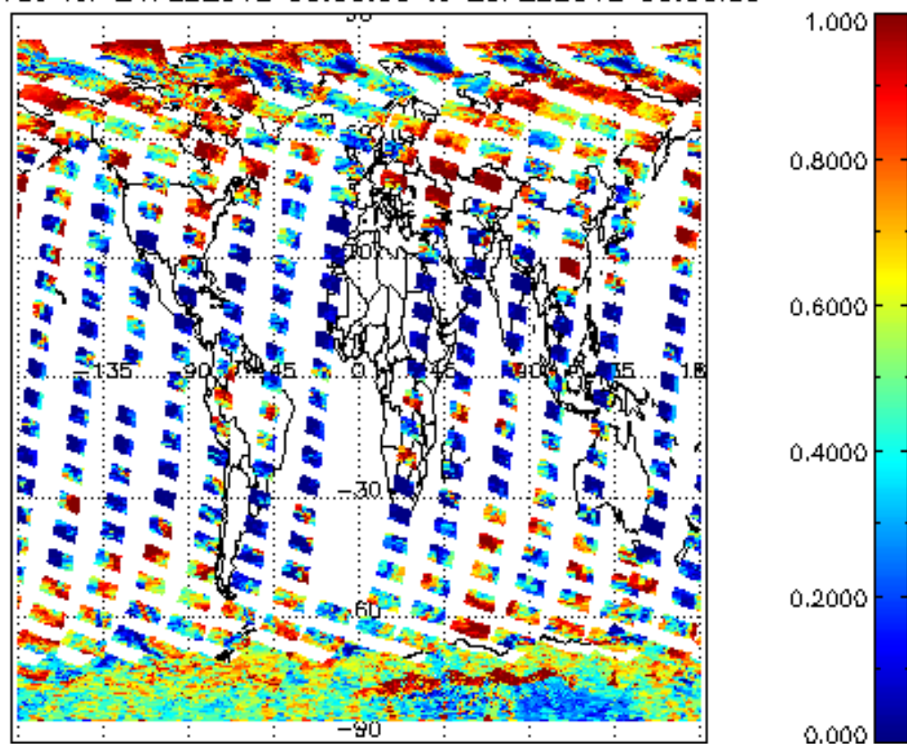
cl_frac for 24FEB2012 00:00:00 to 25FEB2012 00:00:00
