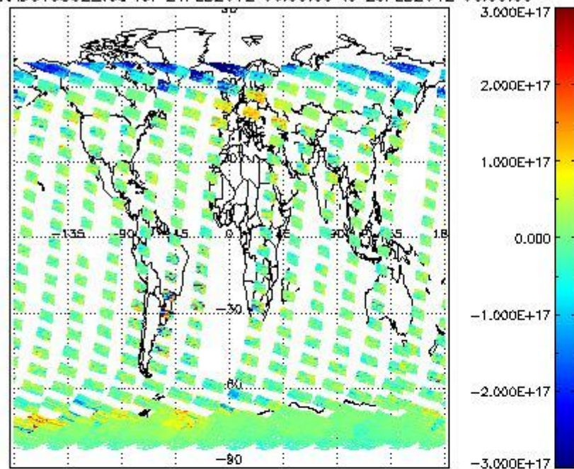
SCIOL2P_NADUV5S02_vcd for 24FEB2012 00:00:00 to 25FEB2012 00:00:00
