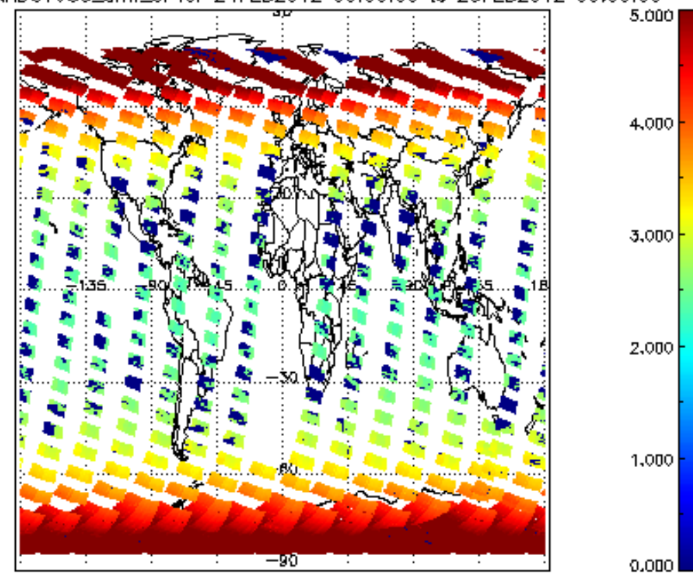
SCIOL2P_NADUV003_amf_cl for 24FEB2012 00:00:00 to 25FEB2012 00:00:00
