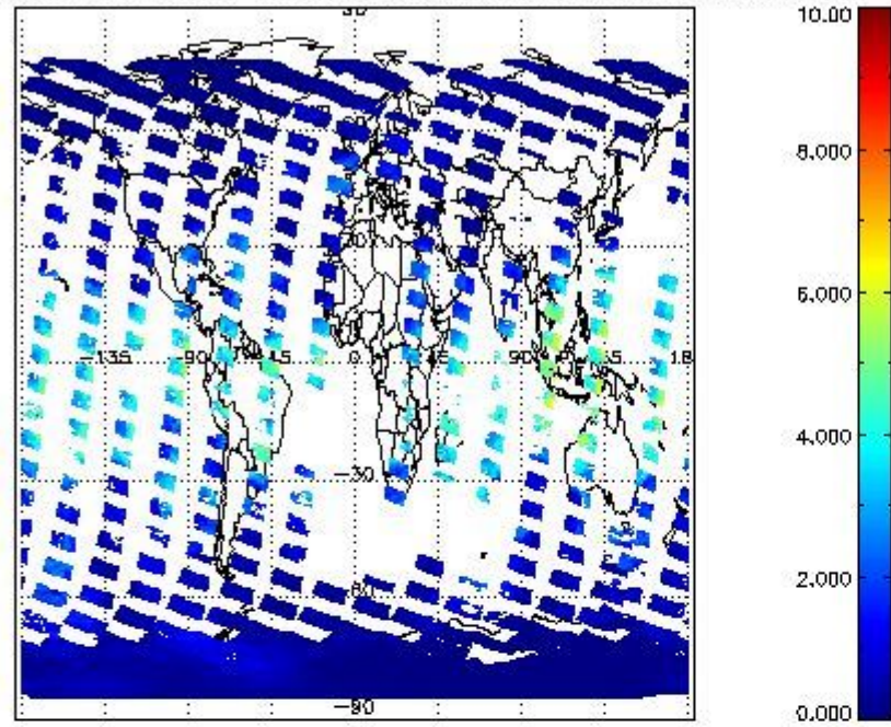
SCIOL2P_NADUV8H2O_vcd for 24FEB2012 00:00:00 to 25FEB2012 00:00:00
