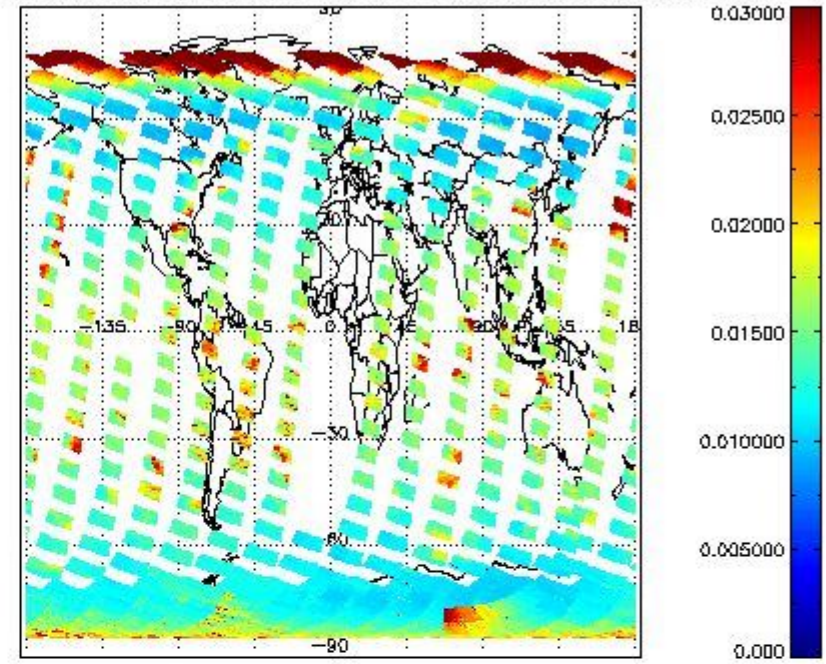
SCIOL2P_NADUV003_vcd_err for 24FEB2012 00:00:00 to 25FEB2012 00:00:00
