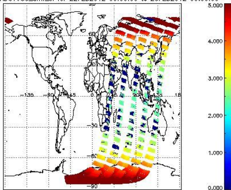
SCIOL2P_NADUV003_amf_cl for 22FEB2012 00:00:00 to 23FEB2012 00:00:00
