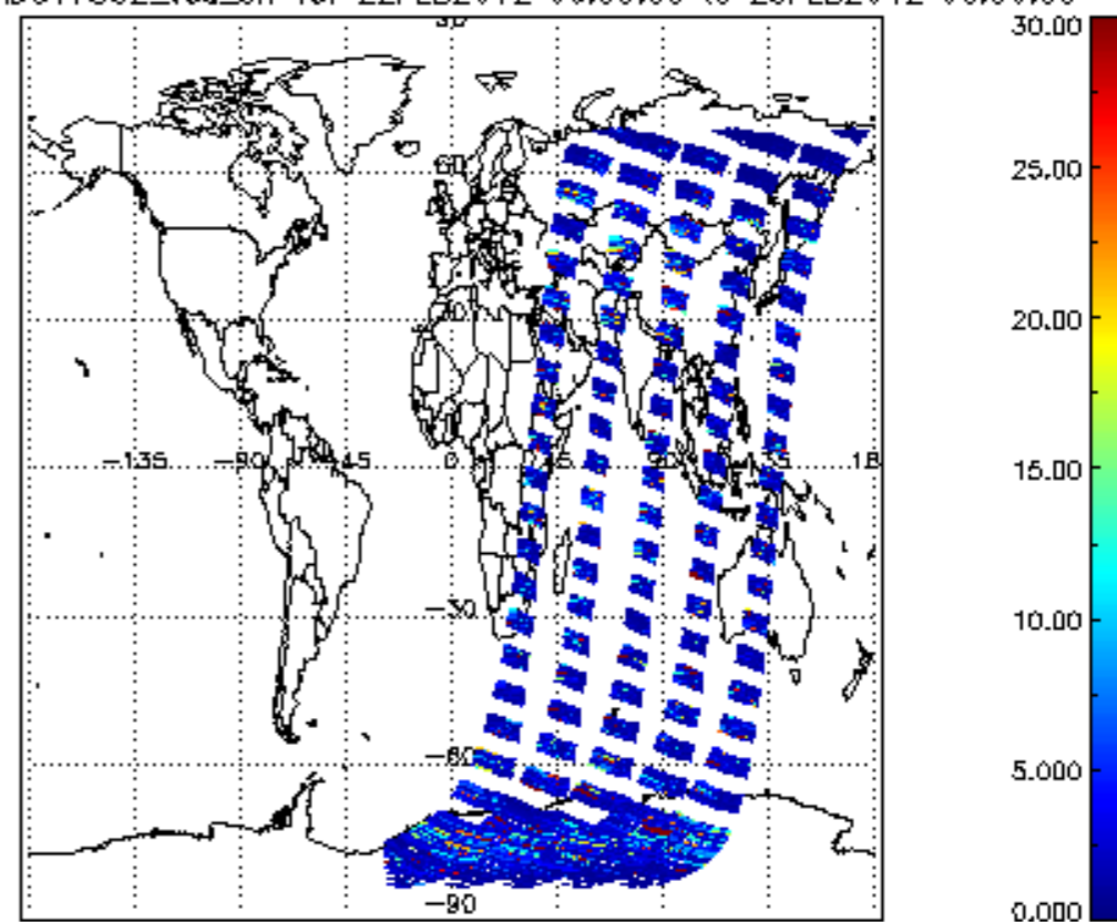
SCIOL2P_NADUV7S02_vcd_err for 22FEB2012 00:00:00 to 23FEB2012 00:00:00
