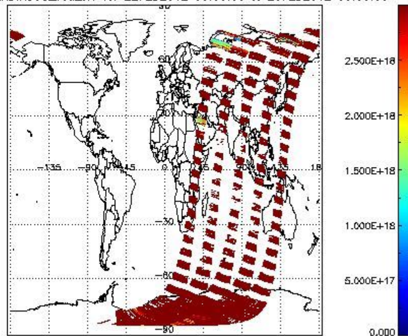
SCIDL2P_NADIR3CO_vcd_err for 22FEB2012 00:00:00 to 23FEB2012 00:00:00
