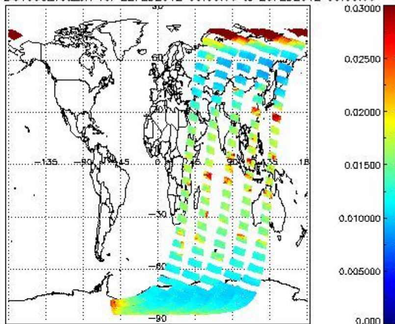
SCIOL2P_NADUV003_vcd_err for 22FEB2012 00:00:00 to 23FEB2012 00:00:00
