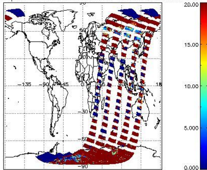
cL_opt_depth for 22FEB2012 00:00:00 to 23FEB2012 00:00:00
