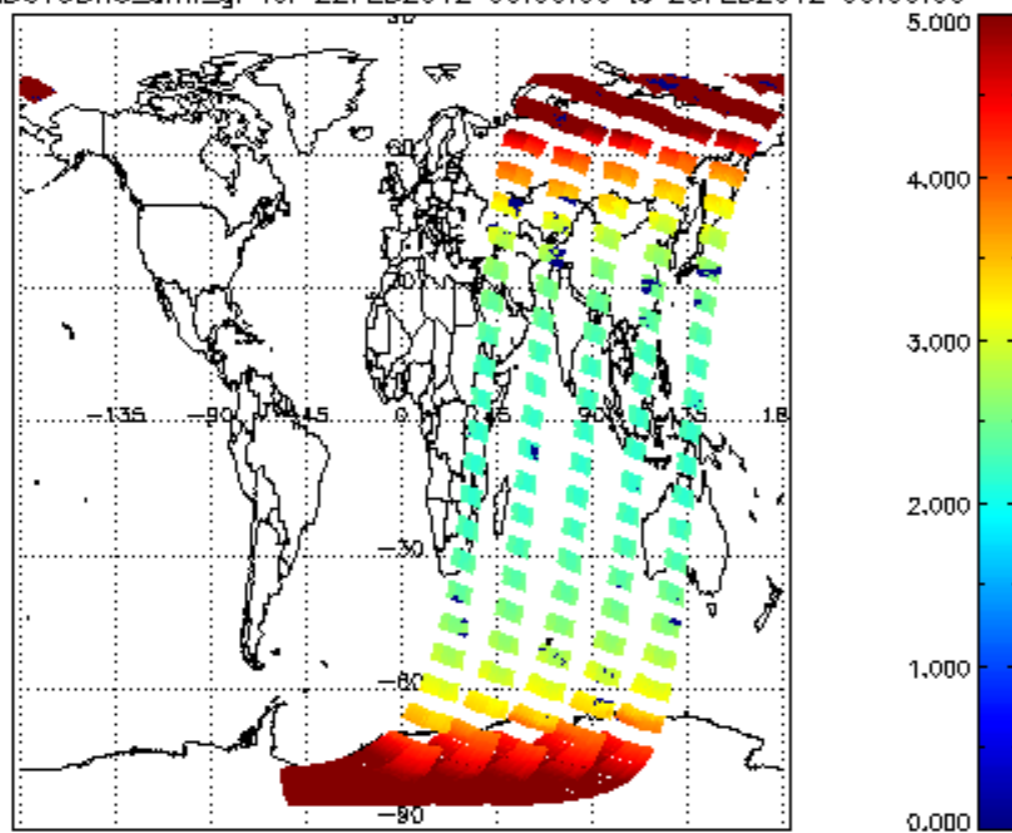
SCIOL2P_NADUV3BRO_amf_gr for 22FEB2012 00:00:00 to 23FEB2012 00:00:00
