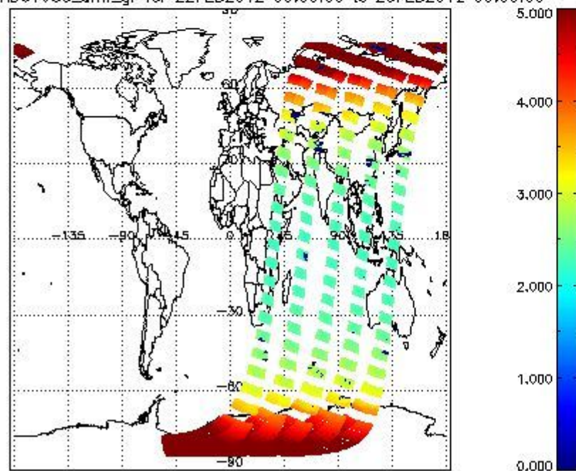
SCIOL2P_NADUV003_amf_gr for 22FEB2012 00:00:00 to 23FEB2012 00:00:00
