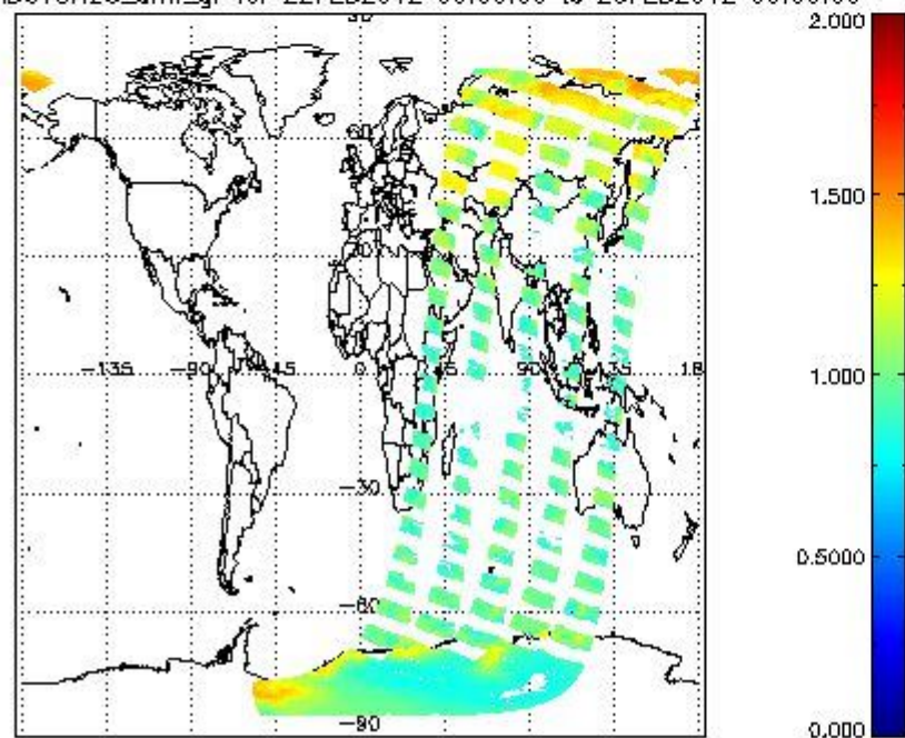
SCIOL2P_NADUV8H2O_amf_gr for 22FEB2012 00:00:00 to 23FEB2012 00:00:00
