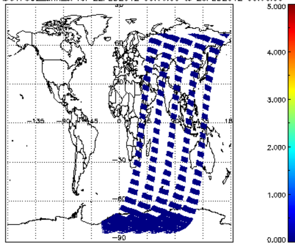
SCIOL2P_NADUV7S02_amf_cl for 22FEB2012 00:00:00 to 23FEB2012 00:00:00
