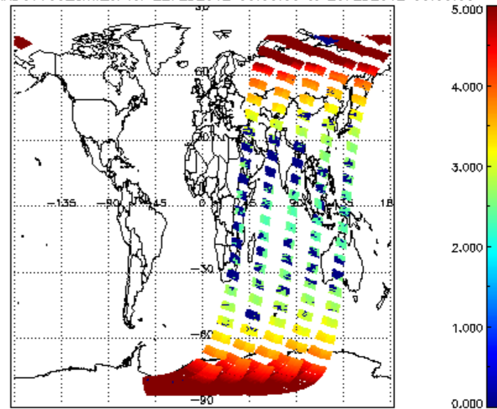
SCIOL2P_NADUV003_amf_cl for 22FEB2012 00:00:00 to 23FEB2012 00:00:00
