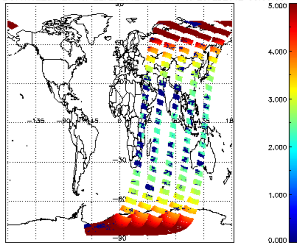
SCIOL2P_NADUV1N02_amf_cl for 22FEB2012 00:00:00 to 23FEB2012 00:00:00
