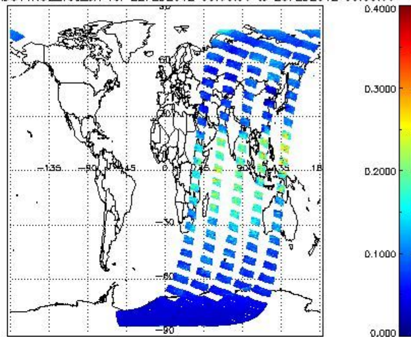
SCIOL2P_NADUV1N02_vcd_err for 22FEB2012 00:00:00 to 23FEB2012 00:00:00
