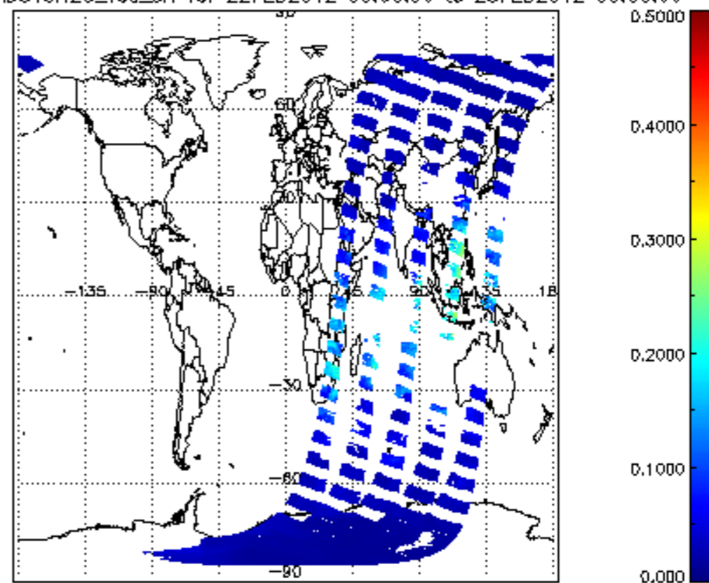
SCIOL2P_NADUV8H2O_vcd_err for 22FEB2012 00:00:00 to 23FEB2012 00:00:00
