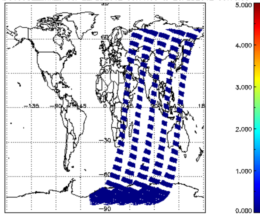
SCIOL2P_NADUV5S02_amf_cl for 22FEB2012 00:00:00 to 23FEB2012 00:00:00
