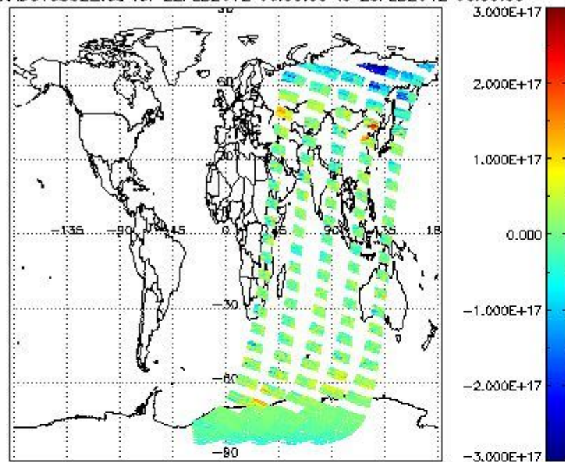
SCIOL2P_NADUV5SO2_vcd for 22FEB2012 00:00:00 to 23FEB2012 00:00:00
