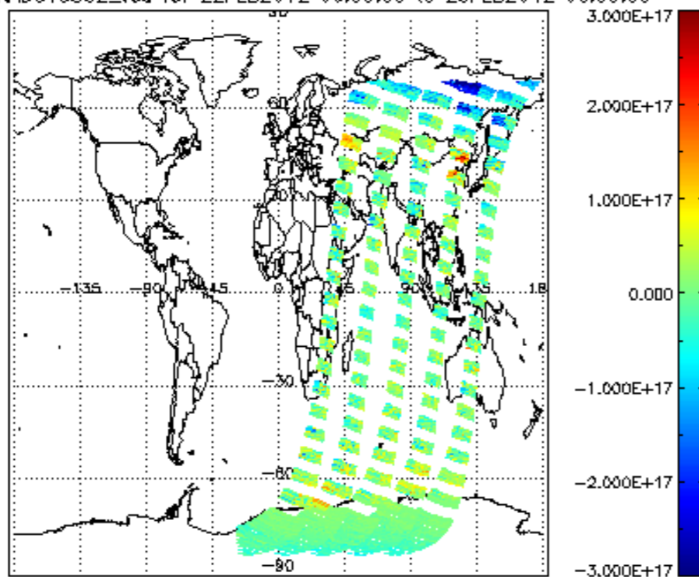
SCIOL2P_NADUV5S02_vcd for 22FEB2012 00:00:00 to 23FEB2012 00:00:00
