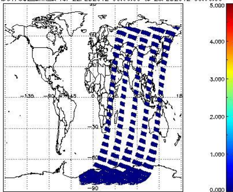
SCIOL2P_NADUV7S02_amf_cl for 22FEB2012 00:00:00 to 23FEB2012 00:00:00
