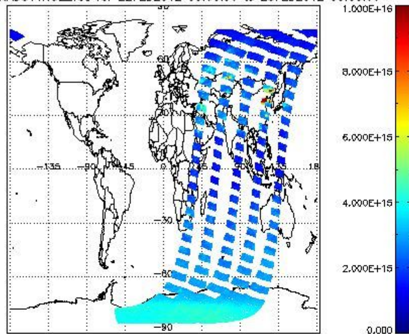
SCIOL2P_NADUV1N02_vcd for 22FEB2012 00:00:00 to 23FEB2012 00:00:00
