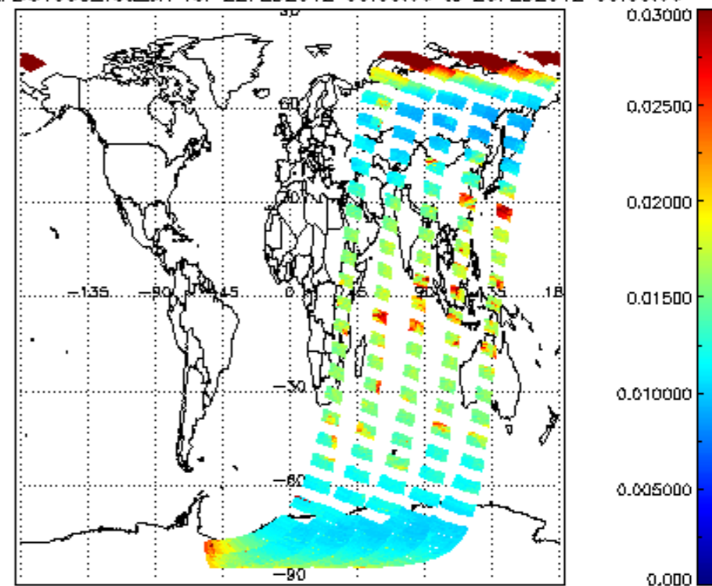
SCIOL2P_NADUV003_vcd_err for 22FEB2012 00:00:00 to 23FEB2012 00:00:00
