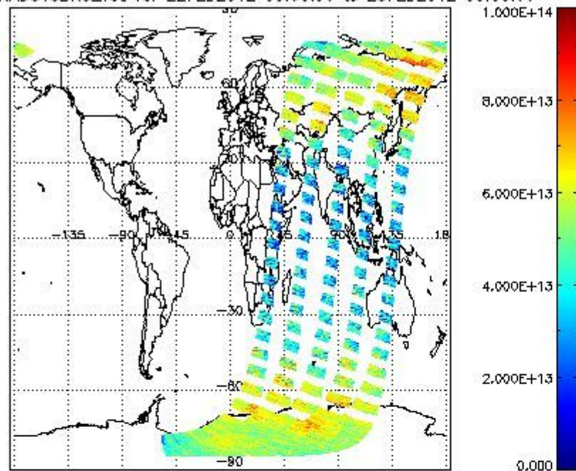
SCIOL2P_NADUV3BRO_vcd for 22FEB2012 00:00:00 to 23FEB2012 00:00:00
