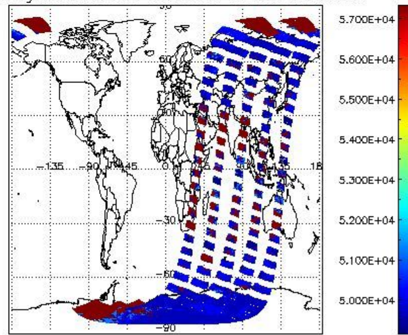
cloud_flags for 22FEB2012 00:00:00 to 23FEB2012 00:00:00
