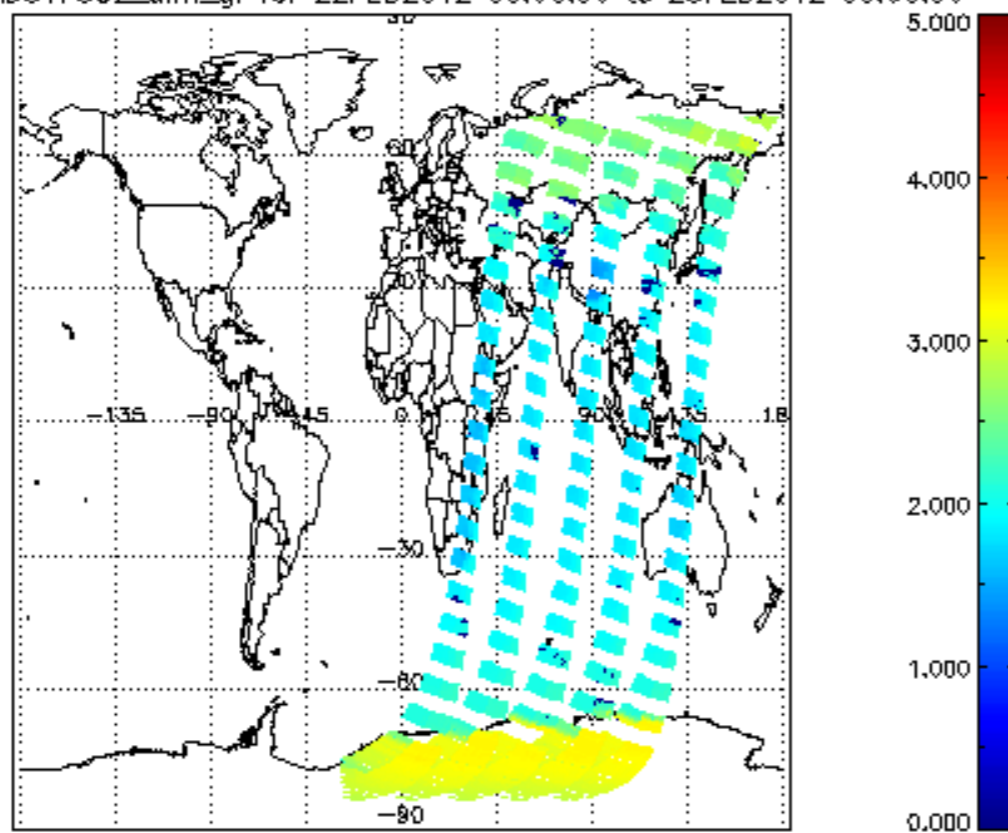
SCIOL2P_NADUV7S02_amf_gr for 22FEB2012 00:00:00 to 23FEB2012 00:00:00
