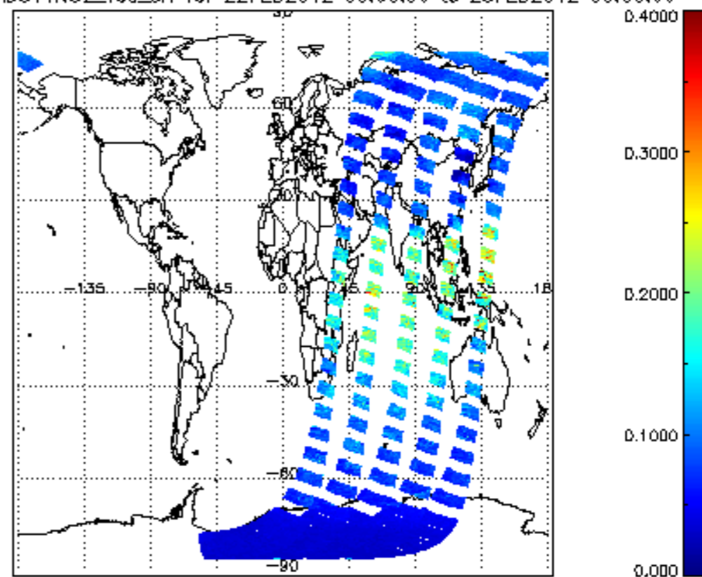
SCIOL2P_NADUV1N02_vcd_err for 22FEB2012 00:00:00 to 23FEB2012 00:00:00
