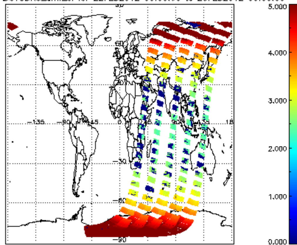
SCIOL2P_NADUV3BRO_amf_cl for 22FEB2012 00:00:00 to 23FEB2012 00:00:00
