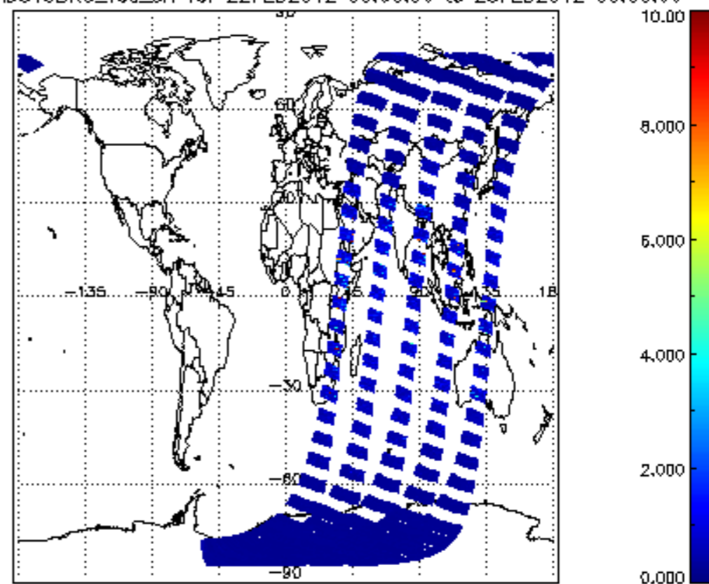
SCIOL2P_NADUV3BRO_vcd_err for 22FEB2012 00:00:00 to 23FEB2012 00:00:00
