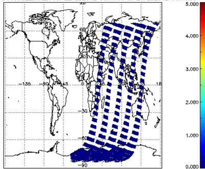
SCIOL2P_NADUV5SO2_amf_cl for 22FEB2012 00:00:00 to 23FEB2012 00:00:00
