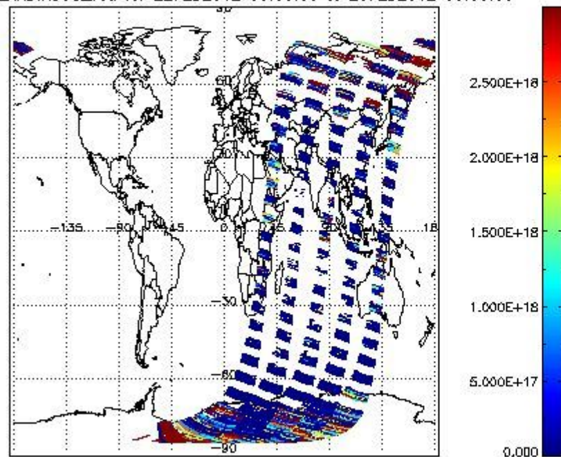
SCIDL2P_NADIR3CO_vcd for 22FEB2012 00:00:00 to 23FEB2012 00:00:00
