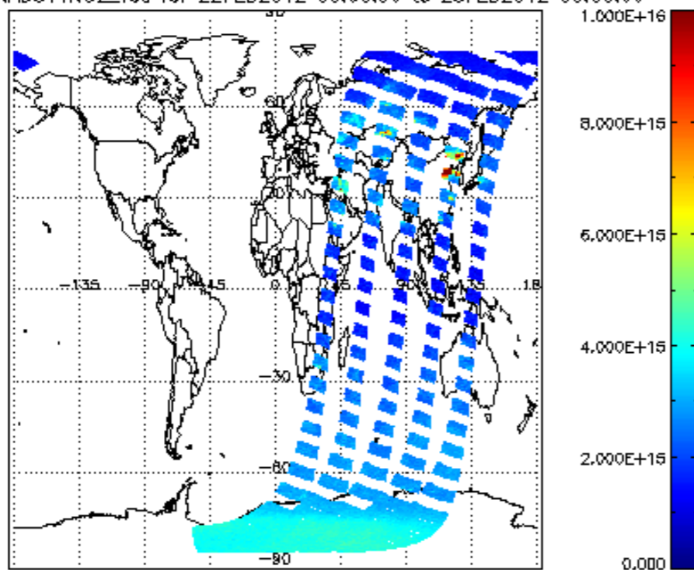
SCIOL2P_NADUV1N02_vcd for 22FEB2012 00:00:00 to 23FEB2012 00:00:00
