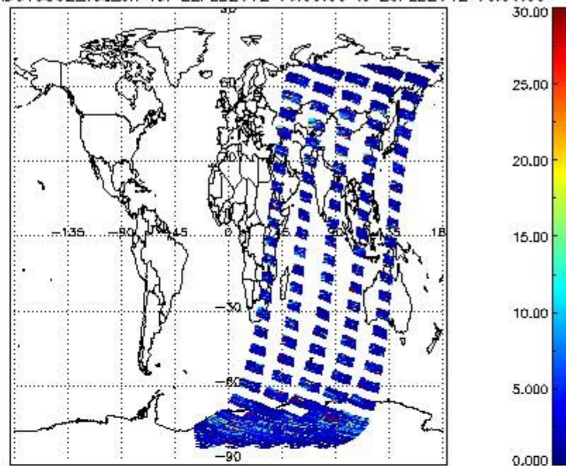
SCIOL2P_NADUV5SO2_vcd_err for 22FEB2012 00:00:00 to 23FEB2012 00:00:00
