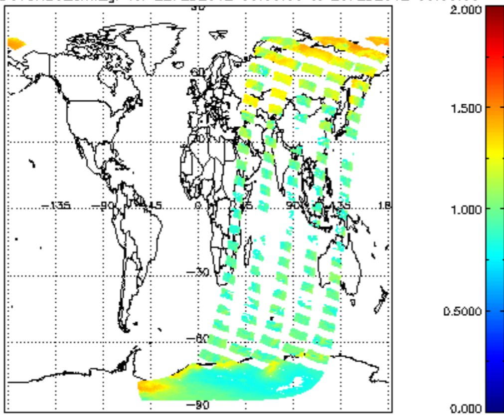
SCIOL2P_NADUV8H2O_amf_gr for 22FEB2012 00:00:00 to 23FEB2012 00:00:00
