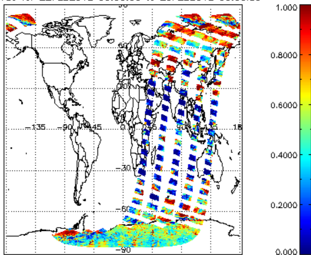
cl_frac for 22FEB2012 00:00:00 to 23FEB2012 00:00:00
