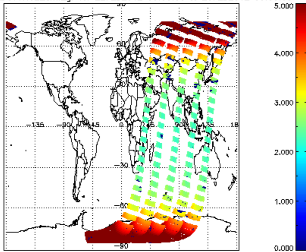
SCIOL2P_NADUV1N02_amf_gr for 22FEB2012 00:00:00 to 23FEB2012 00:00:00
