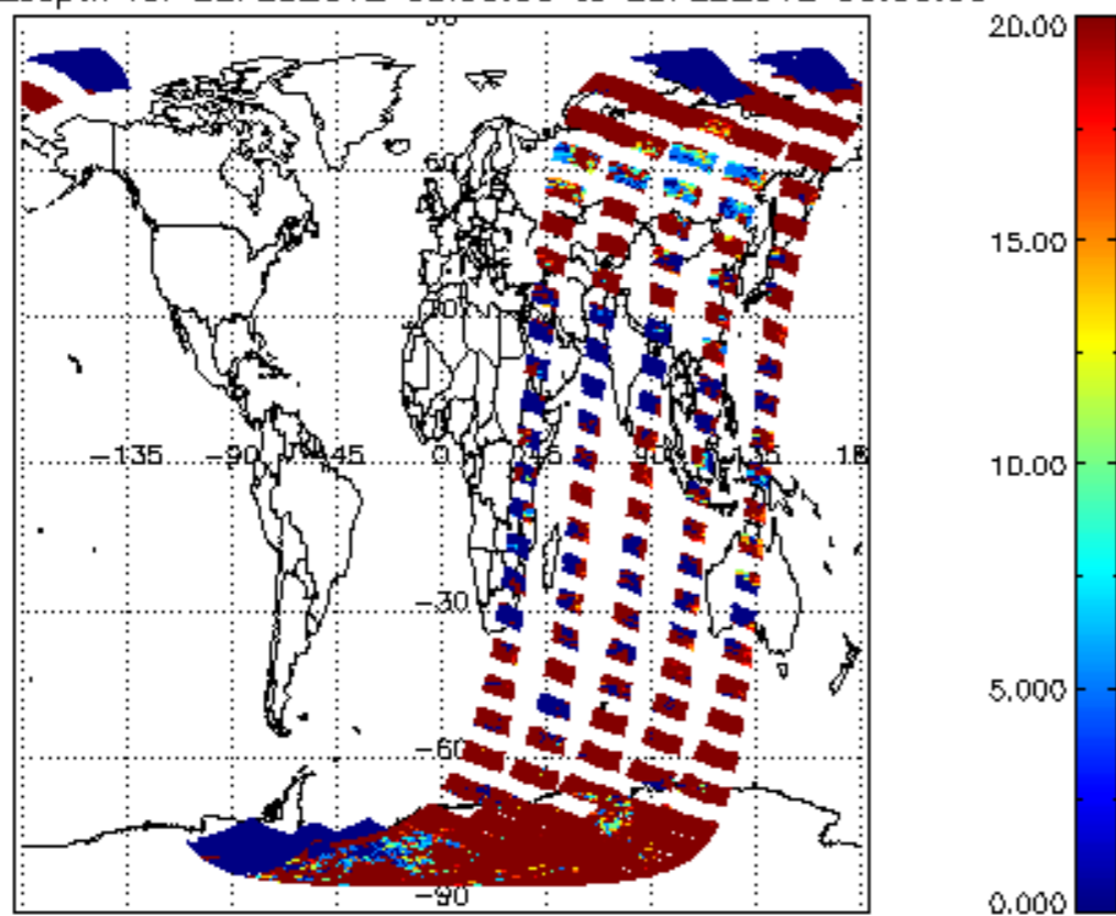
cl_opt_depth for 22FEB2012 00:00:00 to 23FEB2012 00:00:00
