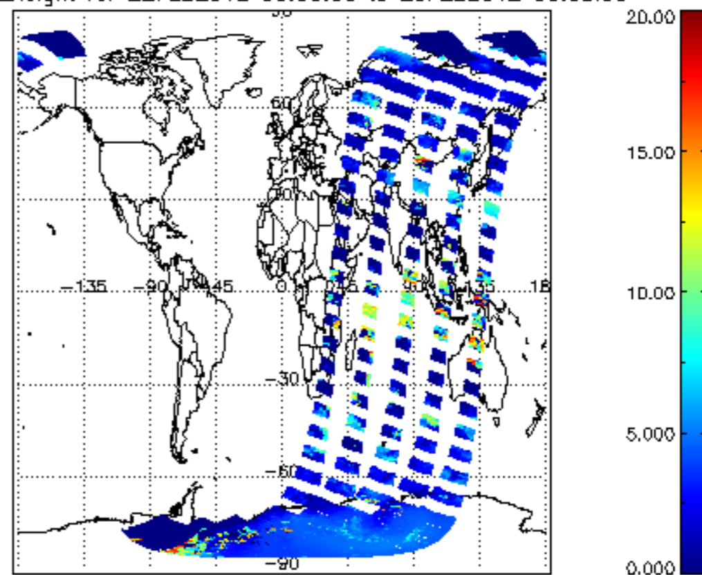
cl_top_height for 22FEB2012 00:00:00 to 23FEB2012 00:00:00
