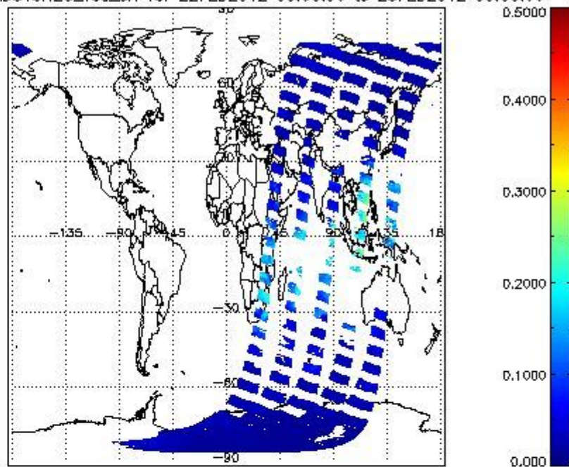
SCIOL2P_NADUV8H2O_vcd_err for 22FEB2012 00:00:00 to 23FEB2012 00:00:00
