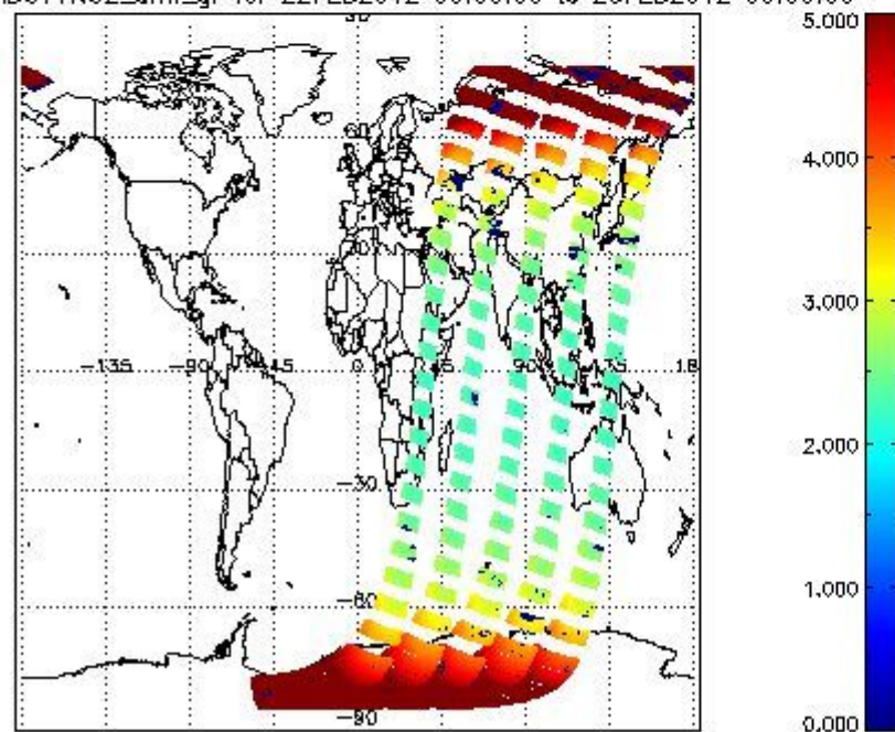
SCIOL2P_NADUV1N02_amf_gr for 22FEB2012 00:00:00 to 23FEB2012 00:00:00
