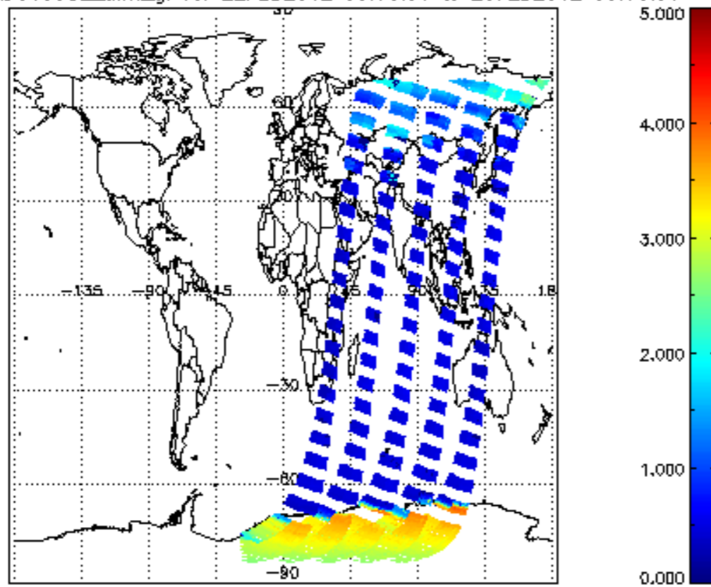
SCIOL2P_NADUV5S02_amf_gr for 22FEB2012 00:00:00 to 23FEB2012 00:00:00
