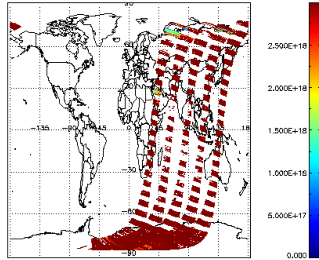
SCIOL2P_NADIR3CO_vcd_err for 22FEB2012 00:00:00 to 23FEB2012 00:00:00
