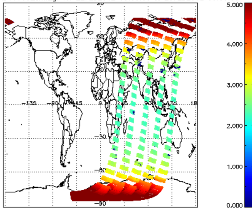
SCIOL2P_NADUV003_amf_gr for 22FEB2012 00:00:00 to 23FEB2012 00:00:00
