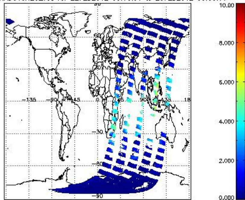
SCIOL2P_NADUV8H2O_vcd for 22FEB2012 00:00:00 to 23FEB2012 00:00:00
