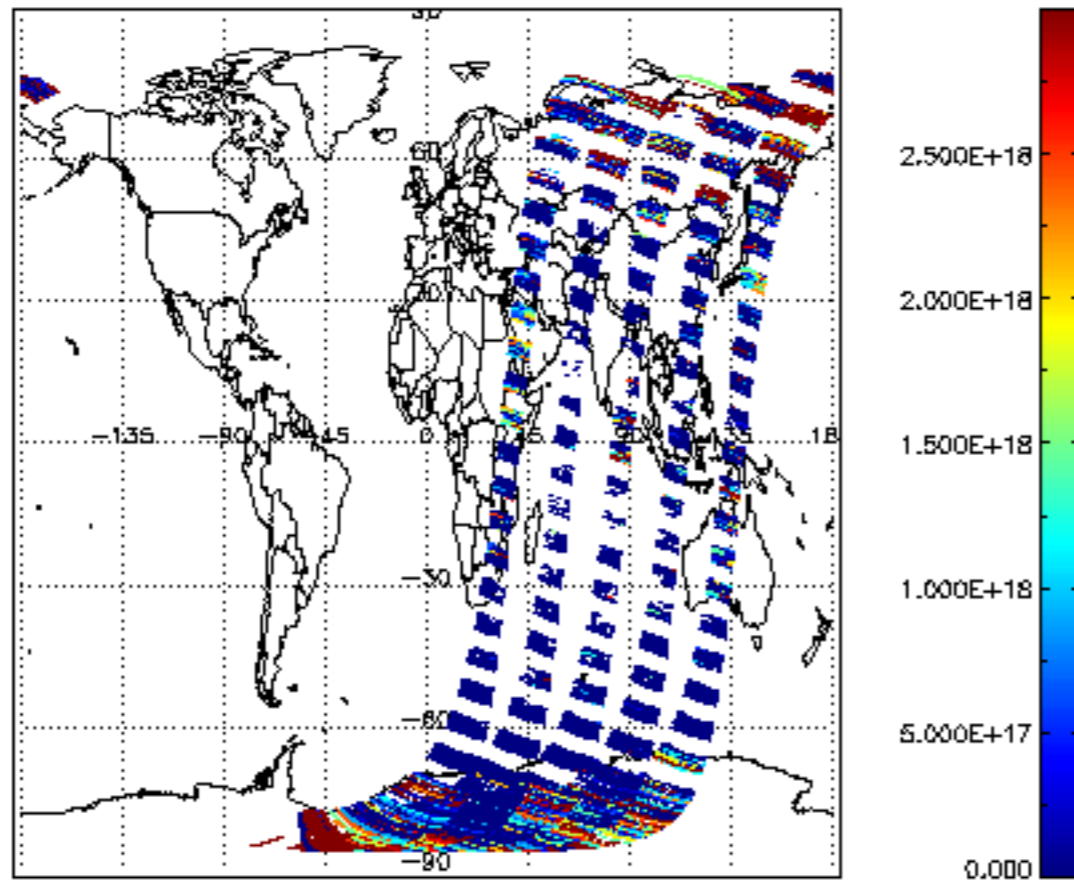
SCIOL2P_NADIR3CO_vcd for 22FEB2012 00:00:00 to 23FEB2012 00:00:00
