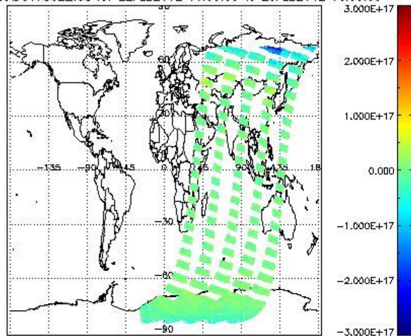
SCIOL2P_NADUV7S02_vcd for 22FEB2012 00:00:00 to 23FEB2012 00:00:00
