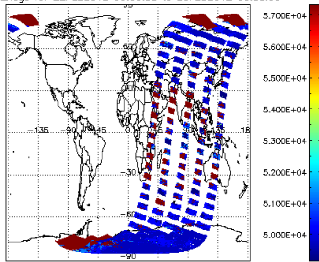
cloud_flags for 22FEB2012 00:00:00 to 23FEB2012 00:00:00
