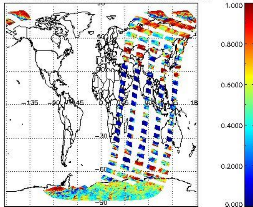
cL_frae for 22FEB2012 00:00:00 to 23FEB2012 00:00:00
