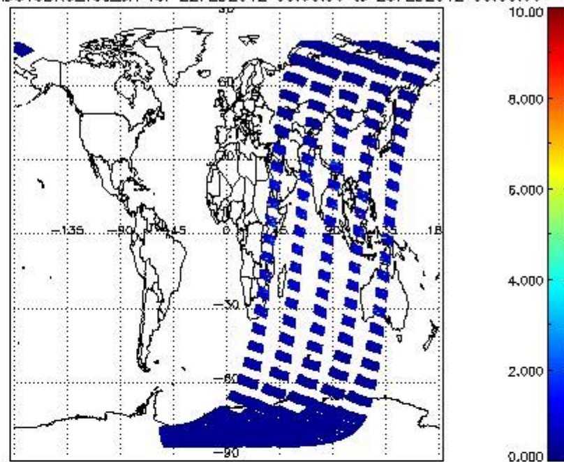
SCIOL2P_NADUV3BRO_vcd_err for 22FEB2012 00:00:00 to 23FEB2012 00:00:00
