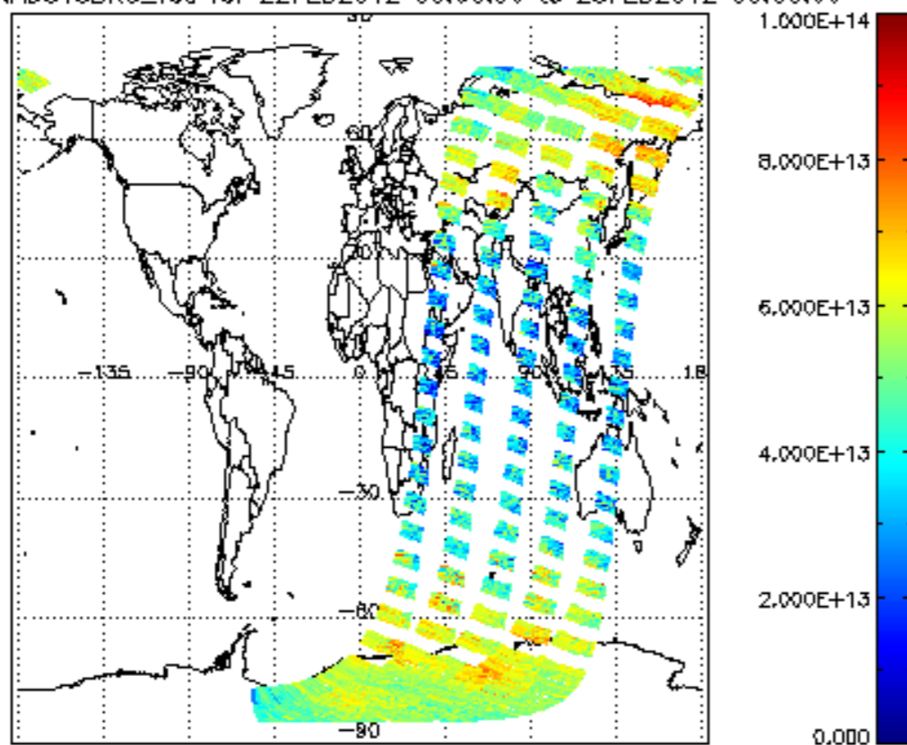
SCIOL2P_NADUV3BRO_vcd for 22FEB2012 00:00:00 to 23FEB2012 00:00:00
