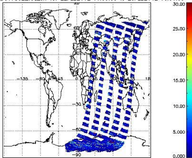
SCIOL2P_NADUV7S02_vcd_err for 22FEB2012 00:00:00 to 23FEB2012 00:00:00
