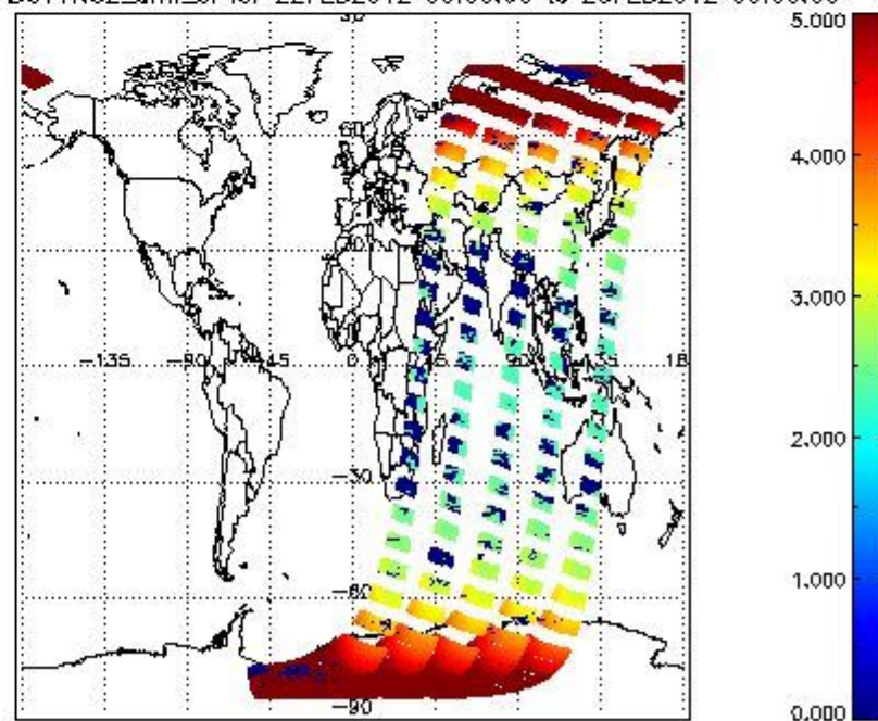
SCIOL2P_NADUV1N02_amf_cl for 22FEB2012 00:00:00 to 23FEB2012 00:00:00
