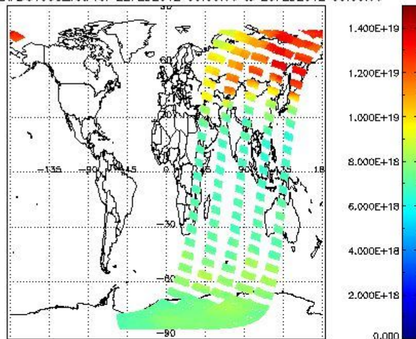
SCIOL2P_NADUV003_vcd for 22FEB2012 00:00:00 to 23FEB2012 00:00:00
