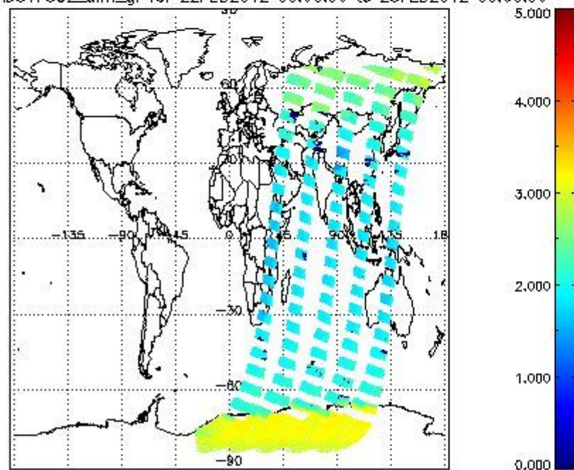
SCIOL2P_NADUV7S02_amf_gr for 22FEB2012 00:00:00 to 23FEB2012 00:00:00
