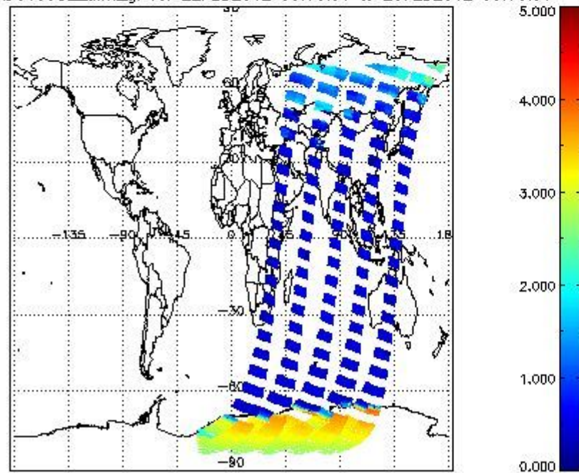
SCIOL2P_NADUV5SO2_amf_gr for 22FEB2012 00:00:00 to 23FEB2012 00:00:00
