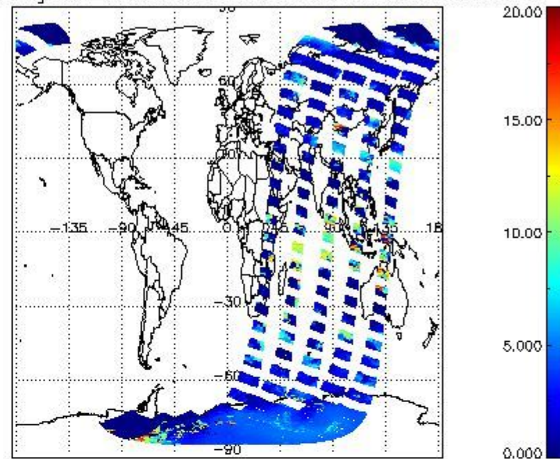
cL_top_height for 22FEB2012 00:00:00 to 23FEB2012 00:00:00
