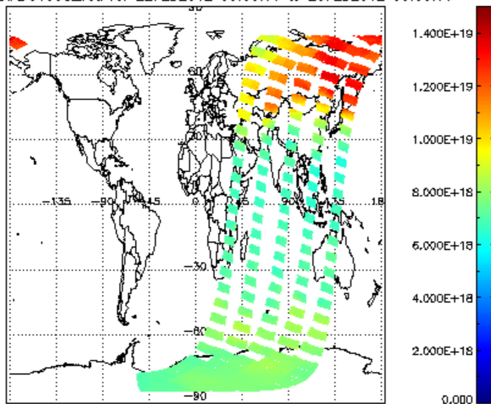
SCIOL2P_NADUV003_vcd for 22FEB2012 00:00:00 to 23FEB2012 00:00:00
