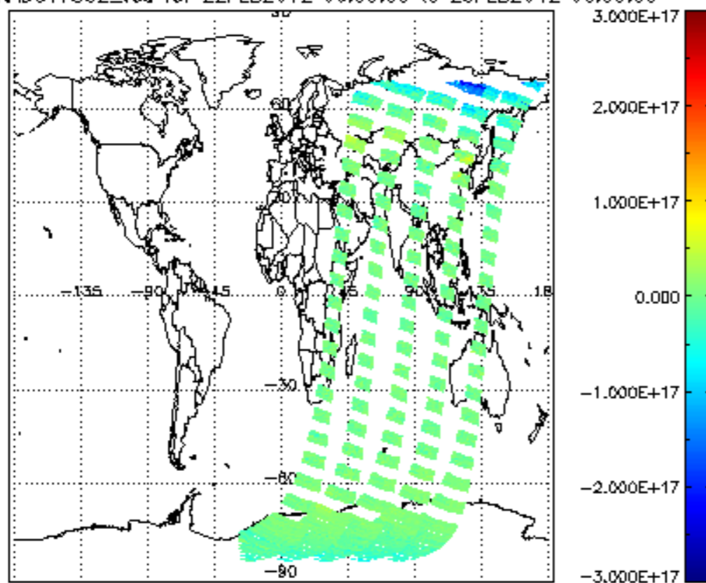
SCIOL2P_NADUV7S02_vcd for 22FEB2012 00:00:00 to 23FEB2012 00:00:00
