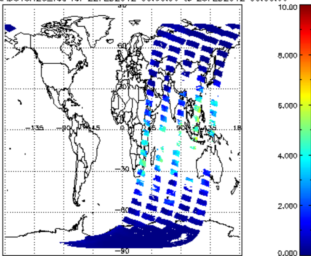
SCIOL2P_NADUV8H2O_vcd for 22FEB2012 00:00:00 to 23FEB2012 00:00:00
