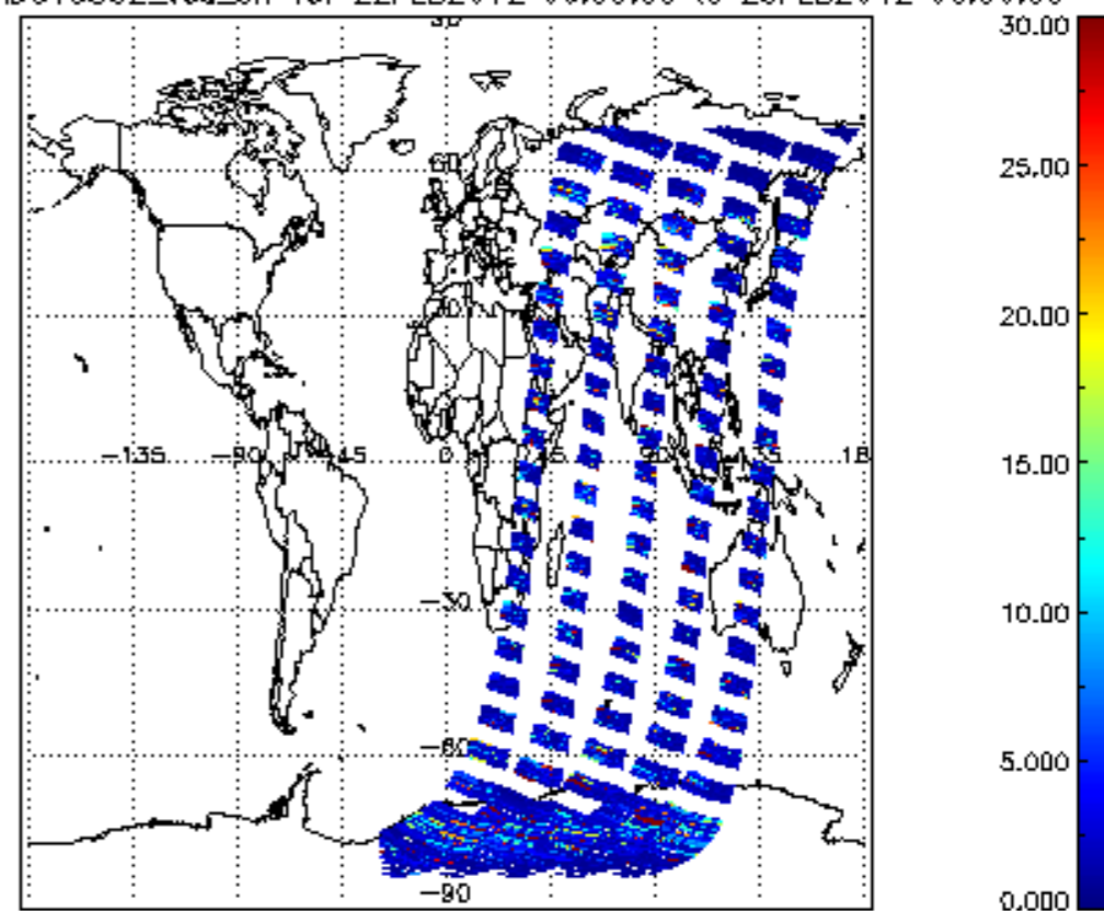
SCIOL2P_NADUV5S02_vcd_err for 22FEB2012 00:00:00 to 23FEB2012 00:00:00
