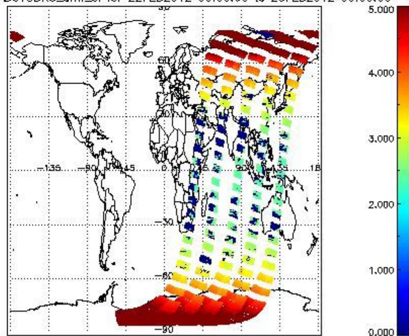
SCIOL2P_NADUV3BRO_amf_cl for 22FEB2012 00:00:00 to 23FEB2012 00:00:00
