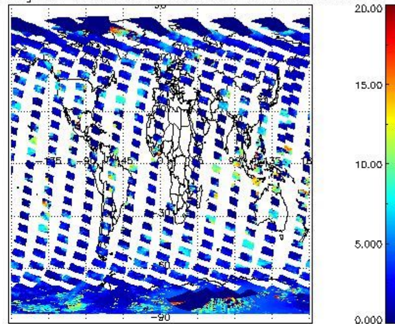
cL_top_height for 20FEB2012 00:00:00 to 21FEB2012 00:00:00
