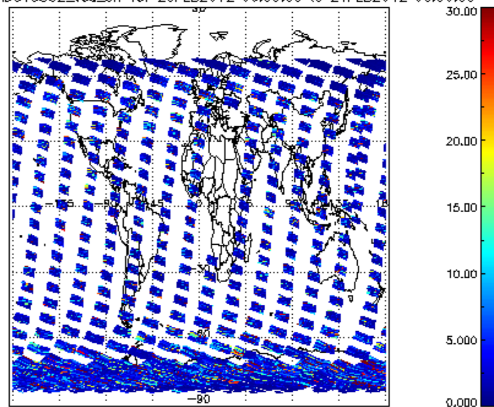
SCIOL2P_NADUV5S02_vcd_err for 20FEB2012 00:00:00 to 21FEB2012 00:00:00
