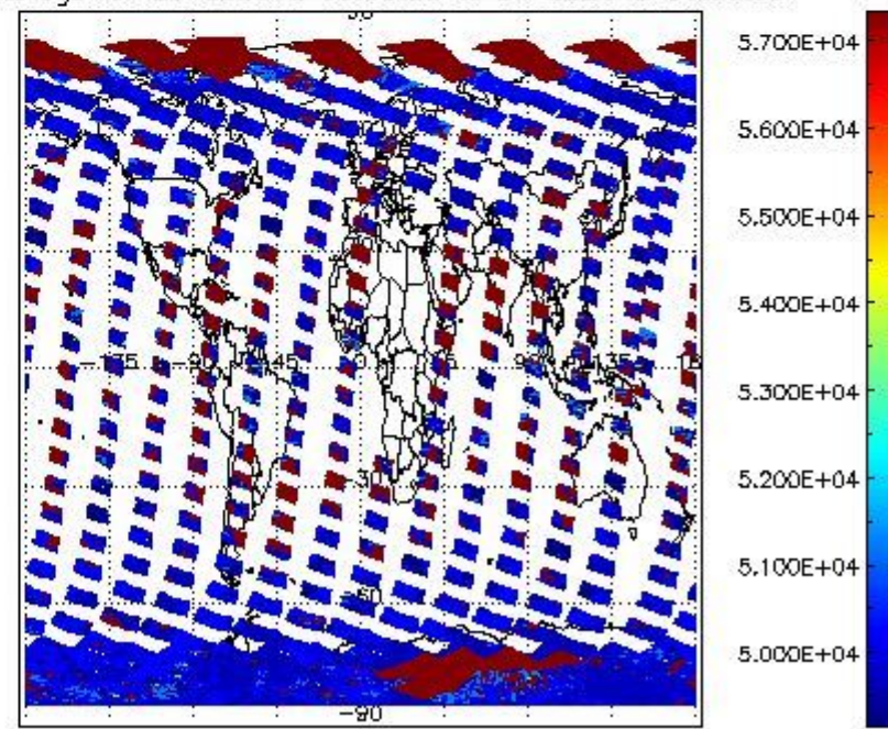
cloud_flags for 20FEB2012 00:00:00 to 21FEB2012 00:00:00
