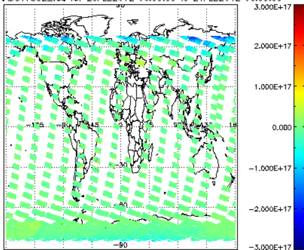
SCIOL2P_NADUV7S02_vcd for 20FEB2012 00:00:00 to 21FEB2012 00:00:00
