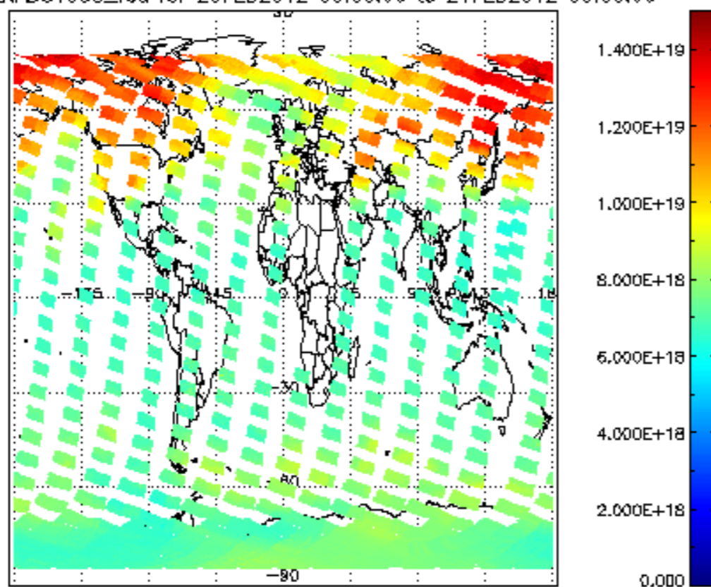
SCIOL2P_NADUV003_vcd for 20FEB2012 00:00:00 to 21FEB2012 00:00:00
