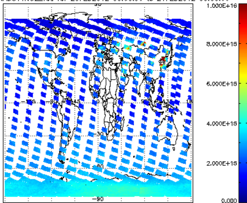
SCIOL2P_NADUV1N02_vcd for 20FEB2012 00:00:00 to 21FEB2012 00:00:00
