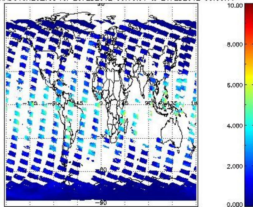
SCIOL2P_NADUV8H2O_vcd for 20FEB2012 00:00:00 to 21FEB2012 00:00:00
