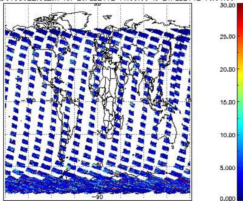
SCIOL2P_NADUV5S02_vcd_err for 20FEB2012 00:00:00 to 21FEB2012 00:00:00
