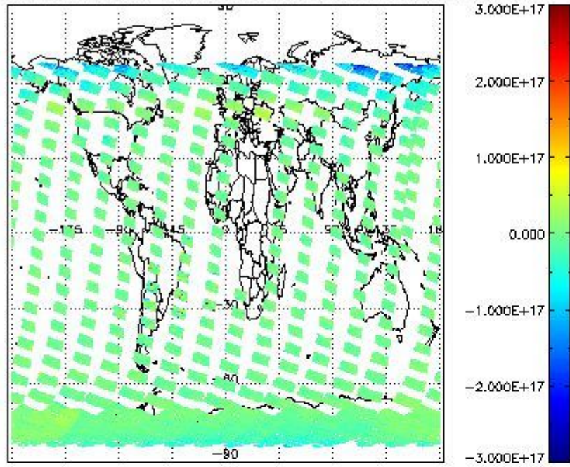
SCIOL2P_NADUV7S02_vcd for 20FEB2012 00:00:00 to 21FEB2012 00:00:00
