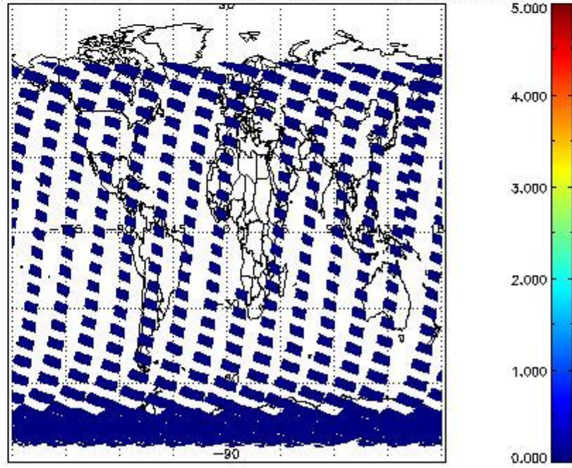
SCIOL2P_NADUV7S02_amf_cl for 20FEB2012 00:00:00 to 21FEB2012 00:00:00
