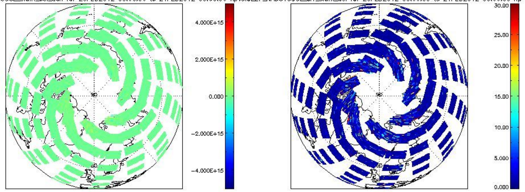
CIOL2P_NADUV6OCL_slant_col_den for 20FEB2012 00:00:00 to 21FEB2012 00:00:00 np; CIOL2P_NADUV6OCL_err_slant_col for 20FEB2012 00:00:00 to 21FEB2012 00:00:00 np
