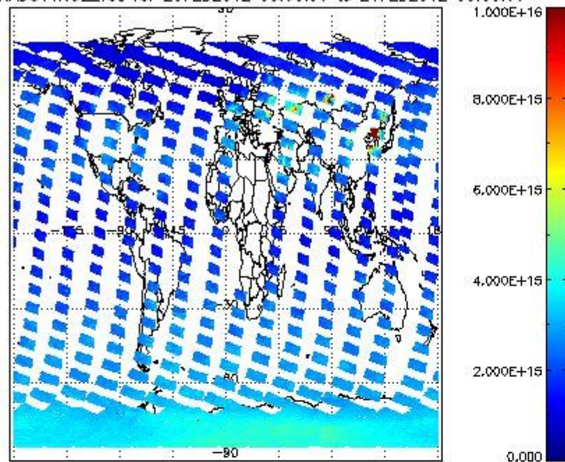
SCIOL2P_NADUV1N02_vcd for 20FEB2012 00:00:00 to 21FEB2012 00:00:00
