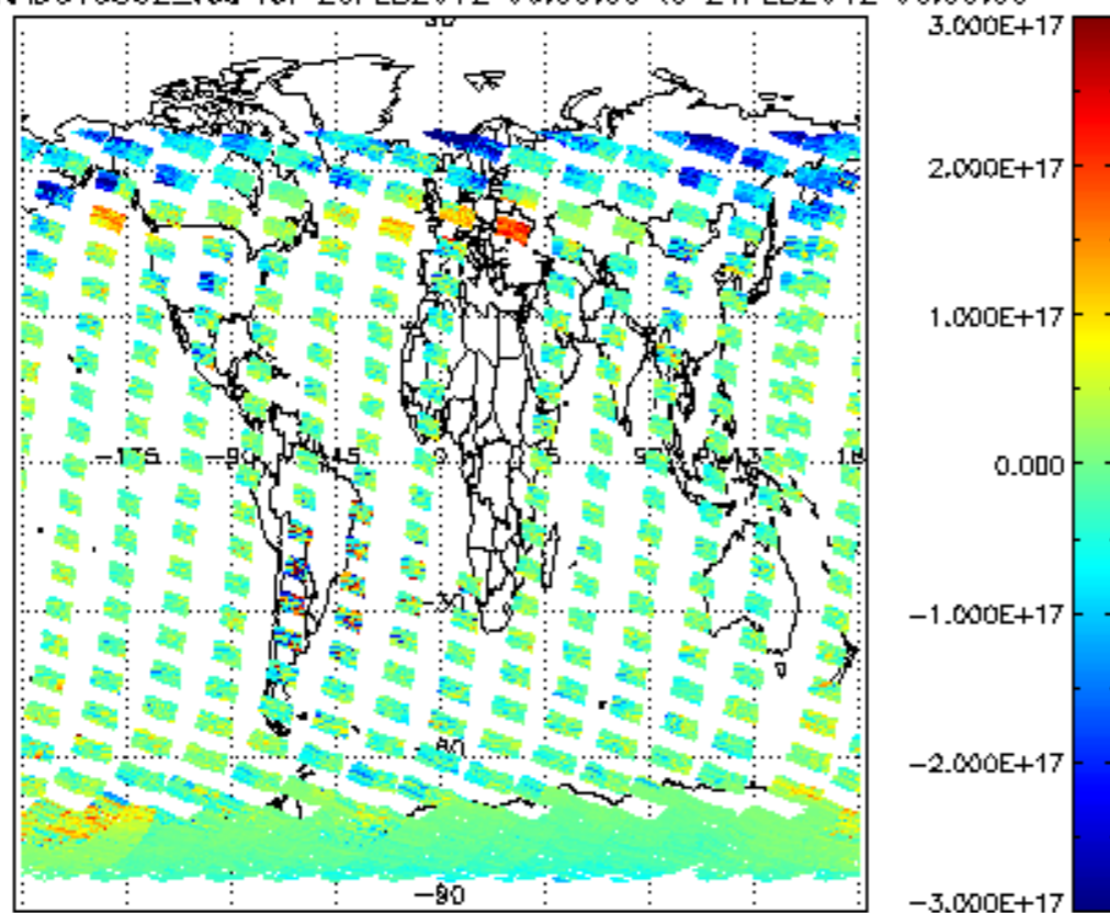
SCIOL2P_NADUV5S02_vcd for 20FEB2012 00:00:00 to 21FEB2012 00:00:00
