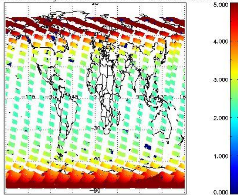
SCIOL2P_NADUV1N02_amf_gr for 20FEB2012 00:00:00 to 21FEB2012 00:00:00
