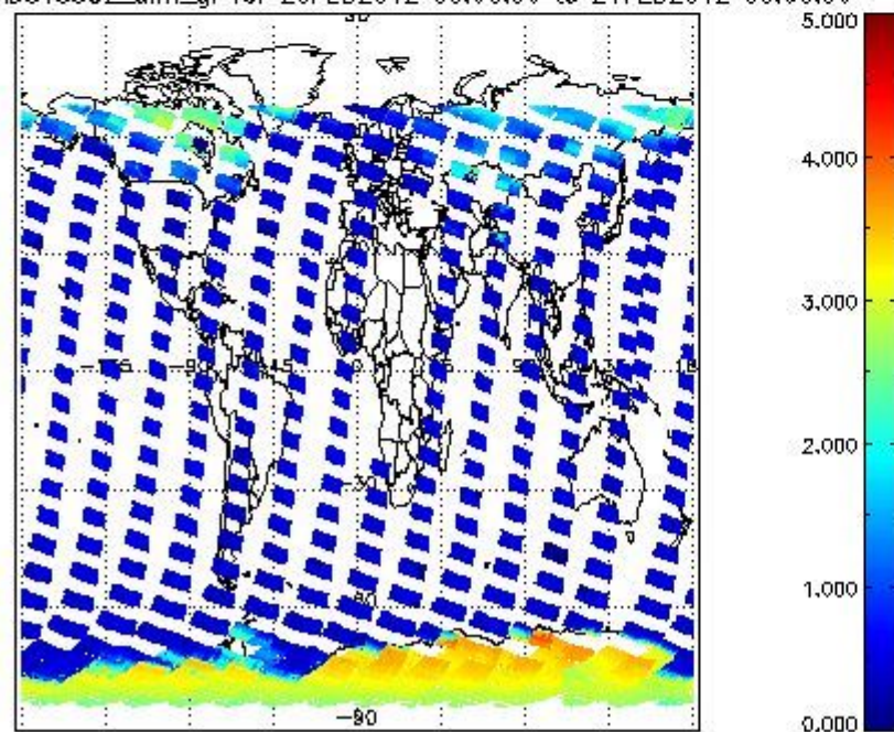
SCIOL2P_NADUV5S02_amf_gr for 20FEB2012 00:00:00 to 21FEB2012 00:00:00
