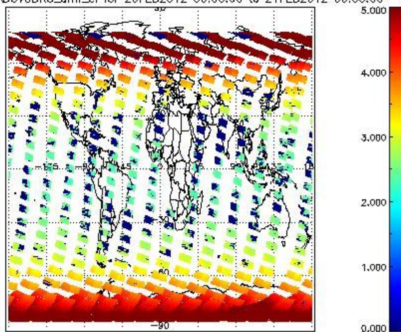
SCIOL2P_NADUV3BRO_amf_cl for 20FEB2012 00:00:00 to 21FEB2012 00:00:00
