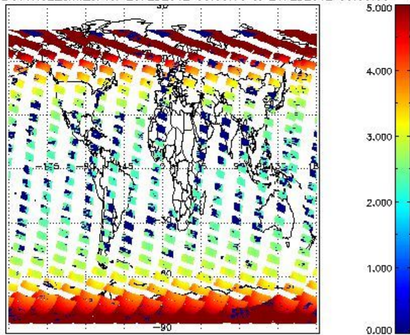
SCIOL2P_NADUV1N02_amf_cl for 20FEB2012 00:00:00 to 21FEB2012 00:00:00
