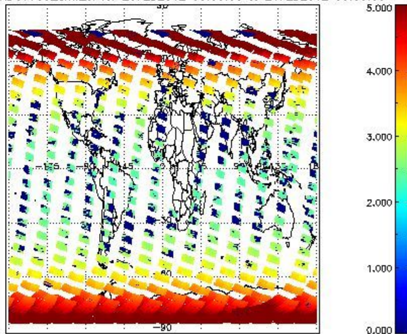
SCIOL2P_NADUV003_amf_cl for 20FEB2012 00:00:00 to 21FEB2012 00:00:00
