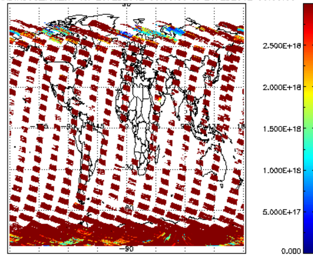
SCIOL2P_NADIR3CO_vcd_err for 20FEB2012 00:00:00 to 21FEB2012 00:00:00
