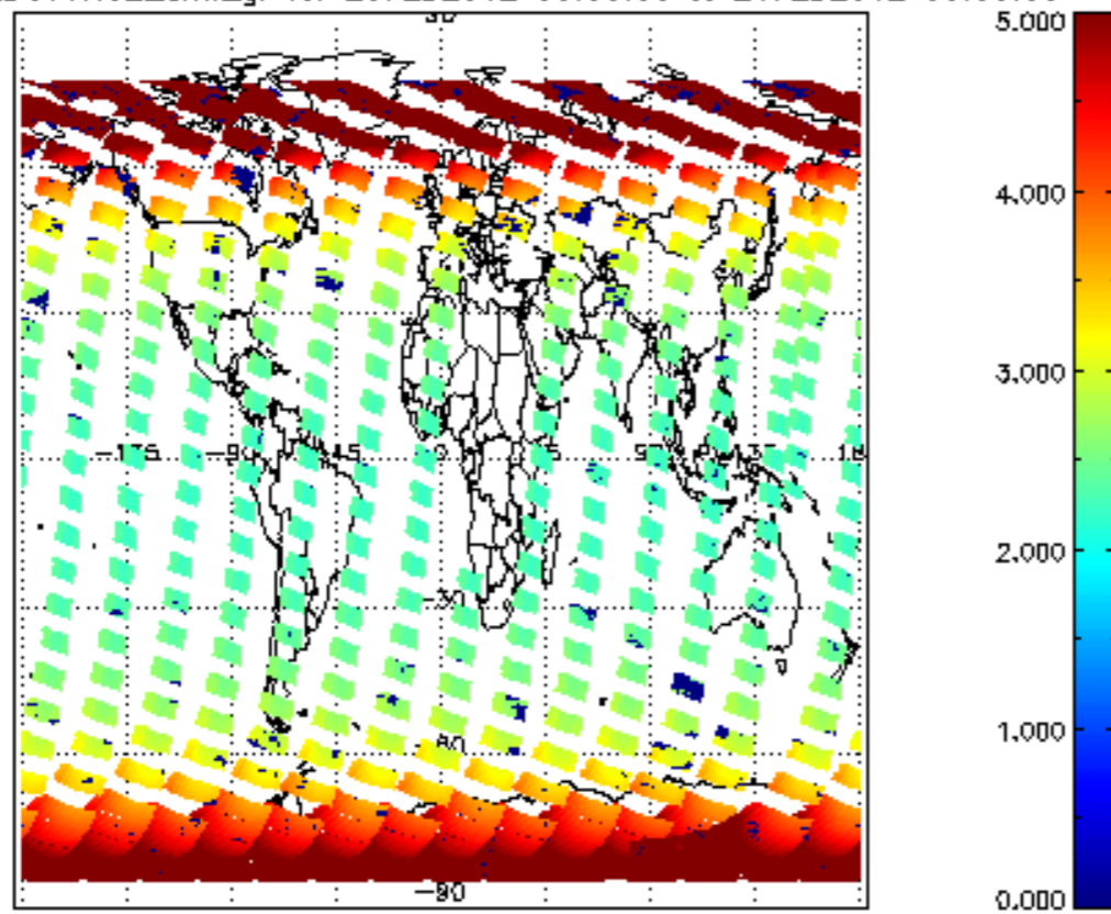
SCIOL2P_NADUV1N02_amf_gr for 20FEB2012 00:00:00 to 21FEB2012 00:00:00
