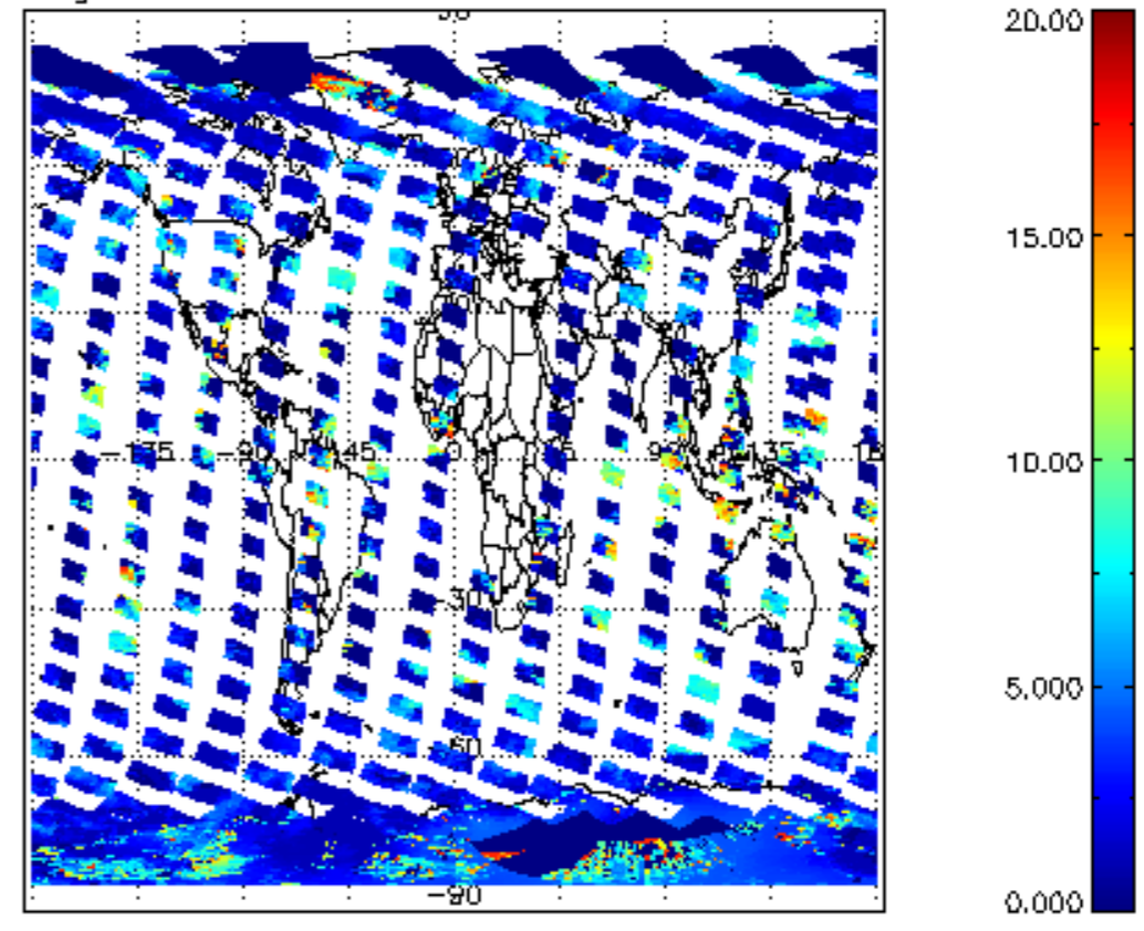
cl_top_height for 20FEB2012 00:00:00 to 21FEB2012 00:00:00
