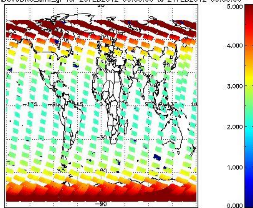
SCIOL2P_NADUV3BRO_amf_gr for 20FEB2012 00:00:00 to 21FEB2012 00:00:00
