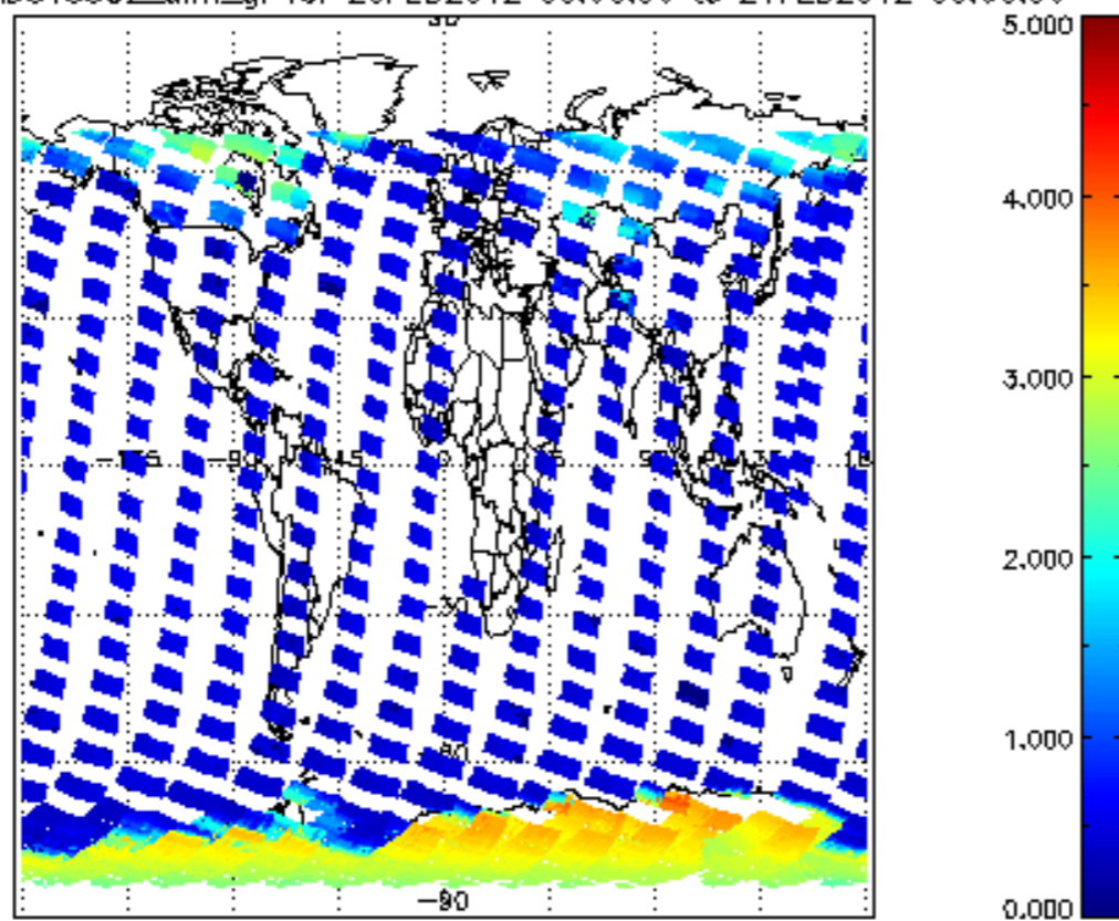
SCIOL2P_NADUV5S02_amf_gr for 20FEB2012 00:00:00 to 21FEB2012 00:00:00
