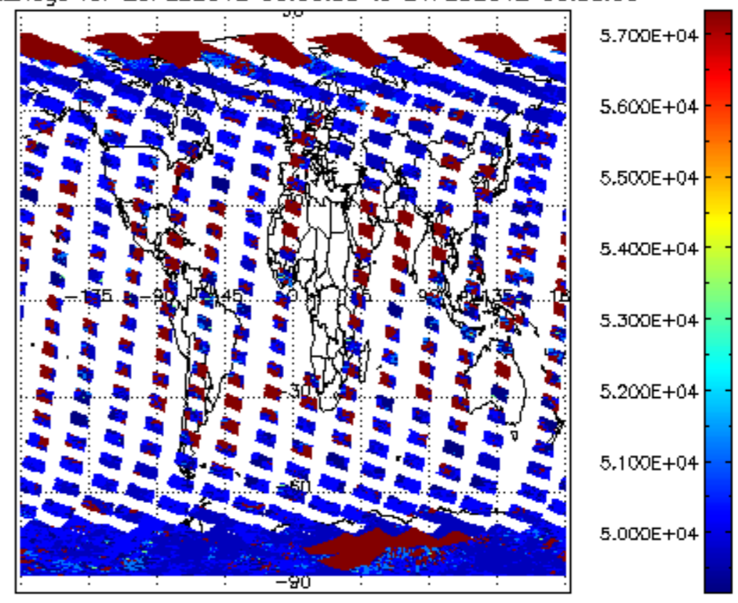
cloud_flags for 20FEB2012 00:00:00 to 21FEB2012 00:00:00
