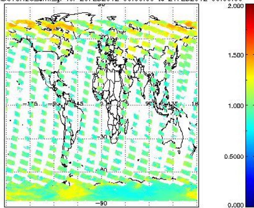
SCIOL2P_NADUV8H2O_amf_gr for 20FEB2012 00:00:00 to 21FEB2012 00:00:00
