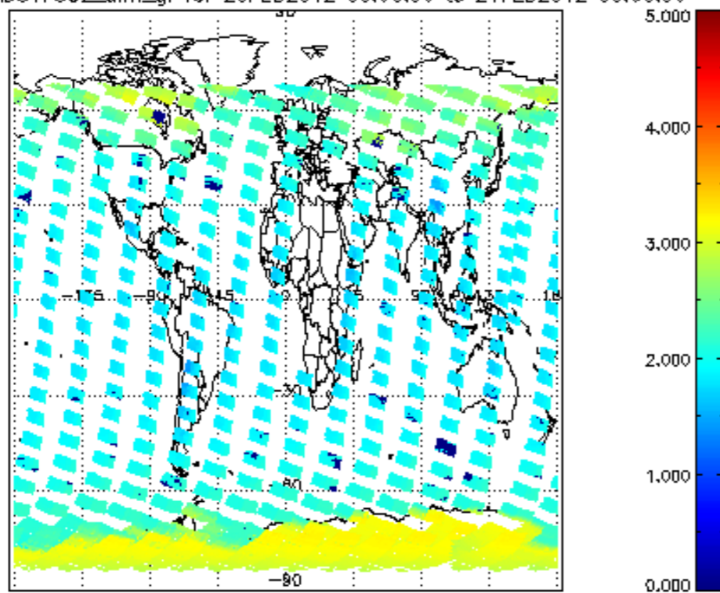
SCIOL2P_NADUV7S02_amf_gr for 20FEB2012 00:00:00 to 21FEB2012 00:00:00
