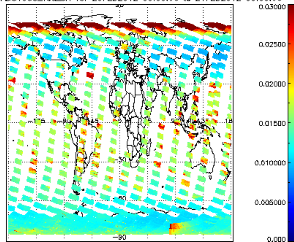
SCIOL2P_NADUV003_vcd_err for 20FEB2012 00:00:00 to 21FEB2012 00:00:00
