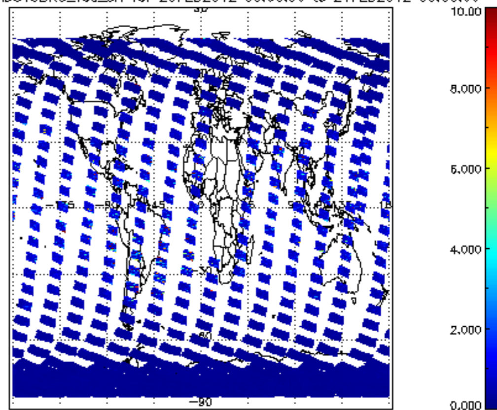
SCIOL2P_NADUV3BRO_vcd_err for 20FEB2012 00:00:00 to 21FEB2012 00:00:00
