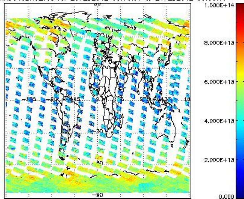
SCIOL2P_NADUV3BRO_vcd for 20FEB2012 00:00:00 to 21FEB2012 00:00:00
