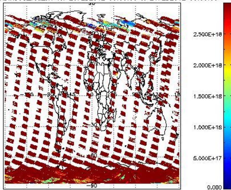
SCIDL2P_NADIR3CO_vcd_err for 20FEB2012 00:00:00 to 21FEB2012 00:00:00
