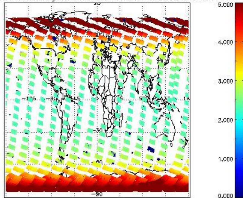
SCIOL2P_NADUV003_amf_gr for 20FEB2012 00:00:00 to 21FEB2012 00:00:00
