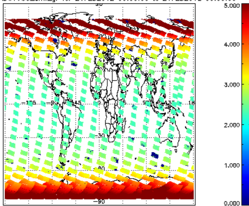
SCIOL2P_NADUV003_amf_gr for 20FEB2012 00:00:00 to 21FEB2012 00:00:00
