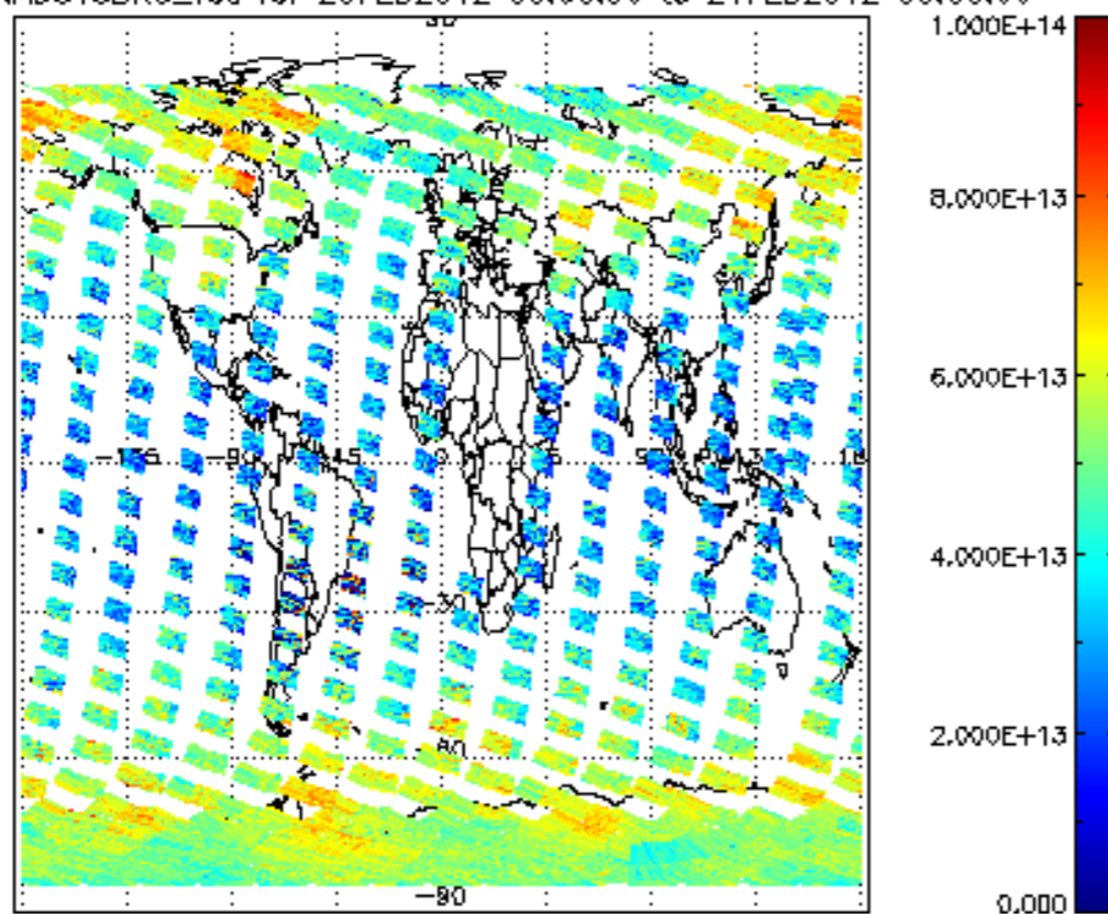
SCIOL2P_NADUV3BRO_vcd for 20FEB2012 00:00:00 to 21FEB2012 00:00:00
