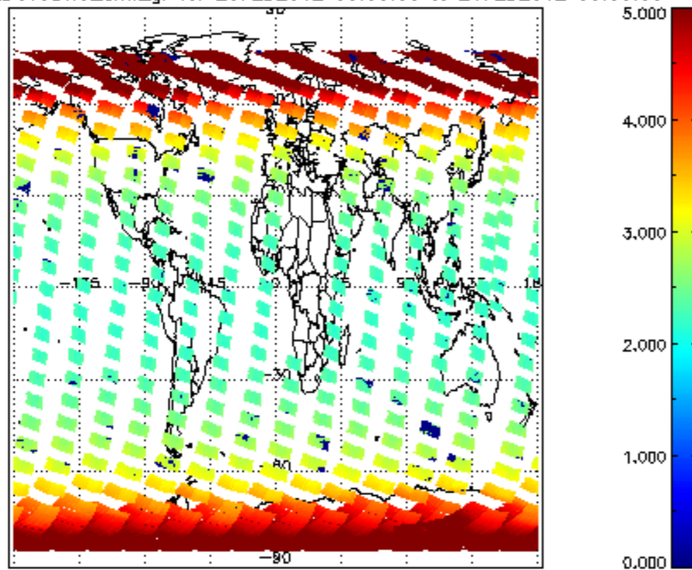
SCIOL2P_NADUV3BRO_amf_gr for 20FEB2012 00:00:00 to 21FEB2012 00:00:00
