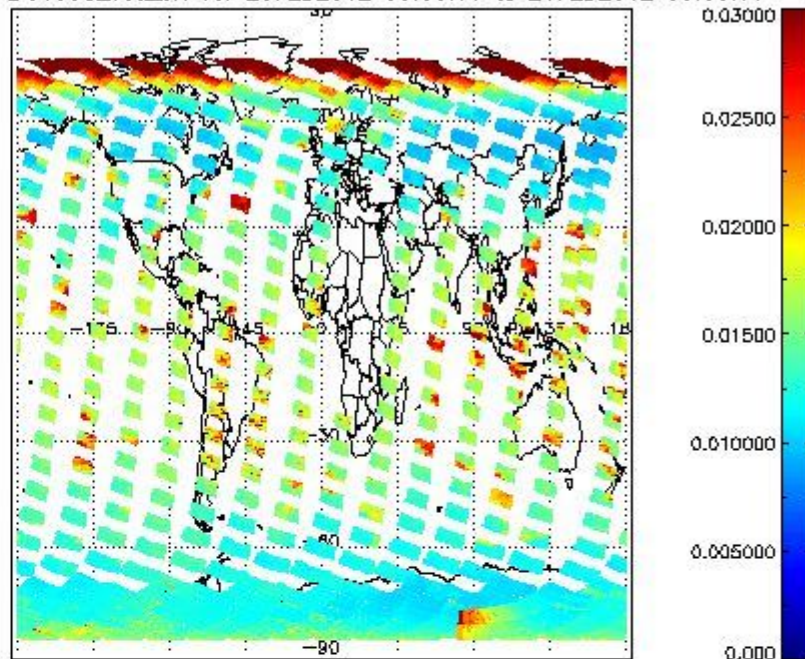
SCIOL2P_NADUV003_vcd_err for 20FEB2012 00:00:00 to 21FEB2012 00:00:00
