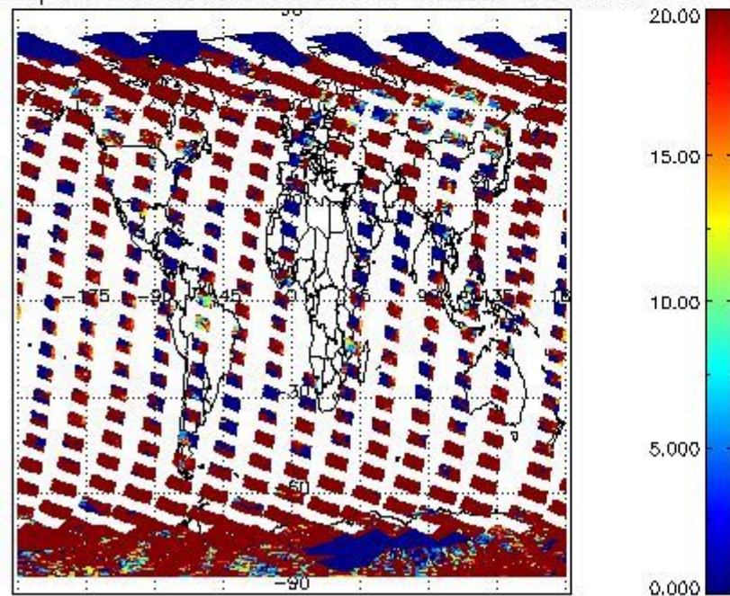
cL_opt_depth for 20FEB2012 00:00:00 to 21FEB2012 00:00:00
