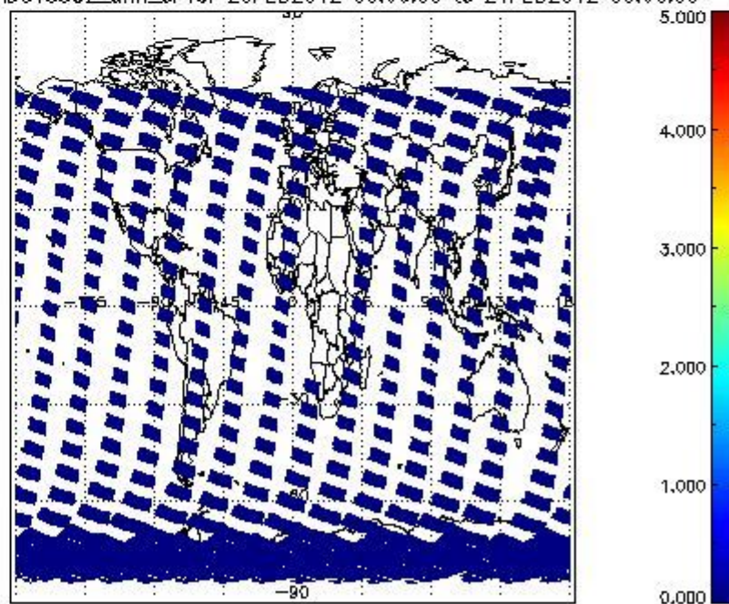
SCIOL2P_NADUV5S02_amf_cl for 20FEB2012 00:00:00 to 21FEB2012 00:00:00
