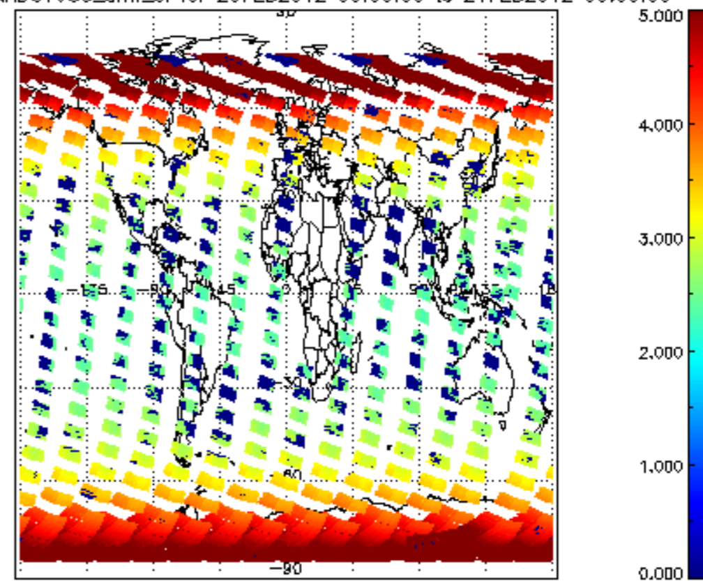
SCIOL2P_NADUV003_amf_cl for 20FEB2012 00:00:00 to 21FEB2012 00:00:00
