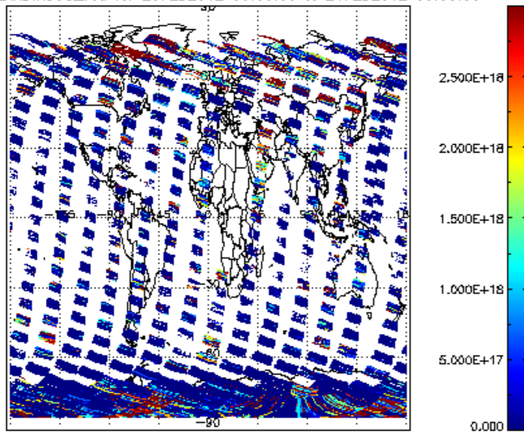
SCIOL2P_NADIR3CO_vcd for 20FEB2012 00:00:00 to 21FEB2012 00:00:00
