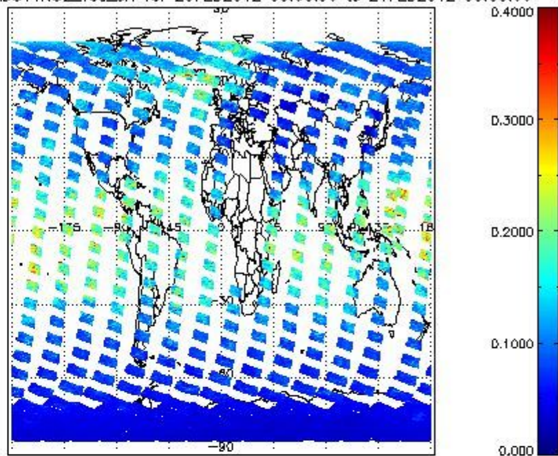
SCIOL2P_NADUV1N02_vcd_err for 20FEB2012 00:00:00 to 21FEB2012 00:00:00
