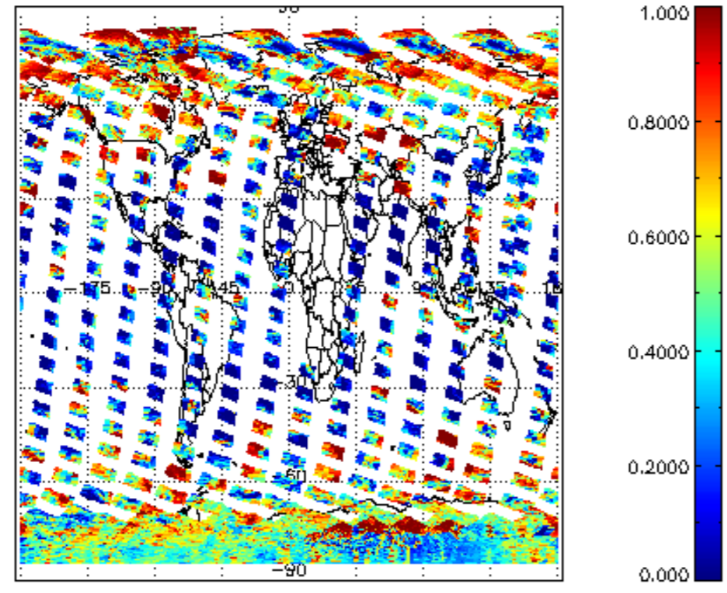
cl_frac for 20FEB2012 00:00:00 to 21FEB2012 00:00:00
