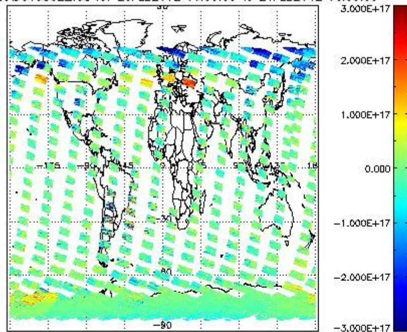
SCIOL2P_NADUV5S02_vcd for 20FEB2012 00:00:00 to 21FEB2012 00:00:00
