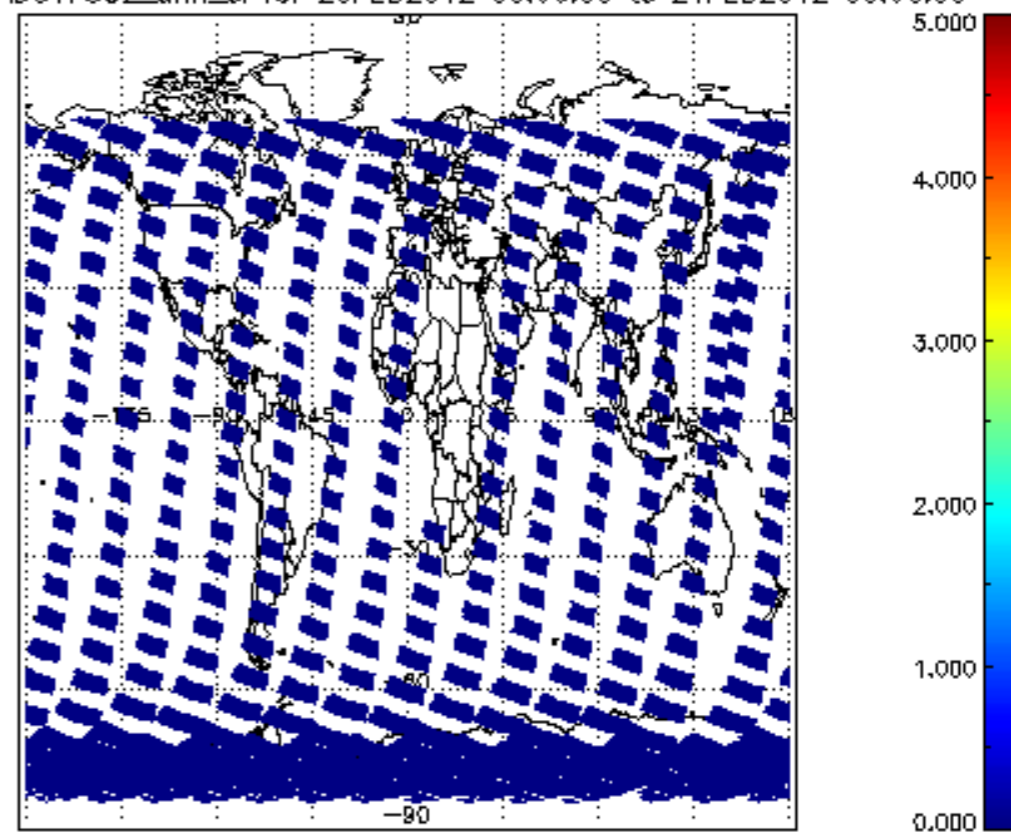
SCIOL2P_NADUV7S02_amf_cl for 20FEB2012 00:00:00 to 21FEB2012 00:00:00
