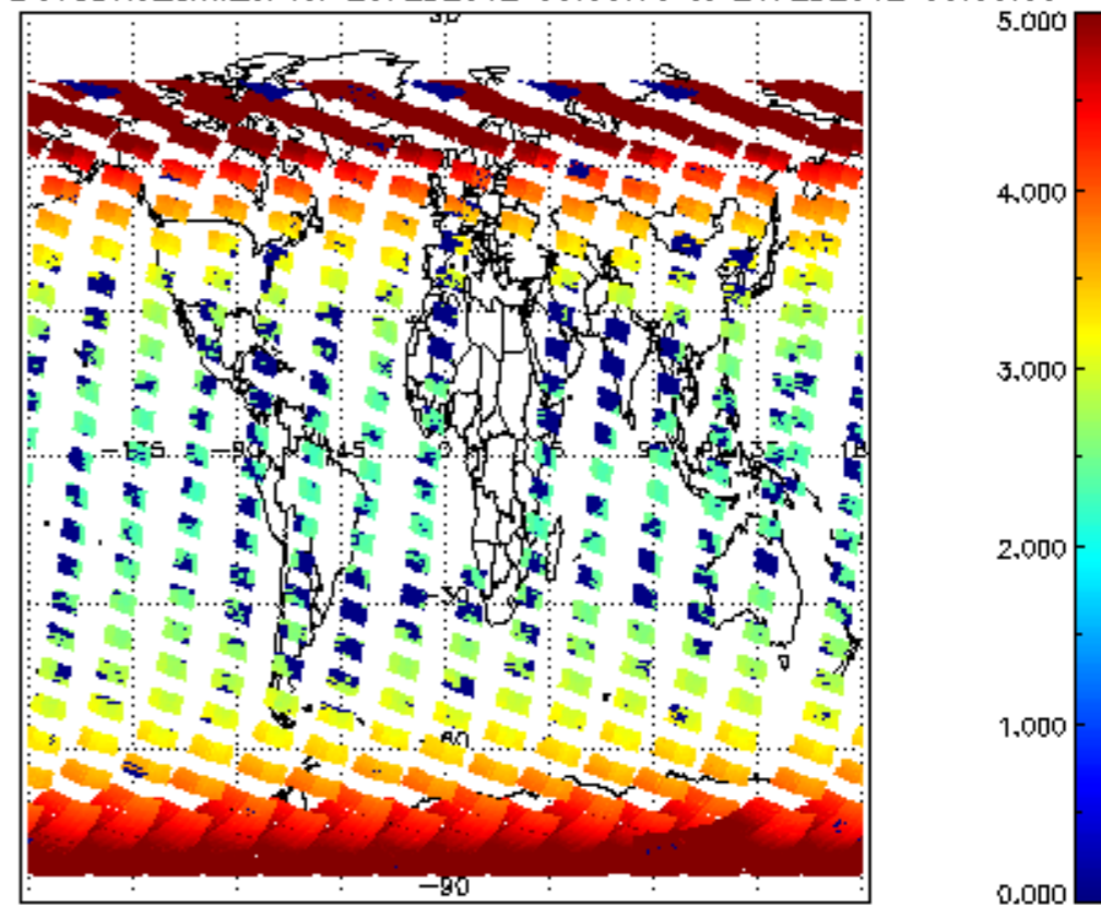
SCIOL2P_NADUV3BRO_amf_cl for 20FEB2012 00:00:00 to 21FEB2012 00:00:00
