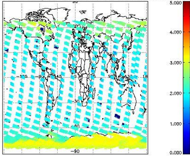
SCIOL2P_NADUV7S02_amf_gr for 20FEB2012 00:00:00 to 21FEB2012 00:00:00
