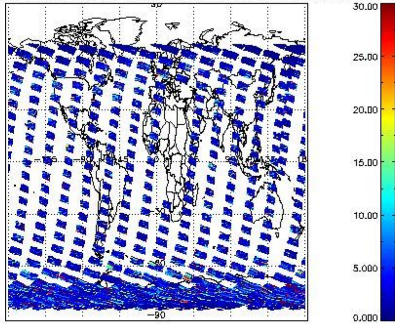
SCIOL2P_NADUV7S02_vcd_err for 20FEB2012 00:00:00 to 21FEB2012 00:00:00
