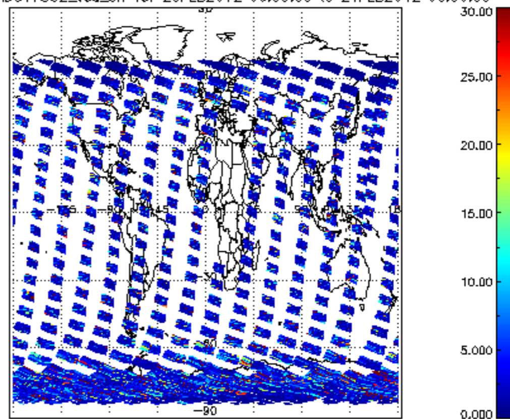
SCIOL2P_NADUV7S02_vcd_err for 20FEB2012 00:00:00 to 21FEB2012 00:00:00
