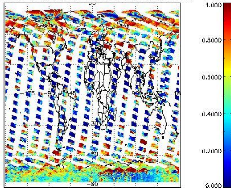
cL_frae for 20FEB2012 00:00:00 to 21FEB2012 00:00:00
