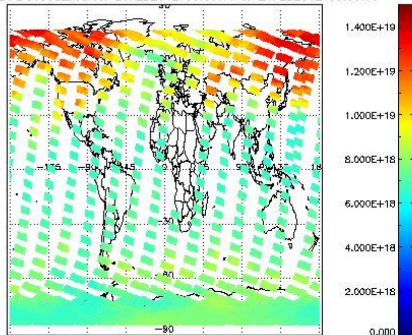
SCIOL2P_NADUV003_vcd for 20FEB2012 00:00:00 to 21FEB2012 00:00:00
