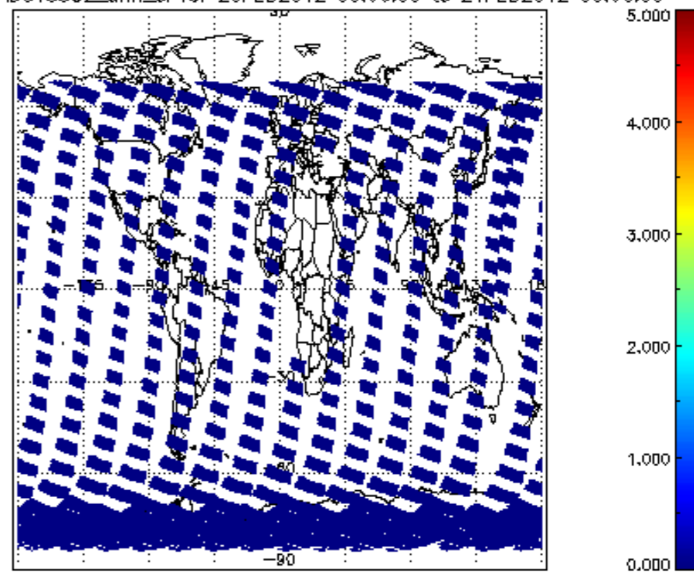
SCIOL2P_NADUV5S02_amf_cl for 20FEB2012 00:00:00 to 21FEB2012 00:00:00
