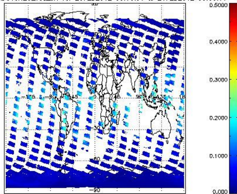
SCIOL2P_NADUV8H2O_vcd_err for 20FEB2012 00:00:00 to 21FEB2012 00:00:00
