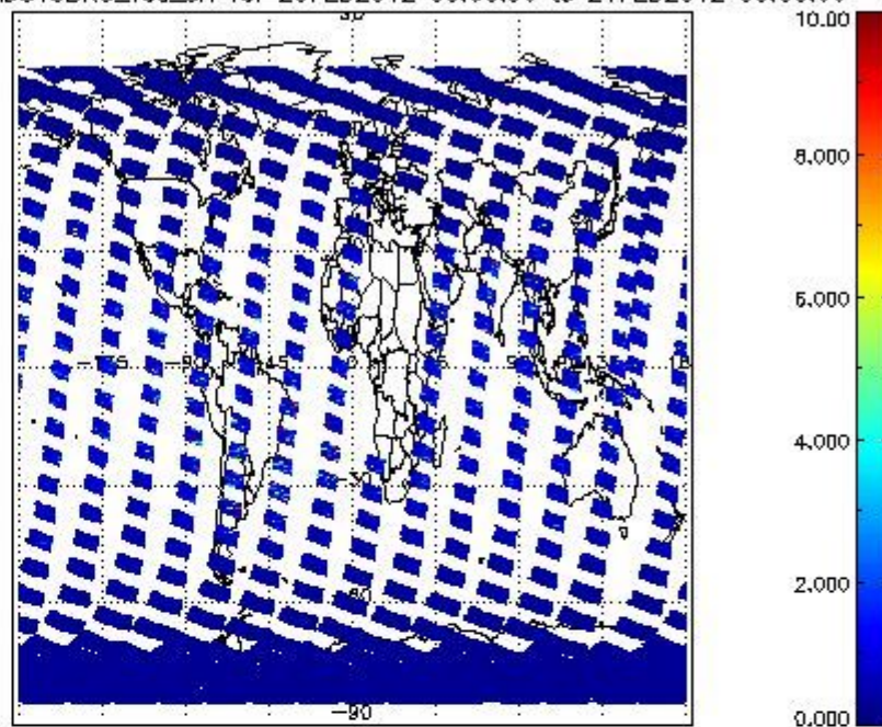
SCIOL2P_NADUV3BRO_vcd_err for 20FEB2012 00:00:00 to 21FEB2012 00:00:00
