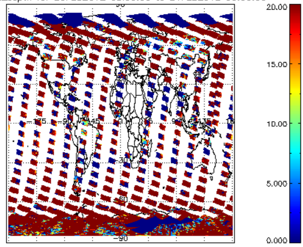
cl_opt_depth for 20FEB2012 00:00:00 to 21FEB2012 00:00:00
