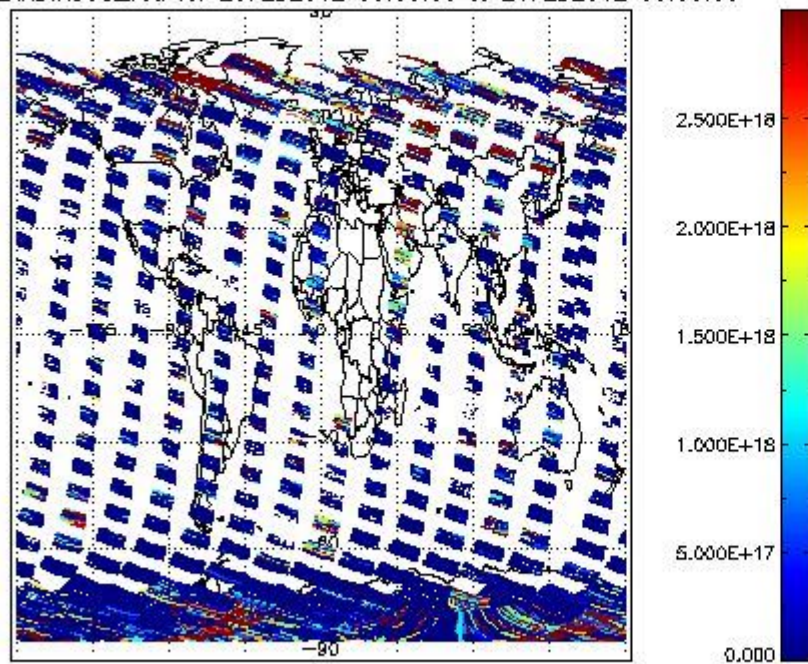
SCIDL2P_NADIR3CO_vcd for 20FEB2012 00:00:00 to 21FEB2012 00:00:00
