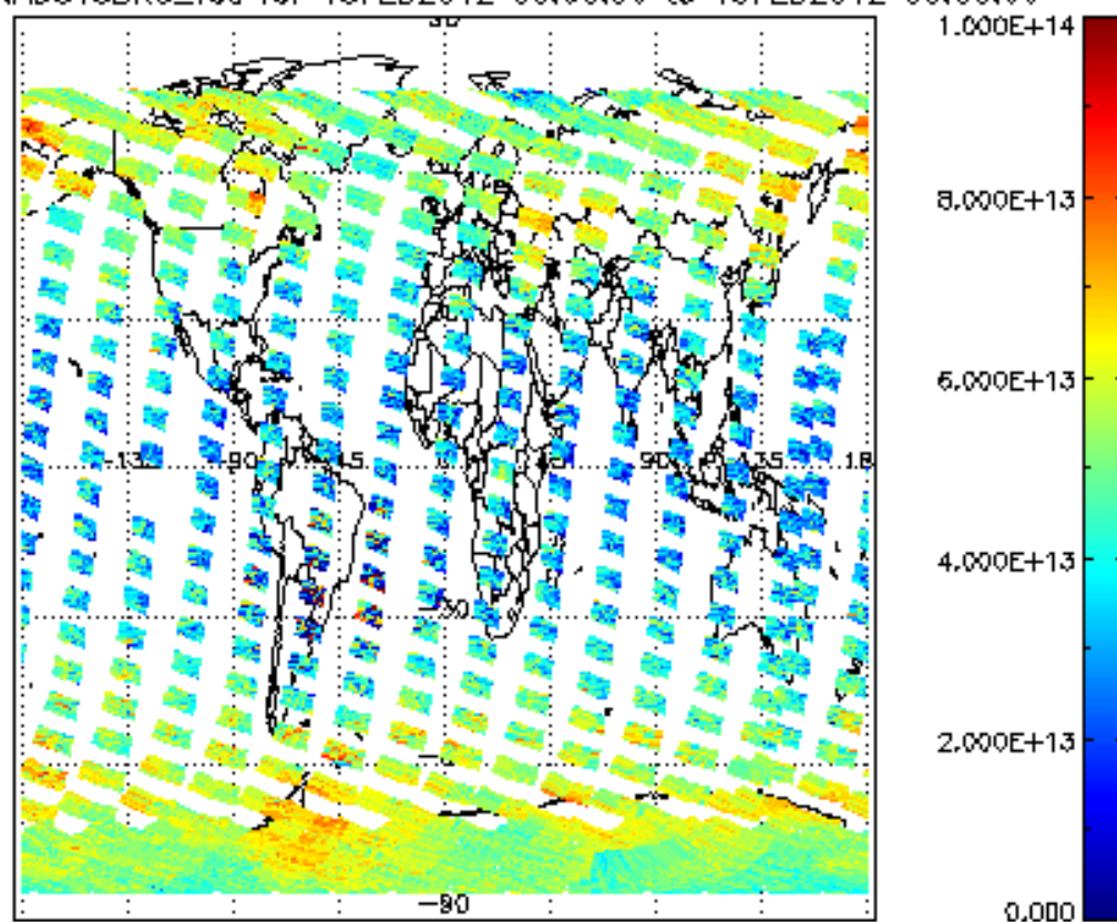
SCIOL2P_NADUV3BRO_vcd for 18FEB2012 00:00:00 to 19FEB2012 00:00:00
