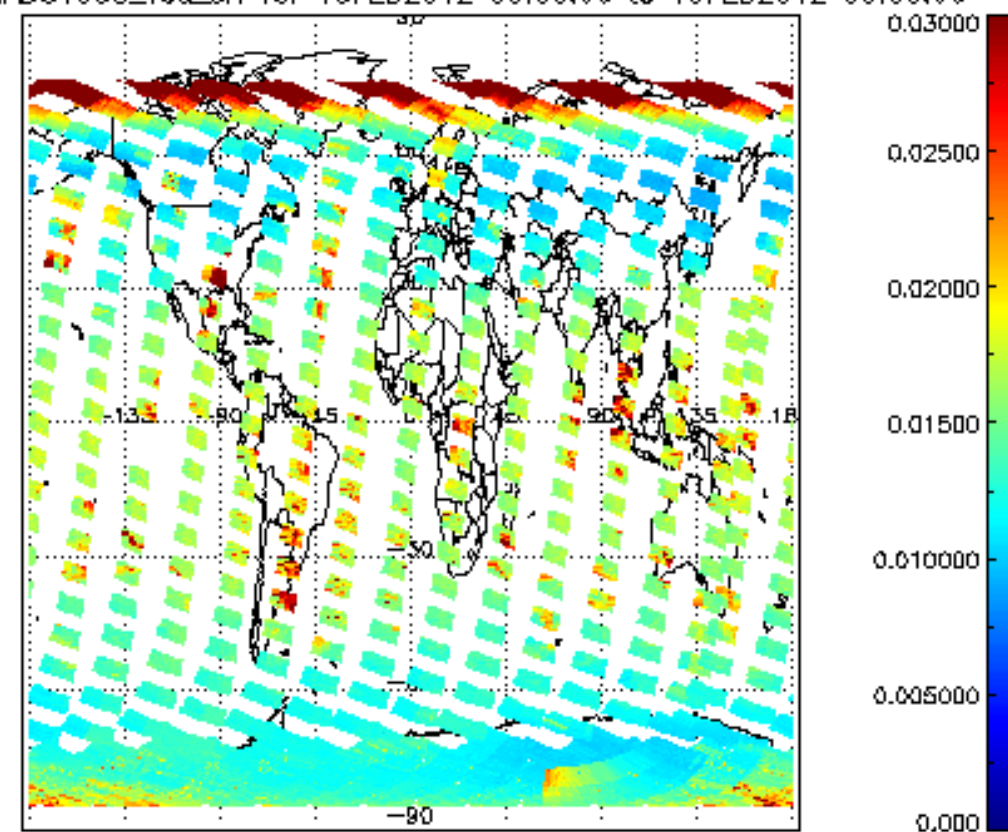
SCIOL2P_NADUV003_vcd_err for 18FEB2012 00:00:00 to 19FEB2012 00:00:00
