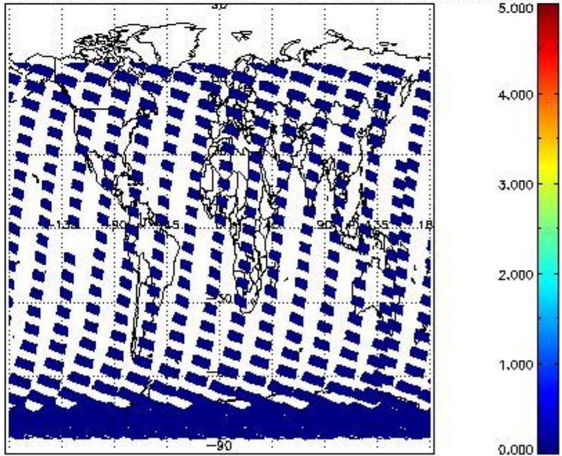
SCIOL2P_NADUV5SO2_amf_cl for 18FEB2012 00:00:00 to 19FEB2012 00:00:00
