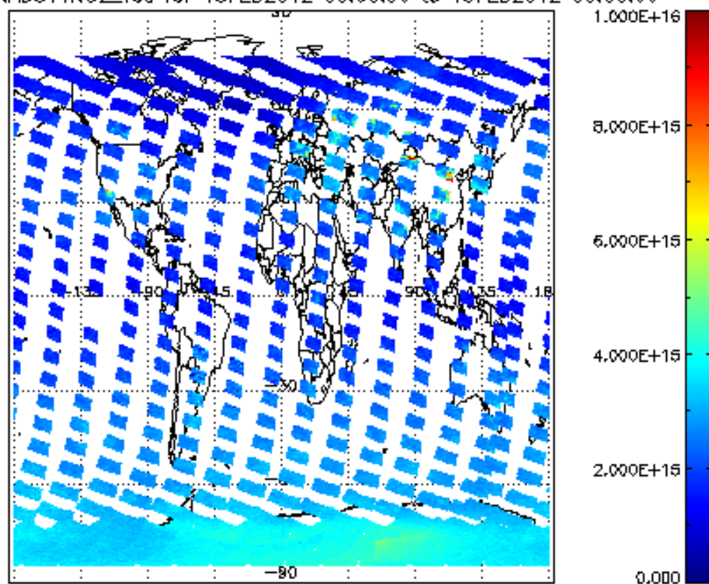
SCIOL2P_NADUV1N02_vcd for 18FEB2012 00:00:00 to 19FEB2012 00:00:00
