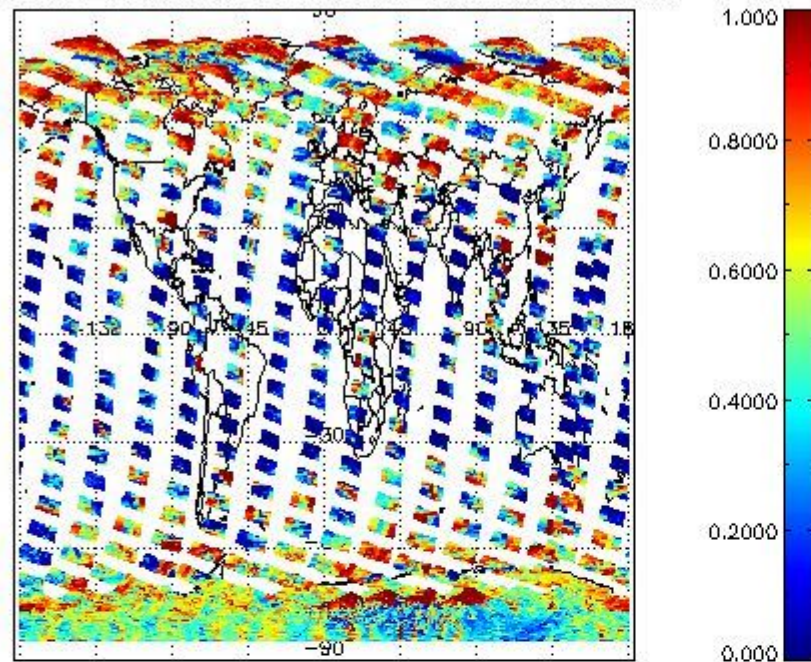
cL_frac for 18FEB2012 00:00:00 to 19FEB2012 00:00:00
