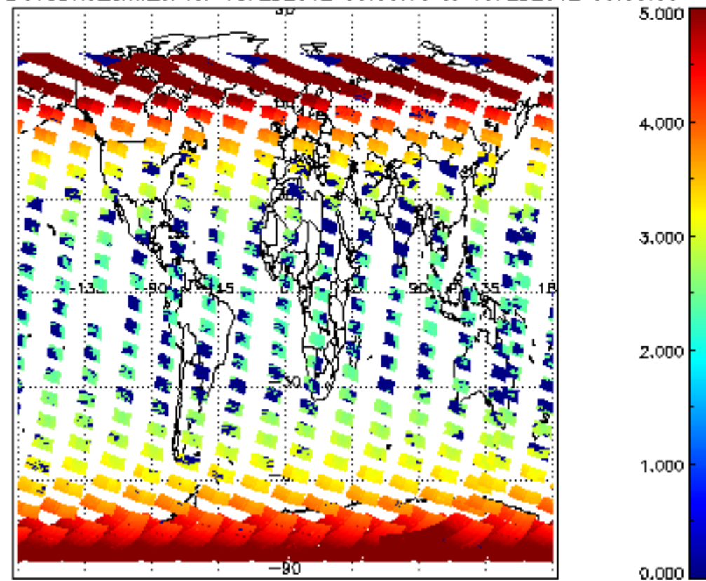
SCIOL2P_NADUV3BRO_amf_cl for 18FEB2012 00:00:00 to 19FEB2012 00:00:00
