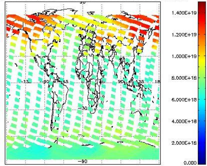
SCIOL2P_NADUV003_vcd for 18FEB2012 00:00:00 to 19FEB2012 00:00:00
