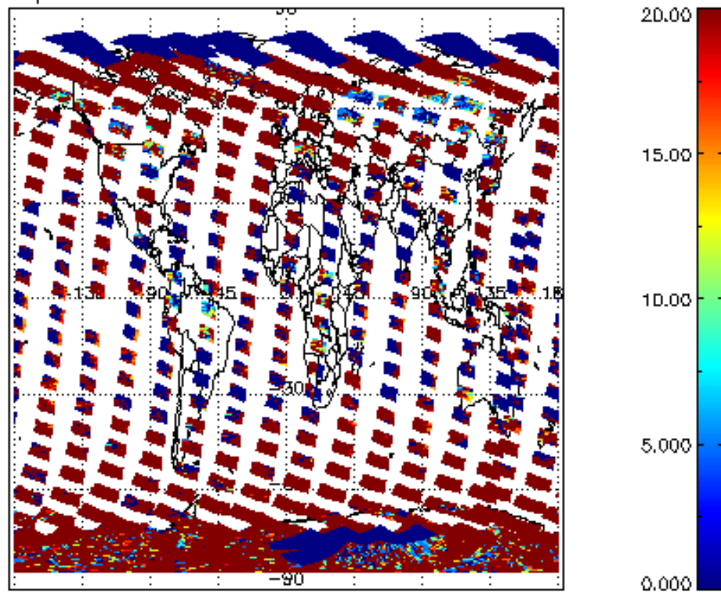
cl_opt_depth for 18FEB2012 00:00:00 to 19FEB2012 00:00:00
