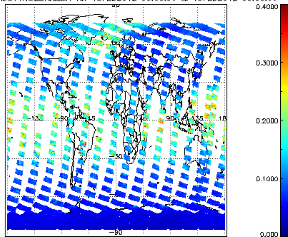
SCIOL2P_NADUV1N02_vcd_err for 18FEB2012 00:00:00 to 19FEB2012 00:00:00
