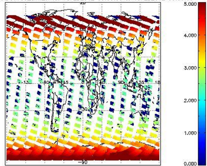
SCIOL2P_NADUV003_amf_cl for 18FEB2012 00:00:00 to 19FEB2012 00:00:00
