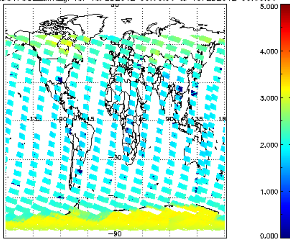
SCIOL2P_NADUV7S02_amf_gr for 18FEB2012 00:00:00 to 19FEB2012 00:00:00
