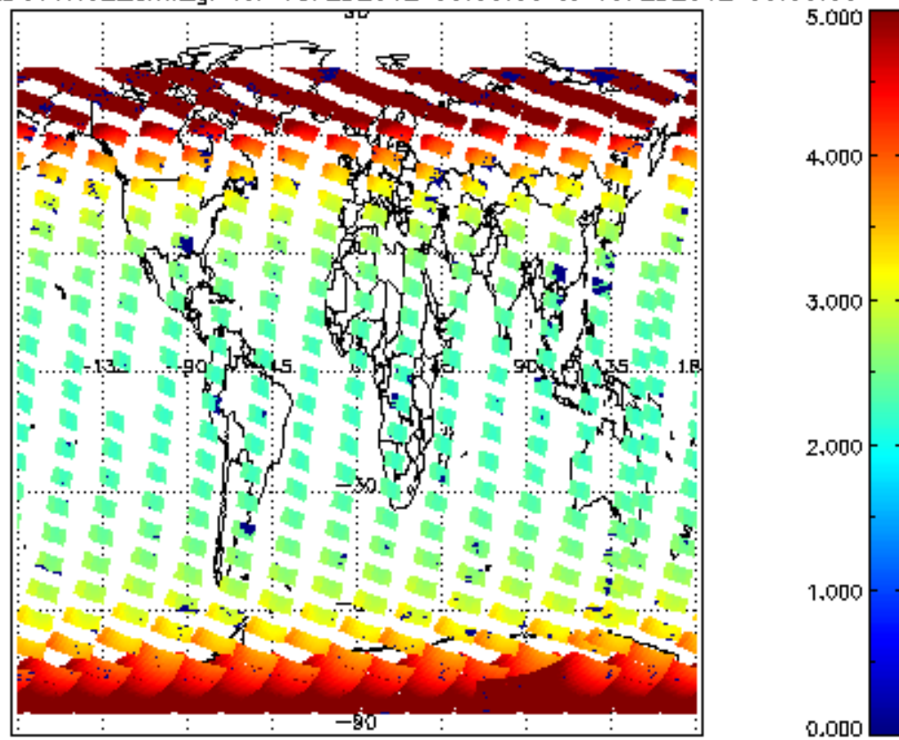
SCIOL2P_NADUV1N02_amf_gr for 18FEB2012 00:00:00 to 19FEB2012 00:00:00
