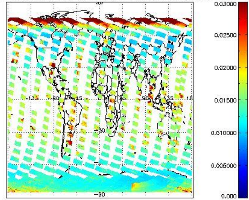
SCIOL2P_NADUV003_vcd_err for 18FEB2012 00:00:00 to 19FEB2012 00:00:00
