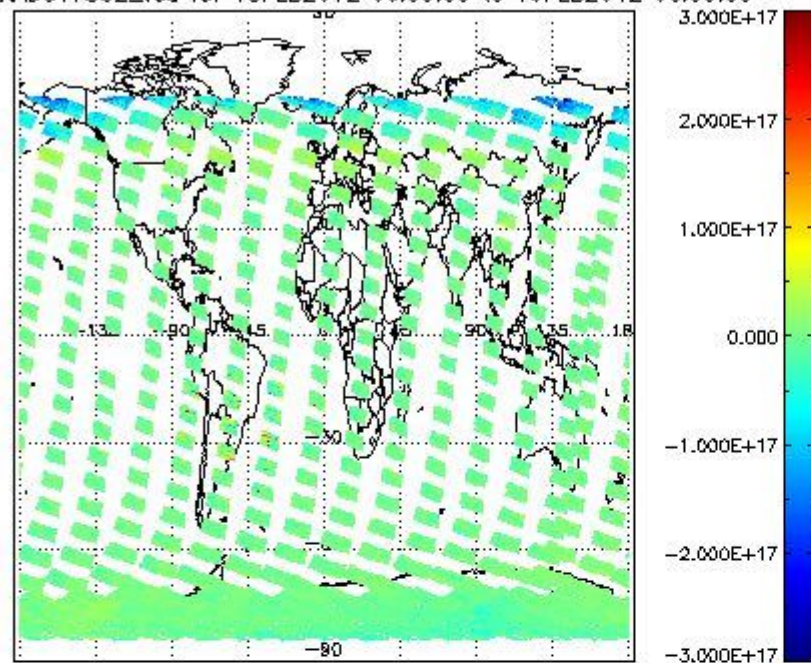
SCIOL2P_NADUV7S02_vcd for 18FEB2012 00:00:00 to 19FEB2012 00:00:00
