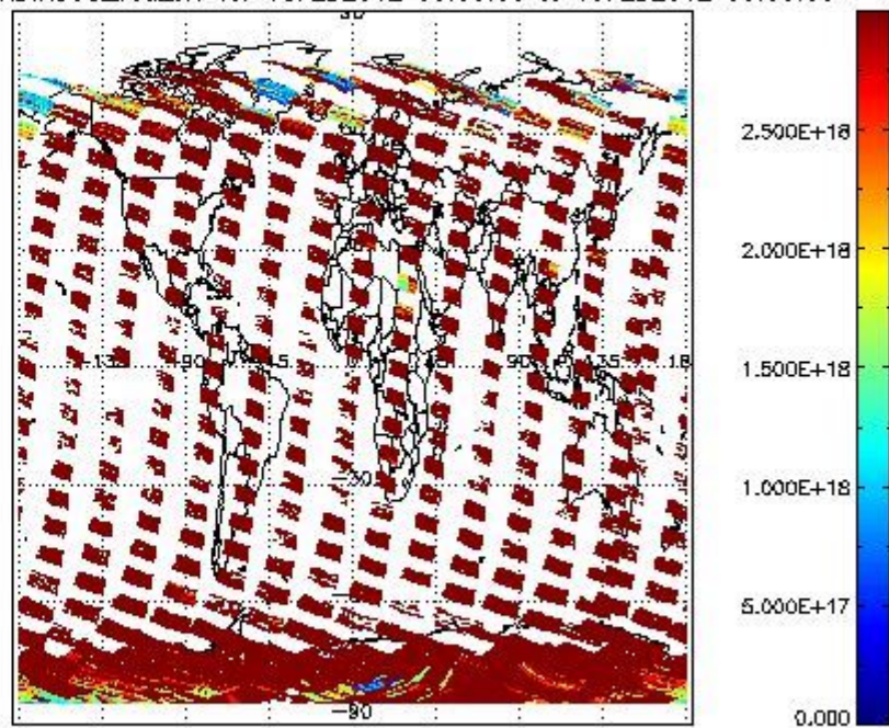
SCIDL2P_NADIR3CO_vcd_err for 18FEB2012 00:00:00 to 19FEB2012 00:00:00
