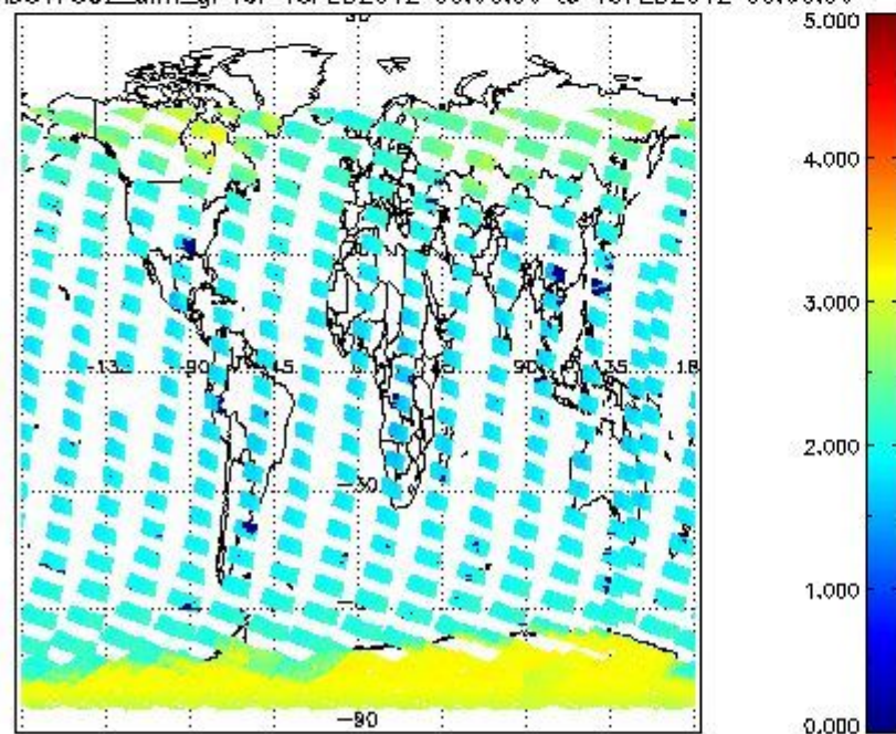
SCIOL2P_NADUV7S02_amf_gr for 18FEB2012 00:00:00 to 19FEB2012 00:00:00
