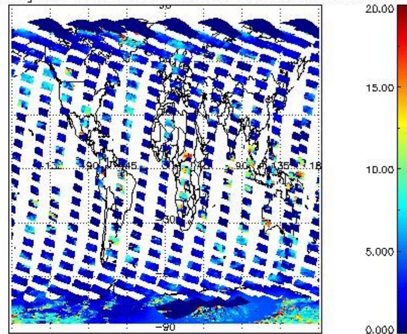
cL_top_height for 18FEB2012 00:00:00 to 19FEB2012 00:00:00
