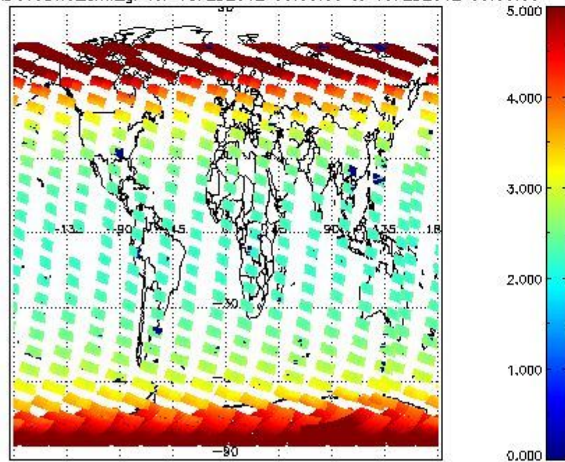
SCIOL2P_NADUV3BRO_amf_gr for 18FEB2012 00:00:00 to 19FEB2012 00:00:00
