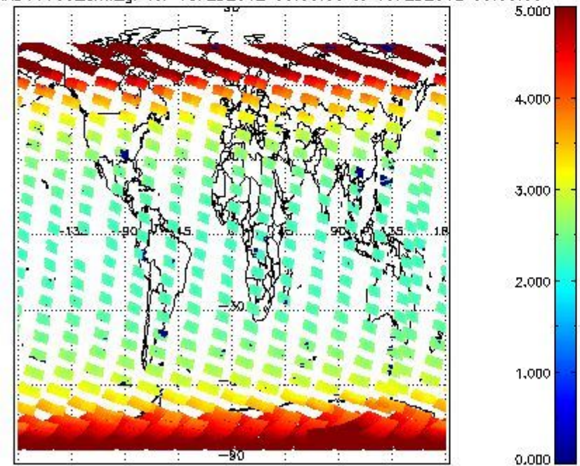
SCIOL2P_NADUV003_amf_gr for 18FEB2012 00:00:00 to 19FEB2012 00:00:00
