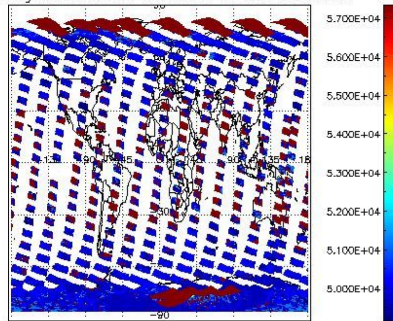
cloud_flags for 18FEB2012 00:00:00 to 19FEB2012 00:00:00
