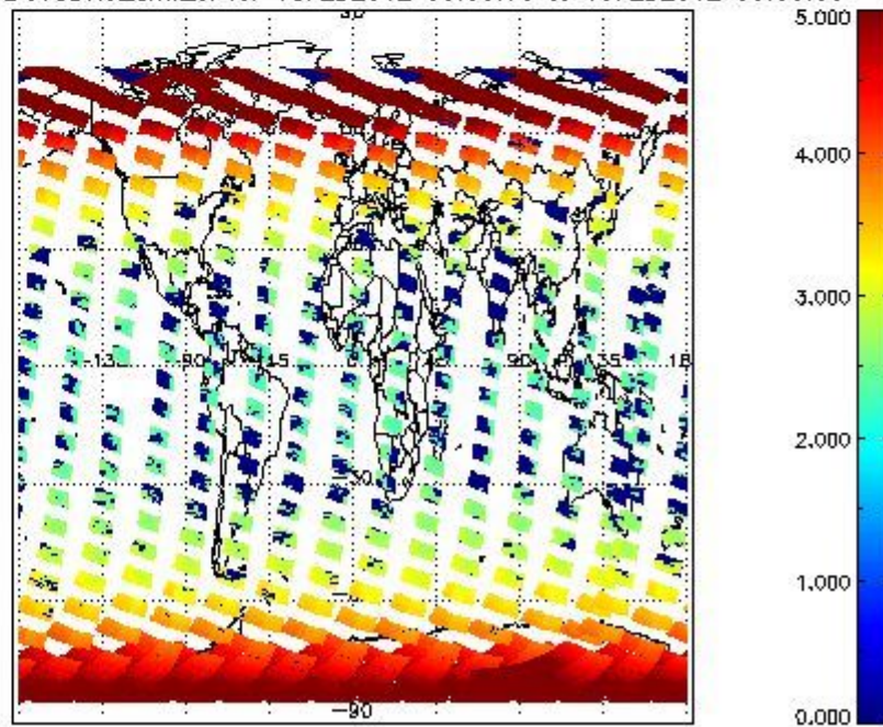
SCIOL2P_NADUV3BRO_amf_cl for 18FEB2012 00:00:00 to 19FEB2012 00:00:00
