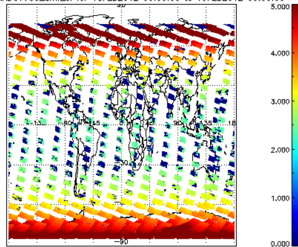
SCIOL2P_NADUV003_amf_cl for 18FEB2012 00:00:00 to 19FEB2012 00:00:00
