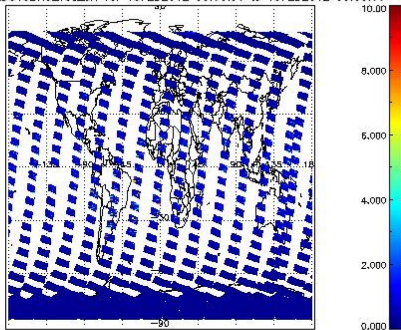
SCIOL2P_NADUV3BRO_vcd_err for 18FEB2012 00:00:00 to 19FEB2012 00:00:00
