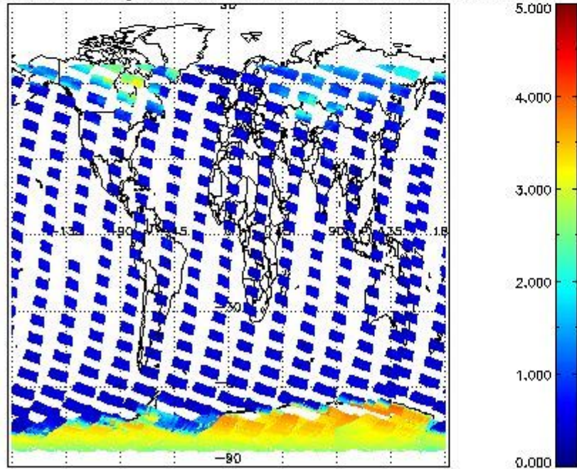
SCIOL2P_NADUV5SO2_amf_gr for 18FEB2012 00:00:00 to 19FEB2012 00:00:00
