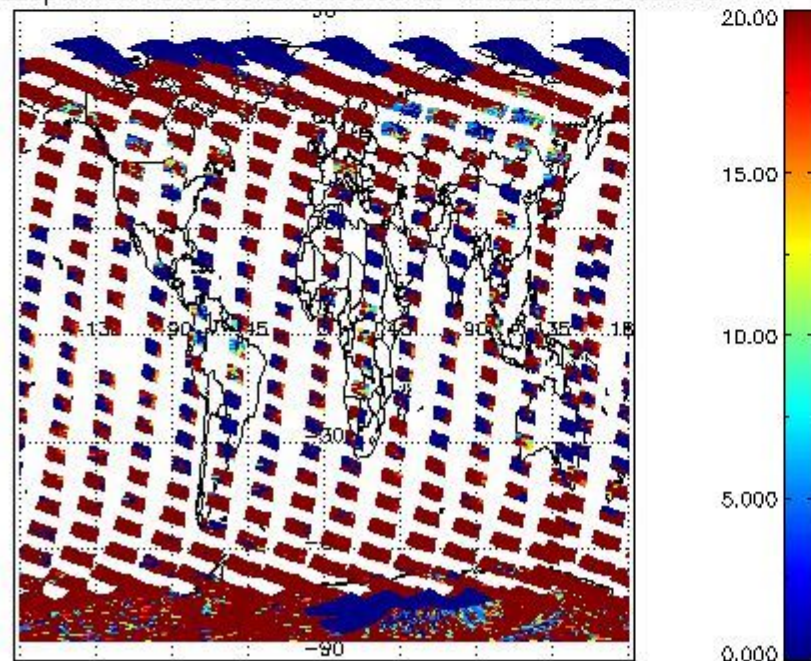
cL_opt_depth for 18FEB2012 00:00:00 to 19FEB2012 00:00:00
