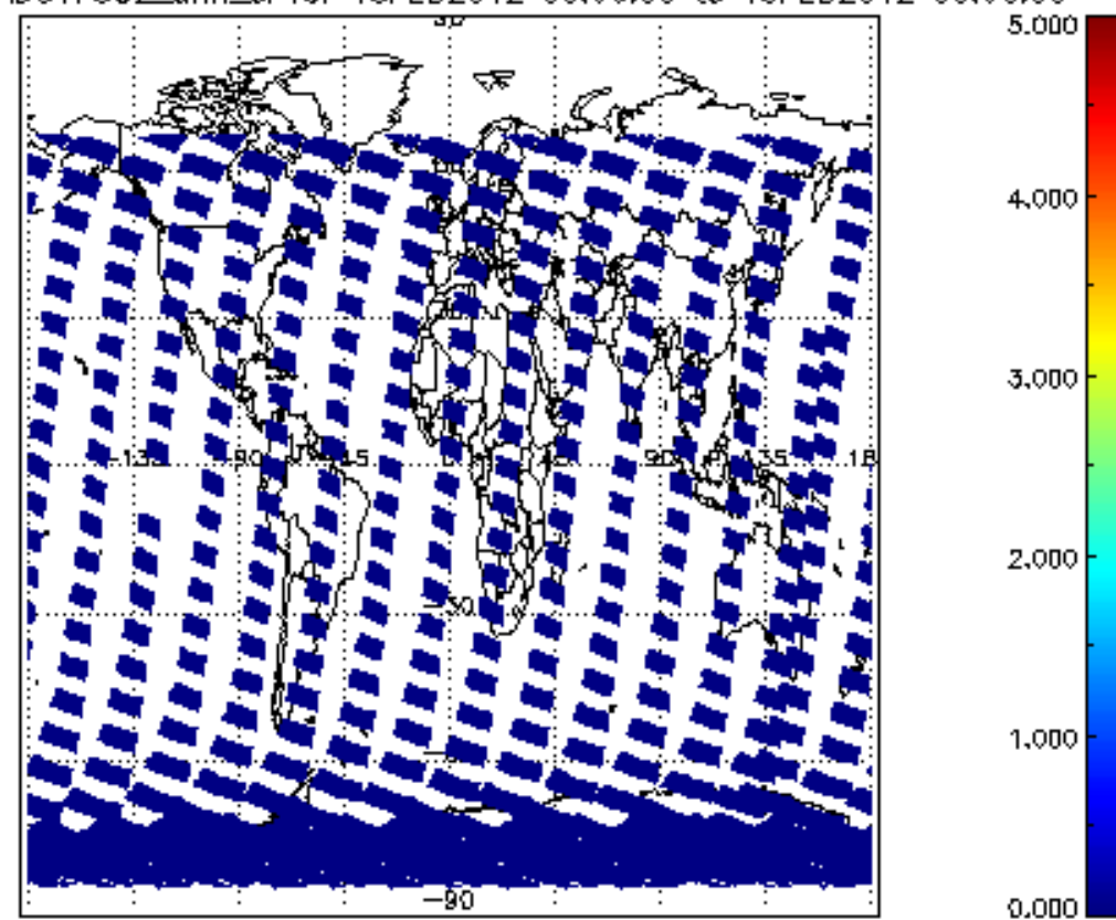
SCIOL2P_NADUV7S02_amf_cl for 18FEB2012 00:00:00 to 19FEB2012 00:00:00
