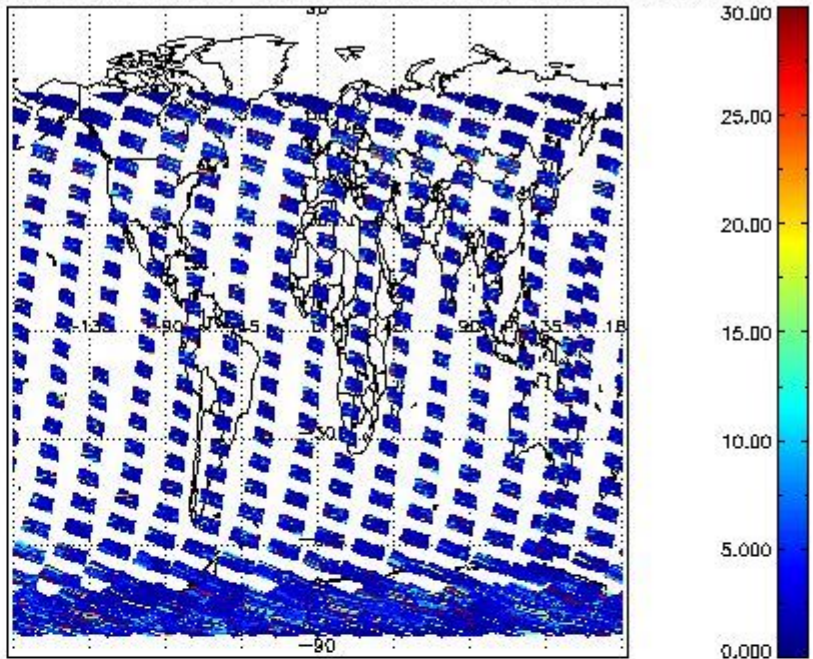
SCIOL2P_NADUV5SO2_vcd_err for 18FEB2012 00:00:00 to 19FEB2012 00:00:00
