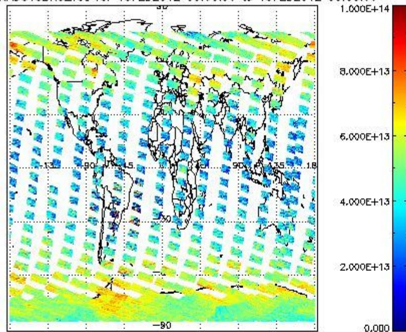
SCIOL2P_NADUV3BRO_vcd for 18FEB2012 00:00:00 to 19FEB2012 00:00:00
