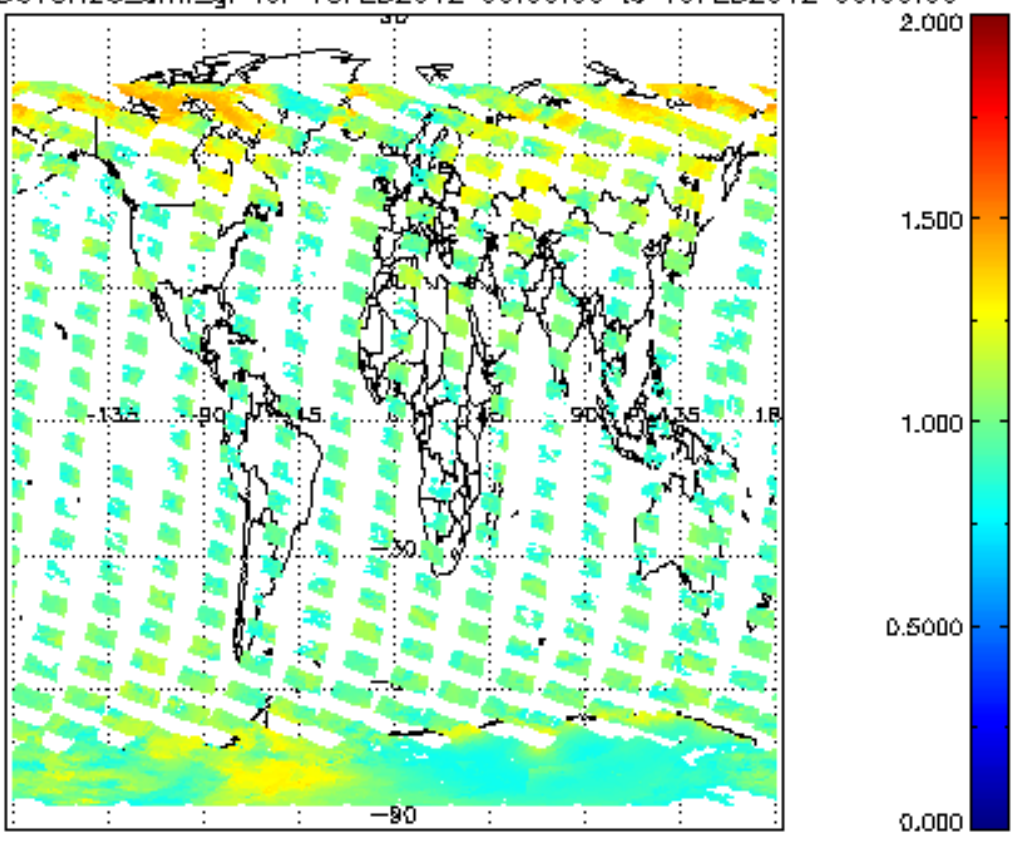
SCIOL2P_NADUV8H20_amf_gr for 18FEB2012 00:00:00 to 19FEB2012 00:00:00
