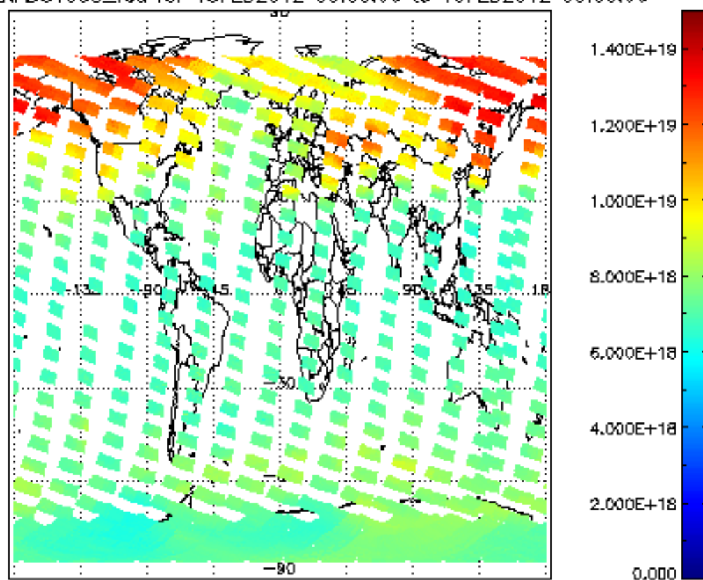
SCIOL2P_NADUV003_vcd for 18FEB2012 00:00:00 to 19FEB2012 00:00:00
