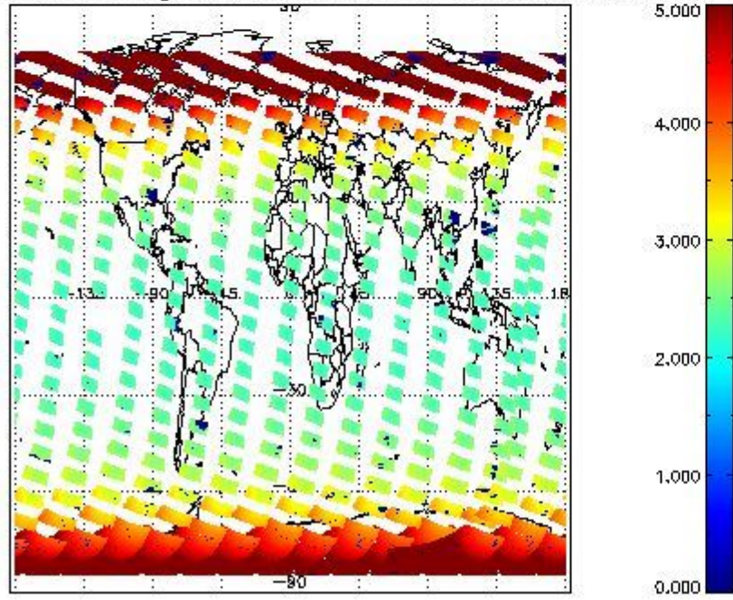
SCIOL2P_NADUV1N02_amf_gr for 18FEB2012 00:00:00 to 19FEB2012 00:00:00
