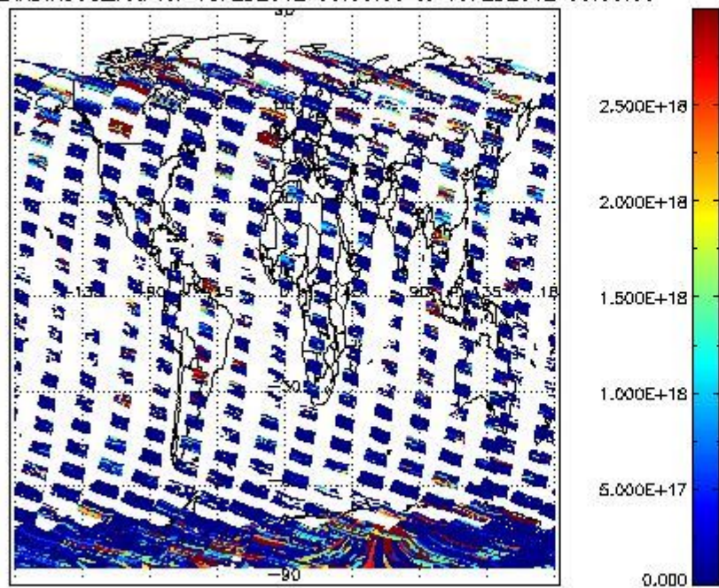
SCIDL2P_NADIR3CO_vcd for 18FEB2012 00:00:00 to 19FEB2012 00:00:00
