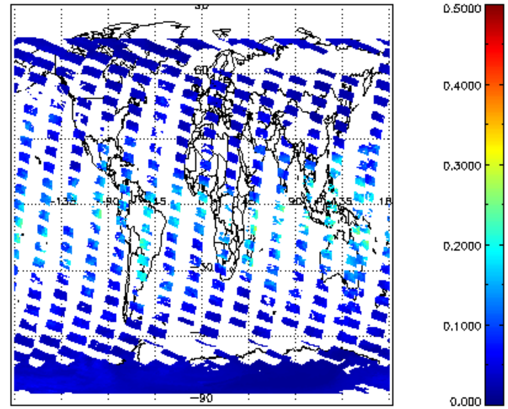
SCIOL2P_NADUV8H20_vcd_err for 18FEB2012 00:00:00 to 19FEB2012 00:00:00
