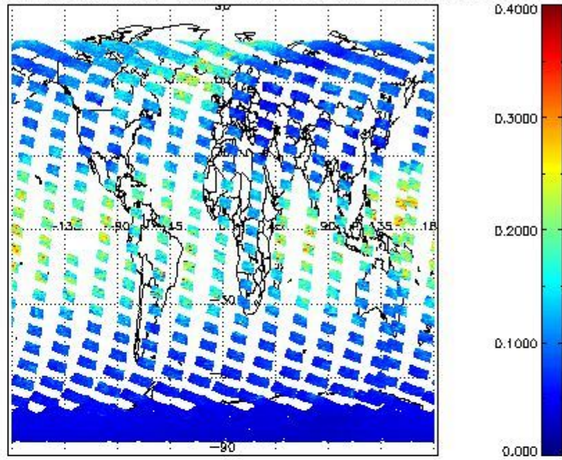
SCIOL2P_NADUV1N02_vcd_err for 18FEB2012 00:00:00 to 19FEB2012 00:00:00
