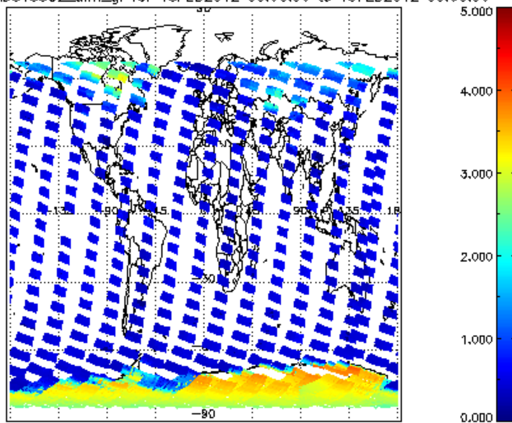
SCIOL2P_NADUV5S02_amf_gr for 18FEB2012 00:00:00 to 19FEB2012 00:00:00
