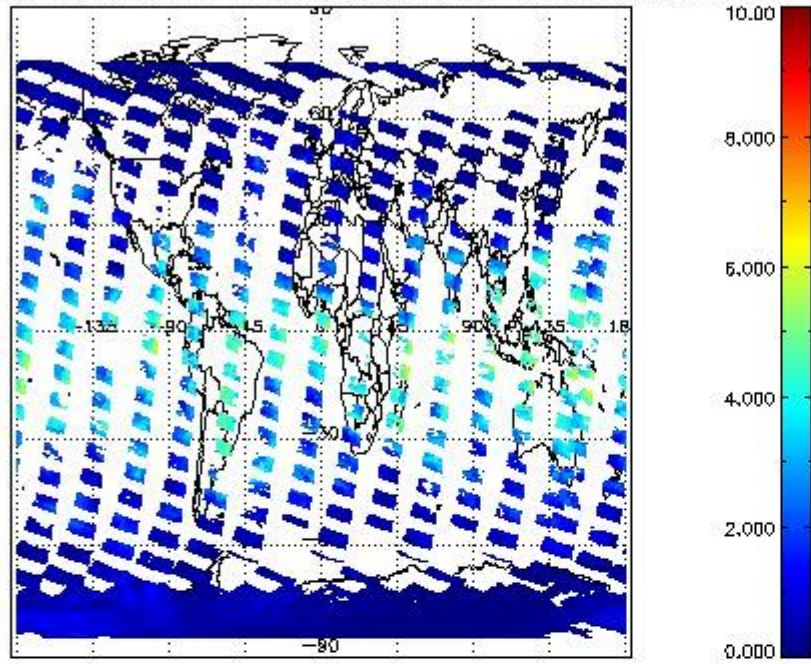
SCIOL2P_NADUV8H2O_vcd for 18FEB2012 00:00:00 to 19FEB2012 00:00:00
