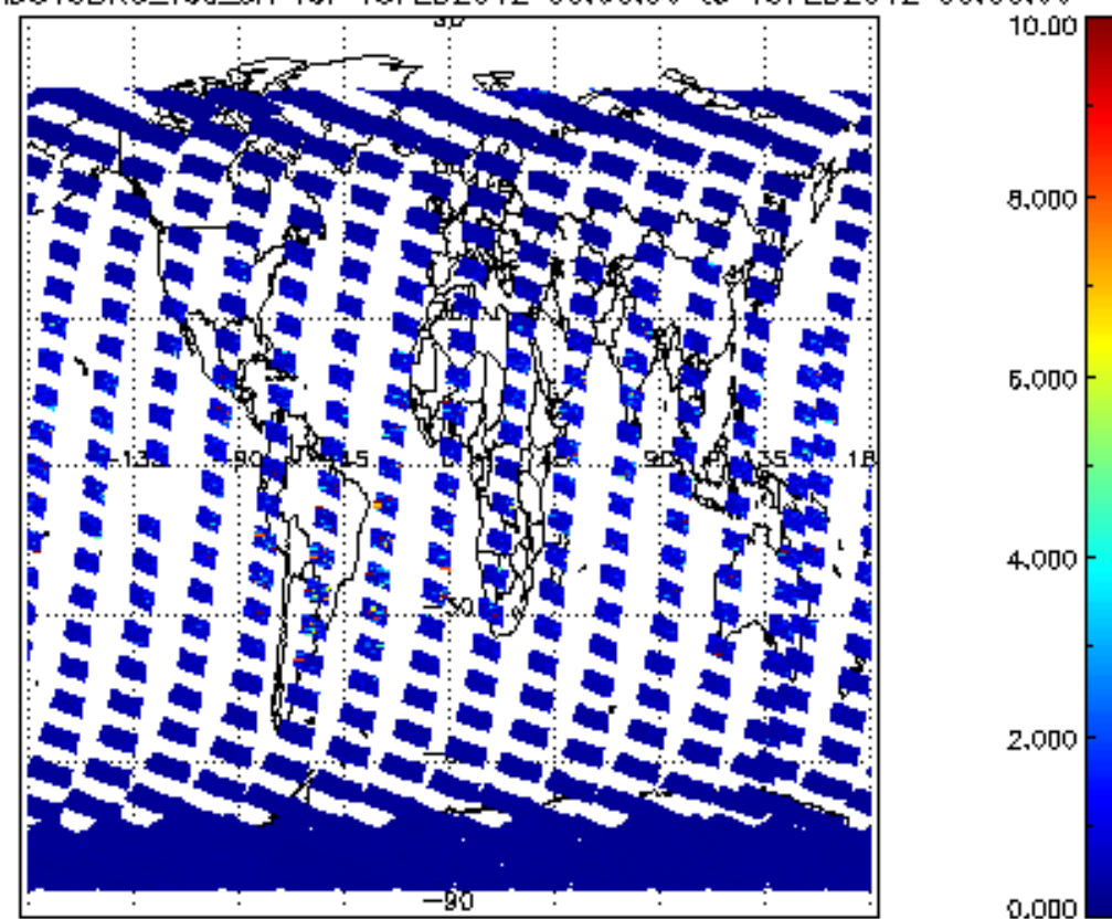
SCIOL2P_NADUV3BRO_vcd_err for 18FEB2012 00:00:00 to 19FEB2012 00:00:00
