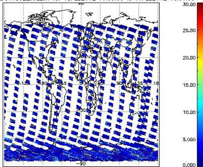
SCIOL2P_NADUV7S02_vcd_err for 18FEB2012 00:00:00 to 19FEB2012 00:00:00
