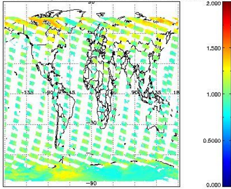
SCIOL2P_NADUV8H2O_amf_gr for 18FEB2012 00:00:00 to 19FEB2012 00:00:00
