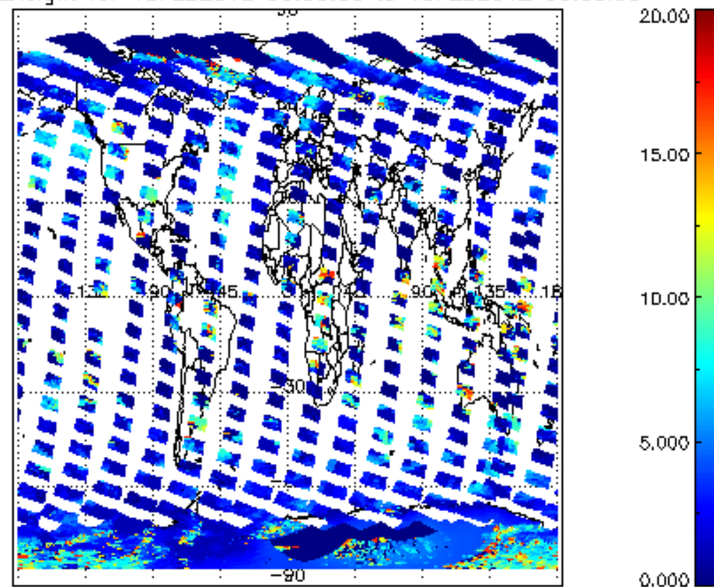
cl_top_height for 18FEB2012 00:00:00 to 19FEB2012 00:00:00
