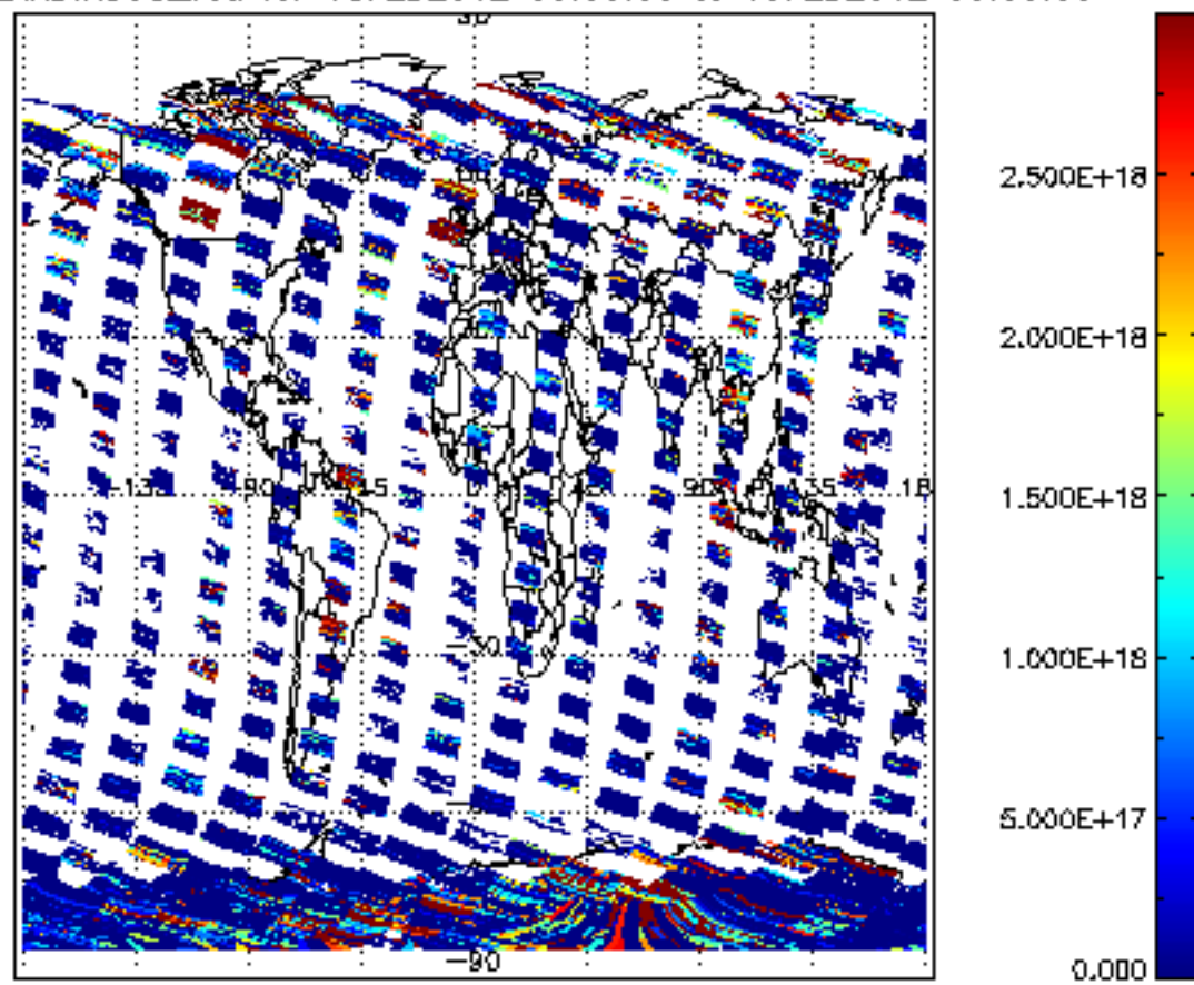
SCIOL2P_NADIR3CO_vcd for 18FEB2012 00:00:00 to 19FEB2012 00:00:00
