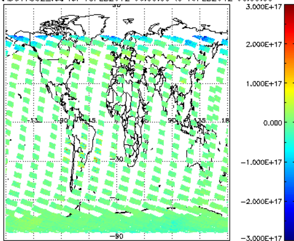
SCIOL2P_NADUV7S02_vcd for 18FEB2012 00:00:00 to 19FEB2012 00:00:00
