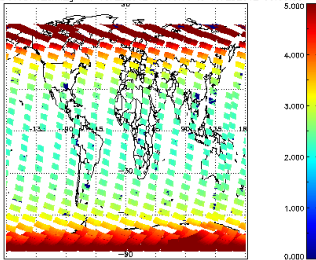
SCIOL2P_NADUV3BRO_amf_gr for 18FEB2012 00:00:00 to 19FEB2012 00:00:00
