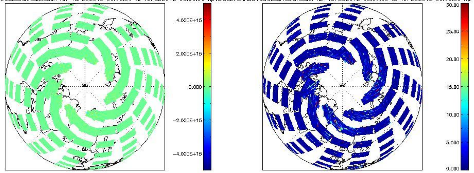
CIOL2P_NADUV60CLslant_col_den for 18FEB2012 00:00:00 to 19FEB2012 00:00:00 np; CIOL2P_NADUV60CLlarr_slant_col for 18FEB2012 00:00:00 to 19FEB2012 00:00:00 np
