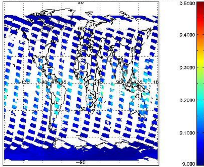
SCIOL2P_NADUV8H2O_vcd_err for 18FEB2012 00:00:00 to 19FEB2012 00:00:00
