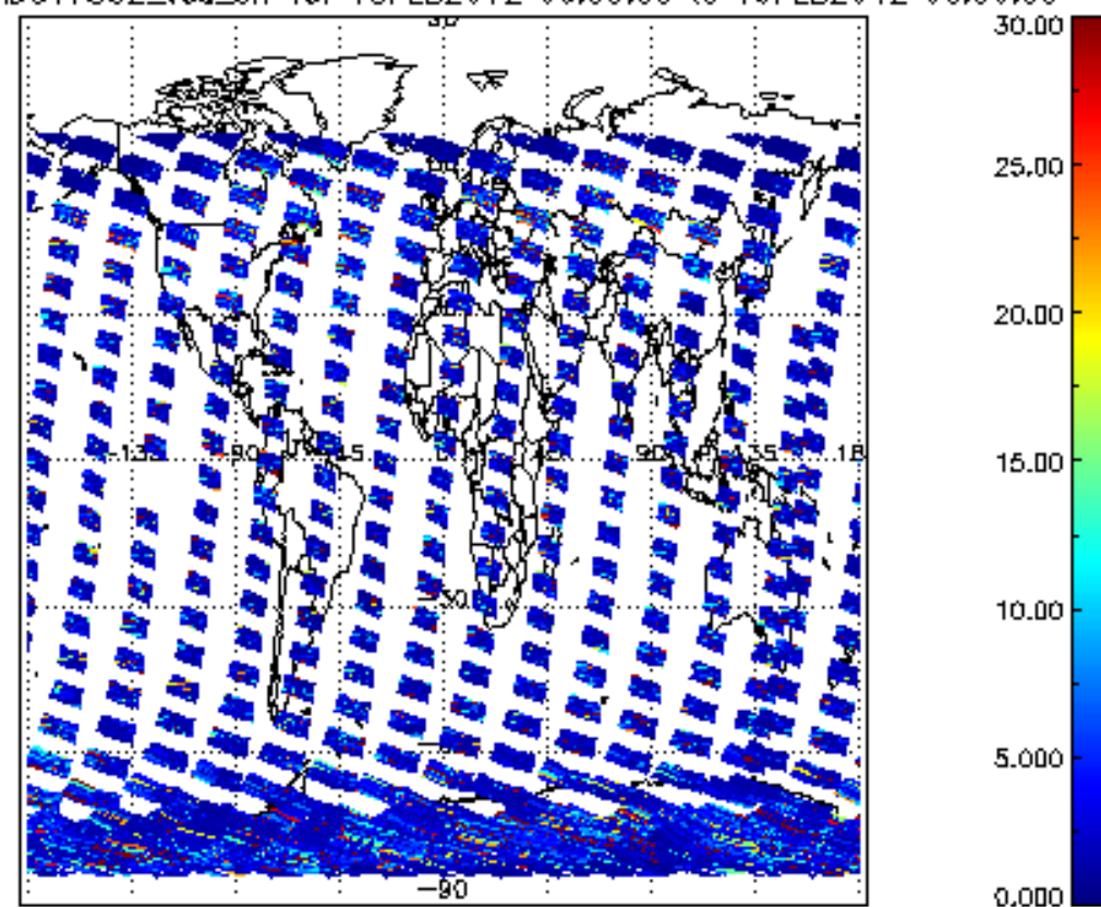
SCIOL2P_NADUV7S02_vcd_err for 18FEB2012 00:00:00 to 19FEB2012 00:00:00
