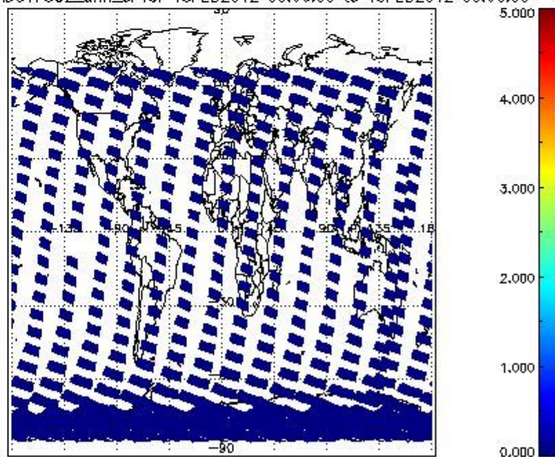
SCIOL2P_NADUV7S02_amf_cl for 18FEB2012 00:00:00 to 19FEB2012 00:00:00
