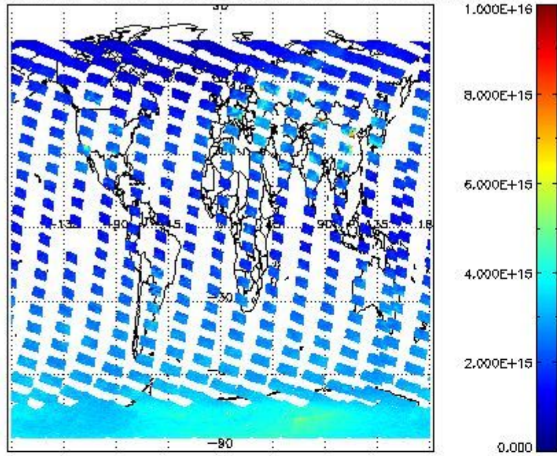
SCIOL2P_NADUV1N02_vcd for 18FEB2012 00:00:00 to 19FEB2012 00:00:00
