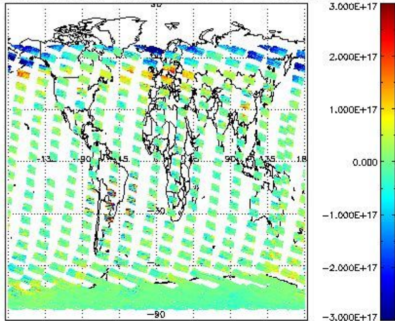
SCIOL2P_NADUV5SO2_vcd for 18FEB2012 00:00:00 to 19FEB2012 00:00:00
