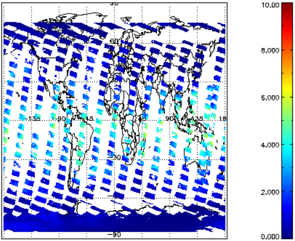
SCIOL2P_NADUV8H20_vcd for 18FEB2012 00:00:00 to 19FEB2012 00:00:00
