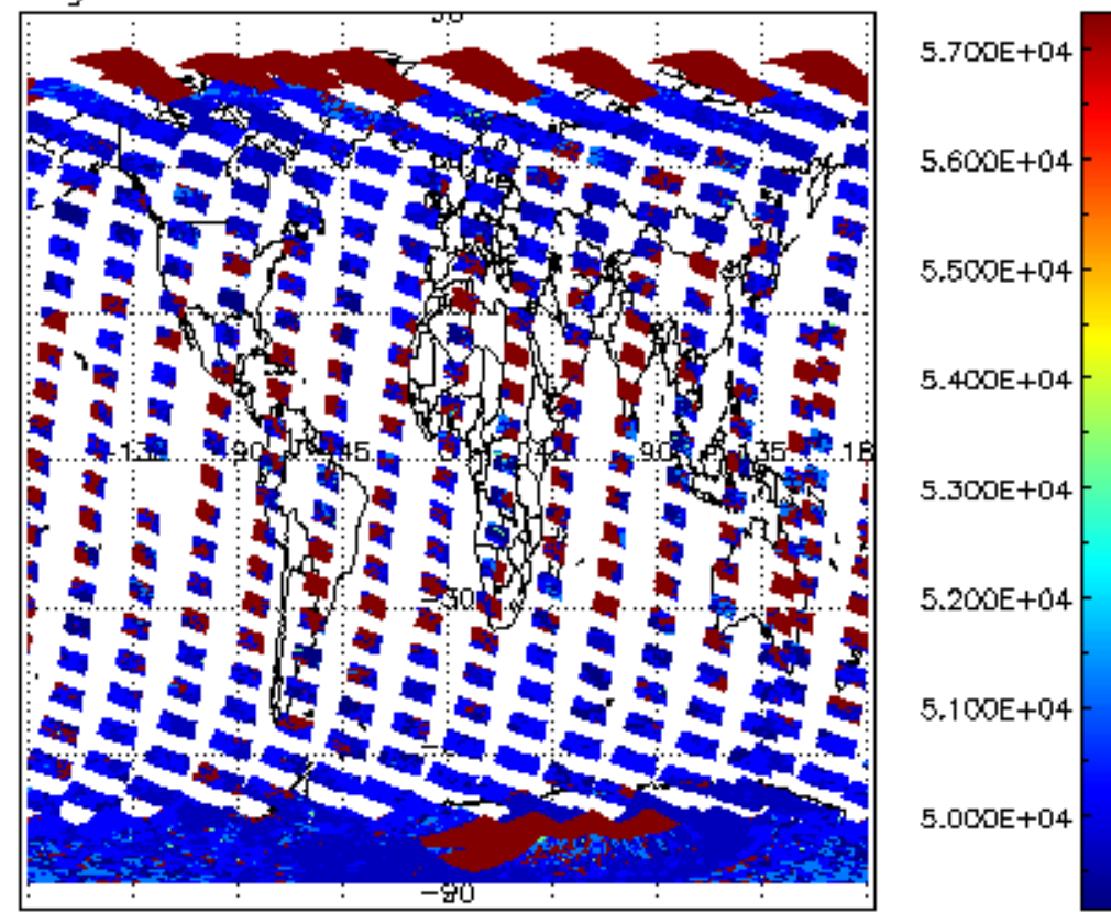
cloud_flags for 18FEB2012 00:00:00 to 19FEB2012 00:00:00
