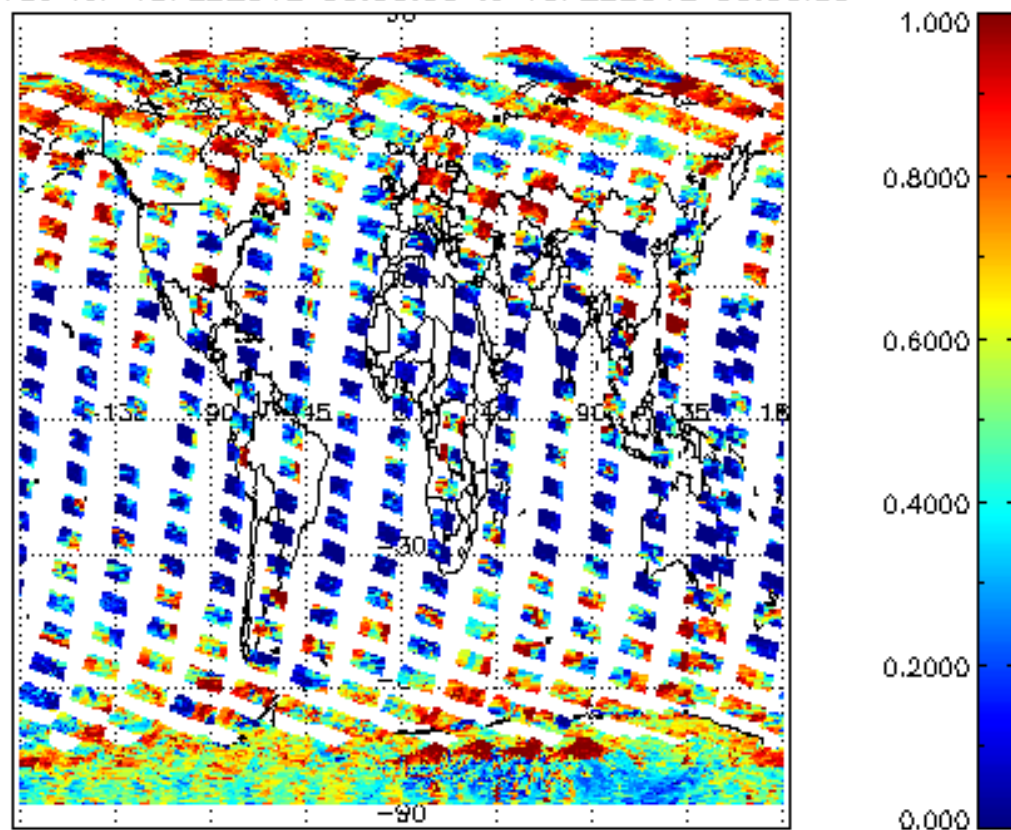
cl_frac for 18FEB2012 00:00:00 to 19FEB2012 00:00:00
