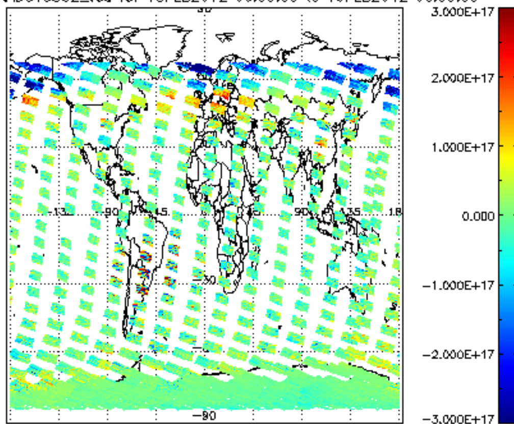
SCIOL2P_NADUV5S02_vcd for 18FEB2012 00:00:00 to 19FEB2012 00:00:00
