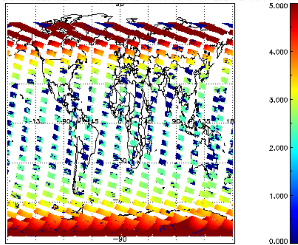
SCIOL2P_NADUV1N02_amf_cl for 18FEB2012 00:00:00 to 19FEB2012 00:00:00
