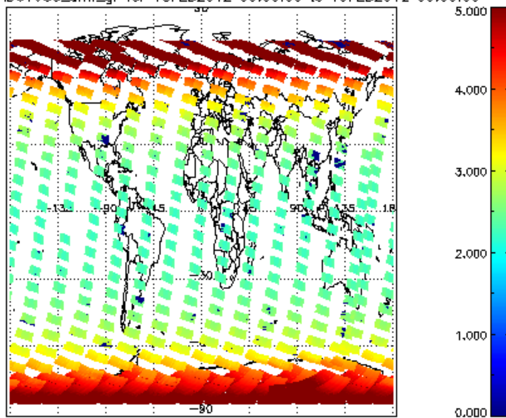
SCIOL2P_NADUV003_amf_gr for 18FEB2012 00:00:00 to 19FEB2012 00:00:00
