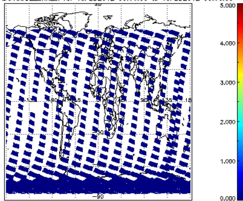
SCIOL2P_NADUV5S02_amf_cl for 18FEB2012 00:00:00 to 19FEB2012 00:00:00
