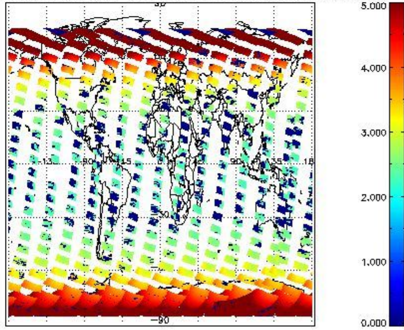
SCIOL2P_NADUV1N02_amf_cl for 18FEB2012 00:00:00 to 19FEB2012 00:00:00
