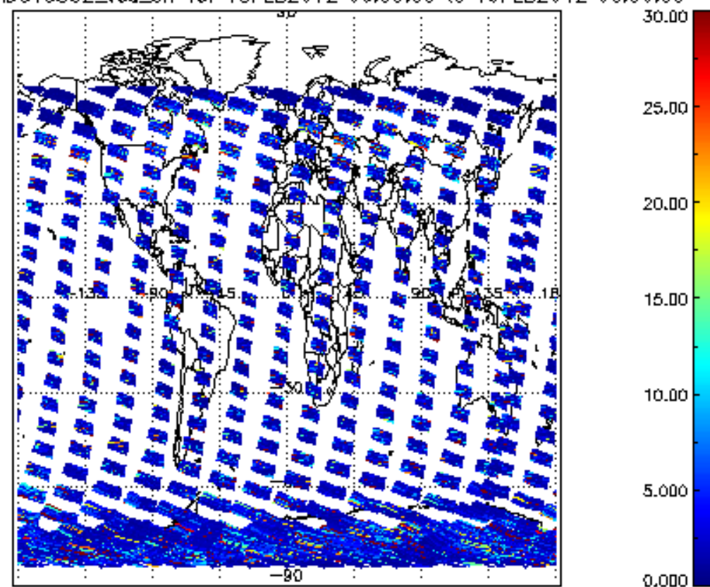
SCIOL2P_NADUV5S02_vcd_err for 18FEB2012 00:00:00 to 19FEB2012 00:00:00
